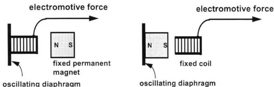
Fig. 5.54 Two designs for a microphone
