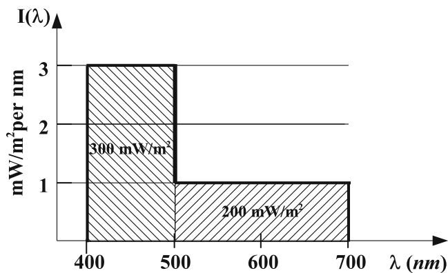
Fig. 13.8 Spectral intensity
