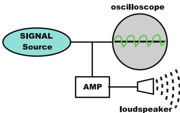
Fig. 3.7 Studying a sound wave
