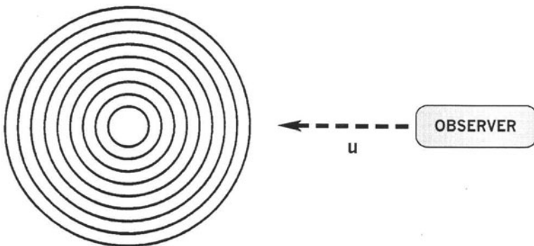
Fig. 8.44 A moving observer in the presence of a stationary source of sound waves
