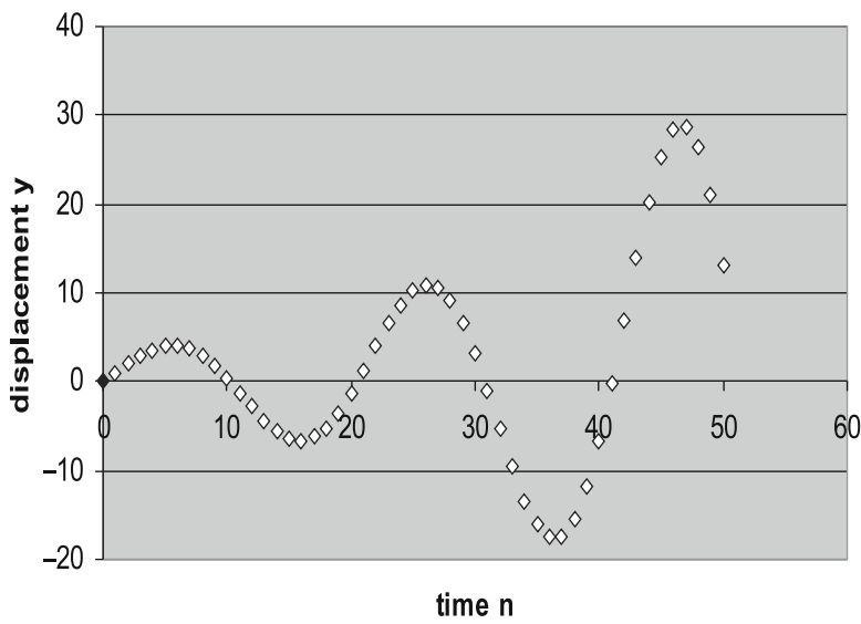
Fig. F.1 Resulting plot of the displacement: a crude numerical integration
