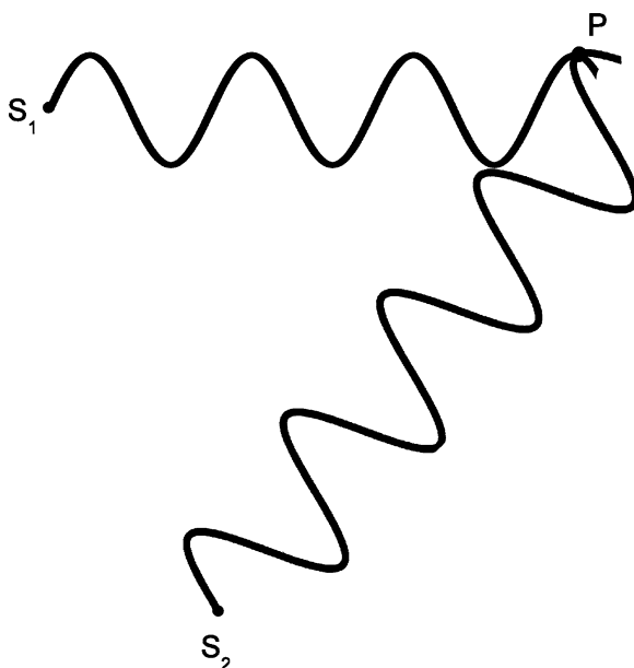
Fig. 7.5 Point where waves arrive in phase
