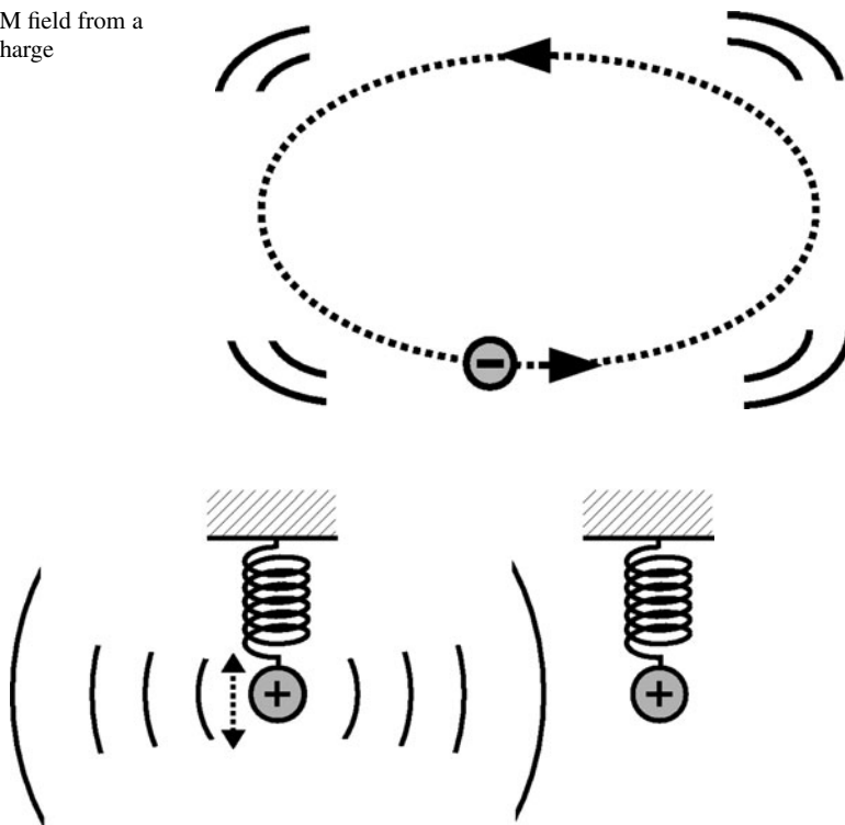
Fig. 5.78 Resonance between two charged SHOs
