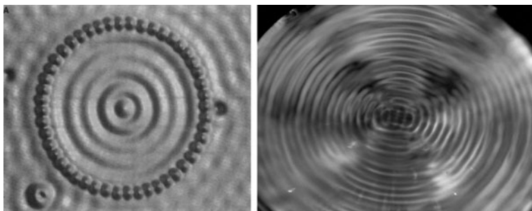
Fig. 6.11 The “Iron Corral”: 48 iron atoms on a copper surface, with a standing wave of probability density; Standing surface wave in a mug of water (sources: Corral: From M. F. Crommie, et al, Science 262 , 218 (1993); Reprinted with permission from AAAS; photo of water surface by Konstantinos Metallinos)
