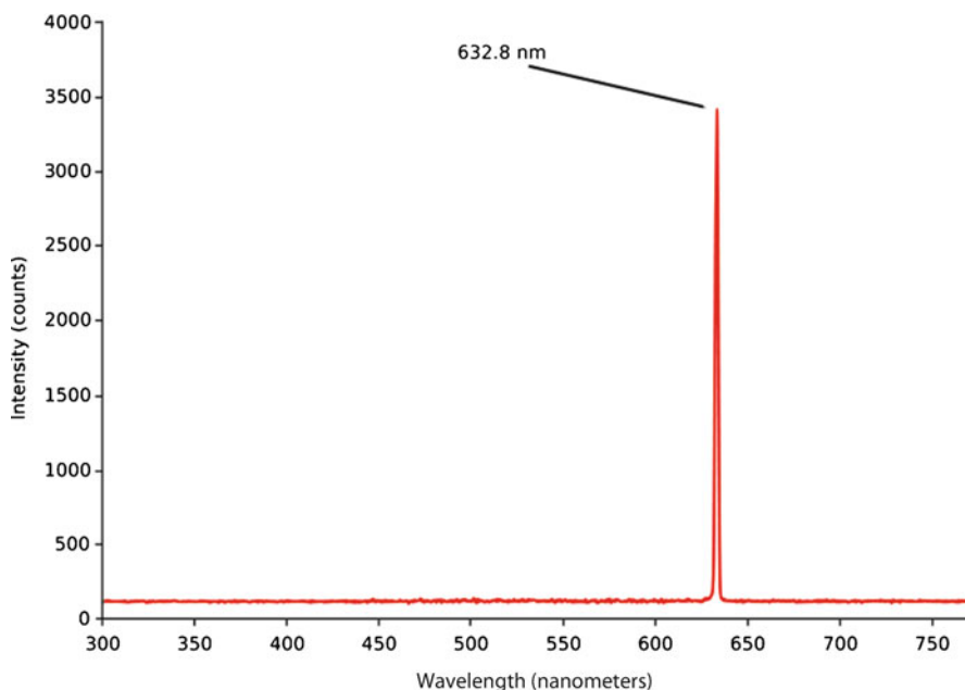
Fig. 6.20 Spectrum of a Helium-Neon laser (source: http://wapedia.mobi/en/Laser )
