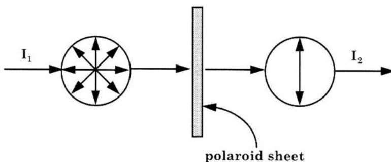
Fig. 8.52 Polaroid-based polarizer
