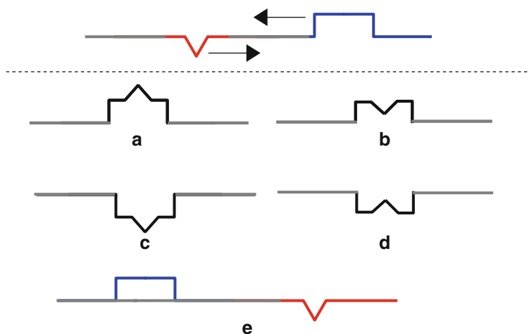
Fig. 7.18 “Colliding” waves
