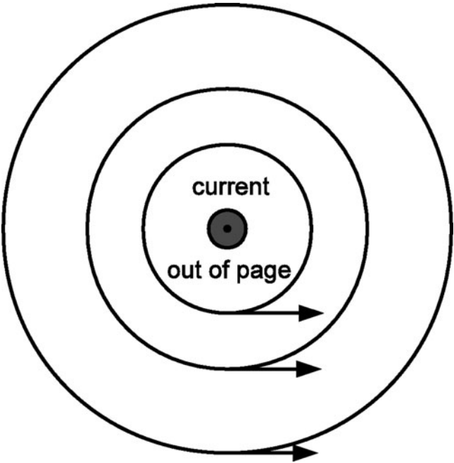
Fig. 5.47 Magnetic field of a straight wire
