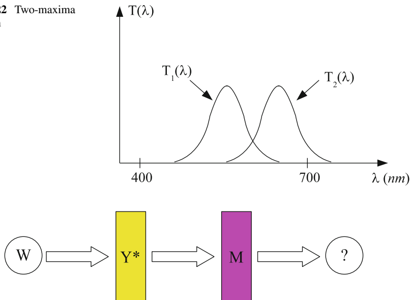
Fig. 13.23 White light enters a yellow and magenta filter
