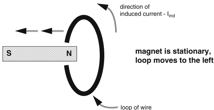
Fig. 5.34 A moving loop with a stationary magnet
