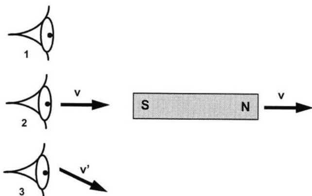
Fig. 5.56 Three observers of a magnet
