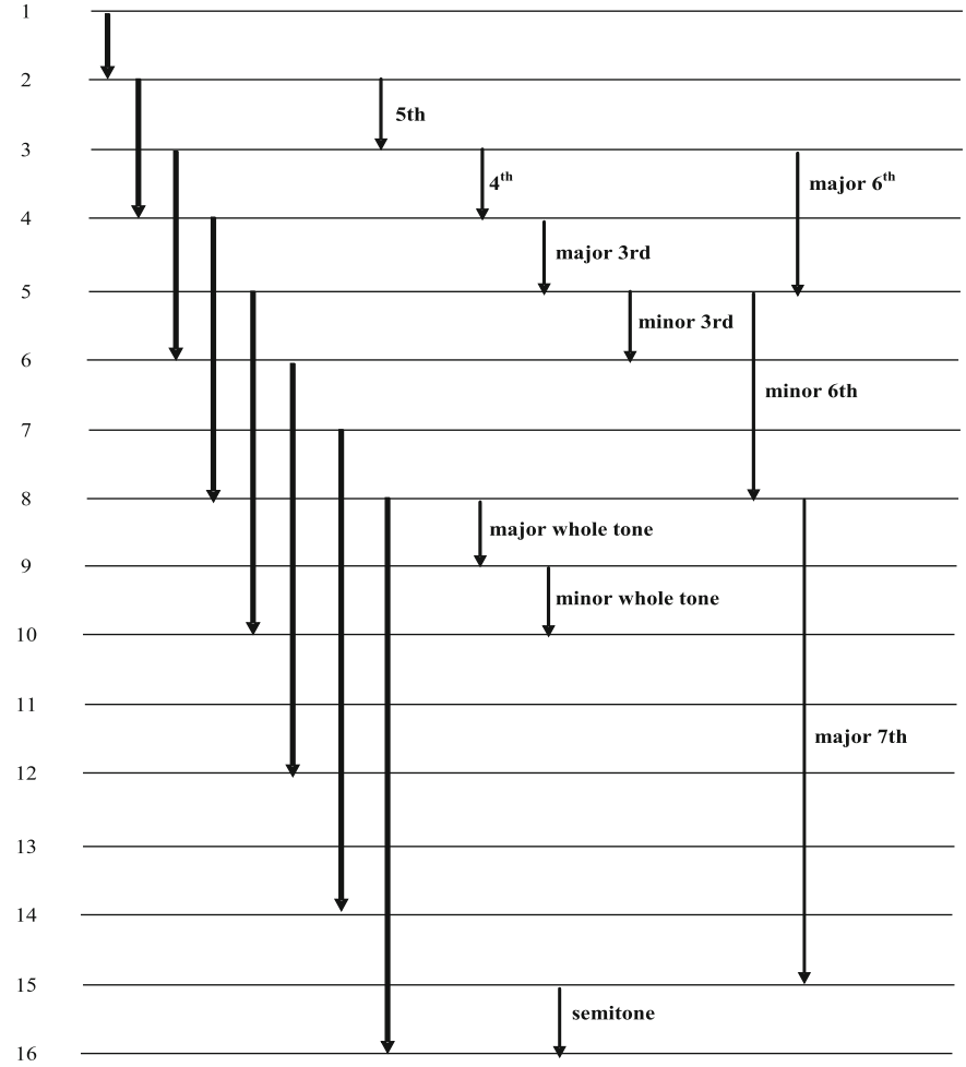
Fig. 11.12 Chart of important Just intervals
