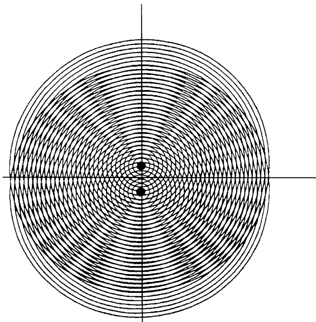
Fig. 7.23 Two spherical sources
