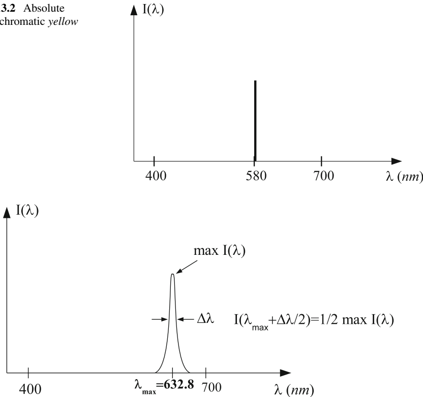
Fig. 13.3 Quasi-monochromatic red
