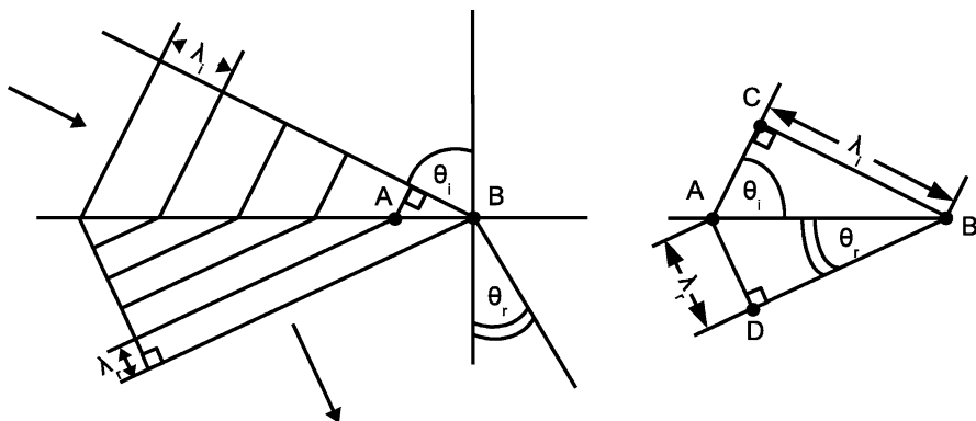
Fig. 8.24 Detailed schematic of the Huyghen's wave theory of refraction
