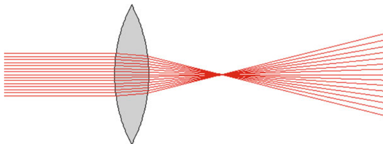
Fig. 8.32 Spherical aberration – weak for rays near the axis
