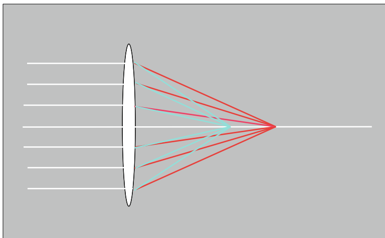
Fig. 8.33 Chromatic aberration
