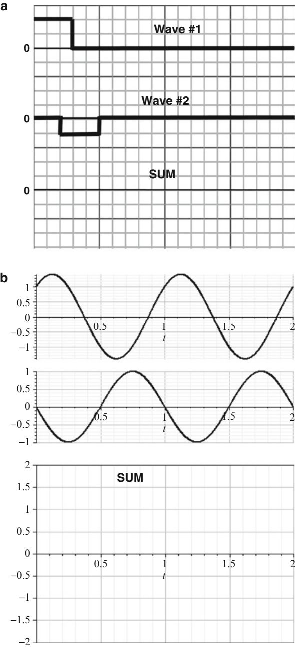
Fig. 7.22 Addition of waves
