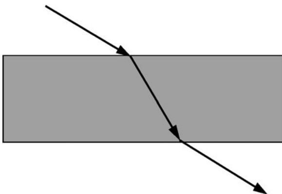
Fig. 8.69 Refraction through a slab of glass
