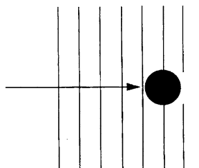
Fig. 8.10 Shadow created by a spherical object – wavelength comparable to the diameter of the object
