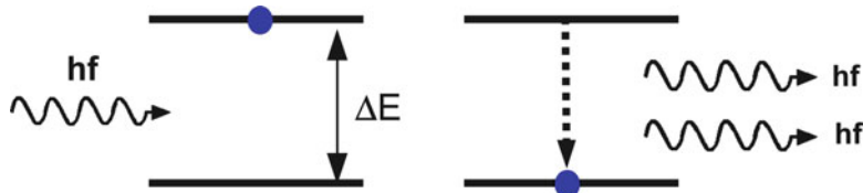
Fig. 6.19 Stimulated emission
