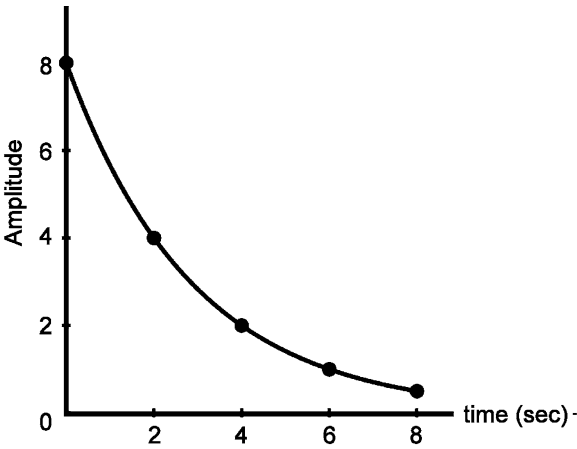
Fig. 4.6 Amplitude vs. time due to attenuation
