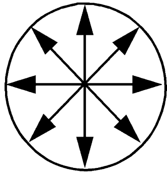
Fig. 8.49 Light as an electromagnetic wave (source: http://en.wikipedia.org/wiki/Wave#Electromagnetic_waves )
