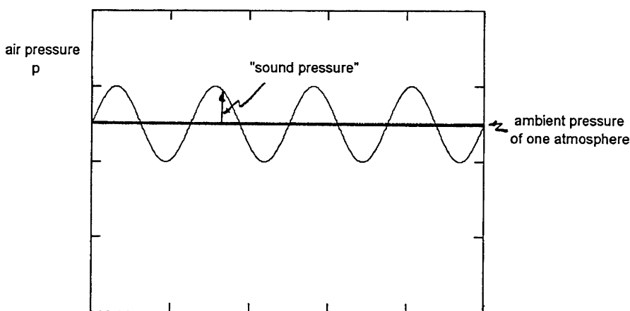
Fig. 3.6 Sound pressure
