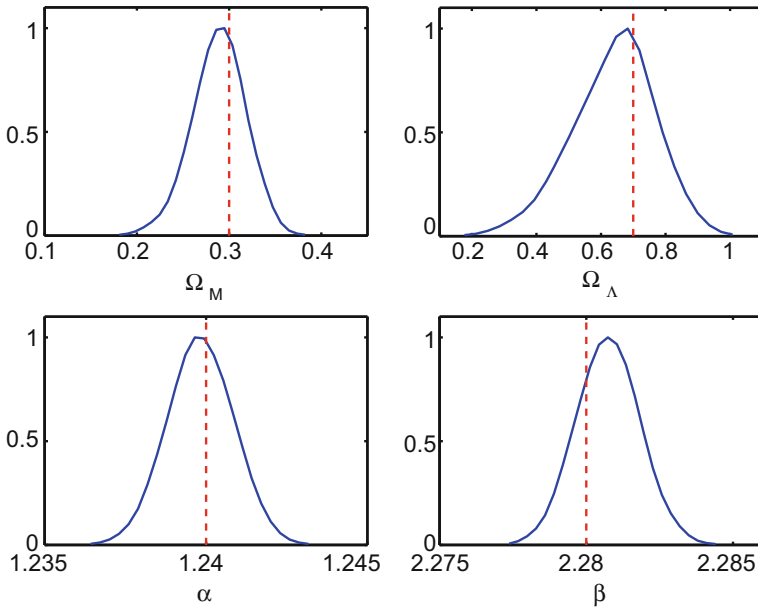
Fig. 7.5 Multinest recovered parameters for data set with \Sigma_x = 10.0 and \Sigma_c = 10.0 , all other parameters are as in Table 7.3. Here there is no bias on \alpha and \beta because the ranges of s and c are much larger than their associated observational noise. There is a small discrepancy between the true and recovered values of \alpha and \beta , but this is due to realization noise rather than a systematic offset
