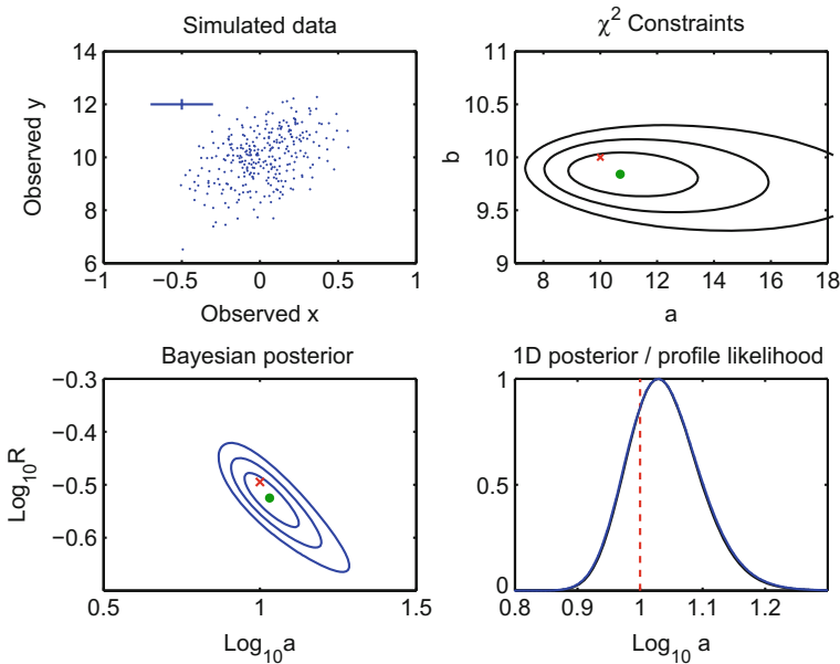
Fig. 7.6 Numerical comparison between the \chi^2 approach and the Bayesian method for linear fitting. Upper left panel: data set of N = 300 observations with errors both in the x and y directions, given by the error bar. Upper right panel: reconstruction of the slope a and intercept b using a \chi^2 likelihood (red cross is the true value, green circle the maximum likelihood value). Lower left panel: Gull's Bayesian posterior Eq. (7.60) in the \log a , \log R plane, with green circle showing posterior mean. In both panels, contours enclose 1\sigma , 2\sigma and 3\sigma regions. Lower right panel: marginalized Bayesian posterior (blue) and profiled \chi^2 likelihood (black, lying exactly on top of the blue curve), with the dashed line showing the true value. The two methods give essentially identical results in this case
