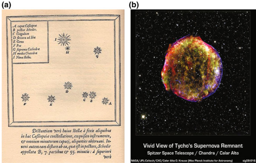
Fig. 4.1 SN 1572: Tycho's SNe. The left hand panel shows Tycho Brahe's sketch included in De nova stella of the 'new star' he observed in Cassiopeia on 11 November 1572. The right hand panel shows a modern composite image of Tycho's supernovae remnant using optical and X-ray data [Image: NASA/JPL-Caltech/CXC/Calar Alto O. Krause (Max Planck Institute for Astronomy)]. Tycho's SN 1572 has been spectroscopically confirmed as a type Ia supernova
