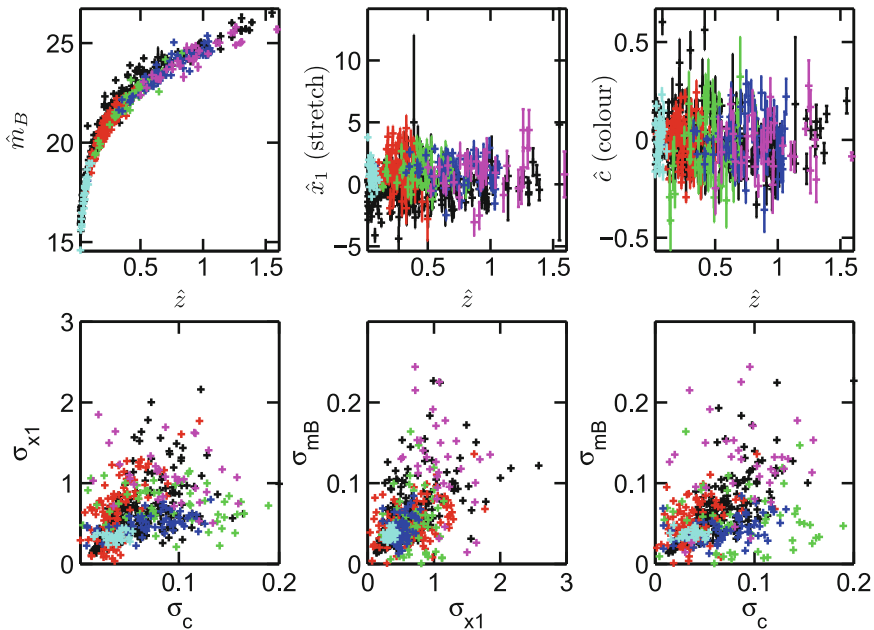
Fig. 7.10 An example realization of our simulated data sets (coloured according to survey), superimposed on real data (black). Colour code for simulated data survey: nearby sample (cyan), ESSENCE (green), SDSS (red), SNLS (blue) and HST (magenta). Fig. from [7]
