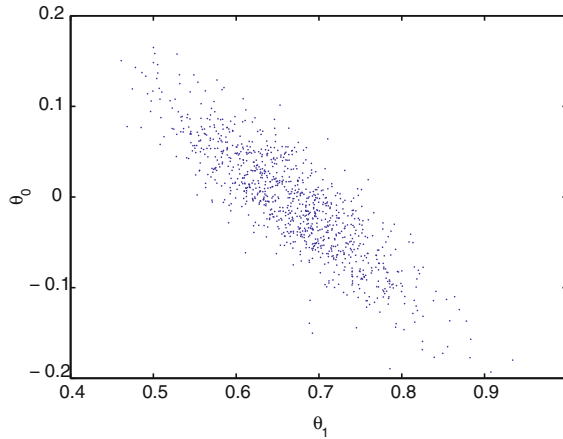
Fig. 5.2 The application of MCMC methodology to the Gaussian linear model described by Eq. (5.13) and Eq. (5.14). The density of the points in parameter space corresponds to the posterior distribution (Here the points are uniformly weighted). The first few points in the chain have been discarded as ‘burn in’ points and the chain has been ‘thinned’ by retaining only every 100th point
