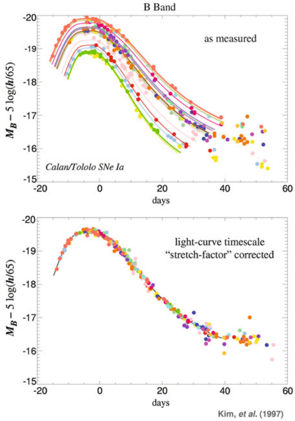
Fig. 4.4 The upper panel shows the light curves from nearby supernovae, for which it can be seen there is considerable scatter \sim \pm 0.8 mag in the maximum magnitude. The lower panel shows the same light curves after the application of the stretch correction, here the scatter in maximum magnitude is greatly reduced but not eliminated. Understanding this residual scatter will be one of the main motivations for my work presented in Chap. 7. Figure from [19]
