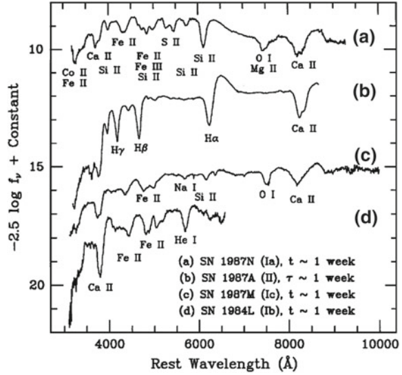
Fig. 4.2 Figure taken from Filippenko [6] showing differentiation of supernovae by their spectra. The supernovae type Ia spectrum is labelled (a), it is distinguished by an absence of hydrogen H_\alpha features and the presence of a strong silicon Si II absorption line
