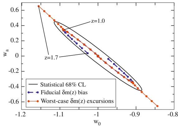
Fig. 8.3 Systematic bias in the w_0 - w_a plane for future SNIa data. The square denotes our fiducial value and the ellipse gives the 68 % CL statistical contour from future SNIa data. The blue curve shows the systematic bias given by Eq. (8.56), with points showing cumulative contributions from each of the 16 redshift bins — that is, cumulative value of the sum in Eq. (8.55). For clarity, we explicitly label bias contributions accumulated by redshifts z = 1 and z = 1.7 . The red segments denote the worst-case bias, where the sign of \delta m(z) at each redshift bin conspires to shift the (w_0, w_a) value away from the true value (“Maximum excursion bias”); see Eq. (8.57). For clarity, we have also plotted the biases with the opposite sign relative to the fiducial model parameter values. This figure is the work of Dragan Huterer, from [9]
