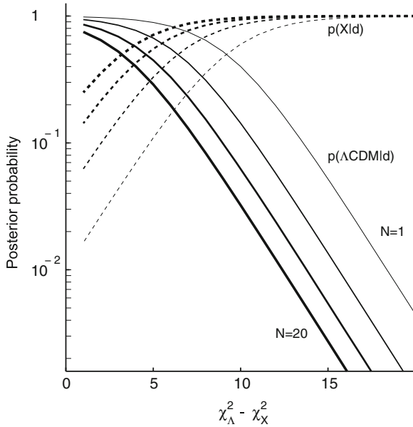
Fig. 6.2 Posterior for doubt ( dashed lines ) and for \Lambda CDM ( solid lines ) as a function of -\Delta\chi^2 = \chi_\Lambda^2 - \chi_X^2 assuming a fixed prior doubt p(X) = 10^{-2} . Different curves are for different numbers of known models, N = 1, 4, 10, 20 (from thin to thick), assuming that \langle B_{i\Lambda} \rangle \approx 1/N . Figure from [2]
