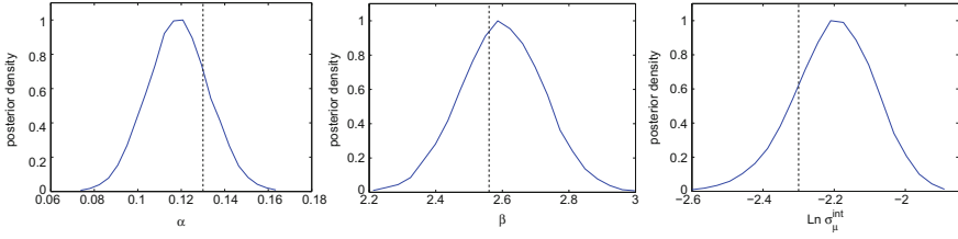
Fig. 7.12 Marginalised posterior for the stretch correction \alpha , colour correction \beta parameter and logarithm of the intrinsic dispersion of SNe, \log \sigma_{\mu}^{\text{int}} , from a simulated data set from our Bayesian method. The vertical, dashed line gives the true value for each quantity. Fig. from [7]
