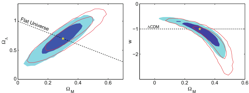
Fig. 7.11 Reconstruction of cosmological parameters from a simulated data set encompassing 288 SNIa, with characteristics matching presently available surveys (including realization noise). Blue regions contain 95.4% and 68.3% of the posterior probability (other parameters marginalized over) from our BHM method, the red contours delimit 95.4% and 68.3% confidence intervals from the standard \chi^2 method (other parameters maximised). The yellow star indicates the true value of the parameters. The left panel assumes w = -1 while the right panel assumes \Omega_\kappa = 0 . Notice how our method produced considerably less biased constraints on the parameters. Fig. from [7]
