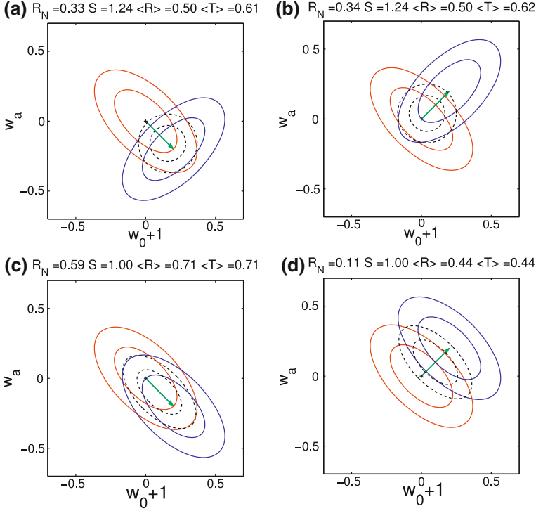
Fig. 8.1 Illustration of statistical and robustness FoM for a future probe ( blue ellipses , 68 % and 95 % C.L.) which is systematically biased w.r.t. the present-day constraints ( red ellipses ) in the direction given by the green bias vector . The black dotted ellipses represent the combined constraints. Notice that the statistical FoM ( S ) does not change in the presence of a systematic bias. Figure from [9]
