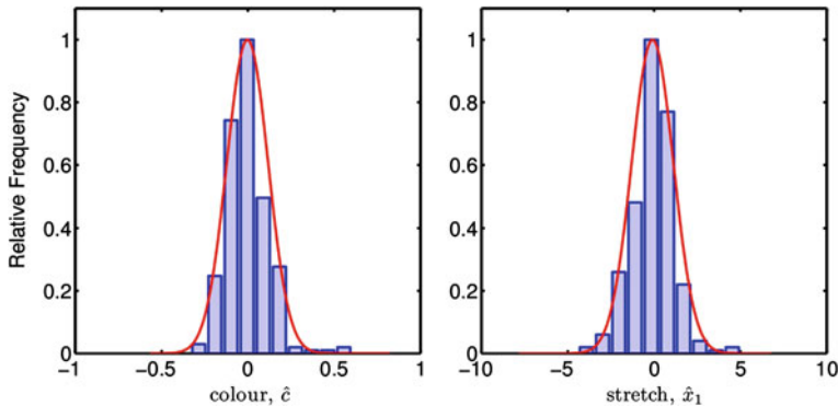
Fig. 7.9 Histogram of observed stretch parameters \hat{x}_{1i} and observed colour parameters \hat{c}_i from the 288 SNIa from Kessler et al. (2009a), compared with a Gaussian fit (red curve). Fig. from [7]
