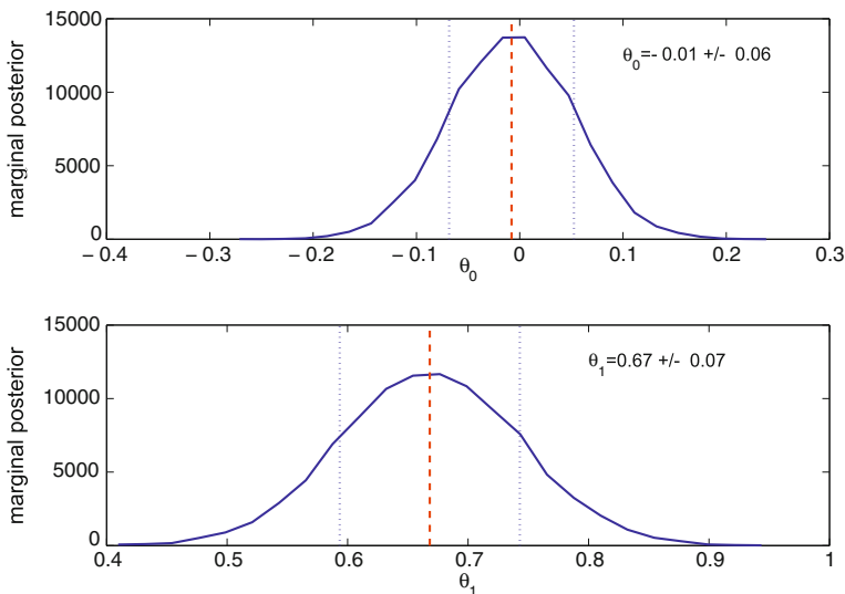
Fig. 5.3 From the simple Gaussian linear model: the marginal posteriors for the two parameters are obtained by integrating out the unwanted parameter, which in practice means binning the points from the chain shown in Fig. 5.2. The dashed line indicates the mean of the distribution, the dotted lines indicate \pm\sigma
