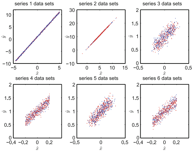
Fig. 7.3 Examples of the simulated linear model data sets from series 1-6. For each series, 100 data sets were simulated. For the characteristics of each data set, see table 7.2. Two example data sets are shown for each series, one in red and one in blue. Each data set has 300 points
