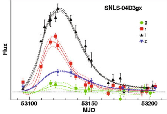
Fig. 4.5 Example light curve from Guy et al. [15]. Solid points are the observed data and their error bars, solid lines are the best fit light curve model and the dashed lines are the 1\sigma uncertainties on that model
