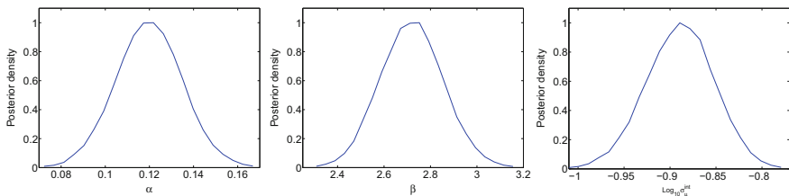
Fig. 7.18 Marginalised posterior for the stretch correction \alpha , colour correction \beta parameter and logarithm of the intrinsic dispersion of SNe, \log \sigma_{\mu}^{\text{int}} from current SNIa data. Fig. from [7]
