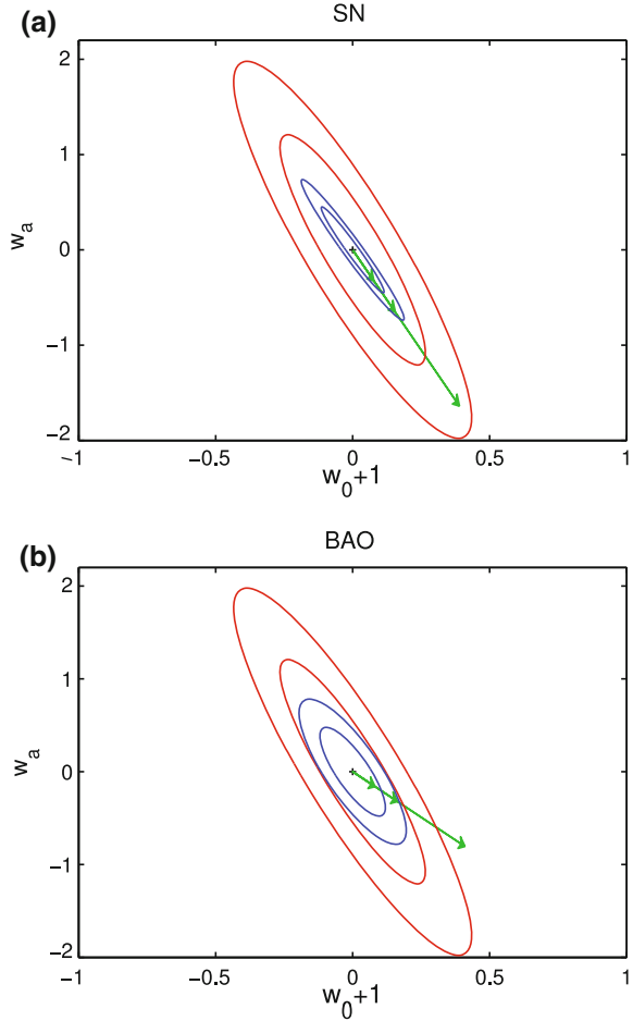
Fig. 8.4 Construction of the robustness FoM for a future SNIa survey ( top panel ) and a future BAO Euclid-like survey ( bottom panel ). Red ellipses show current 68 %, 95 % constraints (in a Gaussian approximation) from a combination of all available probes, blue ellipses show projected constraints from the future probe at the fiducial point (assumed to be \Lambda CDM). The green vectors show the systematic maximum excursion bias (MEB) for systematic errors of 1 %, 2 % and 5 % for SNIa and 0.1 %, 0.2 % and 0.5 % for BAO. Figure from [9]
