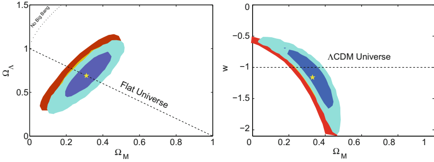
Fig. 7.16 Constraints on the cosmological parameters \Omega_m , \Omega_\Lambda (left panel, assuming w = -1 ) and w , \Omega_m (right panel, assuming \Omega_\kappa = 0 ) from our Bayesian method (light/dark blue regions, 68.3% and 95.4% marginalized posterior), compared with the statistical errors from the usual \chi^2 approach (yellow/red regions, same significance level; from Kessler et al. (2009a)). The yellow star gives the posterior mean from our analysis. Fig. from [7]
