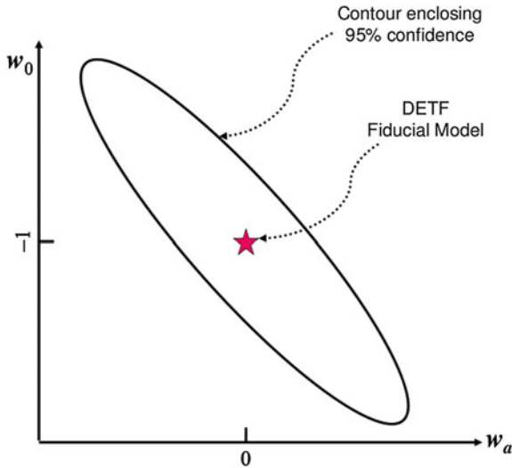
Fig. 5.6 Example 95 % error ellipse derived from the Fisher matrix for the dark energy parameters of interest, w_0 , w_a taken from [28]. The figure of merit is the inverse area of the 95 % confidence level or error ellipse
