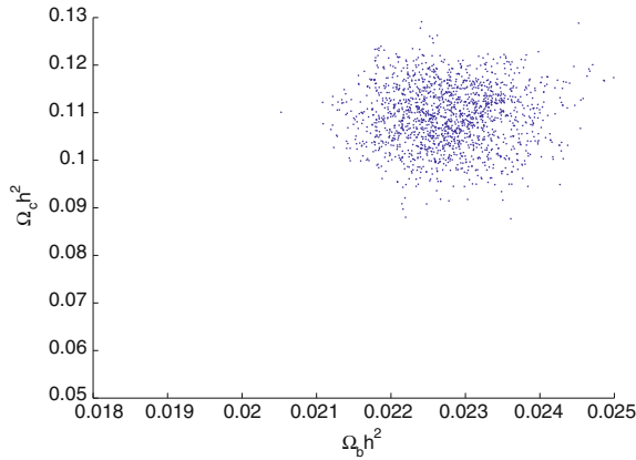
Fig. 5.4 The application of MCMC methodology to WMAP data [18] using CosmoMC. As for Fig. 5.2, but here the samples are weighted. The weighted density of points in parameter space corresponds to the posterior distribution
