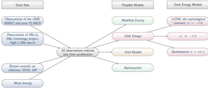
Fig. 1.1 Schematic showing that various observations point towards the apparent late time acceleration of the Universe, and some of the possible different types of models which could explain this. The goal is to be able to use astrophysical observations to discriminate between the different cosmological models and infer the values of the parameters within those models. The research presented in this thesis develops statistical tools with which to do this
