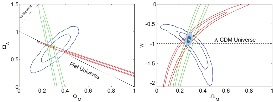
Fig. 7.17 Combined constraints on the cosmological parameters \Omega_m, \Omega_\Lambda (left panel, assuming w = -1 ) and w, \Omega_m (right panel, assuming \Omega_\kappa = 0 ) from SNIa, CMB and BAO data. Red contours give 68.3% and 95.4% regions from CMB alone, green contours from BAO alone, blue contours from SNIa alone from our Bayesian method. The filled regions delimit 68.3% and 95.4% combined constraints, with the yellow star indicating the posterior mean. Fig. from [7]
