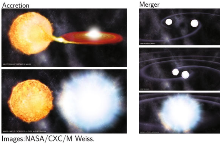
Fig. 4.3 Schematic showing the two most popular SNe Ia progenitor scenarios—both involve mass transfer in a binary system. The left hand panel shows the single degenerate accretion scenario in which a red giant or other main sequence star gradually accretes on to the white dwarf. The right hand panel shows the double degenerate merger scenario in which two white dwarfs merge (Images: NASA/CXC/M. Weiss)
