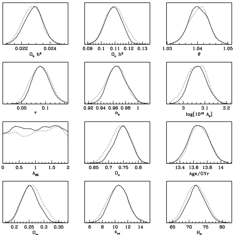
Fig. 5.5 Cosmological parameter inference using WMAP data [18] and CosmoMC. ‘Getdist’ was used with the chains produced by CosmoMC shown in Fig. 5.4 to automatically produce plots of the marginal posteriors, using a similar technique to that demonstrated in Fig. 5.3, but taking into account the weight of the samples. Solid lines show marginal posterior, dotted lines show average likelihood
