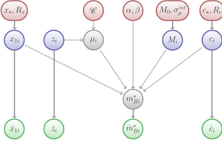
Fig. 7.8 Graphical representation of the Bayesian hierarchical network showing the deterministic (dashed) and probabilistic (solid) connections between variables in our Bayesian hierarchical model (BHM). Variables of interest are in red, latent (unobserved) variables are in blue and observed data (denoted by hats) are in green Fig. from [7]
