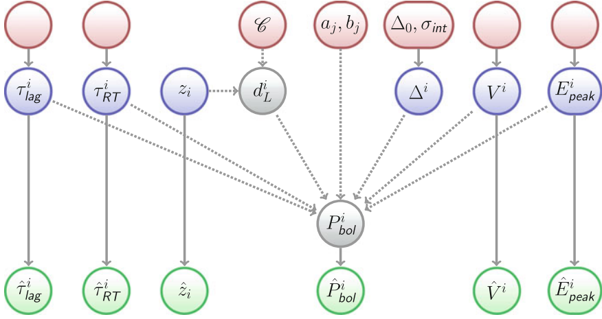
Fig. 7.21 Bayesian hierarchical network showing the deterministic (dashed) and probabilistic (solid) connections between variables in our Gamma Ray Burst Bayesian hierarchical model (GRBBHM). Variables of interest are in red, latent (unobserved) variables are in blue and observed data (denoted by hats) are in green. Note the additional parameter \Delta^i which models the intrinsic dispersion. In this case \Delta_0 \equiv 0
