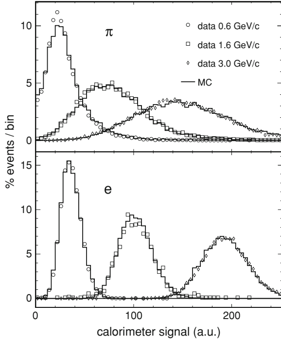
Fig. 3.19 Calorimetric response to pions and electrons at three momenta. The calorimeter-signal scale is in arbitrary units. The data obtained from CalDet is compared to the simulation. Image obtained from [16]
