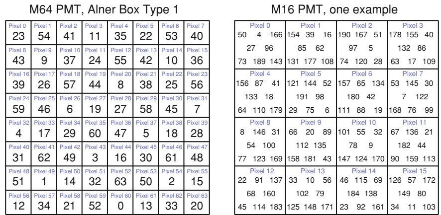
Fig. 8.4 An example of the relationship between pixel number and strip number for the M64 ( left ) and the M16 ( right ). The example on the left serves one partial U plane in the ND, while the one on the right serves 2/3 of a FD plane. Images obtained from [8]
