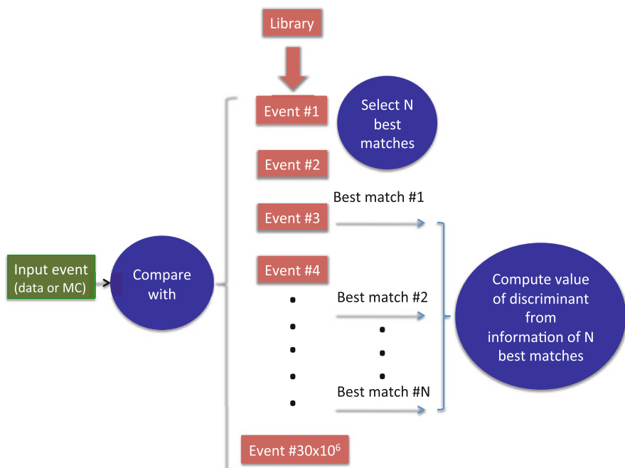
Fig. 5.6 Schematic view of the LEM algorithm. Each input event (represented by the box at the left) is compared to a library consisting of 30M signal and background events (represented by the vertically stacked boxes). At the end of the comparison the N best matches are recorded, and a discriminant is constructed from their information. For instance, the simplest discriminant that can be built is the fraction of the N best matches that are v_e CC events
