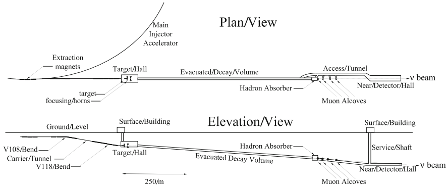
Fig. 3.3 Plan and elevation views of the NuMI facility. A proton beam is directed onto the target at an angle of 58 mrad with respect to the surface. The secondary pions and kaons from the target are focused into an evacuated decay volume via magnetic horns. Ionization chambers at the end of the beamline measure the secondary hadron beam and tertiary muon beam. Image obtained from [6]
