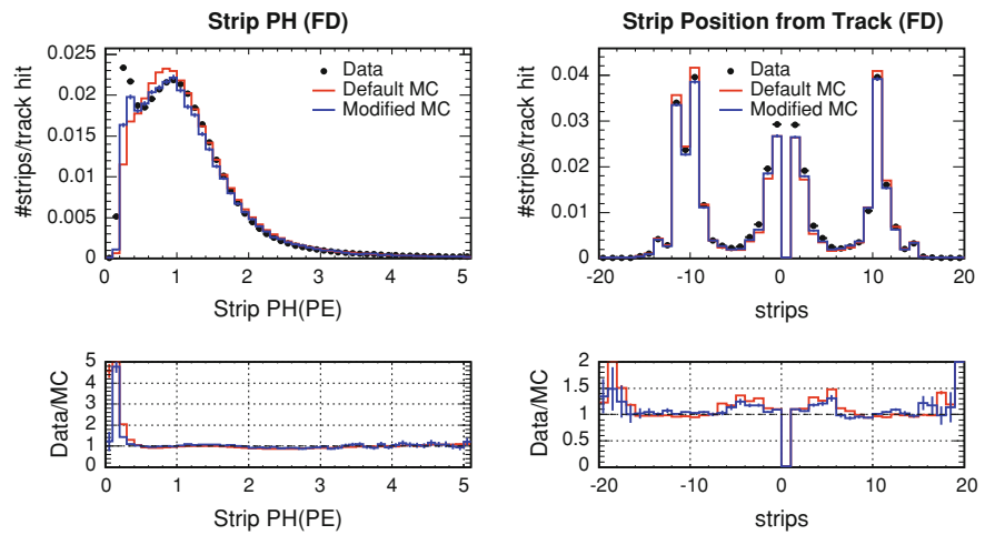
Fig. 8.3 Far Detector strip charge distribution of crosstalk hits around tracks ( left ), and distribution of transverse strip position from track center ( right ). The corresponding ratios of data to MC are shown in the bottom . The modified (retuned) crosstalk simulation improves the data to MC agreement, although the agreement there was already good. The strip charge distribution in the data has a double peak structure, corresponding most likely to the contributions from the electrical (charge) and optical crosstalk. Images obtained from [8]
