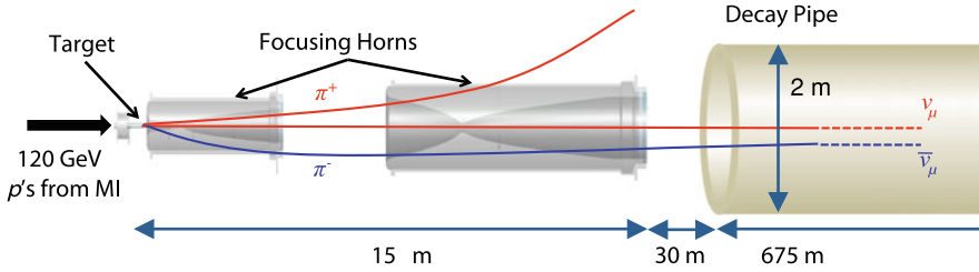
Fig. 10.14 Schematic of the NuMI beamline in Reversed Horn Current (RHC) mode. Positively charged particles from the target are defocused, and negatively charged particles are focused into the decay pipe. Only the positively charged particles that go through the center of the horns make it through. The result is a beam consisting primarily of antineutrinos
