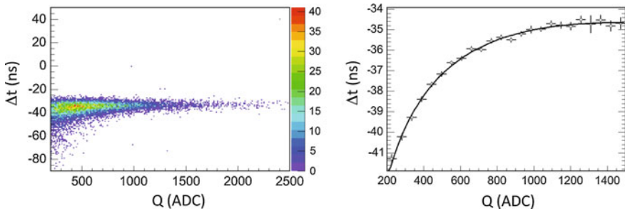
Fig. A.10 \Delta t vs. Q for one particular PMT. The right plot is the profile of the two-dimensional plot on the left shown on an expanded scale, and is fit to a third-degree polynomial up to 1500 ADC counts
