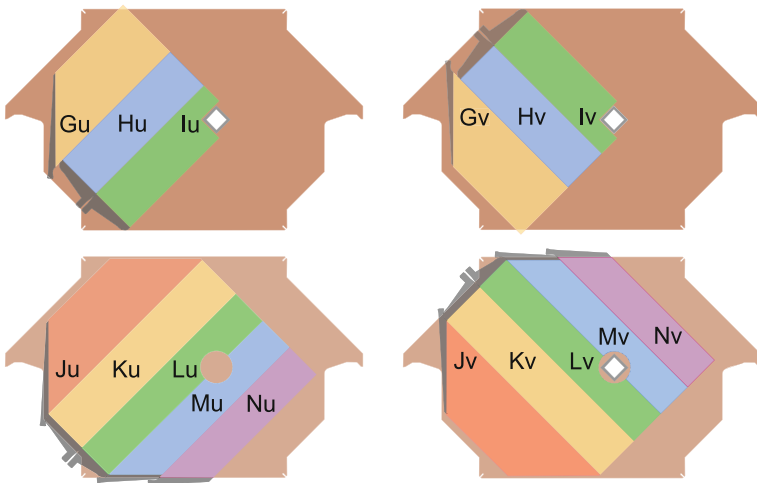
Fig. 3.9 The four different configurations of planes used in the Near Detector. The upper planes are partially instrumented, while the bottom ones are fully instrumented. The left planes are U planes , while the right ones are V planes . The G-N notations denote the different shapes of the scintillator modules. The U and V planes require slight variations in each shape, leading to a total of 16 different modules. Image obtained from [16]
