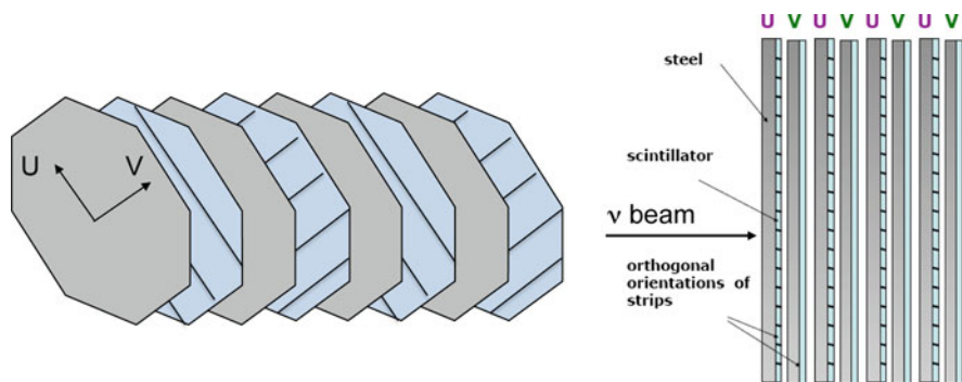
Fig. 3.5 Schematic of the MINOS steel-scintillator sampling calorimeters as viewed from an angle ( left ) and from the side ( right ). The detectors consist of planes of scintillator and steel. Alternating scintillator planes have strips perpendicular to one another. Even though the planes shown here have the octagonal shape of the Far Detector planes, the principle remains the same for the Near Detector
