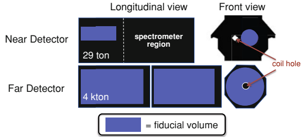
Fig. 5.1 A schematic view of the fiducial volume considered in both detectors. The Near Detector's fiducial volume amounts to 29 ton, and the Far Detector's to 4 kton
