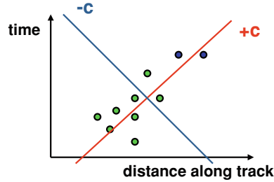
Fig. A.13 Schematic illustration of the determination of a track's direction. Green hits represent the hits in the main detector while blue hits (at the top ) represent the veto shield hits. In order to determine if a track is upward- or downward-going, the hit times are plotted as a function of distance along the track and then fitted to the upward-going and downward-going hypotheses. The RMS deviations for each of the two hypotheses are calculated and the hypothesis with the smallest RMS is chosen
