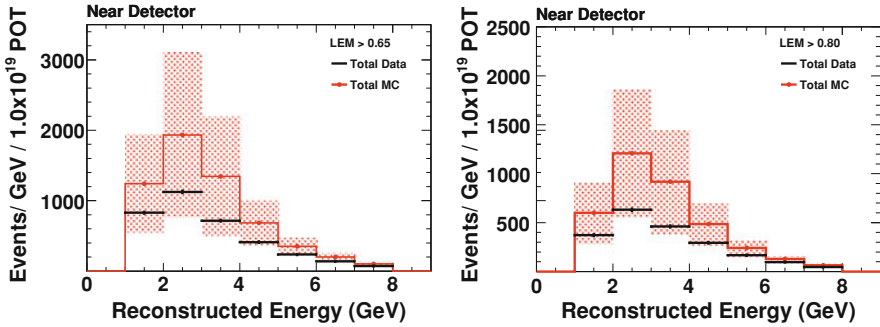
Fig. 6.2 Energy spectra of LEM selected events for a cut at 0.65 ( left ) and at 0.80 ( right ). The band represents the total systematic error on the simulation at the 1\sigma level for each energy bin. For both cuts the data is within the bounds of the systematic error. Note that the vertical scale is different for the two plots
