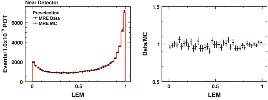
Fig. 7.12 MRE data and MC in the Near Detector for all events passing the MRE quality cuts and the preselection as a function of LEM pid ( left ), and the corresponding data/MC ratio ( right ). There is very good agreement between the MRE data and MC
