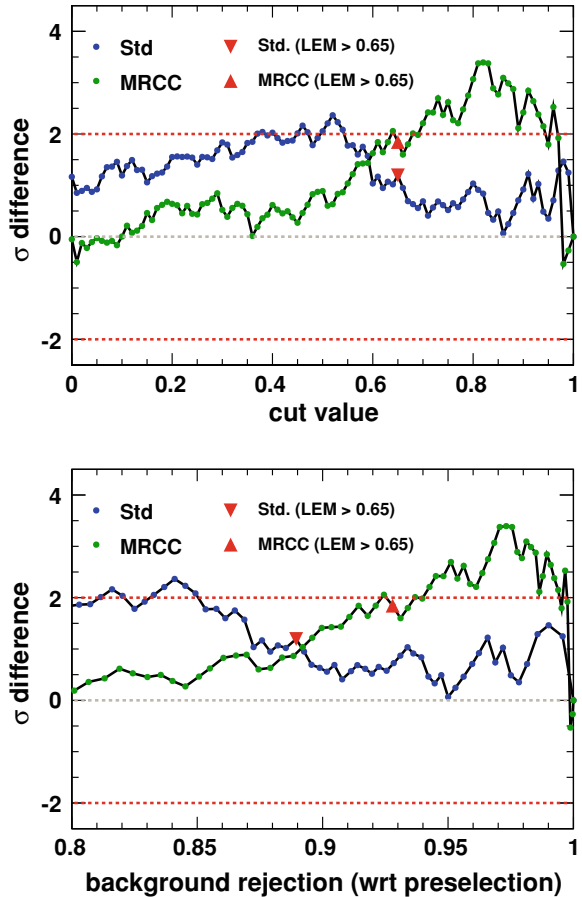
Fig. 9.20 Number of standard deviations from the background-only prediction as a function of cut value ( top ) and background rejection ( bottom ), for LEM selected events in the standard and MRCC samples. Systematic errors of 12% and 10% are used for all cut values in the standard and MRCC predictions respectively, which have a small effect given the dominance of the statistical error in both samples
