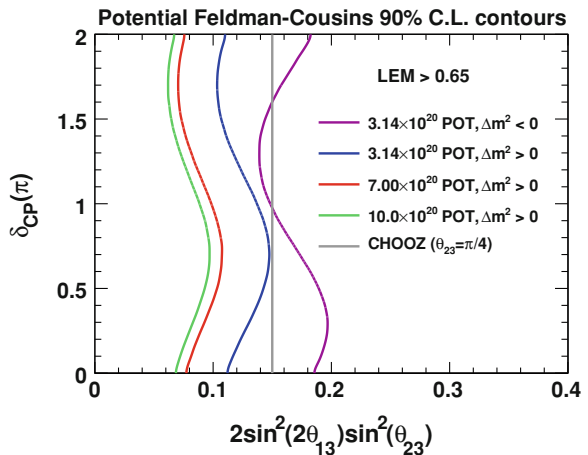
Fig. 10.3 Potential Feldman–Cousins 90% C.L. contours for the LEM > 0.65 selection at different exposures, for the case when the observation matches the background expectation. A systematic error on the background of 12.0% is used for the 3.14 \times 10^{20} POT exposure, and of 9.2% for the other two exposures. There is a very large gain in sensitivity in going from the first analysis to the second, but not so much when going from the second to the third
