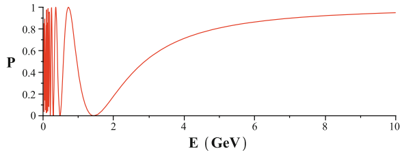
Fig. 2.6 Probability P of \nu_\mu survival in MINOS as a function of energy, with \sin^2(2\theta_{23}) = 1 and \Delta m_{32}^2 = 2.43 \times 10^{-3} \text{ eV}^2 . Oscillations are strongest at low ( \lesssim 5 GeV) energies
