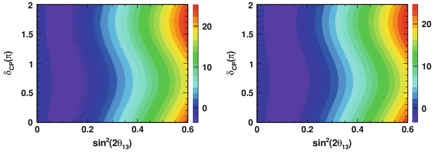
Fig. D.4 \Delta\chi^2_{90\%-\text{diff}} grid before and after smoothing. The edge of the region for which \Delta\chi^2_{90\%-\text{diff}} < 0 delineates the 90% C.L. contour
