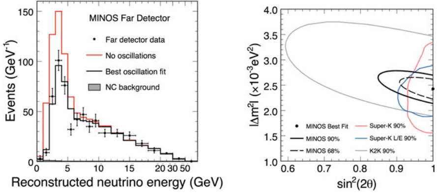
Fig. 2.8 Reconstructed energy spectrum of \nu_\mu CC-like events ( left ) and allowed region for neutrino oscillation parameters from MINOS and Super-Kamiokande ( right )
