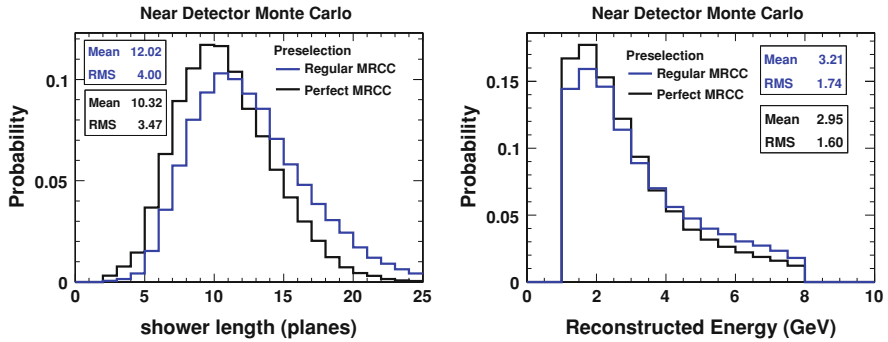
Fig. 9.8 Shower length ( left ) and reconstructed energy ( right ) distributions for perfect and regular MRCC events, normalized to unity. Regular MRCC events are longer and more energetic than perfect MRCC events
