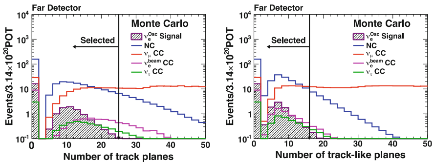
Fig. 5.2 Distributions of the number of track planes and track-like planes for different event types in the fiducial volume of the Far Detector. A track-like plane is a plane with no hits other than the ones associated with the track. By cutting at track planes < 25 and track-like planes < 16 a very significant portion of the NC and \nu_\mu CC background is removed at the expense of practically no signal. The signal corresponds to a value of \theta_{13} at the CHOOZ limit, neglecting matter effects and CP violation
