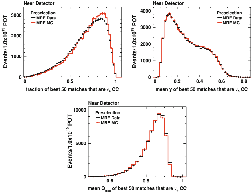
Fig. 7.11 MRE data and MC in the Near Detector for all events passing the MRE quality cuts and the preselection, as a function of the three variables that make up the LEM pid. There is very good agreement between the MRE data and MC
