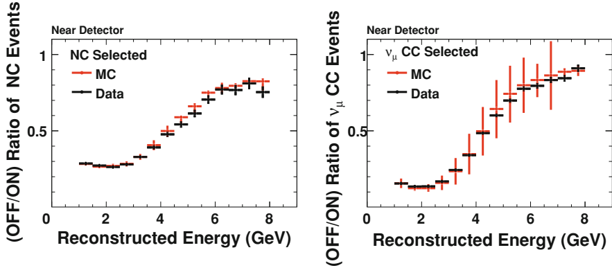
Fig. 6.11 r_{\text{NC}} (left) and r_{\text{CC}} (right) after fiducial volume cuts. The LEM cut value used here is 0.65. Here a \nu_\mu CC event is an event with a clearly defined track, and a NC event is an event with just a shower. The ratios are well modeled in the simulation. The error shown for the MC is the sum of the statistical and systematic errors
