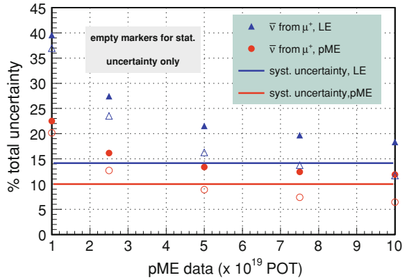
Fig. C.10 The expected uncertainty on p_{\text{LE}} (blue triangles) and p_{\text{ME}} (red circles) as a function of pME exposure. The total uncertainty is indicated by the filled markers and the empty markers represent the statistical uncertainty only. The horizontal lines indicate the total systematic uncertainty
