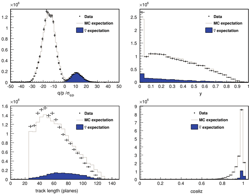
Fig. C.5 Input observables to PID are shown after preselection for ND events in data ( points ) and expected MC ( grey ) in the low energy (LE) beam configuration. The expected \bar{\nu}_\mu contribution as obtained from the simulation is shown by the shaded histograms
