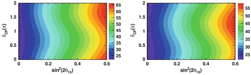
Fig. D.1 Number of expected events N_{\text{exp}} selected with \text{LEM} > 0.65 as a function of \sin^2 2\theta_{13} and \delta_{\text{CP}} , for the normal mass hierarchy (left) and the inverted mass hierarchy (right). N_{\text{exp}} increases with \theta_{13} and depends on \delta_{\text{CP}} . At the \theta_{13} = 0 boundary however there is no dependence on \delta_{\text{CP}}
