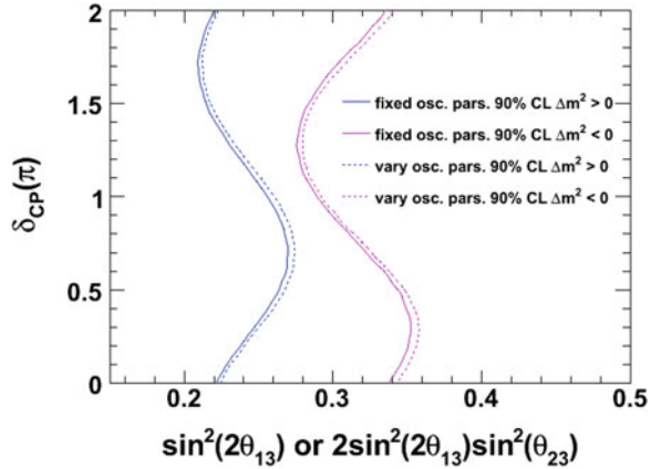
Fig. D.11 A comparison between the contours of Fig. D.10 with those of Fig. D.5. When the x -axis parameterization is changed to 2 \sin^2(2\theta_{13}) \sin^2(\theta_{23}) , the impact of varying the oscillation parameters is very small. If the parameterization is not changed however the contours degrade by approximately 15%, as explained in Sect. D.2.3
