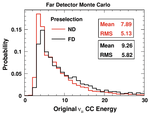
Fig. 9.12 True energy of MRCC parents in the Near and Far Detectors, normalized to unity. Due to oscillations, the average true energy of the \nu_\mu CC parents is \sim 1.4 GeV higher in the Far Detector
