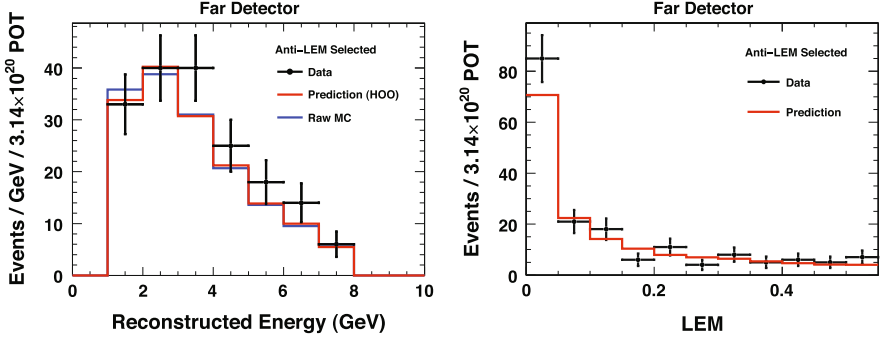
Fig. 9.1 Reconstructed energy spectra ( left ) and LEM pid distribution ( right ) for the events in the anti-LEM sideband. The prediction at each bin on the right plot is calculated using the PORP method. The data-MC agreement is very good in all regions of the distributions, given the available statistics
