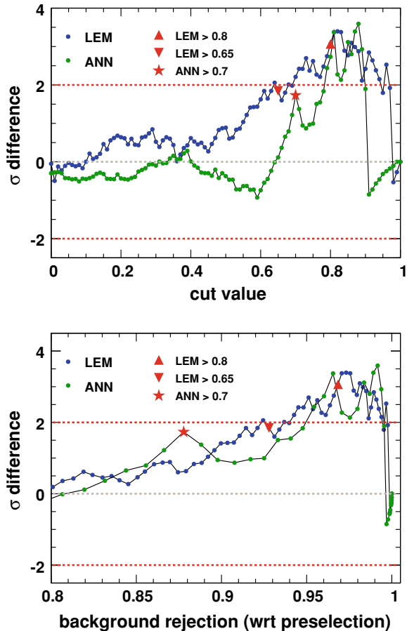
Fig. 9.13 Number of standard deviations from the prediction in the MRCC sideband, as a function of cut value ( top ) and of rejected background ( bottom ). A flat systematic error of 10% and 7.5% on the MRCC prediction is assumed for all cut values of LEM and ANN respectively when calculating the \sigma diff., which has a small impact given the dominance of the statistical error, particularly at medium and high cut values. Both selections see excesses of similar significance at high rejected background
