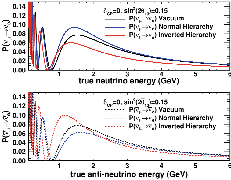
Fig. 4.1 \nu_e and \bar{\nu}_e appearance probability in MINOS as a function of true neutrino energy for \delta = 0 and \sin^2(2\theta_{13}) = 0.15 , with standard oscillation parameters \Delta m_{32}^2 = 2.38 \times 10^{-3} \text{ eV}^2 , \Delta m_{21}^2 = 8.0 \times 10^{-5} \text{ eV}^2 , \theta_{23} = \pi/4 , \theta_{12} = 0.59365 . In MINOS both the selection efficiency and the number of events decrease drastically for E < 1 \text{ GeV} , and thus the first oscillation peak (centered around E \simeq 1.5 \text{ GeV} ) strongly dominates. For that first peak it can be clearly seen that in the case of the normal mass hierarchy matter effects enhance \nu_e appearance for neutrinos while they suppress it for antineutrinos. The situation is reversed in the case of the inverted mass hierarchy
