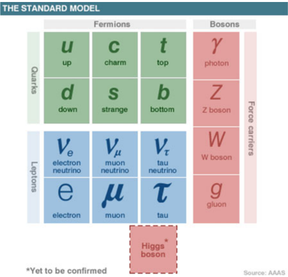
Fig. 2.1 A summary of the particle content of the Standard Model, which is composed of 12 fermions and 4 force carrier gauge bosons. There is also a Higgs boson, whose mechanism is thought to be responsible for the origin of mass. Source: AAAS
