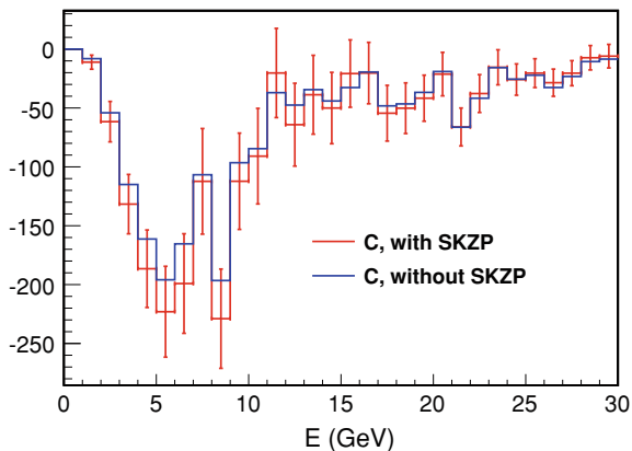
Fig. C.7 The expected difference C \equiv Q_{\text{HE}} - Q_{\text{LE}} in the \bar{\nu}_\mu flux from pions and kaons with (red line) and without (blue line) SKZP-reweighting. The error bars represent the statistical uncertainty due to the size of the available MC samples
