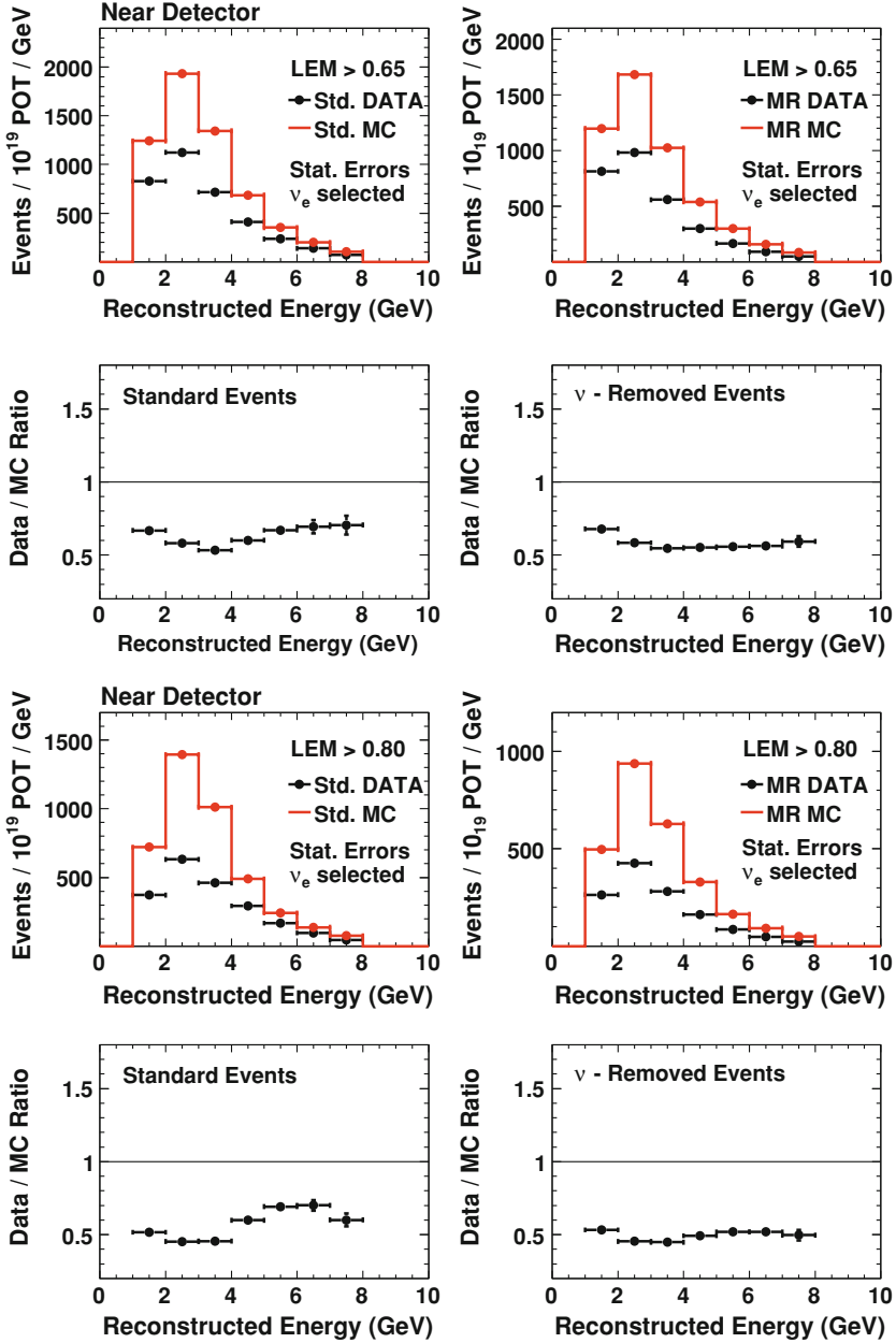
Fig. 6.19 Reconstructed energy spectra of LEM selected events with a cut at 0.65 ( first row ) and at 0.80 ( third row ), in the standard sample ( left ) and in the MRCC sample ( right ). The corresponding ratios of data to MC are also shown in the second and fourth rows for the cut at 0.65 and at 0.80 respectively. The data-MC disagreement is similar between the two samples as a function of reconstructed energy, for the two LEM cut values
