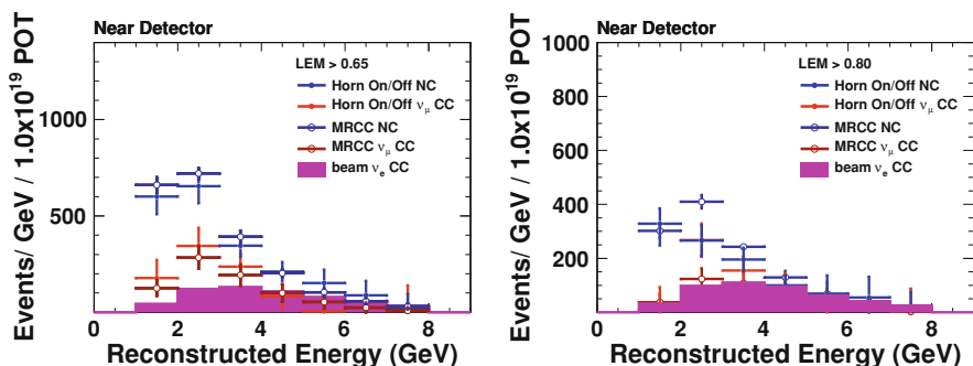
Fig. 6.21 Background decomposition of LEM selected events as given by HOO and by MRCC with a cut at 0.65 ( left ) and at 0.80 ( right ). The two decomposition methods are consistent to each other, and the differences are within 1\sigma for most bins of reconstructed energy
