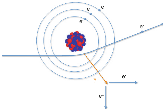
Fig. 4.4 Schematic of the processes responsible for the electromagnetic cascade that occurs when electrons travel in dense matter. The deflection of electrons by the atomic nuclei cause the emission of photons, which in turn materialize through e^+e^- pair production. This process is repeated until the energy of the charged secondaries is low enough in such a way that ionization becomes the dominant mechanism for energy loss
