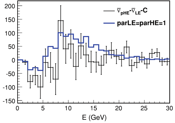
Fig. C.9 The histogram with statistical error bars is the difference in the measured normalized pHE and LE \bar{\nu}_\mu spectra in data corrected by the difference C \equiv Q_{\text{HE}} - Q_{\text{LE}} derived from simulation. The blue solid line represents the expected shape when p_{\text{LE}} and p_{\text{HE}} are set to the nominal value of unity
