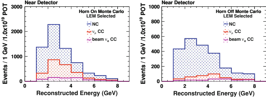
Fig. 6.10 Reconstructed energy spectra of LEM selected events (with a LEM pid cut at 0.65) in the horn-on and horn-off configurations, as simulated in the Near Detector MC. Applying the LEM selection to the data taken in the horn-off configuration results in a NC-enriched sample
