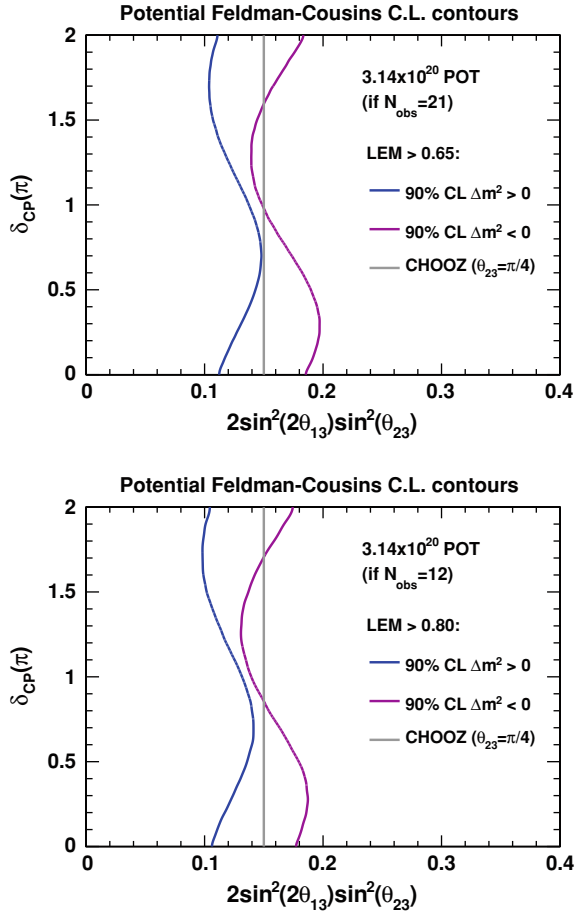
Fig. 8.7 Potential Feldman–Cousins 90% C.L. exclusion contours for the \text{LEM} > 0.65 (top) and \text{LEM} > 0.80 (bottom) selections, for an observation of 21 and 12 events respectively. The region of parameter space to the right of the blue and purple curves would be excluded at 90% C.L. for the normal and inverted mass hierarchy cases. In both situations the CHOOZ limit would be excluded for the case of maximal mixing and the normal hierarchy
