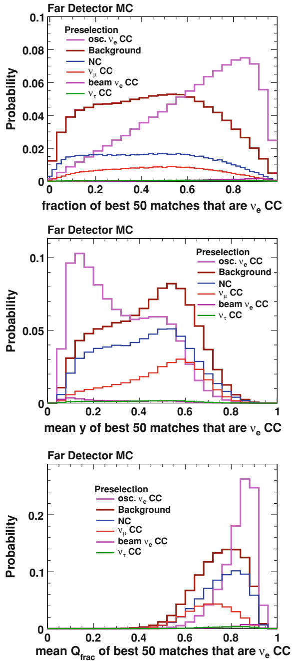
Fig. 5.15 The three variables that are combined into the LEM pid for all events passing the preselection, in the Far Detector. The total background and the signal curves are scaled to unity. The individual background components are scaled so that their proportion to the total background remains correct
