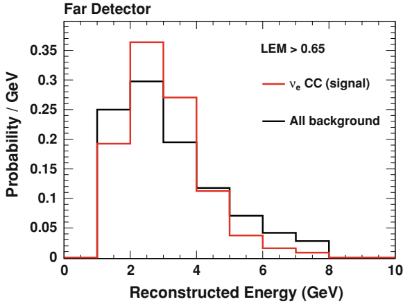
Fig. 7.4 Predicted background and expected signal in the Far Detector for \text{LEM} > 0.65 , normalized to unity. The background is predicted using the PORP method (described in Sect. 5.4.3), which yields a total background of 21.6 events spread over the 1–8 GeV energy range as shown by the black distribution. The shapes of the background and the potential signal are too similar, and the statistics too low, for an energy-dependent fit to improve the sensitivity obtained when the total number of events observed in the data is compared to the total background expectation integrated over all energies
