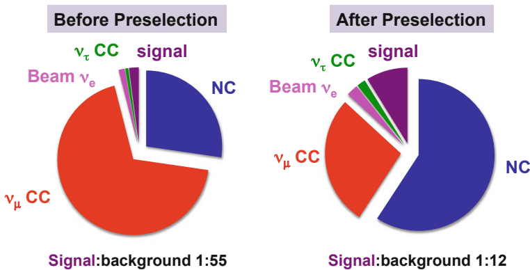
Fig. 5.4 Event type composition in the Far Detector before and after the preselection cuts have been applied. The signal corresponds to a value of \theta_{13} at the CHOOZ limit, neglecting matter effects and CP violation
