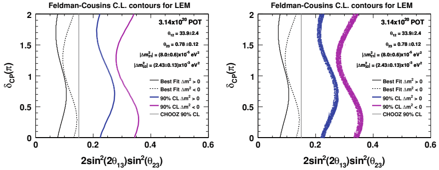
Fig. D.10 Smooth (left) and raw (right) Feldman–Cousins 90% C.L. contours for the LEM > 0.65 selection, for an observation of 28 events. The uncertainties in the oscillation parameters are included
