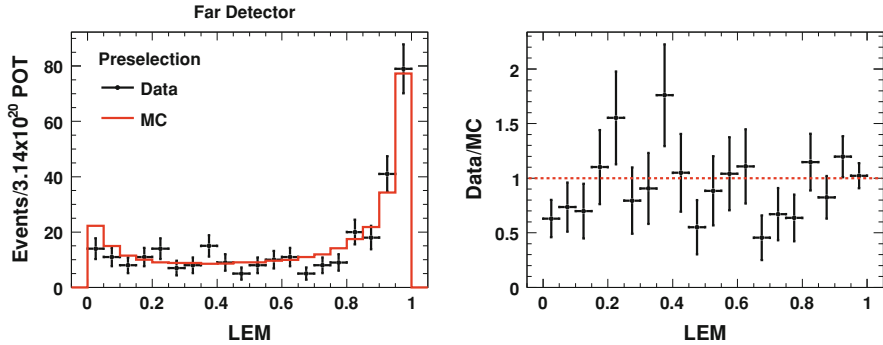
Fig. 9.3 LEM pid distribution of Far Detector MRE events ( left ) and the corresponding data to MC ratio ( right ). The agreement between the data and the MC is very good
