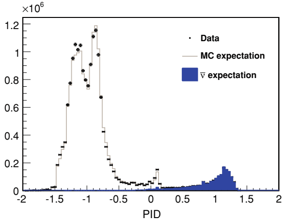
Fig. C.6 Resulting PID distribution used for \bar{\nu}_\mu selection is shown for ND events in data (points) and expected MC (grey) in the low energy (LE) beam configuration. The expected \bar{\nu}_\mu contribution as obtained from the simulation is shown by the shaded histogram
