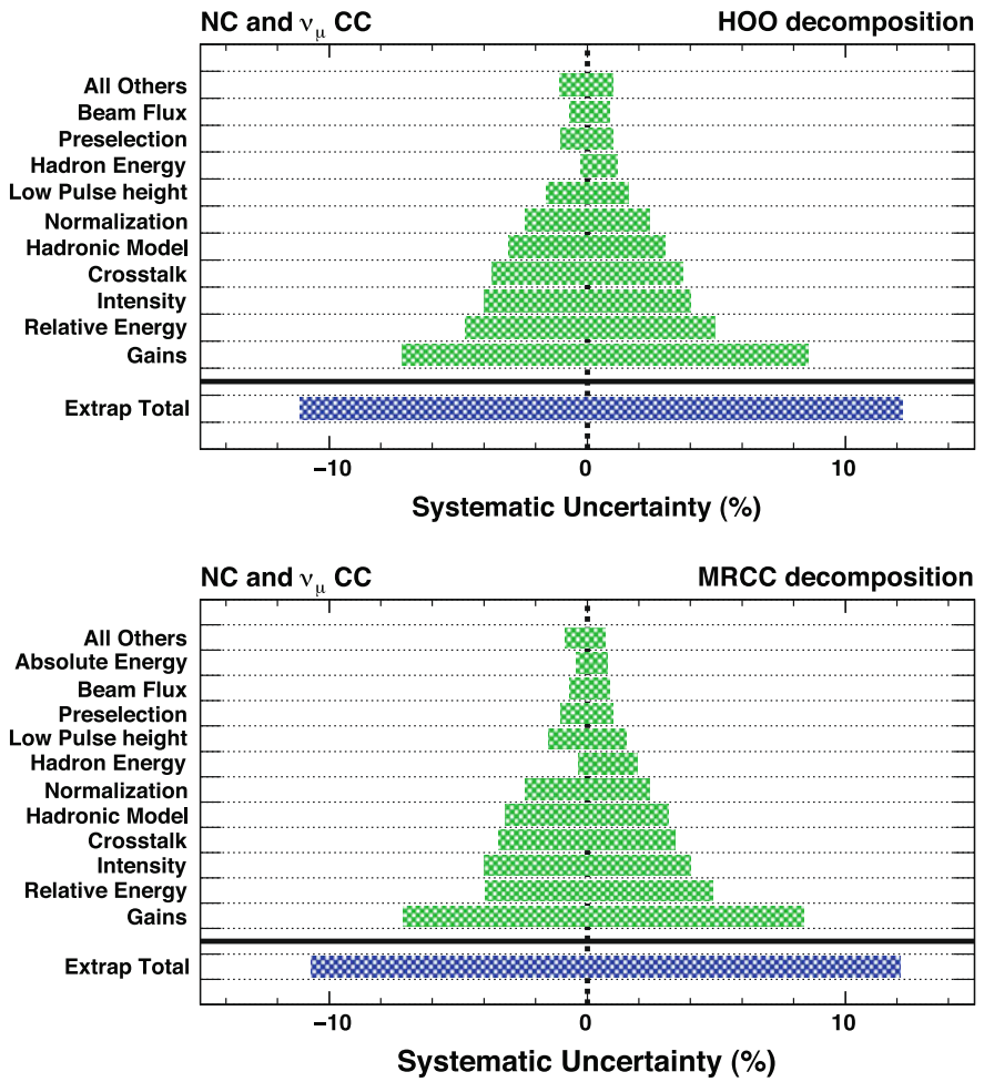
Fig. 8.6 Extrapolation systematic uncertainties in the NC + \nu_\mu CC prediction at the Far Detector, for the HOO decomposition ( top ) and the MRCC decomposition ( bottom ). The sources of systematic error are arranged in order of increasing importance. Systematic effects that contribute less than 0.7% are grouped into the all others category
