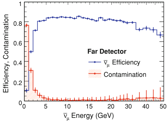
Fig. 10.8 Far Detector efficiency and contamination of the \bar{\nu}_\mu CC selector used in the most recent analysis [8]
