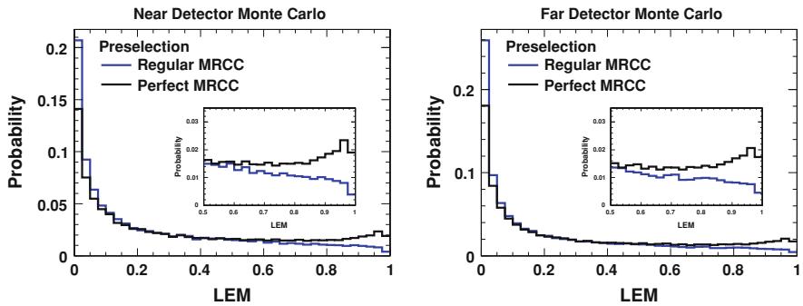
Fig. 9.9 LEM pid distribution of regular and perfect MRCC events in the Near ( left ) and Far ( right ) detectors. Significant differences exist between the two samples, particularly at high-LEM values
