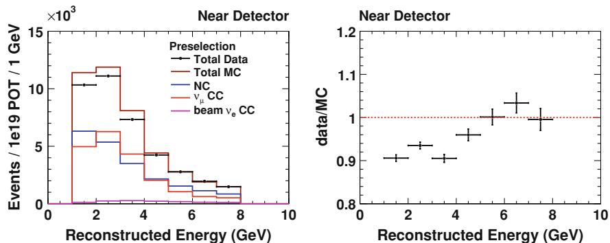
Fig. 5.5 Energy spectrum of preselected events in the Near Detector ( left ) and corresponding data to MC ratio ( right ). The data and the MC agree to within 10% at the preselection level
