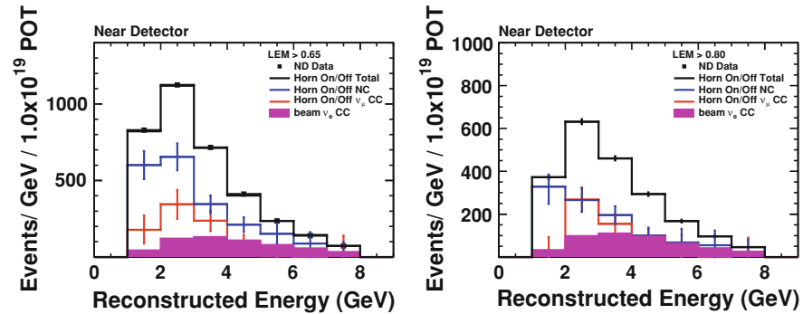
Fig. 6.13 Energy spectra of LEM selected events decomposed by HOO with a cut at 0.65 (left) and at 0.80 (right)
