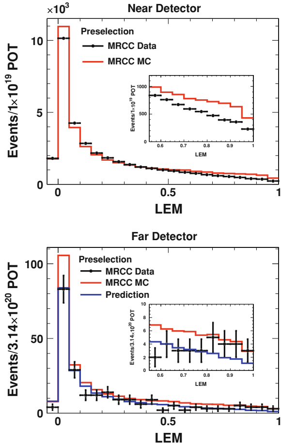
Fig. 9.6 The LEM pid distribution for MRCC preselected events in the Near ( top ) and Far ( bottom ) detectors. The Far Detector data agrees better with the prediction than with the default MC until about LEM \approx 0.8 , at which point a constant excess is observed. The events at LEM pid < 0 are the preselected events that do not get any matches in the LEM library
