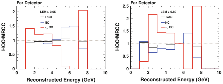
Fig. 7.8 Comparison between the HOO and MRCC Far Detector predictions as a function of energy, for a LEM cut at 0.65 ( left ) and at 0.80 ( right ). Even if the NC (blue) or \nu_\mu CC (red) components disagree somewhat between the HOO and MRCC methods, the total predicted background (black) agrees very well
