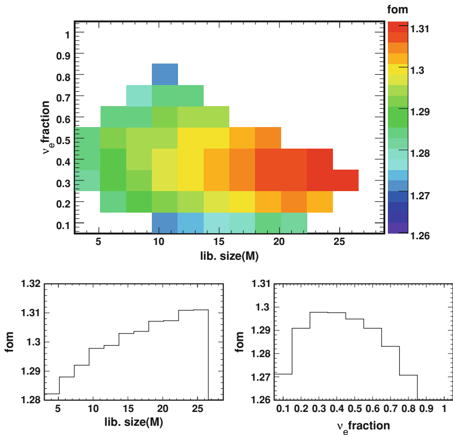
Fig. 5.13 (top) Figure of merit (fom) as a function of the \nu_e fraction and the total library size. The \nu_e fraction is defined as the ratio between the number of \nu_e CC events in the library over the total library size. The cut values for the two variables used in the selection are optimized at every bin based on the fom. A nonstandard preselection is used as well as standard oscillation parameters. (bottom left) A slice of the two-dimensional histogram on the top for a constant \nu_e fraction of 0.3. (bottom right) A slice of the two-dimensional histogram on the top for a constant total library size of 10M
