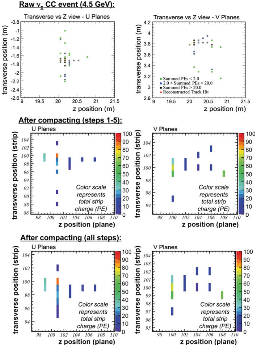
Fig. 5.9 A 4.5 GeV \nu_e CC event in the Far Detector being compacted by the LEM algorithm
