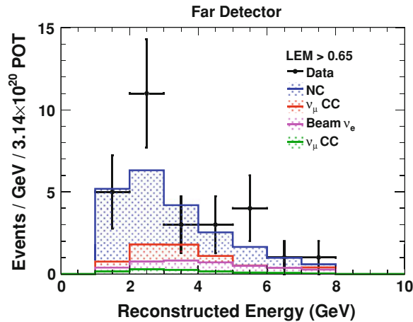
Fig. 9.15 Energy spectrum of the Far Detector data alongside the background prediction as determined using the HOO method. There is an overall excess in the data with respect to the background prediction
