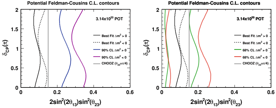
Fig. 9.22 Feldman-Cousins 90% ( left ) and 68% ( right ) C.L. contours for LEM, with the HOO decomposition, for the observation of 28 events. Since these plots constitute the main result of this thesis, they are redone under a different style and shown again in Fig. 9.24
