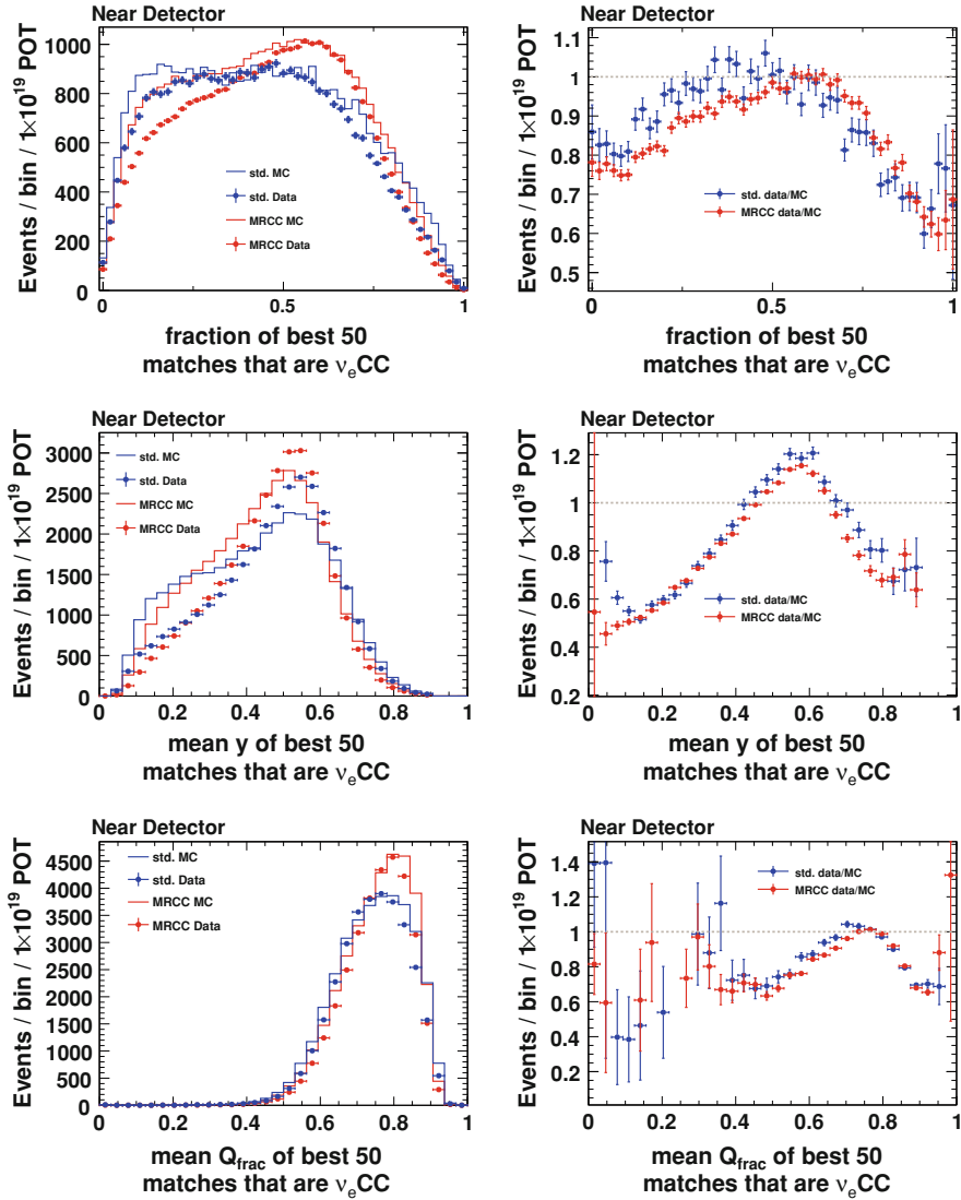
Fig. 6.18 The three variables that form the LEM pid in the standard and the MRCC samples, and the data/MC ratios for each sample ( right ). There are significant differences in the distributions between the two samples, but the data-MC ratios are similar
