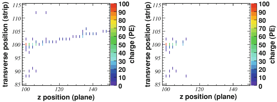
Fig. 6.15 An event in the Far Detector data before ( left ) and after ( right ) muon-removal. Due to the EM nature of the hadronic shower remnant, this MRCC event is selected by LEM as a \nu_e candidate. The clusters of hits below and above the main hadronic shower are due to cross-talk, and are entirely ignored by the LEM algorithm due to the 3.0 PE cut that is applied before events are compared to the library. Sometimes hits that occur in the same snarl (defined in Sect. 3.4.3) and that are not included in the original event end up being included in the muon-removed event. An example of this is the rightmost hit in the lower cross-talk cluster. Also, hits that were present in the original shower remnant can sometimes be lost in the MRCC event, such as the two cross-talk hits in the top
