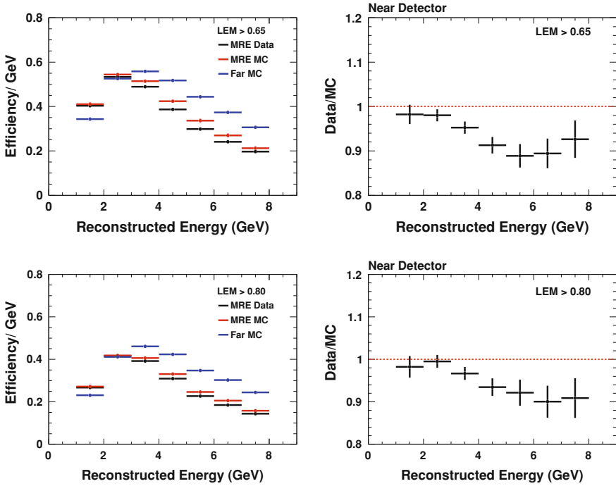
Fig. 7.13 \nu_e CC selection efficiencies in the MRE MC, MRE Data, and Far Detector MC ( left ), and the ratio of data/MC MRE efficiencies ( right ), for the LEM cut at 0.65 ( top ) and at 0.80 ( bottom )
