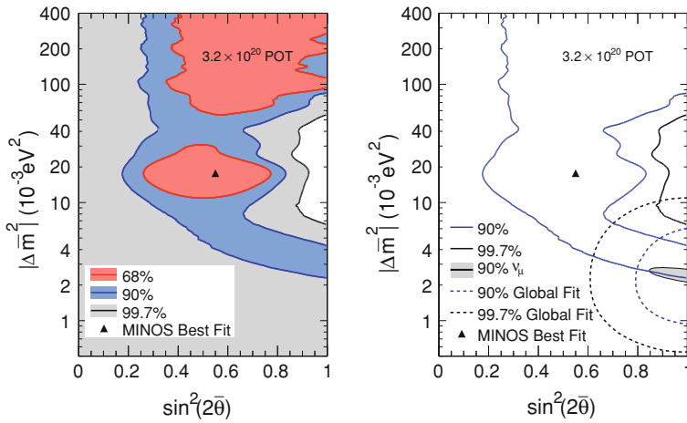
Fig. 10.13 Exclusion contours for the antineutrino disappearance results with 3.2 \times 10^{20} POT. The left plot shows the regions of parameter space allowed at the 68, 90% and 3\sigma C.L. The unshaded region around maximal mixing is excluded at 99.7%. The right plot shows the 90% and 3\sigma contours from our results and from a global fit [21] of all previous data. The most recent \nu_\mu CC disappearance results from MINOS are also shown for comparison
