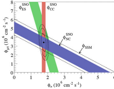
Fig. 2.5 Flux of boron-8 solar neutrinos which are \mu or \tau flavor vs. flux of electron neutrinos deduced from the three neutrino reactions in SNO. The diagonal bands show the total boron-8 flux as predicted by the Solar Standard Model (SSM), while the diagonal solid bands represents the SNO NC measurement. The intercept of these bands with the axes represent the \pm 1\sigma errors. The bands intersect at the fit values for \phi_e and \phi_{\mu\tau} , indicating that the combined flux results are consistent with neutrino flavor transformation with no distortion in the boron-8 neutrino energy spectrum. Image obtained from [47]
