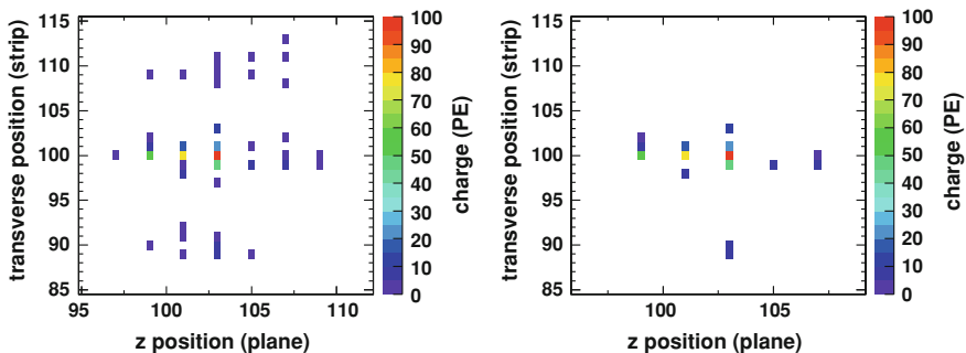
Fig. 8.5 A simulated \nu_e CC event before ( left ) and after ( right ) the 3.0 PE cut applied by the LEM algorithm. The cross-talk hits form a cluster approximately ten strips below and above the shower hits. Practically all of them are removed by the 3.0 PE cut
