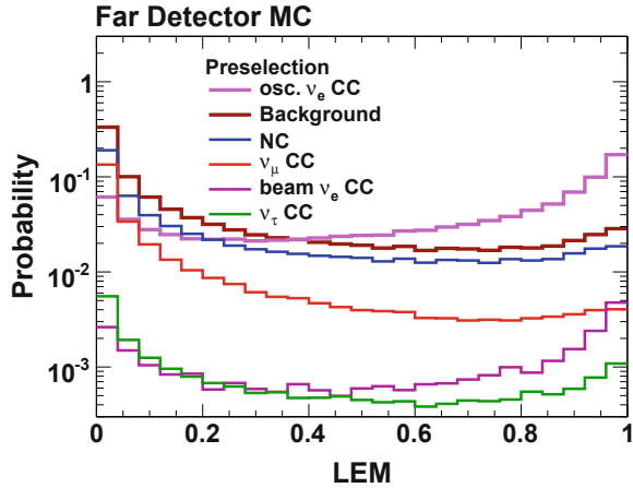
Fig. 5.17 The LEM pid in the Far Detector, on semilogarithmic scale. The total background and the signal curves are scaled to unity. Each of the individual background components is scaled so that its proportion to the total background remains correct. A similar plot in linear scale can be found in Fig. 4.11
