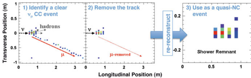
Fig. 6.14 Graphical illustration of the MRCC technique. MRCC events constitute a pure sample of quasi-NC events, and can thus be used to provide a data-based correction to the NC background component from the simulation or as an independent sideband
