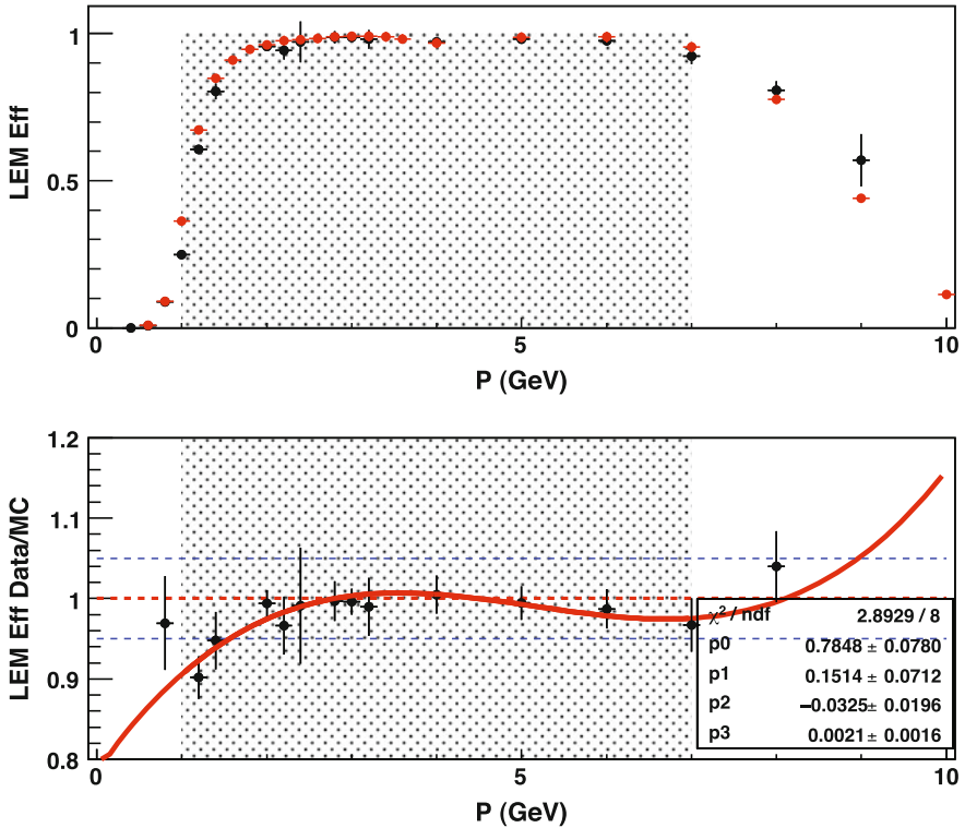
Fig. 7.9 (top) Selection efficiencies of CalDet electrons in the data (points) and the MC (solid curve), and (bottom) the corresponding data to MC ratio. The data to MC ratio is fit to a third-order degree polynomial. The shaded region is where the fit is done, which is also the energy region where most of the signal is
