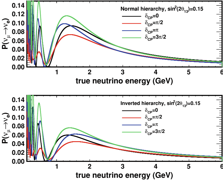
Fig. 4.2 \nu_e appearance probability in MINOS as a function of true neutrino energy for \sin^2(2\theta_{13})=0.15 , with standard oscillation parameters \Delta m_{32}^2 = 2.38 \times 10^{-3} \text{ eV}^2 , \Delta m_{21}^2 = 8.0 \times 10^{-5} \text{ eV}^2 , \theta_{23} = \pi/4 , \theta_{12} = 0.59365 . Varying the CP-violating phase \delta causes significant changes in the oscillation probability, by as much as approximately \pm 25\% for energies higher than 1 GeV
