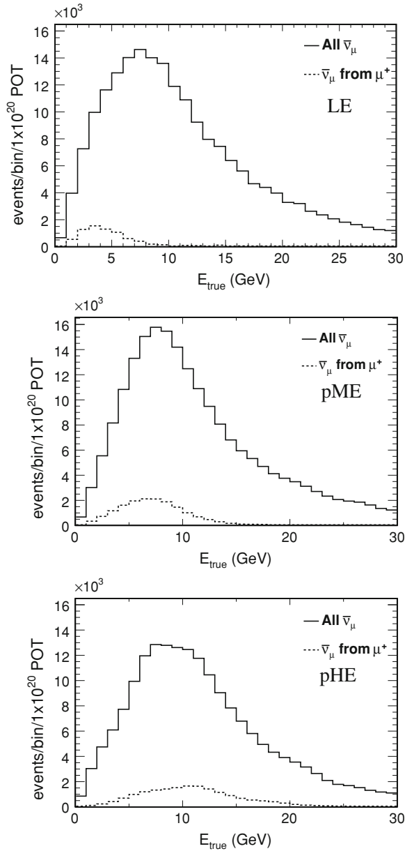
Fig. C.1 True energy spectra in the Near Detector of “all antineutrinos” and “antineutrinos from \mu^+ decay” in the low-energy (LE), pseudo-medium energy (pME) and pseudo-high energy (pHE) beam configurations. All histograms correspond to 1 \times 10^{20} POT (protons-on-target)
