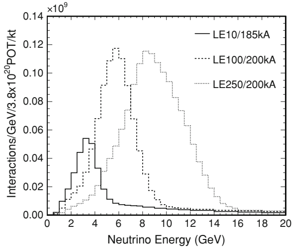
Fig. 3.4 Simulated rate of \nu_\mu CC interactions in the MINOS Near Detector. Three spectra are shown, corresponding to the low-energy (LE), pseudo-medium energy (pME) and pseudo-high energy (pHE) beam configurations. For these configurations the separation between the target and the horns is 10, 100 and 250 cm, and the horn current is 185, 200 and 200 kA respectively. Image obtained from [6]
