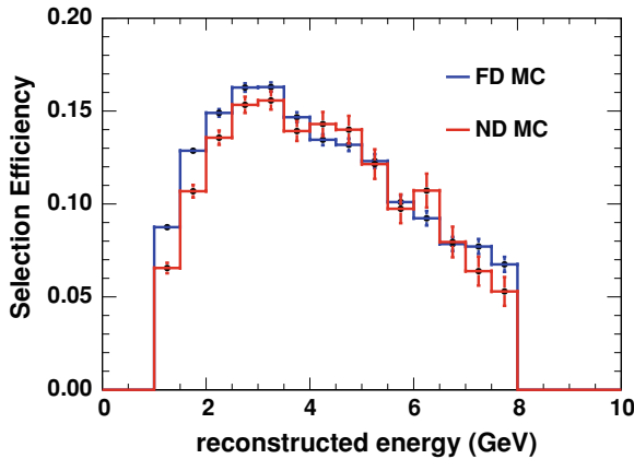
Fig. B.8 Selection efficiency of background events in the two detectors as a function of reconstructed energy. The efficiencies are calculated with respect to the number of preselected events. \nu_\tau CC events are not included for the Far Detector, in order to have a fair comparison between detectors. The similarity between the two curves indicates that LEM acts very similarly in both detectors. All the available MC was used to make this plot
