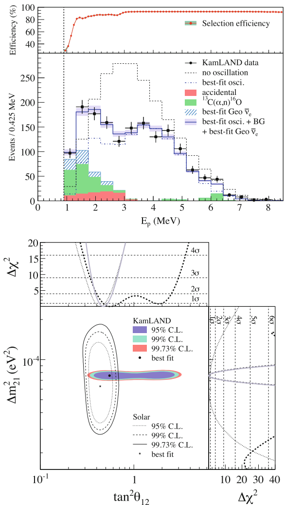
Fig. 2.7 Prompt event energy spectrum of \bar{\nu}_e candidate events (top) and allowed region for neutrino oscillation parameters from KamLAND and solar neutrino experiments (bottom). All histograms corresponding to reactor spectra and expected backgrounds incorporate the energy-dependent selection efficiency shown on the top. For the bottom plot, the side panels show the \Delta\chi^2 -profiles for KamLAND ( dashed ) and solar experiments ( dotted ) individually, as well as their combination (solid). Images obtained from [54]
