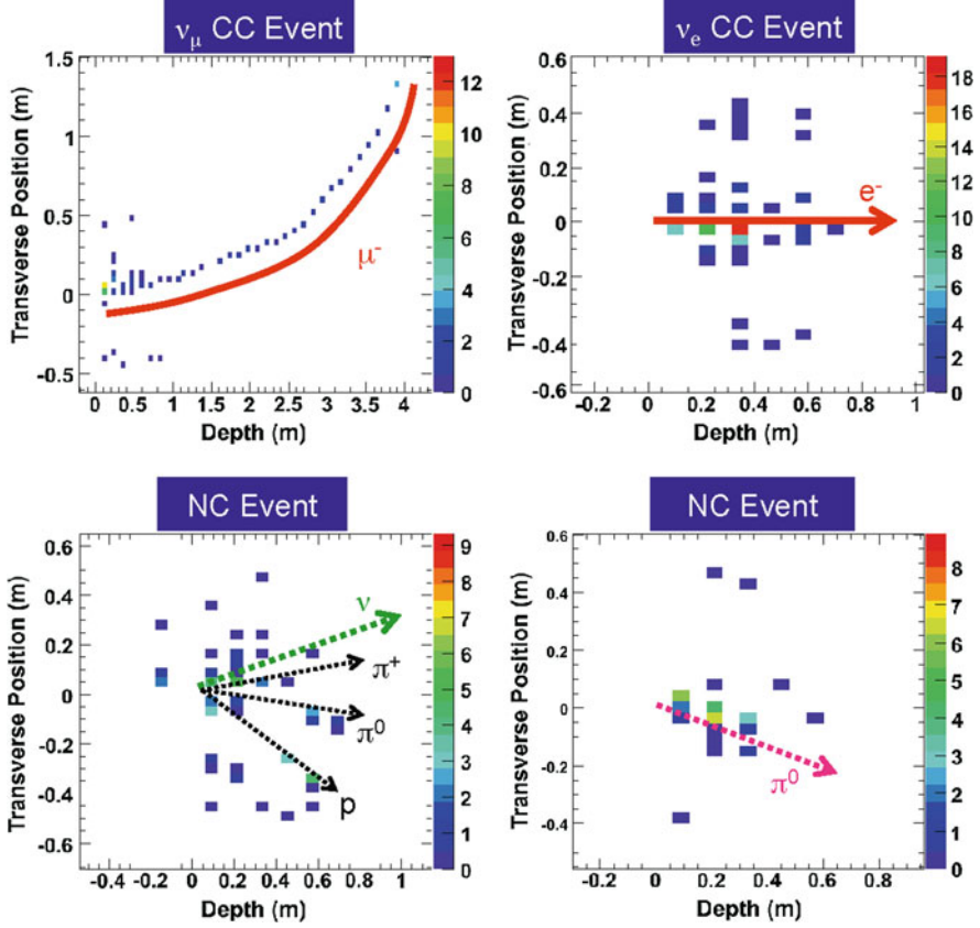
Fig. 4.3 Simulated event topologies in MINOS. The color scale represents the charge deposited per strip in Minimum Ionizing Particle (MIP) units. Most \nu_\mu CC events leave an unmistakable signature in the detector consisting of a long muon track with hadronic activity at the vertex. \nu_e CC events are usually compact showers with a characteristic electromagnetic profile. NC events tend to be more diffuse than EM showers; a typical example is the bottom-left event where a 1.7 GeV proton is produced alongside a 1.9 GeV \pi^+ and a 1.2 GeV \pi^0 (alongside other less energetic particles). Sometimes \pi^0 's that carry an important fraction of the energy transferred to the struck nucleus are produced in NC interactions, giving a significant EM component to the shower, as in the bottom-right event
