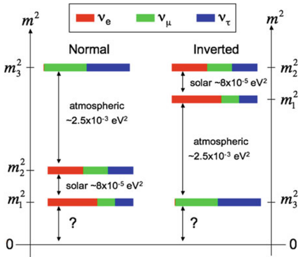
Fig. 2.10 Three-flavor neutrino mass spectrum in the normal and inverted mass hierarchies cases
