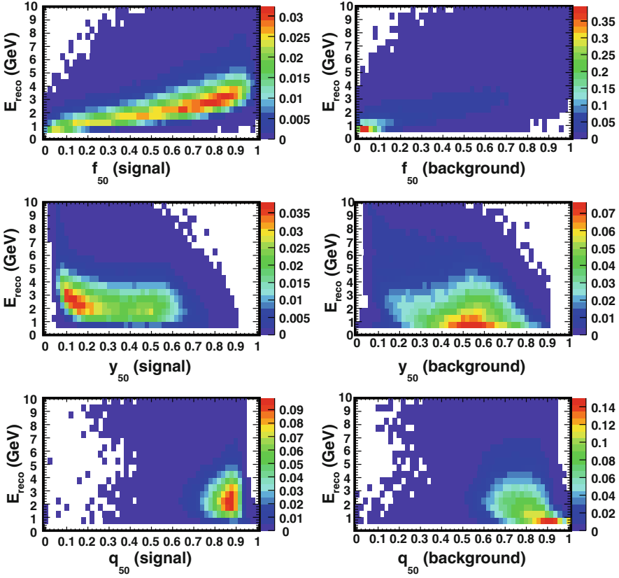
Fig. 5.18 Two-dimensional histograms of reconstructed energy as a function of the three variables used to construct the LEM pid. The Z-axis scale represents the number of Far Detector events per bin per 10^{19} POT. The first column is for signal events and the second column for background events, which includes all four types of background. The \nu_e preselection is applied. All events are weighted by their oscillation probability according to standard oscillation parameters except for \sin^2(2\theta_{13}) = 0.5 . As expected, the signal and the background separate more clearly as the energy increases
