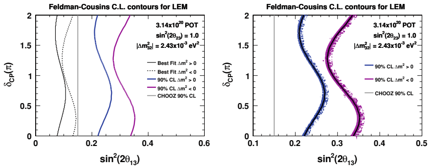
Fig. D.5 Left smooth 90% C.L. contours with the LEM > 0.65 selection for an observation of 28 events. Right a comparison between the raw (in blue and purple) and the smooth contours (superimposed in black). Please note that the x-axis scale is different for the two plots. The smooth contours fall approximately in the middle of the raw contours
