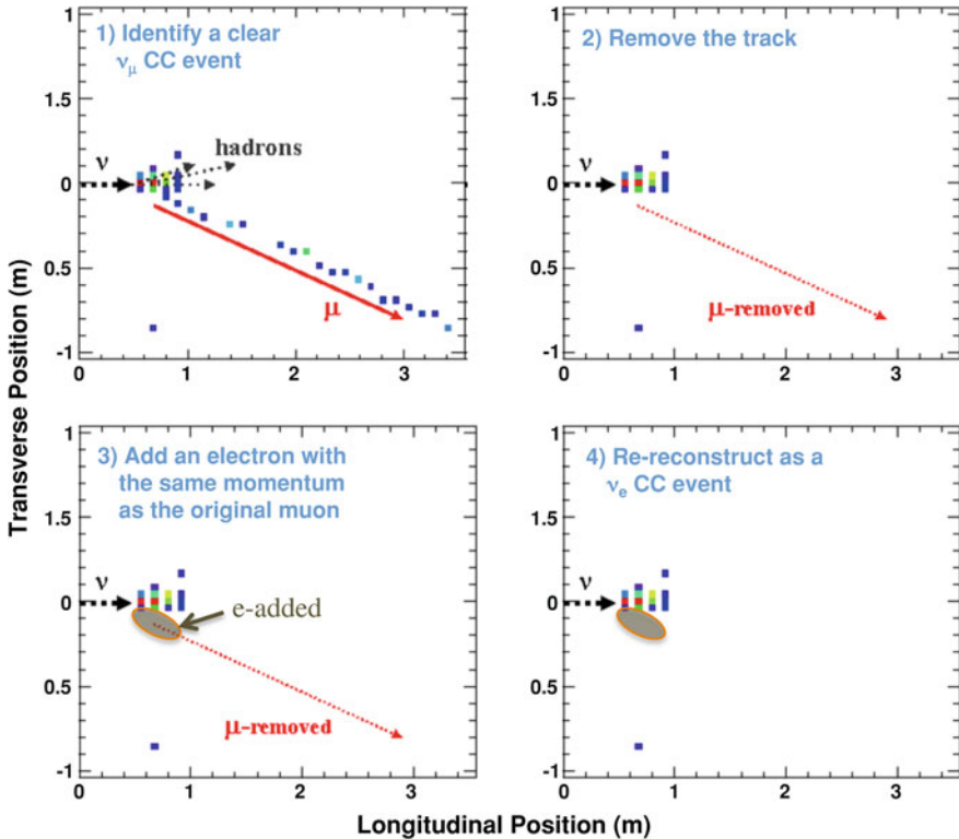
Fig. 7.10 A graphical illustration of the procedure followed to obtain MRE events. First, clear long tracks from \nu_\mu CC events are identified, and the track removed. Then an electron with the same 4-momentum as the original muon is added, and the whole event re-reconstructed
