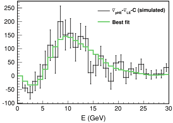
Fig. C.3 The fitted results of a single experiment with “fake” data corresponding to the statistics of Table C.1. The black histogram with error bars represents the ‘fake’ data and the green histogram represents the best fit result. C is the correction due to the antineutrinos from hadron parents, C \equiv Q_{HE} - Q_{LE}
