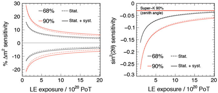
Fig. 10.4 Percentage sensitivity to \Delta m_{32}^2 (left) and to \sin^2(2\theta_{23}) as a function of exposure in POTs. The sensitivities obtained at 7.0 \times 10^{20} POT and at, for instance, 9.0 \times 10^{20} POT, differ only by a few percent, particularly for \Delta m_{32}^2 . Image obtained from [7]
