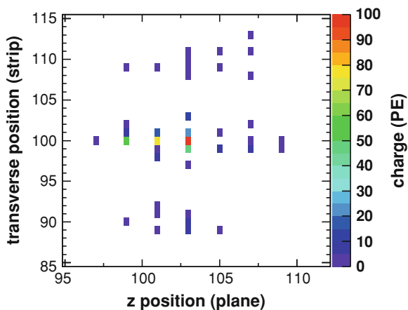
Fig. 3.14 A simulated \nu_e CC event. The crosstalk hits form a cluster approximately ten strips below and above the shower hits
