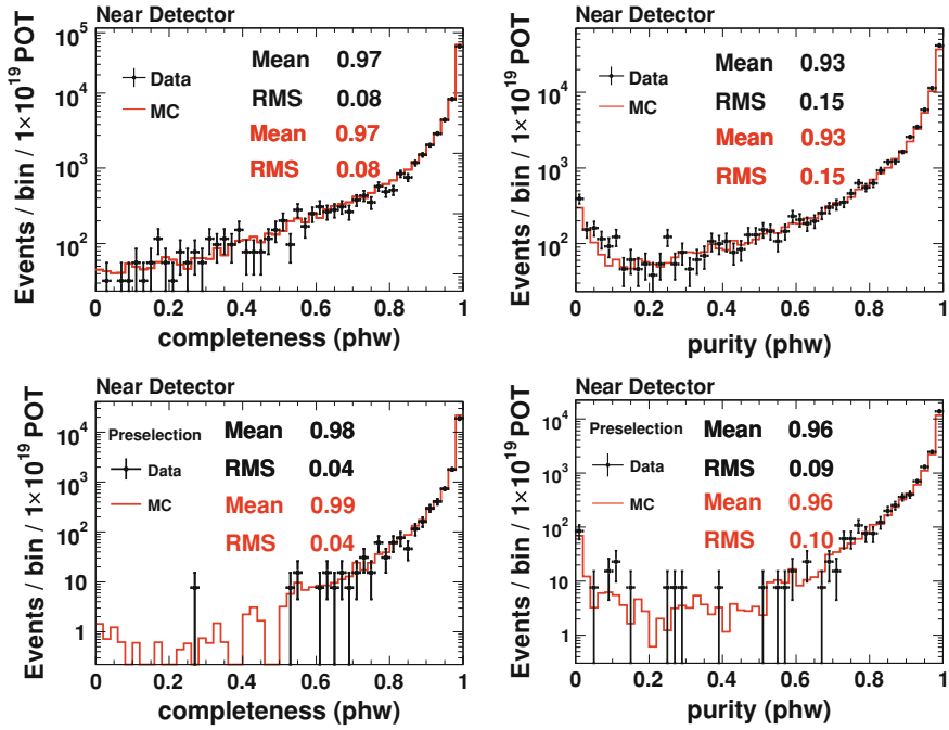
Fig. 6.16 Completeness and purity of MRCC events in the Near Detector, after fiducial cuts ( top row ) and after the preselection ( bottom row ). The MRCC quality cuts are applied. Most MRCC events have very high completeness and purity, especially those that pass the preselection, in which case completeness and purity are 98% and 96% respectively
