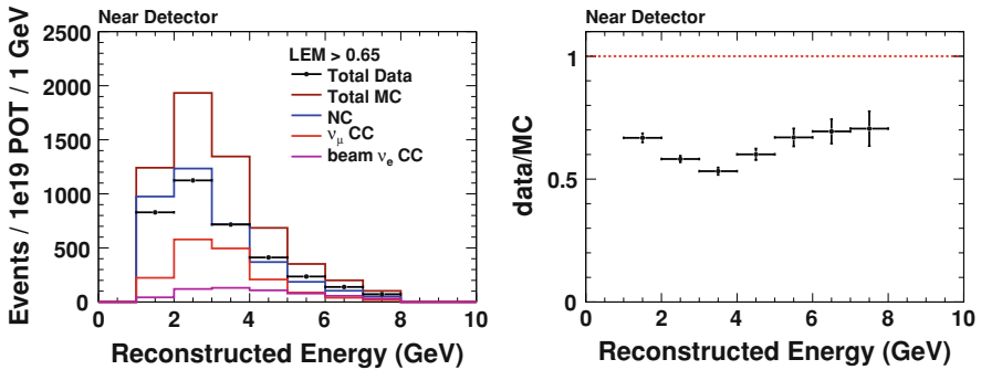
Fig. 5.21 Energy spectrum of Near Detector selected events for a cut at LEM pid > 0.65 ( left ) and the corresponding data to MC ratio ( right ). The integrated data to MC ratio is 60.2%
