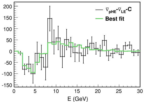
Fig. C.8 The histogram with statistical error bars is the difference in the measured normalized pHE and LE \bar{\nu}_\mu spectra in data corrected by the difference C \equiv Q_{HE} - Q_{LE} derived from simulation. The green solid line is the best fit result
