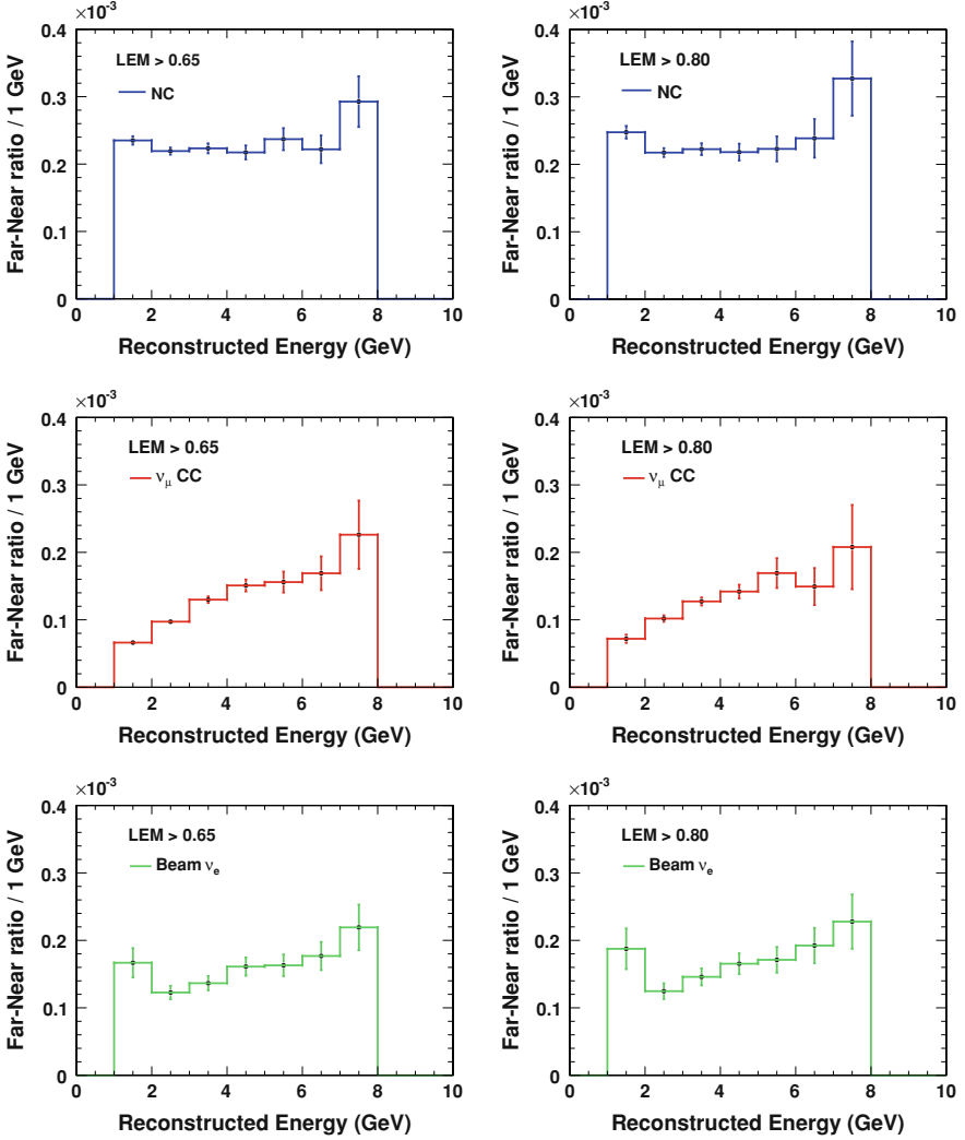
Fig. 7.5 Simulated Far-Near ratios from a LEM cut at 0.65 (left) and at 0.80 (right), for NC (top), \nu_\mu CC (middle) and beam \nu_e (bottom) events. Oscillations are included with standard oscillation parameters \Delta m_{32}^2 = 2.4 \times 10^{-3} \text{eV}^2 and \theta_{23} = \pi/4 . The error shown is statistical only. The ratios do not change when the cut value is tightened, but are significantly different depending on the event type considered
