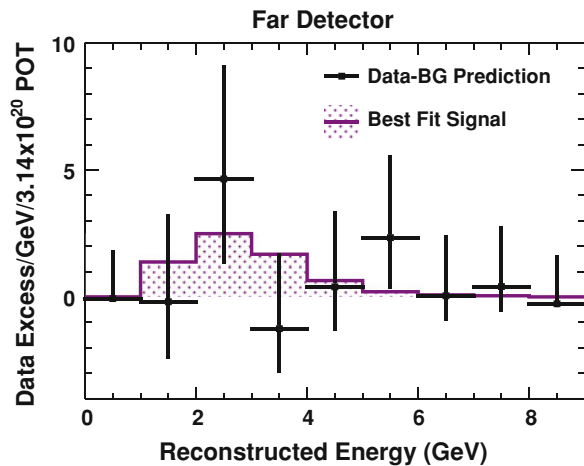
Fig. 9.21 Energy spectrum of the best fit signal, shown alongside the difference between the data and the background prediction
