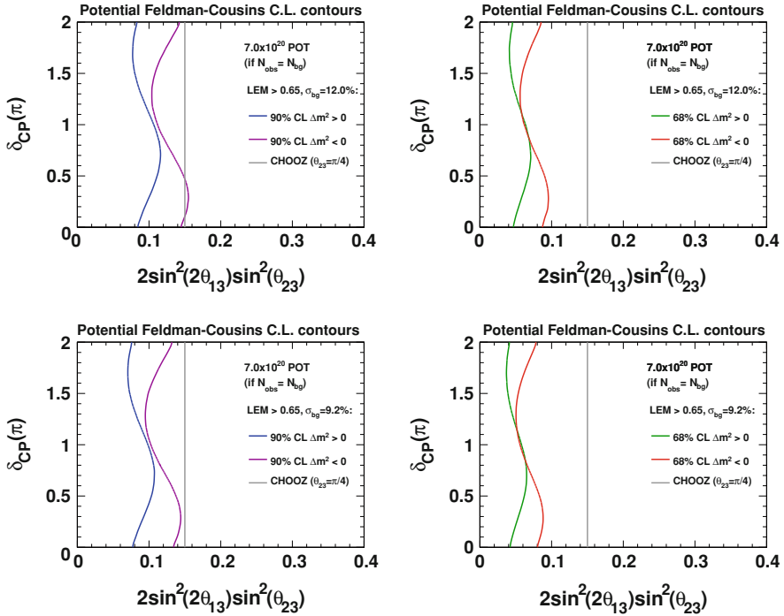
Fig. 10.2 Potential Feldman–Cousins 90% ( left ) and 68% ( right ) C.L. contours for an exposure of 7.0 \times 10^{20} POT and an observation of 48 events, which corresponds to the expected background. A total systematic error on the background prediction \sigma_{bg} of 12.0% ( top ) and of 9.2% ( bottom ) is assumed. The achieved sensitivity is better than CHOOZ (in the case of maximal mixing)
