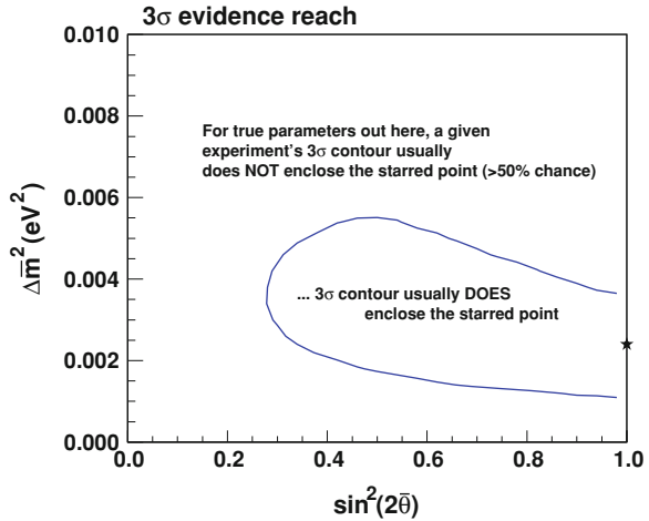
Fig. 10.17 3\sigma evidence reach for 1.0 \times 10^{20} POT of RHC running. The starred point denotes the CPT-conserving input value of \Delta\bar{m}_{32}^2 = 0.0024\text{eV}^2 and \sin^2(2\theta_{23}) = 1 . Image obtained from [25]
