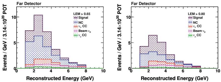
Fig. 7.14 Stacked energy spectra of the possible signal and the predicted background at the Far Detector, for the LEM selection with a cut value at 0.65 ( left ) and at 0.80 ( right ), using the HOO decomposition. The predictions are normalized for an exposure of 3.14 \times 10^{20} POTs. The signal corresponds to a value of \theta_{13} at the CHOOZ limit ( \sin^2(2\theta_{13}) = 0.15 ), ignoring CP violation and matter effects
