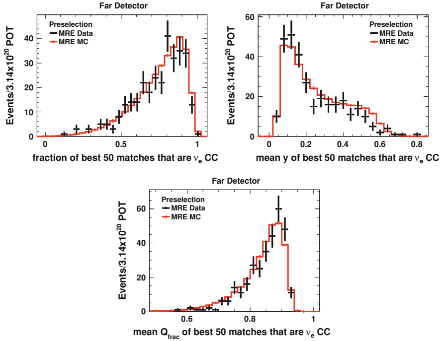
Fig. 9.4 The three variables that make up the LEM pid for events in the MRE sideband. As expected, events concentrate predominantly in the signal dominated regions, such as high f_{50} , low y_{50} and high q_{50} . The agreement between the data and the MC is very good in general
