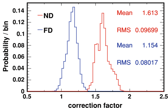
Fig. B.3 Probability distributions of the correction factor Q_{\text{final}}^{\text{total}}/Q_{\text{raw}}^{\text{total}} applied to \nu_e CC events in the fiducial region and with 1 \text{ GeV} < E_{\text{reco}} < 8 \text{ GeV} . The Q_{\text{final}} of each strip is given by Eq. B.6 for the Far Detector and by Eq. B.9 for the Near Detector, with \beta = 1.59 and R = 0.8 . The geometry of the Near Detector is responsible for the double peak structure in the corresponding distribution
