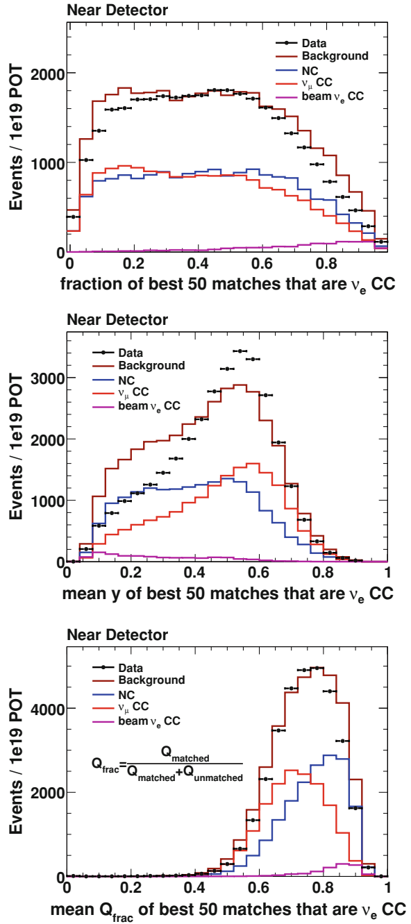
Fig. 5.16 The three variables that are combined into the LEM pid for all events passing the preselection, in the Near Detector. There is a large disagreement between the data and the MC mostly for the signal-like background
