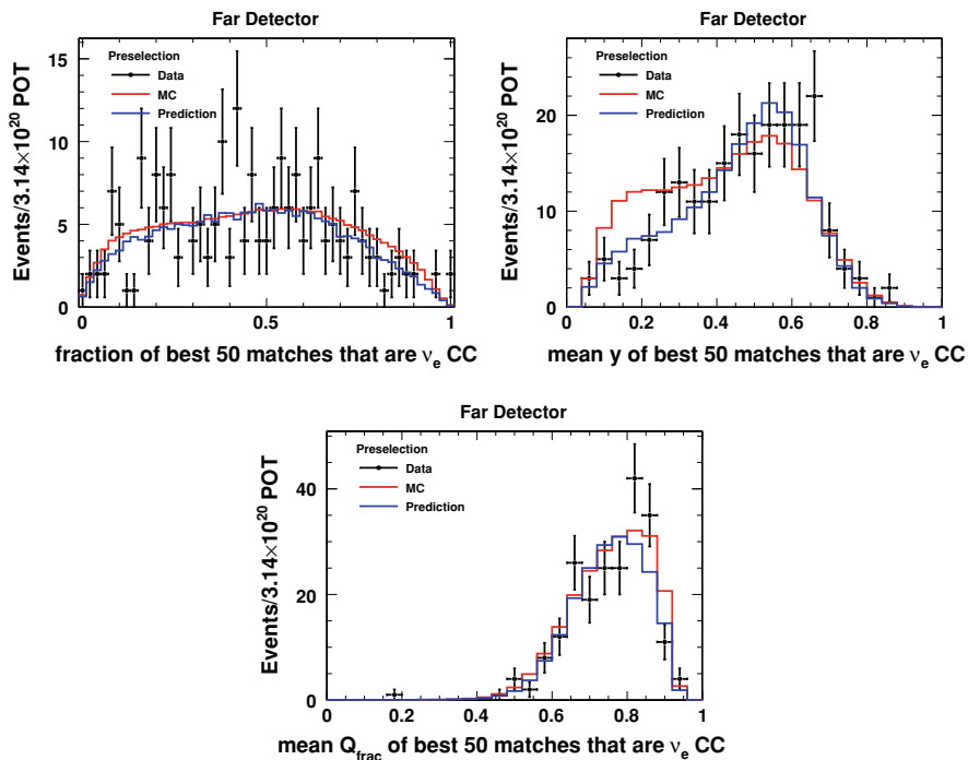
Fig. 9.18 The three variables that make up the LEM pid for preselected events in the Far Detector. The predictions are obtained by reweighing the Far MC expectation by the data to MC ratio observed in the Near Detector. The data distributions look as expected from the Near Detector
