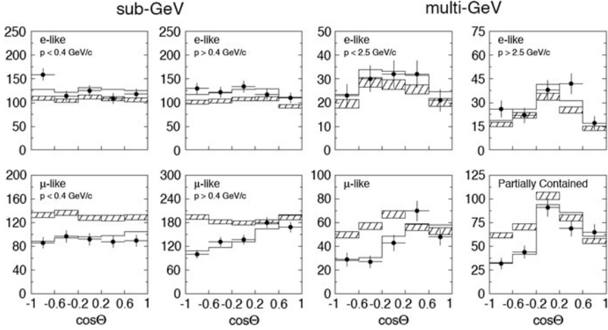
Fig. 2.4 Zenith angle distributions of \mu -like and e -like events in sub-GeV and multi-GeV data sets in Super-Kamiokande. The hatched region shows the MC expectation in the absence of oscillations. The bold line is the best fit under the \nu_\mu \rightarrow \nu_\tau oscillations hypothesis. Image obtained from [42]
