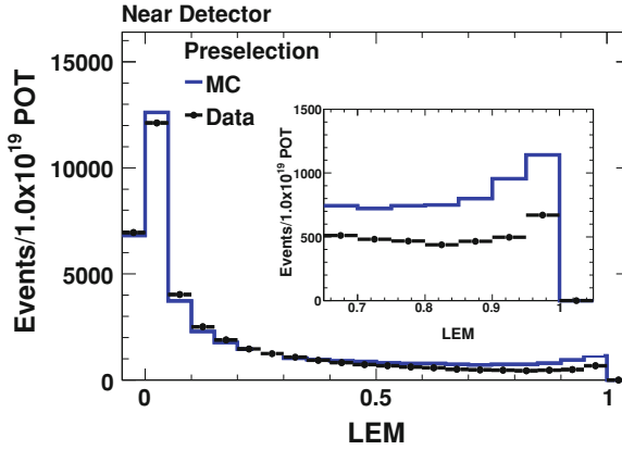
Fig. 6.1 LEM distribution of preselected events in the Near Detector. The plot contains the same data as Fig. 5.19 but in a different format. The simulation clearly overestimates the amount of signal-like background in the data by more than \sim 40\% in the high PID region. The events at LEM pid < 0 are the preselected events that do not get any matches in the LEM library
