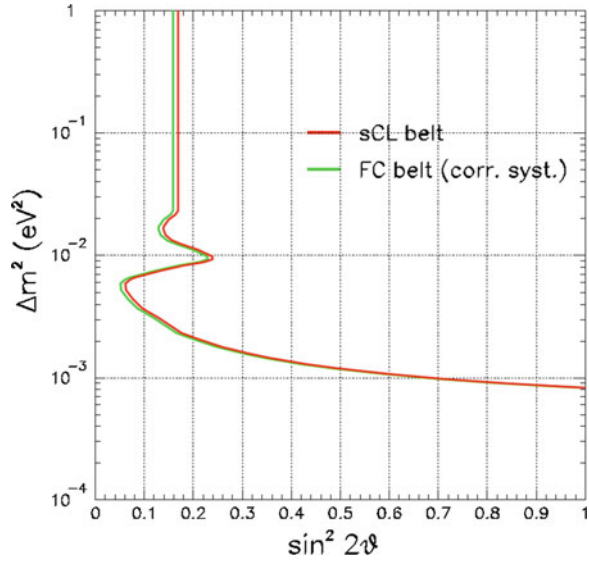
Fig. 2.12 Exclusion plot at 90% C.L. in the \sin^2 2\theta_{13} vs. \Delta m_{31}^2 plane obtained from the CHOOZ experiment. The standard C.L. and the Feldman–Cousins based C.L. contour are shown. Image obtained from [74]
