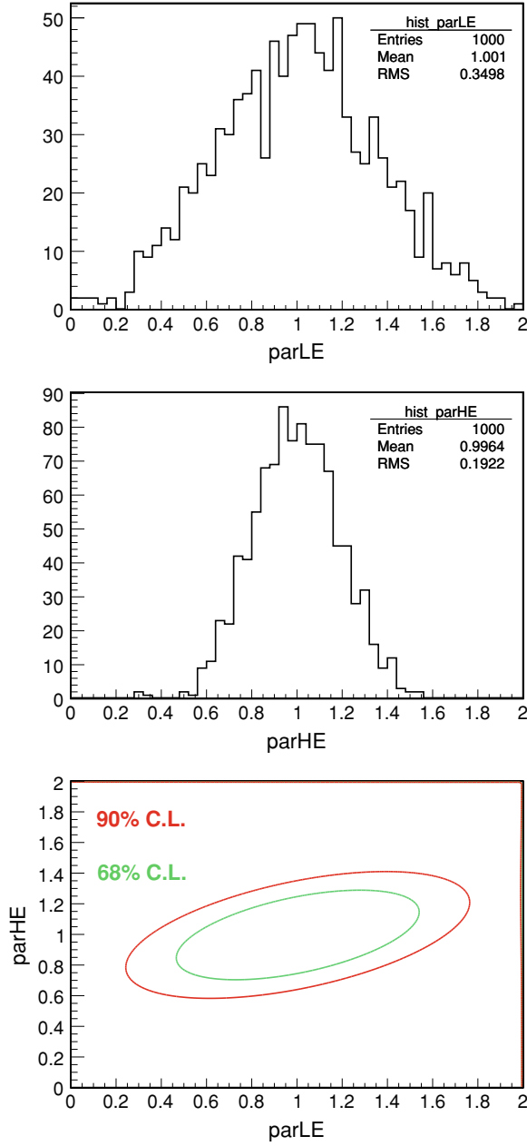
Fig. C.4 The results of 1000 simulated experiments using “fake” data for the parameters p_{\text{LE}} (upper) and p_{\text{HE}} (middle) given the data and MC statistics in Table C.1. The lower plot shows the expected correlation and accuracy of the measurement of p_{\text{LE}} and p_{\text{HE}}
