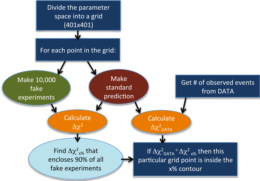
Fig. D.2 Schematic of our Feldman–Cousins implementation. The details of each step are given in the text
