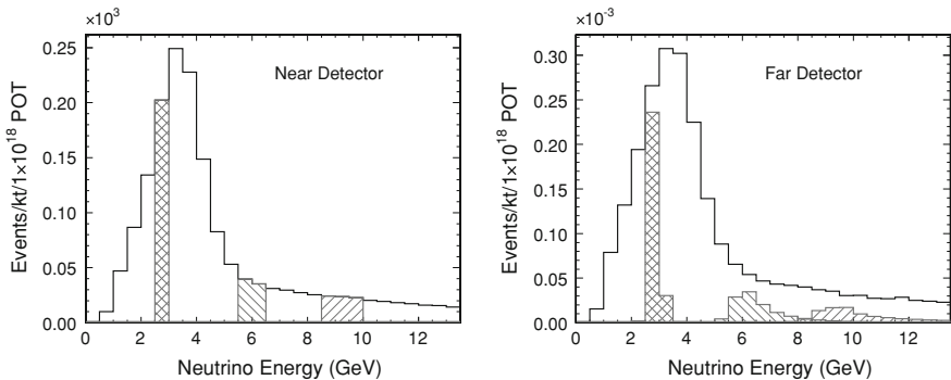
Fig. 7.3 The relationship between the energies observed in the Near Detector and those observed in the Far Detector for the \nu_\mu CC events selected in the analysis of [1]. The cross-hatched and hatched bands illustrate the fact that events with a particular energy in the near detector originate from decays that yield a range of energies in the Far Detector
