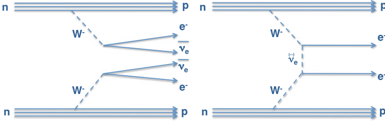
Fig. 2.9 Feynman diagrams for double beta decay ( left ) and neutrinoless double beta decay ( right ). Neutrinoless double beta decay can only occur if neutrinos are Majorana particles
