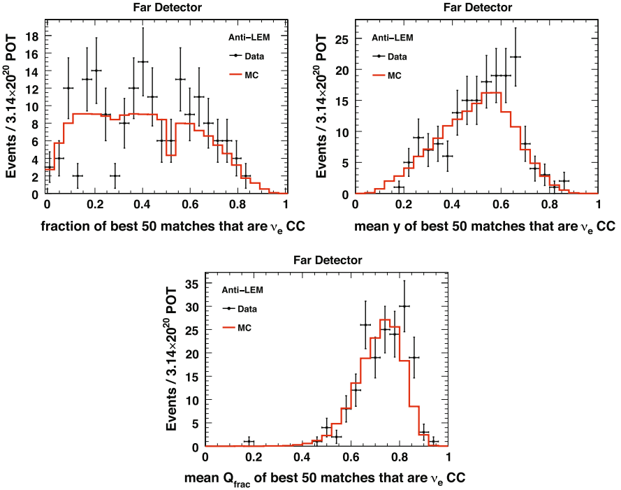
Fig. 9.2 The three variables that make up the LEM pid for events in the anti-LEM sideband. As expected, these events are mostly located in the background dominated regions, such as low f_{50} , high y_{50} and lower q_{50} . The predictions are calculated using the default MC, and are very close to those to what would be obtained with either of the decomposition methods given that the data-MC agreement is very good in the anti-LEM region
