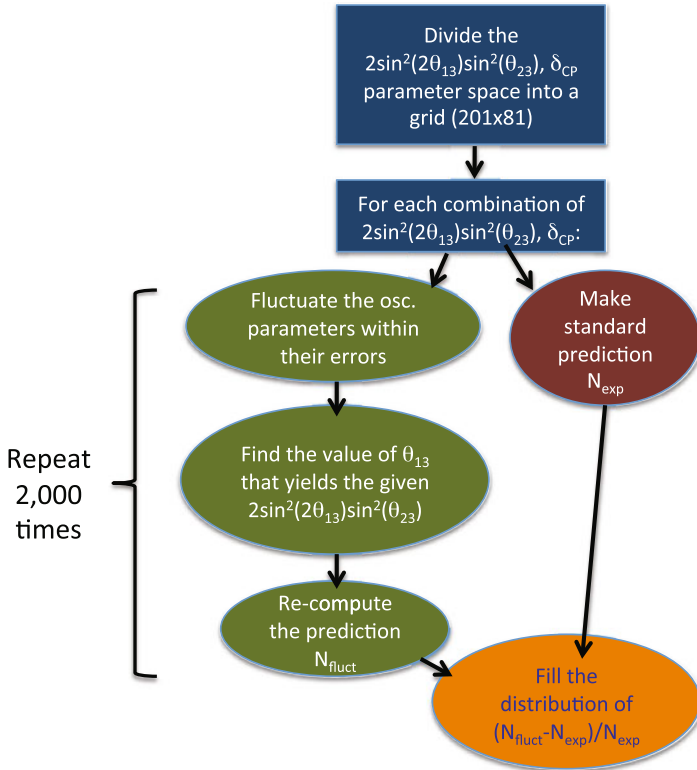
Fig. D.7 An illustration of the procedure followed in order to quantify the error due to the uncertainties in the oscillation parameters when the parameter space is divided in terms of 2\sin^2(2\theta_{13})\sin^2(\theta_{23}) vs. \delta_{CP}
