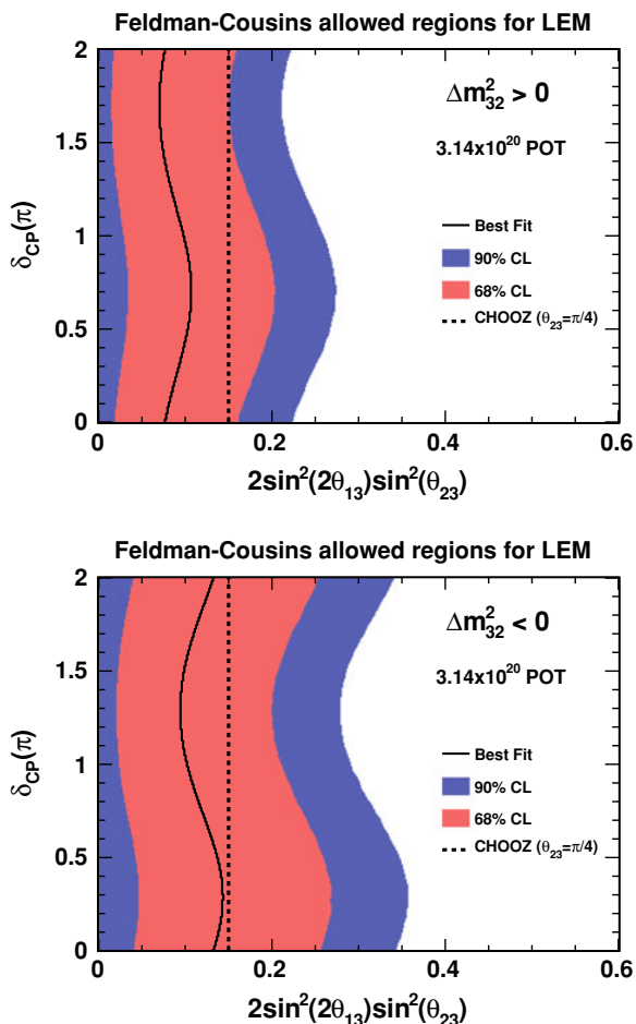
Fig. 9.24 Allowed regions and best fit results for the LEM > 0.65 selection with the HOO decomposition, for the normal hierarchy ( top ) and the inverted hierarchy ( bottom ). The best fit curves lie below the CHOOZ limit for both mass hierarchies. \theta_{13} = 0 is included at 90% C.L. but not at 68% C.L.
