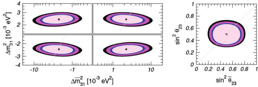
Fig. 10.10 90%, 95%, 99%, and 3\sigma C.L. allowed regions in the \Delta m_{31}^2 vs. \Delta m_{31}^2 parameter space (left) and in the \sin^2(\bar{\theta}_{23}) vs. \sin^2(\theta_{23}) parameter space (right), as obtained from a global fit done on all the existing neutrino data until 2008. The sign of the neutrino and antineutrino mass splittings are still unknown, which is why four different quadrants are considered in the left plot. The best fit point is indicated with a star, and the CPT conserving scenario with a line. The uncertainty in \Delta m_{32}^2 spans more than one order of magnitude at 99% C.L. The images are obtained from [20]
