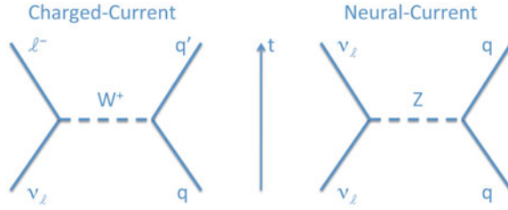
Fig. 2.2 Feynman diagrams of the charged-current and neutral-current neutrino interactions in MINOS. In the case of antineutrinos the sign of the W boson and of the outgoing lepton are reversed. Time flows in the upward direction, as indicated
