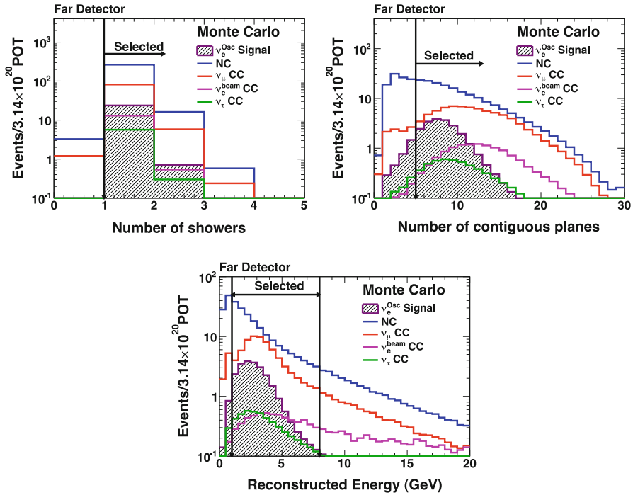
Fig. 5.3 Number of reconstructed showers per event, contiguous planes with at least 0.5 MIP deposition in each, and reconstructed energy spectra for different event types in the fiducial volume of the Far Detector. These plots were done after the track length cuts of Fig. 5.2 have been applied. The signal corresponds to a value of \theta_{13} at the CHOOZ limit, neglecting matter effects and CP violation
