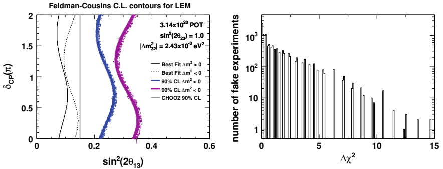
Fig. D.3 Feldman–Cousins 90% C.L. exclusion contours with the LEM > 0.65 selection for an observation of 28 events ( left ), and \Delta\chi^2 distribution of the 10,000 fake experiments for the \sin^2 2\theta_{13} = 0.15 , \delta_{CP} = 0 normal hierarchy grid point ( right ). The \Delta\chi^2 distribution is discrete due to the fact that only an integer number of events can be observed and that such observation is low statistics. Because of this the contours have a certain “thickness” to them. For the right plot, the values that enclose 68 and 90% of all fake experiments are 1.15 and 3.55 respectively
