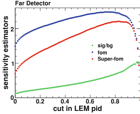
Fig. 5.20 Super-fom, fom and signal-to-background ratio as a function of the cut in LEM pid. All the quantities are data-based with PORP and are calculated using standard oscillation parameters, with \sin^2(2\theta_{13}) = 0.15 (at the CHOOZ limit), and assuming an exposure of 3.14 \times 10^{20} POTs. The cut at LEM pid = 0.80 yields the highest super-fom of 2.2
