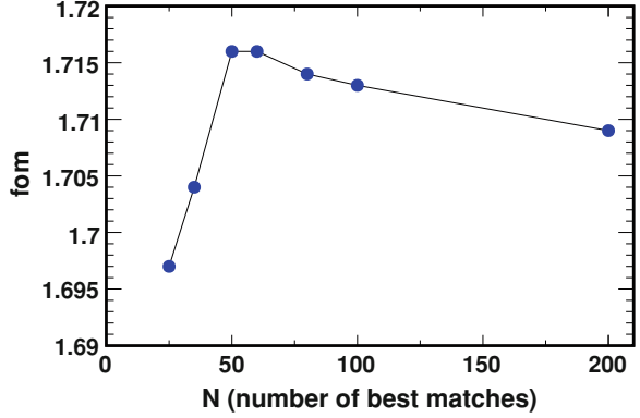
Fig. 5.12 Figure of merit (fom) as a function of the number of best matches N used to calculate \text{fracCC}(y < 0.5) and Q_{\text{frac}}^{\text{mean}} . The cut values for the two variables are optimized for each value of N based on the fom. A nonstandard preselection is used and standard oscillation parameters are assumed
