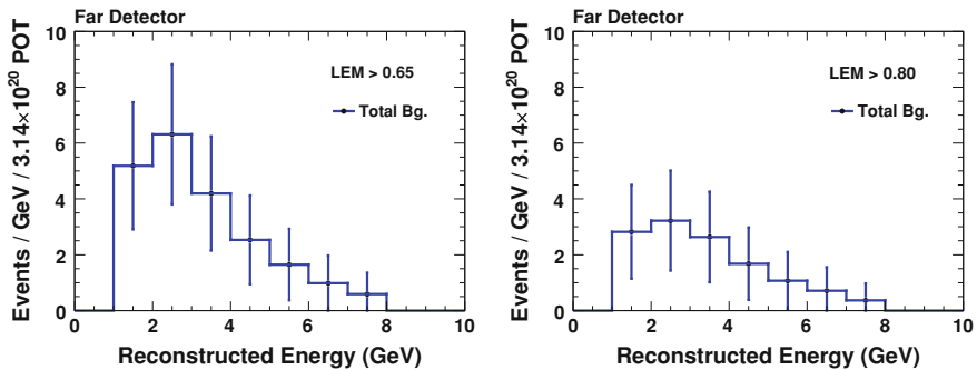
Fig. 7.15 Total background prediction for the LEM selection with a cut value at 0.65 ( left ) and at 0.80 ( right ), using the HOO decomposition. The statistical error at each bin assuming Gaussian statistics is shown
