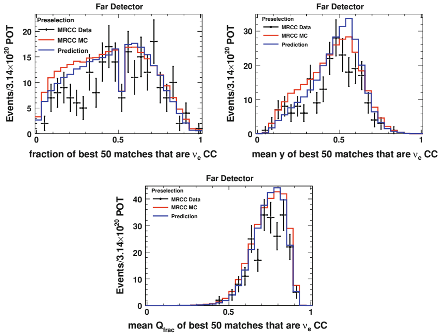
Fig. 9.7 The three variables that make up the LEM pid for events in the MRCC sideband. The data seems to agree better with the prediction than with the simulation, except perhaps in regions such as very low y_{50}
