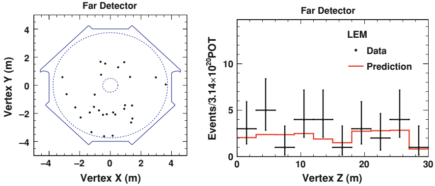
Fig. 9.16 Event vertices for the 28 events selected by the \text{LEM} > 0.65 selection. Selected events are spread all across the Far Detector
