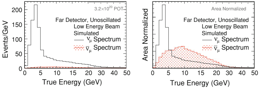
Fig. 10.6 Far Detector neutrino and antineutrino energy spectra, normalized to 3.2 \times 10^{20} POT (left) and to unity (right). Antineutrinos make up for approximately 6.4% of all NuMI interactions at the Far Detector, and have a higher average energy than neutrinos
