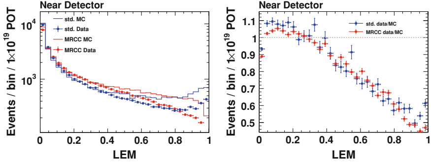
Fig. 6.17 LEM pid distribution in the standard and the MRCC samples ( left ), and the data/MC ratios for each sample ( right ). There are significant differences in the LEM distribution between the two samples (particularly in the high pid region), but the data-MC ratios are very similar
