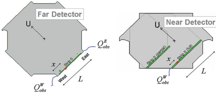
Fig. B.1 Schematics of the Far and Near Detectors. The strips are depicted in green and the clear fiber cables in blue . The location of a hit is symbolized by a red cross
