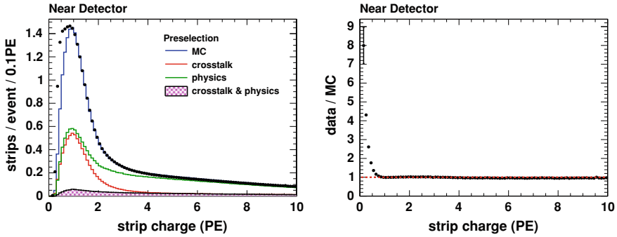
Fig. 8.1 Near Detector strip charge distribution in photoelectrons for events passing the preselection broken ( left ), and the corresponding data to MC ratio ( right ). The sum of the red, green and purple curves does not equal the blue one given that there are other types of hits not mentioned (for instance, hits leaking from other buckets). The data and the MC agree very well, except below \sim 1 PE where there is a very large excess in the data with respect to the simulation
