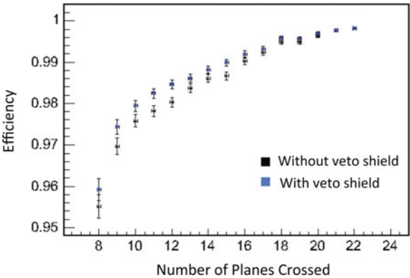
Fig. A.14 Efficiency to reconstruct cosmic ray muons as downward-going as a function of track length, with and without using the veto shield. The veto shield improves the ability to reduce the cosmic ray background when finding short upward-going muons
