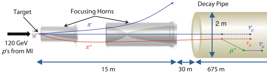
Fig. 10.5 Schematic of the NuMI beamline. Most antineutrinos are produced by those negatively charged mesons that go undeflected through the center of the horns. A small amount of antineutrinos originate from secondary \mu^+ decay
