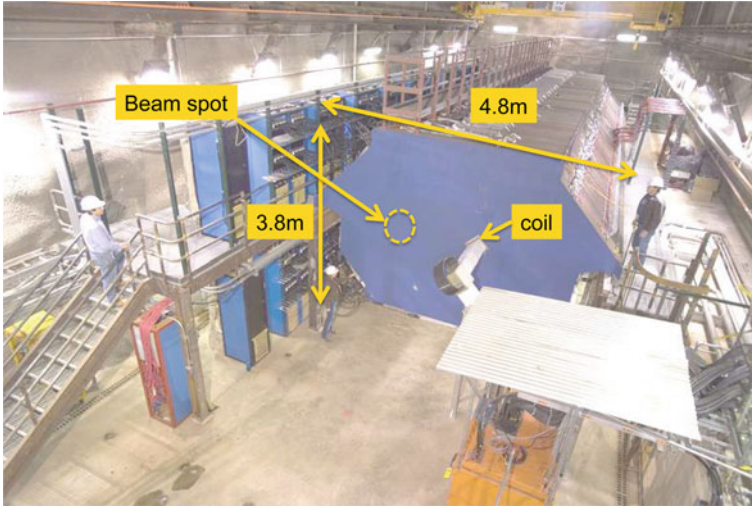
Fig. 3.11 The MINOS Near Detector. The coil hole is located approximately 1.5 m away from the beam center. The crates on the left house all the readout electronics. The detector is only read out from one end
