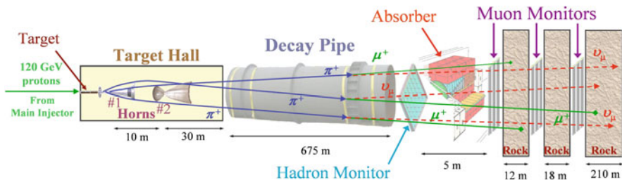
Fig. 3.2 Major components of the NuMI beamline. 120 GeV protons from Fermilab’s Main Injector impinge on a graphite target, producing a spray of secondary particles. The positively charged particles from the target are focused by two parabolic horns into a 675 m evacuated decay pipe, followed by a hadron absorber and 240 m of un-excavated rock
