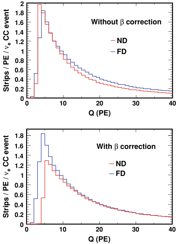
Fig. B.5 The distributions of the total (corrected) charge per strip of \nu_e CC events in the fiducial volume, normalized to number of events. Events satisfy 1 \text{ GeV} < E_{\text{reco}} < 8 \text{ GeV} and are stripped of hits with less than 3.0 photoelectrons before any corrections. The Far Detector charges are corrected according to Eq. B.6 in both cases. The Near Detector charges are corrected according to Eq. B.8 for the top plot and according to Eq. B.9 for the bottom plot . After all corrections have been applied there remains a deficit of low charge strips in the Near Detector with respect to the Far Detector. This is explained by the lower light level in the Near Detector combined with the fact that the same 3.0 PE cut is applied in both detectors. The agreement between the Near Detector and the Far Detector charge distributions is very good for strips with corrected charge above 10 photoelectrons
