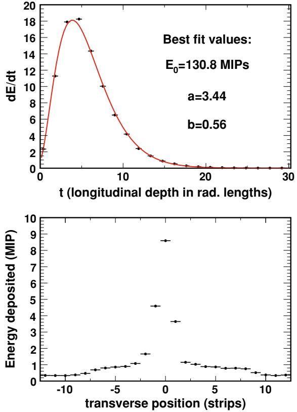
Fig. 4.5 Average longitudinal ( top ) and transverse ( bottom ) energy deposition profiles of 2 GeV electrons in CalDet. The energy is measured in Minimum Ionizing Particle (MIP) units, and t is the depth in radiation lengths. The binning corresponds to the physical dimensions of CalDet, that is one plane per bin (in the longitudinal direction) or one strip per bin (in the transverse direction). The longitudinal energy deposition profile fits very well to a gamma distribution
