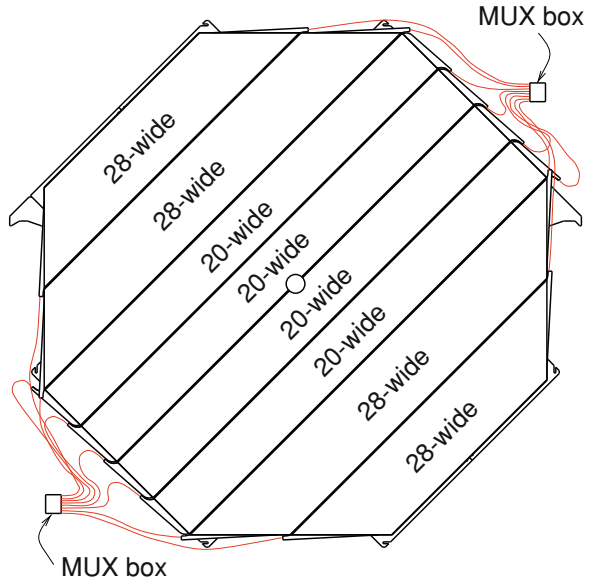
Fig. 3.7 Layout of U modules on a Far Detector plane. The V configuration is equivalent but rotated by 90^\circ . Eight fibers from different modules are directed into a single PMT pixel. Strips are read out from their two ends. The MUX boxes are the enclosures that contain the PMTs. Image obtained from [16]
