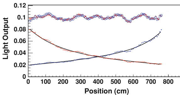
Fig. 3.17 Responses from each end of a typical strip in the Far Detector when illuminated along its length. The least squares fits to the sum of two exponentials are also shown in black . The vertical scale is approximately 1/100 the number of photoelectrons at the PMT for a cosmic ray muon passing normally through the module plane. The top series of data points shows the ratios of these data to their respective fits, normalized to 0.1 for display purposes. The small variations in the light output from a smooth exponential behavior are real and result from variations in scintillator, fiber depth and gluing. Image obtained from [16]
