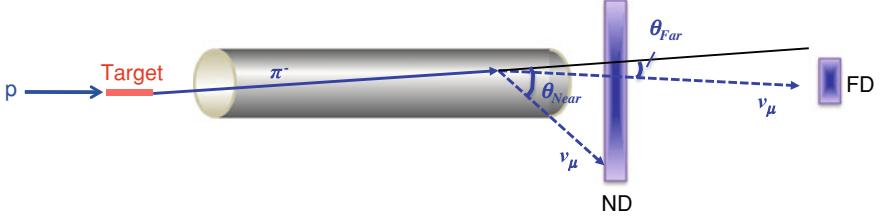
Fig. 7.2 Schematic of the NuMI beamline and the two detectors. Although the Far Detector is in reality larger than the Near Detector, here we display it with a smaller size in order to illustrate how, due to the widening of the beam as it travels, the two detectors subtend different solid angle regions. The Near Detector sees an extended neutrino source (the decay pipe), while the Far Detector essentially sees the source as a point. Also, when neutrinos are created at a finite distance from the beam axis the decay angles \theta_{Near} and \theta_{Far} required for the respective interception of the Near and Far detectors are different
