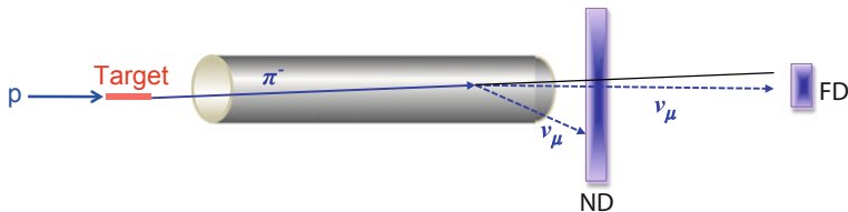
Fig. 4.12 Schematic of the NuMI beamline and the two detectors. Even if the Far Detector is approximately five times more massive than the Near Detector here it is displayed smaller in order to illustrate how, due to the widening of the beam as it travels, the two detectors cover different solid angle regions of it. Also, the Near Detector sees an extended line source (the decay pipe) while the Far Detector sees it as a point source for all practical purposes. Furthermore, the beam's composition changes as it travels due to oscillations, and the detectors have some intrinsic differences (mostly in their readout). All of these factors create a difference in event rates between the two detectors in the order of 10^4
