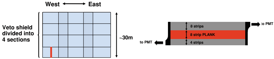
Fig. A.2 The ceiling part of the veto shield as viewed from above ( left ), and one of the 20 strip modules used in the veto shield ( right ). The veto shield planks are groups of eight or four scintillator strips that are read out by the same PMT pixel. One of the eight strip plank is shown in red in both plots
