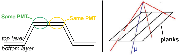
Fig. A.9 An illustration of the two additional considerations that need to be considered when performing the veto shield timing calibration. Some tracks can hit two planks connected to the same PMT, thus making the timing of only one of the hits valid ( left ). Other particles typically come in with the muon and thus affect the timing ( right )
