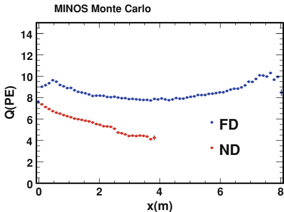
Fig. 5.7 The average total charge per strip Q deposited by muons as a function of the distance from the west end x , as read from the PMTs. For the Far Detector, Q is the sum of the charge from both strip ends. For the Near Detector, light is read out from the west end only. The longest Far Detector strips are 8 m long, whereas the longest Near Detector strips are 4 m long. In the Far Detector the charge is approximately 15% lower if the interaction occurs in the center of the strip than if it occurs near one of the edges. Due to the single ended readout, the Near Detector charge is highest near the west end and diminishes by \sim 50\% if the interaction occurs near the east end. Overall, the charge (or, as we shall refer to in this document, the “light level”) is higher in the Far Detector than in the Near Detector
