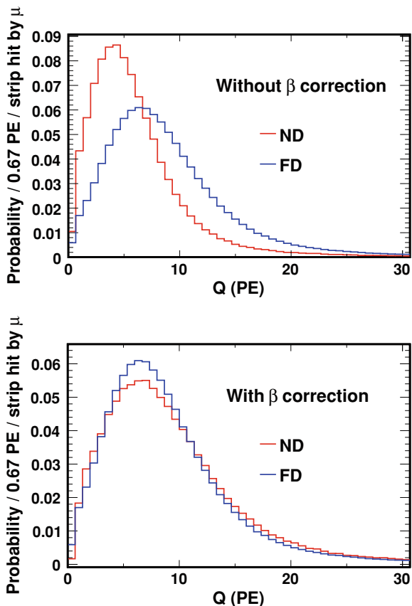
Fig. B.4 The probability distributions of the total (corrected) charge deposited per strip by muons with a track vertex in the fiducial volume. Strips with zero charge are ignored. The Far Detector charges are corrected according to Eq. B.6 in both cases. The Near Detector charges are corrected according to Eq. B.8 in the top plot and according to Eq. B.9 in the bottom plot . The shapes of the Near Detector and Far Detector charge distributions agree well after the \beta correction has been applied
