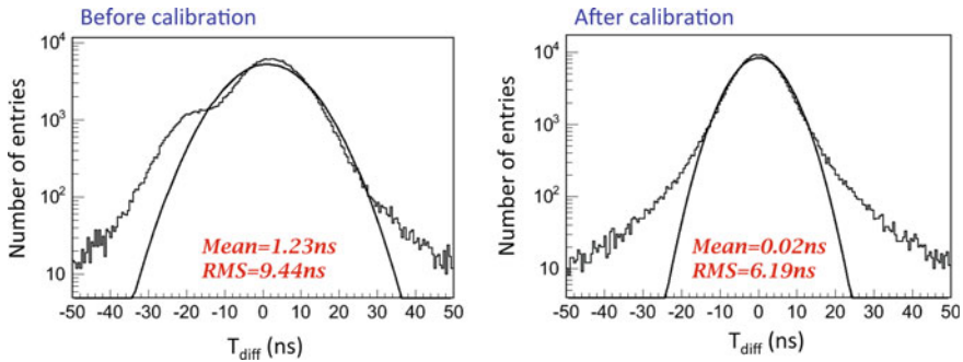
Fig. A.12 North-south time difference distribution for all channels before and after calibration. The single-hit timing resolution is 6.19/\sqrt{2} = 4.4 ns after the calibration
