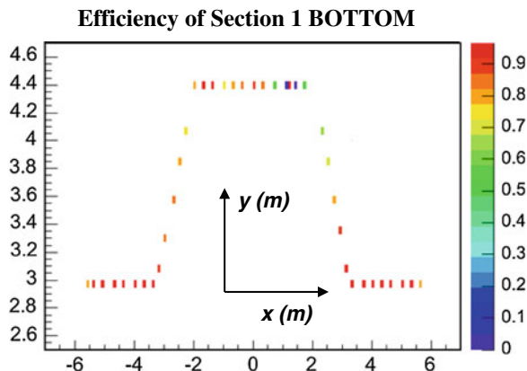
Fig. A.5 Plank efficiencies of the bottom ceiling layer of Sect. A.1. Most planks have efficiencies higher than 85%, except for a group of five contiguous planks in the top-right corner
