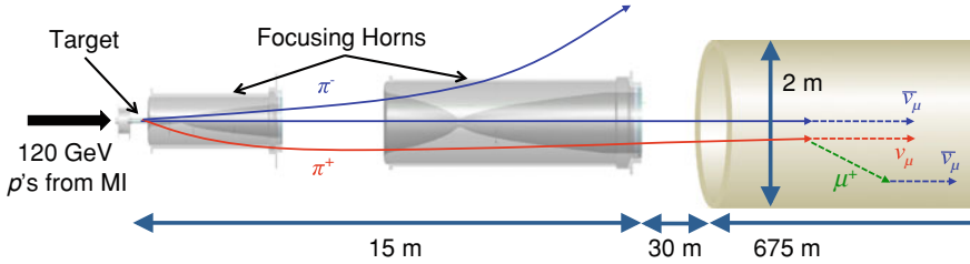
Fig. C.2 Schematic of the NuMI beamline. The antineutrinos from hadron parents \bar{\nu}_\mu(\pi, K) are produced by those negatively charged mesons that go undeflected through the center of the horns. A small amount of antineutrinos originate from \mu^+ decay, and the energy spectrum of those is strongly dependent on the separation between the target and the horns
