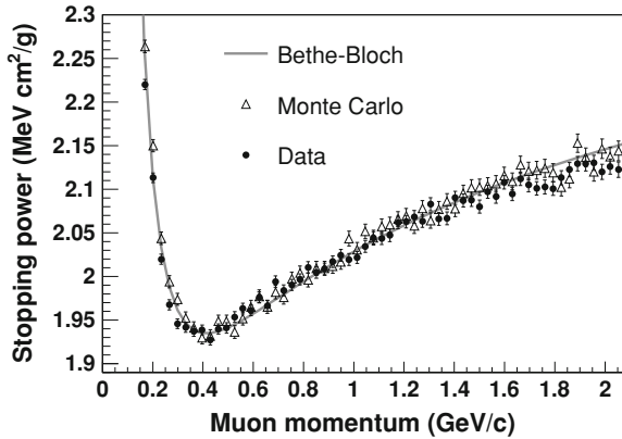
Fig. 3.18 Stopping power of muons as a function of their momentum. The prediction by the Bethe-Bloch equation in polystyrene scintillator agrees very well with the MINOS Far Detector data and the MINOS MC simulation. Both data and MC points have been normalized to the Bethe-Bloch calculation to give the expected stopping power at the minimum ionizing point. Image obtained from [16]
