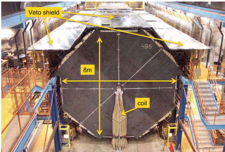
Fig. 3.8 The MINOS Far Detector viewed from the front. The cosmic ray veto shield is visible on the top and on the sides of the detector
