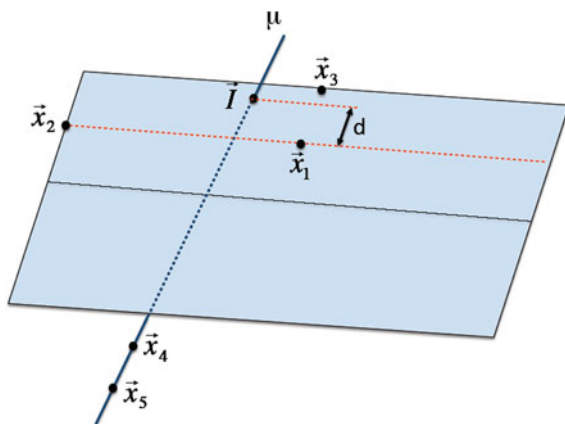
Fig. A.4 Intersection of a muon with a plank in the veto shield
