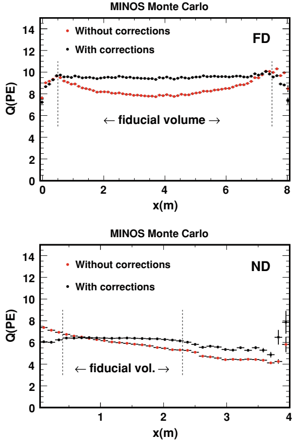
Fig. B.2 The average total charge per strip Q deposited by muons as a function of the distance from the west end x , as read from the PMTs ( red ), and after being corrected ( black ) by Eqs. B.6 and B.8 for the Far Detector and Near Detector cases respectively. Strips with zero charge are ignored. The corrected charge is to first-order flat as a function of x which indicates that the attenuation effects are well accounted for. The dashed lines delineate approximately the region within the fiducial volume. The drop in the corrected Near Detector charge curve occurs in regions outside the fiducial volume ( x \lesssim 0.4 m and x \gtrsim 2.3 m), and is mostly due to strip edge effects (the same can be said for the Far Detector). The average corrected charge is lower in the Near Detector than in the Far Detector, where it is adjusted by the \beta factor included in Eq. B.9
