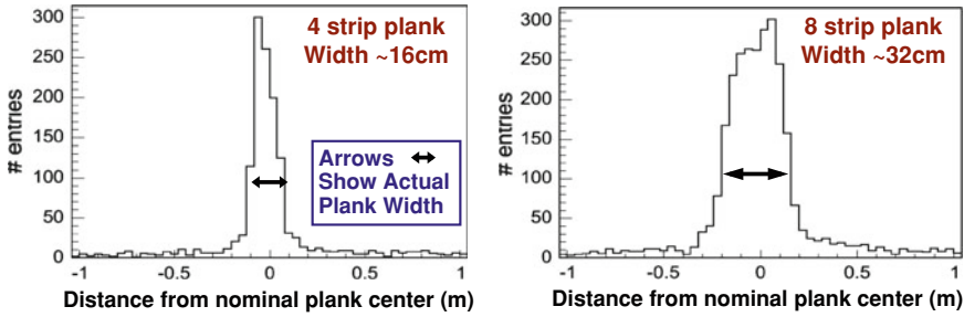
Fig. A.6 Distance from the nominal center of plank x for the interception of cosmic ray tracks with plank x . These distributions are filled every time plank x is hit. Through this technique the planks can be “seen” and the information about the plank’s position in the database can be corrected
