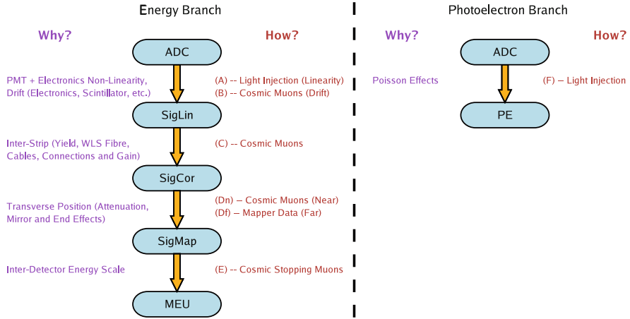
Fig. 3.16 Calibration chains for the MINOS data. The raw energy depositions come in the form of digitized values from the ADCs. Before they can be expressed in terms of an inter-detector energy scale they must be corrected for drift, non-linearity, inter-strip differences and transverse position. SigLin, SigCor and SigMap are the names given in MINOS to the quantities obtained after these corrections have been applied. A conversion to photoelectrons (PEs) is also done by applying the average response per channel to the observed ADC values. Image obtained from [35]
