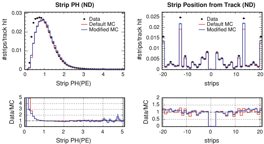
Fig. 8.2 Near Detector strip charge distribution of crosstalk hits around tracks ( left ), and distribution of transverse strip position from track center ( right ). The corresponding ratios of data to MC are shown in the bottom . The modified (retuned) crosstalk simulation improves the data to MC agreement, particularly for the strip position distribution. Images obtained from [8]
