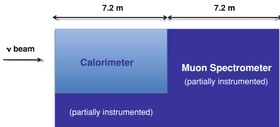
Fig. 3.10 Schematic of the different sections of the Near Detector, as viewed from above. Throughout the entire detector, one of every five planes is fully instrumented. For the first 120 planes the other four are also partially instrumented. Thus the upstream section of the detector is the calorimeter, where every plane is instrumented. In the muon spectrometer only one out of every five planes is instrumented
