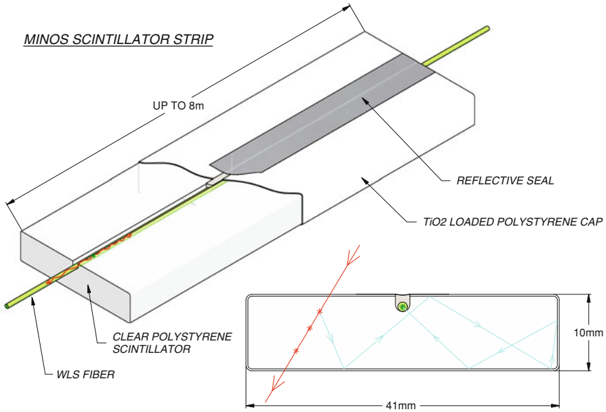
Fig. 3.6 Cutaway drawing of a single scintillator strip. Light produced by an ionizing particle is multiply reflected inside the strip until absorbed by the WLS fiber, at which point it is wavelength shifted and reemitted isotropically. The resulting wave shifted photons whose directions fall within the total internal reflection cones are transported along the fiber to the edges of the detector, subsequently being routed to the photodetectors. Image obtained from [16]
