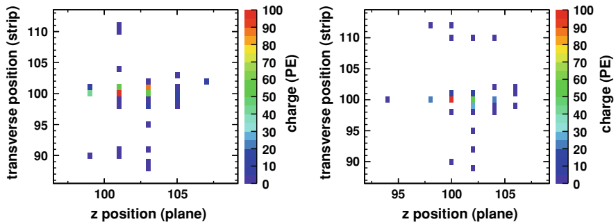
Fig. 9.14 A \nu_e CC candidate in the Far Detector data (run 37980, snarl 225613) as seen in the U (left) and V (right) views. This particular event has a LEM pid value higher than 0.99. It consists of what looks like a tight electromagnetic core surrounded by crosstalk activity
