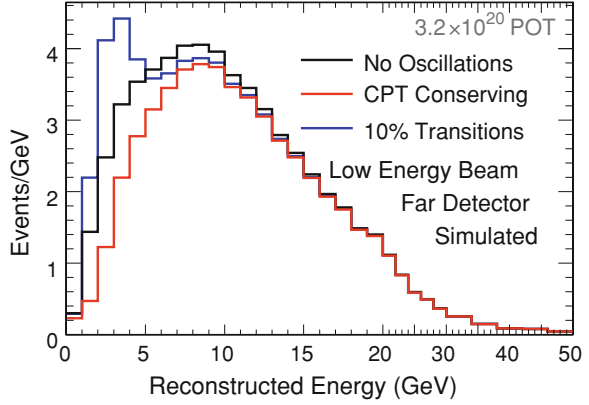
Fig. 10.9 Antineutrino simulated energy spectra for no oscillations, CPT conserving oscillations and CPT conserving oscillations with \alpha = 0.1 transitions. If neutrinos transition to antineutrinos an excess of low energy antineutrinos is expected to appear at low energies
