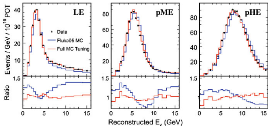
Fig. 3.13 Near Detector spectra of \nu_\mu CC events in the data compared to the predictions from the original simulation and from the tuned simulation, in the low-energy (LE), pseudo-medium energy (pME) and pseudo-high energy (pHE) beam configurations. The corresponding data to MC ratios are shown in the bottom panels, before and after tuning. In all cases the tuned simulation agrees very well with the data
