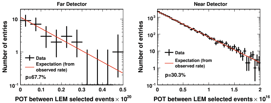
Fig. 9.17 Distributions of POT elapsed between LEM selected events in the Far ( left ) and Near ( right ) detectors. The expectations are calculated from the observed rates as described in [12] and are shown in red. In each case, a \chi^2 is calculated with respect to the expectation. The probability of getting a \chi^2 that is worse than the obtained is determined based on 2,500 pseudo-experiments and indicated on the lower-left corner
