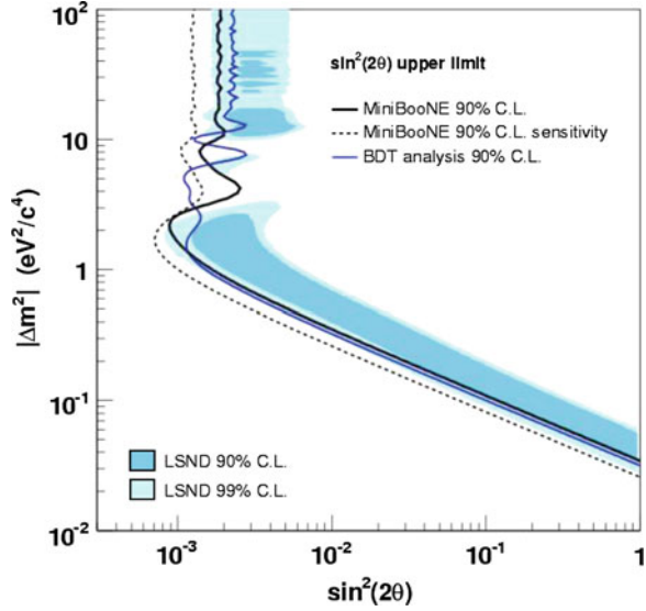
Fig. 2.11 Sensitivity (dashed black line) and limit (solid black line) for MiniBooNE events with 475 < E_\nu < 3000 MeV within a two neutrino oscillation model. Also shown is the limit from the boosted decision tree analysis (thin solid curve) for events with 300 < E_\nu < 3000 MeV. The MiniBooNE limits mostly exclude the allowed regions derived from the results of the LSND experiment. Image obtained from [67]
