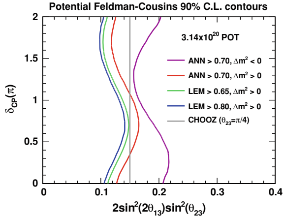
Fig. 8.8 Potential Feldman–Cousins 90% C.L. exclusion contours for the ANN, LEM > 0.65 and LEM > 0.80 selections, for an observation of 26, 21 and 12 events respectively. For LEM only the normal hierarchy contours are shown. LEM > 0.80 is the most sensitive selection, being approximately 15–20% more sensitive than ANN
