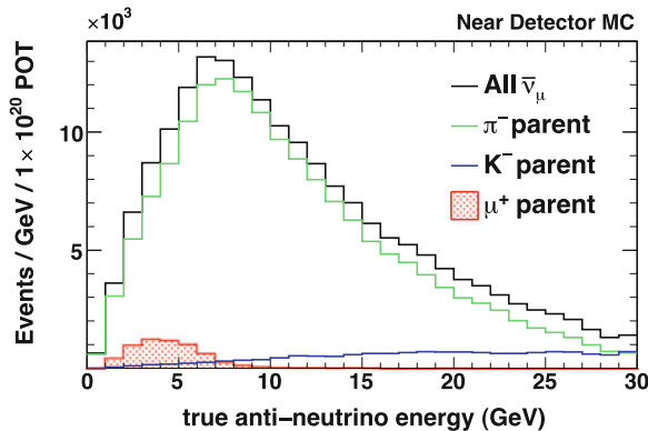
Fig. 6.8 True energy spectrum of antineutrinos in the Near Detector fiducial volume, broken down by antineutrino parent. A very small amount of antineutrinos originates from K_L decay and is not shown here. Most antineutrinos originate from \pi^- decay and, at high energies, from K^- decay. A small amount originates from secondary \mu^+ decay in the beam pipe, as described by Eq. 6.2
