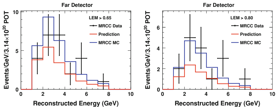
Fig. 9.5 The energy spectra of selected Far Detector LEM selected MRCC events, for a cut value of 0.65 ( left ) and of 0.80 ( right ). The data is shown alongside the prediction obtained from extrapolation from the Near Detector and the default simulation's prediction. These last two differ by almost a factor of two, particularly for the tighter cut at 0.80. In both cases there is an excess of events in the data with respect to the prediction
