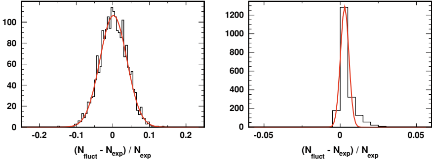
Fig. D.9 The fractional variation distributions of the total number of expected events with LEM > 0.65 , at 2 \sin^2(2\theta_{13}) \sin^2(\theta_{23}) = 0.3 , \delta_{CP} = 0.97\pi and at 2 \sin^2(2\theta_{13}) \sin^2(\theta_{23}) = 0.012 , \delta_{CP} = 0.97\pi (right). Most distributions fit well to a Gaussian, although some distributions near the physical boundary of 2 \sin^2(2\theta_{13}) \sin^2(\theta_{23}) = 0 do not
