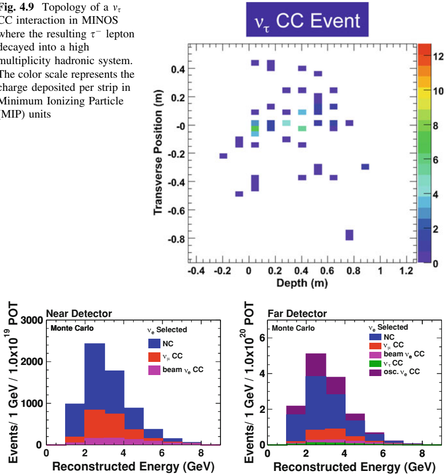
Fig. 4.10 Reconstructed energy spectra for selected events in the Near Detector ( left ) and in the Far Detector ( right ), for one particular \nu_e selection algorithm. The spectra were obtained ignoring matter effects and CP violation effects, and assuming \sin^2(2\theta_{13}) = 0.15 (at the CHOOZ limit), with standard oscillation parameters \Delta m_{32}^2 = 2.38 \times 10^{-3} \text{ eV}^2 and \theta_{23} = \pi/4 . In this particular example it can be seen how the relative amount of \nu_\mu CC background diminishes almost by \sim 40\% when going from the Near Detector to the Far Detector, due to oscillations
