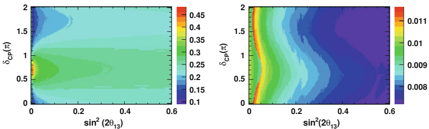
Fig. D.6 Fractional error due to the uncertainties in the oscillation parameters on the number of signal ( left ) and background ( right ) events, as a function of \sin^2(2\theta_{13}) and \delta_{\text{CP}} . The errors correspond to the RMS of the (N_{\text{fluct}} - N_{\text{exp}})/N_{\text{exp}} distributions, with the \text{LEM} > 0.65 selection and in the case of the normal hierarchy. The error is negligible for the background, but quite important for the signal. The same conclusions apply in the case of the inverted mass hierarchy
