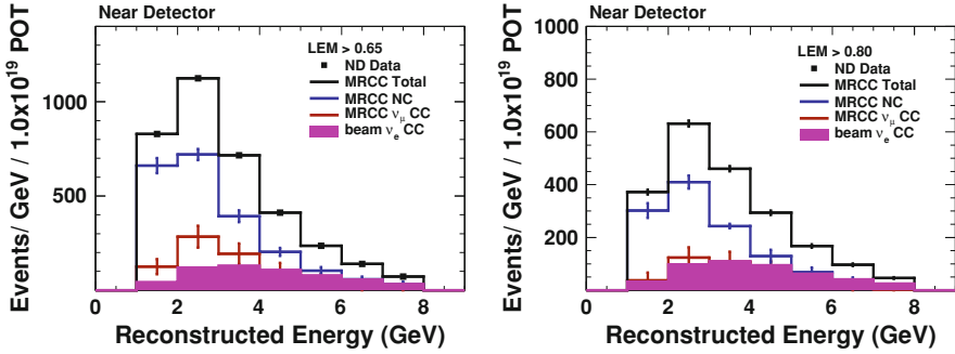
Fig. 6.20 Energy spectra of LEM selected events decomposed by MRCC with a cut at 0.65 ( left ) and at 0.80 ( right )
