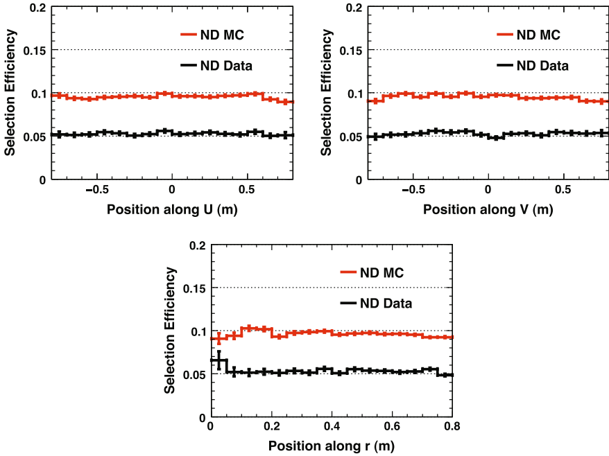
Fig. B.7 Selection efficiencies of background events in the Near Detector as a function of position in the detector. U and V are the mutually orthogonal directions along the scintillator strips, and r is the distance to the beam's center. The efficiencies are calculated with respect to the number of preselected events. There is a large discrepancy between the data and the MC which is addressed in Sect. 6.1
