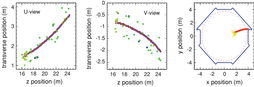
Fig. 10.7 Far Detector data \bar{\nu}_\mu CC Candidate (Run 36770, Snarl 204002), as viewed from the U-direction ( left ), from the V-direction ( middle ) and from the front of the detector ( right ). The track clearly bends towards the outside of the detector. The low pulse height hits (in green ) surrounding the track are due to crosstalk or bremsstrahlung
