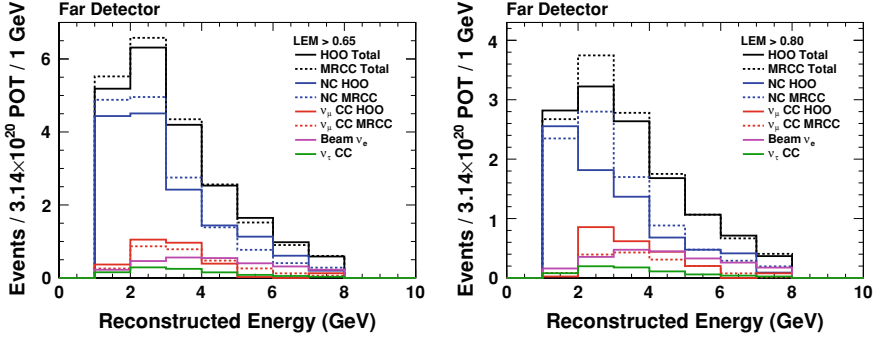
Fig. 7.7 Predicted Far Detector background spectra with the HOO and MRCC methods, for a LEM cut at 0.65 ( left ) and at 0.80 ( right ). Predictions are scaled to 3.14 \times 10^{20} POT
