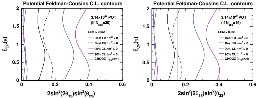
Fig. 8.9 Potential Feldman–Cousins 90% C.L. exclusion contours for the LEM > 0.65 ( left ) and LEM > 0.80 ( right ) selections, for an observation of 30 and 19 events respectively. If the number of observed events is equal to or higher than the values used here then \theta_{13} = 0 will be excluded at 90% C.L.
