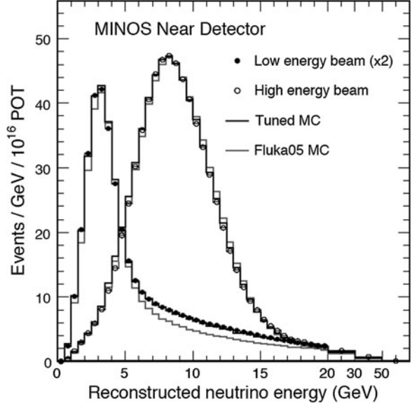
Fig. 7.6 Energy spectra in the Near Detector for \nu_\mu CC-like events in the low-energy (LE) and high-energy (HE) beam configurations, as obtained from [5]. The tuned simulation (which is the one used throughout the \nu_e analysis) agrees very well with the data
