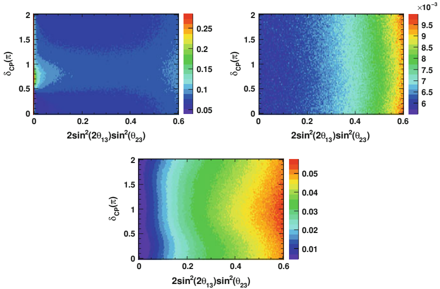
Fig. D.8 fractional error due to the uncertainties in the oscillation parameters on the number of signal ( left ), background ( right ) and total ( bottom ) events, as a function of 2 \sin^2(2\theta_{13}) \sin^2(\theta_{23}) and \delta_{CP} . The errors correspond to the RMS of the (N_{\text{fluct}} - N_{\text{exp}})/N_{\text{exp}} distributions, with the LEM > 0.65 selection and in the case of the normal hierarchy. The error in the total number of expected events is less than 5%. The same conclusion applies in the case of the inverted mass hierarchy
