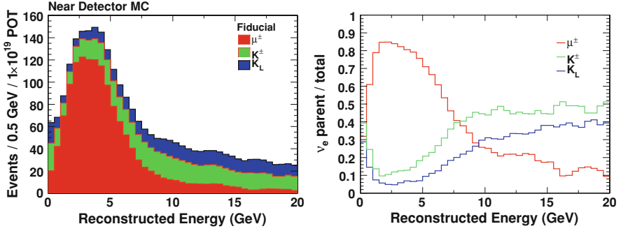
Fig. 6.7 Simulated energy spectra of beam \nu_e 's (and \bar{\nu}_e 's) that interact inside the fiducial volume, broken down by parent type ( left ) and the corresponding proportions of each parent as a function of energy ( right ). Below 8 GeV, approximately 71% of beam \nu_e 's originate from muon decay.
