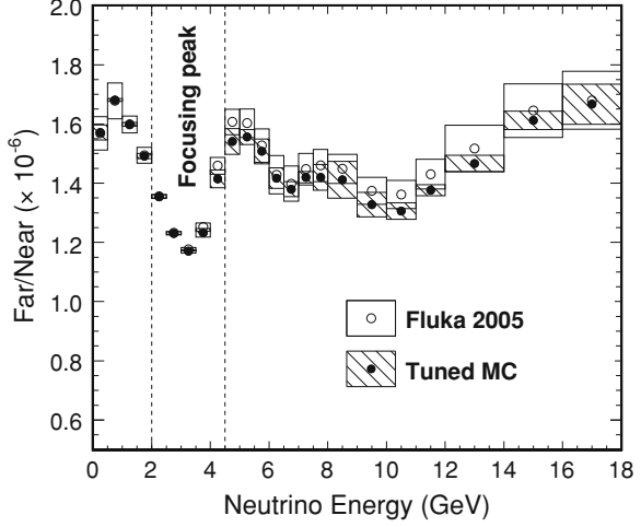
Fig. 7.1 \nu_\mu CC flux ratio between the Far and Near detectors in the absence of oscillations, from [1]. The ratio is shown before and after the beam fit described in Sect. 3.4.2. The fact that the ratio is not strongly affected by the beam fitting shows that the uncertainty in the flux difference between the two detectors is small.
