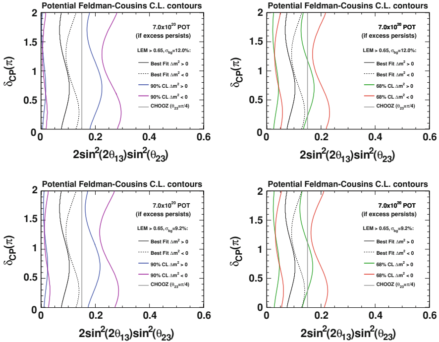
Fig. 10.1 Potential Feldman–Cousins 90% (left) and 68% (right) C.L. contours for an exposure of 7.0 \times 10^{20} POT and an observation of 62 events. A total systematic error on the background prediction \sigma_{bg} of 12.0% (top) and of 9.2% (bottom) is assumed. The contours exclude \theta_{13} = 0 at 90% C.L.
