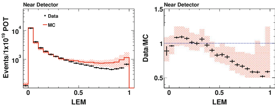
Fig. 6.3 LEM pid of events passing the preselection in the Near Detector ( left ), and the corresponding data to MC ratio ( right ). The orange band represents the systematic error due to uncertainties in the beam flux, the hadronic model and the cross-sections. The data-MC discrepancy is practically covered by these three sources of systematic error to less than 1.5\sigma . Also, the systematic error gets proportionately larger with increasing PID
