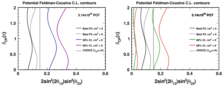
Fig. 9.23 Feldman-Cousins 90% ( left ) and 68% ( right ) C.L. contours for LEM, with the MRCC decomposition, for the observation of 28 events
