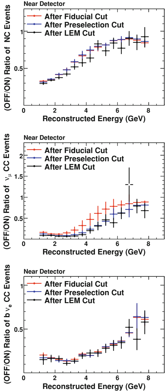
Fig. 6.12 r_{\text{NC}} (top), r_{\text{CC}} (middle) and r_e (bottom), for true NC, \nu_\mu CC and beam \nu_e events respectively. The ratios are obtained from the MC after the application of different cuts. The LEM cut value used to make these plots is 0.65. The ratios shown here at the fiducial level are very similar but not exactly the same as the ones from Fig. 6.10, given that the \nu_\mu CC-like and NC-like samples do not correspond exactly to the true NC and true \nu_\mu CC samples used here. With the exception of r_{\text{CC}} , the ratios do not change very significantly after the application of the different cuts
