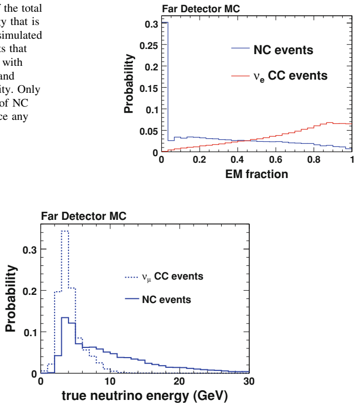
Fig. 4.8 True energy of the simulated \nu_\mu CC and NC events that comprise the background to the search for \nu_e appearance in MINOS, normalized to unity. Events are required to be small showers with a reconstructed energy between 1 and 8 GeV. For CC events we can measure the incoming neutrino energy but not for NC events, and consequently approximately half of the NC events in our background sample originate from the high energy tail ( E_{\text{true}} \gtrsim 7 GeV)
