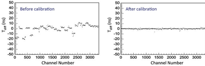
Fig. A.11 North-south time difference average as a function of channel number. The propagation delay corrections of Eq. A.8 are included in both plots. The right plot includes the T_0 offsets as determined from the calibration
