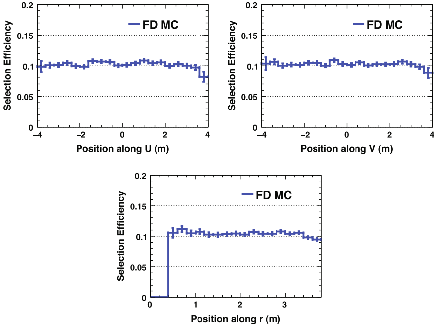
Fig. B.6 Selection efficiencies of background events in the Far Detector as a function of position in the detector. U and V are the mutually orthogonal directions along the scintillator strips, and r is the distance to the detector's center. The efficiencies are calculated with respect to the number of preselected events. \nu_\mu CC events are oscillated assuming \Delta m_{32}^2 = 2.38 \times 10^{-3} \text{eV}^2 and \theta_{23} = \pi/4 . \nu_\tau CC events are not included. In the Far Detector the detector's center coincides with the coil hole, which is why the efficiency goes to zero for r < 0.5 . No data is shown as the statistics are very limited in the Far Detector
