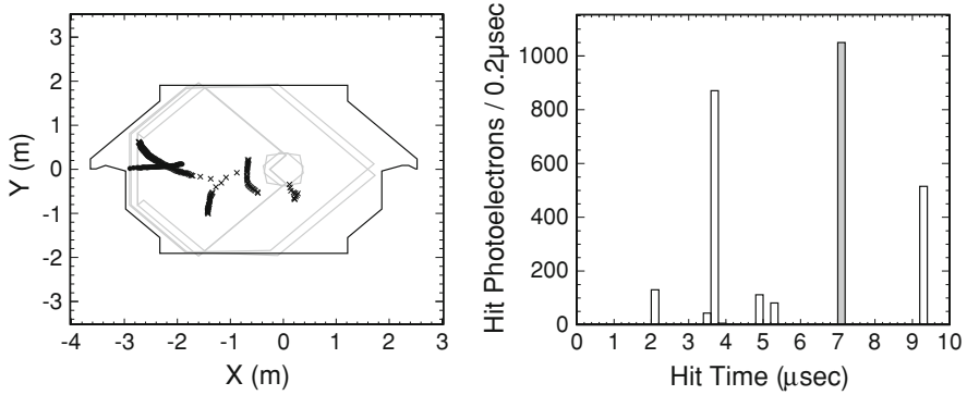
Fig. 3.15 One beam spill as observed in the Near Detector. For clarity a spill containing a smaller than average number of neutrino interactions was chosen. The left plot shows the horizontal and vertical position of track hits. The right plot shows the detector signal as a function of time, where the bin width is about ten times larger than the detector’s timing resolution. Image obtained from [6]
