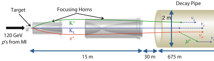
Fig. 6.6 Schematic of the NuMI beamline, illustrating the main three processes that yield \nu_e CC events. The dominant production mechanism is through \mu^+ decay, although the decays of K_L and K^+ mesons also generate \nu_e 's. Note that not all the particles involved in each decay are represented in the picture
