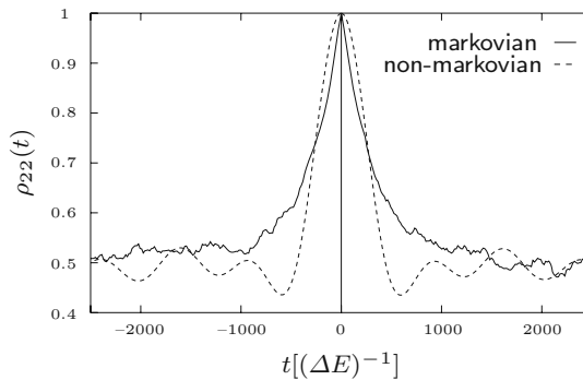
Fig. 19.6 Evolution of the excitation probability before and after full excitation for two different sets of model parameters
