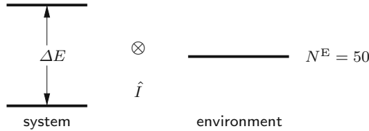
Fig. 16.1 Microcanonical scenario: a two-level system is weakly coupled to a system with one energy level of degeneracy N^E = 50 . This is a model for a system in contact with a much larger environment such that no energy can be exchanged
