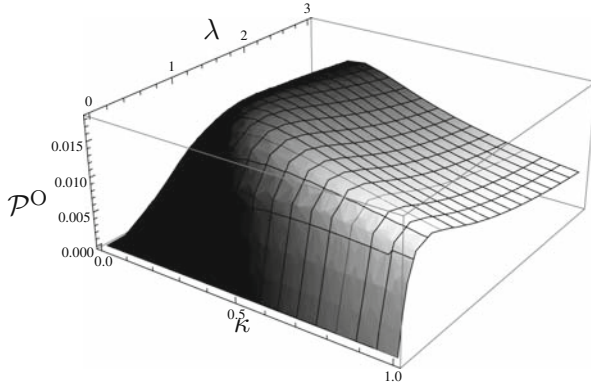
Fig. 25.11 Power of the Otto cycle depending on \kappa and \lambda . The chosen parameters are \{\epsilon_i\}_{i=1}^N = \{-3/2; -1/2; 1/2; 3/2\} , \tau_R = 1 , \delta = 0.8 , \alpha_1 = 1 , \alpha_2 = 2 , \gamma_1 = 1 , \gamma_2 = 2
