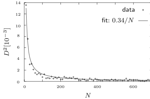
Fig. 19.5 Deviation of the exact evolution of the excitation probability from the HAM prediction for increasing number N of states in the environment
