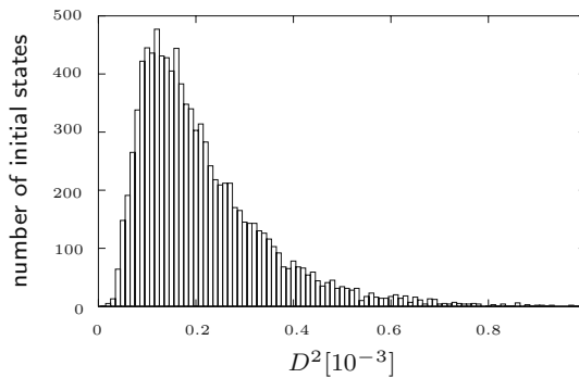
Fig. 19.4 Deviation of the exact evolution of the excitation probability from the prediction for a set of entangled initial states
