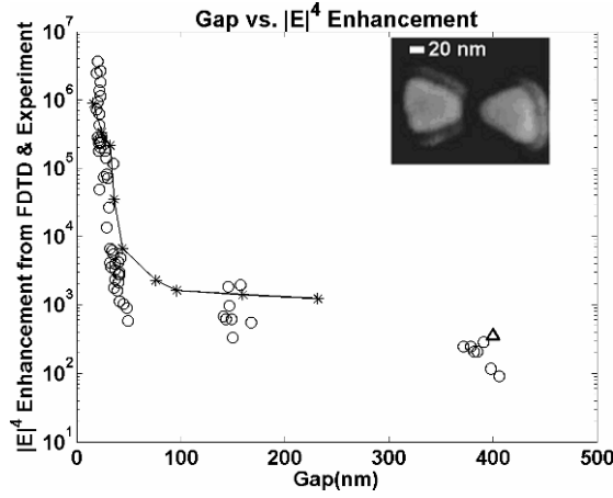
Figure 9.7. Comparison of experimental (circles) and theoretical (asterisks and triangle) values of the square of intensity enhancement, (\alpha_{bt}^i)^2 , for bowties with gaps of 16–406 nm. FDTD simulations for (\alpha_{bt}^i)^2 from an individual triangle are used for comparison to the bowties with nominal gap size of 400 nm. Excellent agreement is observed, especially for the largest and smallest gap sizes where experimental conditions most closely approximate the theoretical treatment.
