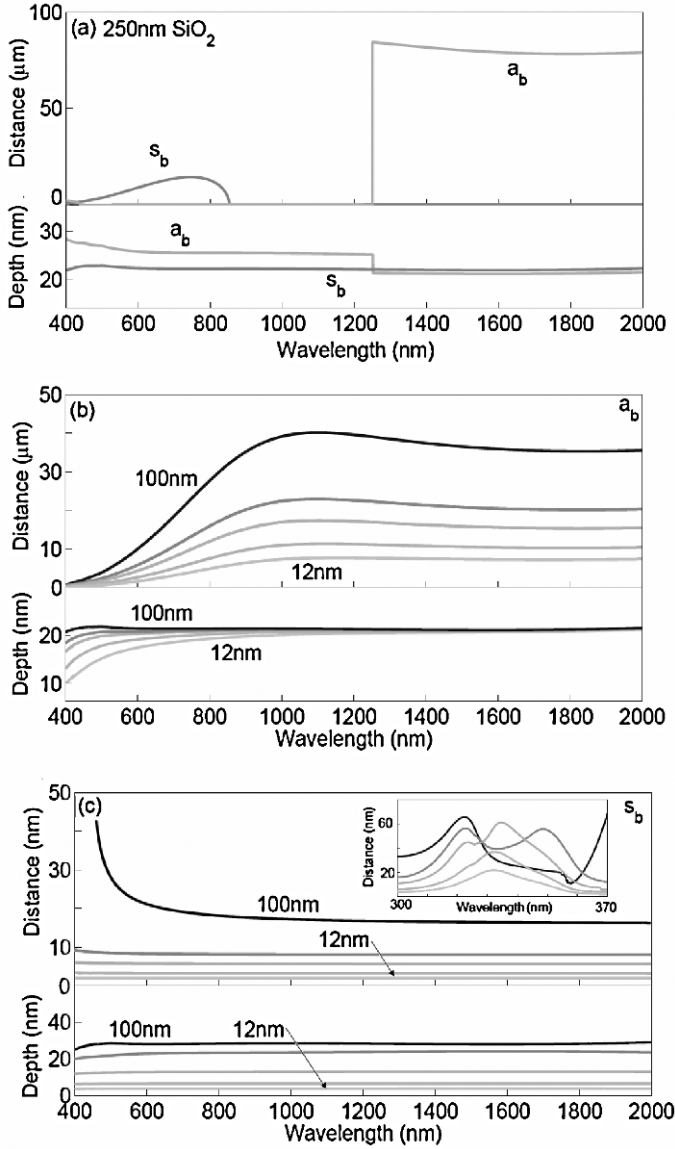
Figure 7.9. MIM (Ag/SiO 2 /Ag) propagation and skin depth plotted as a function of wavelength for core thicknesses of d = 250 nm (a) and d = 12, 20, 35, 50 , and 100 nm (b, c). In panel (a), propagation lengths of conventional (as opposed to plasmonic) waveguiding modes are recovered and correlated with skin depth. In (b), the field anti-symmetric modes of MIM guides are seen to propagate over 10 microns with skin depth never exceeding 20 nm. In (c), the symmetric modes of thinner films ( d \leq 50 nm) remain evanescent for all wavelengths. However, as d approaches 100 nm, conventional waveguiding modes can be accessed, and a region of enhanced propagation is observed for \lambda \leq 400 nm. Inset: Propagation distances of the symmetric mode for wavelengths characteristic of the quasi-bound regime. The dissociation of the thin-film single peak to the thick-film double peak indicates the onset of conventional waveguiding.
