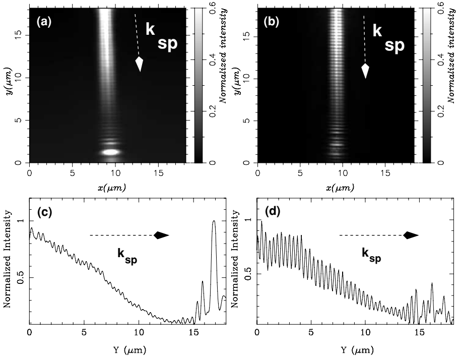
Figure 4.7. (a) PSTM image of an homogeneous MS (width 2.5 \mu\text{m} ). (b) PSTM image of a micro-structured MS equipped with a Bragg mirror [see Fig. 4.6(b)]. The free-space incident wavelength exciting the propagating SPP is 800 \text{ nm} . (c) (resp (d)) Longitudinal cross section taken along the center of the homogeneous (resp. textured) strip.
