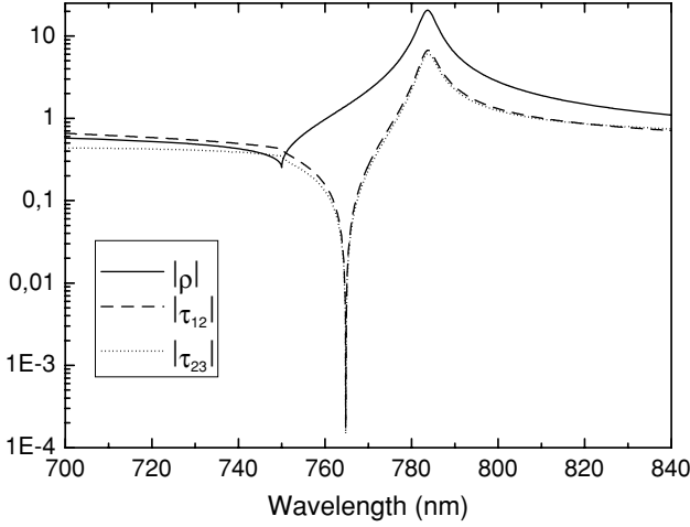
Figure 3.4. Modulus of \rho (solid), \tau_{12} (dashed) and \tau_{23} (dotted) as a function of the wavelength for a silver surface perforated with a 2D array of period d = 750 nm of circular holes with diameter a = 280 nm.
