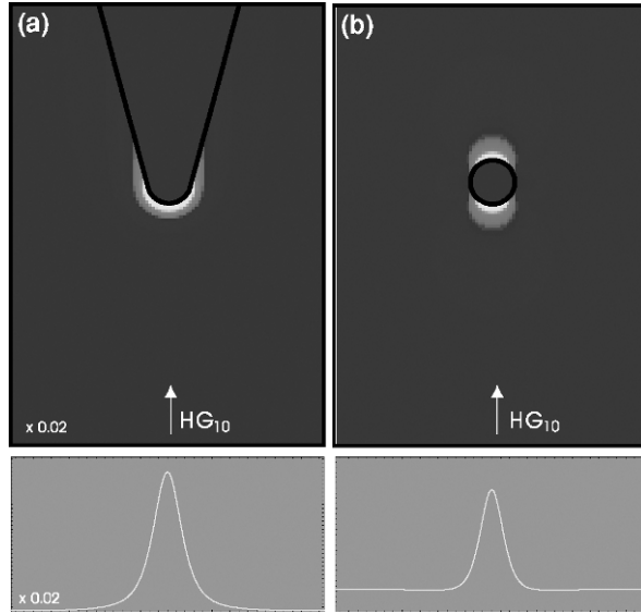
Figure 10.4. Comparison of field distributions ( E^2 ) near a gold tip (a) and a gold particle (b) irradiated by an on-axis focused Hermite-Gaussian (1,0) laser mode. At the apex of tip, the exciting laser field is polarized along the tip axis resulting in a longitudinal polarization . The resulting field is enhanced near the tip apex. The line scans at the bottom represent the field distribution on a transverse line 1 nm in front of tip and particle, respectively. However, the field distribution in case of the metal tip has been scaled by a factor of 0.02. The qualitative agreements between the field distributions indicate that in the case of longitudinal polarization, the tip can be modeled as a polarizable particle, but with a modified polarizability that depends on the field enhancement factor.
