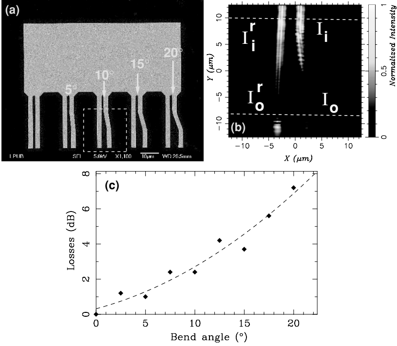
Figure 4.4. (a) SEM image of the sample used to assess bend losses. (b) PSTM image of dual MS consisting of a straight reference waveguide and a doubly bent waveguide (bend angle 10^\circ ). (c) Plot of the bend losses as a function of the bend angle.
