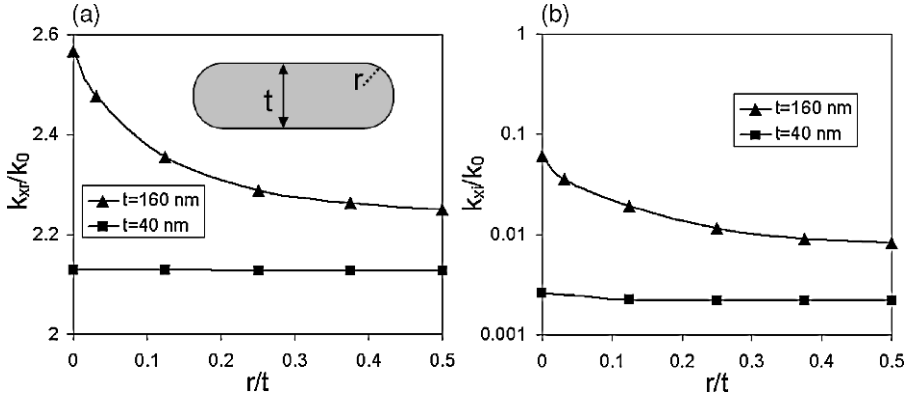
Figure 5.5. Influence of the corner curvature on the ss_b^0 mode for two different thicknesses (a,b) at \lambda_{vac} = 633 nm. Insert: geometry of the strip.
