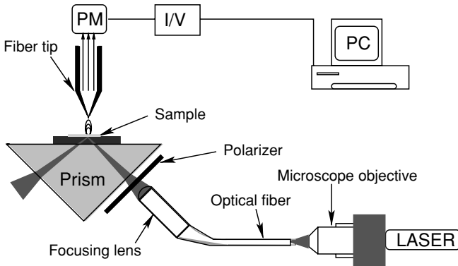
Figure 4.1. Schematic view of the PSTM setup.
