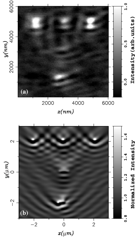
Figure 11.11. (a) PSTM image of the sample shown in Fig. 11.9 obtained by shining a TM polarized laser beam (wavelength 740 nm). (b) Theoretical distribution of the intensity of the electric field associated with the optical near-field (normalized relative to the intensity of the incident field, same illumination conditions as in the experiment).
