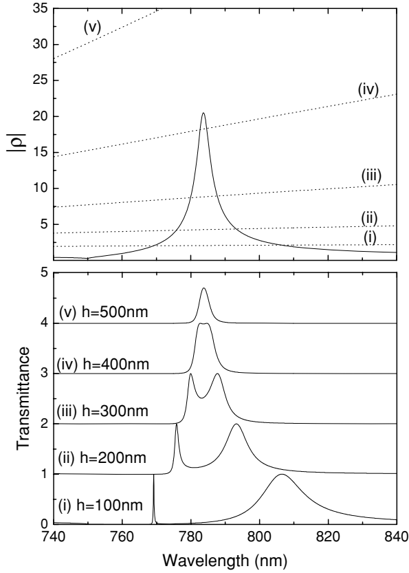
Figure 3.5. Upper panel: modulus of \rho and curves \exp(|k_z|h) for different values of h (100, 200, 300, 400 and 500 nm) for the same geometrical parameters than in the previous figures. Bottom panel: zero-order transmittance versus wavelength for the silver thicknesses considered in the upper panel.
