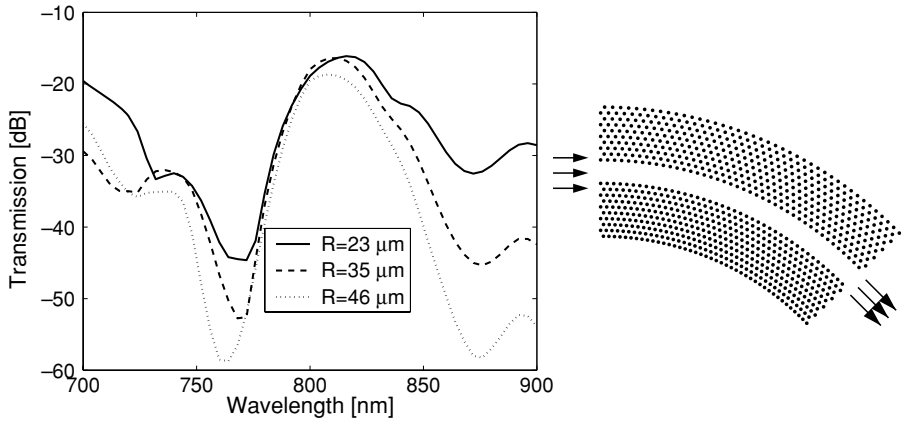
Figure 6.8. Transmission spectra for 45^\circ bends obtained by gradual rotation (with different radii) of a straight waveguide. The structure for the smallest bending radius ( 23\ \mu\text{m} ) is shown to the right.
