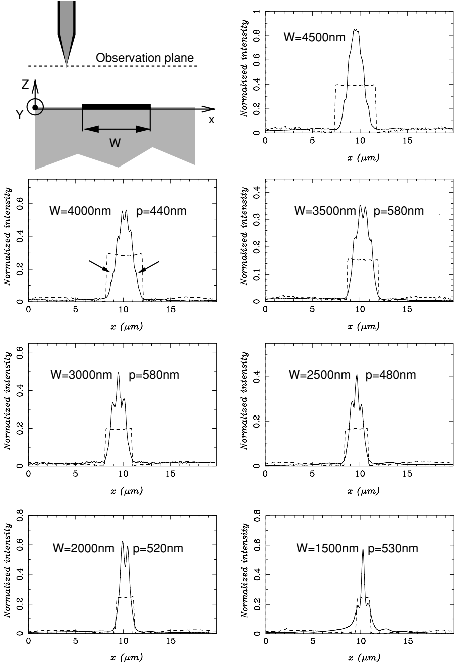
Figure 4.3. (solid lines) Transverse cross sections of the near-field images recorded at constant height over several strips. All these results have been obtained for an incident free-space wavelength of 800 nm. (Dashed lines) Topographic profiles of the considered strips.
