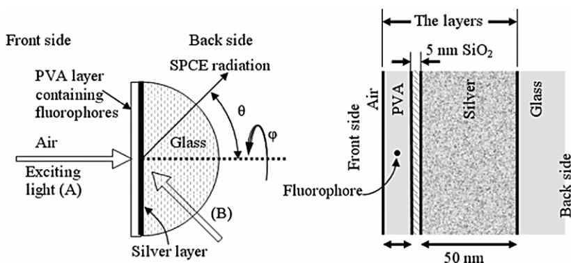
Figure 17.5. The basic configuration of an SPCE experiment. The excitation light is either coming from the left (front side, A) at normal incidence, exciting the fluorophores in the PVA layer directly, or from the right (back side, B) at the surface plasmon angle, exciting the fluorophores in the PVA layer via the SPR evanescent wave.
