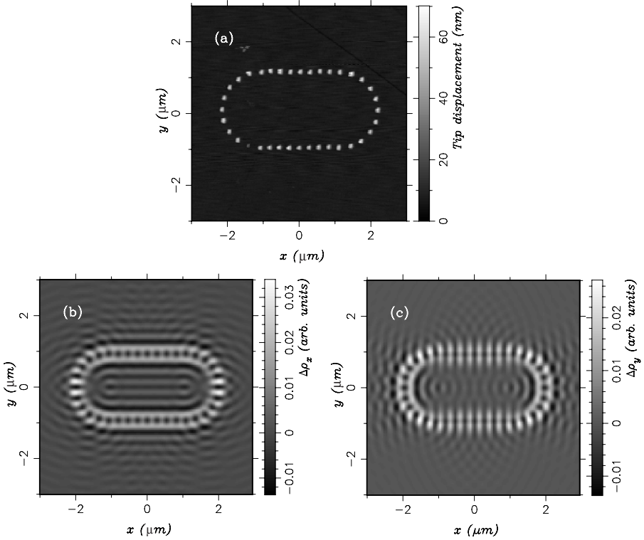
Figure 11.5. (a) AFM images of the reference sample: gold particles (100 nm × 100 nm × 50 nm) deposited on a flat glass surface. Theoretical distributions of partial LDOS change close to the sample relative to the constant value of vacuum (height of calculation plane: z = 160 nm above the substrate) (b) \Delta\rho_x(\mathbf{r}, \omega) , (c) \Delta\rho_y(\mathbf{r}, \omega) .
