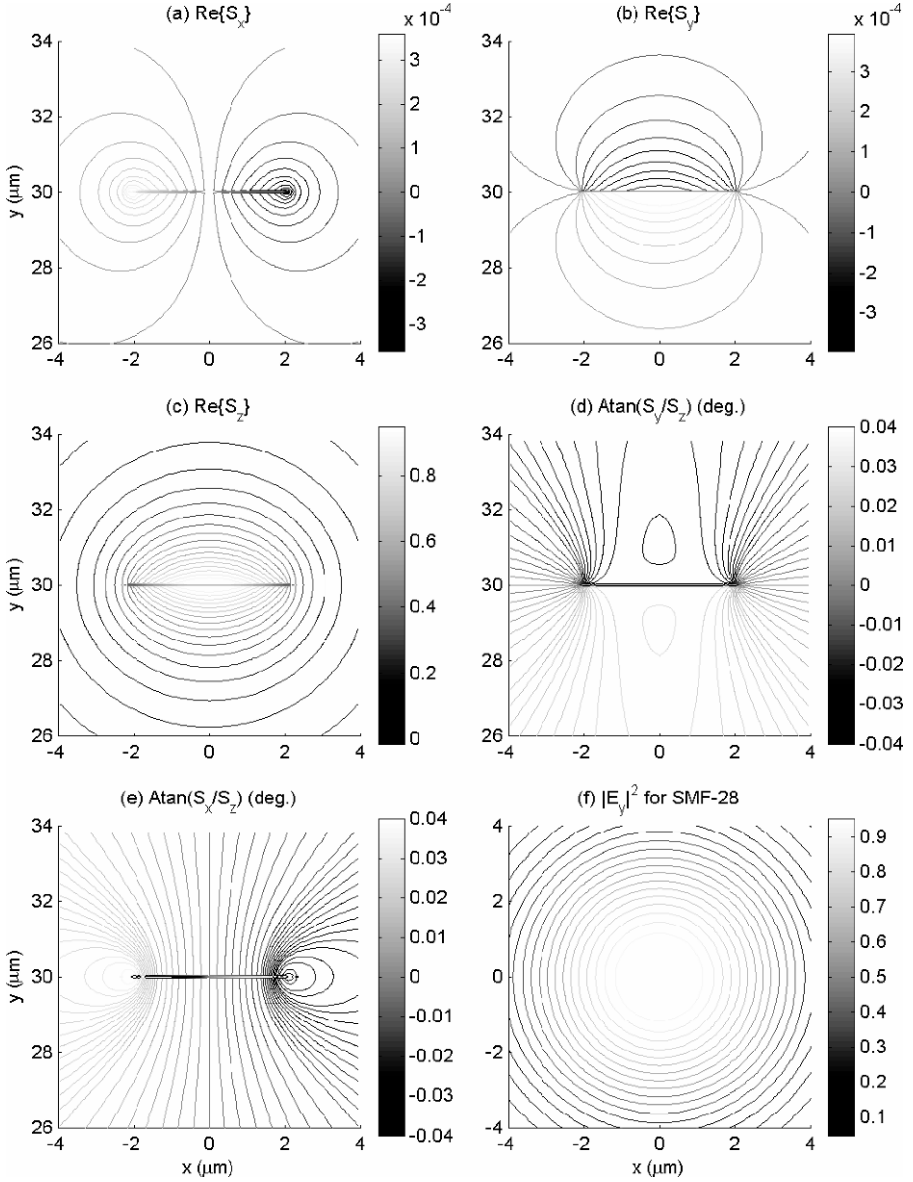
Figure 15.2. Parts (a) through (e) show contours associated with the Poynting vector of the ss_b^0 mode. Part (f) shows normalized intensity contours of standard single mode fibre.
