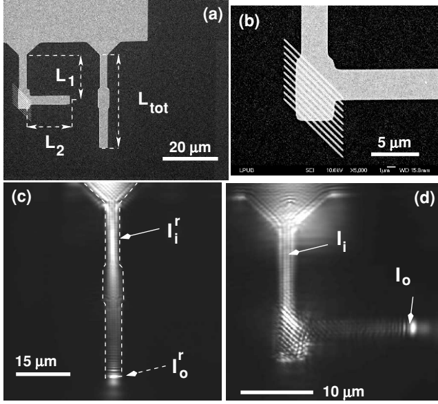
Figure 4.9. (a) and (b) SEM image of the 90° bent strip equipped with tilted Bragg mirrors. The mirror comprised gold ridges with a height of 60 nm. The losses related to the SPP guiding along the right angle bent is measured by comparison with a reference straight strip. (c) and (d) PSTM image of the reference strip and the right angle bent strip.
