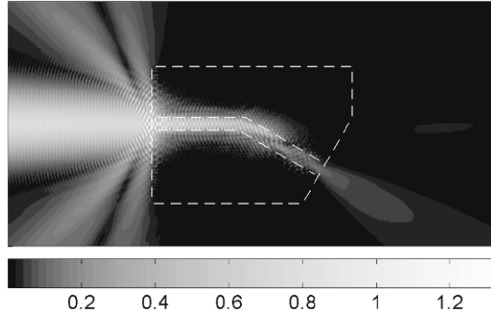
Figure 6.7. Electric field magnitude (wavelength = 800 nm) at the height 300 nm above the gold surface for the 30° bend (smoothened by removing 3 scatterers) considered in Fig. 6.6.
