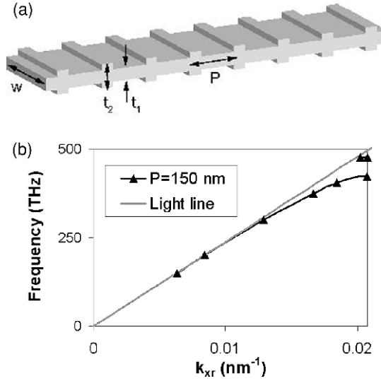
Figure 5.8. (a) Metal strip with periodic corrugations ( P = 150 nm, w = 1 \mu m, t_1 = 20 nm, t_2 = 40 nm). (b) Dispersion relation of the ss_b^0 mode.
