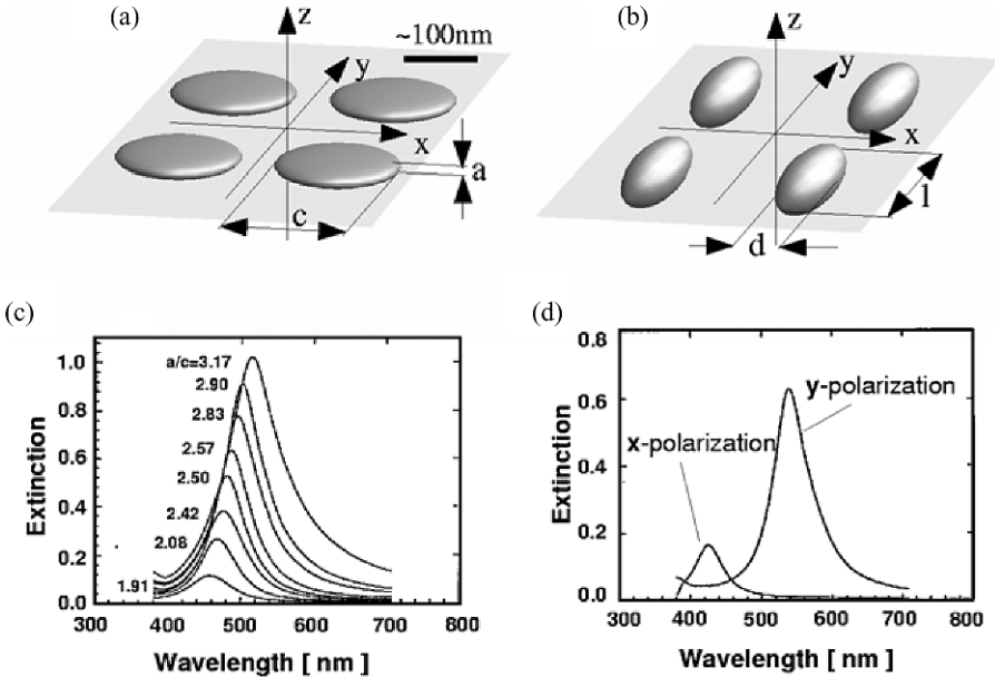
Figure 2.2. Extinction (log 10 (transmission)) spectra of arrays of metal nanoparticles with varying shape. The extinction spectra (c) of rotationally symmetric oblate particles on a glass substrate (a) shift to the red with increasing axis ratio a/c and are independent of polarization for light incident parallel to the direction of z . For prolate particles (b) the extinction is red shifted with respect to spherical particles for a polarization parallel to the long particle axis and blue shifted for a polarization parallel to the short axis (d).
