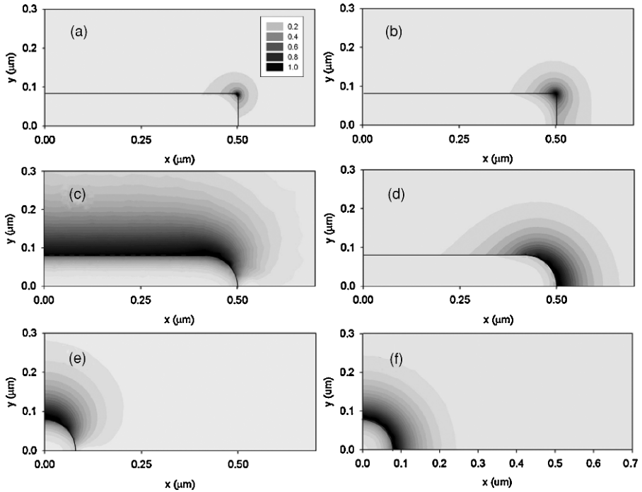
Figure 5.6. Electric field distributions of the ss_b^0 mode (a,c,e) and the sa_b^0 mode (b,d,f) for different geometries at \lambda_{\text{vac}} = 633 nm.
