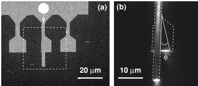
Figure 4.5. (a) SEM image of the sample fabricated to investigate the angular spreading of a MS mode. (b) PSTM image corresponding to the dashed perimeter shown in (a). The input strip has a width of 2.7 \mu\text{m} . When it reaches the wider area, the MS-SPP mode spreads out with an angle of 17^\circ .
