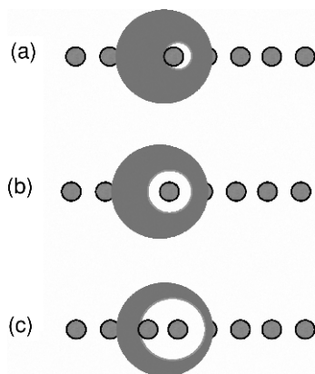
Figure 16.2. In an aperture type super-RENS disc, a transparent optical sub-window is generated in a focused laser spot. As the laser power is increased, the temperature of the Sb mask layer rises and generates a molten Sb region. At low power (a) the window is small and the signal of the small mark is also small. At increasing laser power, the window's size includes one mark: the signal reaches a maximum. As the power increases further, the window gradually begins to include the neighboring mark: the signal gradually drops.
