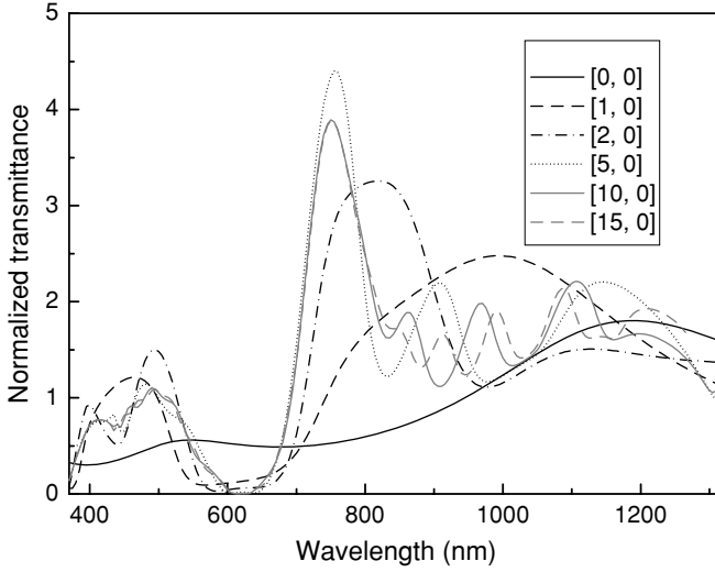
Figure 3.7. Normalized transmittance versus wavelength for a single slit of width a = 100 nm surrounded by 2N grooves ( N ranging from 0 to 15) located symmetrically with respect to the central slit and only disposed in the input surface. In these calculations the output surface is not corrugated. The period of the array is d = 600 nm, the width of the grooves is also 100 nm and their depth is 100 nm. The silver film has a thickness of 400 nm.
