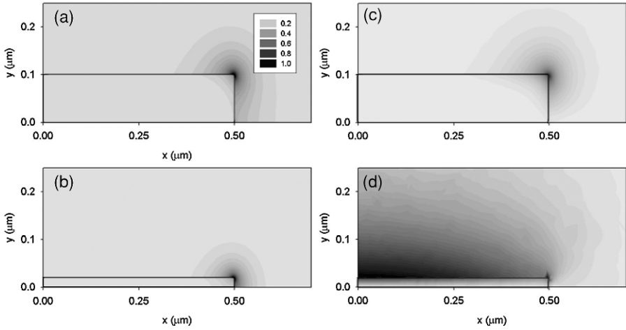
Figure 5.4. Electric field distributions of the sa_0^0 mode (a,b) and the ss_0^0 mode (c,d) for different thicknesses at the free-space wavelength \lambda_{\text{vac}} = 633 nm.
