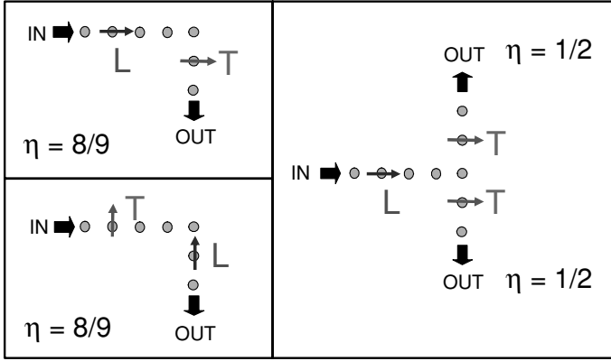
Figure 7.3. Calculated power transmission coefficient \eta in nanoparticle chain arrays for a 90 degree corner and a tee structure. The thick arrows indicate the direction of the energy flow, the thin arrows indicate the direction of polarization corresponding to either the longitudinal mode (L) or the transverse mode (T).
