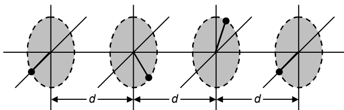
Fig. 1.8. Screw-axis symmetry
