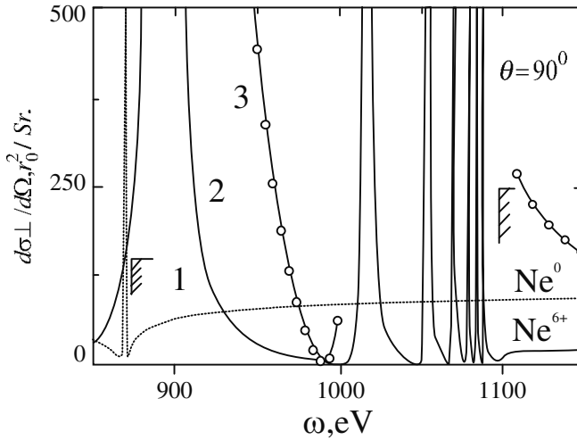
Fig. 2.21. Differential cross-section of the elastic linear polarized (at right angle to the scattering plane) X-ray photon scattering by neon atom and its ion \text{Ne}^{6+} in the energy region of the 1s -shell ionization threshold: 1 – neon atom for \Gamma_{1s} = 0,2660 eV; 2 – ion \text{Ne}^{6+} for \Gamma_{1s} = 0,0486 eV; 3 – ion \text{Ne}^{6+} for \Gamma_{1s} = 0,2660 eV. \theta is the scattering angle, \Omega is the solid angle, \omega is the scattered photon energy. The calculated energy values for the 1s -shell ionization thresholds I_{1s}({}^{10}\text{Ne}) = 872,320 eV and I_{1s}(\text{Ne}^{6+}) = 1099,131 eV are indicated
