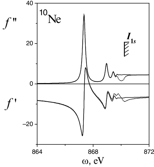
Fig. 2.7. The anomalous dispersing f' - and f'' - components of the elastic scattering amplitude for the neon atom. The symbols are the same as in Fig. 2.6
