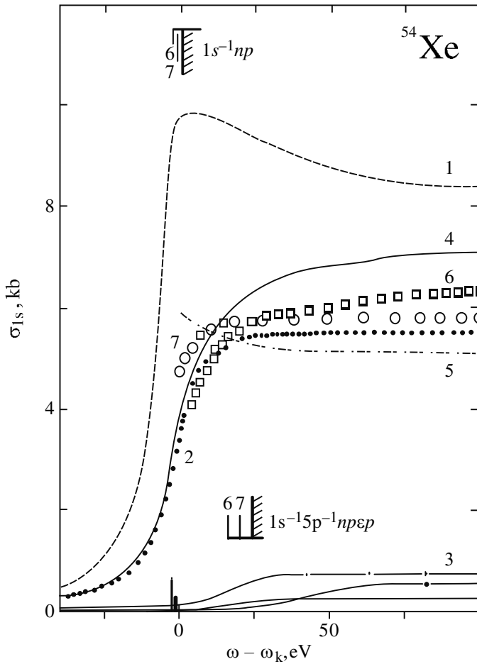
Fig. 2.15. Cross-section of the X-ray photon absorption by xenon atom 1s-shell: 1 – Approximation 1; 2 – Approximation 2; 3 – partial cross-sections of double excitation/ionization for n = 6, 7 and \varepsilon correspondingly; 4 – Approximation 2 (sum spectrum); 5 – the theory from the work [142]; 6 – Approximation 2 considering the result [142]; 7 – the synchrotron experiment from the work [149]. The width of the 1s-vacancy decay \Gamma_{1s} = 11, 49 eV. \omega is the absorbed photon energy. The calculated energy locations for xenon atom ionization thresholds K (34564, 21 eV) and KO_{23} (34587, 03 eV) are marked
