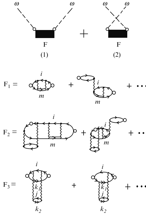
Fig. 2.1. The direct (1) and exchange (2) parts of the anomalous dispersion amplitude of the photon scattering (2.17) by an atom in Goldstone–Hubbard–Feynman diagrams representation [97]: \omega is the scattering photon energy; F = F_1 + F_2 + F_3 + \dots ; line – the state is obtained in the configuration field of the atom ground state; double line – the state is obtained in the i -vacancy field; the double arrows line – the state is obtained in the i - and j -vacancy field. The F_{1,2,3} structures are explained from the physical standpoint in the text. The time-sequential routine of the virtual processes is from left to right. The points stand for the infinite diagrams series
