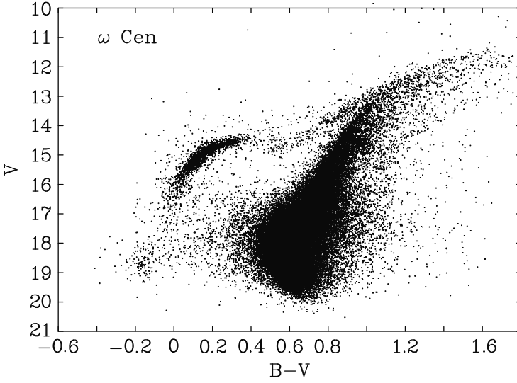
Fig. 5. Colour-magnitude diagram for the moderately metal-poor galactic globular cluster ω Cen ( Z = 0.0006 , [\text{Fe}/\text{H}] = -1.62 ; based on [18])
