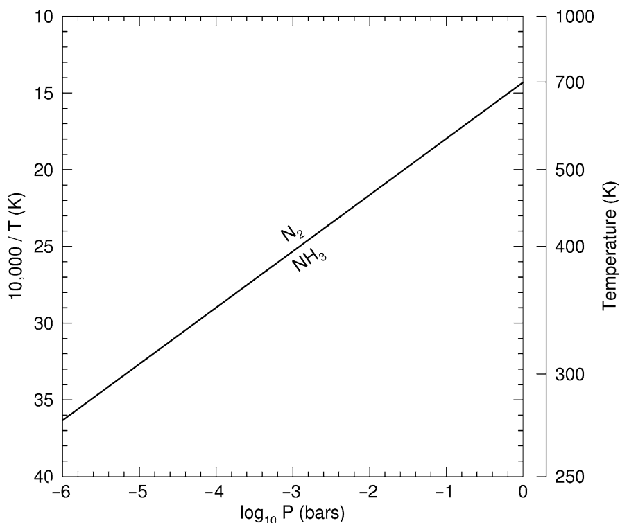
Fig. 15. Percentage distribution of nitrogen between \text{N}_2 and \text{NH}_3 in a solar composition gas as a function of temperature and pressure. The line shows where \text{N}_2 and \text{NH}_3 have equal abundances. Above the line, \text{N}_2 is more abundant, whereas below the line, \text{NH}_3 is more abundant
