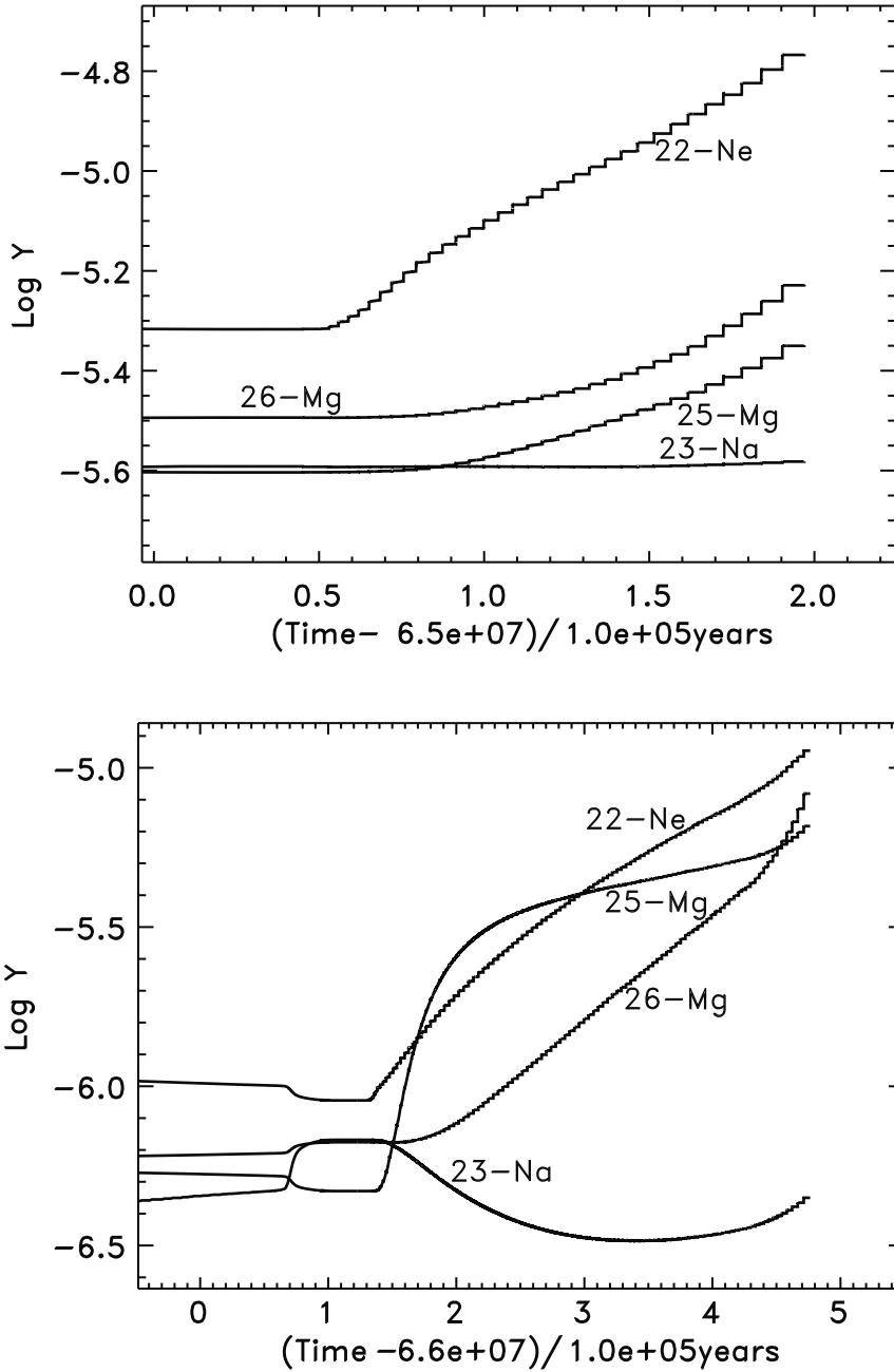
Fig. 28. The surface abundances evolution of ^{22}\text{Ne} , ^{23}\text{Na} , and the neutron-rich Mg isotopes during the TP-AGB for the 6M_{\odot} , Z = 0.02 model (top panel), and for the 6M_{\odot} , Z = 0.004 model (bottom panel)
