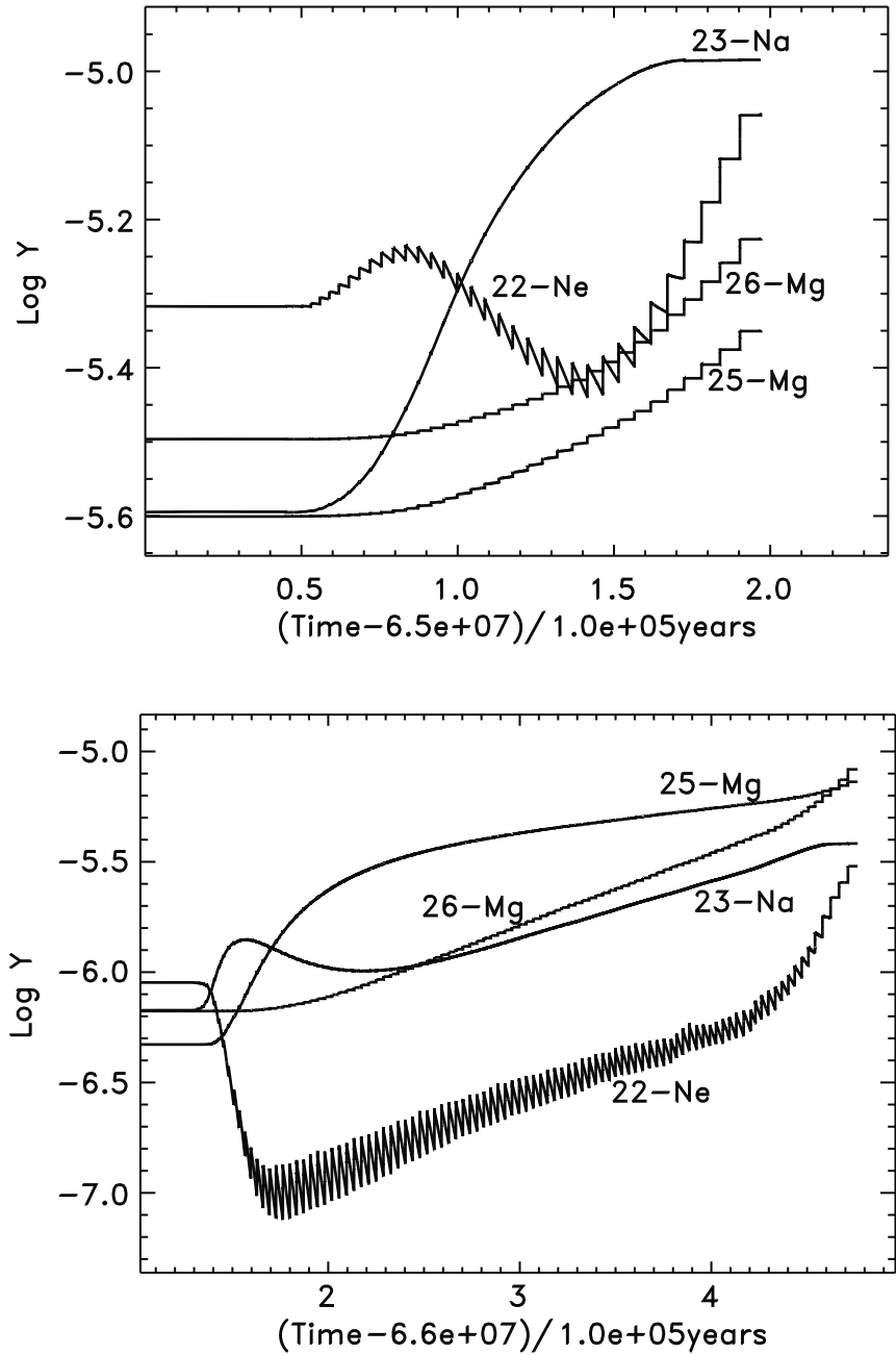
Fig. 29. Same as Figure 28, but using the NACRE rates for the Ne-Na and Mg-Al chains
