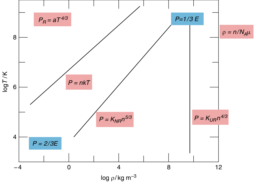
Fig. 16. A map of density-temperature space illustrating the different regimes for the equation of state, including the classical, relativistic, and degenerate limits
