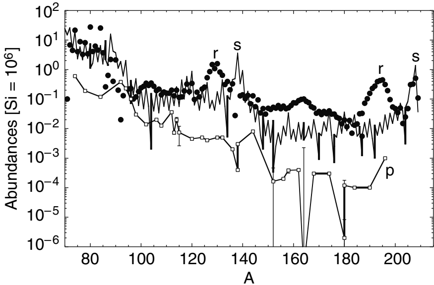
Fig. 12. Decomposition of the solar abundances of heavy nuclides into s-process (solid line), r-process (black dots) and p-process (open squares) contributions. The uncertainties on the abundances of some p-nuclides due to a possible s-process contamination are represented by vertical bars (from [32]). See Figs. 13 - 15 for the uncertainties in the s- and r-nuclide data.
