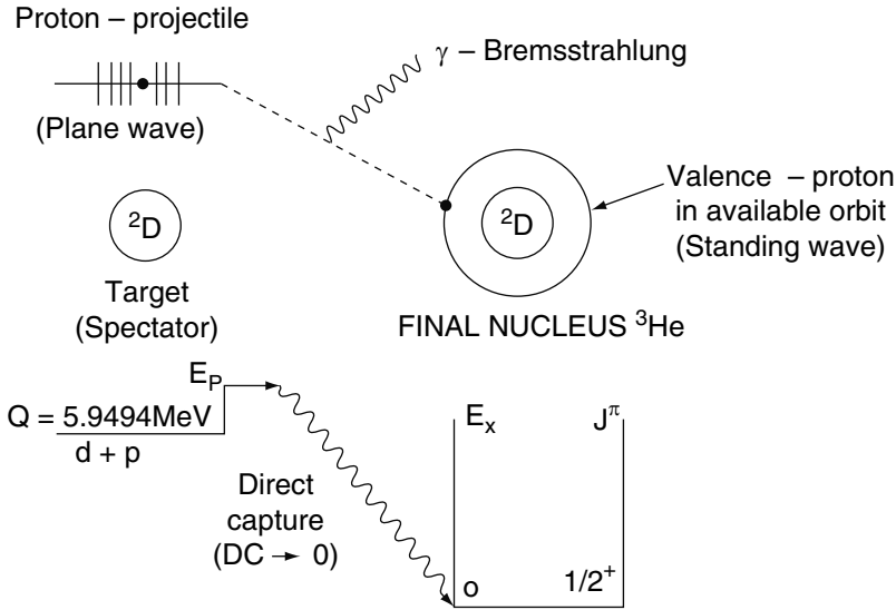
Fig. 6. The Direct Capture reaction d(p, \gamma)^3\text{He} to form ^3\text{He} in its ground state. The proton projectile (shown as a plane wave) radiates away a bremsstrahlung photon to be captured in a “valence” orbital around the ^2\text{D}
