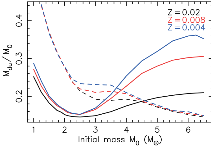
Fig. 6. Innermost mass layer ( M_{\text{du}}/M_0 ) reached by the convective envelope during the first (solid lines) and second dredge-up (dashed lines) as a function of the stellar mass, M_0
