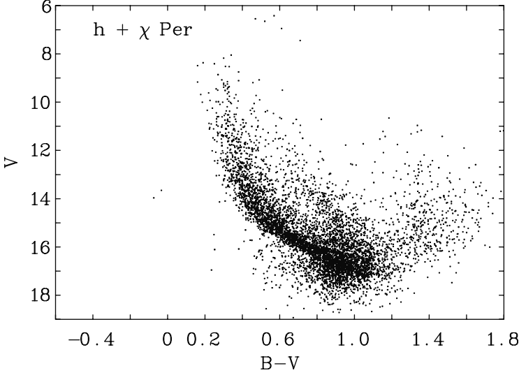
Fig. 2. Colour-magnitude diagram for the young galactic open clusters NGC 869 and NGC 884 (=h and \chi Persei; based on [15])
