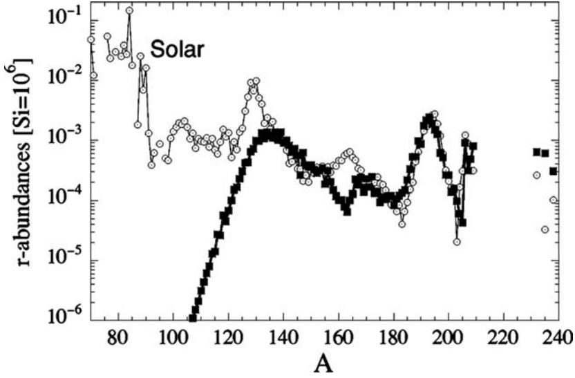
Fig. 31. Final r-abundance distribution (black squares) for a clump of material with initial density \rho = 10^{14} \text{ g/cm}^3 expanding on a timescale \tau_{\text{exp}} = 6.5 \text{ ms} . The SoS r-abundance distribution is also shown
