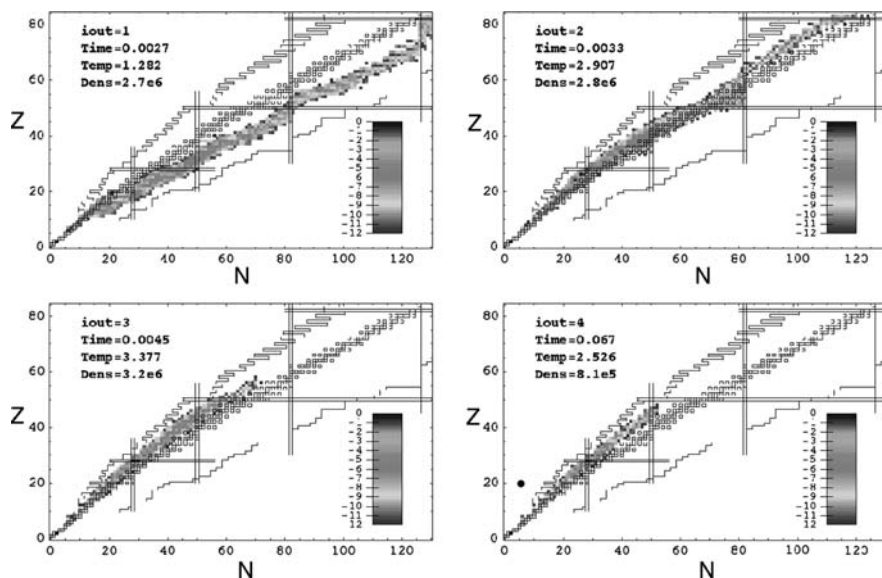
Fig. 36. Snapshots in the nuclidic chart of flow patterns in a 1D model of a detonating He layer accreted onto a 0.8M_{\odot} WD. The selected times and corresponding temperatures or densities are given in different panels. The stable nuclides are indicated with open squares. The magic neutron and proton numbers are identified by vertical and horizontal double lines. The drip lines predicted by a microscopic mass model are also shown. The abundances are coded following the grey scales shown in each panel. At early times (bottom left panel), an r-process type of flow appears on the neutron-rich side of the valley of nuclear stability. At somewhat later times (top left panel), the material is pushed back to the neutron-deficient side rather close to the valley of \beta -stability. As time passes (two right panels), a pn-process [87] develops
