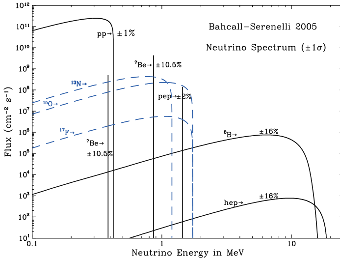
Fig. 10. The spectrum of the neutrinos produced by different reactions in the pp-chain in the sun (taken from [33])
