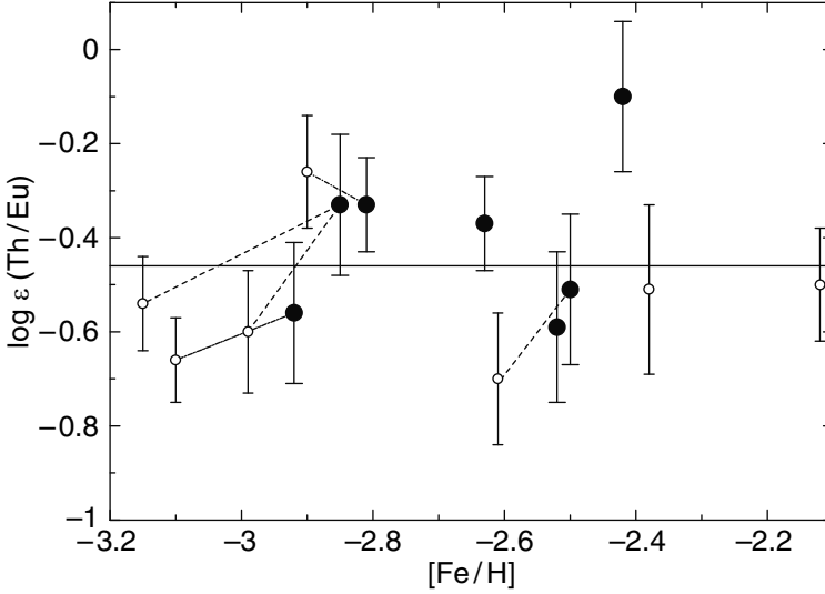
Fig. 21. Values of Th/Eu (in the \epsilon scale defined in Fig. 17) versus [Fe/H] obtained from different observations (from [49]). The black circles are from [49], whereas the open circles are earlier observations with sometimes different [Fe/H] assignments. The solid horizontal line corresponds to the SoS value
