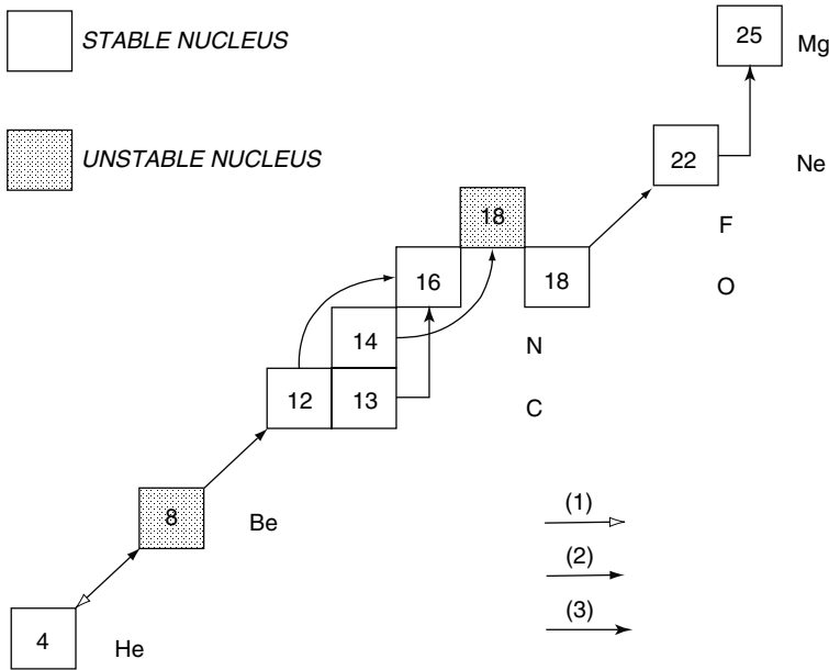
Fig. 4. Main reactions involved in the burning of helium. Arrows of types (1), (2) and (3) refer to (\gamma, \alpha) , (\alpha, \gamma) and (\alpha, n) reactions
