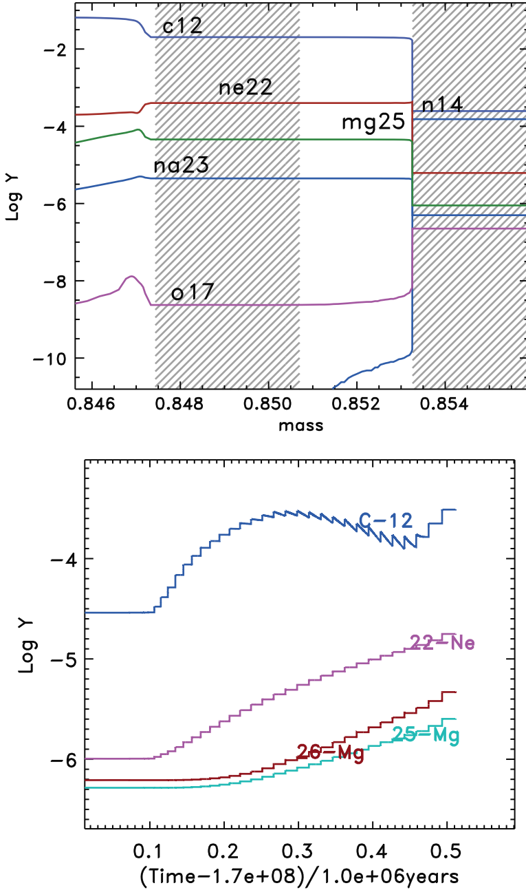
Fig. 19. (Top panel) Composition profile for the 4M_{\odot} , Z = 0.004 model during the 20 th thermal pulse. The peak temperature in the He-shell during this pulse is 360 million K. (Bottom panel) Evolution of the ^{12}\text{C} , ^{22}\text{Ne} , ^{25}\text{Mg} , and ^{26}\text{Mg} surface abundances of the 4M_{\odot} , Z = 0.004 model during the TP-AGB. The effect of HBB can be seen on the surface abundance of ^{12}\text{C}
