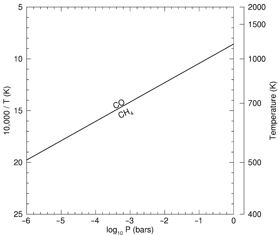
Fig. 14. Percentage distribution of carbon between CO and CH 4 in a solar composition gas as a function of temperature and pressure. The line shows where CO and CH 4 have equal abundances. Above the line, CO is more abundant, whereas below the line, CH 4 is more abundant
