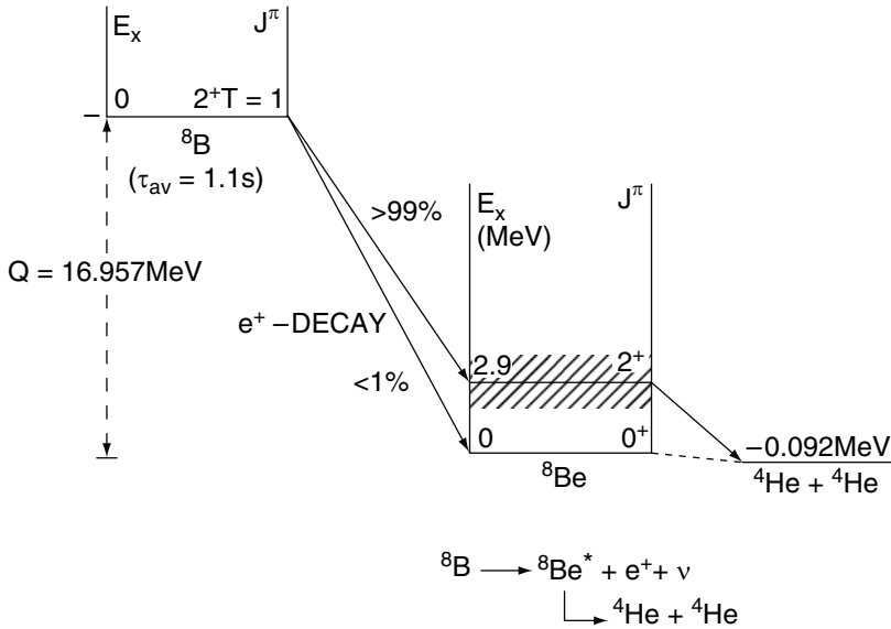
Fig. 8. The decay scheme of {}^8\text{B} with positron emission, which goes to the first excited state of {}^8\text{Be} at E_X = 2.9 MeV with a width of \Gamma = 1.6 MeV. The {}^8\text{Be} nucleus itself fissions into two alpha particles. The neutrinos accompanying the positron decay of {}^8\text{B} are the higher energy solar neutrinos with \bar{E}_\nu = 7.3 MeV
