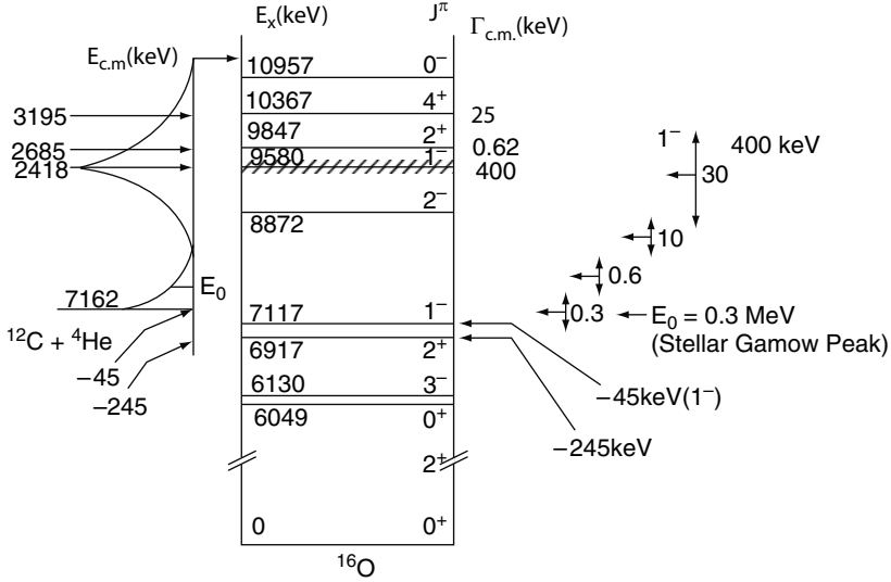
Fig. 12. Energy levels of ^{16}\text{O} nucleus near and above the alpha-particle threshold of capture on ^{12}\text{C} . Shown on the right are effective stellar energy regions corresponding to the temperatures given near the three-way arrows. The reaction rate is influenced mainly by the high energy tails of two sub-threshold resonances in ^{16}\text{O} at E_R = -45 keV and E_R = -245 keV, plus the low energy tail of another high-lying broad resonance at 9580 keV
