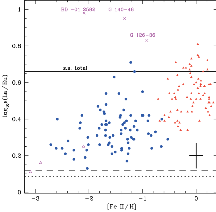
Fig. 17. Values of \log_{10} \epsilon(\text{La}/\text{Eu}) = \log_{10}(\text{N}_{\text{La}}/\text{N}_{\text{H}}) - \log_{10}(\text{N}_{\text{Eu}}/\text{N}_{\text{H}}) versus [\text{Fe}/\text{H}] from various studies (different symbols). A typical error is shown as a dagger. The three labelled points correspond to metal-poor La-rich stars. The solid line is the total SoS La/Eu ratio, and the broken lines indicate the SoS s - and r -process abundance breakdowns (from [36], where the references to the observations are provided)
