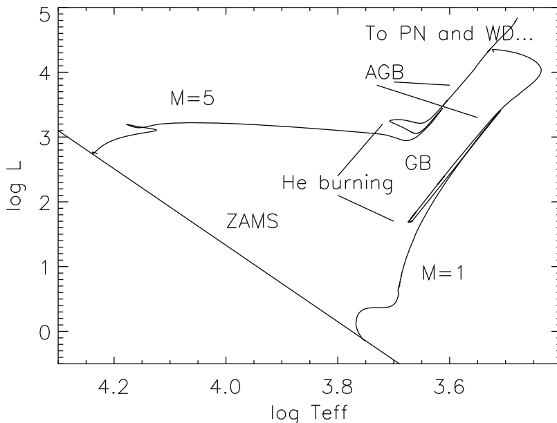
Fig. 8. Schematic L - T_{\text{eff}} diagram showing the evolution of 1 and 5 M_{\odot} mass stars. (Based on a figure by J. Lattanzio. Evolution tracks computed by R. G. Izzard.)
