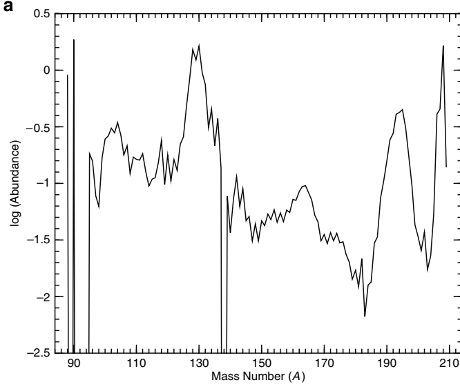
Fig. 14. The r-process abundances by subtracting the s-process abundances from the observed values (taken from [36])
