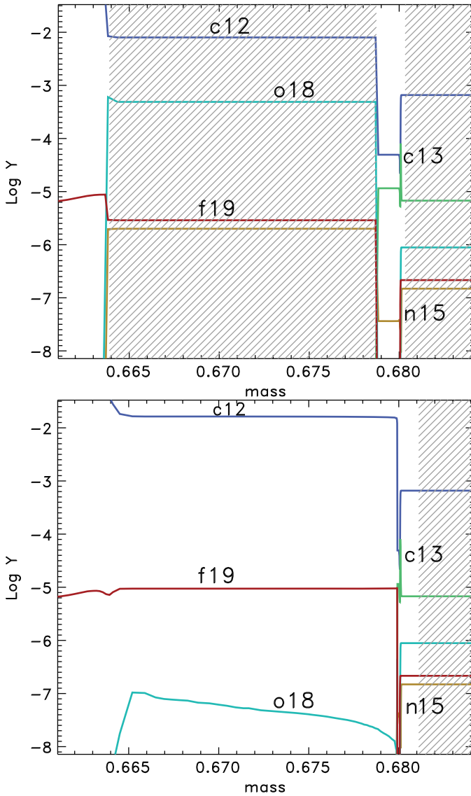
Fig. 22. The composition of the He-intershell for a 3M_{\odot} , Z = 0.02 model. The upper panel shows the composition during a thermal pulse, where the flash-driven convective pocket is shown (at its full extent it reaches from 0.664M_{\odot} almost all the way to the H-shell at 0.679M_{\odot} ). The lower panel shows the composition of the He-intershell after the thermal pulse has died down, before the next third dredge-up takes place. The location of the base of the outer convective envelope is \approx 0.681M_{\odot} .
