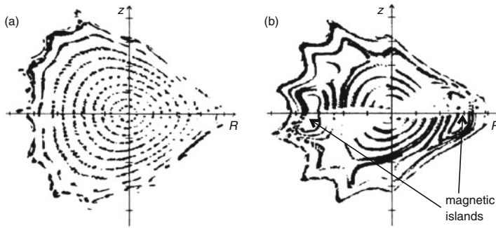
Fig. 3.20 Visualization of the rotational transform by an electron beam and a small movable phosphor screen in the Wendelstein 7-AS stellarator. (a) Nested magnetic surfaces for \iota/2\pi = 0.47 . (b) Magnetic islands form at \iota/2\pi = 1/2 . (Reprinted with permission from [64]. © 1993, IAEA.)
