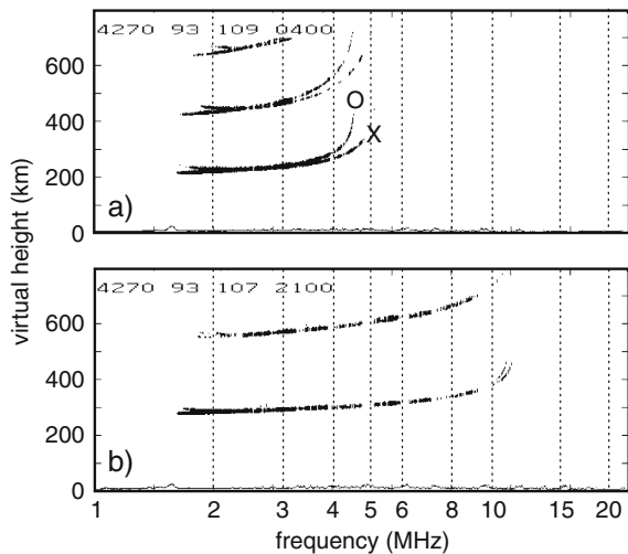
Fig. 6.16 (a) Typical night-time ionogram in the equatorial ionosphere. There appear two-pass and three-pass reflections between ground and ionosphere. The splitting into O-mode and X-mode is clearly visible. (b) Typical evening ionogram with a much higher plasma density
