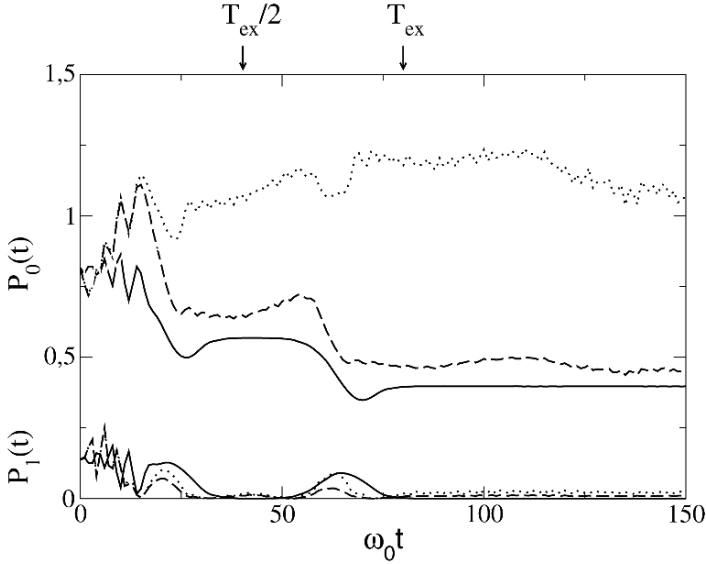
Fig. 4.10. Survival probability for ground ( P_0 ) and first excited state ( P_1 ) of a Morse potential driven by an external sinusoidal field (4.32). Exact (solid), eHK (long-dashed), and HK (dotted) results are shown. For comparison the light grey line depicts results calculated with the conventional HK, but with renormalized wave packets at each time step. T_{\text{ex}} denotes the period of the external driving.
