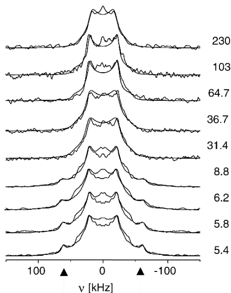
Fig. 5.15. Experimental and simulated (smooth curves) ^2\text{H} NMR spectra of a Ru-D 2 complex, measured in the temperature range from 5.4. to 230 K. At temperatures below 8.8 K a splitting in the line shape is clearly visible (arrows). This splitting can be explained by a coherent tunneling of the deuterons in the Ru-D 2 sample. For the details of the simulations see [98]. Courtesy of G. Buntkowsky, University of Jena.
