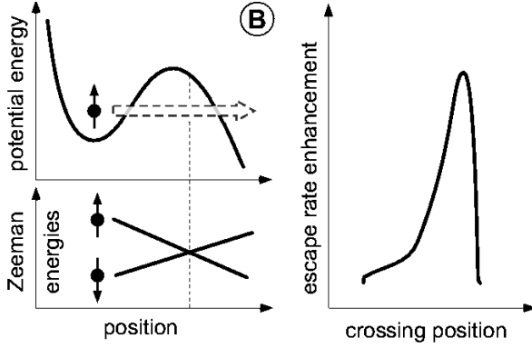
Fig. 3.7. Tunneling of a qubit out of a metastable well can be seen as tunneling of a fictitious particle with spin 1/2 such that its instantaneous position acts a magnetic field. When the corresponding Zeeman levels cross under the barrier, the escape rate is enhanced by spin flips (Zener-flip tunneling).
