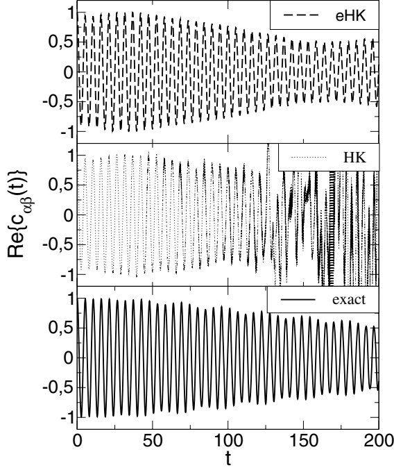
Fig. 4.9. Real part of c_{\text{fi}} vs. time for the driven metastable well for resonant driving. Results for eHK (top), HK (middle), and exact (bottom) dynamics are shown. Parameters are V_b/\hbar\omega_0 = 2 , q_i/l = q_f/l = 0 , and Al = 0.04V_b . Frequencies are \Omega/\omega_0 = 2.135 (exact resonance) and \Omega/\omega_0 = 2.335 (semiclassical resonance).
