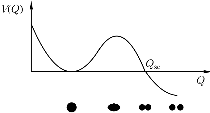
Fig. 6.5. Nuclear fission along a collective coordinate Q as decay from a metastable state. The deformation of the nucleus along the reaction path is sketched below.
