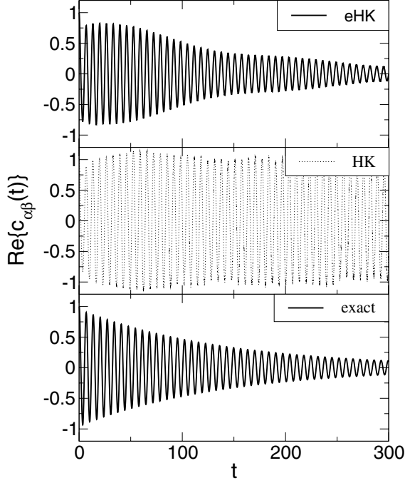
Fig. 4.5. Real part of the correlation c_{\alpha\beta} vs. time for the static metastable well (4.14). Results for eHK (top), HK (middle), and exact (bottom) dynamics are shown. Parameters are V_b/\hbar\omega_0 = 0.93 , and q_i/l = q_f/l = 0 .
