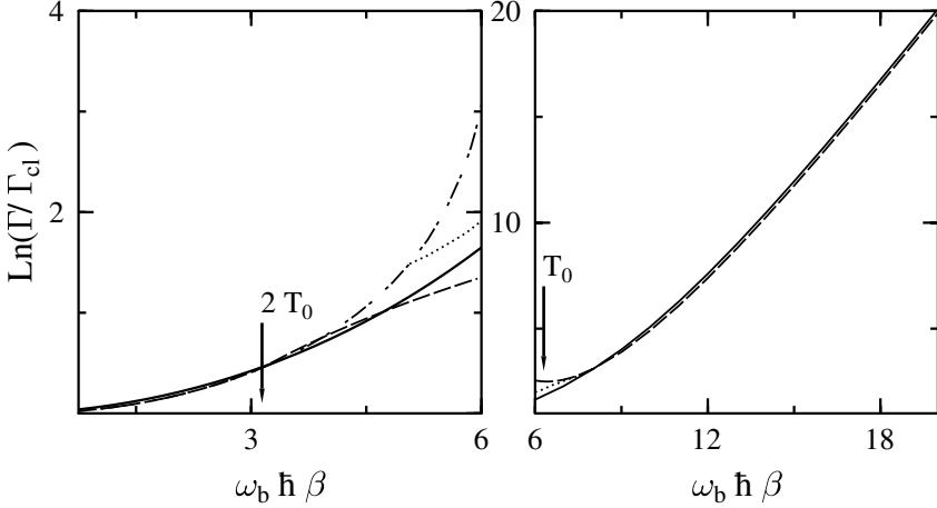
Fig. 7.8. Transmission factor P as a function of inverse temperature for an Eckart barrier with \alpha = 12 , \alpha = 2\pi V_0/\hbar\omega_b . P is defined by P = \Gamma/\Gamma_{\text{cl}} with \Gamma_{\text{cl}} the classical rate, i.e. the high temperature limit to (7.31). The solid line is the exact result. In the left picture the dotted-dashed line shows the parabolic result (7.31), the dashed line represents (7.75), and the arrow indicates the inverse temperature corresponding to T_c . In the right picture the dashed line depicts the result (7.83) and the arrow refers to the crossover temperature T_0 = T_c/2 . The \text{Im}F result beyond the Gaussian approximation around T_0 is represented by the dotted lines.
