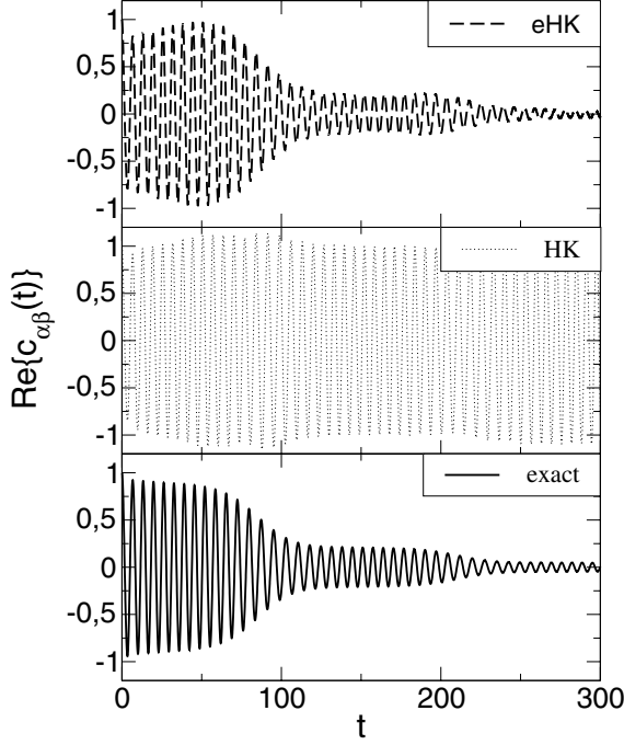
Fig. 4.7. Real part of c_{\beta} vs. time for a driven metastable well with weaker driving. Results for eHK (top), HK (middle), and exact (bottom) dynamics are shown. The external driving is characterized by \Omega/\omega_0 = 0.05 and Al = 0.4V_b . Other parameters are as in Fig. 4.5.
