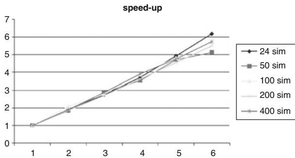
Fig. 3. Speed-up versus the number of nodes (2 subdomains per node).
