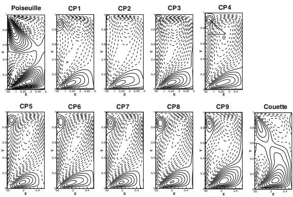
Fig. 2. Streamlines of mean secondary flow; solid lines for counter-clockwise rotation, dashed lines for clockwise rotation.
