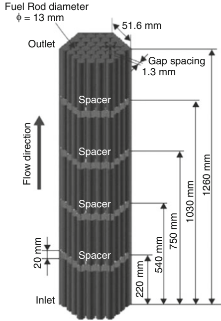
Fig. 3. Outline of three-dimensional analytical geometry of a tight-lattice fuel bundle
