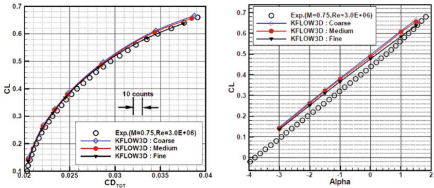
Fig. 2. (left) Drag Polar [3] and (right) CL vs. AOA curves [3]
