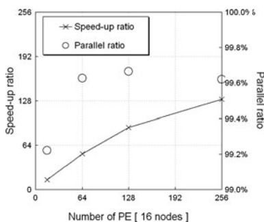
Fig. 9. Parallel performance in 16 multi-node system of SX-9
