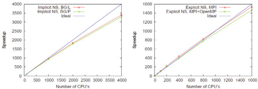
Fig. 1. Speedup, incompressible flow solver. Comparison BlueGene/L and/P.
