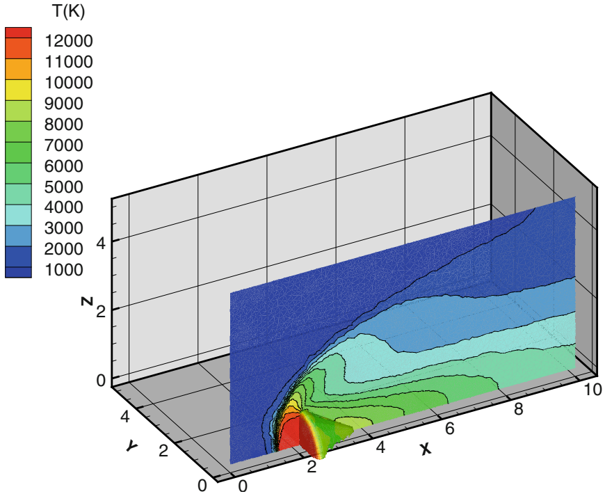
Fig. 5. Temperature distribution (K) around Apollo capsule model at speed 12Ma
