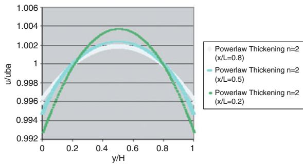
Fig. 6. LB Velocity profiles at the exit of the microchannel for power law shear-thickening fluid .
