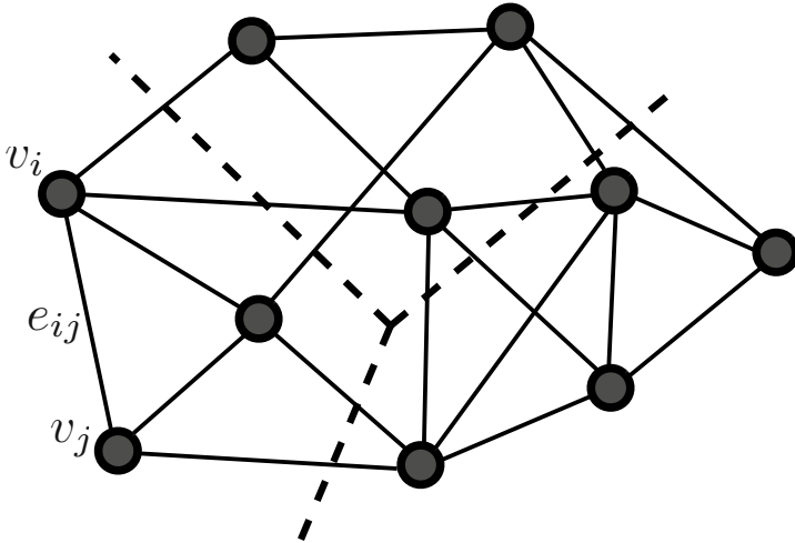
Fig. 4. Sketch that illustrates the graph representation of the sub-trees. The FMM sub-trees are represented as vertex in the graph, and the communication between sub-trees is represented by the edges between corresponding vertices. Each vertex has an associated weight v_i , that represents an estimate of the total work performed by the sub-tree. Each edge has an associated weight e_{ij} , that represents an estimate of the work between sub-trees v_i and v_j . By finding an optimal partitioning of the graph into as many section as processes available, we achieve load balance while minimizing communications. In the figure the graph has been partitioned in three sections, the boundaries between sections are represented by the dashed lines, and all the sub-trees that belongs to the same section are assigned to the same process.
