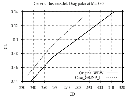
Fig. 3. Generic business jet. Drag polar at M = 0.80 for wing-body configuration. Original wing vs. optimal one ( Case_GBJNP_1 ).
