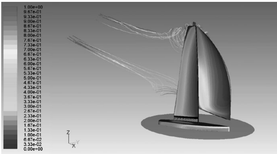
Fig. 1. static pressure coefficient distribution on sails and hull ( C_p=(p-p_0)/q , where p_0 is the outflow undisturbed reference pressure and q is the inflow undisturbed reference dynamic pressure). Path lines colored by time show the boom and the mainsail tip vortices. The yacht is sailing at 45° of apparent wind angle (i.e. the angle between the hull longitudinal axes and the incident wind at the reference height of 10m full scale) and is 5° leeward heeled. The America's Cup Class (version 5) mainsail and asymmetrical spinnaker for light wind are trimmed to produce the maximum driving force in the boat direction.
