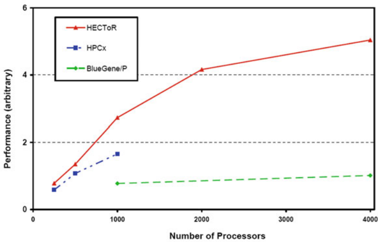
Fig. 8. Strong scaling performance of Senga2-1 Step Arrhenius-type Mechanism with 1000 3 global grid points.
