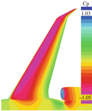
Fig. 1. Generic business jet. Pressure distribution for full aircraft configuration: original geometry.
