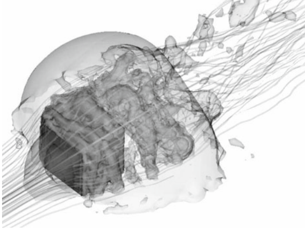
Fig. 3. Surface mounted cube in a channel flow at Re_\tau = 590 (based on the cube height and the bulk velocity Re_h = 7235 ). Pressure iso-surfaces with streamlines.
