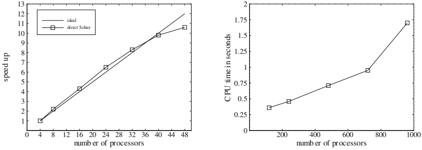
Fig. 2. Left: Strong speedup for direct Schur solver on a 1.08M mesh. Right: Scalability in spanwise direction, constant load per CPU is 1.4 \times 10^5 unknowns.
