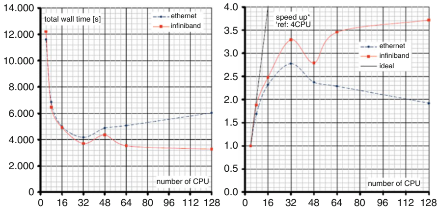
Fig. 3. Results on 100 iterations, left: Total wall time; right: speed-up.
