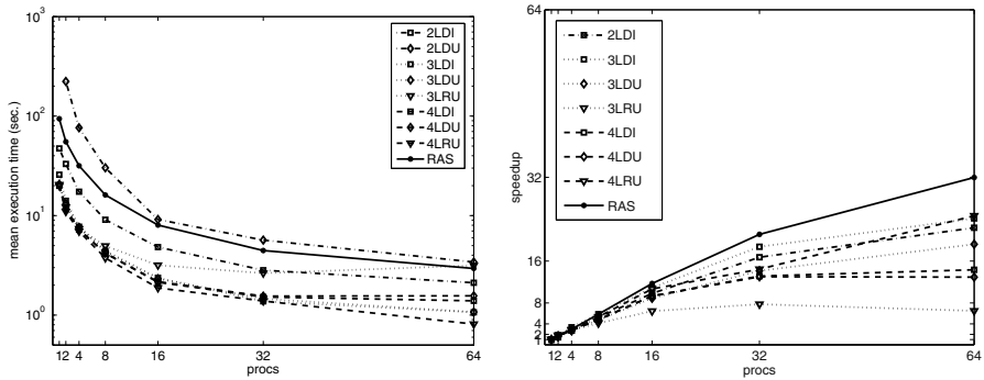
Fig. 1. Mean execution times (left) and speedup (right) of preconditioned RGMRES on the pressure equation.
