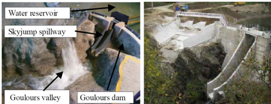
Fig. 7. Left: picture of an EDF physical model of the Goulours structure; right: real Goulours dam and spillway.
