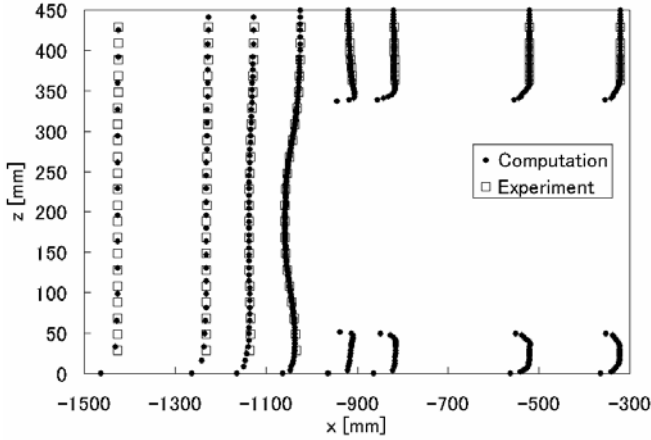
Fig. 9. Mean streamwise velocity profiles at the front body on the symmetry plane
