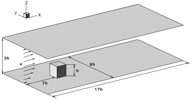
Fig. 1. Geometry of the wall-mounted cube in a channel.
