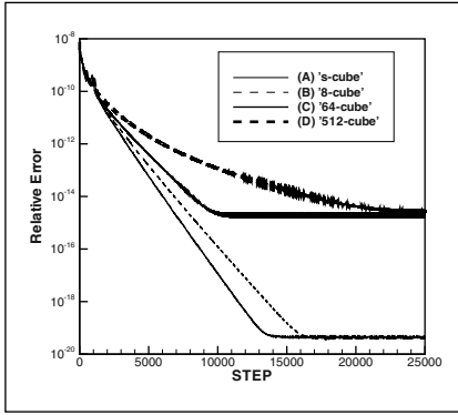
Fig. 10. Convergence history for several cube arrangements w/o IRS.
