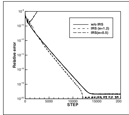
Fig. 11. Convergence history for 's-cube' with and w/o IRS.
