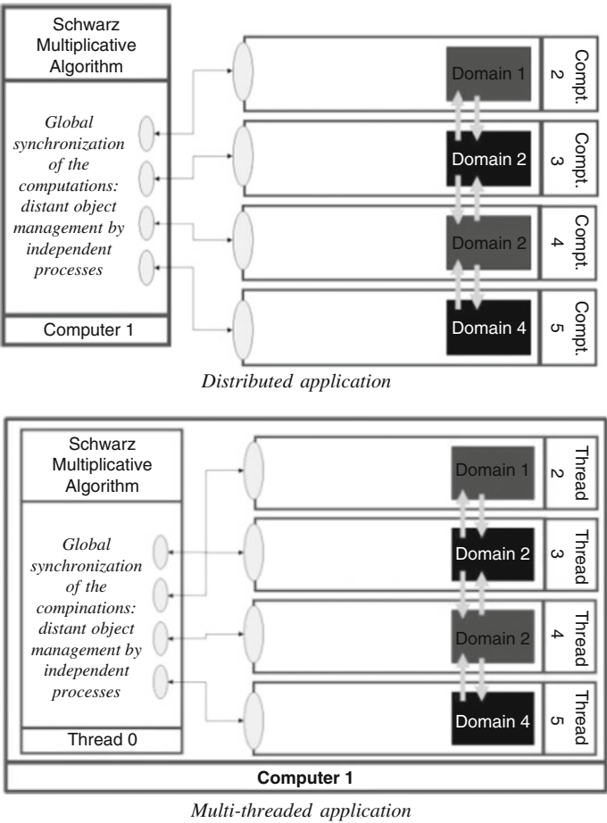
Fig. 1. Multi-threaded application versus distributed application.
