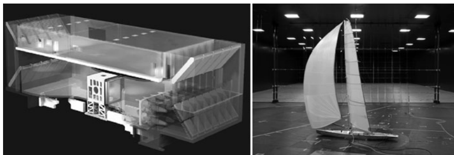
Fig. 2. left: Politecnico di Milano Twisted Flow Wind Tunnel closed circuit; right: sail plan test in the boundary layer test section.
