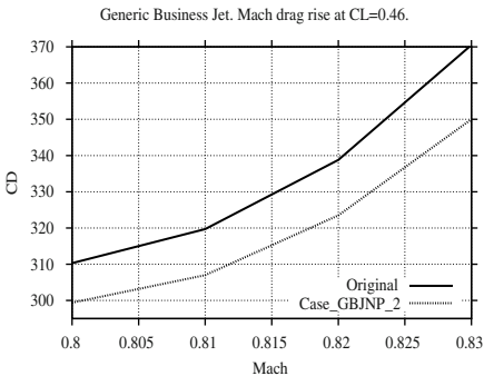
Fig. 9. Generic business jet. Mach drag divergence curve for full aircraft configuration. Original wing vs. optimal one ( Case_GBJNP_2 ).
