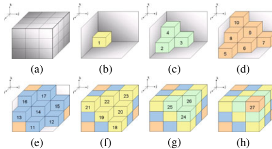
Fig. 8. Schematic diagrams of Domino method ( 3 \times 3 \times 3 ).
