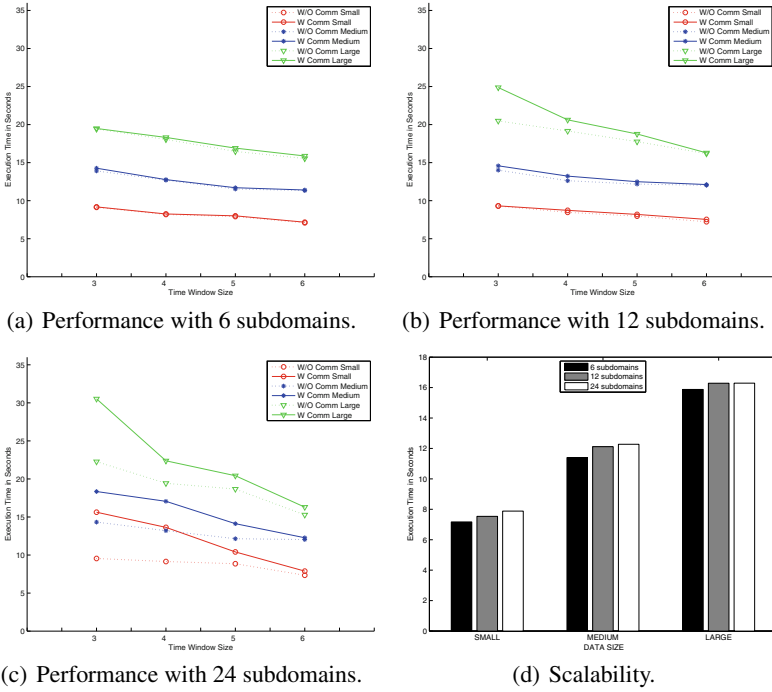
Fig. 4. PAASWR Execution Time in Seconds.
