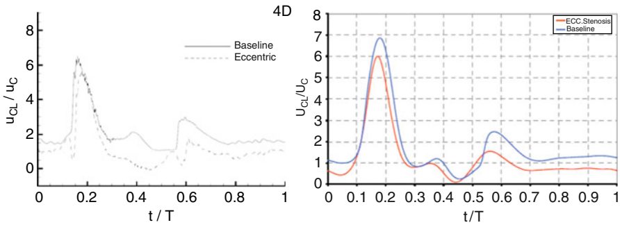
Fig. 15. Experimental (left) and numerical simulation (right) comparison of the jet centerline velocity in the eccentric stenosis at 4D downstream; the baseline case is for the axisymmetric stenosis.
