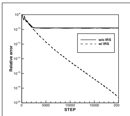
Fig. 14. Convergence history for actual problem w/ and w/o IRS.
