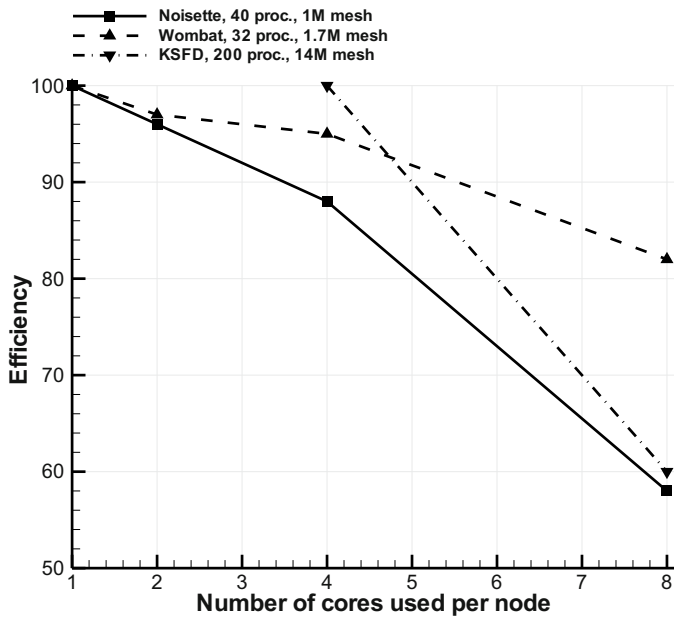
Fig. 1. Efficiency of using cores in 40 CPU case running on 8-core nodes
