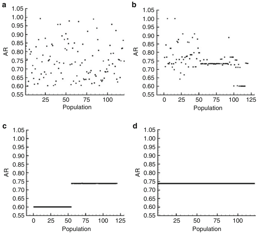
Fig. 3. Selected steps in the convergence history of aspect ratio of the tail (a) Initial, (b) After 30 generations, (c) After 50 generations, (d) After 80 generations
