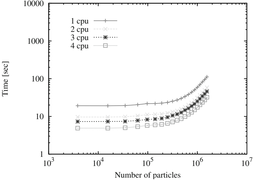
Fig. 5. Log-log plot of the total execution time of the FMM parallel algorithm for fixed parameters (expansion terms p = 17 , and FMM tree level l = 8 ) vs. problem size (number of particles in the system). In the figure, each line represents the total amount of time used by the parallel FMM to compute the interaction in the system when using 1, 2, 3, and 4 processors.
