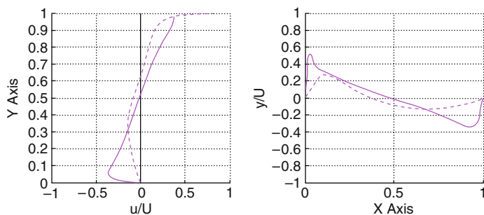
Fig. 3. Identical LB and Fluent solutions for flow in a lid-driven square cavity; Re = 10000 , 512 \times 512 uniform grids, Newtonian fluid ( n = 1 ).
