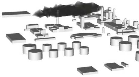
Fig. 5. Pollutant plume around buildings ( 1.5 \times 10^5 cells)
