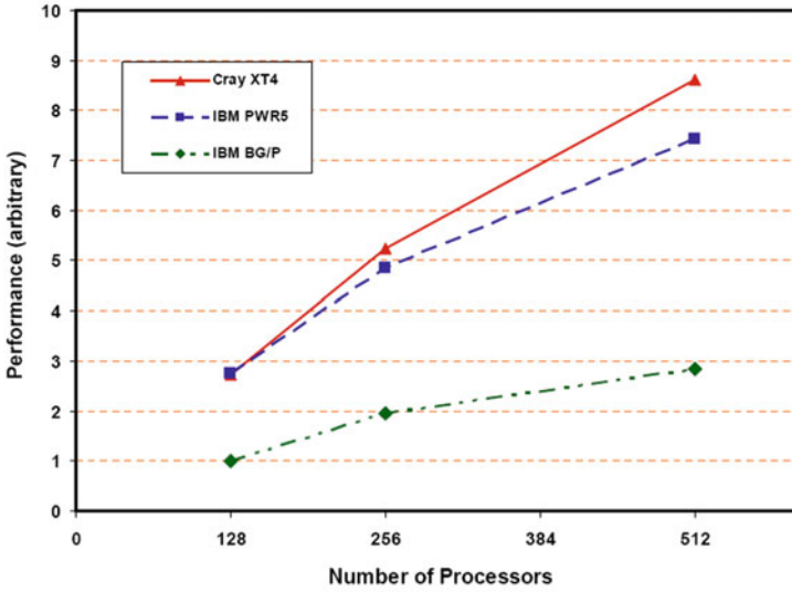
Fig. 3. Performance of STREAMS-LES on high-end systems.
