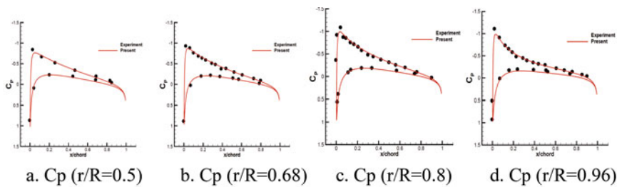
Fig. 5. Pressure coefficient of rotor blades in hover flight
