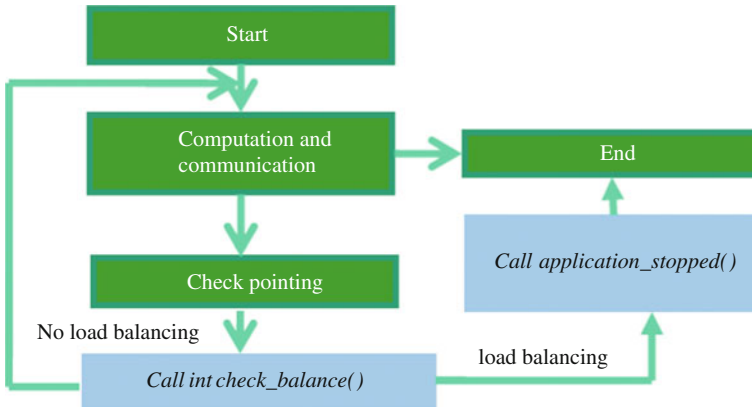
Fig. 1. Inserting profiling library function into application code.
