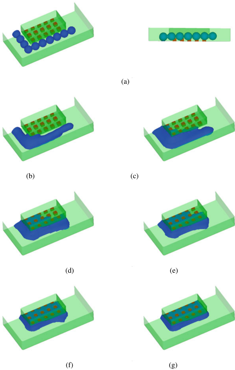
Fig. 5. The initial state of dispensing a sequence of spherical liquids (a), the histories of propagating interface with increasing the time (b)-(f) and the final fillet shape (g) in the existence of solder bumps (case3)
