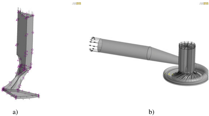
Fig. 1. Problem setup a) single passage b) full machine with volute
