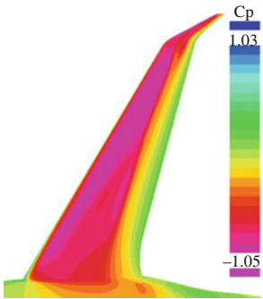
Fig. 2. Generic business jet. Pressure distribution for wing-body configuration: original geometry.
