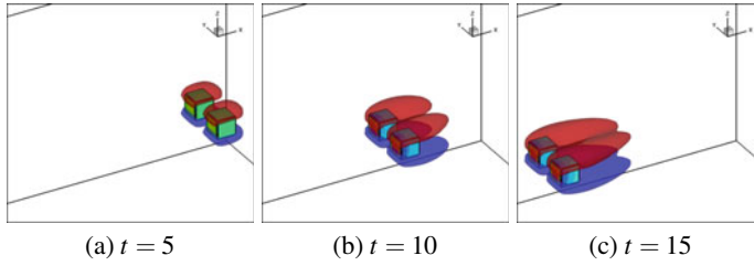
Fig. 7. Surface pressure distribution and vorticity contour.
