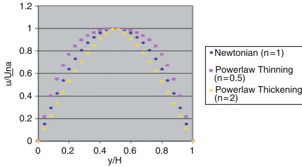
Fig. 5. Velocity profiles at the exit of the microchannel with no slip boundary condition.
