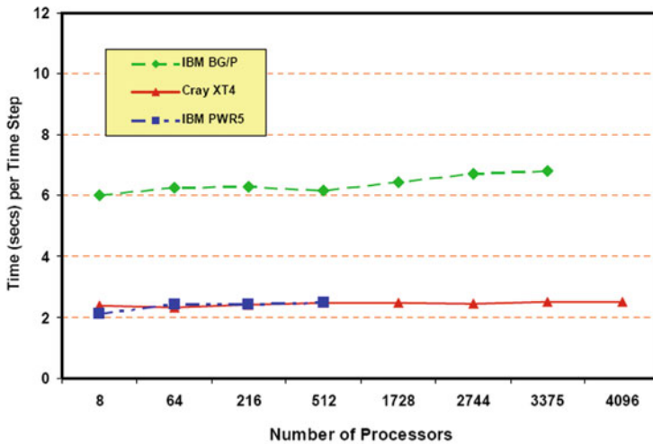
Fig. 6. Weak scaling performance of Senga2-4 Step reduced-air methane mechanism 32^3 grid points per processor.
