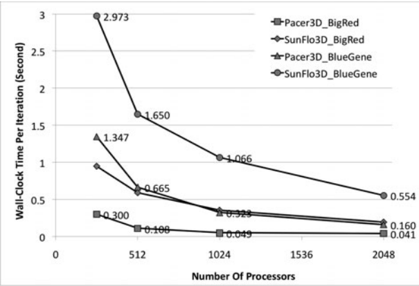
Fig. 2. Timing comparison of the solvers on two parallel computing platforms
