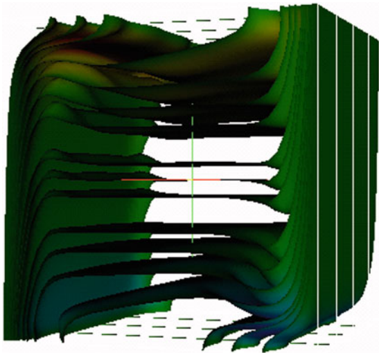
Fig. 3. Isotherms at Ra = 10^6 . The domain in y direction is divided into 4 subdomains.
