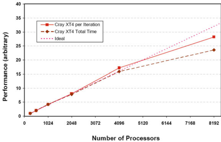
Fig. 5. Performance of Code_Saturne for a 100M cell "Mixing Grid" dataset on Hector (Cray XT4).
