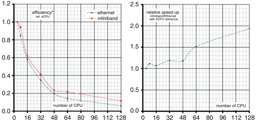
Fig. 4. Results on 100 iterations, left: efficiency; right: gain on speed-up computed as in equation (1).
