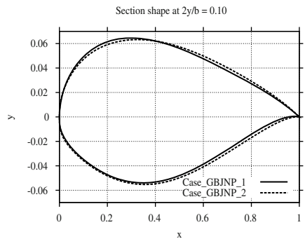
Fig. 10. Generic business jet. Wing sectional shape at 2y/b = 0.10 . Case_GBJNP_1 vs. Case_GBJNP_2 .
