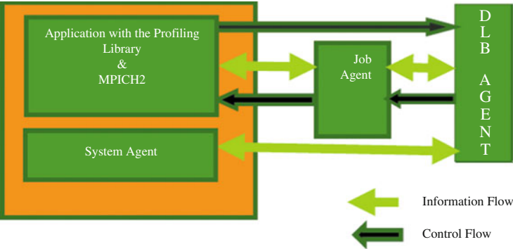
Fig. 2. The components of DLB.
