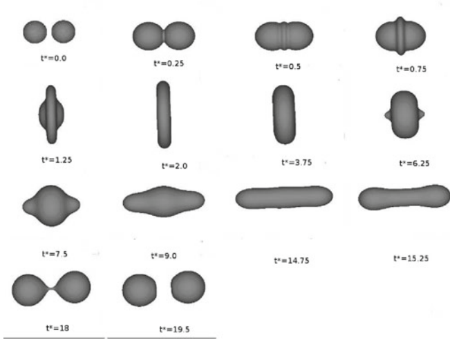
Fig. 5. Simulation of case g from [12]. The nondimensional time is t^* = tU/2R
