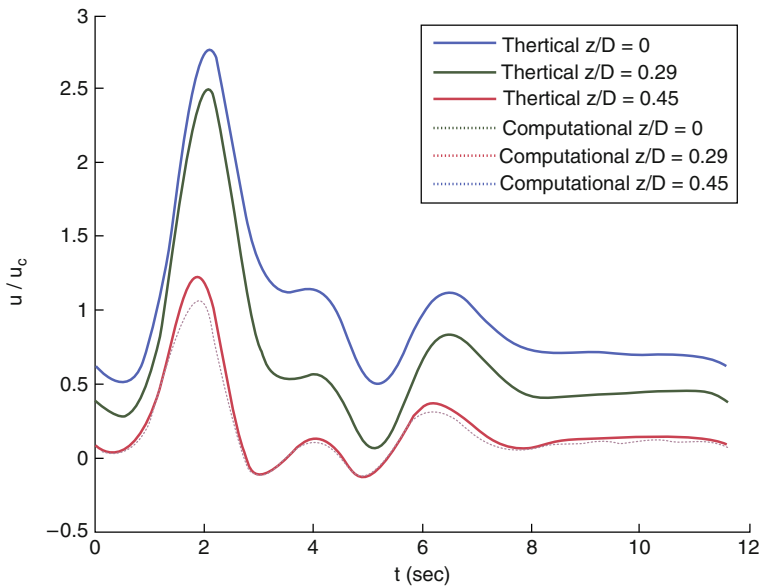
Fig. 2. Comparison of computed and theoretical Womersley solution for velocity at various radial locations.
