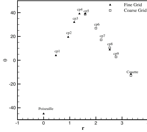
Fig. 3. Angles between vortex cores near the top corners
