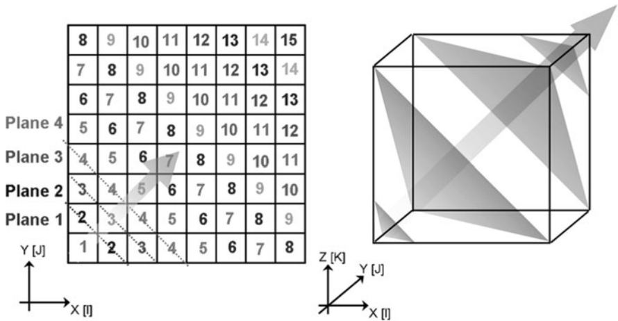
Fig. 3. Schematics of hyper-plane and traveling direction in 2D and 3D
