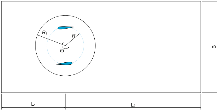
Fig. 2. Domain geometry. L_1 = 2B = 30R , R_1 = 2R , L_2 = 50R .
