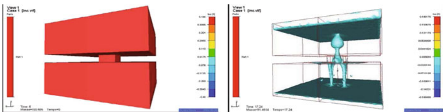
Fig. 3. simulation of jerrican poor: sequences at t=0s (left) and t=18s (right)
