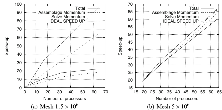
Fig. 4. Speed up performance of Navier Stokes solver
