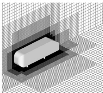
Fig. 8. Mesh cells around the body
