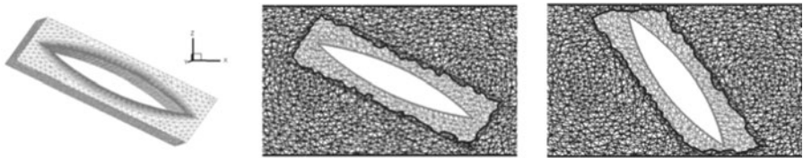
Fig. 4. Valve viscous mesh at 30 degrees and overset mesh at 30 and 60 degrees
