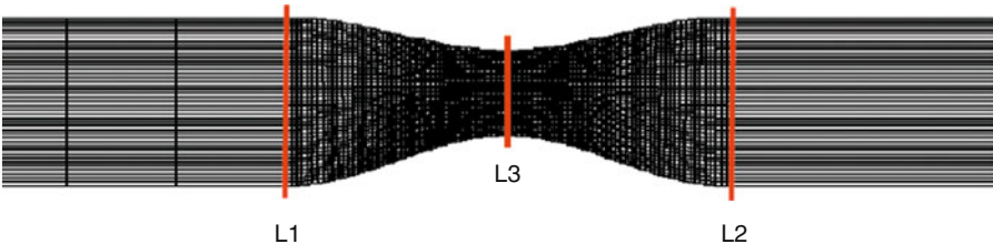
Fig. 6. Axisymmetric stenosis (Equation 2) with specific locations at which pressure was computed.
