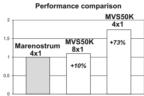
Fig. 3. Performance comparison of MareNostrum and MVS-50000 on a relatively small parallel task
