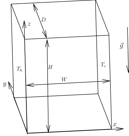
Fig. 1. Configuration of a differentially heated cavity. The vertical walls at x = 0 and W are submitted to a temperature difference \Delta T = T_h - T_c and other walls are adiabatic.
