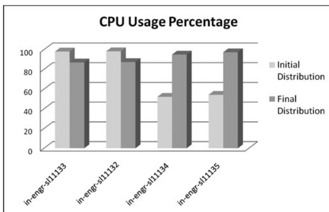
Fig. 3. Comparison of CPU usage percentage between initial load distribution and DLB suggested balanced load distribution.
