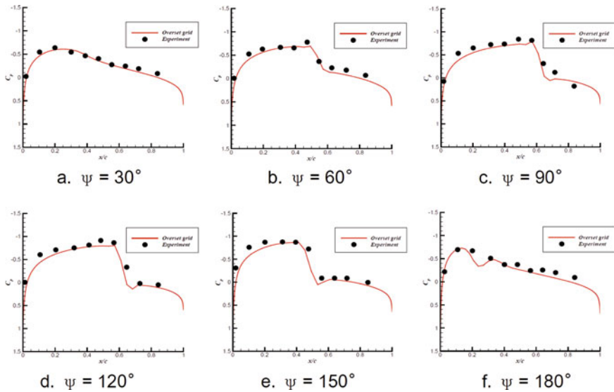
Fig. 7. Pressure coefficient at 0.8925 of span location ( r/R )
