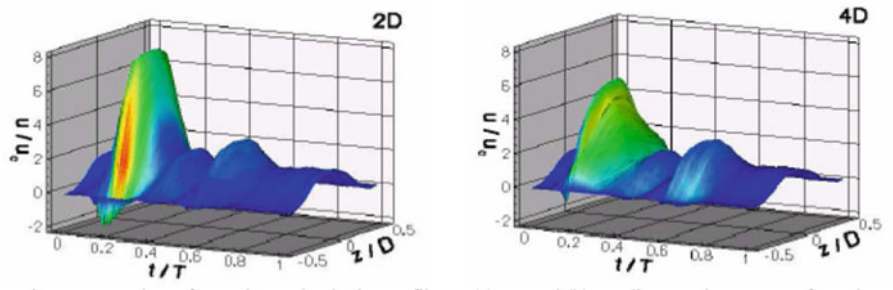
Fig. 5. 3D plots of experimental velocity profiles at (a) 2D and (b) 4D distance downstream from the beginning of the stenosis given by equation (2).
