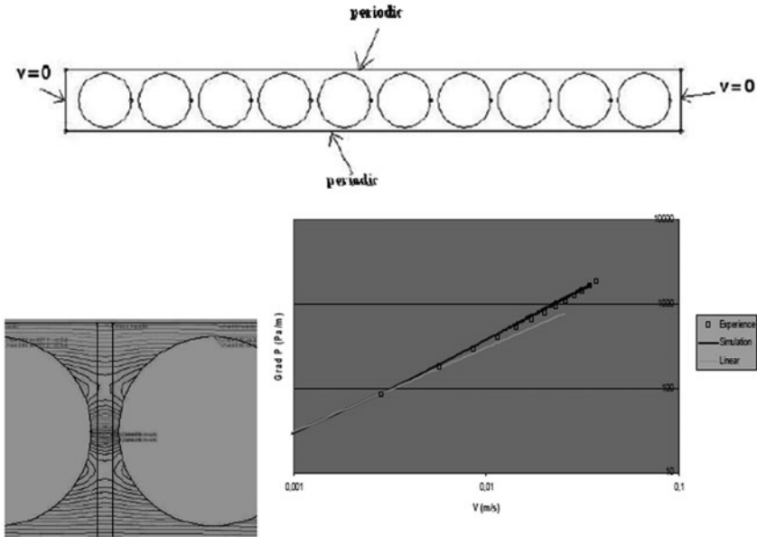
Fig. 3. Flow through cylinders. Computational domain, decomposed domain, numerical results: detail of iso-pressures, curve velocity/gradient of pressure (Experiment and simulation).
