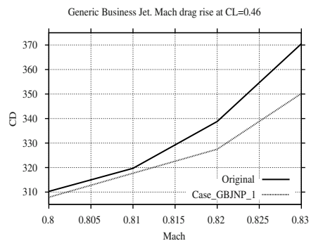
Fig. 5. Generic business jet. Mach drag divergence curve for full aircraft configuration. Original wing vs. optimal one ( Case_GBJNP_1 ).
