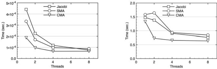
Fig. 4. Timing for in-cache size (NX = 33, left) and out-of-cache size (NX = 513) against number of threads. Vertical and horizontal axes indicate time and number of threads, respectively. In all cases, the CMA code shows the best performance.
