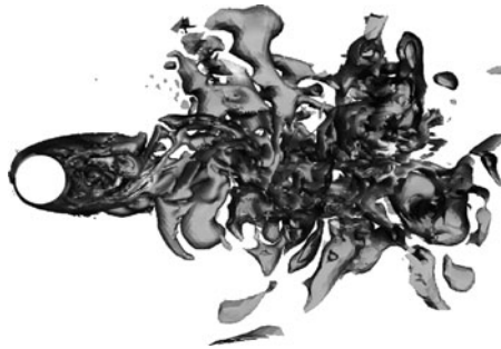
Fig. 1. Snapshot of the vorticity isosurfaces of periodic component for flow past circular cylinder at Re = 1 \times 10^4 .
