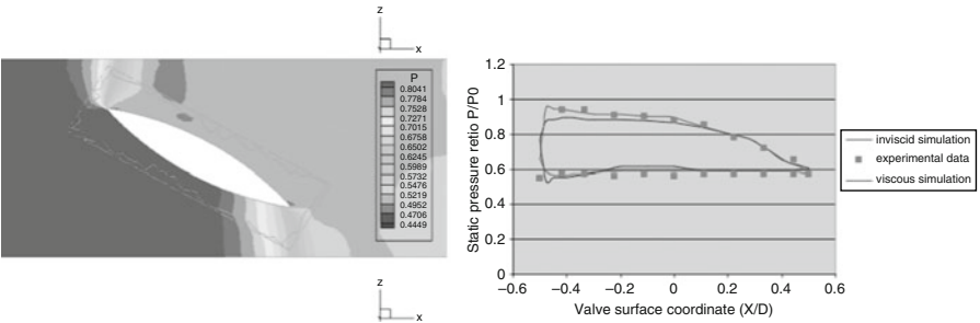
Fig. 5. Pressure contours and comparison with the experiment at 30 degrees of valve position
