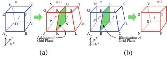
Fig. 3. Control volumes for (a) adding grid plane and (b) eliminating grid plane.
