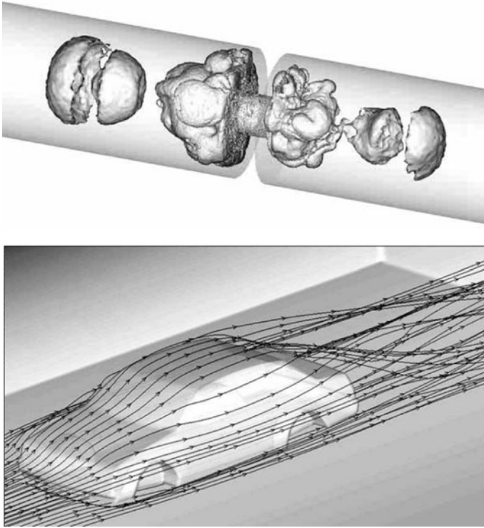
Fig. 4. Illustrative DNS snapshots. Turbulence in a resonator chamber, mesh 10^6 nodes (top); flow around a car body, mesh 2 \times 10^8 (bottom)
