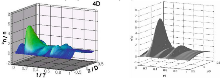
Fig. 13. Experimental (left) and numerical (right) velocity profiles at distance 4D downstream from the beginning of the stenosis along the asymmetric y -axis.
