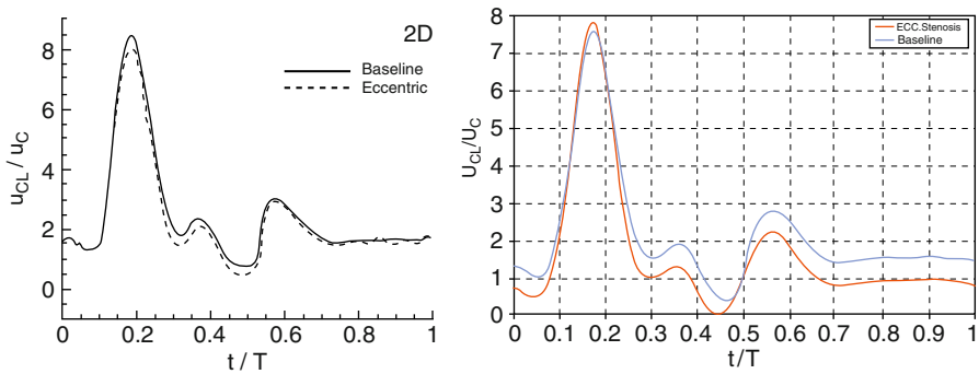
Fig. 14. Experimental (left) and numerical simulation (right) comparison of the jet centerline velocity in the eccentric stenosis at 2D downstream; the baseline case is for the axisymmetric stenosis.
