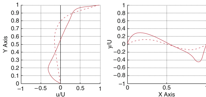
Fig. 2. Identical LB and Fluent solutions for flow in a lid-driven square cavity; Re = 1000 , 128 \times 128 uniform grid, solid line: Newtonian fluid ( n = 1 ), dashed line: Power law fluid ( n = 0.5 ).
