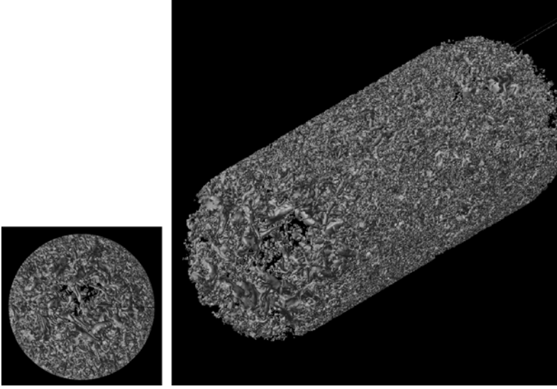
Fig. 5. Second invariant contour surface of velocity tensor of single-phase turbulent flow in a pipe Re=78,000 , 7,200 Mega grids, 2 Tera Bytes
