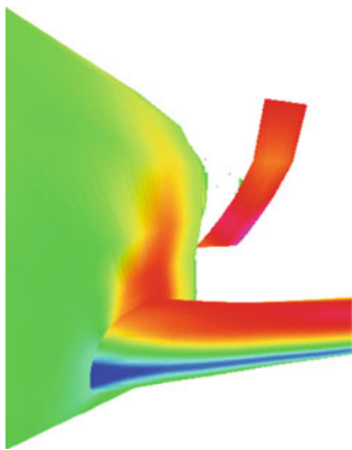
Fig. 6. General view of a generic business jet: computational model.
