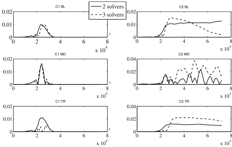
Fig. 2. Relative error in time compared to the reference solution at individual sample points: 2-solver and 3-solver solution compared to the reference solution
