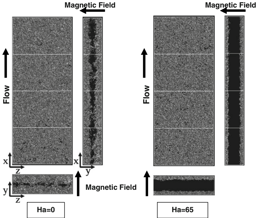
Fig. 6. Magnetic field effect on turbulent flow in a parallel channel: Second invariant contour of velocity tensor
