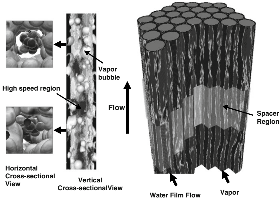
Fig. 4. Predicted vapor structure around fuel rods; black region indicates the water (void fraction is 0), and light grey region indicates an interface between water and vapor which means the void fraction is in between 0 and 1.
