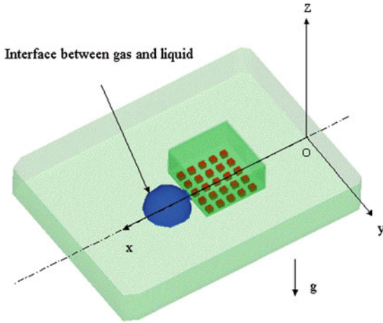
Fig. 2. The analytical model for the conventional capillary flow type
