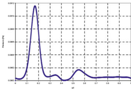
Fig. 7. Average pressure at location L1 upstream of the stenosis.
