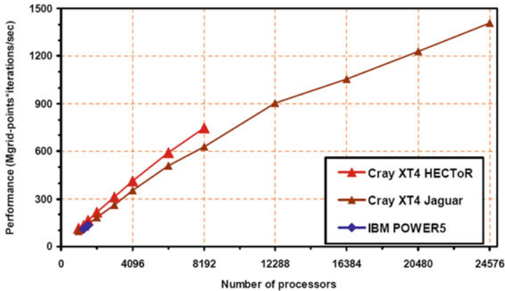
Fig. 2. Performance of SBLI on the HECToR, jaguar and HPCx systems for the 1024^3 grid size.
