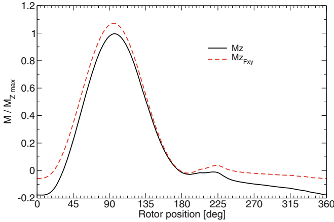
Fig. 5. The effect of the pitching moment, \lambda = 2.5 .
