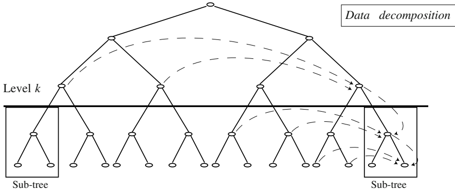
Fig. 3. Sketch to illustrate the parallelization strategy. The image depicts the FMM algorithm as a tree, this tree is then “cut” at a chosen level k , and all the resulting sub-trees are distributed among the available processes.
