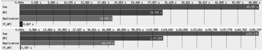
Fig. 3. Timing for Pacer3D and SunFlo3D flow solvers for 100 time steps obtained by Vampir tool, respectively
