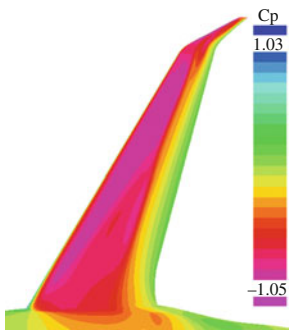
Fig. 7. Generic business jet. Pressure distribution for full aircraft configuration: Case_GBJNP_2 .
