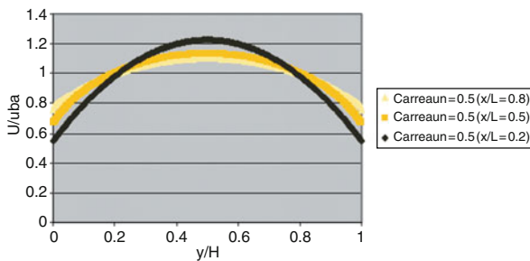
Fig. 8. LB Velocity profiles at the exit of the microchannel for Carreau-Yasuda shear-thinning fluid.
