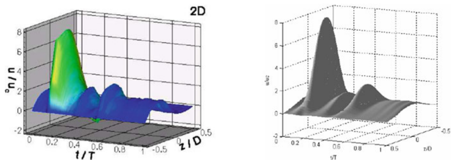
Fig. 11. Experimental (left) and numerical (right) velocity profiles at distance 2D downstream from the beginning of the stenosis along the asymmetric y - axis.
