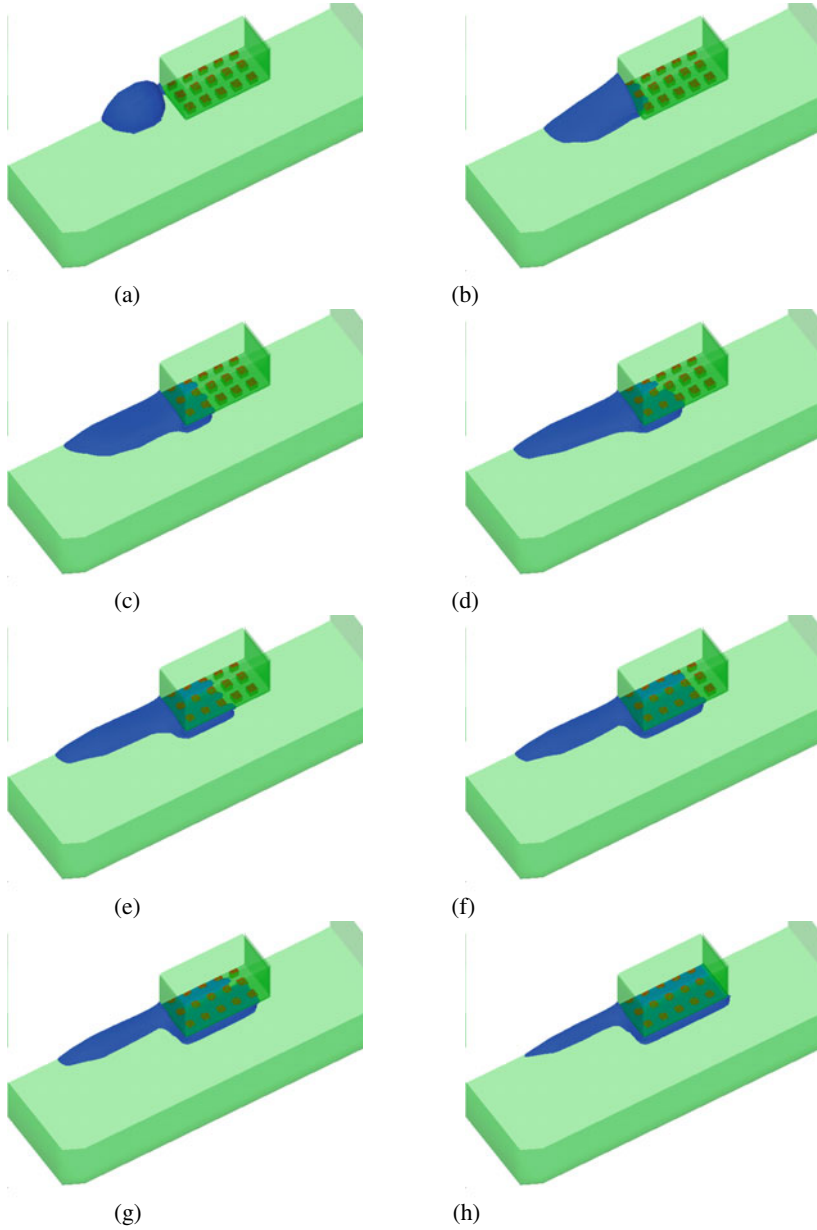
Fig. 4. The initial state of dispensing a semi-spherical liquid (a), the histories of propagating interface with increasing the time (b)-(g) and the final fillet shape (h) in the existence of solder bumps (case2)
