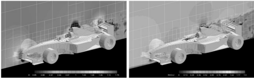
Fig. 6. Instantaneous pressure and velocity field
