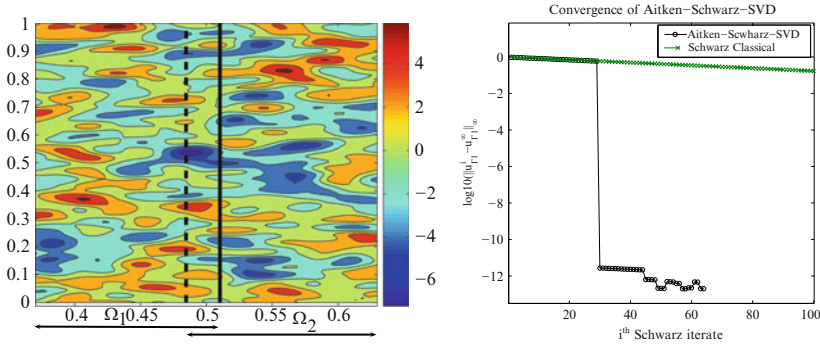
Fig. 1. Schwarz DDM accelerated by the Aitken SVD procedure: (left) random distribution of K along the interfaces, (right) the convergence of the Aitken-Schwarz
