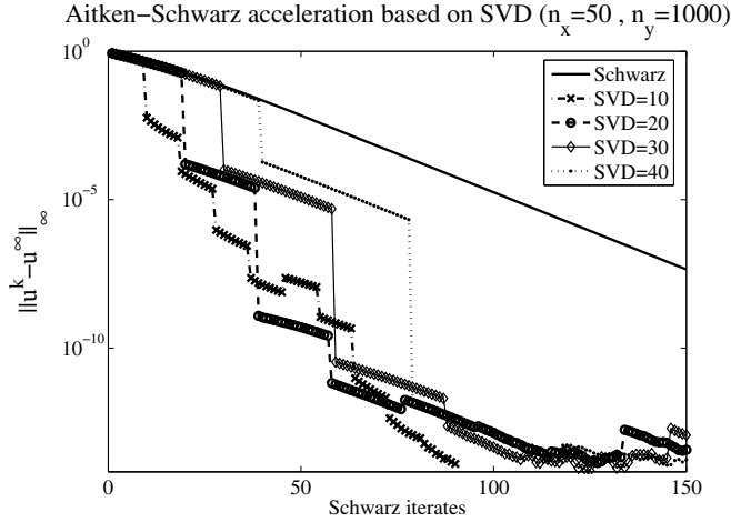
Fig. 2. Convergence of Aitken-Schwarz with respect to the number of iterates in the SVD
