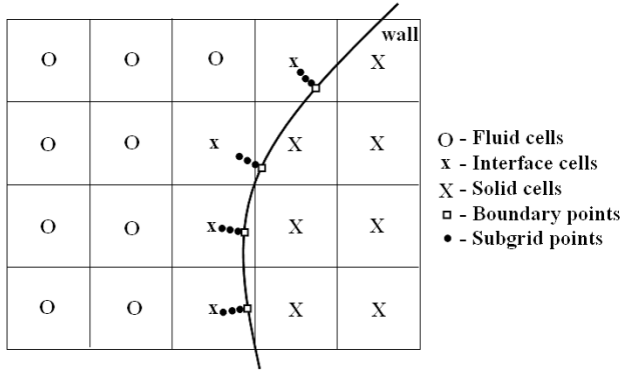
Fig. 4. Nodal assignment for boundary conditions with Subgrid
