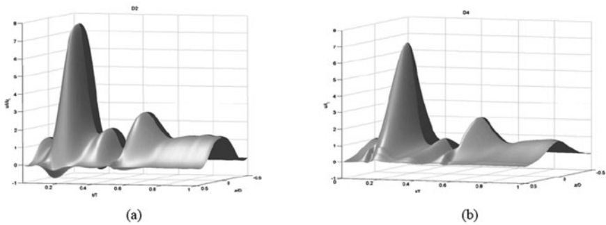
Fig. 4. 3D plots of computed velocity profiles at (a) 2D and (b) 4D distance downstream from the beginning of the stenosis given by equation (2).
