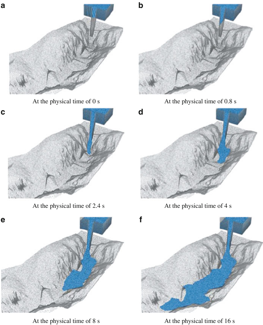
Fig. 8. Snapshots of the simulated flow at different physical time.
