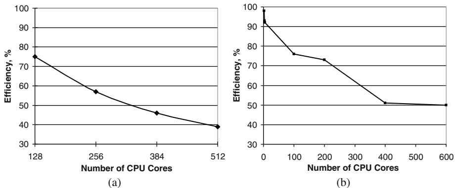
Fig. 3. Parallelization efficiency for 10^6 nodes task, 1 MPI process per core on “SKIF MSU” (a) and efficiency for 2 \cdot 10^6 nodes, 1 MPI process per core on “MVS-100k” (b)
