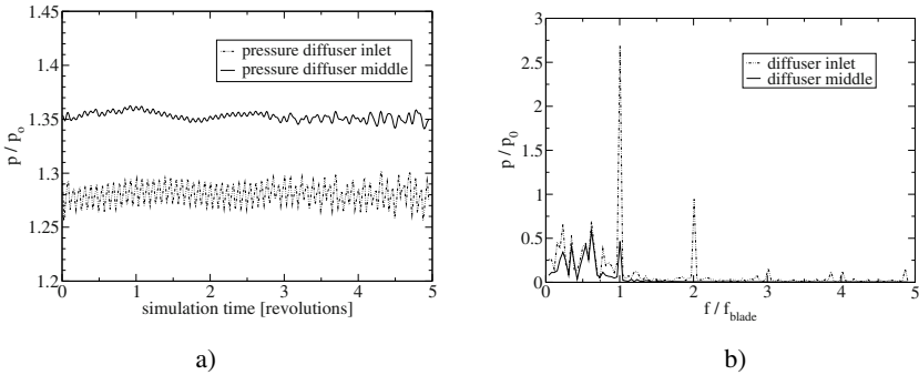
Fig. 2. Simulated pressure at two locations, a) variation in time b) FFT transformed signal
