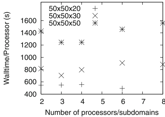
Fig. 2. Walltime per subdomain (or processor) for different spatial resolution. The domain in z direction is divided into subdomains.
