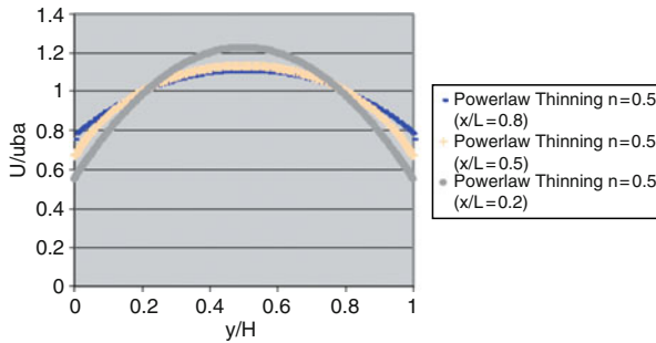
Fig. 7. LB Velocity profiles at the exit of the microchannel for power law shear-thinning fluid.
