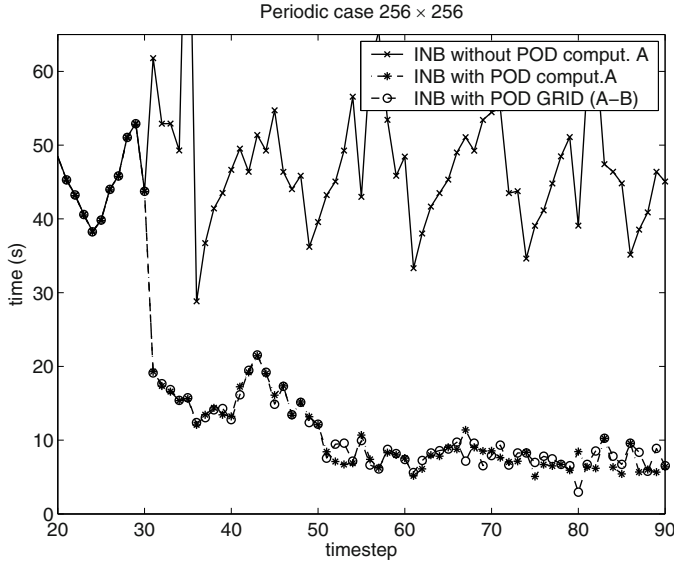
Fig. 2. Elapsed time of GRID computation A-B and computation on homogeneous parallel computer A.
