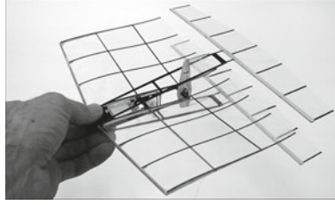
Fig. 1. Flapping-wing MAV model
