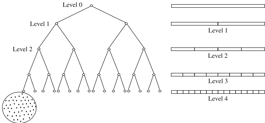
Fig. 1. Sketch of a one-dimensional domain (right), divided hierarchically using a binary tree (left), to illustrate the meaning of levels in a tree and the idea of a final leaf holding a set of particles at the deepest level.
