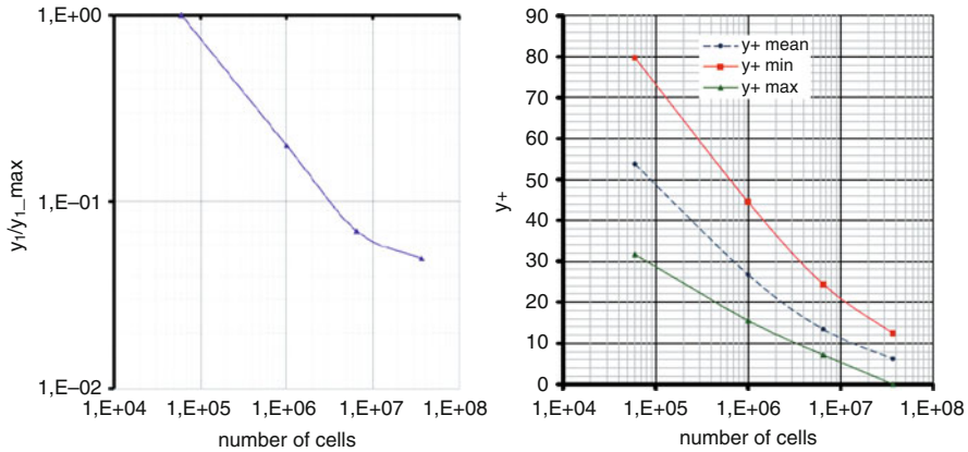
Fig. 6. left: first cell-centre-height of each mesh divided by the first cell-centre-height of the coarser mesh of 0.06 million cells are plotted versus the overall mesh size; right: maximum, minimum and average y^+ values computed at the last iteration stage and collected from the cells of the asymmetrical spinnaker at 1/3 height of the yacht model from the water-plane are plotted versus the overall mesh size.
