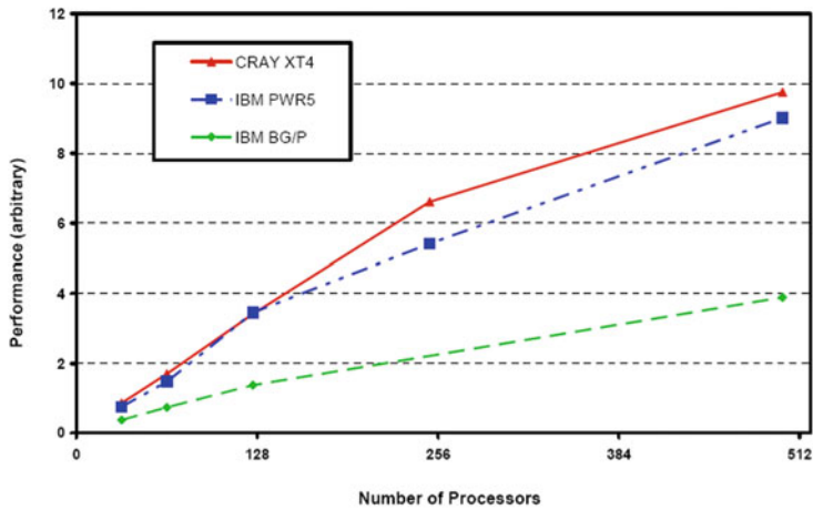
Fig. 7. Strong scaling performance of Senga2-1 Step Arrhenius-type Mechanism with 500 3 global grid points.
