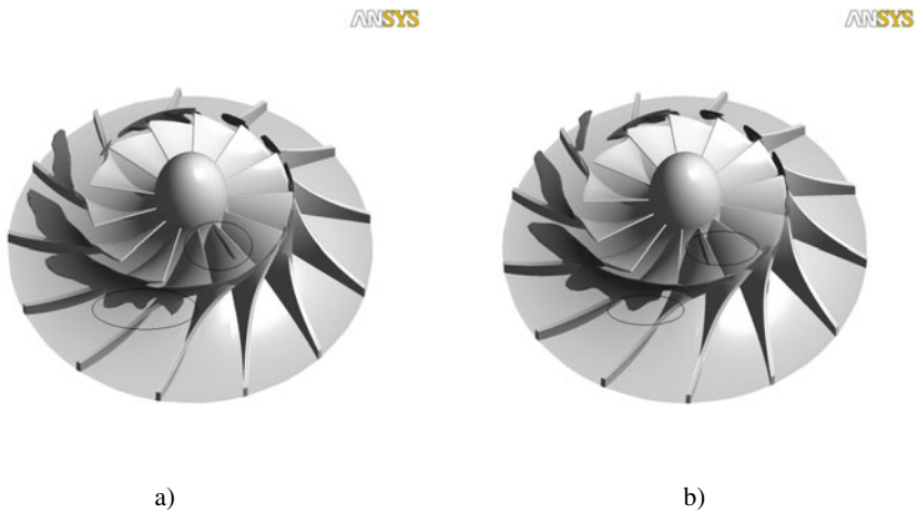
Fig. 3. Travelling rotating stall cells displayed as negative streamwise velocity, a) and b) two different time steps
