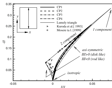
Fig. 4. Anisotropy invariant map - cases CP1-CP4
