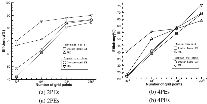
Figure 2. Parallel efficiency of test problem.
