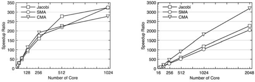
Fig. 5. Comparison of performance on Core2Duo cluster. Intel Compiler 10.1, option O3 was used. The left figure shows the scalability based on elapsed time. The right figure shows the scalability based on only calculation time. CMA indicates super-linear behavior and the other methods show good scalability.
