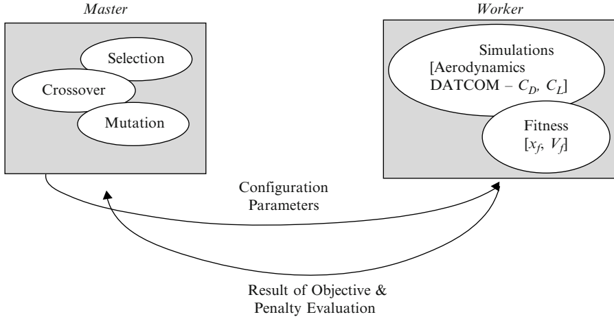
Fig. 2. Illustration of an overall solution flow where the master acts as the genetic engine and each worker calculates the fitness values.
