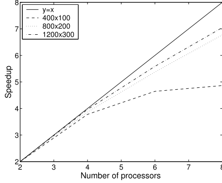
Fig. 1. Speedup of the flow solver with respect to the number of processors and for three different domain sizes
