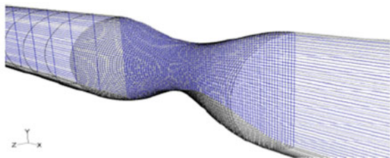
Fig. 9. Geometry of the stenosed asymmetric phantom [7].
