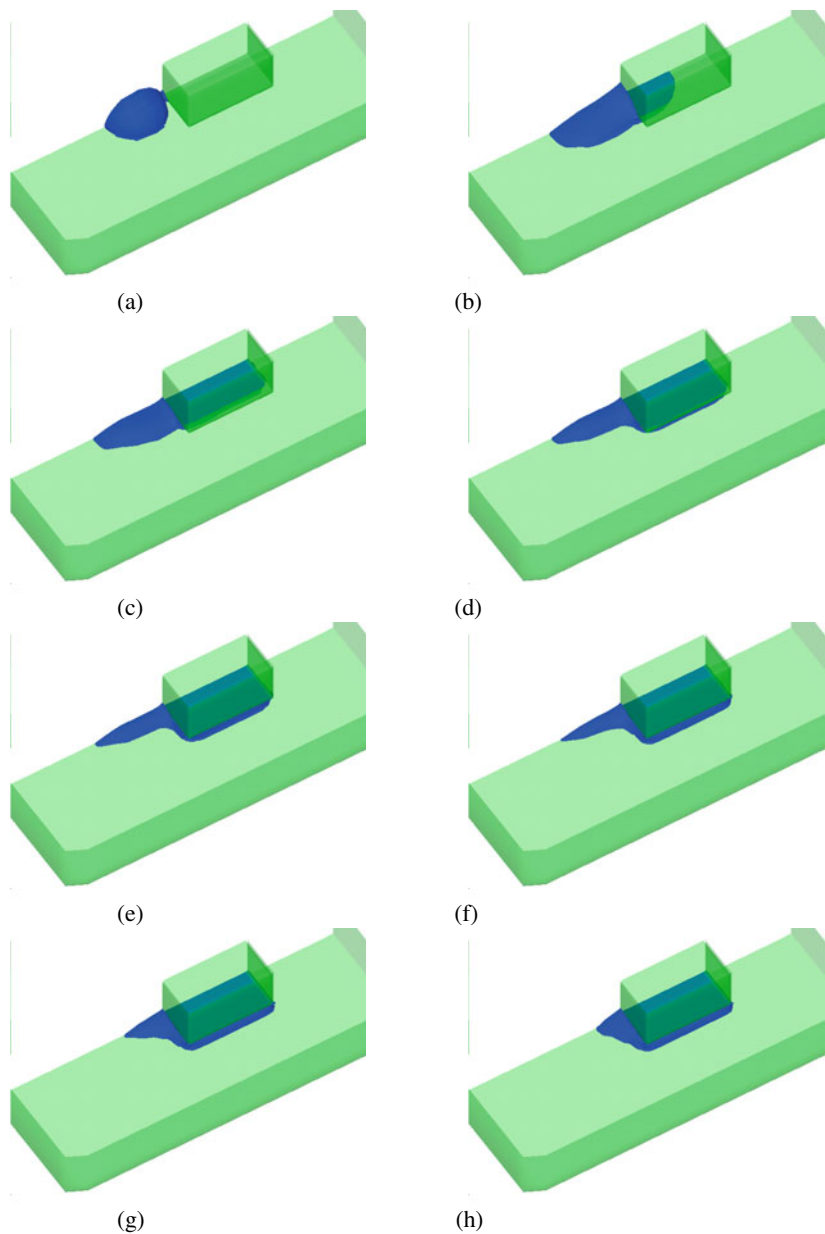
Fig. 3. The initial state of dispensing a semi-spherical liquid (a), the histories of propagating interface with increasing the time (b)-(g) and the final fillet shape (h) in the existence of no solder bumps (case1)
