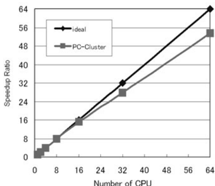
Fig. 6. Scalability test on the Opteron computer
