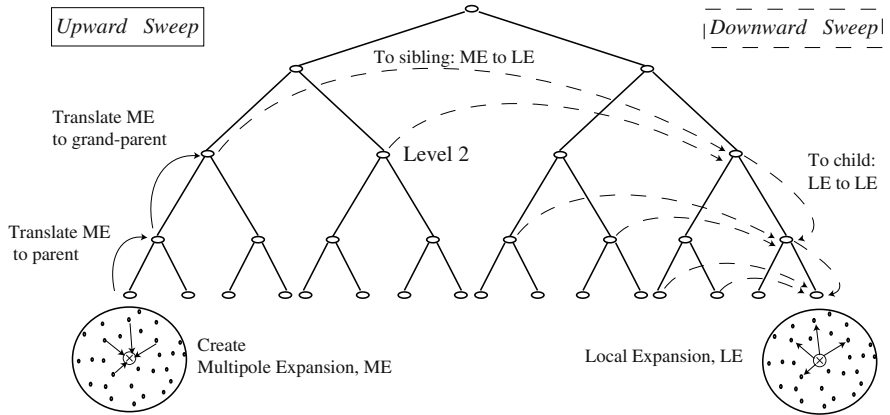
Fig. 2. Illustration of the upward sweep and the downward sweep of the tree. The multipole expansions (ME) are created at the deepest level, then translated upwards to the center of the parent cells. The MEs are then translated to a local expansion (LE) for the siblings at all levels deeper than level 2, and then translated downward to children cells. Finally, the LEs are created at the deepest levels.
