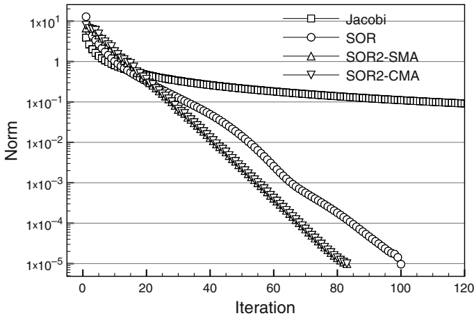
Fig. 2. Convergence history for several iterative methods against norm defined by Equation (2).
