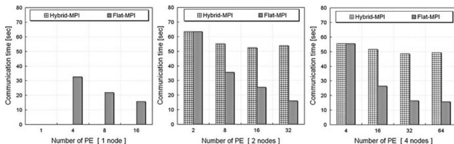
Fig. 8. Communication time
