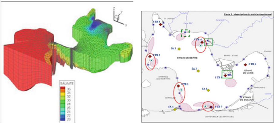
Fig. 3. Berre lake (right) and its Telemac-3D modeling (left).
