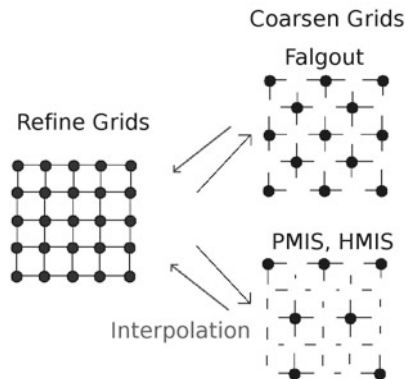
Fig. 1. Coarsening schemes and interpolation
