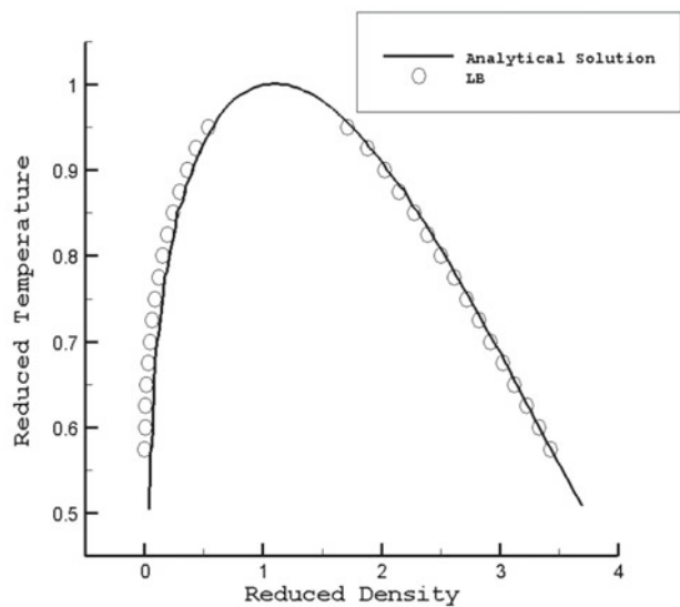
Fig. 2. Comparison between coexistence curve obtained from simulation and theoretical one relative to the CS-EOS.
