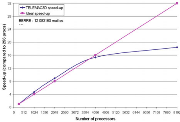
Fig. 5. Telemac-3D speed-up.
