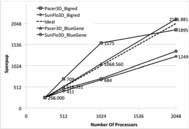
Fig. 1. Speedup of the solvers on two computing platforms
