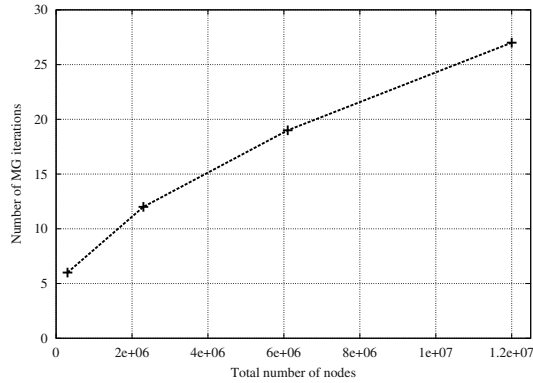
Fig. 2. Scalability test: number of MG iterations with mesh growth
