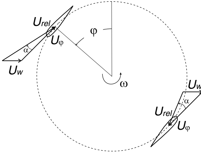
Fig. 1. Definition of Coordinate Systems and velocities.
