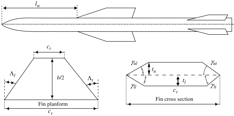
Fig. 1. Airframe geometry.
