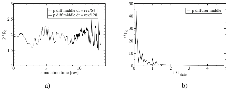
Fig. 4. a) Pressure history during rotating stall b) FFT transformed signal
