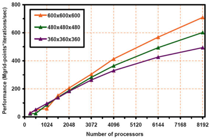
Fig. 1. Performance of SBLI on up to 8192 processors of the HECToR Cray XT4 for three grid sizes.
