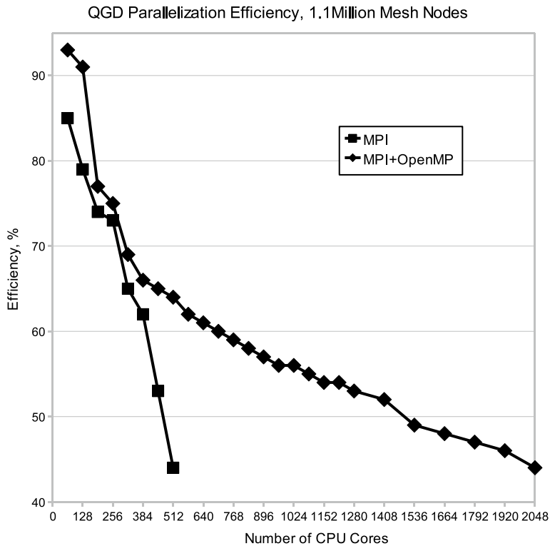
Fig. 4. Comparison of pure MPI parallelization efficiency with hybrid MPI+OpenMP approach (“MVS-100k”)
