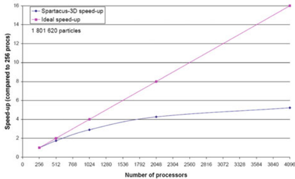
Fig. 6. Spartacus-3D speed-up.
