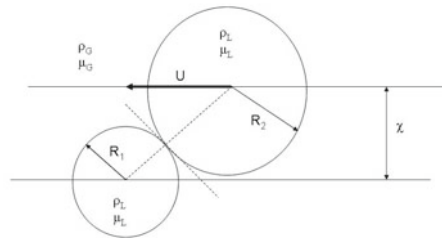
Fig. 1. Physical and geometrical parameters characterizing binary droplet collision.
