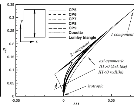
Fig. 5. Anisotropy invariant map - cases CP5-CP9
