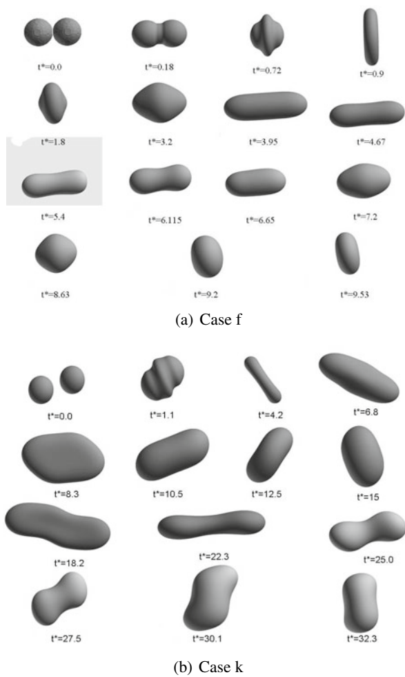
Fig. 4. Simulations of cases relative to Regime III from [12]. The nondimensional time is t^* = tU/2R
