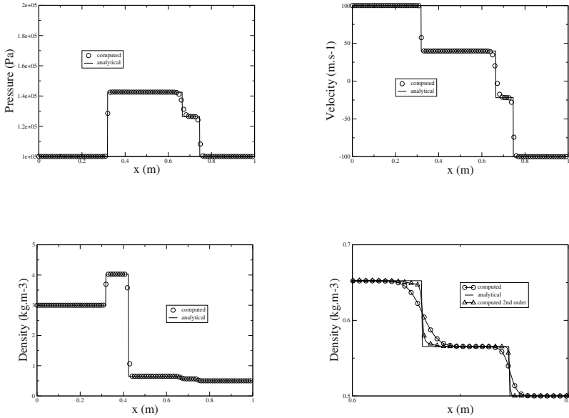
Fig. 3. Comparison of the numerical solution obtained and the analytical one for a shock splitting, for density, pressure and velocity. The last figure is a zoom on the split shock, in which we compare the first and second order computed solutions.
