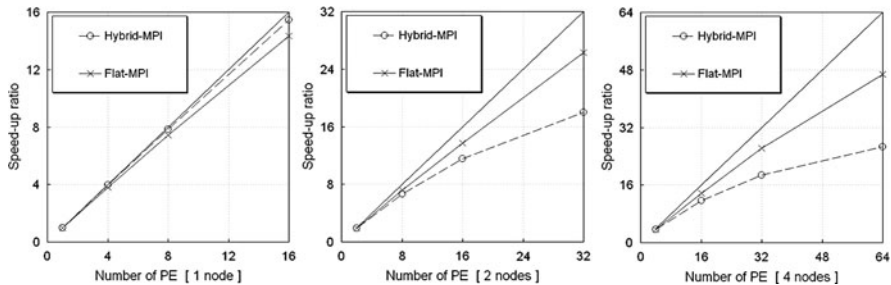
Fig. 7. Speed-up ratio
