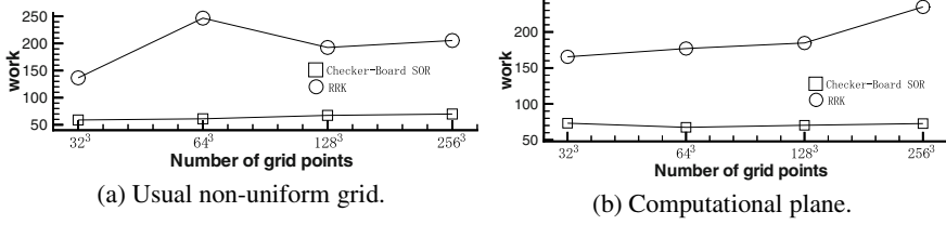
Figure 1. Multigrid property on non-uniform grid.
