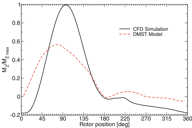
Fig. 4. Normalized moment of the single airfoil with respect to the rotor position. \lambda = 2.5
