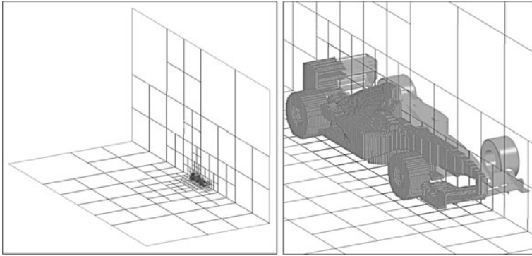
Fig. 1. Example of computational mesh around formula-1 car
