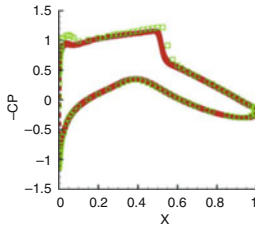
Fig. 7. Comparison of computed surface pressure coefficient with experimental data.
