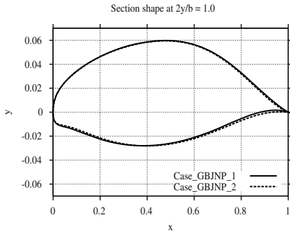
Fig. 12. Generic business jet. Wing sectional shape at 2y/b = 1.0 . Case_GBJNP_1 vs. Case_GBJNP_2 .
