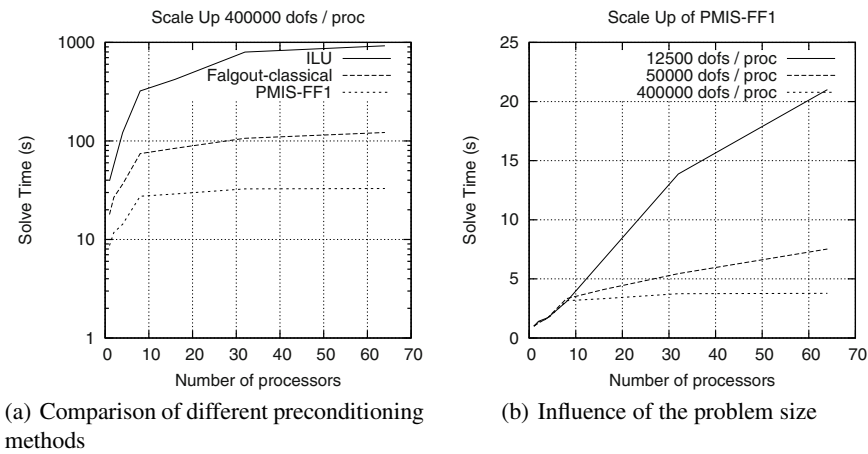
Fig. 3. Scale up Results on a Laplace equation
