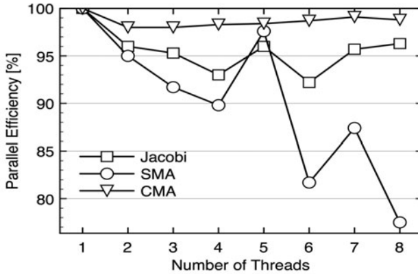
Fig. 3. Efficiency of thread parallelization on a Cray C90.
