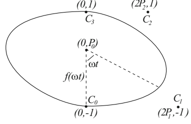
Fig. 3. Flapping path defined by a 3 rd degree NURBS
