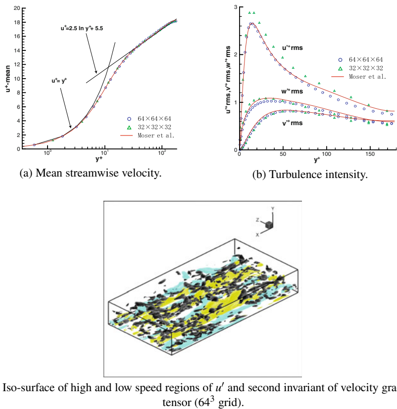
Figure 3. Statistical quantities and instantaneous flow field.
