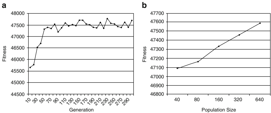
Fig. 4. (a) Maximum fitness values achieved at each 10th generation where population size is fixed at 40. (b) Maximum fitness values achieved for different population sizes after 100 generations.
