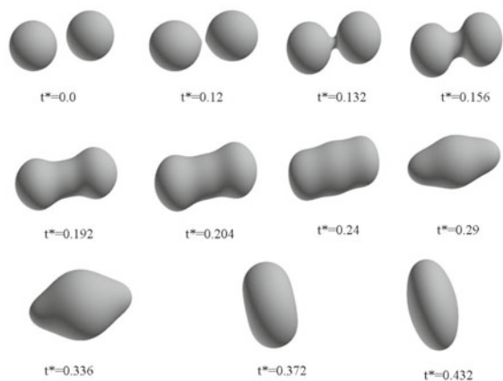
Fig. 3. Simulation of case a from [12]. The nondimensional time is computed as t^* = tU/2R
