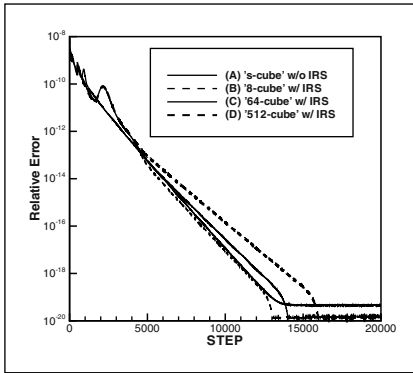
Fig. 12. Convergence history for several cube arrangements w/ IRS.
