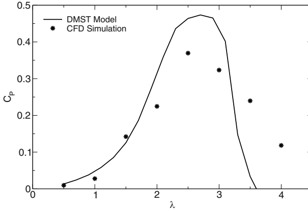
Fig. 3. Power coefficient of the VAWT C_p = P/(\rho U_w^3 HR) . 2D-CFD simulations versus DMST model. For the parameters see table 1.
