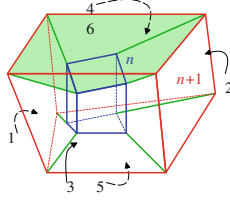
Fig. 1. Schematic view of control volume in (x, y, z, t) space-time unified domain.
