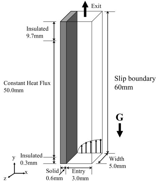
Fig. 1. Computational domain for forced convective flow boiling
