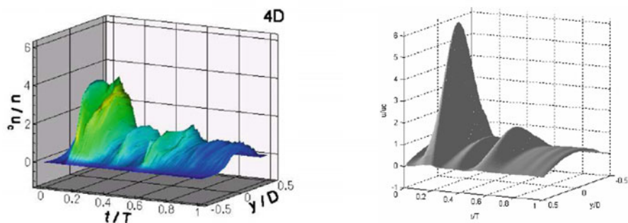
Fig. 12. Experimental (left) and numerical (right) velocity profiles at distance 4D downstream from the beginning of the stenosis along the symmetric z -axis .
