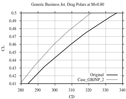
Fig. 8. Generic business jet. Drag polar at M = 0.80 for full aircraft configuration. Original wing vs. optimal one ( Case_GBJNP_2 ).
