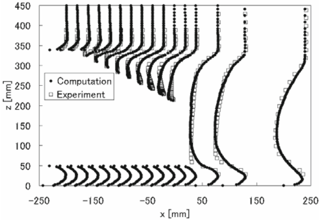
Fig. 10. Mean streamwise velocity profiles at the rear body and near wake on the symmetry plane
