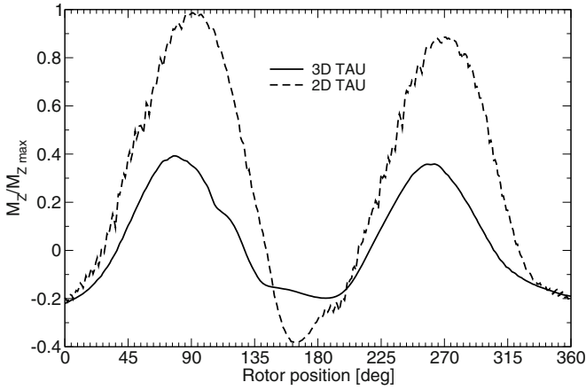
Fig. 6. Normalized resulting moment of the rotor during the second rotor revolution.
