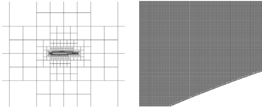
Fig. 1. Cube boundaries around RAE2822 air-foil Fig. 2. Cartesian mesh inside the cube (256x256 cells)
