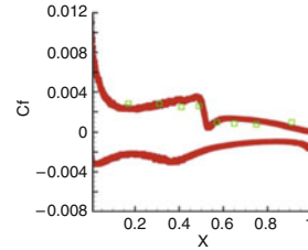
Fig. 8. Comparison of computed skin friction coefficient with experimental data.
