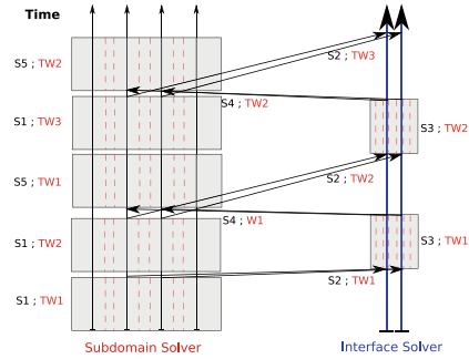
Fig. 2. The Parallel Non Blocking Windowed Approach.
