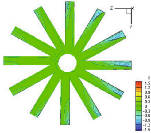
Fig. 6. Pressure coefficient of rotor blades in non-lift forward flight
