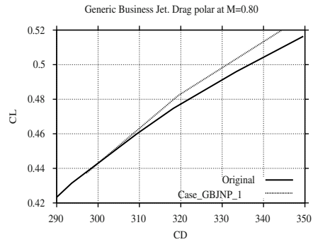
Fig. 4. Generic business jet. Drag polar at M = 0.80 for full aircraft configuration. Original wing vs. optimal one ( Case_GBJNP_1 ).
