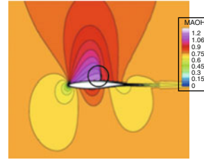
Fig. 6. Mach number contours.
