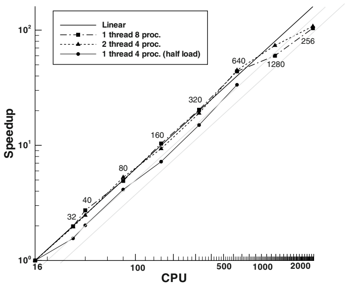
Fig. 2. Comparison of MPI and MPI+OpenMP parallelization in a speedup test using a small mesh
