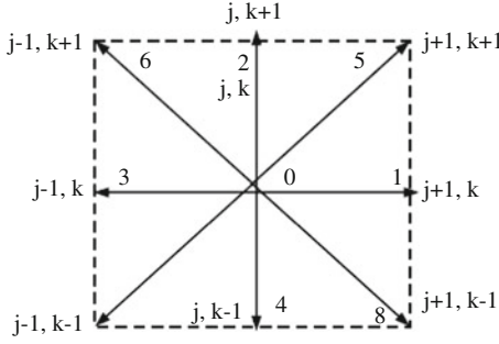
Fig. 1. Nine-Speed Square Lattice.
