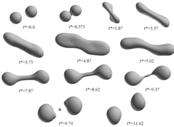
Fig. 6. Simulation of case m from [12]. The nondimensional time is t^* = tU/2R
