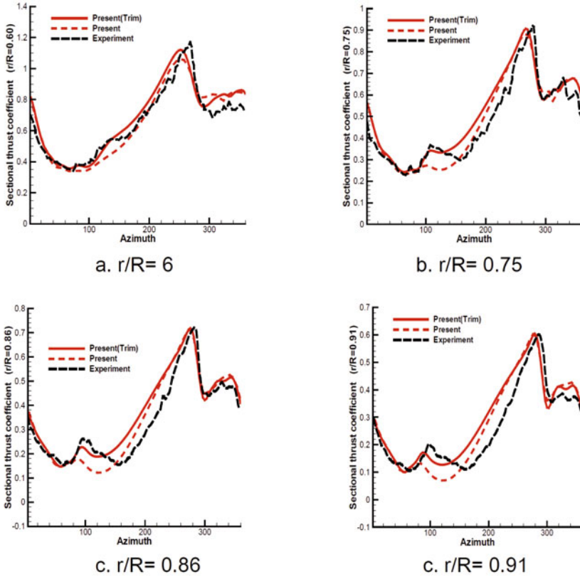
Fig. 8. Sectional Thrust coefficient as Azimuth angle
