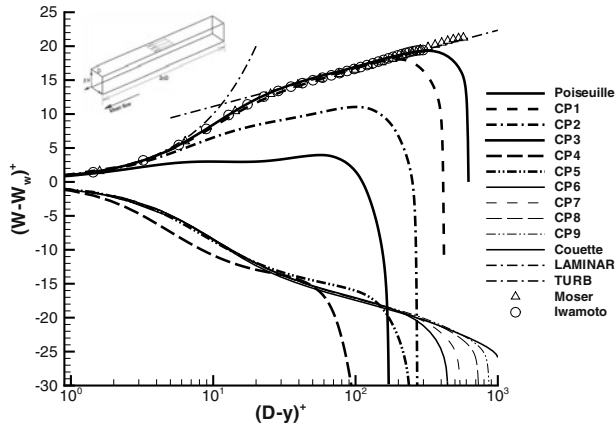
Fig. 1. Geometry and mean streamwise velocity along the wall-bisector.
