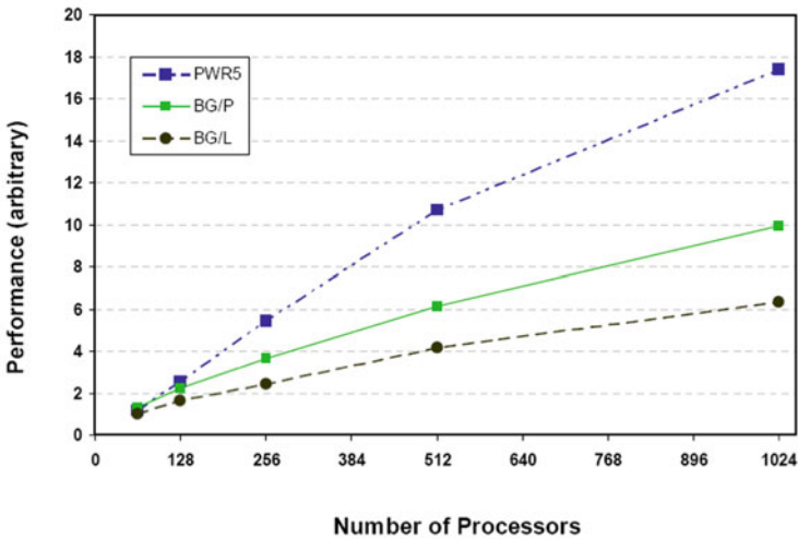
Fig. 4. Performance of Code_Saturne for a 16M cell open channel dataset on IBM platforms.
