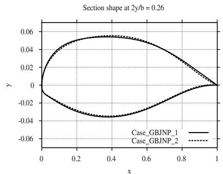
Fig. 11. Generic business jet. Wing sectional shape at 2y/b = 0.26 . Case_GBJNP_1 vs. Case_GBJNP_2 .
