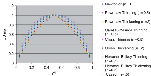
Fig. 4. Velocity profiles at the exit of the microchannel with no slip boundary condition.
