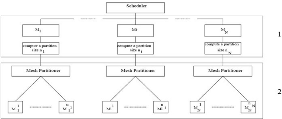
Fig. 1. A diagram of the global multi-mesh partitioning approach
