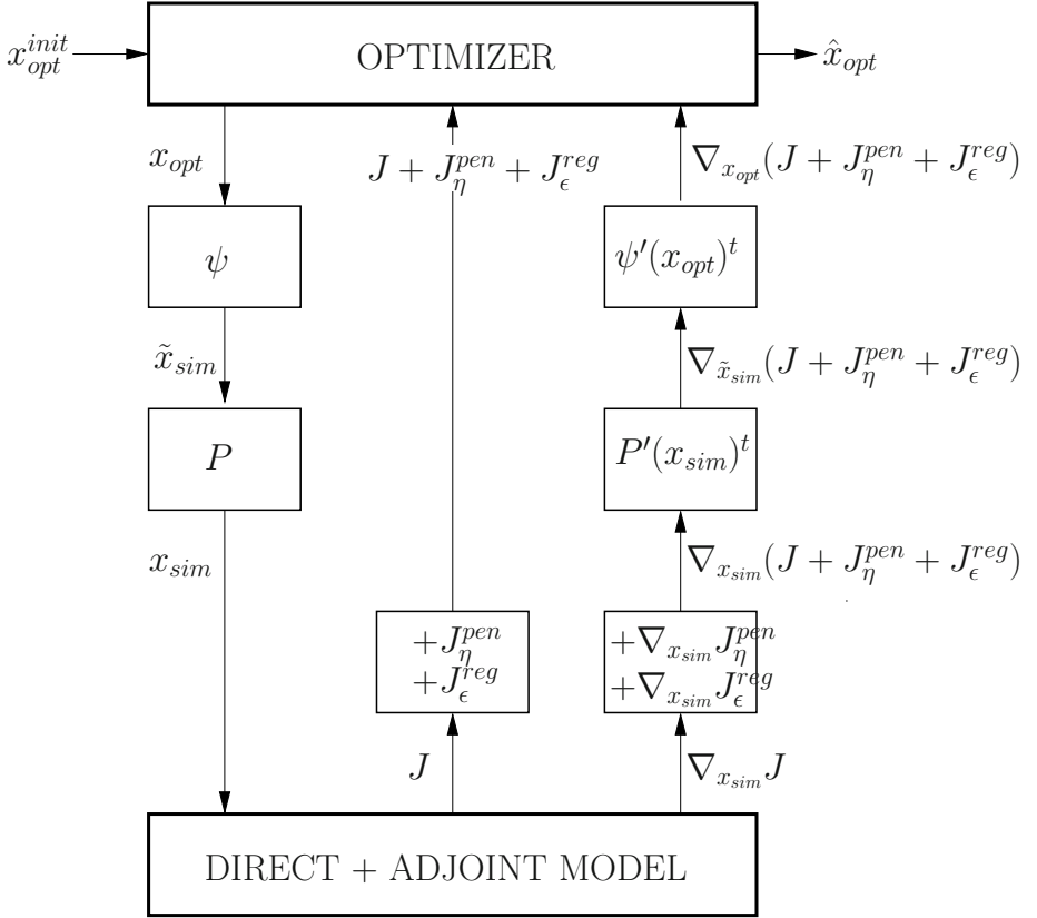
Figure 3.8: Organization of a nonlinear inversion code. Bottom : direct and adjoint simulation code, top : optimization code, \psi : parameterization routine, P : projection on box constraints, \psi'(x_{opt})^t : adjoint parameterization routine, P'(x_{sim})^t : adjoint projection routine
