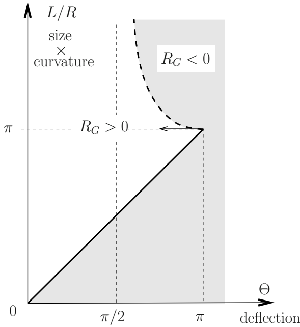
Figure 8.2: The domain of deflection \Theta and size \times curvature product L/R , which ensure strict quasi-convexity of a finite curvature set (D, \mathcal{P}) (extended deflection conditions (8.18) or (8.19))
