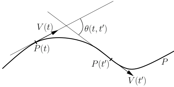
Figure 4.1: The deflection \theta between two points of a curve P
