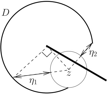
Figure 6.2: Quasi-convex arcs of circle
