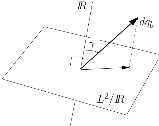
Figure 4.3: The decomposition L^2(\Omega) = L^2(\Omega)/\mathbb{R} \oplus \mathbb{R} and the indetermination angle \gamma
