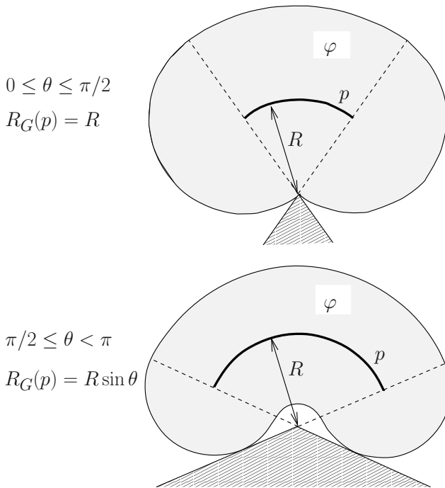
Figure 7.3: Largest regular enlargement s.q.c. neighborhood of size R_G(p) ( in gray ) for paths p made of an arc of circle of radius R and length L = R\theta (the overall largest s.q.c. neighborhoods correspond to the complementary of the dashed areas )
