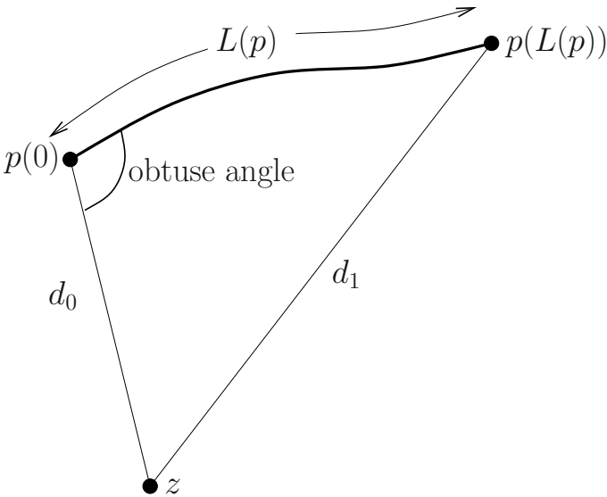
Figure 6.4: Illustration of the obtuse angle lemma
