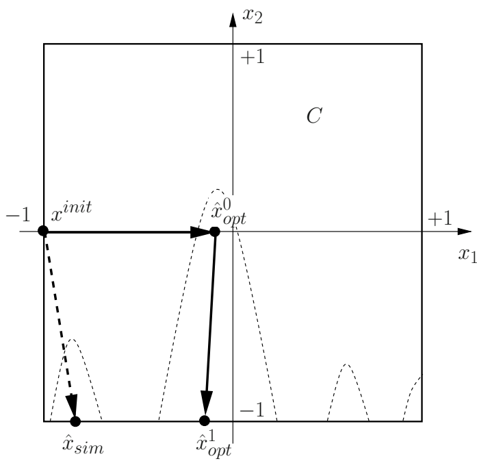
Figure 3.4: Optimization paths in C for the local ( dashed line ) and the multiscale ( full line ) resolution. The thin dashed lines correspond to one level line of the objective function
