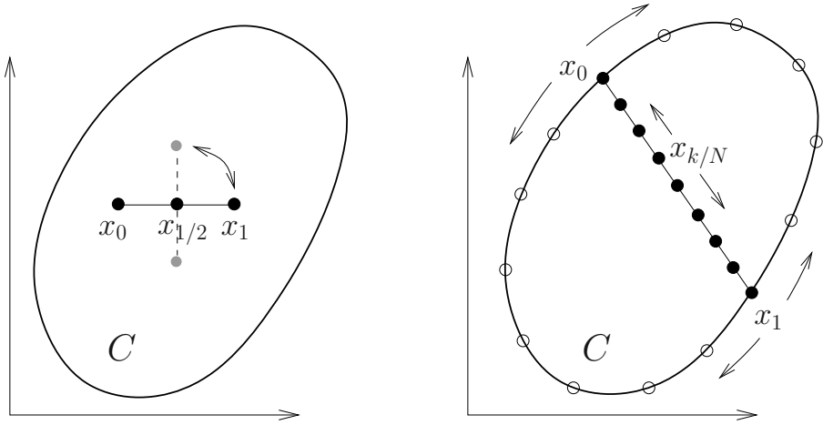
Figure 4.2: Very scarce ( left ) and comprehensive ( right ) coverage of the points and directions in C
