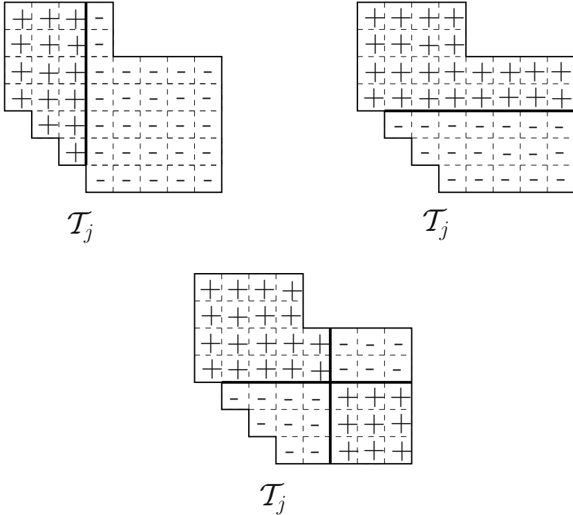
Figure 3.6: Examples of vertical, horizontal, and checkerboard cuts for one zone \mathcal{T}_j of a mesh \mathcal{T}_h made of rectangles. The vector \epsilon takes value +1 in cells with a plus sign, and -1 in cells with a minus
