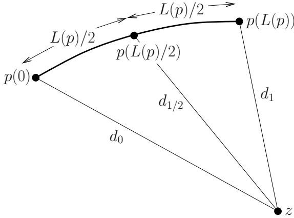
Figure 6.3: Notations for the median lemma
