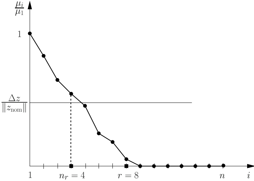
Figure 3.1: Graphical determination of the number of retrievable parameters: \mu_1, \dots, \mu_n = singular values, in decreasing order
