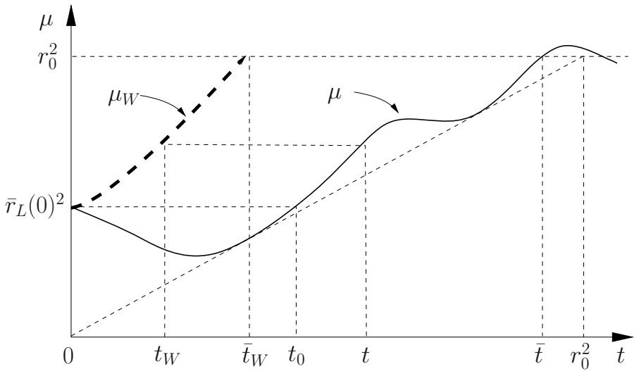
Figure 3.10: Properties of the \mu_W and \mu functions
