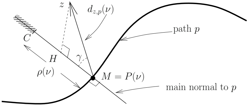
Figure 6.1: Notations for formula (6.25)
