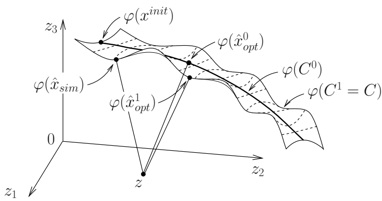
Figure 3.3: Comparison of local vs. multiscale parameterization for the convergence of gradient algorithms
