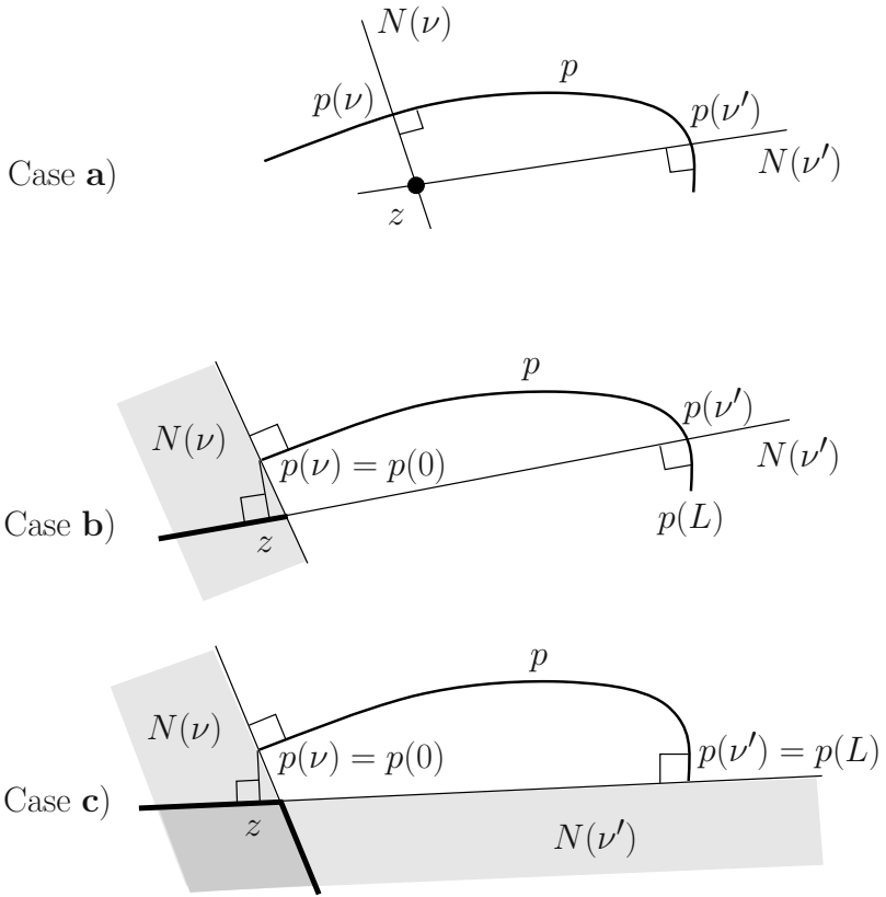
Figure 7.2: Intersection of affine normal cones at two points of a given paths p
