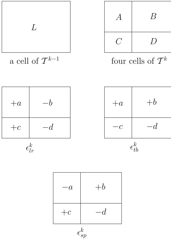
Figure 3.5: Definition of the three basis functions of \mathbf{W}^k associated to the cell L of \mathcal{T}^{k-1}
