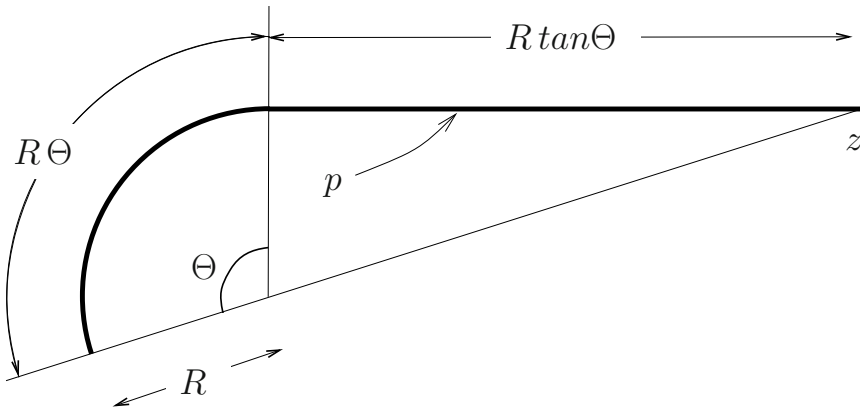
Figure 8.3: Illustration of the sharpness of the extended deflection condition (8.57)
