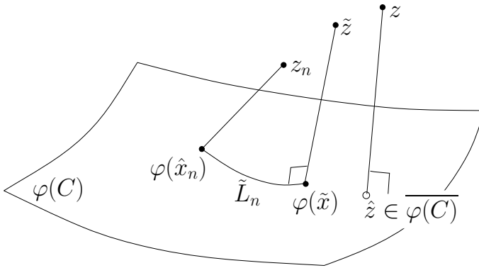
Figure 5.1: Notations for the nonlinear case
