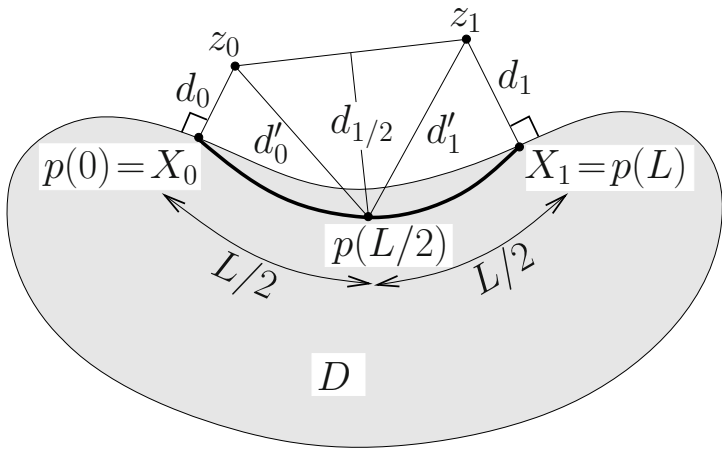
Figure 6.5: Notations for the continuity lemma
