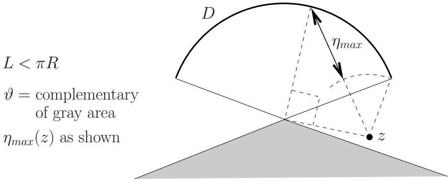
Figure 7.1: s.q.c. arc of circle
