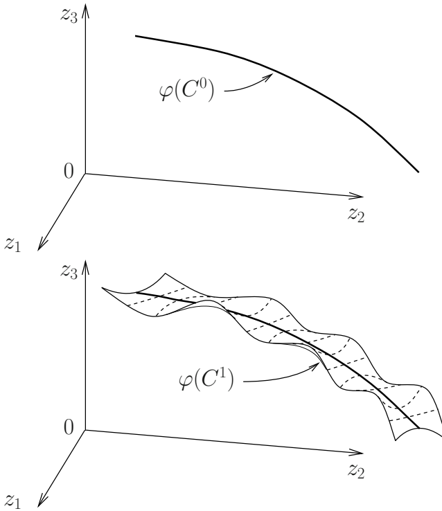
Figure 3.2: A representation of the attainable set for the prototype example at scale 0 and 1
