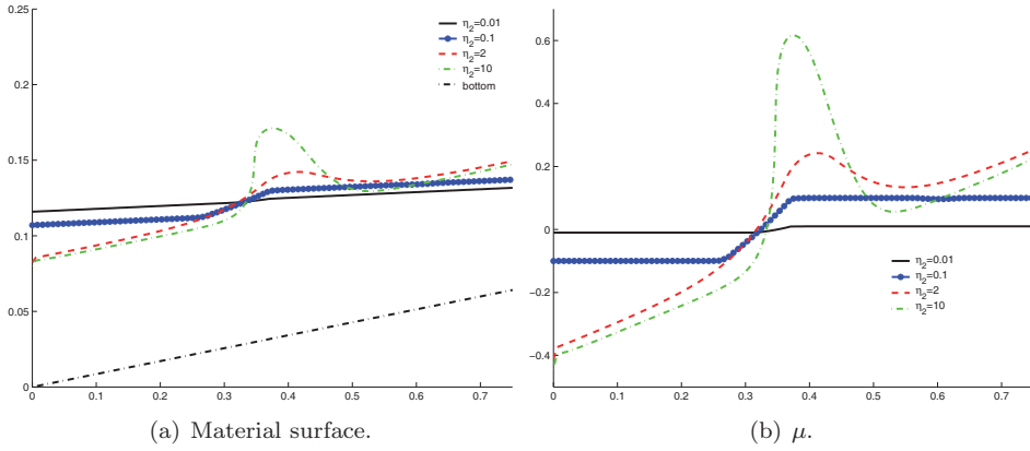
FIGURE 9. Test 1: Left: Material surface, Right: \mu , for the stationary solutions obtained with \eta_2 = 10, 2, 0.1 and 0.01
