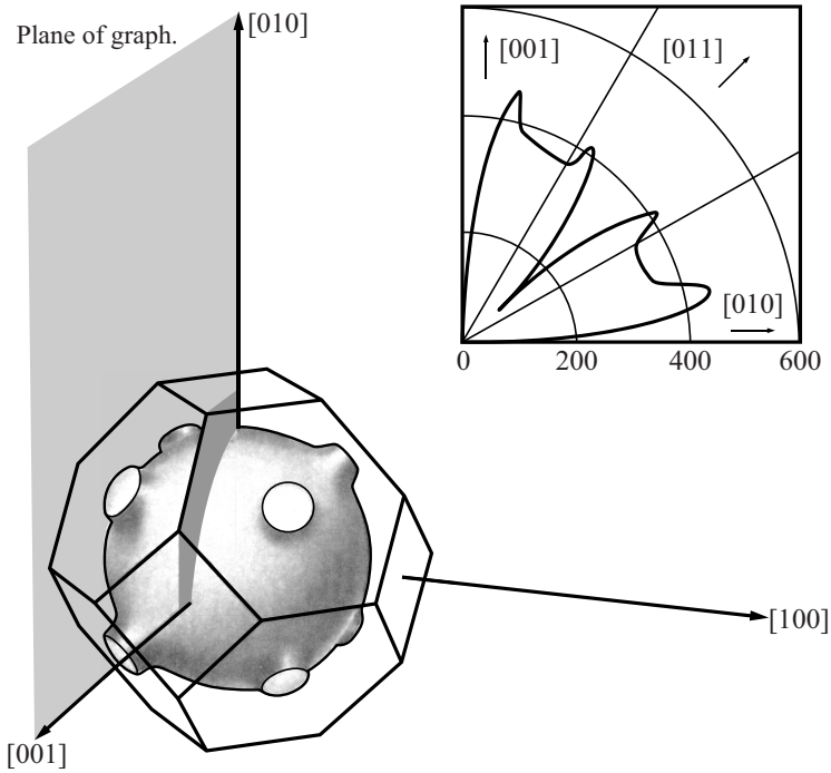
Figure 12.3: The striking anisotropy of the MR \Delta\rho in Cu after Klauder and Kunzler [2]. The [001] and [010] directions of the copper crystal are shown, and the current flows in the [100] direction perpendicular to the graph. The magnetic field is in the plane of the graph. Its magnitude is fixed at 18 kilogauss, and its direction varied continuously from [001] to [010].
