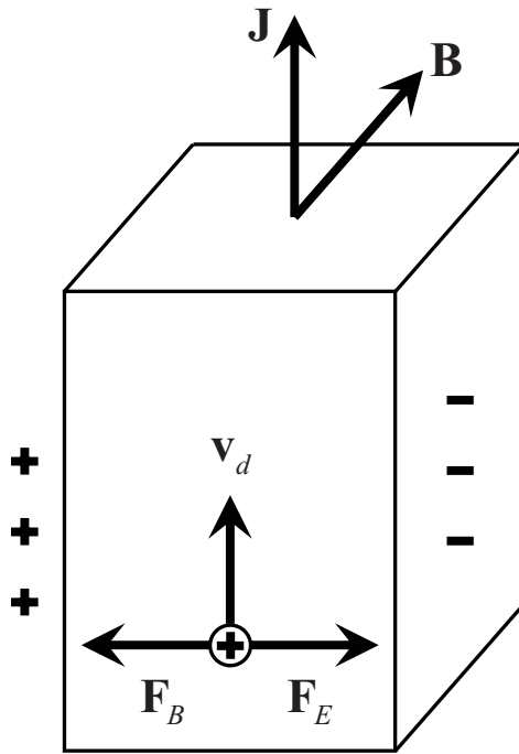
Figure 4.6: The magnetic and electric forces ( \mathbf{F}_B , \mathbf{F}_E ) are balanced to zero in the Hall effect measurement.
