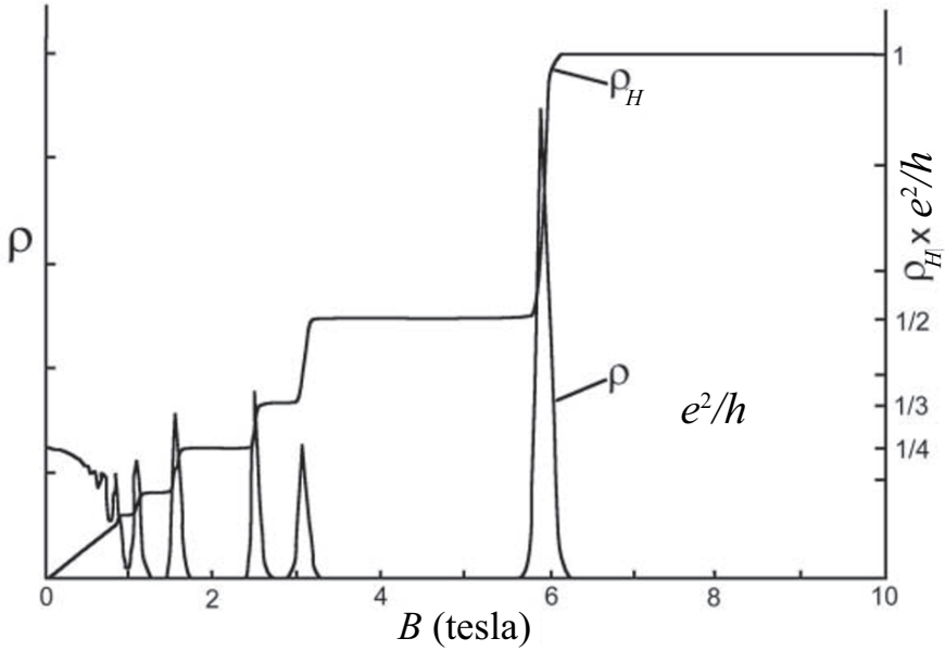
Figure 12.7: Observed QHE in heterojunction GaAs/AlGaAs at 60 mK, after Tsui [11]. The Hall resistivity \rho_H and the resistance \rho are shown as a function of the magnetic field B in tesla.
