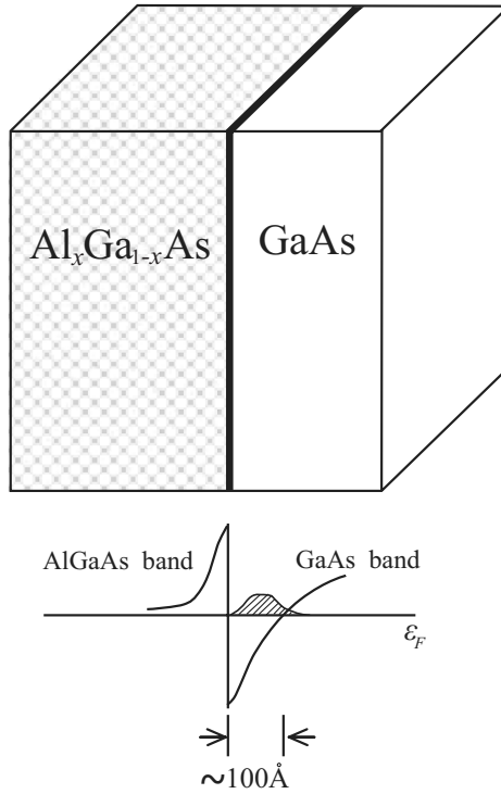
Figure 12.4: The electrons are localized in less than 100 \text{ \AA} near the interface \text{GaAs}/\text{AlGaAs} . The shaded area represents the electron distribution.
