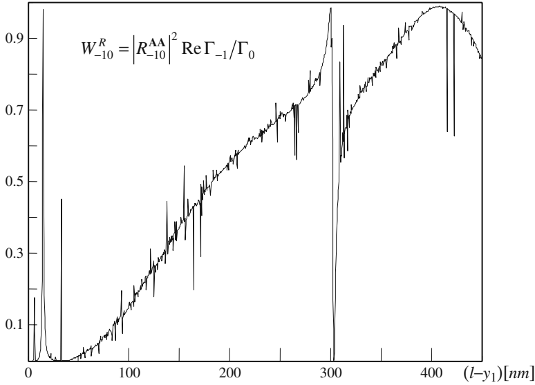
Fig. 3.6 Groove width dependence of the minus first-order diffraction efficiency. Computation is done by using classical Fourier modal method with a truncation order N = 15 : \varepsilon_{21} = -100 , \varepsilon_{22} = 1.0 , \tilde{\varepsilon}_3 = -100 , H -polarization
