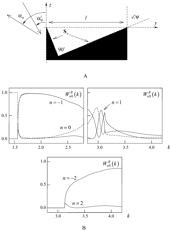
Fig. 4.14 (a) The echelette geometry and (b) its electrodynamic characteristics in the frequency band 1.4 \leq k \leq 4.2 : H -polarization, \alpha_0^i = 0 ( \Phi = 0 ), l = 4.02 , \psi = 67.5^\circ , L_1 = 8.4
