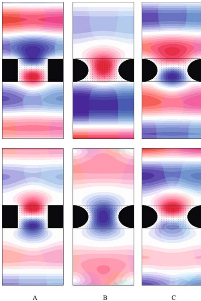
Fig. 4.11 The grating excitation by quasi-monochromatic wave (4.119) with the central frequency: (a) \tilde{k} = K_{12} ; (b) \tilde{k} = K_{21} ; and (c) \tilde{k} = K_{22} : the E_x(g, t) spatial distribution, g \in \mathbf{Q}_L at the time t \approx 80 (the upper row ; forced oscillations of the field) and t \approx 205 (the lower row ; free oscillations of the field)
