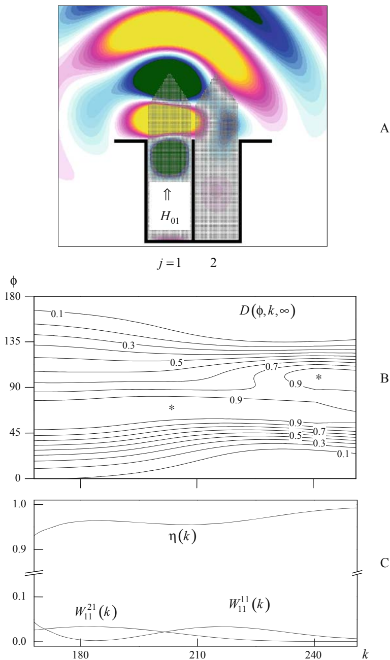
Fig. 4.52 The excitation of a system ( l = 0.014 ) of two radiation elements 2 ( d = 0.5c ) by the pulsed H_{01} -wave (4.140): (a) The E_x(g,t) spatial distribution, g \in \mathbf{Q}_L , t = 1.1 ; (b) radiation pattern D(\phi, k, \infty) in the frequency band 168 \leq k \leq 251 ; (c) energy characteristics of the system Look: 4-52-A.exe – the E_x(g,t) spatial–time distribution, g \in \mathbf{Q}_L at the time 1.0 < t < 1.15 (the pulse major part crosses the computational space \mathbf{Q}_L ; U_{\max}(t) = 0.5 )
