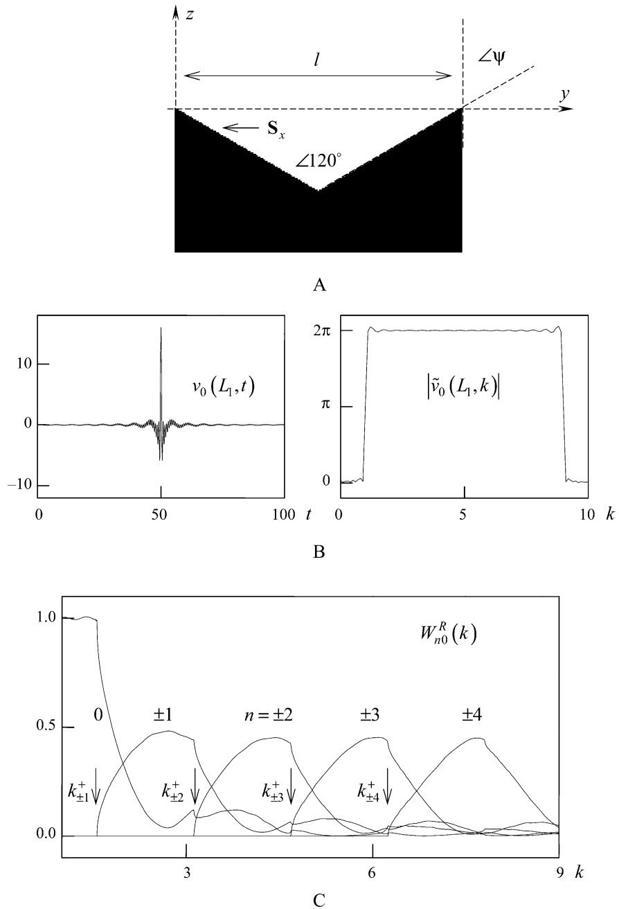
Fig. 4.24 The mode-frequency exfoliation of a superbroadband pulse: (a) Grating geometry ( \psi = 60^\circ , l = 4.02 , L_1 = 8.0 ); (b) the amplitudes of the incident E -polarized pulsed wave \tilde{U}_0^i(g, t) ( \Phi = 0 ); (c) the energy distribution among spatial harmonics of the field \tilde{U}^s(g, k) in the structure reflection zone
