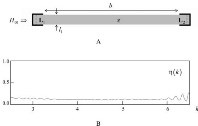
Fig. 4.33 (a) A planar dielectric waveguide ( l_1 = 1 , b = 13.58 , \varepsilon = 2.1 , all proportions of the actual object are retained) and (b) its loss by the radiation into the free space
