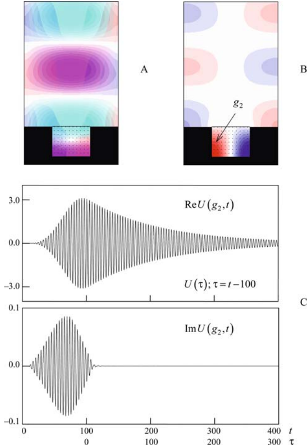
Fig. 4.18 The reflective grating excitation (geometry 2) by an H -polarized quasi-monochromatic wave U_0^i(g,t) : \Phi = 0.5; v_0(L_1,t) = F_3(t); \tilde{k} = 1.565, \tilde{T} = 0.5, \tilde{T} = 100 : (a and b) The H_x(g,t) spatial distribution, g \in \mathbf{Q}_L at the time t = 90 and t = 205 ; (c) functions U(g_2,t) and U(\tau) Look: 4-18-A.exe and 4-18-B.exe – the H_x(g,t) spatial–time distribution, g \in \mathbf{Q}_L , 80 \leq t \leq 95 and 200 \leq t \leq 210
