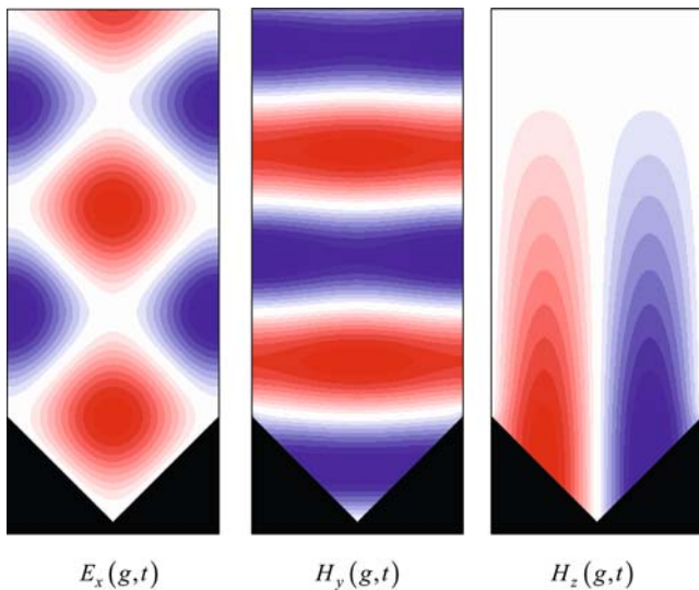
Fig. 4.22 (Complementation to Fig. 4.21). The E_x(g,t) , H_y(g,t) , and H_z(g,t) spatial distributions, g \in \mathbf{Q}_L , t = 189.75
