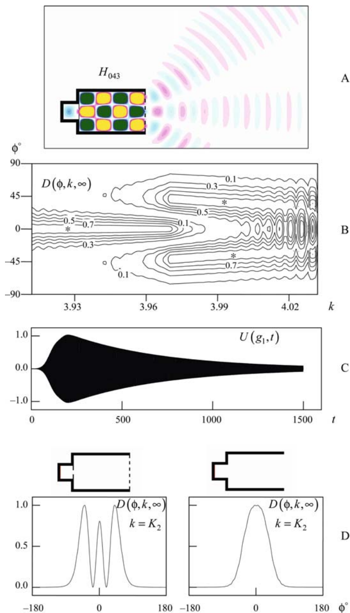
Fig. 4.48 The same as in Fig. 4.47, except that \tilde{k} = K_2
