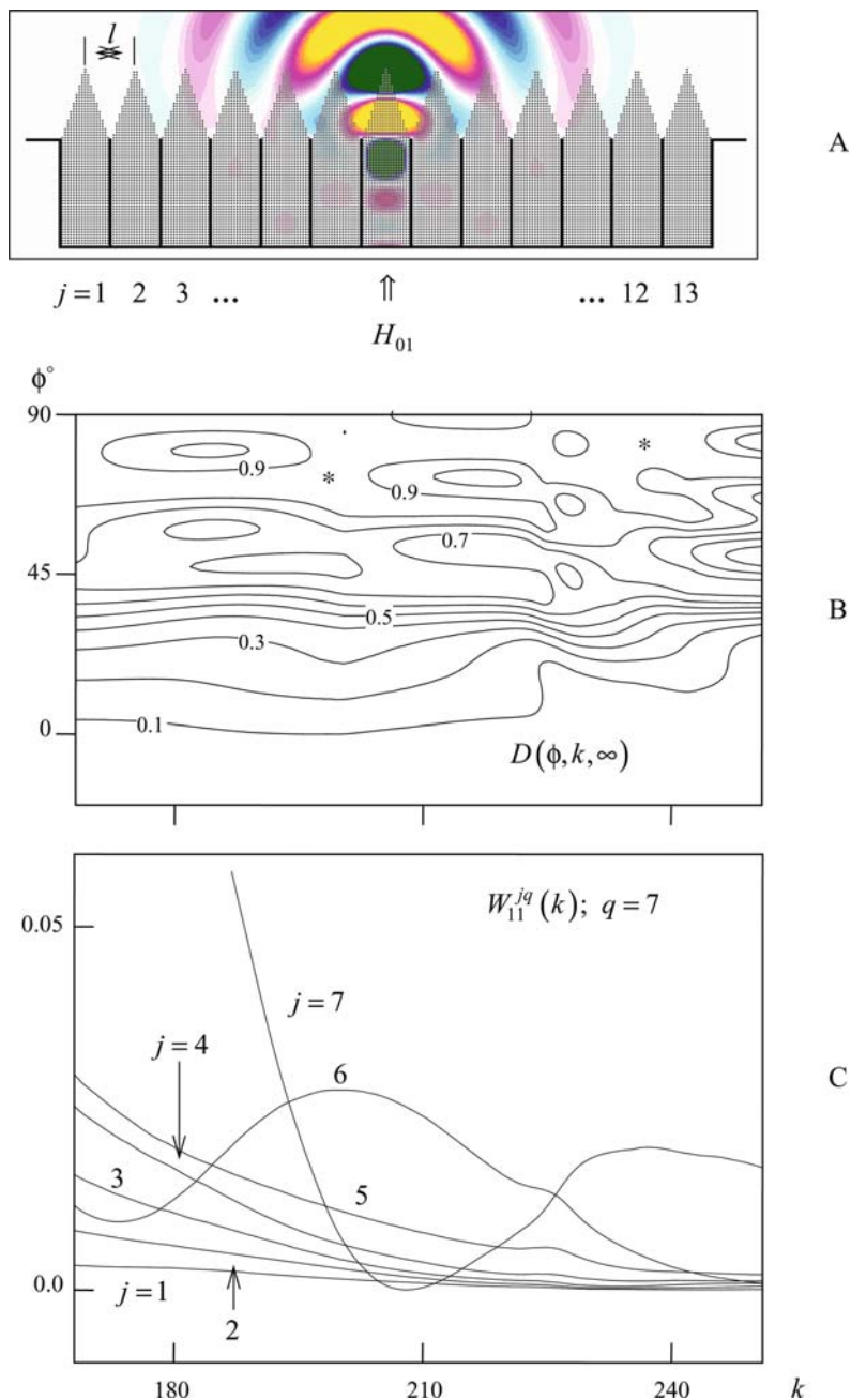
Fig. 4.54 The excitation of a system of 13 radiating elements 3 by the pulsed H_{01} -wave (4.140), q = 7 : (a) The E_x(g,t) spatial distribution, g \in \mathbf{Q}_L , t = 1.1 ; (b) radiation pattern D(\phi, k, \infty) in the frequency band 168 \leq k \leq 251 ; (c) the coefficients of the power coupling between the active ( j = 7 ) and passive ( j = 1, 2, \dots, 6 ) elements
