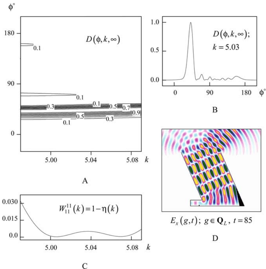
Fig. 4.37 The radiator providing a strong H_{01} - to H_{0,10} -wave conversion ( l_1 = 1 , l_2 = 6.56 , b = 9.8 , d_1 = 0.84 , d_2 = 3.91 , d_3 = 0.1 , d_4 = 0.53 , d_5 = 0.83 , d_6 = 1.5 , \beta = 66.3^\circ , the unit walls are 0.05 thick). The radiator excitation by a quasi-monochromatic wave (4.134): (a and b) Radiation patterns in a frequency band and at the frequency k = 5.03 ; (c) the dependence W_{11}^{11}(k) = 1 - \eta(k) characterizing the radiation efficiency; (d) the E_x(g, t) spatial distribution, g \in \mathbf{Q}_L , t = 85 Look: 4-37-D.exe – the E_x(g, t) spatial–time distribution, g \in \mathbf{Q}_L , 60 < t < 70 ( U_{\max}(t) = 0.5 )
