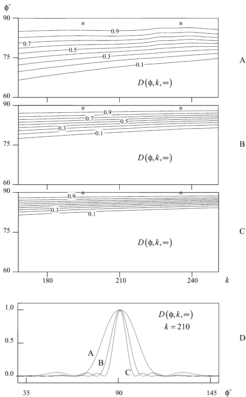
Fig. 4.55 The radiation patterns of a system of 13 radiating elements 3. Pulsed waves (4.140) excite (a) 5 central elements; (b) 9 central elements; and (c) all the 13 elements Look: 4-55-A.exe, 4-55-B.exe и 4-55-C.exe – the E_x(g, t) spatial–time distribution, g \in Q_L at the time 1.0 < t < 1.3 ( U_{\max}(t) = 0.5 )
