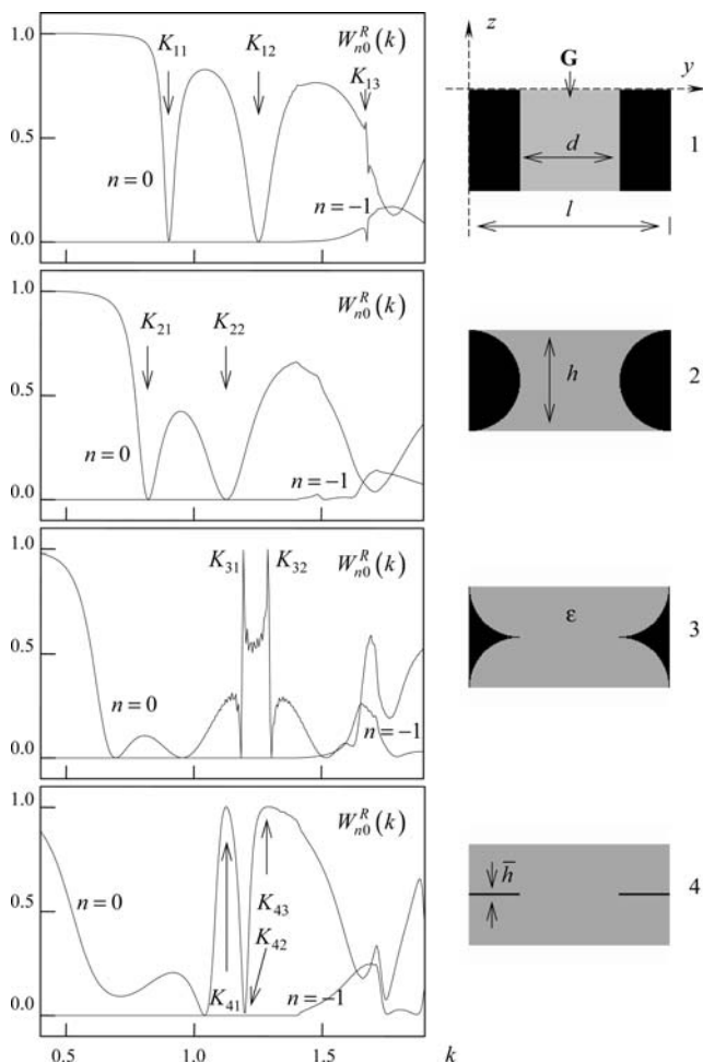
Fig. 4.9 E -polarization. Functions W_{n0}^R(k) of different semitransparent gratings of perfectly conducting bars inside a \epsilon = 4.0 dielectric layer. Geometries 1–4: grating period l = 4.02 , height h = 2.0 , period open part is d = 2.0 long, metal strips are \bar{h} = 0.02 thick, L_1 = L_2 = 5.0 . Look: 4-09-1.exe, 4-09-2.exe, 4-09-3.exe, 4-09-4.exe – the E_x(g, t) spatial–time distribution, g \in \mathbf{Q}_L , 50 \leq t \leq 65 (forced oscillations mode; U_{\max}(t) = 1.0 ) in the excitation of gratings 1–4 by pulsed wave (4.117)
