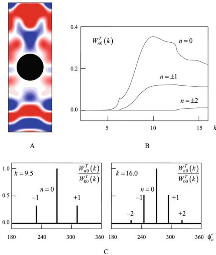
Fig. 4.29 (Complementation to Fig. 4.28). An infinite grating ( l = 1 , L_1 = 1.19 ) in the field of a pulsed wave U_0^i(g,t) : \Phi = 0; v_0(L_1,t) = F_2(t); \tilde{k} = 9, \Delta k = 7, \tilde{T} = 12.5, \bar{T} = 25 . (a) The E_x(g,t) spatial distribution, g \in \mathbf{Q}_L , t = 15.5 ; (b and c) the functions W_{n0}^T(k) ( k_{\pm 1}^+ \approx 6.28 , k_{\pm 2}^+ \approx 12.57 ) and ray radiation patterns W_{n0}^T(k)/W_{00}^T(k) ; k = 9.5 and k = 16.0 , for spatial harmonics propagating in the grating transition zone Look: 4-29-A.exe – the E_x(g,t) spatial–time distribution, g \in \mathbf{Q}_L , 12.5 \leq t \leq 16.25 ( U_{\max}(t) = 1.0 )
