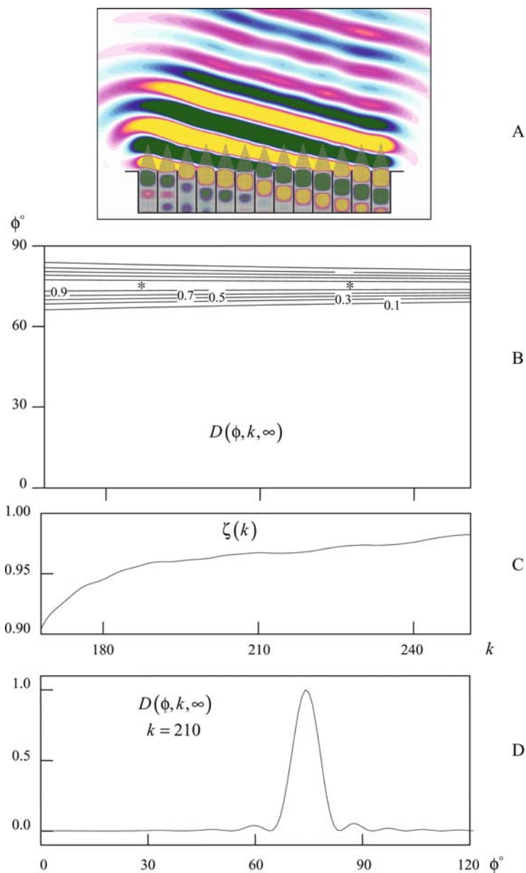
Fig. 4.57 The phased array excitation by a set of pulsed waves U_1^{i(q)}(g, t) satisfying condition (4.142), \Delta t = \sin(15^\circ)l \approx 0.36 : (a) The E_x(g, t) spatial distribution, g \in \mathbf{Q}_L , t = 1.1 ; (b) radiation pattern D(\phi, k, \infty) ; (c) array efficiency in the frequency band 168 \leq k \leq 251 ; and (d) radiation pattern D(\phi, k, \infty) at the frequency k = 210
