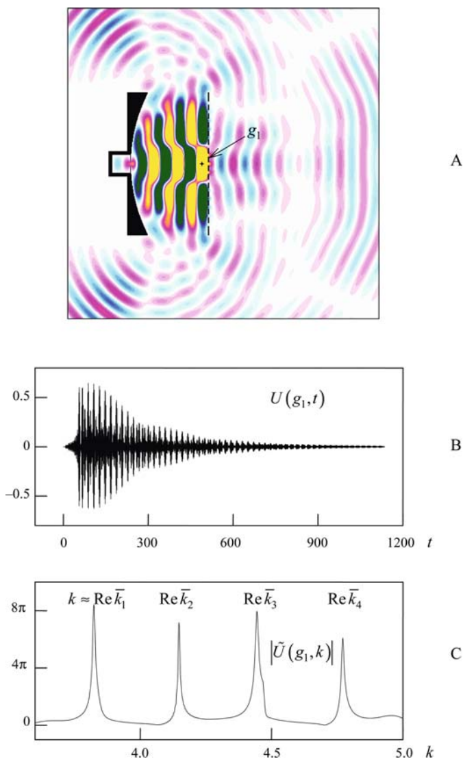
Fig. 4.41 The radiator excitation (geometry 4) by the pulsed H_{01} -wave (4.135): (a) The E_x(g, t) spatial distribution, g \in \mathbf{Q}_L , t = 300 ; (b and c) the temporal and the spectral amplitudes of the field at the point g = g_1 near the semitransparent mirror of the resonant antenna
