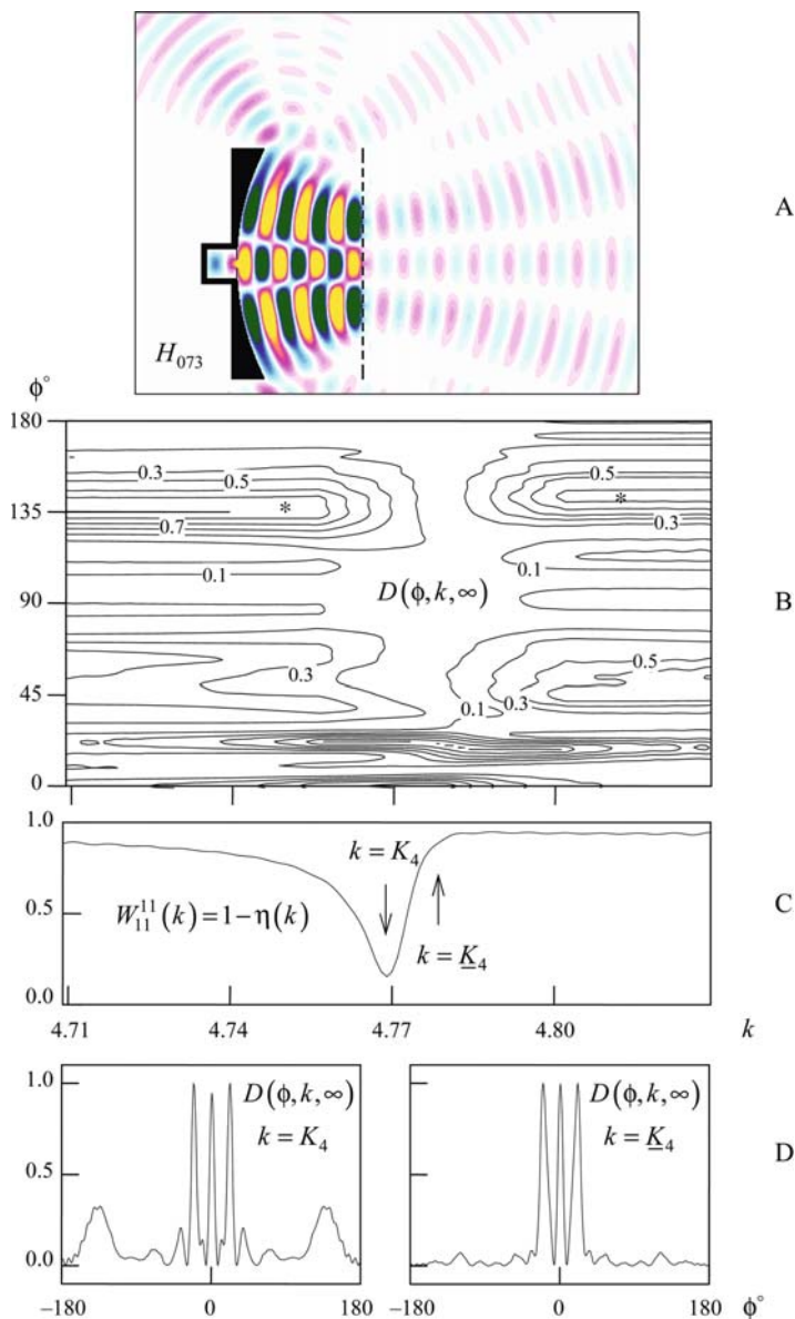
Fig. 4.45 The same as in Fig. 4.42 except that \tilde{k} = K_4
