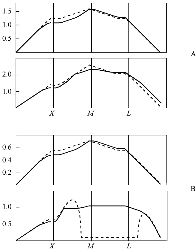
Fig. 5.5 Dispersion relations k_n(\gamma) for a laminated structure corresponding to Fig. 5.4 for the contrasts (a) \varepsilon_1/\varepsilon_2 = 10 and (b) \varepsilon_1/\varepsilon_2 = 50 . It is seen that for the highest contrast, there is a large region where the asymptotic solution ( dashed curve ) fails to approximate the true dispersion relation for one of the polarizations
