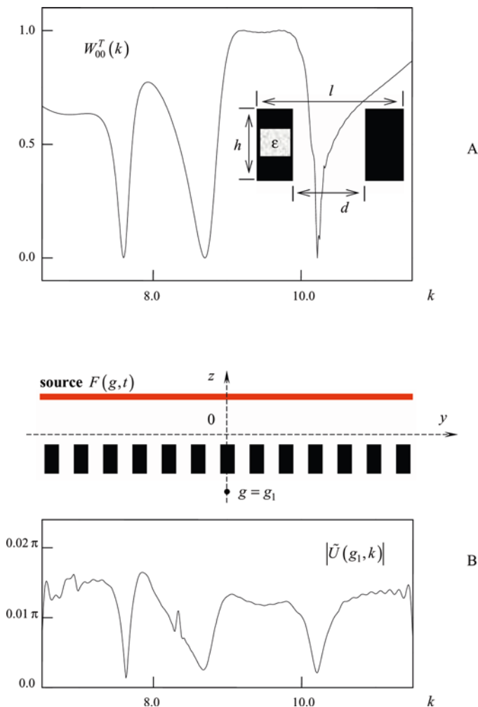
Fig. 4.30 The functions (a) W_{00}^T(k) ; \Phi = 0 , and (b) |\tilde{U}(g_1, k)| characterizing the transparency of the infinite (a) ( l = 0.61 , h = 0.61 , d = 0.31 and \epsilon = 5.0 ) and (b) finite (13 periods) dielectric gratings
