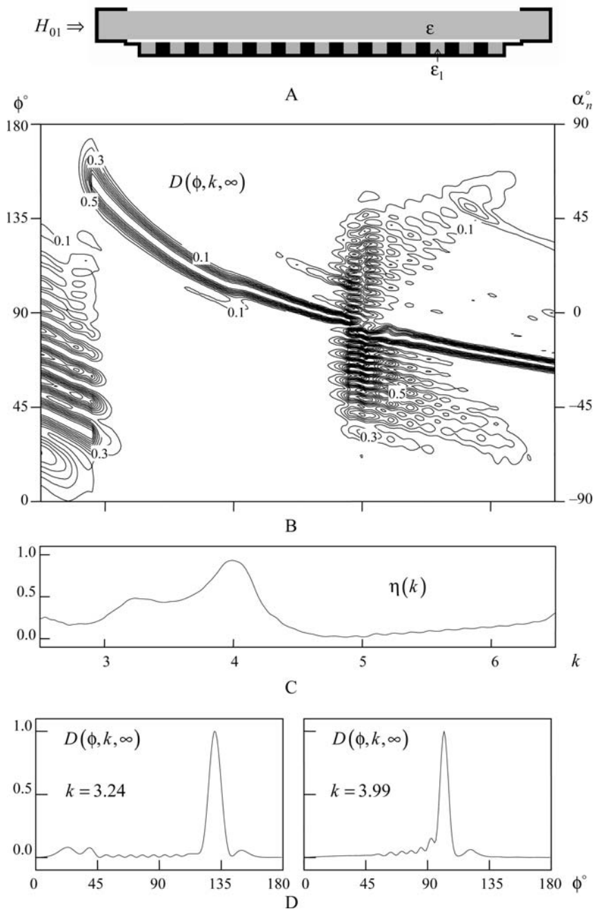
Fig. 4.35 (a) Geometry ( \epsilon = 2.1 , \epsilon_1 = 4 , l = 1 ), (b and d) radiation patterns, and (c) efficiency of the pattern-generating plane structure
