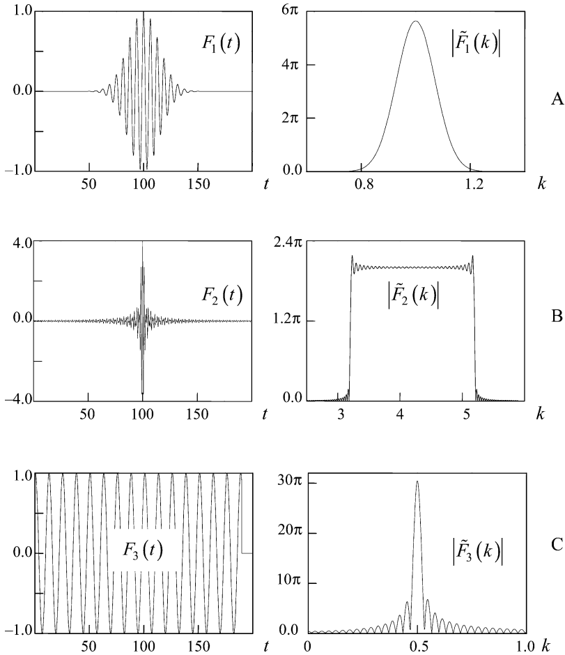
Fig. 4.3 Dynamical and spectral characteristics of current sources for pulsed waves: (a) Source (4.94), \tilde{k} = 1.0 , \tilde{\alpha} = 1.0 , \tilde{T} = 100 , and \tilde{T} = 200 ; (b) source (4.95), \tilde{k} = 4.2 , \Delta k = 1 , \tilde{T} = 100 , \tilde{T} = 200 ; (c) source (4.96), \tilde{k} = 0.5 , \tilde{T} = 0.5 , and \tilde{T} = 190
