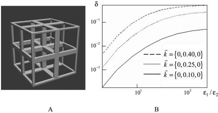
Fig. 5.8 (a) Scaffold structure, which is the same as in Fig. 5.1. (b) The relative deviations \delta depending on \varepsilon_1/\varepsilon_2 for a wave propagating along a main coordinate axis. As in Fig. 5.7, the results for E - and H -polarizations are similar due to symmetry
