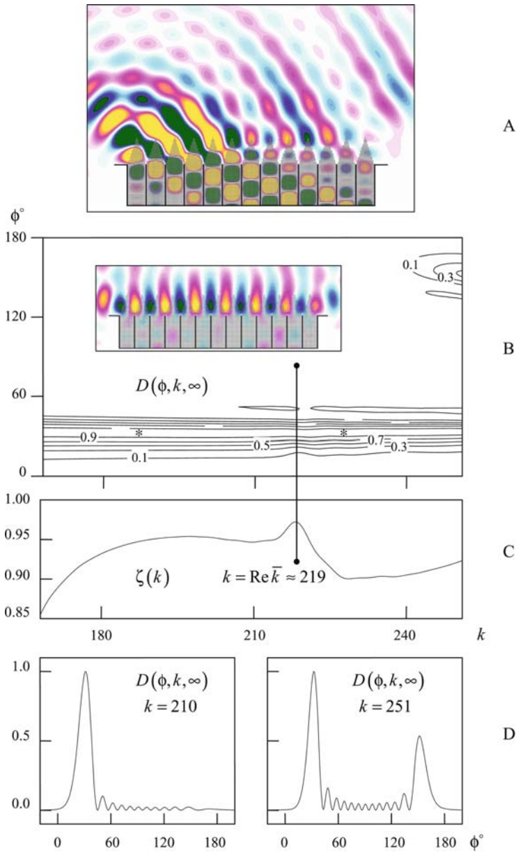
Fig. 4.60 The phased array excitation by a set of pulsed waves U_1^{i(q)}(g, t) satisfying condition (4.142), \Delta t = \sin(60^\circ)l \approx 1.21 : (a) The E_x(g, t) spatial distribution; g \in \mathbf{Q}_L , t = 1.1 ; (b) radiation pattern D(\phi, k, \infty) ; (c) array efficiency in the frequency band 168 \leq k \leq 251 ; (d) radiation patterns D(\phi, k, \infty) at the frequencies k = 210 and k = 251
