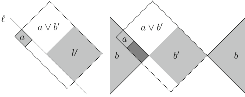
Fig. 4.2 The two figures show that \text{Caus}(\mathbb{M}^n) is not orthomodular. The first thing to note is that \text{Caus}(\mathbb{M}^n) contains open (4.15) as well as closed (4.59) diamond sets. In the left picture we consider the join of a small closed diamond a with a large open diamond b' . (Closed sets are indicated by a solid boundary line.) Their edges are aligned along the lightlike line \ell . Even though these regions are causally disjoint, their causal completion is much larger than their union and given by the open (for n > 2 ) enveloping diamond a \vee b' framed by the dashed line. (This also shows that the join of two regions can be larger than the domain of dependence of their union; compare footnote 19.) Next we consider the situation depicted on the right side. The closed double-wedge region b contains the small closed diamond a . The causal complement b' of b is the open diamond in the middle. a \vee b' is, according to the first picture, given by the large open diamond enclosed by the dashed line. The intersection of a \vee b' with b is strictly larger than a , the difference being the dark-shaded region in the left wedge of b below a . Hence a \neq b \wedge (a \vee b') , in contradiction to (4.68a)
