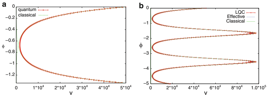
Fig. 7.3 In the LQC evolution of models under consideration, the big bang and big crunch singularities are replaced by quantum bounces. Expectation values and dispersion of |\hat{V}|_\phi , are compared with the classical trajectory and the trajectory from effective Friedmann dynamics. The classical trajectory deviates significantly from the quantum evolution at Planck scale and evolves into singularities. The effective trajectory provides an excellent approximation to quantum evolution at all scales. (a) The k=0 case. In the backward evolution, the quantum evolution follows our post big-bang branch at low densities and curvatures but undergoes a quantum bounce at matter density \rho \sim 0.82\rho_{\text{Pl}} and joins on to the classical trajectory that was contracting to the future. (b) The k=1 case. The quantum bounce occurs again at \rho \sim 0.82\rho_{\text{Pl}} . Since the big bang and the big crunch singularities are resolved the evolution undergoes cycles. In this simulation p_{(\phi)}^* = 5 \times 10^3 , \Delta p_{(\phi)}/p_{(\phi)}^* = 0.018 , and v^* = 5 \times 10^4
