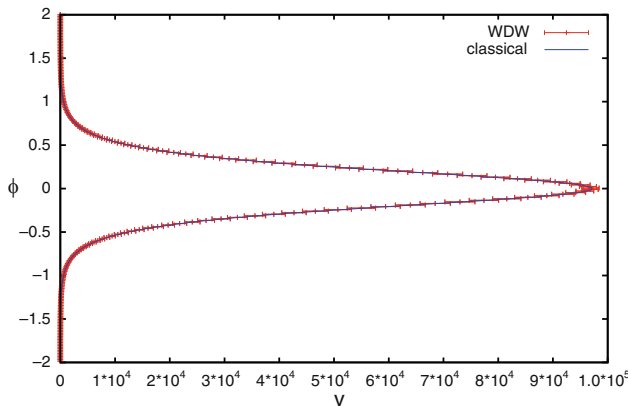
Fig. 7.2 Expectation values (and dispersions) of |\hat{v}|_\phi for the WDW wave function in the k = 1 model. The WDW wave function follows the classical trajectory into the big-bang and big-crunch singularities (In this simulation, the parameters were: p_\phi^* = 5000 , and \Delta p_\phi / p_\phi^* = 0.02 )
