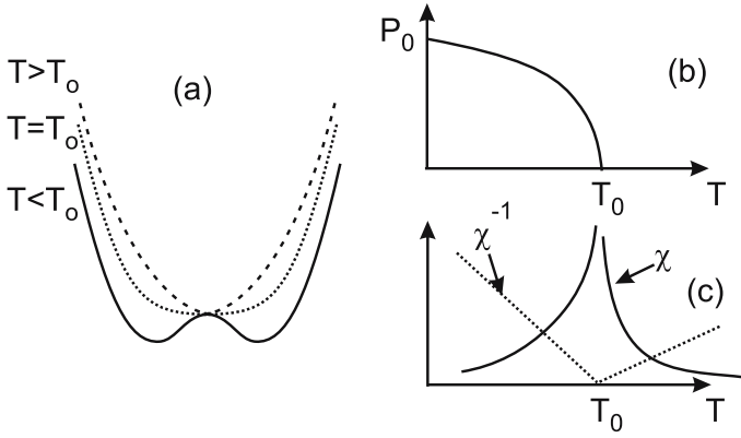
Fig. 3. Second-order phase transition. (a) Free energy as a function of the polarization at T > T_0 , T = T_0 , and T < T_0 ; (b) Spontaneous polarization P_0(T) as a function of temperature; (c) The susceptibility \chi and its inverse, where \chi = \partial P / \partial E|_{P_0} is evaluated at the equilibrium polarization P_0(T)
