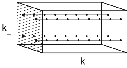
Fig. 7. Arrangement of Brillouin zone for computation of component of \mathbf{P} along k_{\parallel} direction
