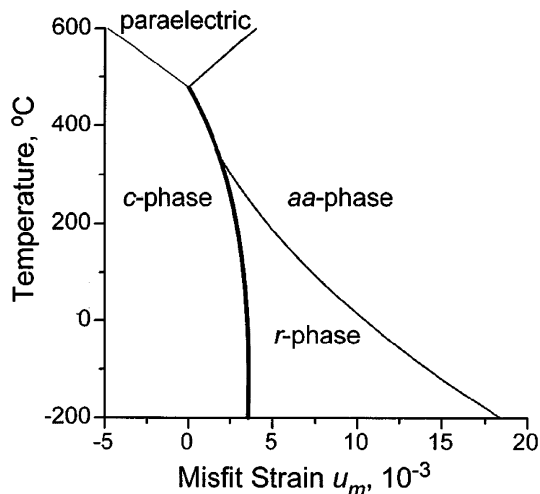
Fig. 25. Phase diagram of (001) single-domain PbTiO 3 thin films epitaxially grown on different cubic substrates providing various misfit strains in the heterostructures. The second- and first-order phase transitions are shown by thin and thick lines, respectively [185]. The aa-phase is orthorhombic, the r-phase monolitic, and the c-phase tetragonal
