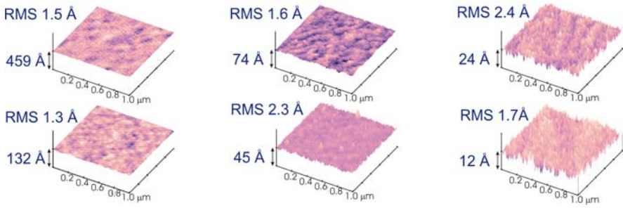
Fig. 2. Topography images in three dimensions obtained for scan areas of 1 \mu\text{m}^2 on \text{PbTiO}_3 thin films of \sim 459 , 132, 74, 45, 24 and 12 Å thickness, giving root-mean-square values of 1.5, 1.3, 1.6, 2.3, 2.4 and 1.7 Å respectively. The vertical scales used in these 3D representations are equal to the thickness of the samples, allowing a comparison of the roughness of the surface with the total film thickness. As can be seen from the data, the average thickness remains well defined, even for ultrathin films down to three unit cells
