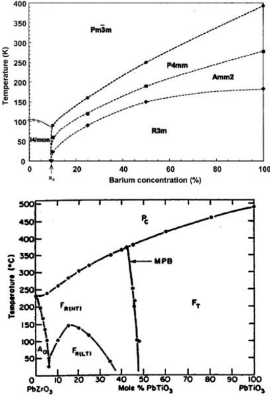
Fig. 7. (a) Critical temperature vs. concentration phase diagram of \text{Sr}_{1-x}\text{Ba}_x\text{TiO}_3 , deduced from X-ray and neutron-diffraction studies. From [37]. (b) PZT phase diagram. From [38], after Jaffe et al. [39]
