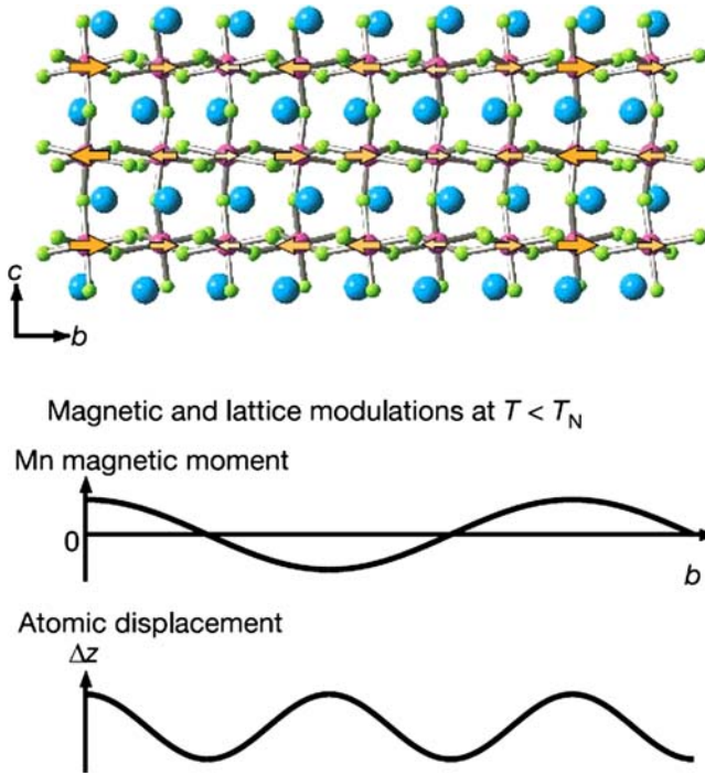
Fig. 27. Sketch of the crystal structure of TbMnO 3 . The arrows indicate the magnitudes of the local magnetic moments at the Mn ions. The lower plots show how the atomic displacements from the ideal centrosymmetric positions correlate with the magnitude of the Mn magnetic moments. Adapted by permission from [57]
