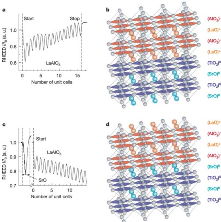
Fig. 30. (a) RHEED intensity oscillations of the specular reflected beam for the growth of LaAlO 3 directly on the TiO 2 -terminated SrTiO 3 (001) surface. (b) Schematic of the resulting (LaO) + /(TiO 2 ) 0 interface, showing the composition of each layer and the ionic charge state of each layer. (c) RHEED oscillations for the growth of LaAlO 3 , after a monolayer of SrO was deposited on the TiO 2 surface. (d) Schematic of the resulting (AlO 2 ) - /(SrO) 0 interface [216]
