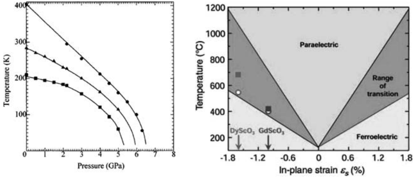
Fig. 6. (a) Critical temperature vs. pressure phase diagram of \text{BaTiO}_3 , deduced from X-ray and neutron-diffraction studies. From [32]. (b) Expected T_c of (001) \text{BaTiO}_3 under biaxial inplane strain \sigma , based on thermodynamic analysis. The green region represents the range (error bars) in the predicted T_c resulting from the spread in reported property coefficients for \text{BaTiO}_3 that enter into the thermodynamic analysis. The data points show the observed \sigma and T_c values of coherent \text{BaTiO}_3 films grown by molecular beam epitaxy (MBE) on \text{GdScO}_3 (blue circle) and \text{DyScO}_3 (red circle) substrates and by pulsed laser deposition (PLD) on \text{GdScO}_3 (blue square) and \text{DyScO}_3 (red square) substrates. From [34]
