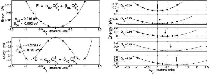
Fig. 5. Energetics of YMnO 3 . Left: Energy as a function of the amplitude of the zone-center polar distortion \Gamma_2^- ( top ) and the zone-boundary rotational mode K_3 ( bottom ). Right: Energy as a function of the amplitude of the zone-center polar distortion \Gamma_2^- at fixed amplitude of the zone-boundary rotational mode K_3 . From [45]
