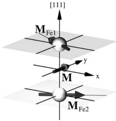
Fig. 22. Calculated magnetic structure including the spin-orbit interaction: The two iron magnetic moments rotate in the (111) plane so that there is a resulting spontaneous magnetization, \mathbf{M} . From [66]. Copyright (2005) by the American Physical Society
