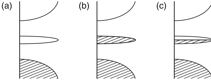
Fig. 12. Sketch of density of states that could be associated with the epitaxial interface of Fig. 11. Valence bands of materials 1 and 2 are hashed; conduction bands are unfilled; and a band of interface states may either be (a) entirely empty; (b) entirely filled; or (c) partially filled (i.e., metallic)
