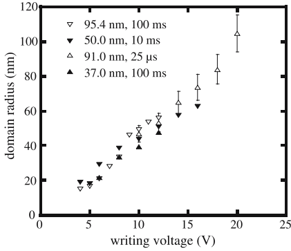
Fig. 3. Domain radius as a function of the writing voltage for 37.0-, 50.0-, 91.0- and 95.4-nm thick \text{PbZr}_{0.2}\text{Ti}_{0.8}\text{O}_3 films, where writing times of 100 ms, 10 ms, 25 μs and 100 ms, respectively, were used. The domain radius appears to depend linearly on the writing voltage applied to create the domain. The error bars shown for the 91.0 nm sample are representative of those in the other samples, and are due to the spread of domain radii for a given writing voltage and writing time
