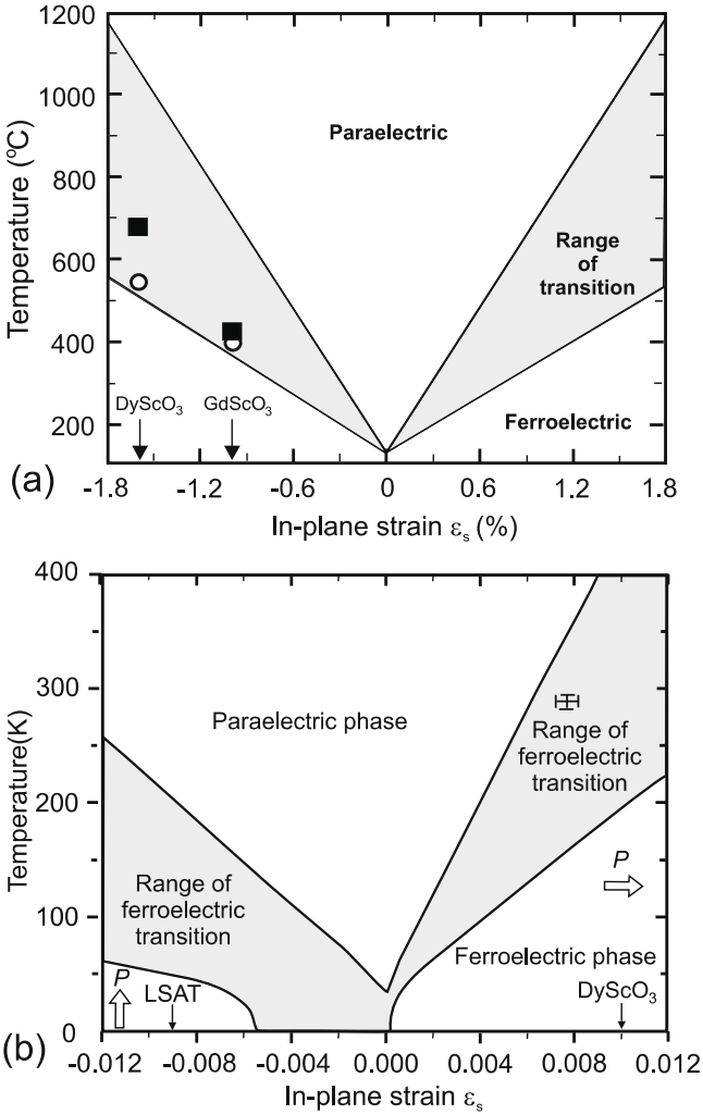
Fig. 26. Expected T_c of (a) (001) \text{BaTiO}_3 (from [177]) and (b) (001) \text{SrTiO}_3 (from [176]) based on a thermodynamic analysis. The range of transitions represents the uncertainty in the predicted T_c resulting from the spread in reported property coefficients. Note that the vertical scales are in K ( bottom ) and ^{\circ}\text{C} ( top ), and strains are in % for the top figure as in the original work
