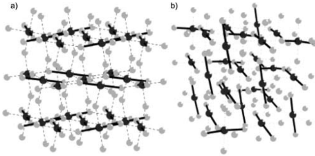
Fig. 24. The two-dimensional orbital ordering in LaMnO 3 (a) is compared with the three-dimensional orbital ordering in BiMnO 3 (b). The bold lines represent the orientation of the d_{z^2} orbitals, as revealed by elongations of the MnO 6 octahedra. The black circles show the positions of the Mn ions, and the gray circles represent the oxygens. From [92]. Copyright (2002) by the American Physical Society
