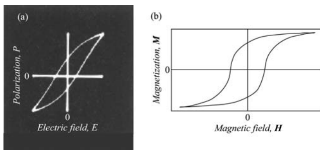
Fig. 1. Comparison of hysteresis loops in (a) \text{BaTiO}_3 , a typical ferroelectric [2] (copyright (1950) by the American Physical Society), and (b) \text{Fe} , a typical ferromagnet [3]. Note that the forms of the hysteresis curves are rather similar in the two cases
