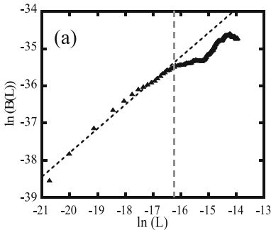
Fig. 9. Typical \ln\text{--}\ln plot of B(L) . Fitting the linear part of the curve (left of the vertical line) gives 2\zeta . Average values of the characteristic roughness exponent \zeta extracted from the equilibrium portion of the B(L) data are 0.26, 0.29 and 0.22 in the 50-, 66- and 91-nm thick \text{PbZr}_{0.2}\text{Ti}_{0.8}\text{O}_3 samples, respectively (figure after [9]).
