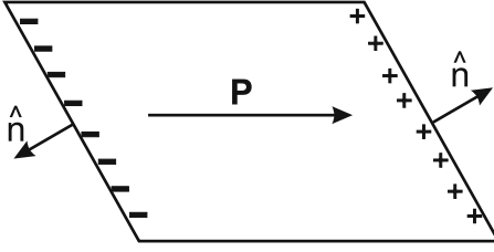
Fig. 6. Surface charge density generated by a bulk polarization at an interface
