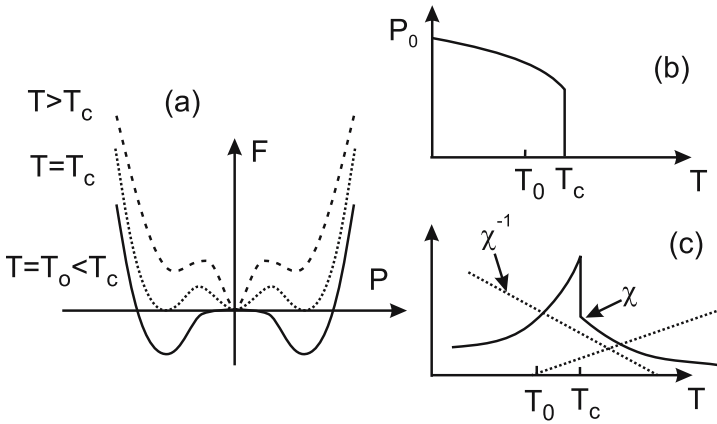
Fig. 4. First-order phase transition. (a) Free energy as a function of the polarization at T > T_c , T = T_c , and T = T_0 < T_c ; (b) Spontaneous polarization P_0(T) as a function of temperature; (c) Susceptibility \chi
