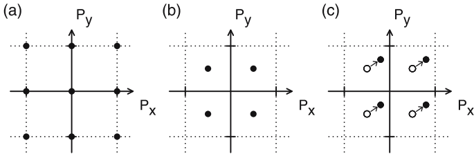
Fig. 8. Polarization as a lattice-valued quantity, illustrated for a 2D square-lattice system. Here, (a) and (b) illustrate the two possible states of polarization consistent with full square-lattice symmetry, while (c) illustrates a possible change in polarization induced by some symmetry-lowering change of the Hamiltonian. In (c), the arrows show the “effective polarization” as defined in (13)
