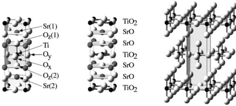
Fig. 11. The structure of \text{Sr}_2\text{TiO}_4 (space group I4/mmm ) can be viewed as (a) a stacking of SrO-terminated \text{SrTiO}_3 perovskite [001] slabs, (b) a stacking of \text{TiO}_2 and of SrO planes along [001], and (c) a series of Ti–O chains, infinitely long in the plane along [001] and [010], and of finite extent along [001] (the Sr atoms have been removed for clarity.) From [49]
