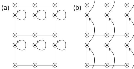
Fig. 10. Possible evolution of positions of Wannier centers (−), relative to the lattice of ions (+), as the Hamiltonian evolves adiabatically around a closed loop. Wannier functions must return to themselves, but can do so either (a) without, or (b) with, a coherent shift by a lattice vector
