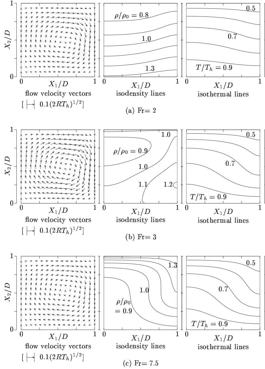
Figure 8.2. Flow velocity, isodensity lines, and isothermal lines ( L/D = 1 , T_c/T_h = 0.4 , \text{Kn} = 0.02 ). (a) \text{Fr} = 2 , (b) \text{Fr} = 3 , and (c) \text{Fr} = 7.5 . The contours of \rho/\rho_0 = 0.1n and T/T_h = 0.1m are shown in the figures. The arrows indicate the flow velocity at their starting points; the scale (v_i^2)^{1/2}/(2RT_h)^{1/2} = 0.1 is shown in the figures. The arrow is not shown on the upper and lower boundaries.
