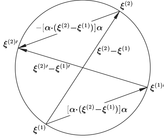
Figure A.1. Relation between (\xi^{(1)}, \xi^{(2)}) and (\xi^{(1)'}, \xi^{(2)'}) . The velocities \xi^{(1)'} and \xi^{(2)'} are antipodal points on the sphere with \xi^{(1)} and \xi^{(2)} as its antipodal points.
