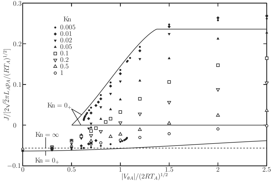
Figure 8.18. Bifurcation diagram: J/[2\sqrt{2}\pi L_A p_A / (RT_A)^{1/2}] vs |V_{\theta A}|/(2RT_A)^{1/2} ( J : the mass flow from the inner cylinder to the outer per unit time and per unit length of the cylinders) of the axially symmetric and uniform solution for various Knudsen numbers Kn ( L_B/L_A = 2 , V_{\theta B} = 0 , p_B/p_A = 1.2 , T_B/T_A = 1 ).
