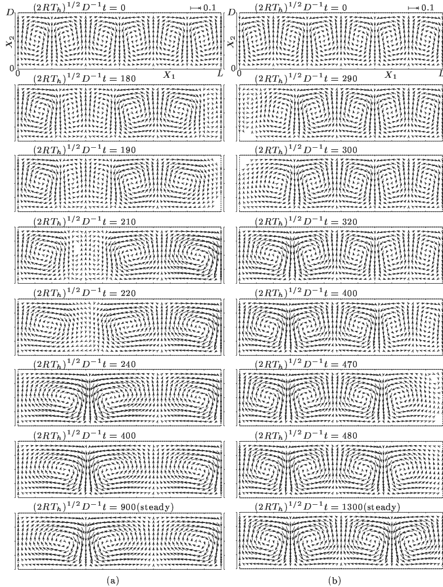
Figure 8.3. Transition process of the perturbed 6-roll solutions (8.8) and (8.9) with \varepsilon = 0.01 ( N = 6 , L/D = 3.6 , \text{Fr} = 3 , T_c/T_h = 0.4 , and \text{Kn} = 0.02 ). (a) Initial condition (8.8) and (b) initial condition (8.9). The arrows indicate the flow velocity (v_1, v_2) at their starting points; the scale (v_1^2 + v_2^2)^{1/2} / (2RT_h)^{1/2} = 0.1 is shown in the figure. The arrow is not shown when (v_1^2 + v_2^2)^{1/2} / (2RT_h)^{1/2} < 2 \times 10^{-3} . The arrows on the upper and lower boundaries are omitted for clearness of the figure.
