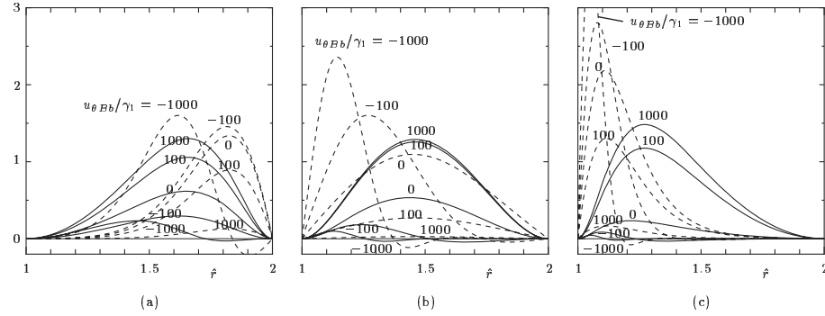
Figure 8.31. The various profiles (U_{11}, V_{11})/||f_{11}|| vs \hat{r} , where ||f_{11}|| = [\int_1^{\hat{r}_B} (U_{11}^2 + V_{11}^2) \hat{r} d\hat{r}]^{1/2} ( \alpha = \pi , \hat{r}_B = 2 , the first branch of the bifurcation curves). (a) P_{Bb}/(-\gamma_1 C_4^*) = -10 , (b) P_{Bb}/(-\gamma_1 C_4^*) = 0 , and (c) P_{Bb}/(-\gamma_1 C_4^*) = 10 . The dashed lines --- are U_{11}/||f_{11}|| and the solid lines — are V_{11}/||f_{11}|| .
