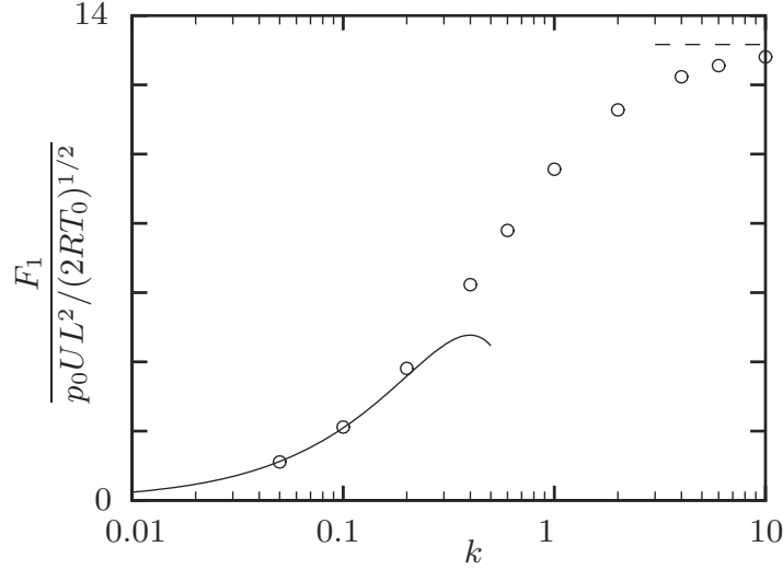
Figure 4.12. The force, F_1/p_0 U L^2 (2RT_0)^{-1/2} vs k , acting on the sphere with a uniform temperature in a uniform flow (a hard-sphere gas). The white circles \circ are the numerical solution, the solid line — is the asymptotic solution (4.113) up to the order of k^2 , and the dashed line --- indicates the free molecular solution (4.117).
