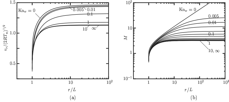
Figure 6.30. The profiles of the macroscopic variables for various Knudsen numbers \text{Kn}_w in the evaporating flow from a sphere into a vacuum II: flow velocity and Mach number. (a) v_r / (2RT_w)^{1/2} vs r/L and (b) M vs r/L . In panel (a), the curves for \text{Kn}_w = 0, 0.005, 0.01, 0.1, 1, 10 , and \infty are shown. In panel (b), the curves for \text{Kn}_w = 0, 0.005, 0.01, 0.02, 0.05, 0.1, 0.2, 0.5, 1, 2, 5, 10 , and \infty are shown.
