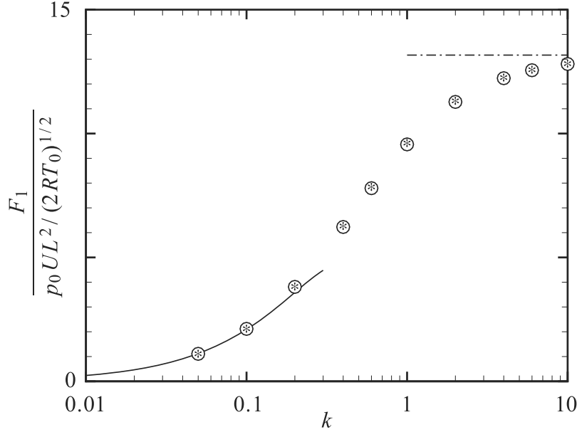
Figure 4.18. The force (or drag), F_1/p_0UL^2(2RT_0)^{-1/2} vs k , acting on a sphere with arbitrary thermal conductivity in a uniform flow of a gas (a hard-sphere gas). The white circles \circ are the numerical solution for \lambda_p/\lambda_g = \infty (or for the sphere with a uniform temperature) and the stars * are the numerical solution for \lambda_p/\lambda_g = 1 . The solid line — is the asymptotic solution for small k [Eq. (4.148) up to the order of k^2 ], and the dot-dash line --- indicates the free molecular solution (4.149); they are independent of \lambda_p/\lambda_g .
