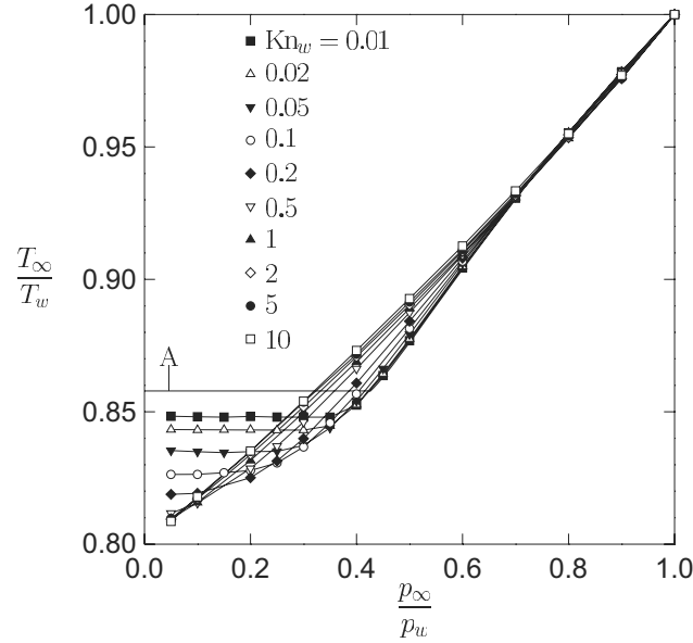
Figure 6.22. Temperature ratio T_\infty/T_w vs pressure ratio p_\infty/p_w for various Knudsen numbers \text{Kn}_w in the evaporating flow from a cylinder into a gas. The curve with the mark A is the solution in the continuum limit, i.e., Eqs. (6.32) and (6.34).
