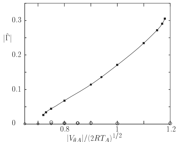
Figure 8.23. The circulation \hat{\Gamma} [= \Gamma/L_A(2RT_A)^{1/2}] vs |V_{\theta A}|/(2RT_A)^{1/2} on the branch of the roll-type solution (● and ■ in Fig. 8.20) I: \text{Kn} = 0.005 . The circulation \Gamma is defined by the circulation around the circle on the section \theta = \text{const} with the radius 0.3L_A and its center at the center of the domain under discussion (the shaded region in Fig. 8.19). The black circle ● and black square ■ correspond, respectively, to the solutions marked by ● and ■ in Fig. 8.20; the smaller white circle corresponds to a stable axially uniform solution on the lower branch, and the larger one to that on the upper branch.
