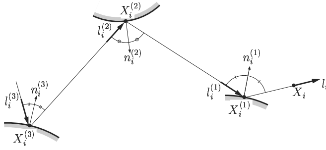
Figure 2.5. Path of a specularly reflecting molecule and X_i^{(m)} , l_i^{(m)} , and n_i^{(m)} .
