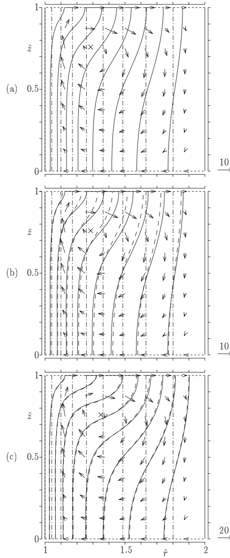
Figure 8.12. Bifurcated temperature fields for a hard-sphere gas II: \hat{T}_B = 10 , U_B = 0 , \hat{r}_B = 2 , and \hat{z}_B = 1 . (a) U_A = 79 , (b) U_A = 80 , and (c) U_A = 100 . The solid lines — indicate the isothermal lines of the bifurcated temperature field [ \hat{T} = n ( n = 1, 2, \dots, 10 ) from the left wall to the right]. The dashed lines --- indicate the corresponding results with the thermal stress neglected, and the dot-dash lines -.- indicate the isothermal lines for the ASU solution. The arrows indicate (u_r, u_z) at their starting points and their scale is shown on the lower right corner of each panel, and \times indicates the point where u_r = u_z = 0 . The maximum of (u_r^2 + u_z^2)^{1/2} is 12.4 at U_A = 79 in (a), 13.3 at U_A = 80 in (b), and 23.8 at U_A = 100 in (c).
