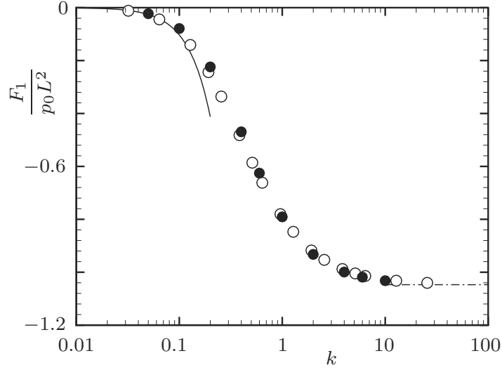
Figure 4.17. The force, F_1/p_0 L^2 vs k , acting on a sphere with a nonuniform temperature in a gas (a hard-sphere gas). The black circles \bullet are the numerical solution for a hard-sphere gas, the white circles \circ are the numerical solution for the BKW model, the solid line — is the asymptotic solution for a hard-sphere gas for small k [Eq. (4.137) up to the order of k^2 ], and the dot-dash line --- indicates the free molecular solution (4.141). In the above figure, the data for the BKW model are those where the original k is replaced by 1.562492k (see Footnote 37 in Section 4.6.2).
