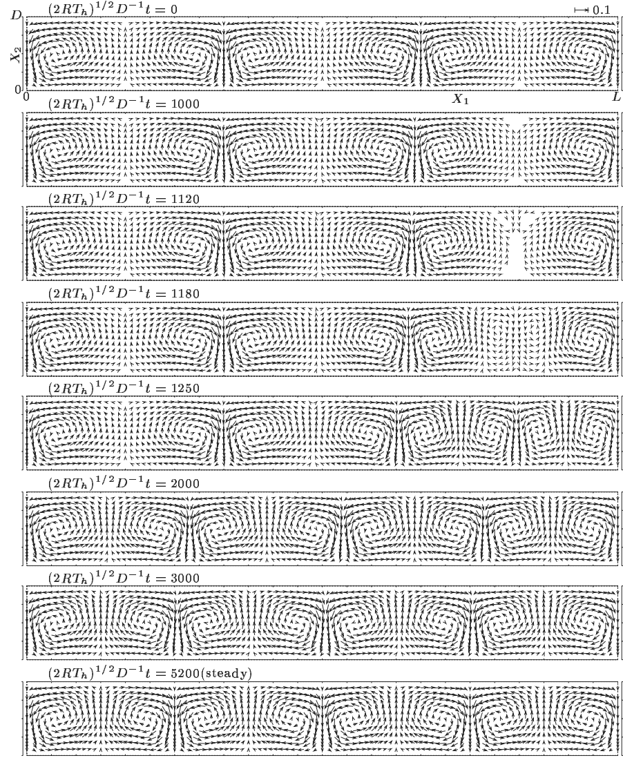
Figure 8.4. Transition process of the perturbed 6-roll solution (8.9) with \varepsilon = 0.01 ( N = 6 , L/D = 8 , \text{Fr} = 3 , T_c/T_h = 0.4 , and \text{Kn} = 0.02 ). The arrows indicate the flow velocity (v_1, v_2) at their starting points; the scale (v_1^2 + v_2^2)^{1/2} / (2RT_h)^{1/2} = 0.1 is shown in the figure. The arrow is not shown when (v_1^2 + v_2^2)^{1/2} / (2RT_h)^{1/2} < 2 \times 10^{-3} . The arrows on the upper and lower boundaries are omitted for clearness of the figure.
