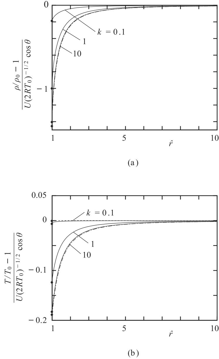
Figure 4.10. The density and temperature profiles in a uniform flow past a sphere with a uniform temperature (a hard-sphere gas). (a) (\rho/\rho_0 - 1)/U(2RT_0)^{-1/2} \cos \theta vs \hat{r} ( = r/L ) and (b) (T/T_0 - 1)/U(2RT_0)^{-1/2} \cos \theta vs \hat{r} . The solid lines — are the numerical solution and the black circles • indicate the values on the sphere. The dashed line --- is the asymptotic solution (4.112a) or (4.112d) with k = 0 , the former of which coincides with the thick upper frame and is invisible, and the dot-dash lines -.- are the free molecular solution (4.115a) or (4.115d).
