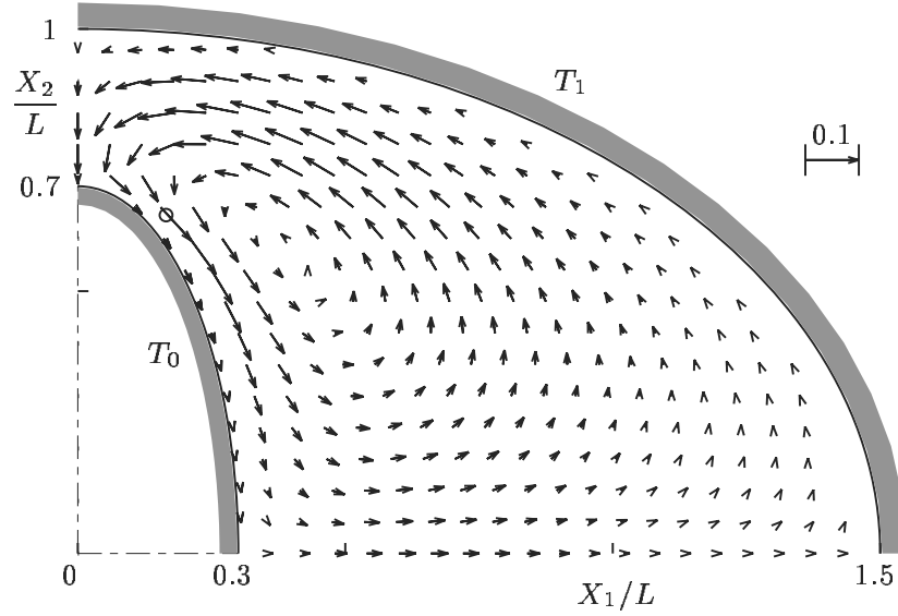
Figure 5.11. Nonlinear-thermal-stress flow induced between two coaxial elliptic cylinders with different uniform temperatures for a hard-sphere gas ( T_1/T_0 = 5 ; T_0 : temperature of the inner cylinder and T_1 : temperature of the outer cylinder). In view of the symmetry situation, the result in the first quadrant is shown. The arrows indicate the flow velocity \hat{v}_{iSB1} [ = \lim_{k \rightarrow 0} \mathbf{v}/(2RT_0)^{1/2}k ] at their starting points and the scale 0.1 of (\hat{v}_{iSB1}^2)^{1/2} is shown in the right upper space in the figure. The symbol \circ represents the point of the maximum speed. As is apparent in the figure, L is the half length of the minor axis of the outer ellipse. See the corresponding flow at various Knudsen numbers in Fig. 5.13 and note the direction of the flow. (The numerical computation of the asymptotic equations in Section 3.3.3 is carried out by Doi.)
