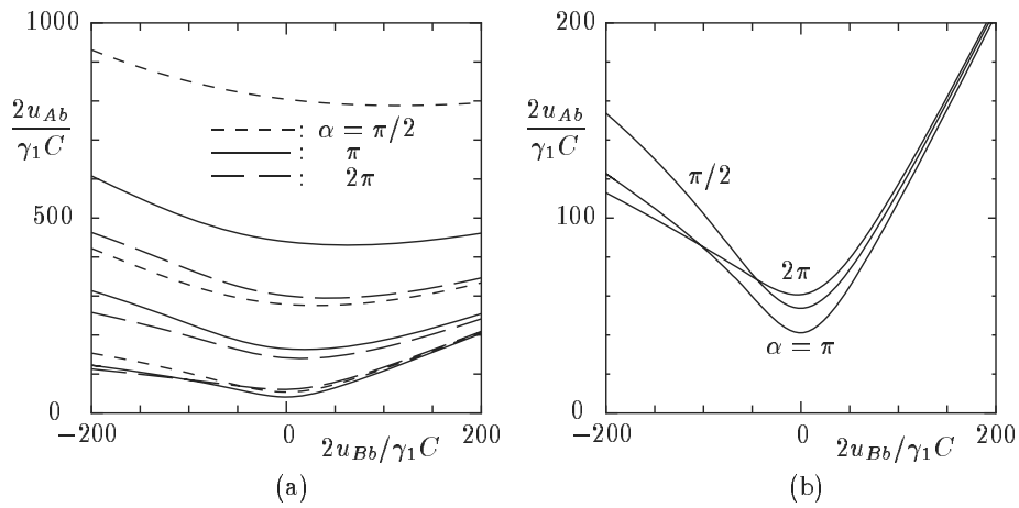
Figure 9.1. Bifurcation curves: 2u_{Ab}/\gamma_1 C vs 2u_{Bb}/\gamma_1 C for \alpha = \pi/2 , \pi , and 2\pi . (a) Wider range of 2u_{Ab}/\gamma_1 C showing three branches and (b) magnified figure of the first branch.
