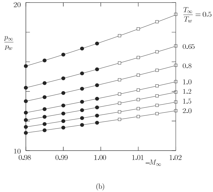
Figure 7.2. The surfaces F_s and F_{es} . (a) F_s and F_{es} in the neighborhood of M_\infty = -1 ; (b) Their sections T_\infty/T_w = 0.5, 0.65, 0.8, 1, 1.2, 1.5 , and 2 . In (a), the sonic line on the surfaces is shown as B-curve. In (b), the data ( \square ) for F_{es} lie on the extrapolated curves (—) of the data ( \bullet ) of F_s . The two surfaces are joined smoothly at the sonic points (along the B-curve).
