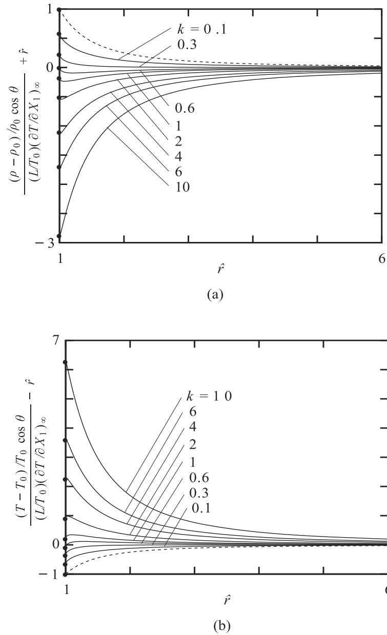
Figure 5.15. Density and temperature profiles in thermophoresis around a spherical particle with a uniform temperature for various k (a hard-sphere gas). (a) Density and (b) temperature. The solid lines — are the numerical solution, and the dashed lines --- are the asymptotic solution (5.11c) or (5.11d) with k = 0 . The black circle • indicate the values on the sphere.
