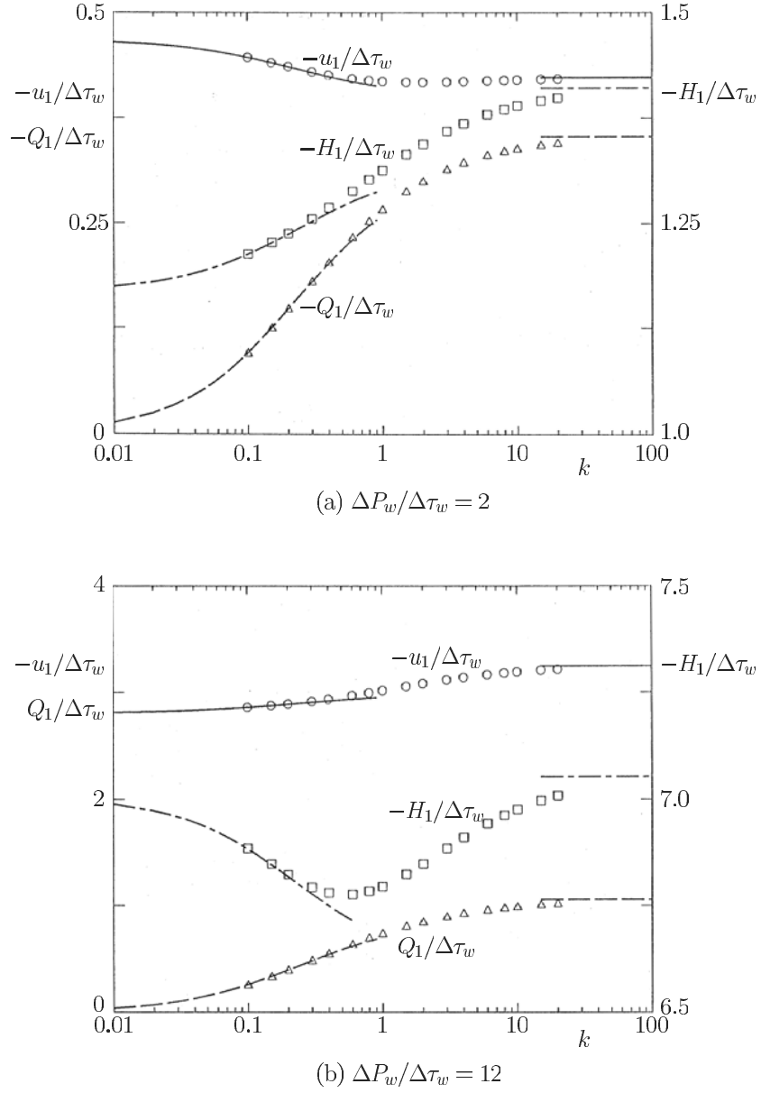
Figure 6.38. The variations of u_1 , Q_1 , and H_1 with k (a hard-sphere gas). (a) \Delta P_w/\Delta\tau_w = 2 and (b) \Delta P_w/\Delta\tau_w = 12 . The symbols \bigcirc , \triangle , \square : the numerical results, the curves for small k : the analytical results by the asymptotic theory (Section 3.1), and the straight lines for large k : those for the free molecular flow (Chapter 2). Note the difference of the sign of Q_1 in panels (a) and (b).
