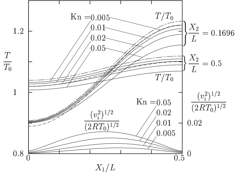
Figure 3.4. Comparison of the three kinds of solutions for the problem shown in Fig. 3.3 with \Delta\tau_w = 0.5 : I: Temperature distributions along X_2/L = 0.1696 and X_2/L = 0.5 and flow-speed distribution along X_2/L = 0.0227 . The solid lines —: the BKW equation for \text{Kn} = 0.005, 0.01, 0.02 , and 0.05 , the dot-dash lines ---: the asymptotic theory, and the dashed lines ---: the heat-conduction equation. Note the difference of the ordinate of T/T_0 from that of (v_i^2)^{1/2}/(2RT_0)^{1/2} . The solution of the kinetic equation converges to the solution by the asymptotic theory.
