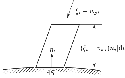
Figure 1.1. Explanatory figure for the formulas (1.3a)–(1.3c). The molecules with velocity \xi in the cylinder with its generatrices parallel to the relative velocity \xi_i - v_{wi} , its base given by the surface element dS , and its height given by |(\xi_i - v_{wi})n_i|dt will reach the surface element dS within time dt when (\xi_i - v_{wi})n_i < 0 and have left dS within time dt in the past when (\xi_i - v_{wi})n_i > 0 . Thus, total mass, momentum, and energy transferred by the molecules with their velocities in d\xi at \xi to the surface element dS in time dt are, respectively given by -f(\mathbf{X}, \xi, t)d\xi(\xi_j - v_{wj})n_j dS dt , -\xi_i f(\mathbf{X}, \xi, t)d\xi(\xi_j - v_{wj})n_j dS dt , and -\frac{1}{2}\xi_i^2 f(\mathbf{X}, \xi, t)d\xi(\xi_j - v_{wj})n_j dS dt . Summing up for all molecular velocities, we obtain the formulas (1.3a)–(1.3c).
