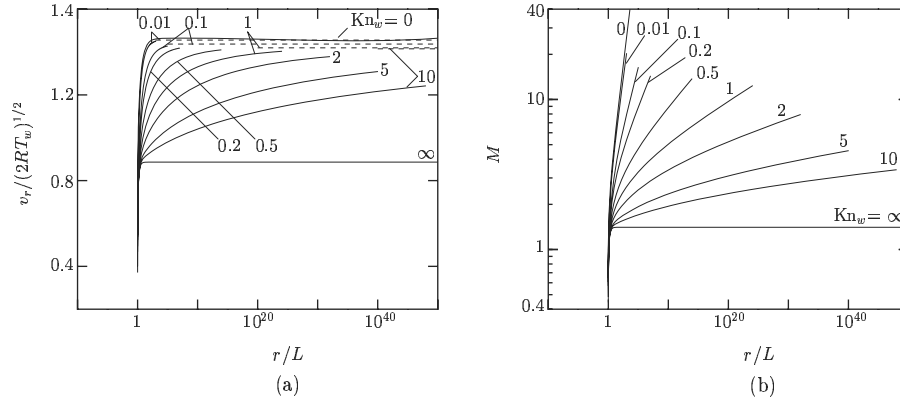
Figure 6.18. The profile of the macroscopic variables for various Knudsen numbers Kn_w in the evaporating flow from a cylinder into a vacuum II: flow velocity and Mach number. (a) v_r/(2RT_w)^{1/2} vs r/L and (b) M vs r/L . The data for Kn_w = 0, 0.01, 0.1, 0.2, 0.5, 1, 2, 5, 10 , and \infty are shown. The dashed lines in panel (a) indicate the limiting values of v_r (i.e., v_{r\infty} ) as r/L \rightarrow \infty [Eq. (6.29)] for Kn_w = 0.01, 0.1, 1 , and 10 .
