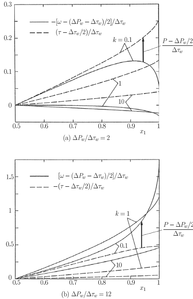
Figure 6.37. The distributions of the temperature \tau and density \omega in the gas for k = 0.1, 1 , and 10 in the negative temperature gradient problem (a hard-sphere gas). (a) \Delta P_w / \Delta \tau_w = 2 and (b) \Delta P_w / \Delta \tau_w = 12 . The profiles are antisymmetric with respect to x_1 = 0.5 . Note the difference of the signs for the curves in panels (a) and (b).
