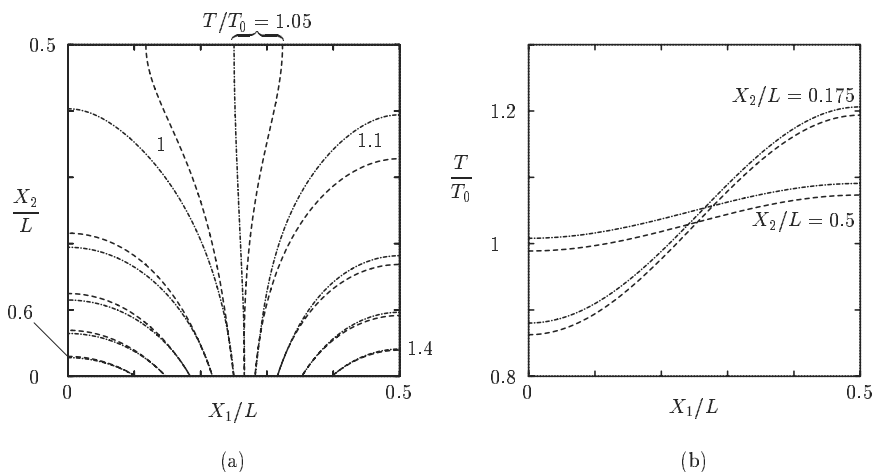
Figure 3.6. Comparison of the solutions of the asymptotic theory and heat-conduction equation for a hard-sphere gas in the problem shown in Fig. 3.3 with \Delta\tau_w = 0.5 . (a) The isothermal lines T/T_0 = 0.6 + 0.1m ( m = 0, 1, \dots, 8 ) and 1.05. (b) The temperature distributions along X_2/L = 0.175 and X_2/L = 0.5 . Here, the dot-dash lines \cdots : asymptotic theory and the dashed lines --- : heat-conduction equation.
