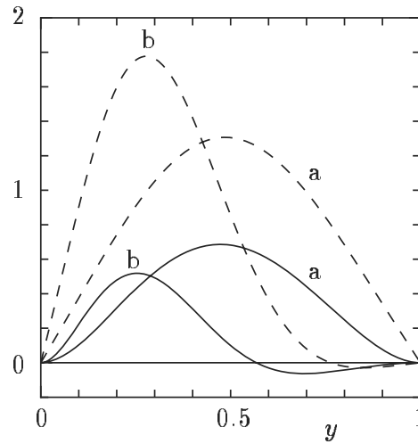
Figure 9.2. The profile U_{11}/||f_{11}|| and V_{11}/||f_{11}|| vs y , where ||f_{11}|| = [\int_0^1 (U_{11}^2 + V_{11}^2) dy]^{1/2} . The dashed lines --- are U_{11}/||f_{11}|| and the solid lines — are V_{11}/||f_{11}|| . The symbol a is for the case \alpha = \pi and 2u_{Bb}/\gamma_1 C = 0 , for which 2u_{Ab}/\gamma_1 C = 41.1705 , and the symbol b is for \alpha = 2\pi and 2u_{Bb}/\gamma_1 C = -150 , for which 2u_{Ab}/\gamma_1 C = 99.4753 .
