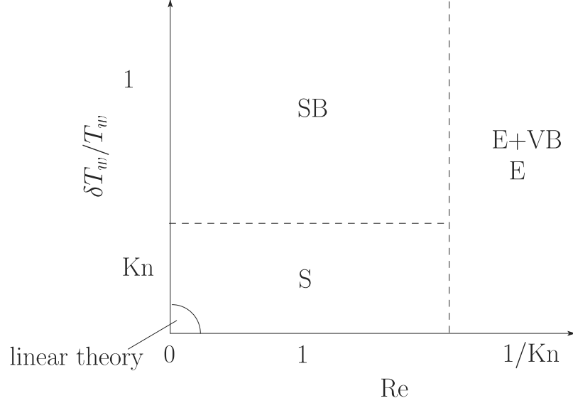
Figure 3.9. Fluid-dynamic-type systems describing the behavior of a gas of small Knudsen numbers ( \text{Kn} \ll 1 ) in the parameter plane (\text{Re}, \delta T_w/T_w) . In the region SB, the classical gas dynamics is inapplicable.
