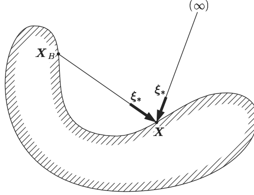
Figure 2.2. Free molecular gas around a nonconvex body.
