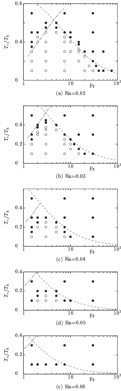
Figure 8.1. The range of the parameters Fr and T_c/T_h where a convection roll exists ( L/D = 1 and \varepsilon = 0.5 ). (a) Kn = 0.02 , (b) Kn = 0.03 , (c) Kn = 0.04 , (d) Kn = 0.05 , and (e) Kn = 0.06 . The white circle \circ indicates that convection occurs there; the black circle \bullet indicates that no flow occurs. See the main text for the dashed line --- and the dot-dash line — · —.
