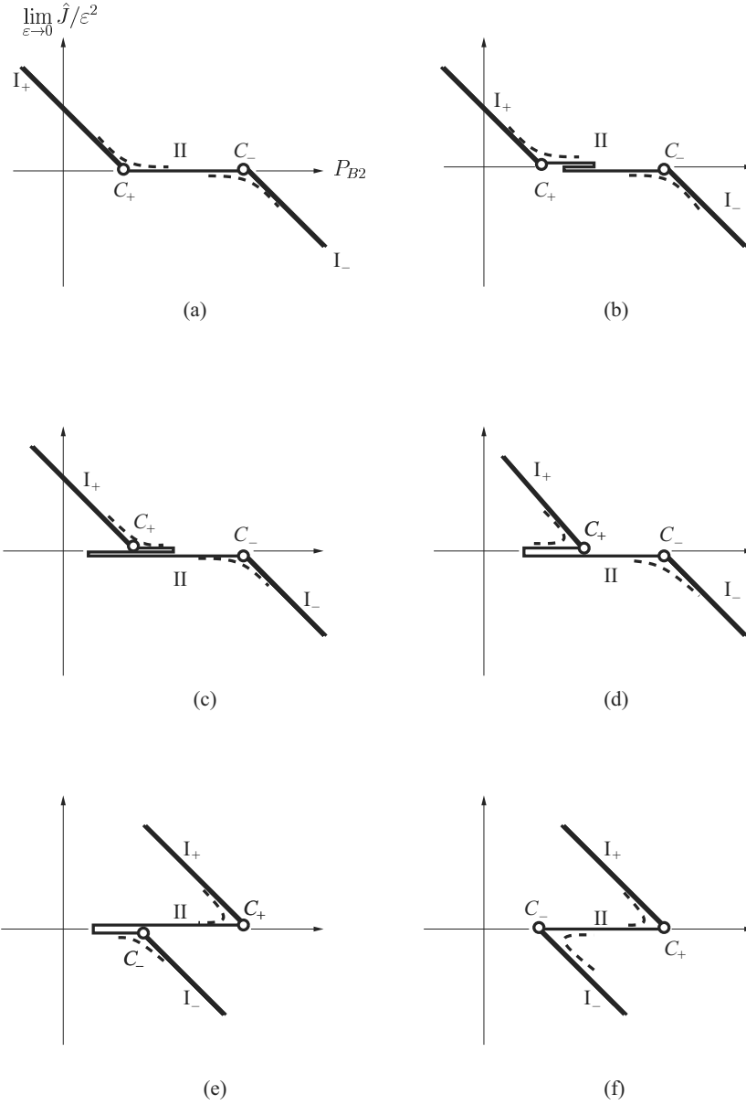
Figure 8.16. Bifurcation diagram (or schematic profiles \lim_{\varepsilon \rightarrow 0} \hat{J}/\varepsilon^2 vs P_{B2} ) of the axially uniform flow in the limit \varepsilon \rightarrow 0 for the parameter size given by Eq. (8.70) with m \geq 3 II: The two cylinders are rotating in opposite directions ( u_{\theta A1} u_{\theta B1} < 0 ). (a) (u_{\theta A1}/u_{\theta B1} \hat{r}_B)^2 \leq 1/9c_1 , (b) 1/9c_1 < (u_{\theta A1}/u_{\theta B1} \hat{r}_B)^2 < 1/9c_2 , (c) 1/9c_2 < (u_{\theta A1}/u_{\theta B1} \hat{r}_B)^2 < 1/9 , (d) 1/9 \leq (u_{\theta A1}/u_{\theta B1} \hat{r}_B)^2 < 1 , (e) 1 < (u_{\theta A1}/u_{\theta B1} \hat{r}_B)^2 < 9 , and (f) (u_{\theta A1}/u_{\theta B1} \hat{r}_B)^2 \geq 9 , where c_1 and c_2 depend on \hat{r}_B . The solution is indicated by thick or medium solid lines. The connection of the two solutions I and II by a transition solution is shown by a dashed line.
