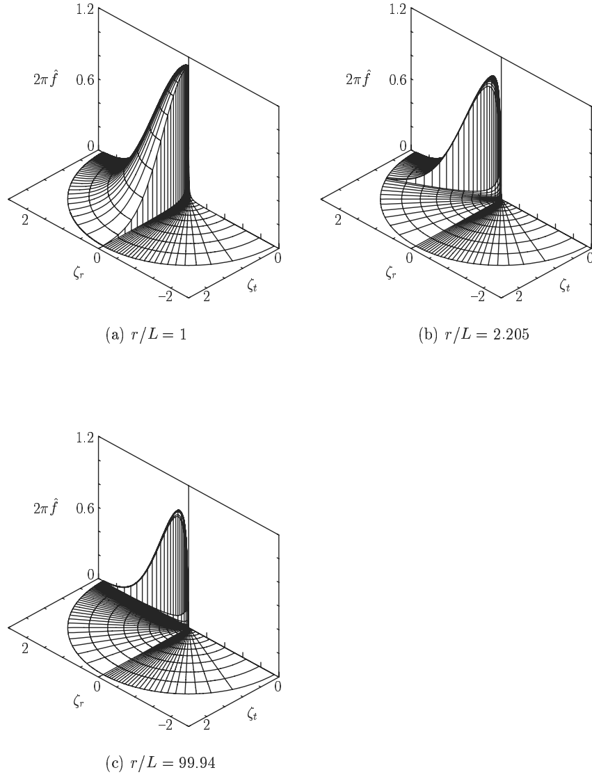
Figure 6.32. The velocity distribution function \hat{f} at various points in the evaporating flow from a sphere into a vacuum at \text{Kn}_w = 10 . (a) r/L = 1 , (b) r/L = 2.205 , and (c) r/L = 99.94 . The \zeta_t is defined by \zeta_t = (\zeta_\theta^2 + \zeta_\varphi^2)^{1/2} . The vertical stripes show the discontinuity of \hat{f} .
