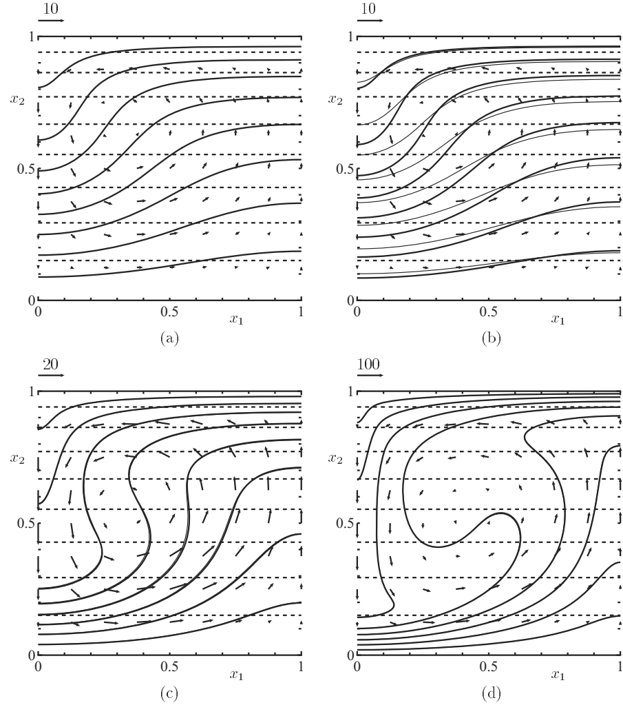
Figure 8.7. The bifurcated temperature field for a hard-sphere gas I: \hat{T}_B = 0.1 and x_{1B} = 1 . (a) \hat{g} = 320 , (b) \hat{g} = 328 , (c) \hat{g} = 1000 , (d) \hat{g} = 7000 . The solid lines indicate the isothermal lines [ \hat{T} = 0.1n ( n = 1, 2, \dots, 10 ) from the upper wall to the lower]; the arrows indicate u_i at their starting points and their scale is shown on the left shoulder of the figure. The thin lines indicate the corresponding results with the thermal stress effect neglected, and the dashed lines --- indicate the 1D solution.
