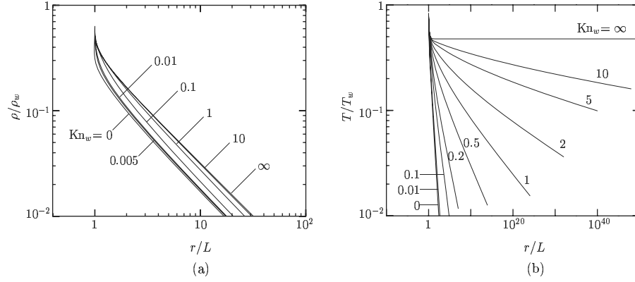
Figure 6.17. The profile of the macroscopic variables for various Knudsen numbers Kn_w of the evaporating flows from a cylinder into a vacuum I: density and temperature. (a) \rho/\rho_w vs r/L and (b) T/T_w vs r/L . In panel (a), the data for Kn_w = 0 (the continuum limit), 0.005, 0.01, 0.1, 1, 10, and \infty are shown. In panel (b), the data for Kn_w = 0, 0.01, 0.1, 0.2, 0.5, 1, 2, 5, 10 , and \infty are shown.
