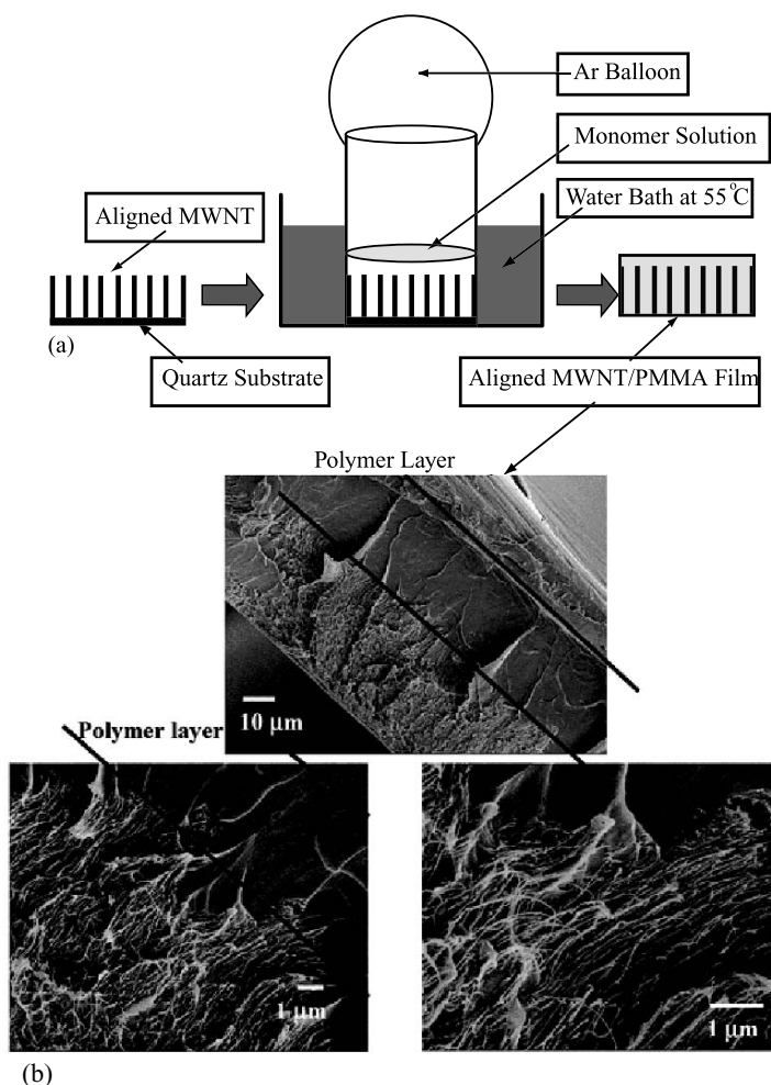
FIGURE 8.9. Schematics of process for making thickness-aligned MWNT/PMMA films: (a) Composite synthesis; (b) Cross-section of MWNT/PMMA films shows thickness-aligned MWNT ( \sim 30\ \mu\text{m} long) in PMMA matrix. An extra polymer ( \sim 20\ \mu\text{m} ) is observed over the nanotube arrays [84].
