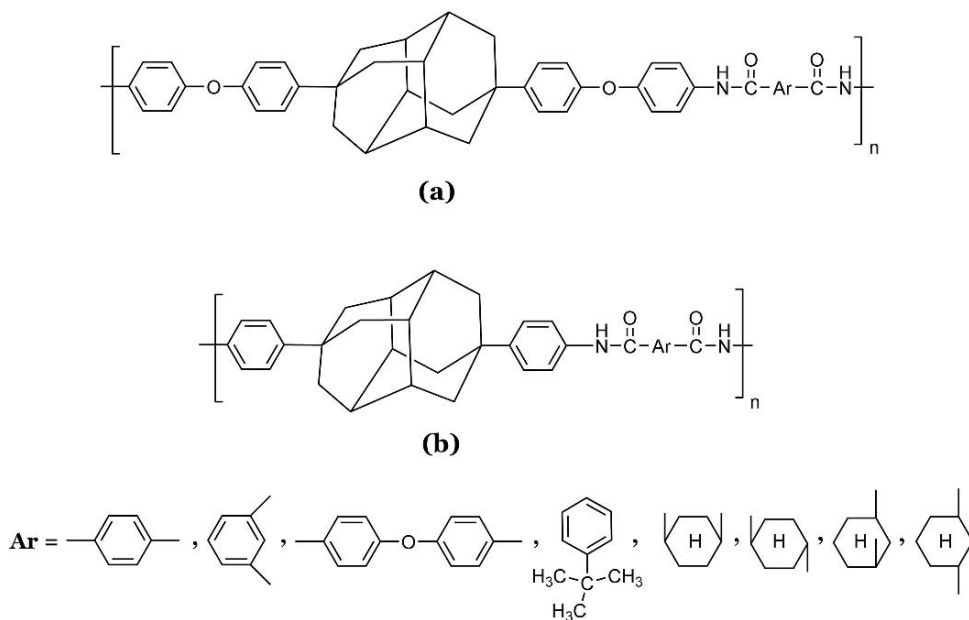
FIGURE 3.7. Diamantane-based polyamides; (a) derived from 4,9-bis[4-(4-aminophenoxy)phenyl]diamantane and (b) derived from 4,9-bis(4-aminophenyl)adamantane [42,43].
