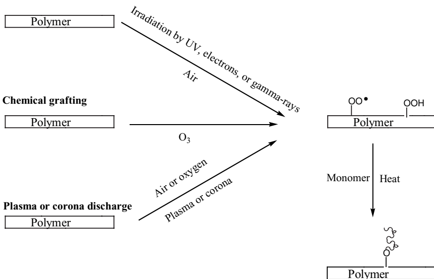
FIGURE 4.1. Various graft polymerization methods.
