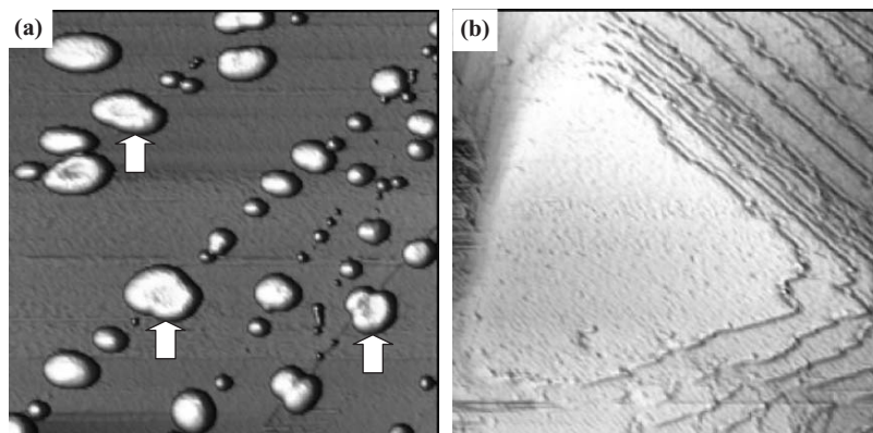
FIGURE 6.5. STM images of 3-D Sb islands on HOPG. (a) After 1.8-nm Sb deposited at RT and a flux of 1.8 \text{ \AA}/\text{min} ; (b) a facet on top of a 3-D island. Image area: (a) (2.5 \text{ }\mu\text{m})^2 ; (b) (60 \text{ nm})^2 .
