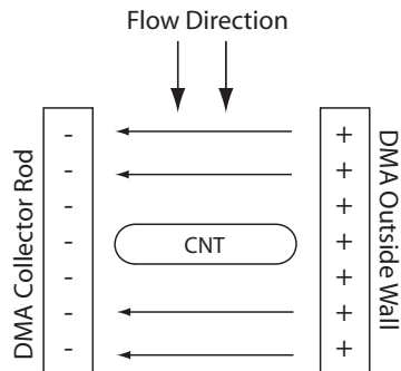
FIGURE 9.5. A schematic of a nanotube in the field of a DMA showing the CNT aligned with the electric field and normal to the flow direction.
