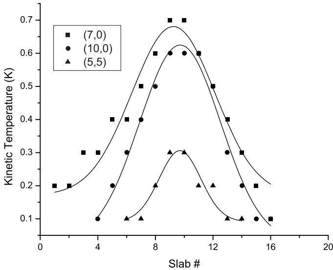
FIGURE 7.16. Shape of LA leading mode peak in (10,0), (7,0), and (5,5) SWNT at time = 4 ps. The line through the data points represents the best Guassian fit [62].
