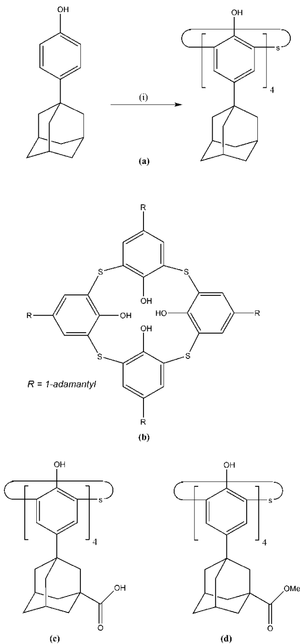
FIGURE 3.13. (a) Synthesis route of the molecule (b): (i) S8, NaOH, tetraethyleneglycol dimethyl ether, heat, (28%). (b) Adamantane Upper rim derivative based on the thiacalix[4]arene platform. (c),(d) The carboxylic acid and ester derivative of adamantane can be also used as substituents [61].
