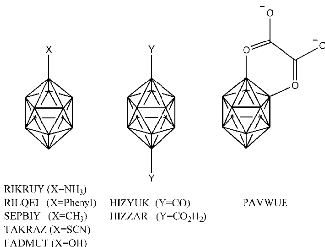
FIGURE 11.2. Some derivatives of closo -[B 12 H 12 ] 2- . Each vertex of the polyhedron represents a BH moiety.
