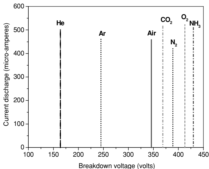
FIGURE 8.7. I–V curves for \text{NH}_3 , \text{CO}_2 , \text{N}_2 , \text{O}_2 , He, Ar and air, showing distinct breakdown voltages. Ammonia displays the highest breakdown voltage, and helium the lowest [56].
