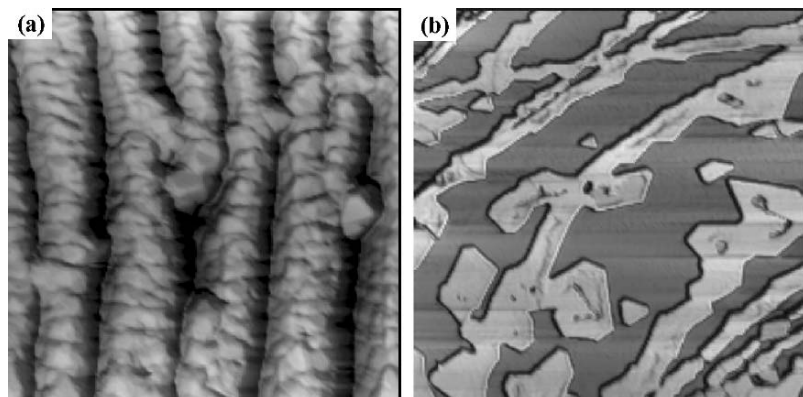
FIGURE 6.14. STM images of near-continuous films on HOPG. (a) After 30-nm Ge deposited at 190°C; and (b) 10-nm Al deposited at RT. Image area: (a) (1.5 \mu\text{m})^2 ; (b) (3.5 \mu\text{m})^2 .
