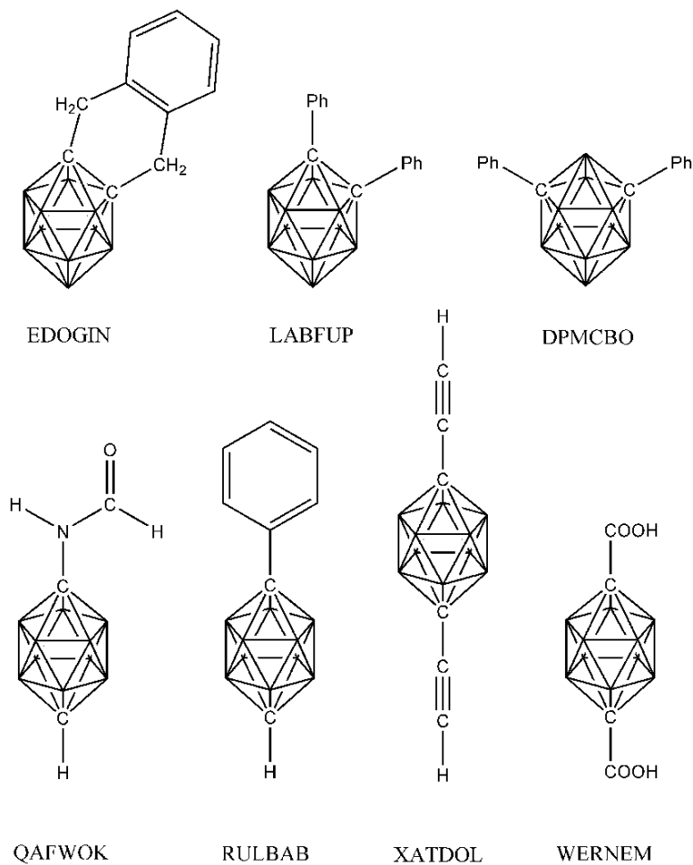
FIGURE 11.5. Some derivatives of o -, m -, and p -closo- \text{C}_2\text{B}_{10}\text{H}_{12} .
