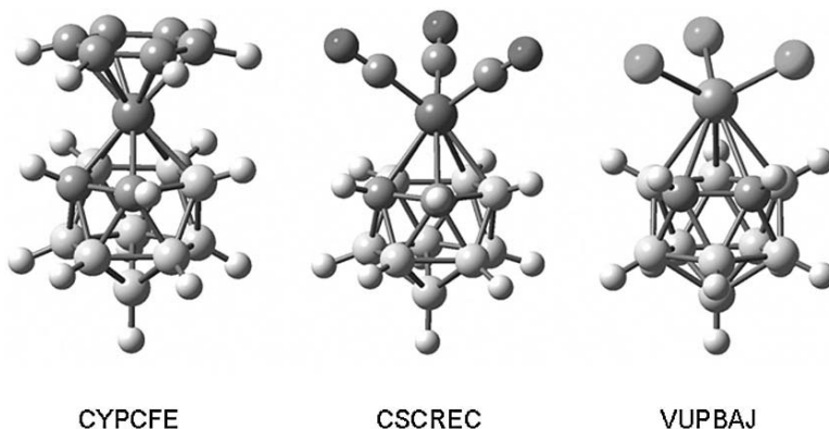
FIGURE 11.7. The structures of three metallacarboranes.
