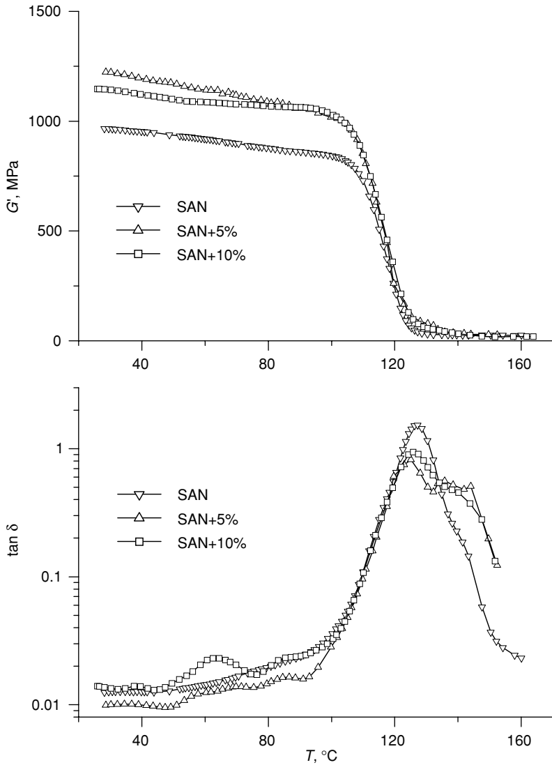
FIGURE 2.6. Temperature-dependences of G' and \tan \delta of SAN composites with diamond nanoparticles.
