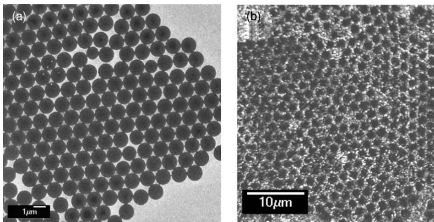
FIGURE 5.8. Selective growth of ZnO nanorods on patterned Al dots: (a) Patterned Al dots formed by the microsphere lithography methods, the triangularly shaped white regions between the black circles are areas coated with Al; (b) Selective nucleation of ZnO on the Al-coated regions.
