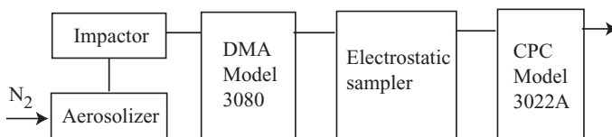
FIGURE 9.7. A flow diagram for the experimental setup.
