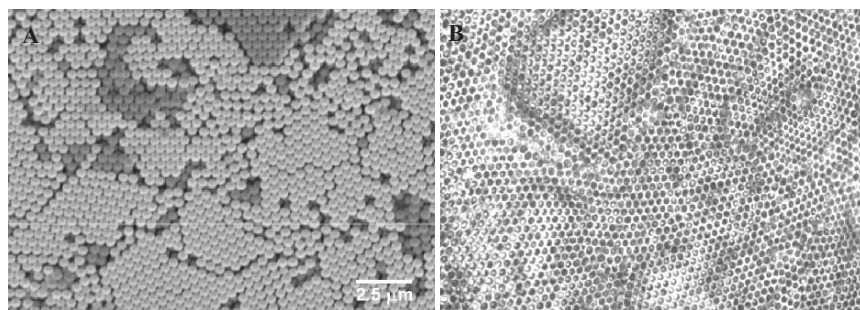
FIGURE 14.9. SEM image of polystyrene nanoparticles self-assembled on silicon substrate (A) and optical photograph of porous silica film fabricated using polystyrene nanoparticles as templates (B).
