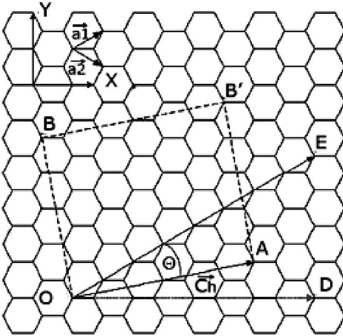
FIGURE 7.1. The unrolled hexagonal lattice of a nanotube.
