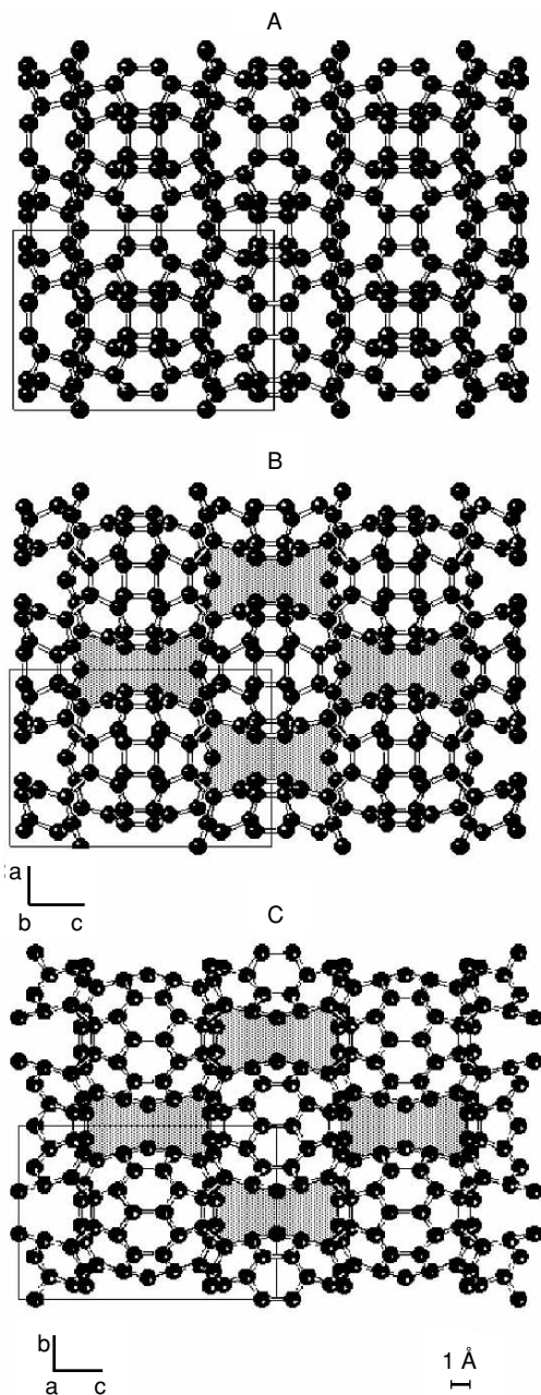
FIGURE 16.10. Projections of the structures of superhard phases A, B, and C on the lateral faces. Thin lines are unit cells; hatched areas are zeolite-like channels on the projections of the structures of phases B and C.
