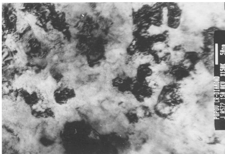
FIGURE 2.2. Structure of the chromium-nanodiamond coating (planar section).
