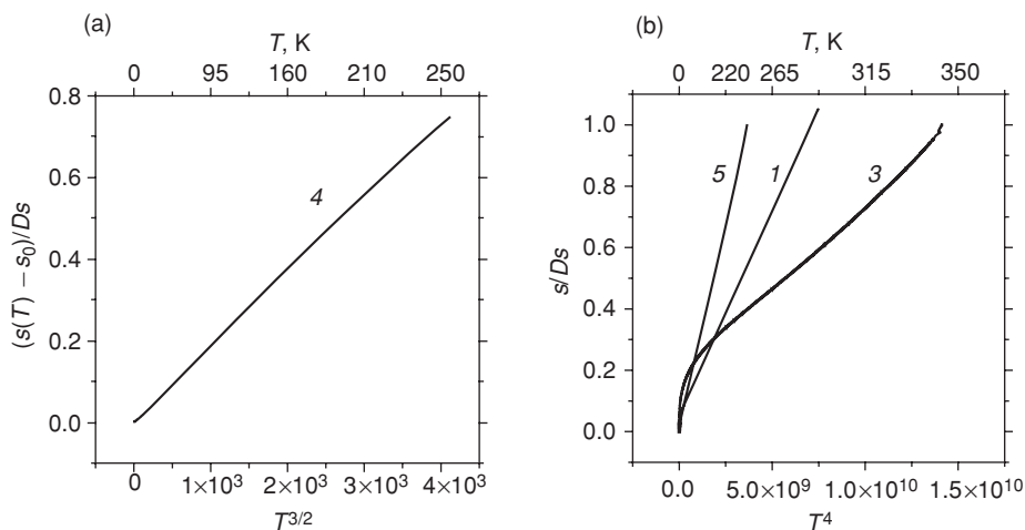
FIGURE 16.19. Power-law temperature dependences of the conductance of C_{60} samples with crystal and disordered 3-D-polymerized structures obtained at P = 11.5 -15 GPa and various temperatures of synthesis.
