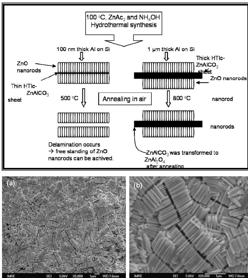
FIGURE 5.6. (Top) Schematic showing how the HTlc- \text{ZnAlCO}_3 -ZnO assembly can separate into free-standing ZnO bundles after thermal annealing. (Bottom) (a) and (b) SEM images of ZnO bundles after annealing in air at 500\text{ }^{\circ}\text{C} for 2 h; the HTlc- \text{ZnAlCO}_3 template has vanished.
