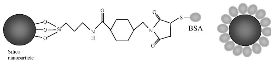
FIGURE 14.4. Conjugation of bovine serum albumin (BSA) to silica nanoparticles through 3-[(2-aminoethyl) amino] propyltrimethoxysilane (APTES) and 4-(N-maleimidomethyl) cycohexane-1-carboxylic acid 3-sulfo-N-hydroxysuccinimideester (sulfo-SMCC).
