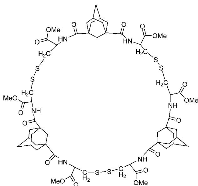
FIGURE 3.17. The cyclo (Adm-Cyst) 3 adopts a figure-eightlike helical structure. The chiral amino acid, cystine, configuration determines the helix disposition (right-handed or left-handed helix). Adamantane plays an important role as a ring size-controlling agent [66].
