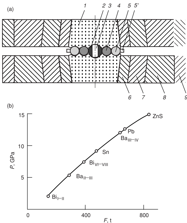
FIGURE 16.1. A method of high-pressure and high-temperature (HPHT) treatment of fullerenes. (a) The schematic of a toroid-type HPHT apparatus with the working-chamber diameter of 15 mm [1]. 1: hard-alloy punches; 6, 7, 8, 9: supporting steel rings; 3: zone where the heater and sample are placed; 2: container; 4: first sealing ring; 5 and 5': second and third sealing rings; (b) A calibration curve plotted by the changes of electrical resistance of the reference metals.
