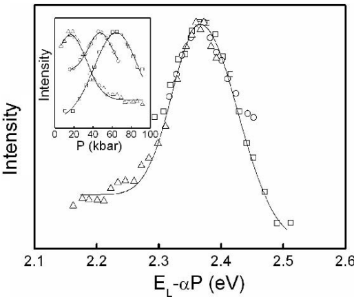
FIGURE 12.9. Normalized intensities of the Ge–Ge mode versus energies ( E_L - \alpha P ). The inset shows the normalized intensities of Ge–Ge mode resonant at different pressures for different excitation energies at 2.541 eV (squares), 2.496 eV (circles), and 2.41 eV (triangles). The solid curves are guides for the eye [3].
