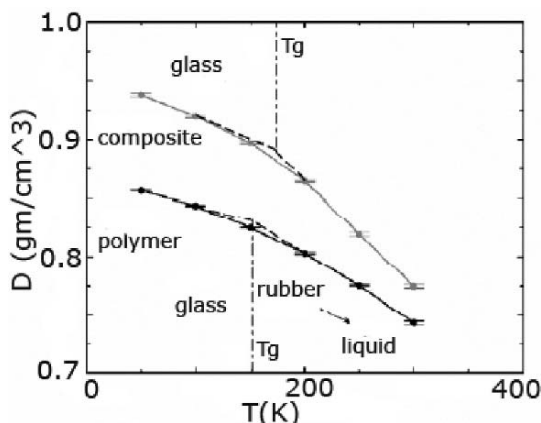
FIGURE 7.13. Density as a function of temperature for short-chained PE ( NP = 10 ) and its composite with 20 Å long (10,0) CNTs embedded (averaged from six sample sets; the error bars are shown in the plot). Below T_g , the systems are glassy state, and above T_g , will be in a rubberlike or liquid state if temperature is higher than melting point T_m [54].
