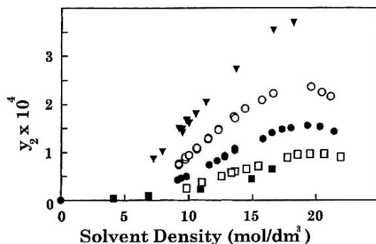
FIGURE 1.4. Comparison of solubilities of adamantane in CO 2 : (■), Smith and Teja (333 K); Swaid et al. (□) (343 K), (●) (362.5 K), (○) (382 K), (▼) (402 K).
