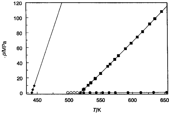
FIGURE 1.9. Phase diagram of diamantane. ■, Poot et al. (2003), ( s_2 + l ); ●, ( l + v ) Ref. (1 in Poot et al.); ▲, triple point; ○, ( s_2 + v ) Ref. (1 in Poot et al. 2003); ◆, ( s_2 + s_1 ) at temperature T and pressure p .
