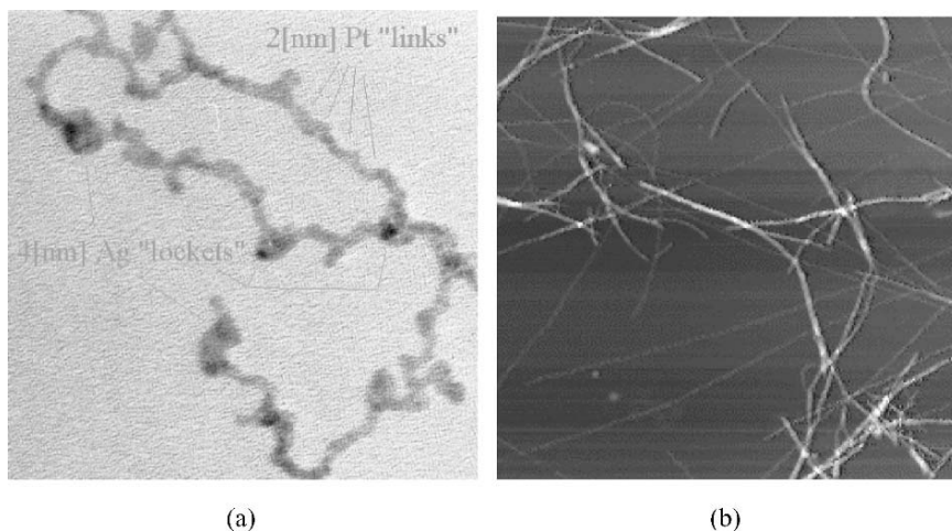
FIGURE 9.15. Two wet-mounted nanoassemblages: (a) “necklace” of 2-nm Pt crystals with Ag “loquets” in a 90-nm field, mounted on holey carbon film for TEM [82]; (b) 10- \mu\text{m} field of 10-nm wide amyloid protein fibrils mounted for SPM work on mica. Molecule affinities played a role in both (see text).
