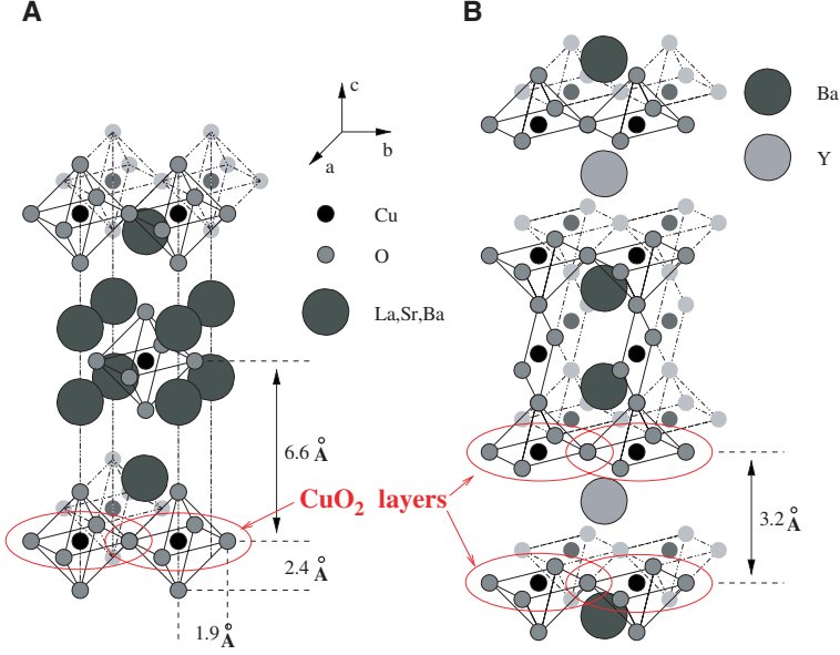
Fig. 9: Crystal structure of \text{La}_2\text{CuO}_4 (A) and \text{YBa}_2\text{Cu}_3\text{O}_7 (B)
