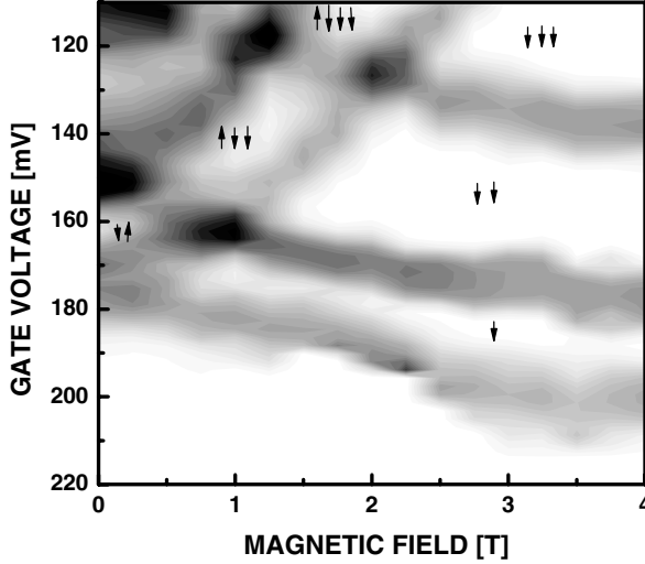
Fig. 3: Transconductance dG/dV_g ( gray scale ) showing dependence of 1D subbands on the magnetic field and gate voltage for PbTe nanoconstriction of a wide (Pb, Eu)Te/PbTe/(Pb, Eu)Te quantum well (after Grabecki et al. [35])
