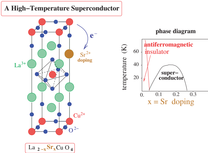
Fig. 8: Crystal structure of \text{La}_{2-x}\text{Sr}_x\text{CuO}_4 , and the effect of replacing (doping) La with Sr. Phase diagram as a function of doping x and temperature T
