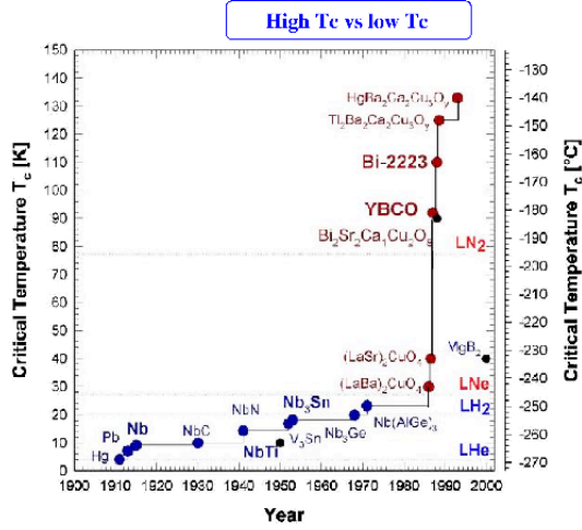
Fig. 2: The discovery of superconductivity: T_c versus years
