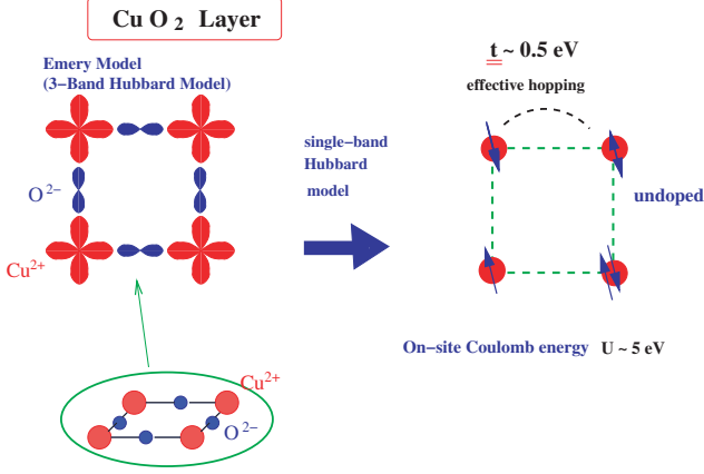
Fig. 10: The copper-oxide planes with their relevant orbitals. Modeling of these planes via a three- ( left ) and a single-band ( right ) Hubbard model
