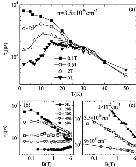
Fig. 1: Spin scattering time \tau_z of n-GaN at various magnetic fields (a), temperatures (b) ( n = 3.5 \times 10^{16} \text{ cm}^{-3} ), and electron concentrations at 5 K (c) (after Beschoten et al. [31])
