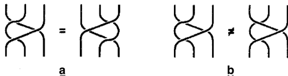
Fig. 5: Graphical representation of Eq. (25) (a) and Eq. (26) (b)
