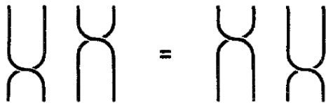
Fig. 6: Graphical representation of Eq. (27)
