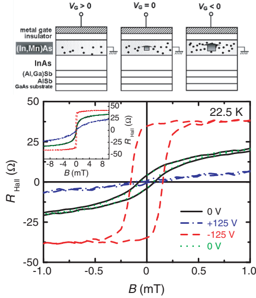
Fig. 14: Magnetization hysteresis loops determined by measurements of anomalous Hall effect at constant temperature of 22.5 K for various gate voltages in field-effect transistor with (In,Mn)As channel (after Ohno et al. [160])
