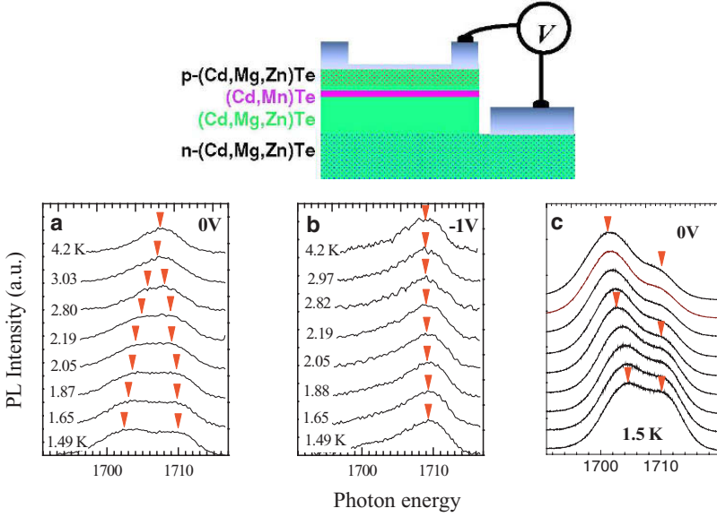
Fig. 15: Effect of temperature (a), bias voltage (b), and illumination (c) on photoluminescence of structure consisting of modulation doped p-(Cd,Mn)Te quantum well and n-type barrier. Zero-field line splitting (marked by arrows) witnesses the appearance of a ferromagnetic ordering (a) which does not show up if the quantum well is depleted from the holes by reverse bias of p-i-n diode (b). Low-temperature splitting is enhanced by additional illumination by white light (c), which increases hole concentration in quantum well (after Boukari et al. [161])
