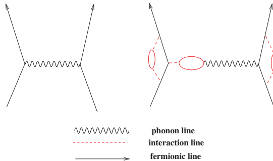
Fig. 16: A vertex correction to the phonon-mediated electron-electron interaction. Dashed lines describe the bare electron-electron interaction U , and wavy lines describe the phonon propagator
