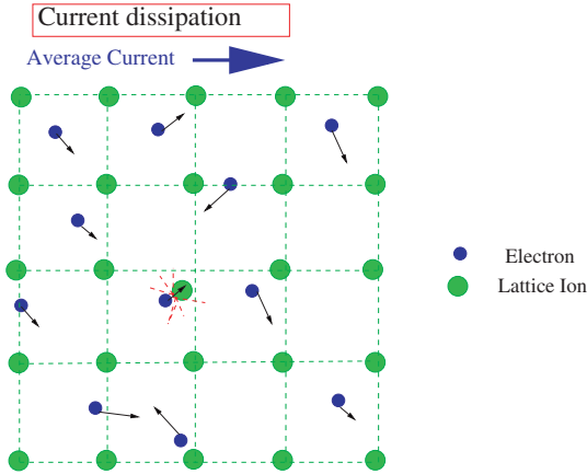
Fig. 3: Current dissipation in a non-superconducting state
