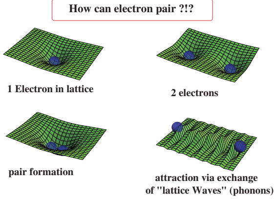
Fig. 5: Simple picture of the attraction between two “particles” due to a minimization of the elastic energy
