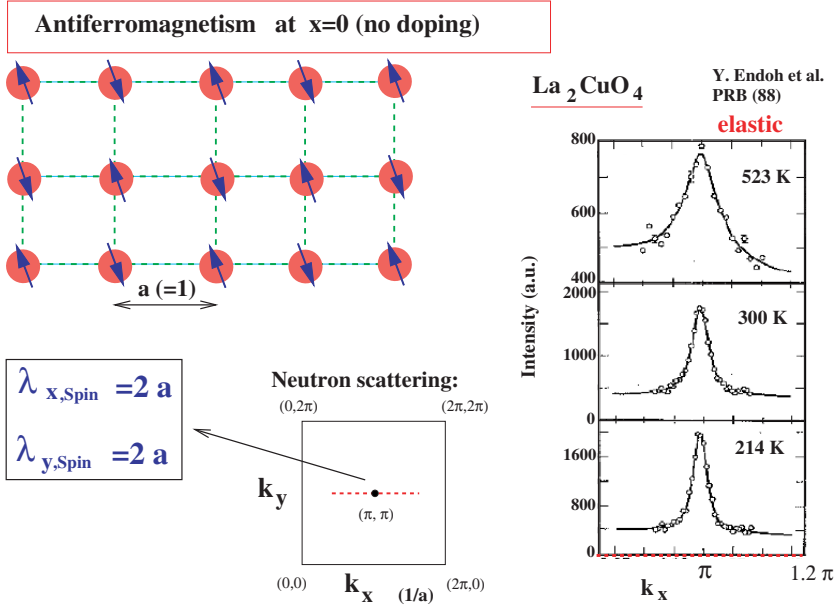
Fig. 14: Detecting antiferromagnetic order via neutron scattering
