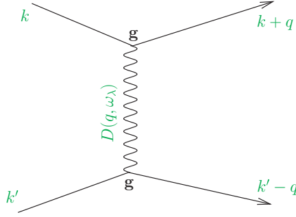
Fig. 7: Diagrammatic representation of the effective phonon-mediated electron-electron interaction. Solid lines are ingoing and outgoing electron lines (whose propagators don't contribute to the diagram). The wavy line is the phononic propagator D(q, \omega_\lambda)
