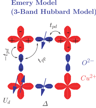
Fig. 11: Parameters of the three-band Hubbard model describing the most relevant orbitals in the \text{CuO}_2 layers
