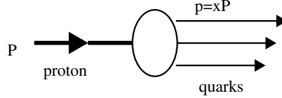
Fig. 3: The unpolarized quark density q(x)
