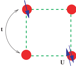
Fig. 12: Single-band Hubbard model
