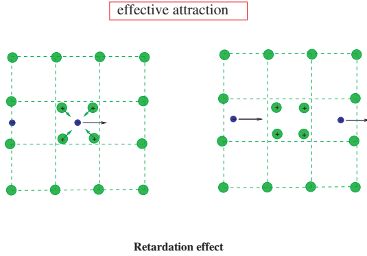
Fig. 6: Illustration of the retardation effect
