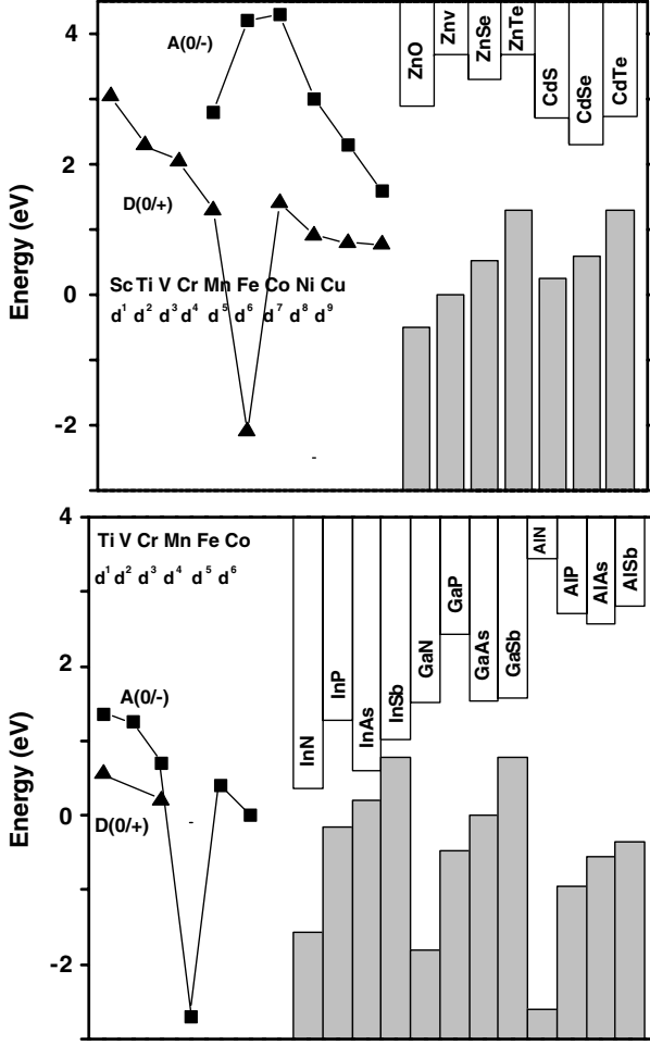
Fig. 6: Approximate positions of transition metals levels relative to the conduction and valence band edges of II-VI ( left panel ) and III-V ( right panel ) compounds. By triangles the d^N/d^{N-1} donor and by squares the d^N/d^{N+1} acceptor states are denoted (adapted from Langer et al. [57] and Zunger [58])
