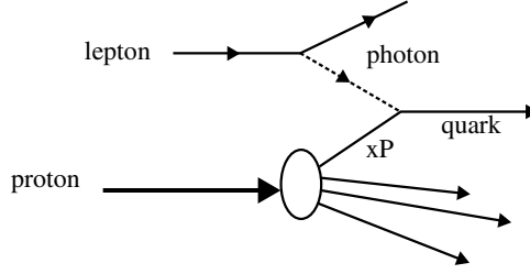
Fig. 2: Parton model interpretation of inelastic lepton-hadron scattering
