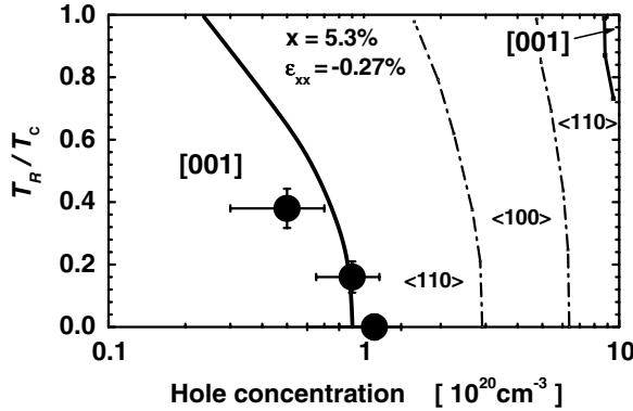
Fig. 7: Experimental ( full points ) and computed values ( thick lines ) of the ratio of the reorientation to Curie temperature for the transition from perpendicular to in-plane magnetic anisotropy. Dashed lines mark expected temperatures for the reorientation of the easy axis between \langle 100 \rangle and \langle 110 \rangle in-plane directions (after Sawicki et al. [111])
