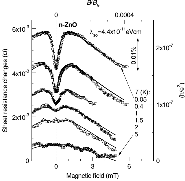
Fig. 2: Resistance changes in the magnetic field for n-ZnO ( symbols ) compared to calculations ( solid lines ) within the weak localization theory for the 2D case. Curves are vertically shifted for clarity (after Andrearczyk et al. [32])
