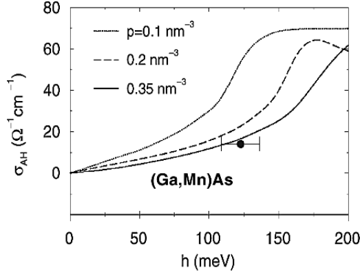
Fig. 11: Full numerical simulations of the anomalous Hall conductivity \sigma_{AH} for GaAs host with hole densities p = 10^{20} , (dotted lines), 2 \times 10^{20} (dashed lines), and 3.5 \times 10^{20} \text{ cm}^{-3} (solid lines). Filled circle represents measured Hall conductivity (Fig. 2). The saturation mean-field value of the splitting h between \Gamma_8 heavy hole subbands was estimated from nominal sample parameters. Horizontal error bar corresponds to the experimental uncertainty of the p-d exchange integral. Experimental hole density in the (Ga,Mn)As sample is 3.5 \times 10^{20} \text{ cm}^{-3} (after Jungwirth et al. [129])
