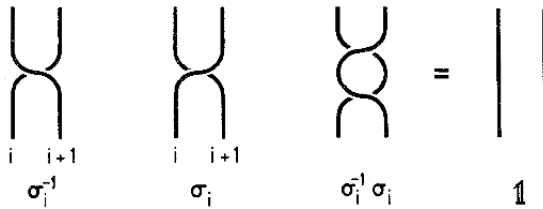
Fig. 4: The exchange operator \sigma_i and its inverse
