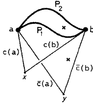
Fig. 1: Paths P_i are assigned to homotopy classes by connecting them to a base point through a mesh. Changing the base point from x to y can change the absolute class assignment of a path, but not the relative assignment of a pair of paths
