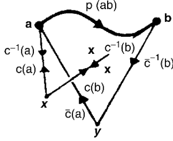
Fig. 2: Graphical representation of Eq. (20)
