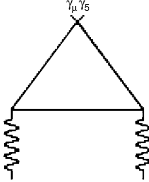
Fig. 6: The anomalous triangle diagram
