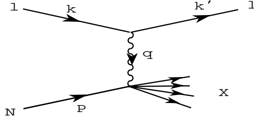
Fig. 1: Feynman diagram for inelastic lepton-hadron scattering
