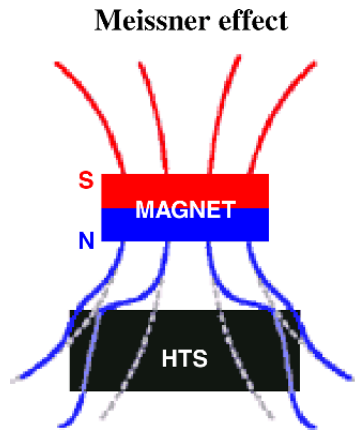
Fig. 1: Meissner effect. Magnetic-field lines are expelled from the bulk of a superconductor. Due to this effect, a magnet levitates on top of a superconductor
