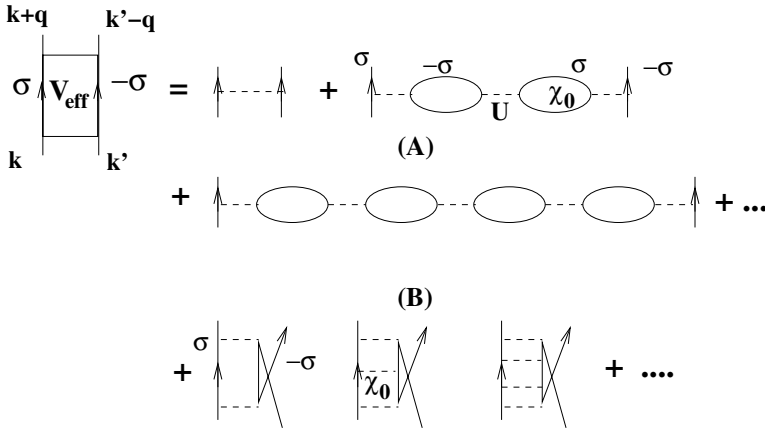
Fig. 15: Diagrams contributing to the effective interaction V_{eff,\uparrow\downarrow} between opposite spins. Diagrams in (B) contain the contribution from transverse spin fluctuations, not taken into account in Eq. (35). Dashed lines represent the Hubbard interaction U , solid lines are Fermion propagators. One closed fermionic loop (bubble) corresponds to the polarisability \chi_0
