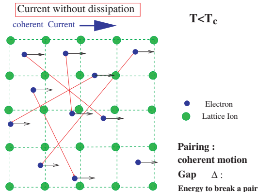
Fig. 4: Superconducting state made of a rigid coherent state of Cooper pairs
