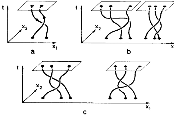
Fig. 3: Braids defined by particles' trajectories
