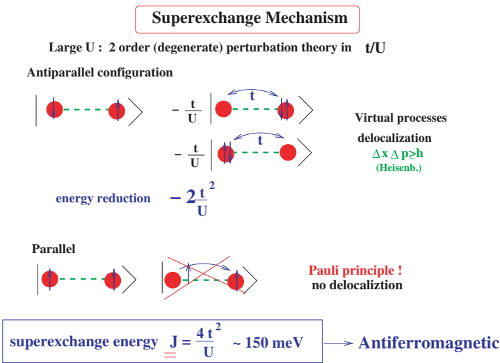
Fig. 13: Superexchange mechanism: due to Pauli principle, the electron spins on two neighboring site prefer to stay antiparallel in order to gain the energy \propto -t^2/U
