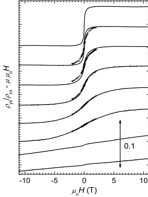
Fig. 12: Comparison of the normalized anomalous Hall effect ( lines ) with the normalized magnetization M/M_S ( crosses ); from top to bottom : 1.7, 2.8, 4.2, 7, 10, 30, and 50 K; the data are shifted for clarity (after [138])
