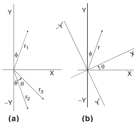
Fig. 6.2. Two interpretations of the orthogonal matrix A_2 whose determinant is -1 . (a) As an operator, it flips the vector r_1 to r_2 symmetrically with respect to X -axis, and then rotates r_2 to r_3 . (b) As the transformation matrix between the tip of a fixed vector when the Y -axis is inverted and then the coordinate axes are rotated. Note that the rotation in (b) seems to be in the same direction as in (a)
