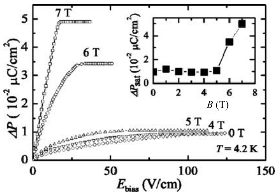
Fig. 7.14. Relative change of polarization \Delta P in \lambda -(BETS) _2\text{FeCl}_4 as a function of E_{\text{bias}} at T = 4.2 \text{ K} and B = 0 - 7 \text{ T} . The inset shows the magnetic-field dependence of the saturation value \Delta P_{\text{sat}} . After [1108].
