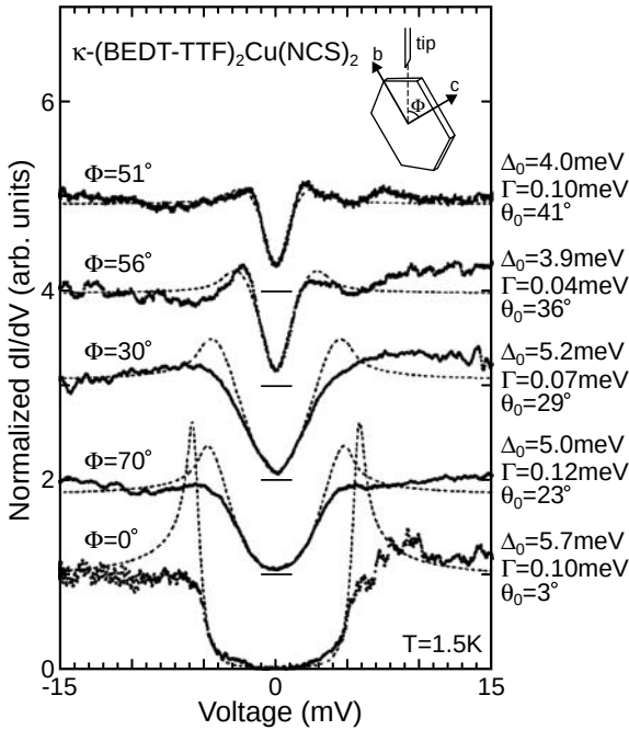
Fig. 6.24. dI/dV - V curves taken at 1.5 K on the lateral surfaces of \kappa -(ET) _2 Cu(NCS) _2 single crystals. Data have been taken along various tunneling directions at different angles \phi as defined in the inset. The dashed line represents the calculated curve based on the d -wave gap model with a k -dependent tunneling. After [941].
