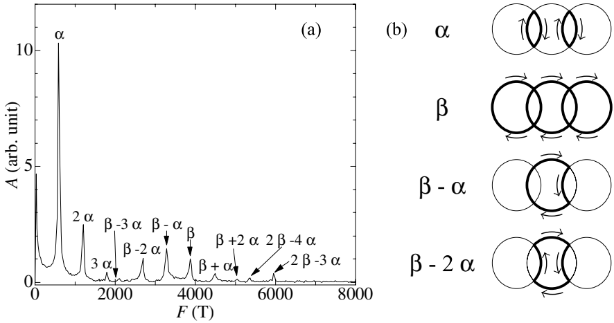
Fig. 5.7. (a) Fourier-transform spectrum of the SdH oscillations in \kappa -(ET) 2 Cu(NCS) 2 shown in Fig.5.6(a). (b) Schematic illustrations for the typical orbits corresponding to the spectrum's peaks at F_\alpha , F_\beta , F_{\beta-\alpha} and F_{\beta-2\alpha} . After [447].
