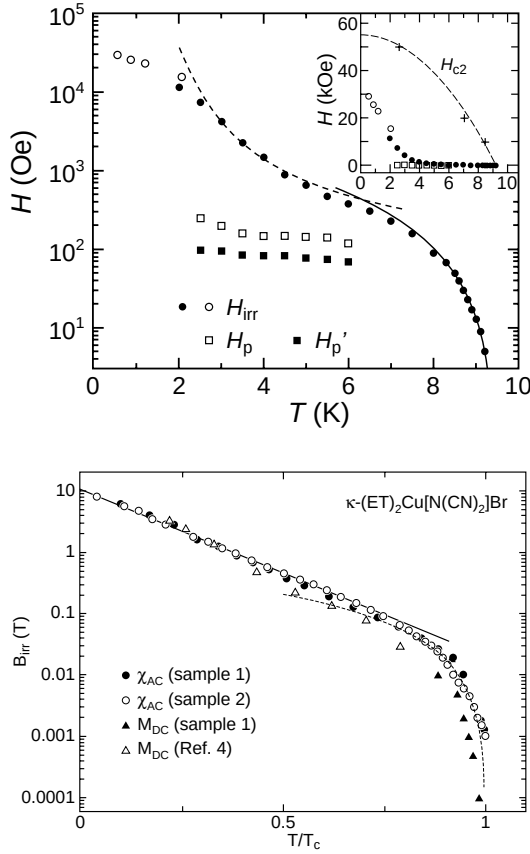
Fig. 6.14. Irreversibility field on a logarithmic scale as a function of temperature for \kappa-(ET)_2Cu(NCS)_2 (linear temperature scale, top) and \kappa-(ET)_2Cu[N(CN)_2]Br (reduced temperature scale, bottom), after [892] and [860], respectively. The vortex lattice is melted in the field and temperature region above the irreversibility lines in each case (see text). In both cases the data can be described by an exponential dependence B_{irr} \propto \exp(a/T) in the high-field/low-temperature (quasi-2D) regime and a power law B_{irr} \propto (1 - T/T_c)^\alpha in the low-field/high-temperature (3D) regime marking a dimensional crossover in the vortex system. For \kappa-(ET)_2Cu(NCS)_2 (upper panel) the second peak in magnetization B_p (or the peak in the magnetic field derivative B_p' ) mark the almost temperature-independent crossover field. The inset also shows the upper critical field curve.
