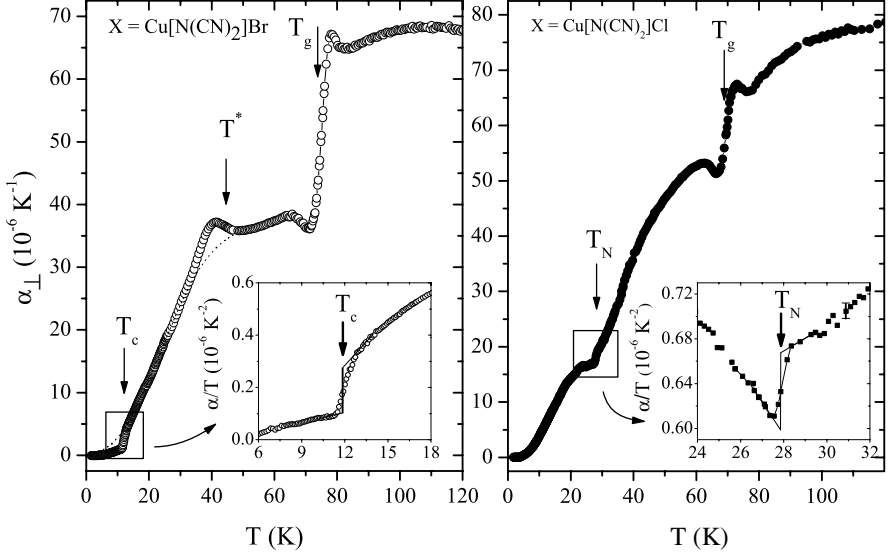
Fig. 4.19. Linear thermal expansion coefficient perpendicular to the planes of highest conductivity, \alpha_{\perp} , as a function of temperature for superconducting \kappa -(ET) 2 Cu[N(CN) 2 ]Br (left panel) and insulating \kappa -(ET) 2 Cu[N(CN) 2 ]Cl (right panel). The inset shows details of \alpha_{\perp} for both salts as \alpha_{\perp}/T vs T at the superconducting ( X=\text{Cu}[\text{N}(\text{CN})_2]\text{Br} ) and antiferromagnetic ( X=\text{Cu}[\text{N}(\text{CN})_2]\text{Cl} ) phase transition. Arrows indicate different kinds of anomalies as explained in the text. After [155]
