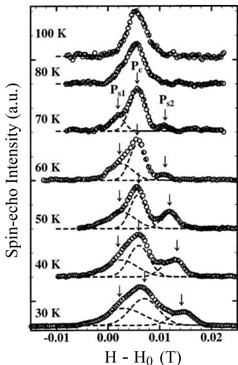
Fig. 7.11. Profiles of field-swept ^1\text{H} -NMR spectra (94.95 MHz) in \lambda -(BETS) _2\text{FeCl}_4 . The dashed lines indicate the Gaussian deconvolution with three components, P_c , P_{s1} , and P_{s2} , the peak positions of which are shown by arrows. After [1100].
