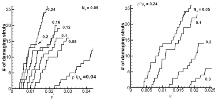
Fig. 4 Effect of relative density and N_s on the damage development
