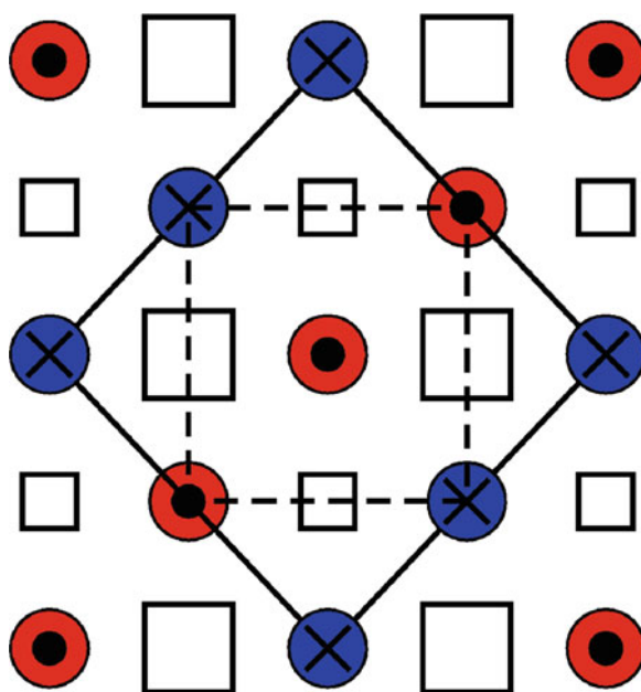
Fig. 5.1 Top view of a FeAs layer. The Fe atoms are marked by dark circles . The As atoms above the plane are indicated by larger squares , below the plane – by smaller squares [88]
