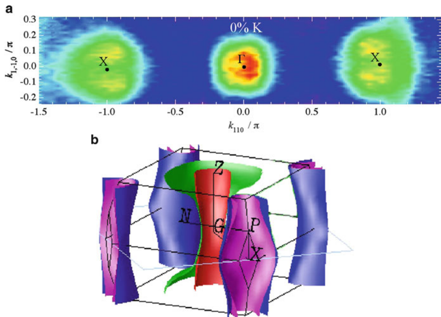
Fig. 3.7 ARPES data for \text{BaFe}_2\text{As}_2 (a) in comparison with the calculated Fermi surface (b) [147]
