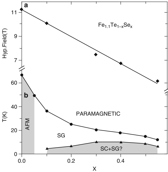
Fig. 5.44 Phase diagram of the \text{Fe}_{1.1}\text{Se}_x\text{Te}_{1-x} system with a region of coexistence of superconductivity and spin glass, as established by Mössbauer spectroscopy [458]: (a) variation of the mean hyperfine field at the Fe nucleus with the Se concentration; (b) phase diagram in the (T, x) -plane
