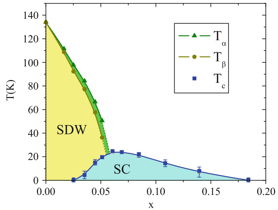
Fig. 3.14 Phase diagram of the \text{Ba}_{1-x}\text{Co}_x\text{Fe}_2\text{As}_2 with the electron doping [182]
