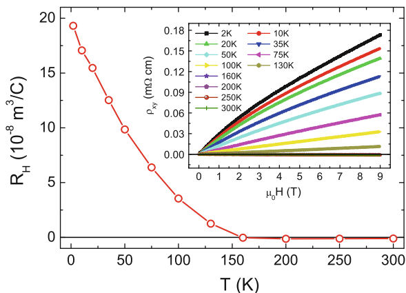
Fig. 4.12 Temperature dependence of the Hall constant for a sample of SrFeAs [354]. Inset: Hall resistivity \rho_{xy} as function of magnetic field at different temperatures
