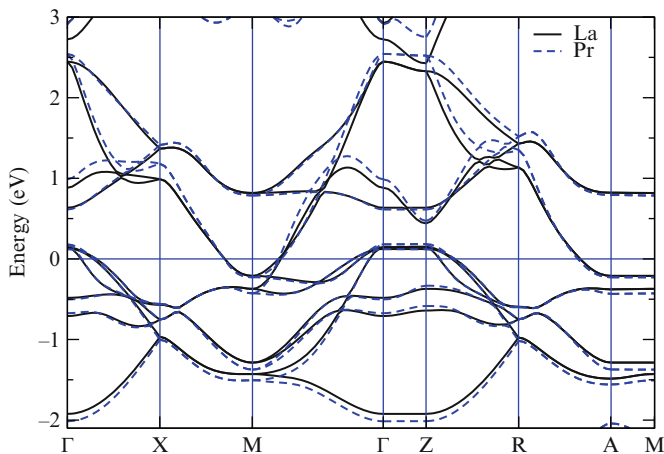
Fig. 2.26 Band structure of LaOFeAs (solid line) and PrOFeAs (dashed line), after [82]
