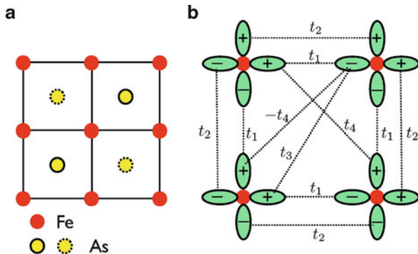
Fig. 5.21 Crystal and electron structure of the FeAs layer. (a) Positions of Fe atoms (in the plane) and As atoms above and below the Fe-plane ( solid and dotted circles, correspondingly); (b) orientation of the d_{xz} and d_{yz} orbitals of the Fe atoms and matrix elements of the electron hopping between the nearest and the next-nearest Fe neighbours [404]
