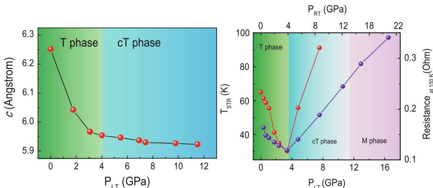
Fig. 4.5 Pressure dependence of the lattice parameter and the structural phase transition temperature in \text{Fe}_{1.05}\text{Te} , after [325]
