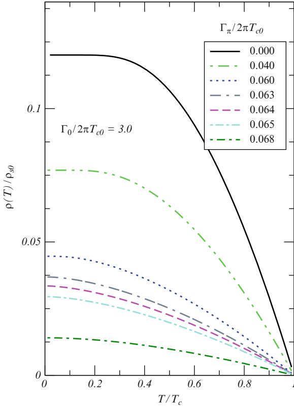
Fig. 5.45 Superfluid density \rho_s(T) depending on the magnitude of the depairing parameter \Gamma_\pi/T_{c0} for a superconductor with the s^\pm -symmetry of the order parameter [459]
