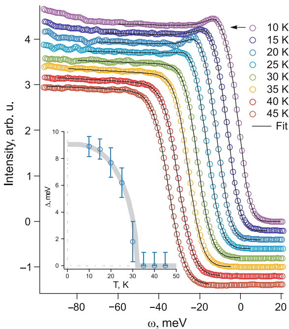
Fig. 3.32 Evolution of the emission spectra along the cut1 of the inner sheet of the Fermi surface (see Fig. 3.31) near \Gamma with temperature. In the inset: temperature dependence of the superconducting gap extracted from these data with the use of the BKFA fitting [246]
