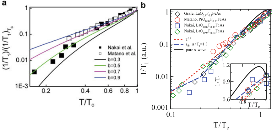
Fig. 5.30 Temperature dependence of 1/T_1 for a superconductor of the s^\pm -type with non-magnetic impurities, as calculated in [423] (a) and [424] (b), in comparison with experimental NMR data
