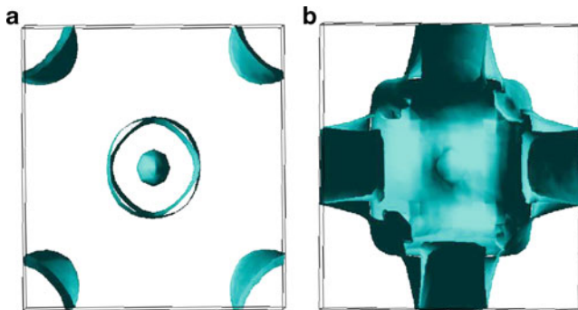
Fig. 4.8 Fermi surface of FeTe as function of doping \delta : (a) \delta \sim 0.0 , (b) \delta \sim 0.5 electrons per formula unit [323]
