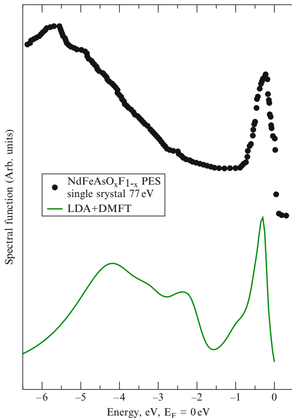
Fig. 5.17 Calculated full spectral function ( solid line ) and experimental photoemission spectrum of LaOFeAs [392]
