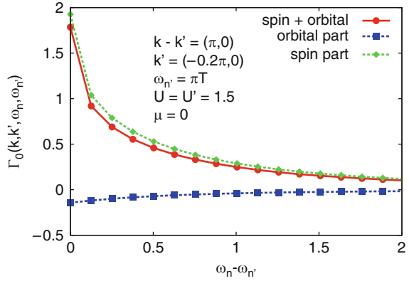
Fig. 5.36 Frequency dependence of the spin and charge contributions into the pairing interaction \Gamma(\mathbf{k}, \mathbf{k}', \omega_n, \omega_{n'}) [430]
