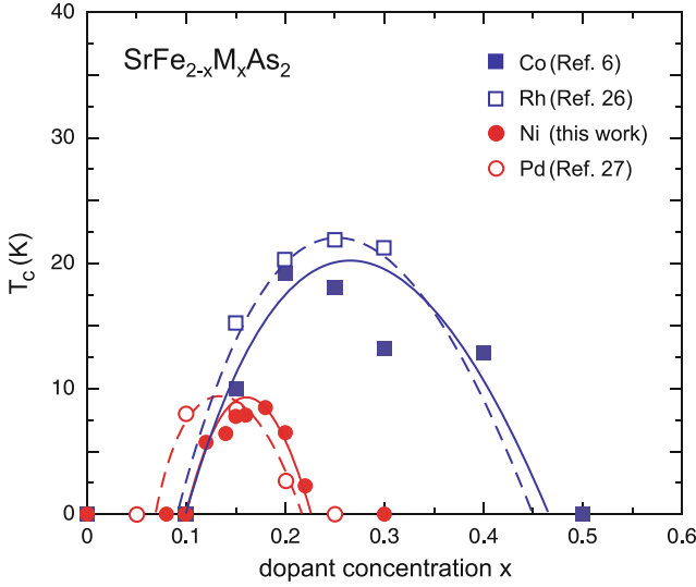
Fig. 3.15 Comparison of T_c(x) dependencies for some \text{SrFe}_{2-x}\text{M}_x\text{As}_2 compounds at different dopants M substituting Fe; M = Co [204], Rh [205], Ni [206], Pd [194]
