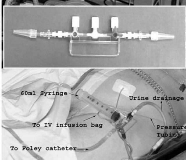
Fig. 4 A A closed needle-free revised method for measurement of intra-abdominal pressure. A standard intravenous infusion set is connected to a bag of 1,000 ml of normal saline and attached to the first stopcock. A 60-ml syringe is connected to the second stopcock and the third stopcock is connected to a pressure transducer via rigid pressure tubing. The system is flushed with normal saline and the pressure transducer is zeroed at the symphysis pubis. To measure IAP, the urinary drainage tubing is clamped distal to the ramp-device, 50 ml of normal saline is aspirated from the IV bag into the syringe and then instilled in the bladder. After opening the stopcocks to the pressure transducer mean IAP can be read from the bedside monitor. See ESM addendum 4 for explanation. B Mounted patient view of the device and close up of manifold and conical connection pieces
