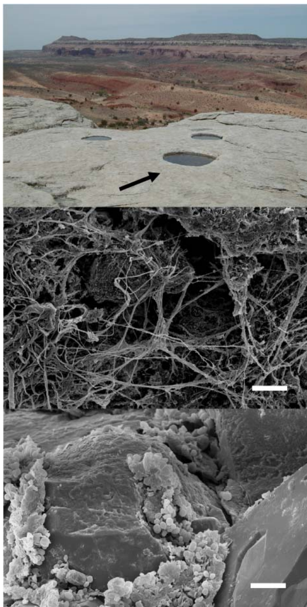
Fig. 2 A photograph of a pothole at Barlett Wash, near Moab, NM. Upon hydration, the previously desiccated biofilm in bottom of the pothole (the black lining seen in top panel ) begins to grow and can be observed using scanning electron microscopy ( middle ). Growth of these surface exposed biofilms ( middle ) is presumably more ephemeral than the endolithic organisms found within the sandstone ( bottom ). Higher, eukaryotic organisms, such as snails are supported by this bacterially-based food chain (see Chan et al. 2005). Micrographs provided by A. Welty. The pothole indicated by the arrow is approximately 1 m in diameter; bars equal 50 \mu\text{m} and 10 \mu\text{m} , respectively
