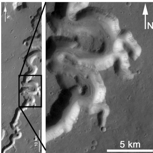
Fig. 15 Nanedi Vallis on Mars. Meander, terraces and interior channels indicate fluvial origin of the sinuous surface feature. (Mars Express HRSC image ESA/DLR/FUB (G. Neukum) HSRC orbit 905, 5.25°N 311.8°E)
