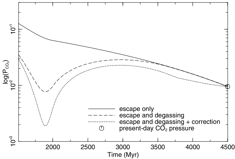
Fig. 3 Evolution of the maximum \text{CO}_2 pressure in the atmosphere of Mars over the last three billion years. The solid curve shows only atmospheric escape as described in Chassefière et al. (2007). The dashed curve shows escape and includes degassing of \text{CO}_2 by crust production using results from Breuer and Spohn (2006). The dotted curve uses the same model as the dashed one but adds a corrective factor for late activity which is not present in the crust production model
