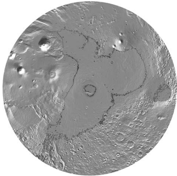
Fig. 7 Possible shoreline. This view, looking down on the north poles, shows the -3760 m contour, which roughly corresponds to the lowest shoreline proposed by Parker et al. (1989, 1993). The volume below the contour is 2 \times 10^7 \text{ km}^3 , and is indicative of the size of a body of water that would be left after one of the largest floods
