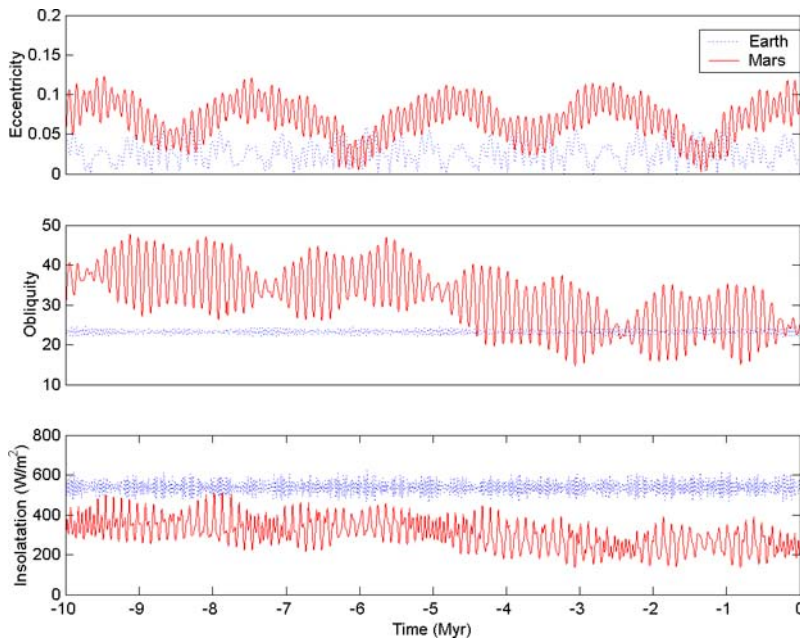
Fig. 1 Variations of the Martian orbital parameters and of the Martian North Pole summer insolation over the last 10 Myr (from the calculations of Laskar et al. 2002, 2004a)
