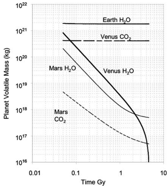
Fig. 16 Model describing the mass loss of \text{H}_2\text{O} and \text{CO}_2 on Venus, Earth and Mars by solar forcing. Strong magnetic shielding assumed for the Earth, no magnetic shielding for Venus, and options with and without magnetic shielding (up to 0.5 Gyr) for Mars. The \text{H}_2\text{O} inventory on the Earth remains essentially unaltered, while Mars and Venus have been subject to major losses
