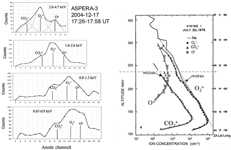
Fig. 13 Left: Ion mass spectra illustrating the composition of ionospheric outflow from Mars, with \text{O}_2^+ being most abundant, \text{O}^+ coming second and \text{CO}_2^+ coming third. The composition is similar to that observed by the Viking-1 spacecraft at an altitude of about 240 km (figure obtained from Hanson et al. 1977)
