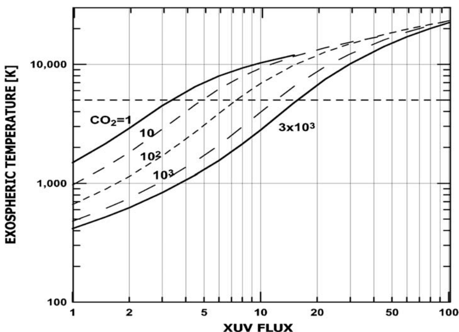
Fig. 4 Earth's exospheric temperatures for different levels of CO 2 abundance in units of PAL in the thermosphere as a function of solar XUV flux. The numbers by the curves correspond to CO 2 volume mixing ratios expressed in PAL (Present Atmospheric Level: 1 PAL for CO 2 = 3.3 \times 10^{-4} ). The horizontal dashed line shows the blow-off temperature of atomic hydrogen
