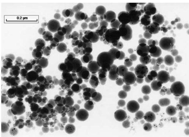
Fig. 5 Transmission electron microscope image of typical condensed particles. These are formed in an expanding vapor plume after high-temperature vaporization of a pyroxene (from Gerasimov et al. 1999)
