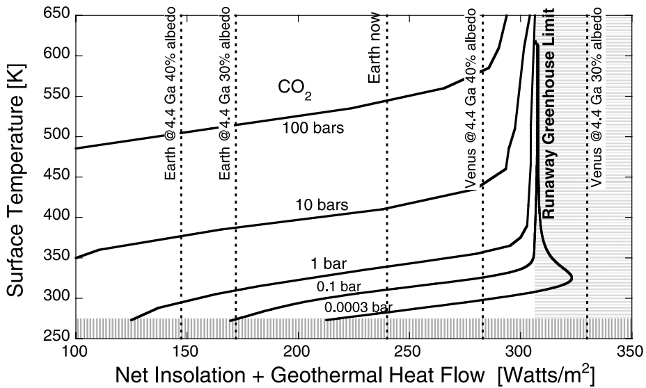
Fig. 10 The \text{H}_2\text{O}-\text{CO}_2 greenhouse. The plot shows the surface temperature as a function of radiated heat for different amounts of atmospheric \text{CO}_2 (after Abe 1993). The albedo is the fraction of sunlight that is not absorbed (the appropriate albedo to use is the Bond albedo, which refers to all sunlight visible and invisible). Modern Earth has an albedo of 30%. Net insolation for Earth and Venus ca. 4.5 Ga (after the Sun reached the main sequence) are shown at 30% and 40% albedo. Earth entered the runaway greenhouse state only ephemerally after big impacts that generated big pulses of geothermal heat. For example, after the Moon-forming impact the atmosphere would have been in a runaway greenhouse state for \sim 2 million years, during which the heat flow would have made up the difference between net insolation and the runaway greenhouse limit. A plausible trajectory takes Earth from \sim 100 bars of \text{CO}_2 and 40% albedo down to 0.1–1 bar and 30% albedo, at which point the oceans ice over and albedo jumps. Note that \text{CO}_2 does not by itself cause a runaway. Also note that Venus would enter the runaway state when its albedo dropped below 35%
