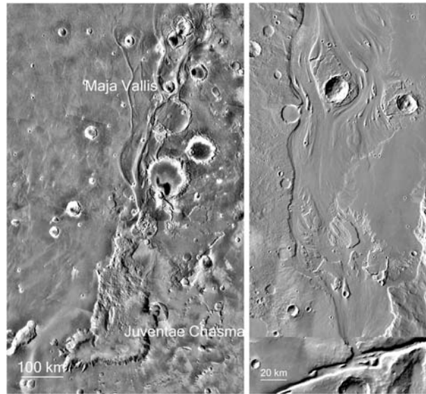
Fig. 2 Left: Maja Vallis and Juventae Chasma. Maja Vallis emerges from a 5 km deep rubble-filled depression. The outlet is at an elevation 4 km above the floor of the depression, so after Maja Vallis formed a lake must have been left in the depression, consistent with detection of sulfates there (Gendrin et al. 2005). The relations indicate that Maja Vallis formed by a massive eruption of groundwater (Viking Orbiter camera MDIM2). Right: Mangala Vallis. The channel starts at a notch in a graben, which suggests eruption of groundwater as a result of faulting and/or dike injection. (Mars Thermal Emission Imaging System, THEMIS mosaic, Mars Odyssey)
