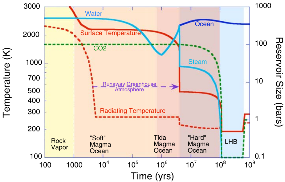
Fig. 5 A cartoon history of temperature, water, and \text{CO}_2 during the Hadean. The Hadean begins with the Moon-forming impact. For 1,000 years Earth is enveloped in rock vapor. \text{CO}_2 and other gases are presumed to degas from the convecting silicate gas, while water mostly partitions into the interior. A substantial greenhouse effect and tidal heating maintain the magma ocean for some 2 million years. Most of Earth's water and the rest of the \text{CO}_2 degassed as the mantle solidified. After the mantle solidified the steam atmosphere condensed to form a warm ( \sim 500 K) water ocean under \sim 100 bars of \text{CO}_2 . This warm, wet early Earth would have lasted while Earth's \text{CO}_2 stayed in the atmosphere. In this illustration \text{CO}_2 is assumed to subduct into the mantle on either a 10 Myr (solid curves) or a 100 Myr (dotted curves) time scale. The asymptotic \text{CO}_2 partial pressure is assumed to be controlled at low levels by chemical weathering of oceanic crust and abundant ultramafic impact ejecta. Prior to the origin of life, in the absence of an abundant potent greenhouse gas, the surface should have been ice covered and very cold, although occasional impacts brought brief thaws. Finally, after the late bombardment, the \text{CO}_2 is allowed to return to \sim 1 bar levels in order that the surface be clement; this too is arbitrary
