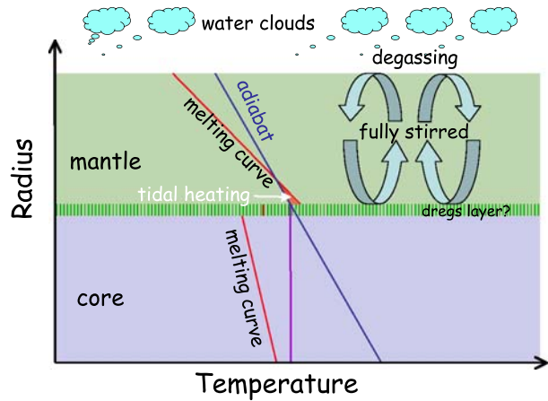
Fig. 7 A cartoon illustrating conditions inside the Earth ca. 1 million years after the Moon-forming impact. Schematic adiabats and melting curves are indicated. Tidal heating is concentrated at the base of the mantle. The mostly liquid mantle is probably fully stirred and equilibrated with the atmosphere. Temperature in the mantle follows the adiabat. At this early time the core is liquid but probably not convective. It is more likely that is heated from above by conduction. Therefore there is no reason to expect a substantial magnetic field. Slag layers may form at the top and bottom of the mantle
