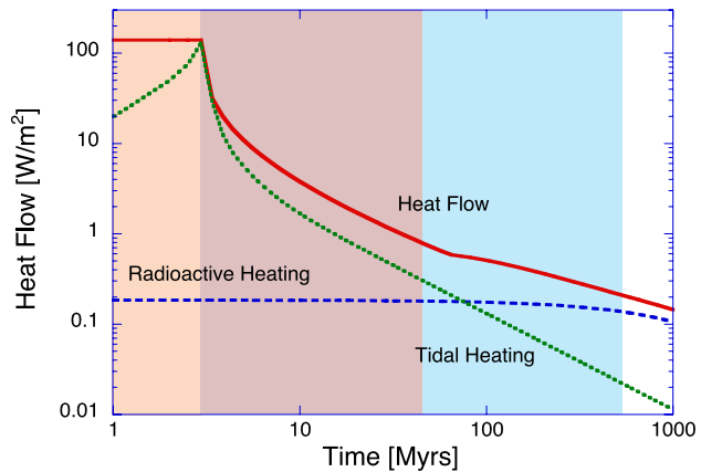
Fig. 8 A cartoon history of mean heat flow during the first billion years after the Moon-forming impact. Epochs correspond to those in Fig. 5. Tidal heating plays an important role in prolonging the magma ocean. Tidal forcing wanes as the Moon evolves away from the Earth. Thereafter heat flow is controlled by convection of the solid mantle. By 4.4 Ga the global average heat flow would have been \sim 0.5 \text{ W/m}^2 . Later in the Hadean typical heat flows would have been 0.2\text{--}0.3 \text{ W/m}^2 , not enormously larger than what they are now. For comparison heat flow today is 0.065 \text{ W/m}^2 through the continents and 0.1 \text{ W/m}^2 through the ocean crust. Computational assumptions are given in the text
