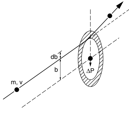
FIGURE 6.5. Schematic of an electron of momentum mv interacting with a free electron at an impact parameter b .
