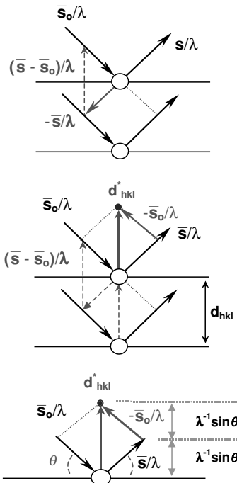
FIGURE 8.5. Development of Bragg's Law in vector form.
