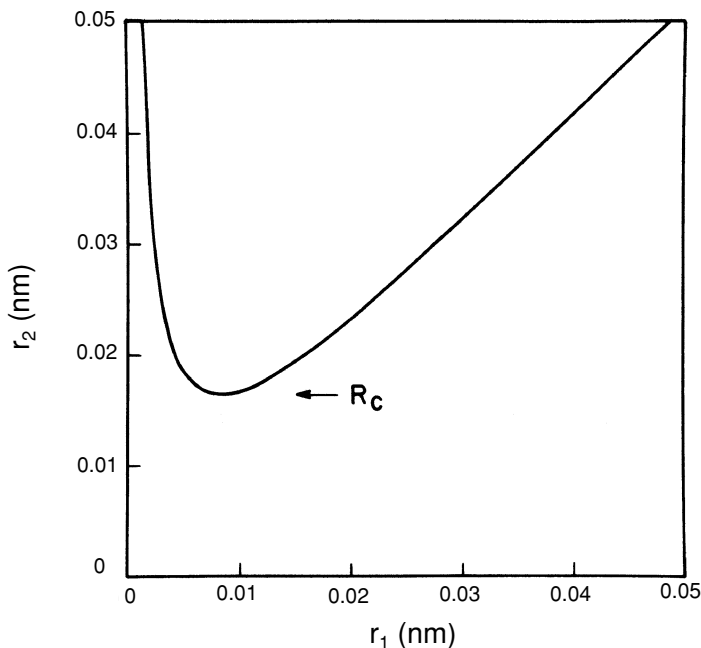
FIGURE 5.10. The dependence of r_2 on the initial impact parameter r_1 for the case of 1.0 MeV \text{He}^+ ions on \text{W}(100) ; r_2 is calculated for d = 0.316 nm corresponding to the atom spacing in the \langle 001 \rangle direction. The minimum value of r_2 is the Coulomb shadow cone with radius R_C .
