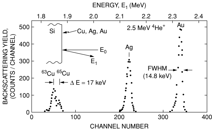
FIGURE 2.4. Backscattering spectrum for \theta = 170^\circ and 2.5 MeV ^4\text{He}^+ ions incident on a target with approximately one monolayer coverage of Cu, Ag, and Au. The spectrum is displayed as raw data from a multichannel analyzer, i.e., in counts/channel and channel number.
