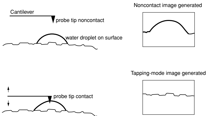
FIGURE 14.12. (a) Schematic displaying the consequence of adsorbed moisture from the ambient during AFM analysis. (b) Tapping-mode AFM is used to avoid the false image of the surface.
