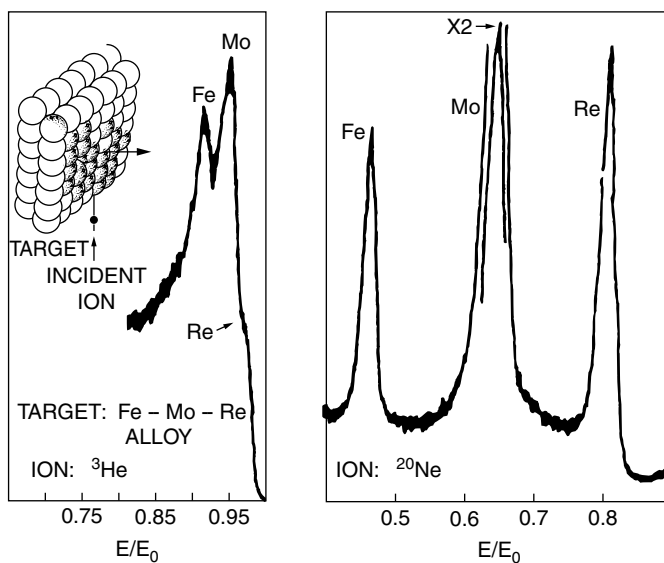
FIGURE 2.14. Energy spectra for 3 He + scattering and 20 Ne scattering from a Fe–Mo–Re alloy. Incident energy was 1.5 keV. [From J.T. McKinney and J.A. Leys, 8 th National Conference on Electron Probe Analysis, New Orleans, LA, 1973.]
