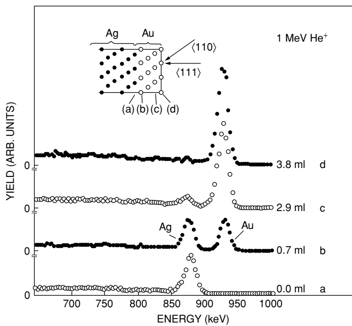
FIGURE 5.17. Backscattering spectra for 1.0 MeV \text{He}^+ ions incident along the \langle 110 \rangle axis of a clean Ag(111) surface (a) and an Au-covered surface (b), (c), and (d). The Ag surface peak decreases because of the Au absorption.
