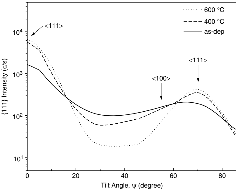
FIGURE 7.6. \{111\} pole-figures obtained from Ag thin films on \text{SiO}_2 substrates, as-deposited (solid line) and annealed at 400 °C (dashed line) and 600 °C (dotted line) for 1 hour in vacuum.
