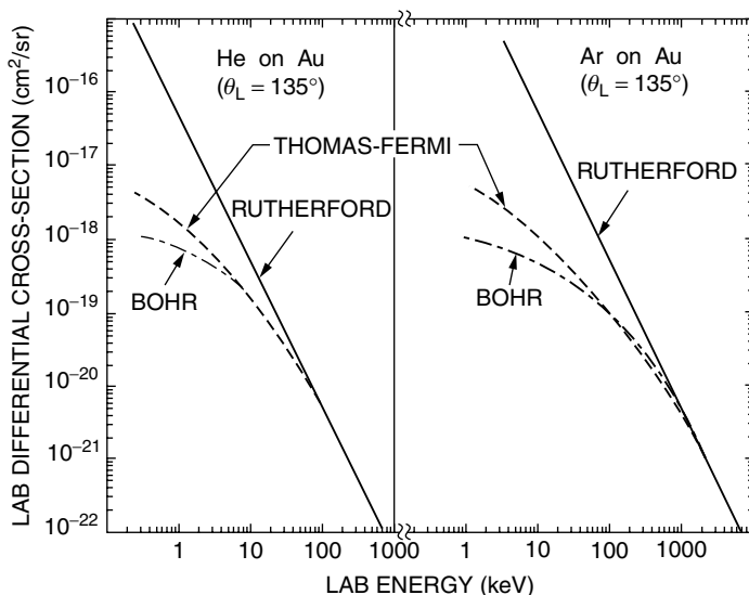
FIGURE 2.13. Energy dependence of the Rutherford, Thomas–Fermi, and Bohr cross sections for a laboratory scattering angle of 135°. The Thomas–Fermi and Bohr potentials are two common approximations to a screened Coulomb potential: (a) He + on Au and (b) Ar on Au. From J.M. Poate and T.M. Buck, Experimental Methods in Catalytic Research , Vol. 3. [Academic Press, New York, 1976, vol. 3.]
