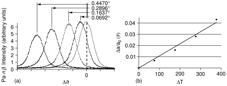
FIGURE 7.4. a) X-ray spectra of the (hkl) reflection of \beta -parylene- n at room temperature, 100, 200, 300, and 375 °C; b) a/a_0 is calculated and plotted against the change in temperature.
