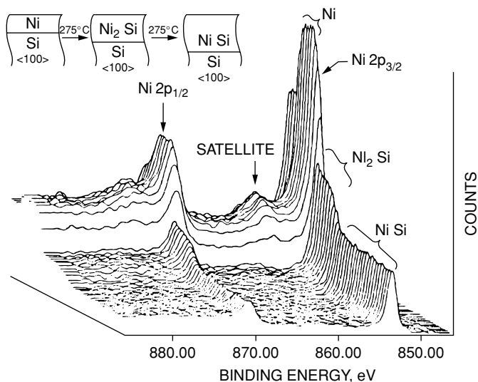
FIGURE 10.13. Three-dimensional plot of the Ni 2 p XPS spectra, with the z-axis representing time during heat treatment. The spectra illustrate the planar growth of different forms of nickel silicide, as shown in the inset. Here chemical shifts are relatively small, but the change in intensity indicates a change in composition. [From P.J. Grunthaner, Ph.D. thesis, Caltech, 1980.]
