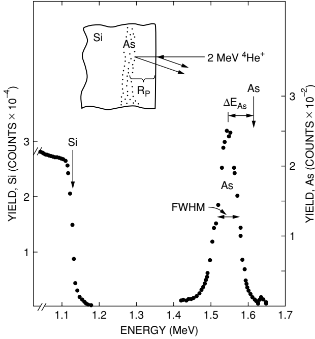
FIGURE 3.9. Energy spectrum of 2 MeV ^4\text{He}^+ ions backscattered from a silicon crystal implanted with a nominal dose of 1.2 \times 10^{15} As ions/cm ^2 at 250 keV. The vertical arrows indicate the energies of particles scattered from surface atoms of ^{28}\text{Si} and ^{75}\text{As} .
