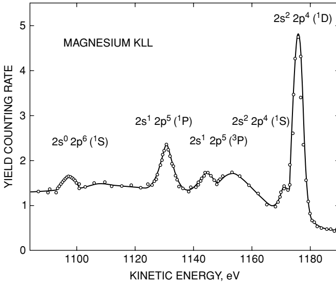
FIGURE 12.3. KLL spectrum of magnesium containing 5 of the 6 lines predicated in L-S coupling. [From Siegbahn et al., 1967.]
