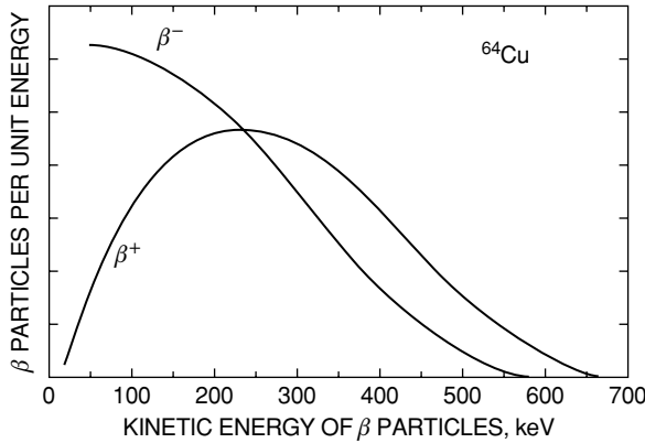
FIGURE 13.6. Energy spectra of the positive ( \beta^+ ) and negative ( \beta^- ) electrons emitted by ^{64}\text{Cu} . The pronounced difference between the two spectral shapes results largely from the Coulomb effect.
