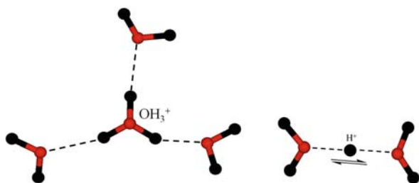
Fig. 7 Eigen complex [\text{H}_3\text{O} \cdot (\text{H}_2\text{O})_3]^+ ( left panel ), with the \text{OH}_3^+ at the center, surrounded by its three hydrogen bonded \text{H}_2\text{O} molecules and Zundel complex [\text{H} \cdot (\text{H}_2\text{O})_2]^+ ( right panel ) in which the extra proton is shared between two water molecules. \text{H}_2\text{O} molecules are represented as v-shaped stick and balls (H atoms are black and O atoms dark-gray), dashed lines indicate H-bonds, and the shared proton in the Zundel complex is labeled as \text{H}^+ and shown as a black ball
