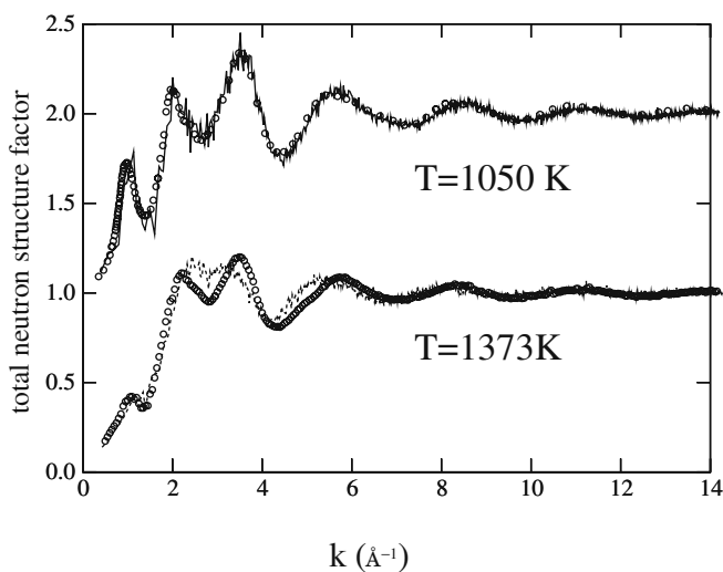
Fig. 1 Total neutron structure factors for liquid GeSe_2 at T = 1,050 K and T = 1,373 K. Open circles : experimental results at T = 1,050 K [5] and at T = 1,373 K [7] Full line (upper part) and dotted line (lower part) : FPMD calculation, T = 1,050 K [6], T = 1,373 K [8]
