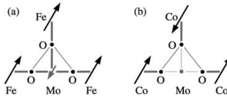
Fig. 10 Sketch of the bonds into (a) Sr_2FeMoO_6 and (b) Sr_2CoMoO_6 . The strength of the inter-atomic interaction is given by the style of the line representing the bond where the strongest is the thick solid line, the weakest is the thin dashed line and the medium is the thin solid line
