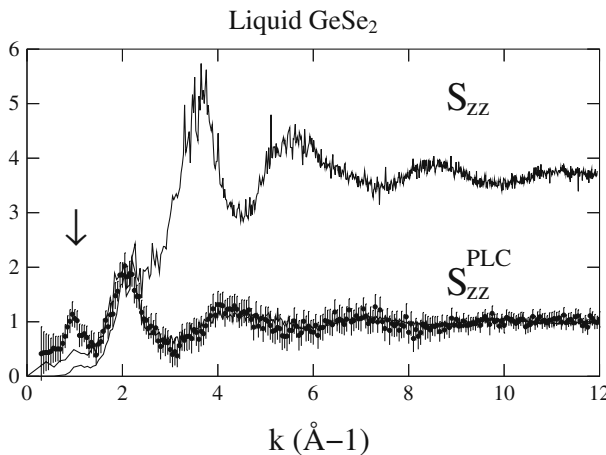
Fig. 9 Charge-charge structure factor S_{zz}(k) and concentration-concentration structure factor S_{CC}(k) of liquid \text{GeSe}_2 at T = 1,050 K. S_{CC}(k) is normalized as in Eq. (11), i.e., S_{zz}^{\text{PLC}}(k) = (c_{\text{ACX}})^{-1} S_{CC}(k) . Dots with error bars: experimental results [5]. The arrows indicate the location of the FSDP in the total neutron structure factor ( k_{\text{FSDP}} = 1.0 \text{ \AA}^{-1} )
