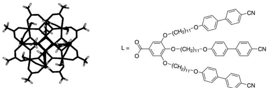
Fig. 15 Chemical structure of the gallate derivative substituent and of the \text{Mn}_{12} cluster forming 5
