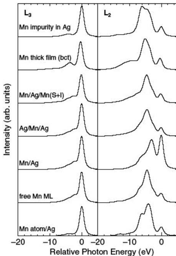
Fig. 9 Calculated 2p \rightarrow 3d \rightarrow 2p resonant X-ray emission at the photon energies marked by vertical arrows in the L_{23} spectrum of Fig. 8. Left part: calculated RXES results for L_3 excitation. Right part: calculated RXES results for L_2 excitation (from [113])
