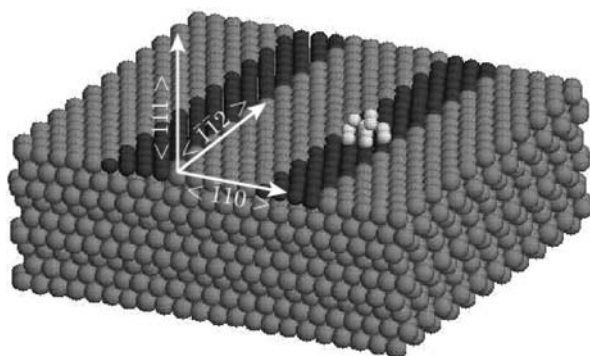
Fig. 18 Slab used in the simulations. Two discommensuration lines of highest corrugation run along the \langle 112 \rangle direction. The DLs (black atoms) separate regions (gray atoms) of a regular fcc stacking from a smaller region with hcp faulted stackings. White atoms are the Co atoms (from [33])
