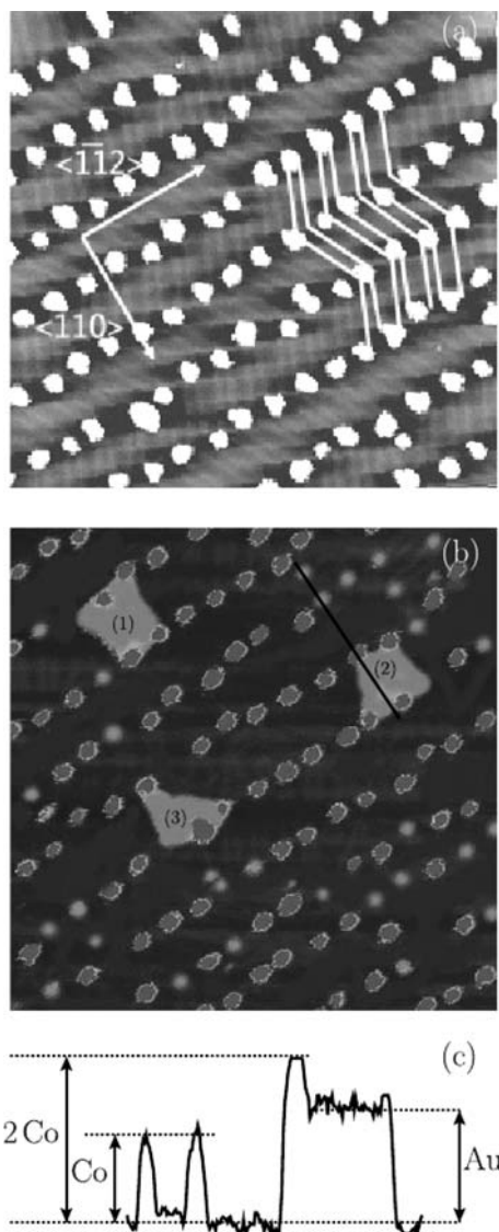
Fig. 16 (a) STM image of a self-organized Co cluster as obtained after deposition at 300 K. Zigzag DLs have been highlighted with white lines. (b) False color STM image of the Co cluster network after annealing at 450 K. Dark gray patches represent the Co bilayer clusters. Light gray patches are the sunken Co clusters. Large bright patches labeled (1), (2), and (3) are the gold rims. (c) The line scan confirms the presence of fully emerged and sunken Co clusters (4.0 and 2.0 Å above the surface, respectively) as well as monolayer high Au rims (2.36 Å). Images 100 \times 100 nm (from [33])
