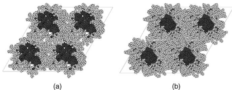
Fig. 10 Snapshots of packing of 2b (a) and 3b (b) after MD in the hexagonal 2D lattice of the \text{Col}_h phase
