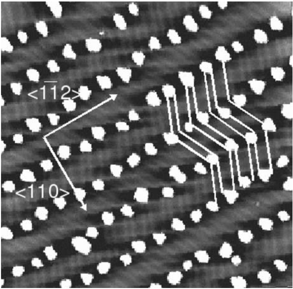
Fig. 5 STM image of self-organized Co clusters as obtained after deposition at 300 K. Zigzag DLs have been highlighted with white lines . Images 100×100 nm [33]
