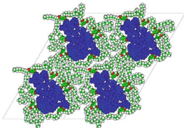
Fig. 8 Snapshot showing the organization of 2a in the \text{Col}_h phase (in dark polar central core). Only one layer (6.75 Å) is represented, the apparent empty zones, being actually filled by neighbored layers
