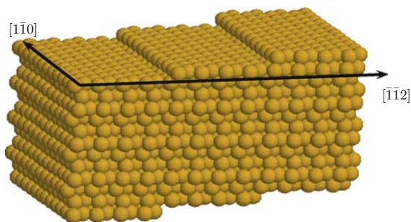
Fig. 7 Pt(997) vicinal surface in perspective view
