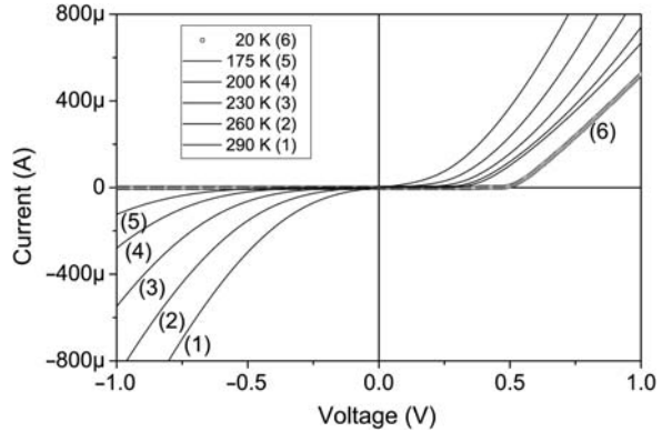
Fig. 14 Current vs. voltage curves of a 50 \times 50 \mu\text{m}^2 junction for different temperatures between 20 and 290 K
