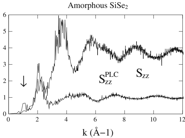
Fig. 8 Charge-charge structure factor S_{zz}(k) and concentration-concentration structure factor S_{CC}(k) of amorphous \text{SiSe}_2 at T = 300 K. S_{CC}(k) is normalized as in Eq. (11), i.e., S_{zz}^{\text{PLC}}(k) = (c_{\text{ACX}})^{-1} S_{CC}(k) . The arrows indicate the location of the FSDP in the total neutron structure factor ( k_{\text{FSDP}} = 1.0 \text{ \AA}^{-1} )
