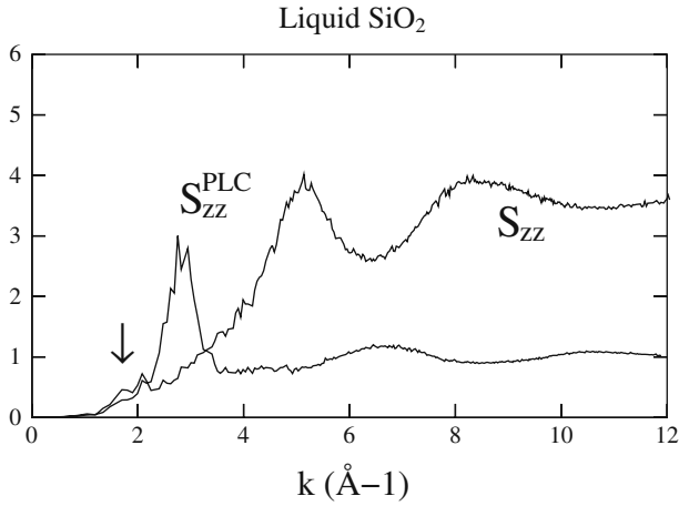
Fig. 7 Charge-charge structure factor S_{zz}(k) and concentration-concentration structure factor S_{cc}(k) of liquid \text{SiO}_2 at T = 3,500 K. S_{cc}(k) is normalized as in Eq. (11), i.e., S_{zz}^{\text{PLC}}(k) = (c_{\text{A}c_{\text{X}}})^{-1} S_{cc}(k) . The arrows indicate the location of the FSDP in the total neutron structure factor ( k_{\text{FSDP}} = 1.6 \text{ \AA}^{-1} )
