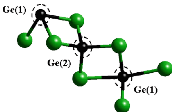
Fig. 11 Snapshots of structural subunits found in liquid \text{GeSe}_2 . Ge atoms are dark and Se atoms are light . Bonds are drawn when two atoms are separated by less than 3 Å, the first minimum in the Ge–Se radial pair distribution function. Ge atoms forming a \text{Ge}^* subunit are surrounded by a dashed line
