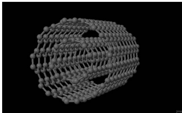
Fig. 20 Atomic configuration of a CNT 4 \times 4 inserted in a CNT 10 \times 10
