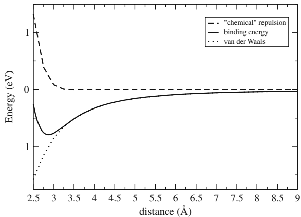
Fig. 17 Binding energy, “chemical” repulsion, and van der Waals energy of C_{60} adsorbed on CNT 10 \times 10 , calculated with our approach
