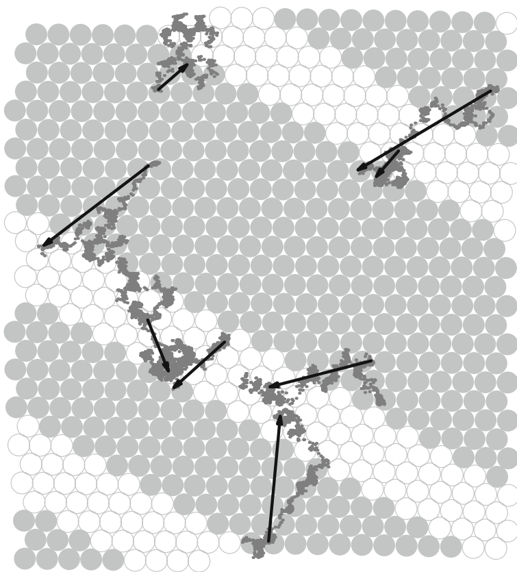
Fig. 13 Trajectories (gray dots) of Co adatoms on the herringbone reconstruction of Au(111) along a time interval of 96 ps at T = 600 K. The unfilled circles give the position of the gold surface atoms belonging to the discommensuration lines. The black arrows give the net displacement of the cobalt adatoms along the time interval
