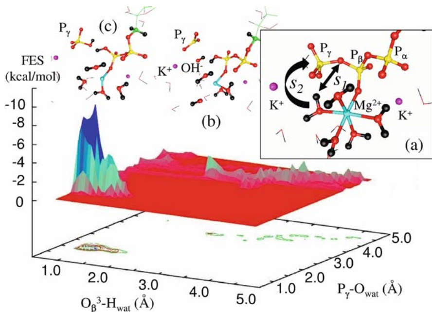
Fig. 5 ATP hydrolysis in Hsc70. The initial system (a) reaches a transition state (b) via deprotonation of a specific water molecule. This results in the bond cleavage P_{\beta}-O_{\beta}^3-P_{\gamma} \rightarrow P_{\beta}-O_{\beta}^3 P_{\gamma} with subsequent ADP formation and release of the inorganic phosphate (c). The two collective variables used in the metadynamics are the distances s_1 = O_{\beta}^3 - H_{water} and s_2 = P_{\gamma} - O_{water} shown by the arrows
