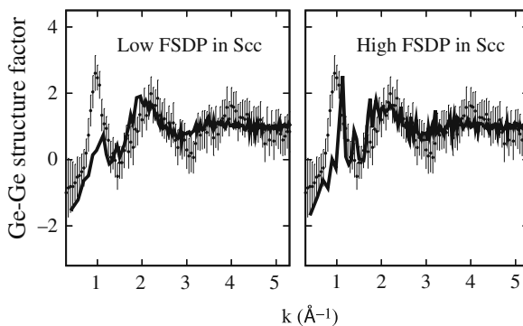
Fig. 10 Ge–Ge partial structure factor for liquid GeSe 2 : experiment (dots with error bars) [5] compared to the theoretical result obtained by averaging separately over all configurations in \mathcal{E}_{\text{low}} (left panel) and \mathcal{E}_{\text{high}} (right panel)
