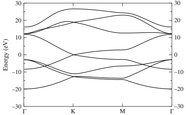
Fig. 2 Band structure of an isolated plane of graphene calculated with Fireball. The origin of energy corresponds to the Fermi level of the system
