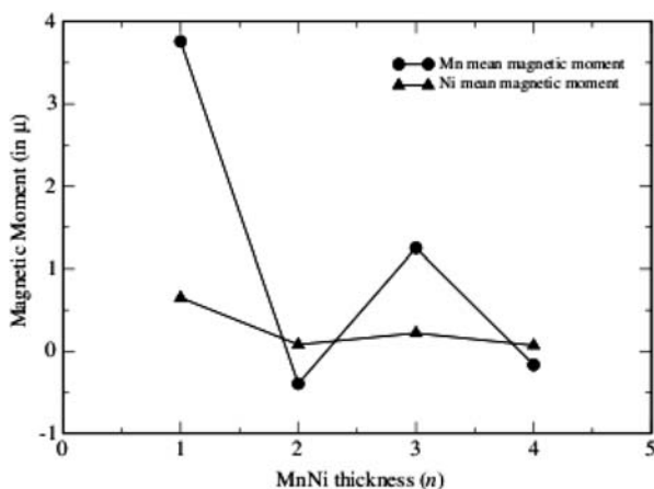
Fig. 5 Mean magnetic moment per atom (in \mu_B ) for (\text{Ni}_{0.5}\text{Mn}_{0.5})_n monolayers on Co(001), “ n ” is the thickness of MnNi over-layers, for Ni and Mn atoms as a function of the Mn–Ni thickness. Line with circles (triangles) represent the mean magnetic moment for Mn (Ni) atoms (from [99])
