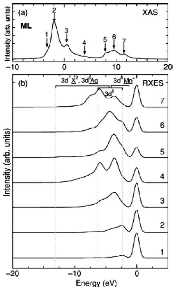
Fig. 10 (a) Absorption spectrum in the Mn L_{23} region with indication of the excitation energies used in the RXES calculation. X stands for \text{Mn}^{2+} and Ag. All RXES spectra have been rescaled to the same amplitude. (b) Calculated RXES spectra for a Mn monolayer on Ag (from [117])
