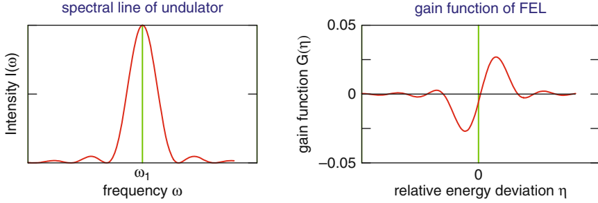
Fig. 3.8. Left: the line-shape curve I(\omega) for the first harmonic \omega_1 \equiv \omega_\ell of undulator radiation. Right: a typical gain function G(\eta) of the low-gain FEL
