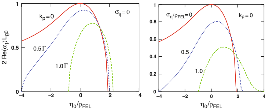
Fig. 6.2. Left: the growth rate function f_{gr}(\eta_0) = 2 \Re(\alpha_1(\eta_0)) L_{g0} is plotted versus \eta_0/\rho_{\text{FEL}} for different values of the space charge parameter k_p . Continuous red curve: k_p = 0 , dotted blue curve: k_p = 0.5 \Gamma , dashed green curve: k_p = 1.0 \Gamma . The energy spread is put to zero.
