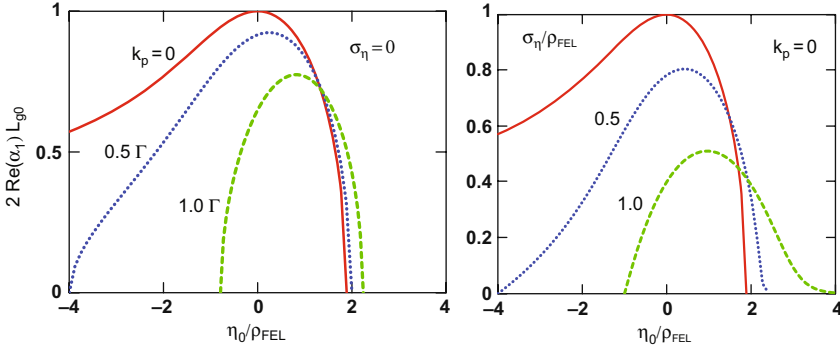
Fig. E.2. Left: the growth rate function f_{gr}(\eta_0) = 2\Re(\alpha_1(\eta_0))L_{g0} plotted versus \eta_0/\rho_{FEL} for different values of the space charge parameter k_p . Continuous red curve: k_p = 0 , dotted blue curve: k_p = 0.5\Gamma , dashed green curve: k_p = 1.0\Gamma . The energy spread is put to zero. Right: the growth rate function f_{gr}(\eta_0) = 2\Re(\alpha_1(\eta_0))L_{g0} is plotted versus \eta_0/\rho_{FEL} for different values of the relative beam energy spread \sigma_\eta = \sigma_W/W_r . Continuous red curve: \sigma_\eta = 0 , dotted blue curve: \sigma_\eta = 0.5\rho_{FEL} , dashed green curve: \sigma_\eta = 1.0\rho_{FEL} . Here the space charge parameter is set to zero
