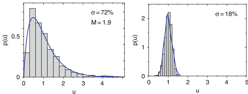
Fig. 7.13. Left: measured probability distribution of FEL pulse energy in the exponential regime at a wavelength of 13.7 nm [13]. Solid curve: gamma distribution. The average pulse energy is 1 \mu J. Right: probability distribution of FEL pulse energy in the saturation regime. Here the gamma distribution is not applicable, the solid curve has been computed with the code FAST. The average pulse energy is 40 \mu J.
