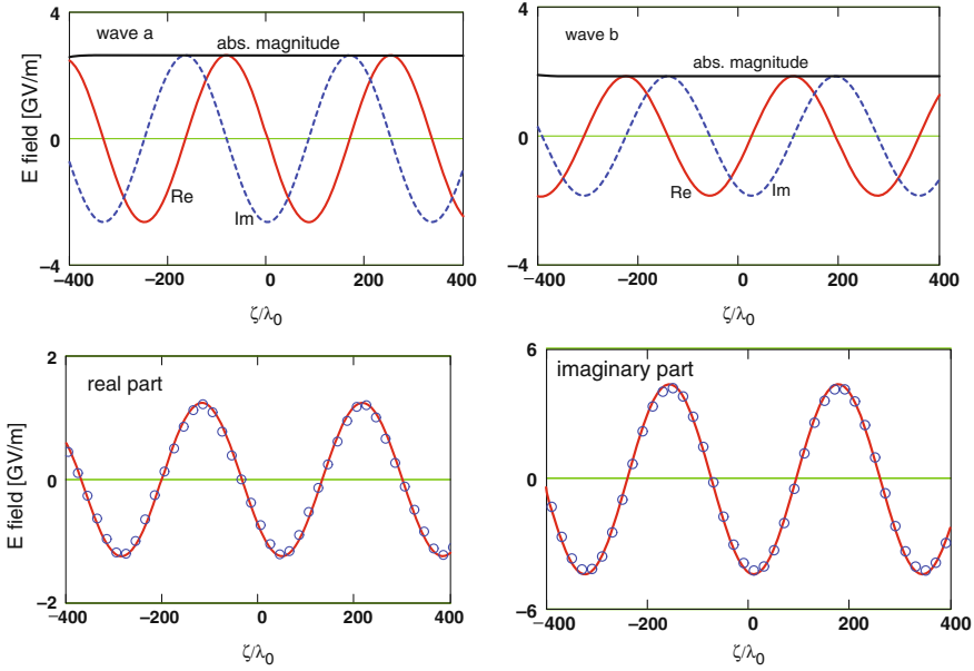
Fig. 5.6. Response of the FEL in the linear regime at z = 15 L_{g0} . Top left graph: real part, imaginary part and absolute magnitude of the field \hat{E}^a(z, \zeta) of frequency \omega_a , plotted versus \zeta/\lambda_0 ( \lambda_0 denotes the FEL wavelength corresponding to the resonance energy). Top right graph: real part, imaginary part and absolute magnitude of the field \hat{E}^b(z, \zeta) of frequency \omega_b . Bottom left graph: the sum of the real parts \Re\{\hat{E}^a(z, \zeta) + \hat{E}^b(z, \zeta)\} of the individual responses is shown as solid red curve, the real part \Re\{\hat{E}^s(z, \zeta)\} of the sum-response (5.18) is shown as the blue circles. Bottom right graph: same for the imaginary parts
