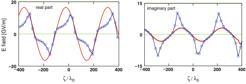
Fig. 5.7. FEL response in the nonlinear regime at z = 20 L_{g0} . Left graph: the sum of the real parts \Re\{\hat{E}^a(z, \zeta) + \hat{E}^b(z, \zeta)\} of the individual responses is shown as solid red curve, the real part of the sum-response \Re\{\hat{E}^s(z, \zeta)\} is shown by the blue circles . Right graph: comparison of the imaginary parts
