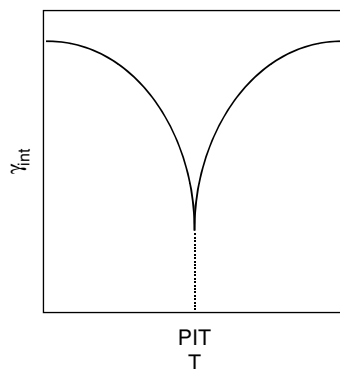
FIGURE 1.5. Influence of temperature on the interfacial tension between oil and water in the presence of a polyethoxylated surfactant.
