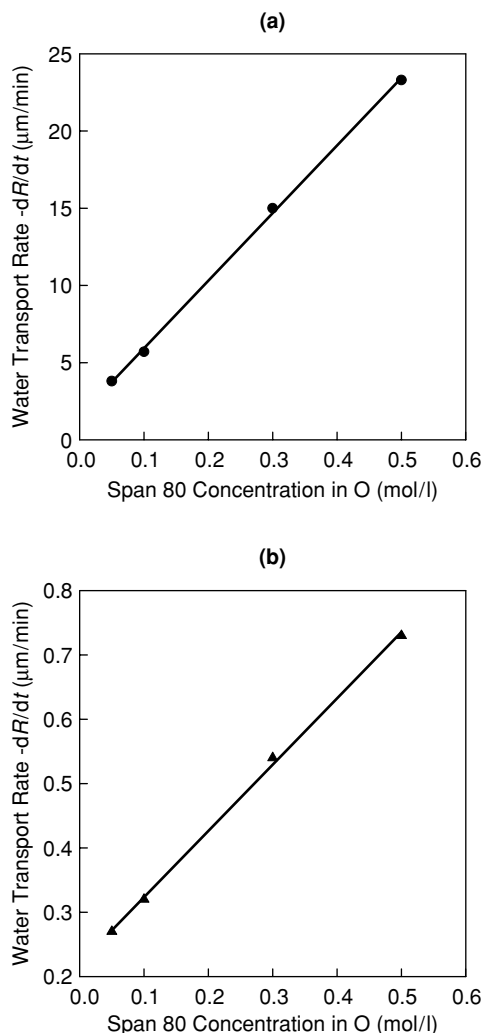
FIGURE 6.17. Effects of SMO (span 80) concentration in the rate of radius variation in W/O/W, when W1/O and O/W2 interfaces are at (a) visual contact and (b) no visual contact. W1 = pure water; O = n -hexadecane + SMO, W2 = 5 \cdot 10^{-3} mol/l NaCl solution. (Reproduced with permission from [32].)
