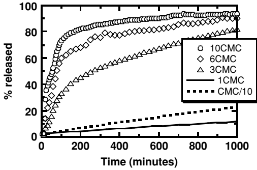
FIGURE 6.10. Influence of SDS concentration in the external water phase on the kinetics of release. d_g = 4 \mu\text{m} , d_i = 0.36 \mu\text{m} , \phi_i^0 = 20\% , \phi_g = 10\% , C_l = 2 \text{ wt}\% . (Adapted from [10].)
