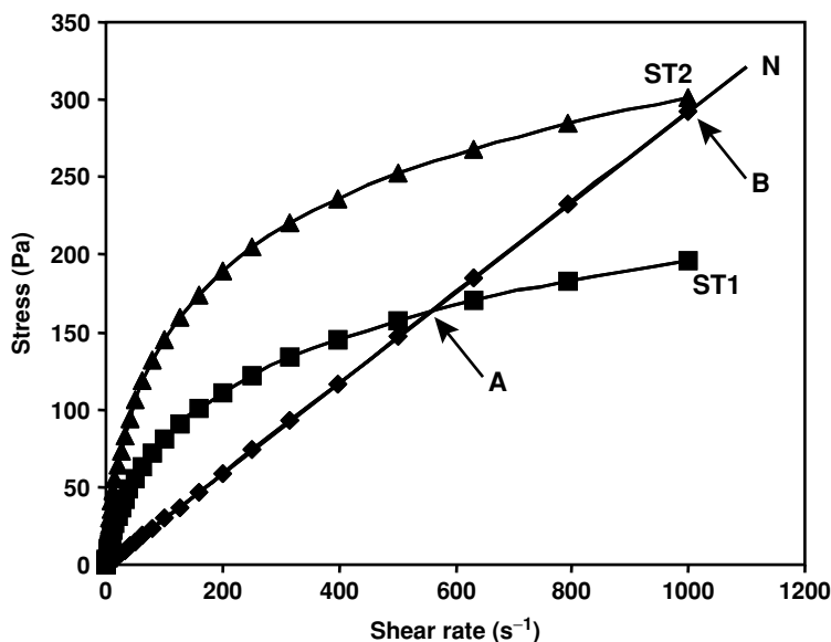
FIGURE 1.22. Rheograms of a newtonian ( \diamond ) N and two shear-thinning ST1 and ST2 emulsions obtained by adding 1.5 wt% ( \blacksquare ) and 1.9 wt% ( \blacktriangle ) of a nonadsorbing polymer in the continuous phase. (Adapted from [150].)
