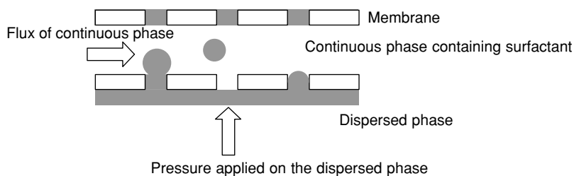
FIGURE 1.1. Schematic principle of membrane emulsification.
