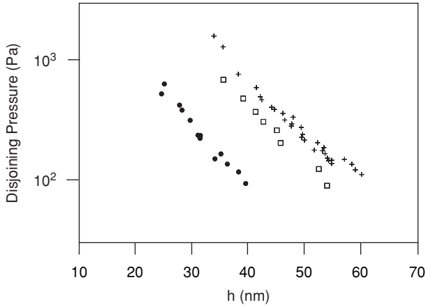
FIGURE 2.12. Influence of a nonionic surfactant concentration (NP10 of \text{CMC} = 7 \cdot 10^{-5} \text{ mol/l} ) on the pressure isotherms (air–water interface). PVA–Vac concentration = 0.5 wt%. (+) [NP10] = 0; (□) [NP10] = \text{CMC}/10 ; (●) [NP10] = \text{CMC} . (Adapted from [30].)
