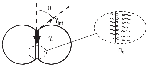
FIGURE 2.30. Two adhesive emulsion droplets. A flat liquid film stabilized by the surfactant layers is located between the droplets. This film being very thin, it can be usually considered as a surfactant bilayer. \gamma_f is the tension of the film and \gamma_{\text{int}} the tension of single isolated interface.
