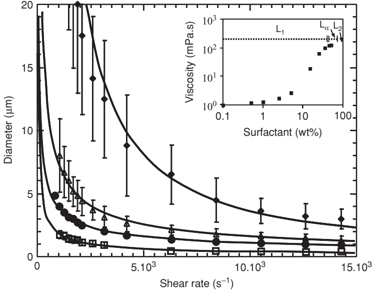
FIGURE 1.25. Influence of the emulsifier concentration C_{\text{surf}} on the size profiles: (♦) C_{\text{surf}} = 15 wt%; ( \Delta ) C_{\text{surf}} = 25 wt%; (●) C_{\text{surf}} = 30 wt%; and ( \square ) C_{\text{surf}} = 45 wt% of surfactant. The dispersed phase is kept constant at 75 wt% of a 350 mPa.s silicone oil. The lines are guides to the eye. Inset: Zero-shear viscosity as a function of surfactant concentration. (Adapted from [137].)
