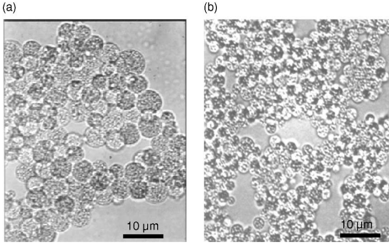
FIGURE 1.31. Images of W/O/W emulsions obtained at different shear rates. The emulsions were diluted with water and glucose to facilitate observation. (a) \dot{\gamma} = 1000 \text{ s}^{-1} and (b) \dot{\gamma} = 14,200 \text{ s}^{-1} . (Adapted from [162].)
