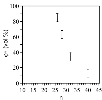
FIGURE 3.8. Volume fraction of n -alkane at the onset of flocculation as a function of n -alkane chain length ( C_nH_{2n+2} ). The continuous phase is made of a mixture of n -alkane, dodecane, and SMO (1 wt%). Glycerol droplets (5% in volume) have a diameter of 0.38 \mu\text{m} . T = 65^\circ\text{C} . (Adapted from [13].)
