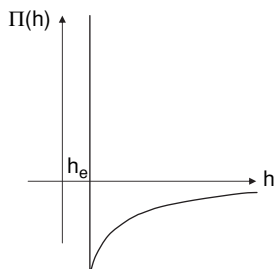
FIGURE 2.29. Disjoining pressure between interfaces of a liquid film.
