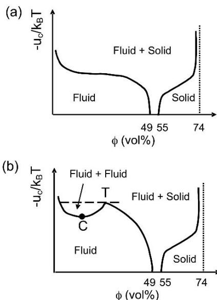
FIGURE 3.10. Phase diagrams of attractive monodisperse dispersions. u_c is the contact pair potential and \phi is the particle volume fraction. For u_c/k_B T = 0 , the only accessible one-phase transition is the hard sphere transition. If u_c/k_B T \neq 0 , two distinct scenarios are possible according to the value of the ratio \xi (range of the pair potential over particle radius). For \xi < 0.3 (a), only fluid–solid equilibrium is predicted. For \xi > 0.3 (b), in addition to fluid–solid equilibrium, a fluid–fluid (liquid–gas) coexistence is predicted with a critical point (C) and a triple point (T).
