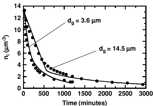
FIGURE 6.13. Number density of internal droplets for two globule diameters. d_i = 0.36 \text{ }\mu\text{m} , \phi_g = 10\% , C_h = 3 \text{ CMC} , C_l = 2 \text{ wt\%} . The continuous lines are theoretical predictions. (Adapted from [10].)
