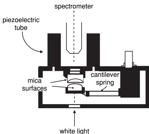
FIGURE 2.1. Scheme of the surface force apparatus (SFA).
