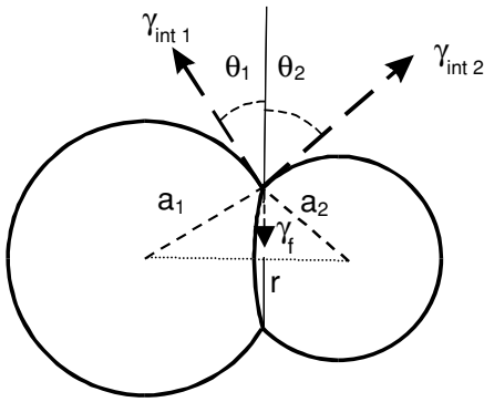
FIGURE 2.32. Two adhesive droplets of size a_1 and a_2 . If the droplets are of the same nature \gamma_{\text{int } 1} = \gamma_{\text{int } 2} = \gamma_{\text{int}} and \theta_1 = \theta_2 .
