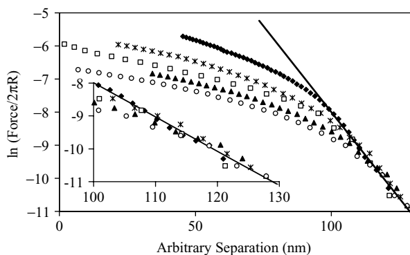
FIGURE 2.28. Log force vs. arbitrary separation curves for the approach of a glass probe and a droplet from emulsion. The symbols correspond to different levels of cross-linking of PDMS droplets: ( \blacklozenge ) 50%; ( \ast ) 45%; ( \square ) 40%; ( \blacktriangle ) 35%; ( \circ ) 30%. The background electrolyte solution contains \text{KNO}_3 at 10^{-3} mol/l and \text{pH} = 9.5 . Solid line represents the theoretical electrostatic repulsion with a Debye length of 9.6 nm. All forces were determined at 1 \mu\text{m/s} . (Reproduced from [97], with permission.)
