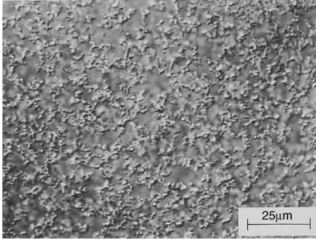
FIGURE 3.11. Emulsion gel. The droplets are about 0.5\ \mu\text{m} in diameter. They form large and ramified aggregates.
