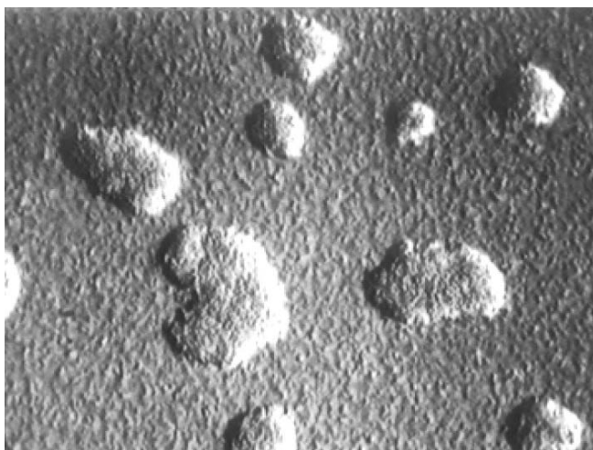
FIGURE 3.3. Microscopic image showing the effect of adding excess surfactant in the continuous phase of the emulsions: flocs separate from a coexisting fluid phase.
