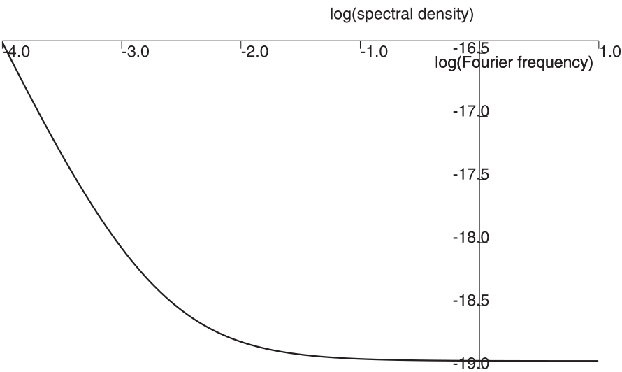
Fig. 6.24. Frequency noise spectral density of the oscillator of [72]
