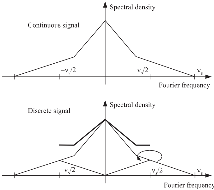
Fig. 6.7. Aliasing when frequency is measured without a dead time
