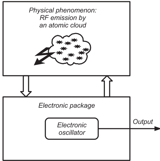
Fig. 2.4. Block diagram of an active hydrogen maser
