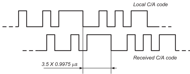
Fig. 8.5. Measurement of the raw pseudo-range (modulo 299 792.458 m)
