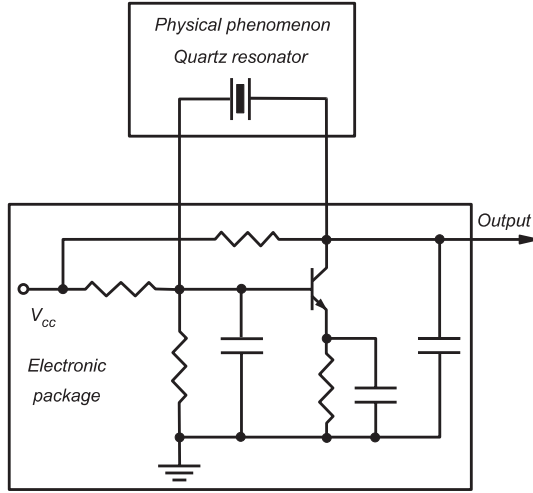
Fig. 2.3. Pierce oscillator
