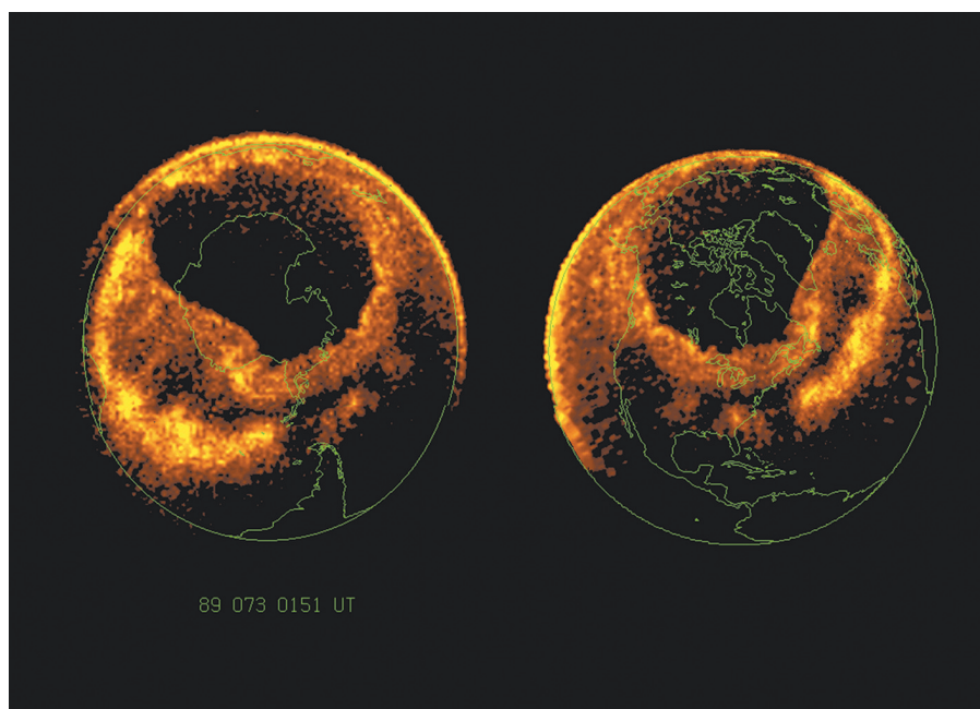
Figure 2.15. Dynamics Explorer image of the auroral oval during the Great Aurora of 13–14 March 1989, demonstrating the sheer extent of activity—for example, to Mediterranean latitudes and lower—during this extreme event. Image: University of Iowa.
