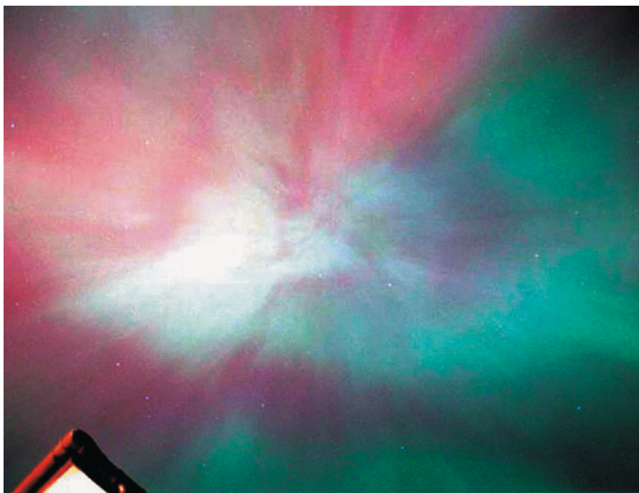
Figure 5.14. Coronal aurora over Falkirk, central Scotland on 20–21 November 2003. Image: Malcolm Gibb.
