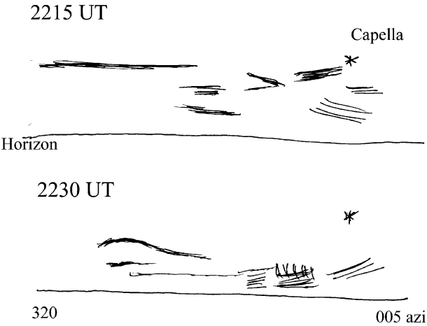
Figure 8.9. Sketches of the 6–7 July 2005 noctilucent cloud display (see Table 8–2) from the Author’s observing log.
