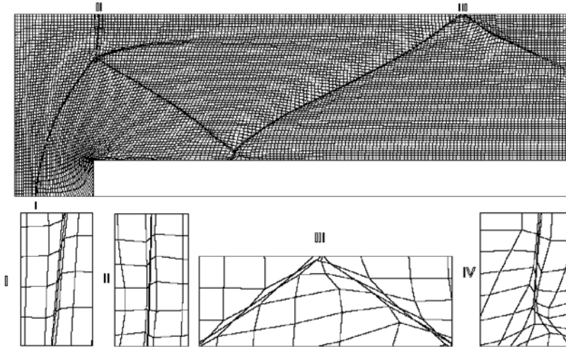
Fig. 7.13. Supersonic flow in the mach wind tunnel containing a step. The boundary nodes are distributed using constrained minimization. Adaptive mesh with fragments I, II, III near the boundary and IV comprising the triple point.
