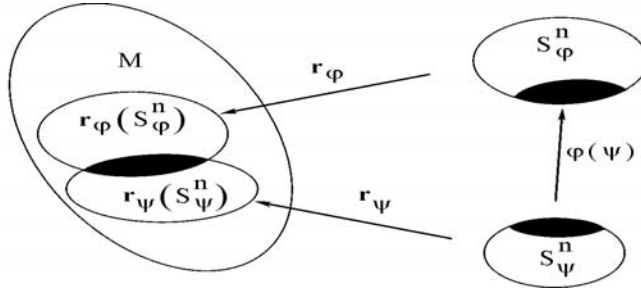
Fig. 4.3. Illustration for Riemannian manifold maps
