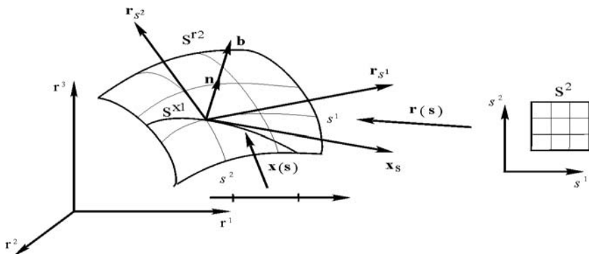
Fig. 4.7. Normal vector to the curve on the surface
