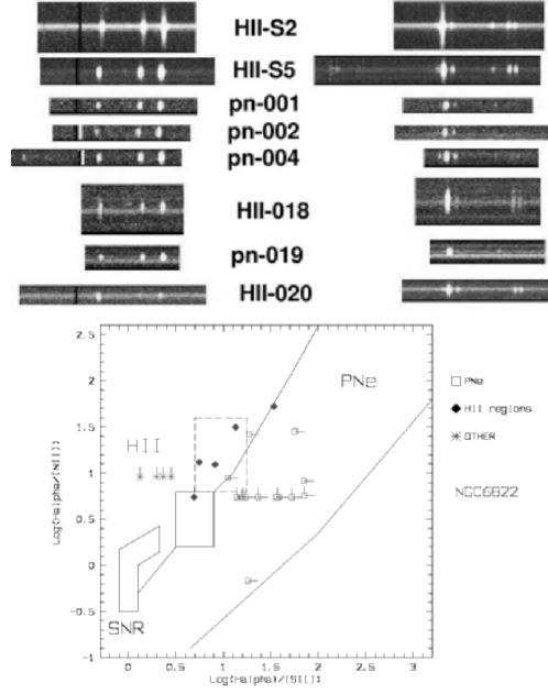
Fig. 2. 2-D NTT spectra: ( upper ): ( left ) blue spectra shortward of [\text{OIII}] 5007Å; and ( right ) red spectra in the H_\alpha region. ( bottom ) [\text{NII}]/H_\alpha - [\text{SII}]/H_\alpha diagnostic diagram to disentangle the different emission line objects.
