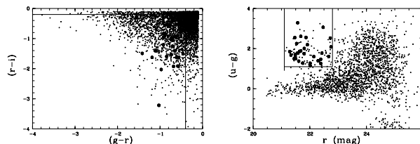
Fig. 1. Color-magnitude diagrams for stellar sources from SDSS M31 data to which we applied our selection procedure. All previously known re-identified PNe from the literature are shown with fat dots. Our color-magnitude criteria for selecting these candidates are indicated by solid lines. All previously identified PNe are located within a relatively small range of luminosities of \sim 1.5 mag that shows the depth of previously published surveys for PNe in the outer disk and halo of M31.
