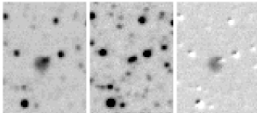
Fig. 1. An SMC PN identified by Jacoby & De Marco with the CTIO 4-m showing the on-band (left) and off-band (center) images. The right panel shows the “difference” image (with aliasing from imperfect subtractions). This candidate is not yet confirmed, but has coordinates \alpha_{2000} = 00\ 49\ 53.8 , \delta_{2000} = -71\ 47\ 33 and is \sim 4 arcsec in diameter.
