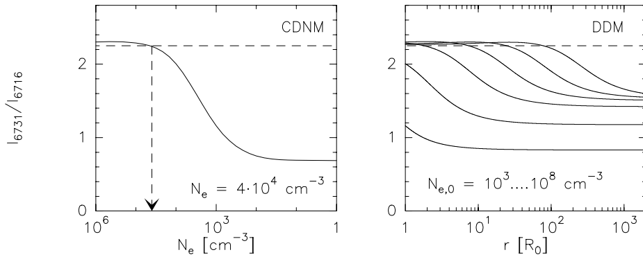
Fig. 3. Left: Constant electron density in CDNM derived from the observed (dashed line) sulfur line ratio. Right: The sulfur line ratios in case of DDM for N_{\text{e},0} ranging from 10^3 \text{ cm}^{-3} (lower left) to 10^8 \text{ cm}^{-3} (upper right). The observed ratio (dashed line) limits N_{\text{e},0} to values \gtrsim 10^5 \text{ cm}^{-3} . The crossing point between model and observation defines the outer edge of the emitting shell for each model
