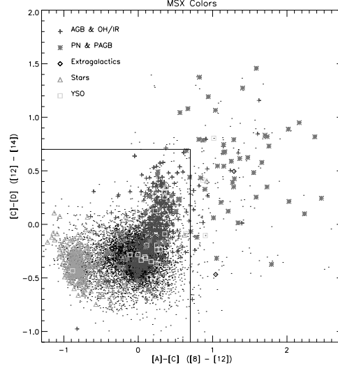
Fig. 2. [A] - [C] vs. [C] - [D] two-colour diagram showing all the sources with a good identification in SIMBAD (see legend), together with those for which their nature is unknown (small dots). Note the characteristic colours shown by different types of source. The solid lines indicate the colour criteria defined in the text to search for new PNe among the unidentified sources.
