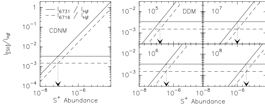
Fig. 4. [S II] over H \beta intensity ratio as a function of S ^+ abundance for CDNM (left) and DDM (right) for the different possible N_{e,0} values as indicated. Horizontal lines indicate observed ratios, arrows indicate the derived S ^+ abundance. All abundances found with DDM are clearly larger than that for CDNM.
