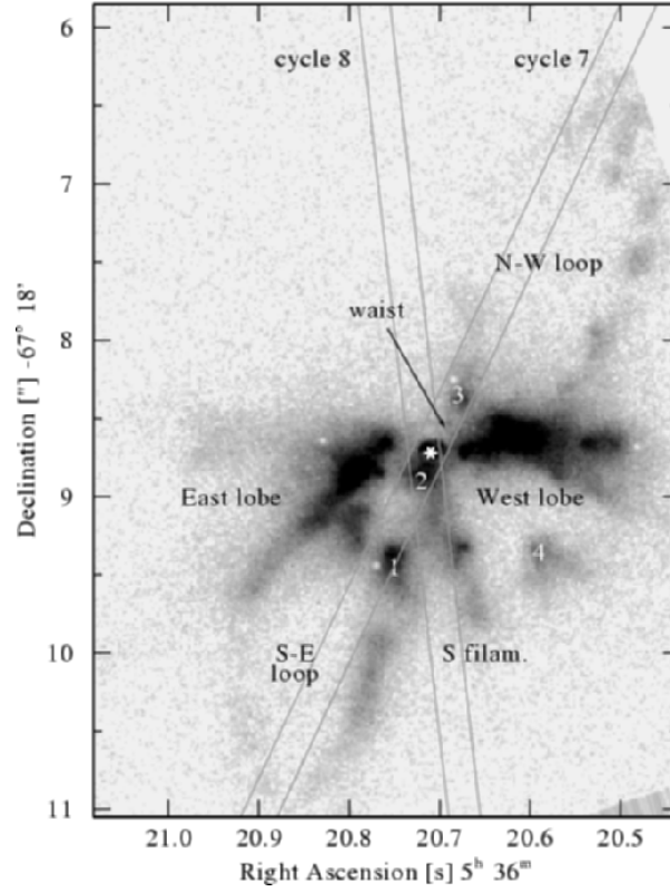
Fig. 12. HST Faint Object Camera (not WFPC) image of LMC N66 (=WS35) in the [O III] 5007 Å line, acquired in February 1994 when the central star was near peak brightness. From Peña et al. (2004).
