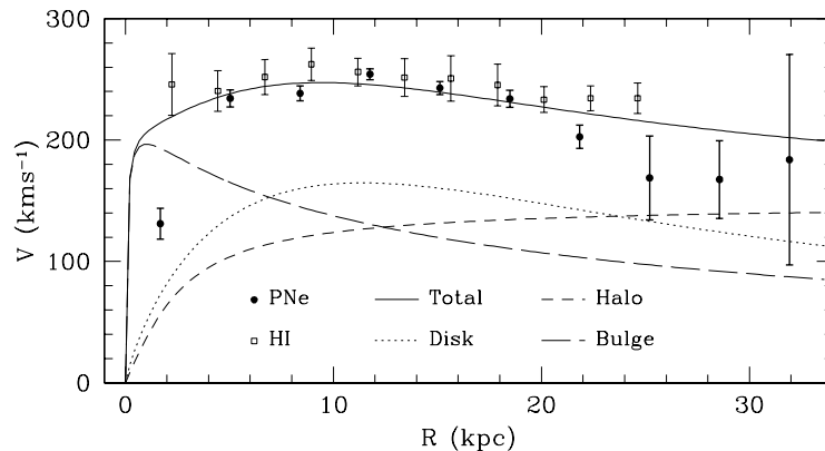
Fig. 2. PNe rotation curve. The filled circles are the PNe data (binned into 10 concentric rings with the PNe nearest the minor axis eliminated), corrected for the line-of-sight integration through a disk of scale height z_0 and the asymmetric drift. The open squares show the averaged HI data presented in [12]. The lines are model fits for a three component model, fit to all the corrected PNe beyond 3.36 kpc
