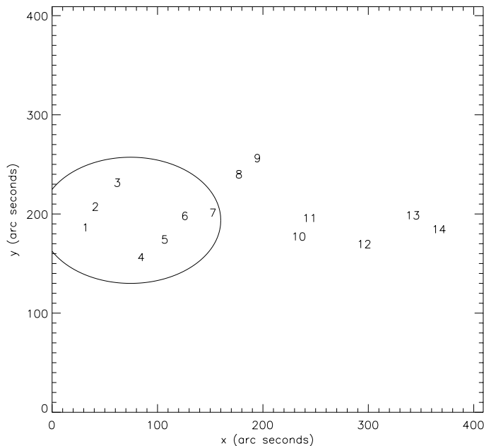
Fig. 2. Positions of the 14 bright PNs relative to the core of NGC 4697. The area and orientation of this figure are as in Fig. 7 of Méndez et al. (2001). The effective radius of NGC 4697 is 95 arc seconds
