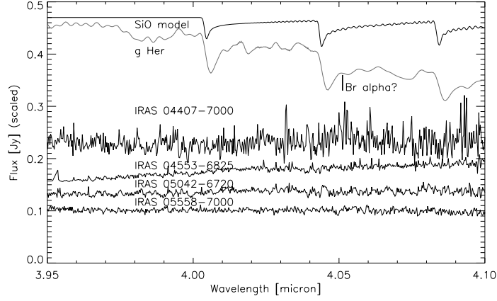
Fig. 3. The spectra of the oxygen-rich stars
