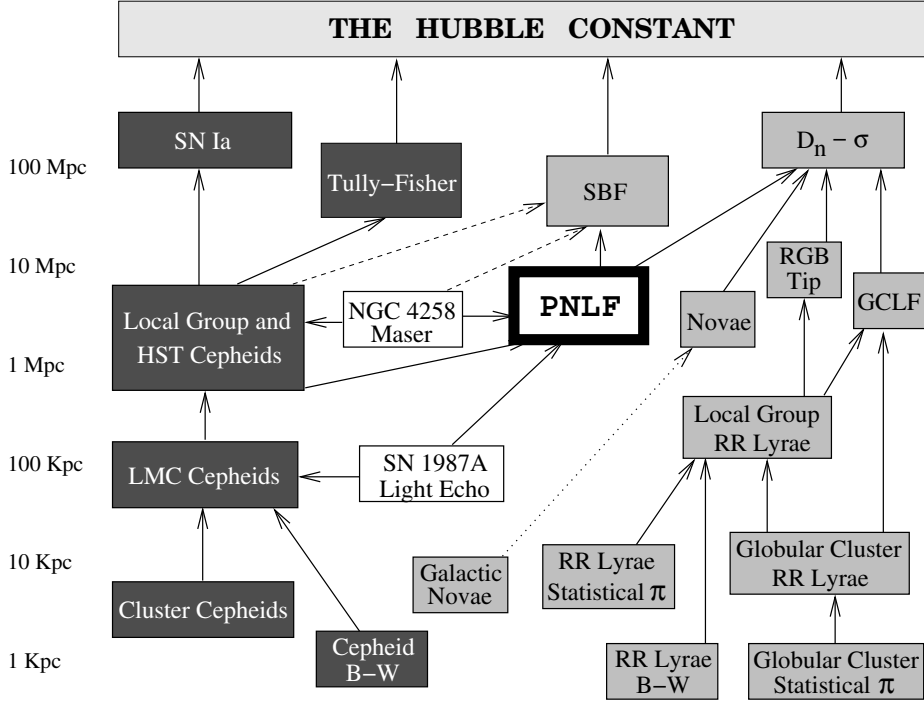
Fig. 1. The extragalactic distance ladder. The dark boxes show techniques useful in star-forming galaxies, the lightly-filled boxes give methods that work in Pop II systems, and the open boxes represent geometric distance determinations. Uncertain calibrations are noted as dashed lines. The PNLf is the only method that is equally effective in all the populations of the Local Supercluster.
