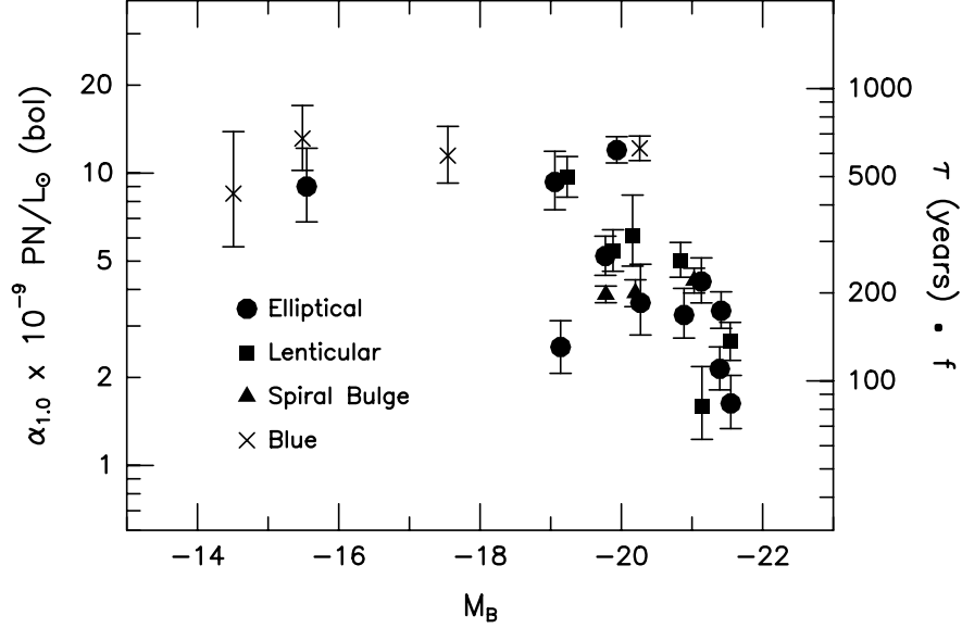
Fig. 5. The bolometric luminosity-specific number of PNe in the top 1 mag of the [O III] \lambda 5007 PNLF plotted as a function of galactic absolute B magnitude. The right side of the y -axis translates this number into a constraint on the PN lifetime using a luminosity-specific stellar evolutionary flux of 2 \times 10^{-11} stars \text{yr}^{-1} L_{\odot} . Either the [O III]-bright PNe of giant ellipticals live very short lives, or a substantial fraction of the stars in these galaxies do not contribute to the bright-end of the PNLF.
