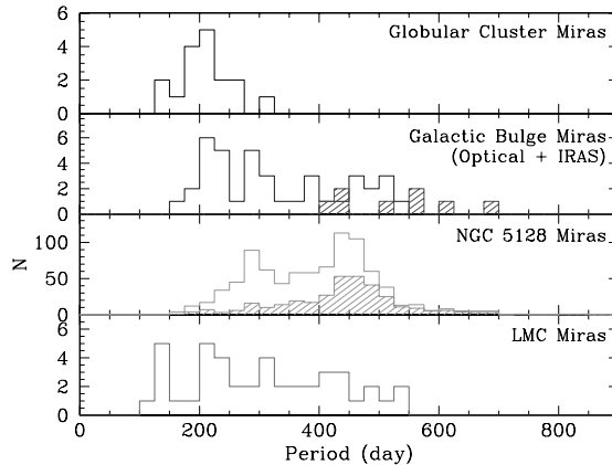
Fig. 3. Period distribution of LPVs in NGC 5128 (second panel from bottom) is compared with: Galactic globular clusters (age \sim 12 Gyr; [M/H] > -1 dex) Miras; Milky Way Bulge (age \sim 10 Gyr, [M/H] \sim 0.0 dex); and the LMC (mostly age < 3 Gyr, [M/H] \sim -0.7 dex) Miras. See Rejkuba (2003b) for further details.
