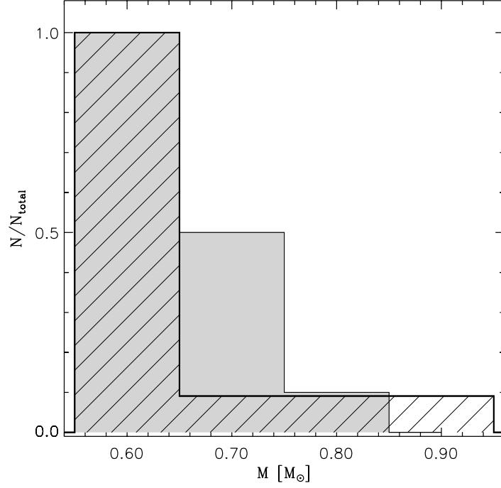
Fig. 3. Normalized mass distribution for the CSs in the SMC (dashed) and LMC (in gray) [62].
