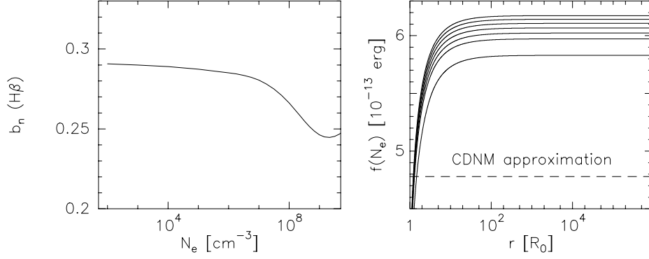
Fig. 1. Left: b_n factor for H\beta as a function of electron density. For low values of N_e , it is fairly constant. Right: The function f(N_e) of Eq. (2) for values of N_{e,0} ranging from 10^2 \text{ cm}^{-3} (top) to 10^8 \text{ cm}^{-3} (bottom). Also shown is the CDNM value (dashed line)
