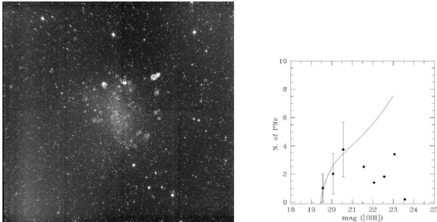
Fig. 1. (a): Image of NGC 6822 showing spatial distribution of the 17 PNe. (b): PNLF of the 17 PNe in NGC 6822.
