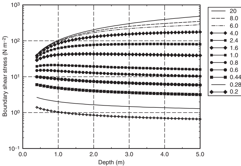
FIG. 10 Boundary shear stress on the average floodplain from a one-layer model as a function of flow depth and stem spacing. At a stem spacing of 20 m, the form drag on the shrubs is negligible, so the top curve represents the same boundary shear stress from the depth-slope product as did the top curve on Fig. 8. This line would be straight if the y-axis were arithmetic and not logarithmic. When the shrubs affect the flow all the way to the surface, the boundary shear stress decreases with flow depth at first, then becomes nearly independent of it. In fact, it does not increase with flow depth for flows deeper than 2 m until there is only one stem in a square 1.6 m on a side. At a stem spacing of 1.0 m the boundary shear stress does not increase with flow depth for depths greater than 1.0 m. The magnitude of the boundary shear stress in a carr of stiff shrubs, therefore, is controlled by stem spacing, not flow depth, as long as the depth is not less than the stem spacing.
