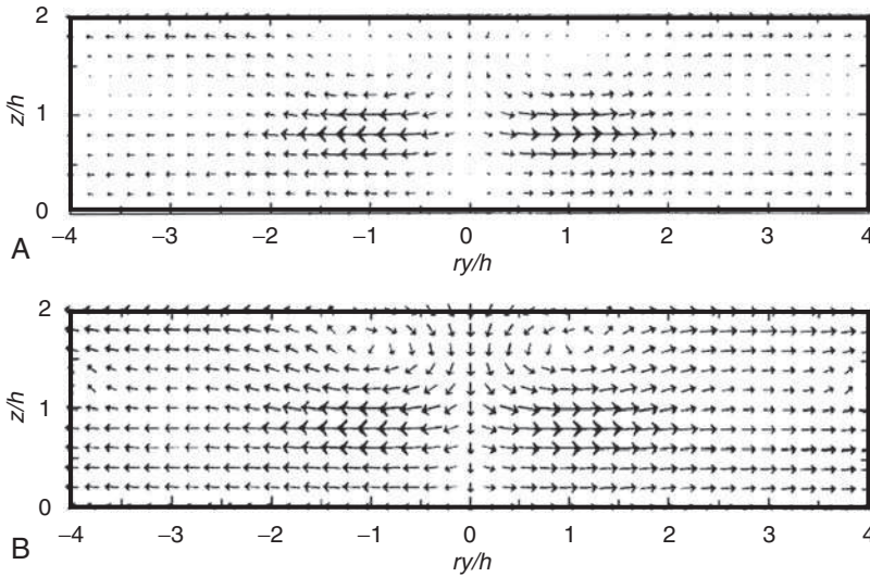
FIG. 7 The v', w' vector field of the characteristic eddy projected onto the (ry, 0, z) plane, where the horizontal coordinate ry is relative to the notional center of the eddy. (A) Arrow lengths are proportional to the magnitude of the velocity vector. (B) Arrow lengths in regions of low velocity are magnified to show the flow direction more clearly. (From Finnigan and Shaw [2000], reprinted with permission of Springer Science and Business Media.)
