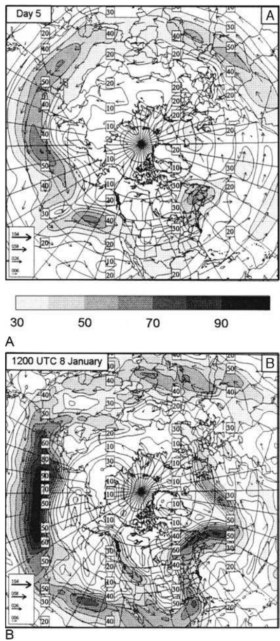
FIG. 9 Winds ( \text{m s}^{-1} ) at 250 hPa, showing jet streams at (A) day 5 of the composite average and (B) 1200 UTC, January 8, 1998. (Adapted from Higuchi et al. [2000].)
