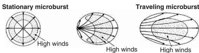
FIG. 16 Schematic of microburst outflows affected by storm movement. Stationary microburst with radial outflow, moderate speed, and high-speed traveling microburst (Fujita, 1985; courtesy of the Tetsuya “Ted” Fujita Collection, Southwest Collection/Special Collections Library, Texas Tech University, Lubbock, TX).
