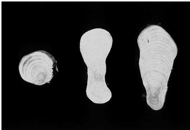
FIG. 10 Examples of the adaptive growth of roots in response to mechanical stresses showing uneven growth leading to roots resembling I beams and T beams.
