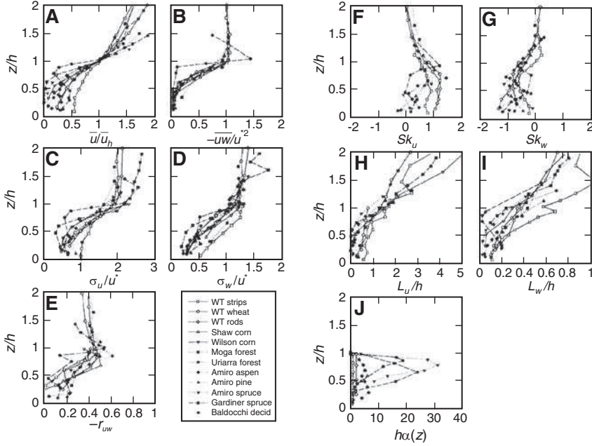
FIG. 4 A “family portrait” of canopy turbulence for canopies A to L in Table 1, showing profiles with normalized height z/h of (A) U/U_b = \bar{u}(z)/\bar{u}(h) ; (B) -\overline{u'w'}/u^*{}^2 ; (C) \sigma_u/u^* ; (D) \sigma_w/u^* ; (E) -\overline{r_{uw}} = -\overline{u'w'}/\sigma_u\sigma_w ; (F) Sk_u ; (G) Sk_w ; (H) L_u ; (I) L_w ; (J) h\alpha(z) , where \alpha(z) is leaf area per unit volume. L_u and L_w are integral length scales derived by applying Taylor’s hypothesis to the point-valued integral time scales of the fluctuating velocity (Finnigan, 2000). (From Raupach et al. [1996], reprinted with permission of Springer Science and Business Media.)
