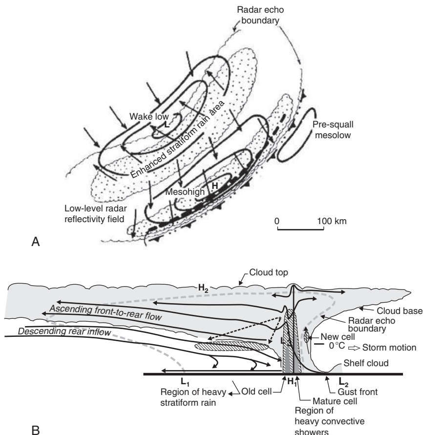
FIG. 12 Schematic diagrams of a large squall line: (A) Surface plot. Shading denotes moderate-heavy rain areas. Wake low and mesohigh pressure areas are contoured (from Johnson and Hamilton, [1988]). (B) Vertical cross-section. Shaded areas denote higher reflectivity associated with convective line and bright band. Ascending front-to-rear outflow in deep anvil and descending rear-to-front flow at midlevels are also shown (Houze et al. [1989]).
