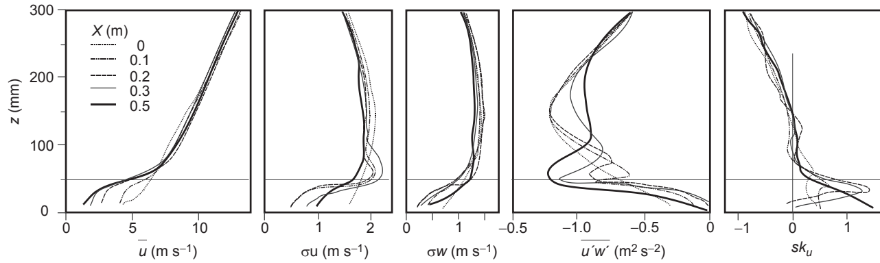
FIG. 18 Consecutive vertical profiles of velocity statistics at and behind a forest edge. The wind tunnel model canopy is 0.05 m high so profiles are at x/h = 0, 2, 4, 6 , and 10. (From Raupach et al. [1987], reprinted with permission from CSIRO Marine and Atmospheric Research.)
