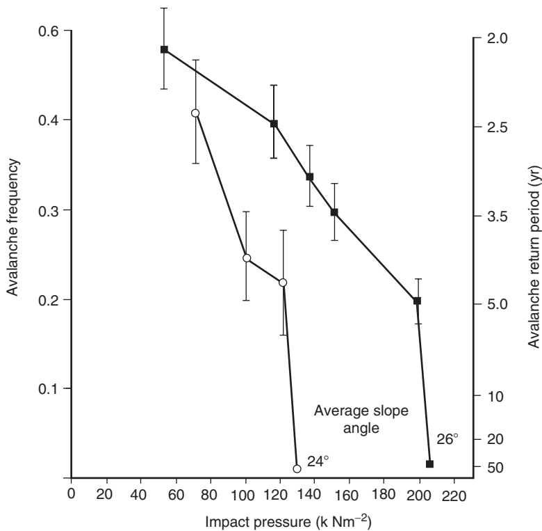
FIG. 4 Changes in impact pressure ( \text{k Nm}^{-2} ) of avalanches down slope.
