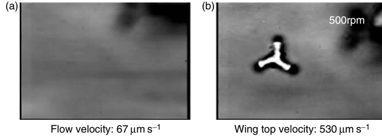
Fig. 4.67. Visualization of two-liquid mixing: without mixer (a), with mixer (b); 20% milk fat colloid for visualization was included only in the NaOH solution
