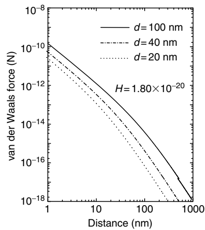
Fig. A.18. van der Waals force dependence on distance between particle and wall
