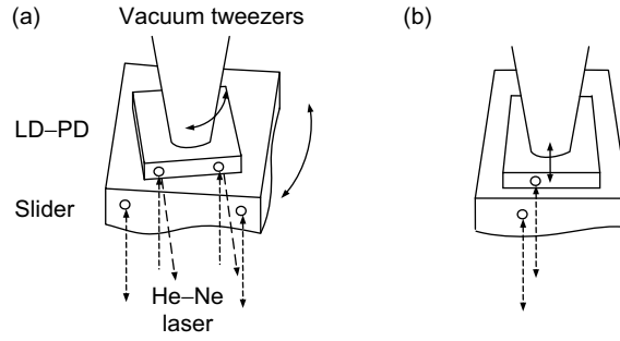
Fig. 2.10. Method of bonding an LD-PD chip on a slider. First, the LD-PD chip is pushed onto the electrode of the slider's back end with vacuum tweezers and then rotated to align it parallel to the slider surface (a). Second, the moving stage on which the LD-PD chip is mounted is translated (b)
