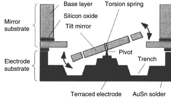
Fig. 1.20. Single-crystalline mirror actuated by electrostatic force applied via terraced electrodes. Reprinted from [1.40] with permission by T. Yamamoto, NTT, Japan
