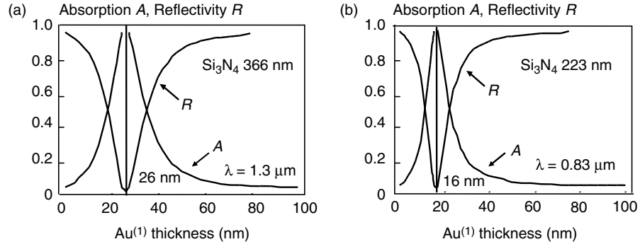
Fig. 2.52. Total absorption A and reflectivity R of \text{Au}/\text{Si}_3\text{N}_4/\text{Au} versus the \text{Au} thickness at the optimum \text{Si}_3\text{N}_4 thickness for wavelengths of 1.3\mu\text{m} (a), and 0.83\mu\text{m} (b)
