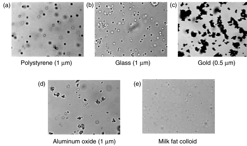
Fig. 4.50. Various particles used to visualize microflow
