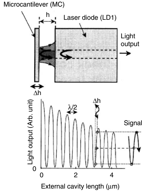
Fig. 2.25. Maximum peaks in the light output occur every \lambda/2 and their amplitude decays exponentially in proportion to the external cavity length
