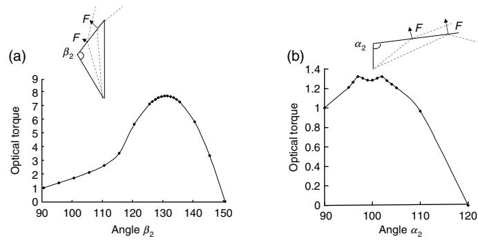
Fig. A.8. Relationship between optical torque and side wall angle \beta_2 (a), and side wall angle \alpha_2 (b), both simulated in two dimension for simplicity
