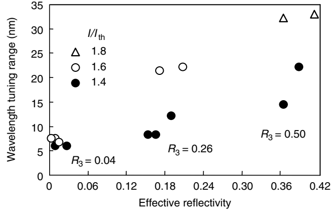
Fig. 2.18. Dependence of wavelength tuning range on the effective reflectivity R_2^{\text{eff}} , with I/I_{\text{th}} as a parameter
