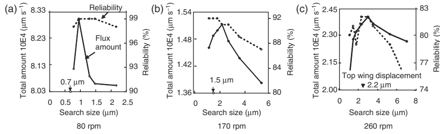
Fig. 4.56. Determination of optimum search size for rotation rates of 80, 170, and 260 rpms; arrow shows displacement of wing top per frame (1/120 s). The optimum search size is that at which flux amount reaches a maximum
