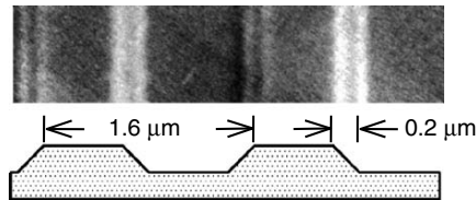
Fig. 5.30. SEM photograph of optical disk groove and its profile
