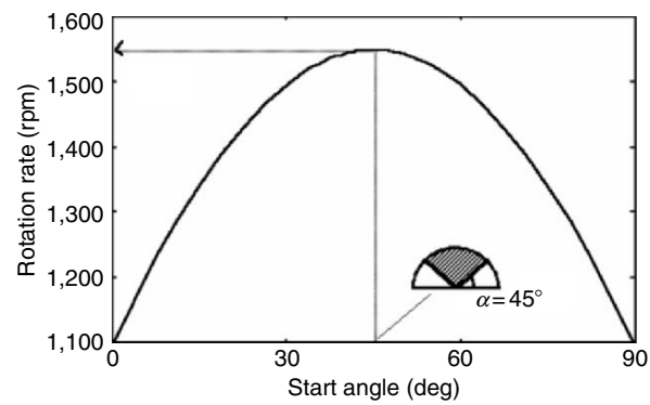
Fig. A.12. Relationship between rotation rate and starting angle \alpha of the slope. The span of the slope forms from \alpha to \alpha + 90^\circ
