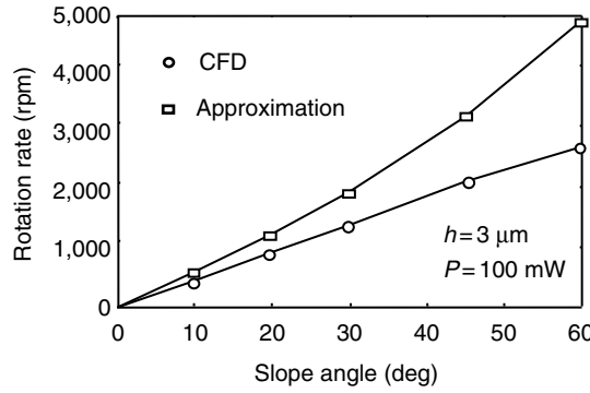
Fig. 4.35. Rotation rate obtained by approximation and CFD with slope angle as a parameter
