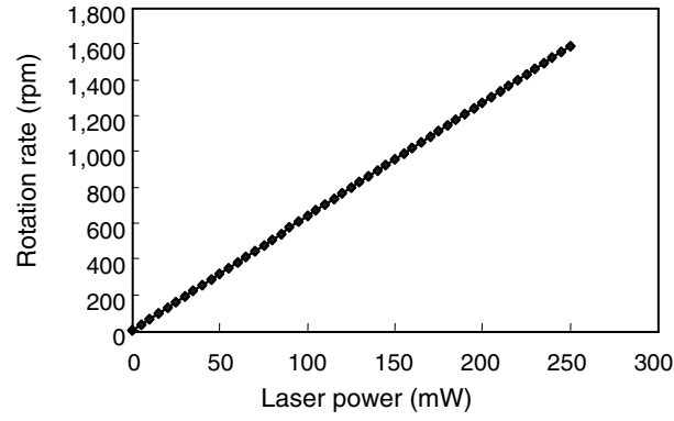
Fig. 4.30. Shuttlecock rotor rotation rate dependence on a laser power
