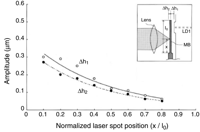
Fig. 2.28. Variation in MC vibration amplitude as a function of the illuminated spot position on the MC
