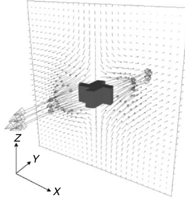
Fig. 4.23. Squint view of velocity vectors in the proximity of optical rotor for 200 rpm
