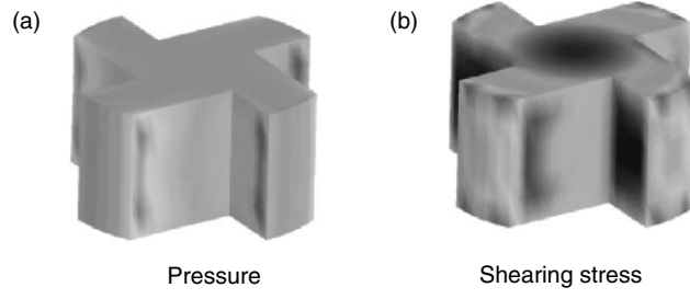
Fig. 4.28. 3-D images of the pressure distribution (a), and the shearing stress distribution (b)
