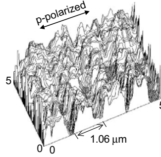
Fig. 5.27. SNOM images (scattered light intensity) of refractive index grating obtained by gold particle probe with p-polarized illumination
