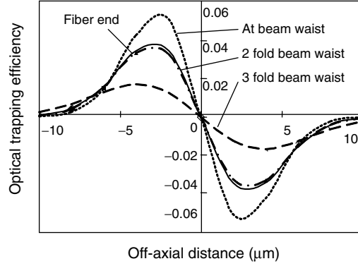
Fig. 3.21. Variation in transverse trapping efficiency for a 2.5- \mu\text{m} -radius microsphere as function of off-axial distance, with beam axial distance as a parameter
