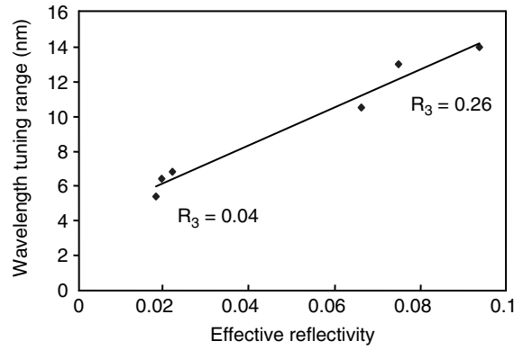
Fig. 2.21. Dependence of tuning range on R_2^{\text{eff}}
