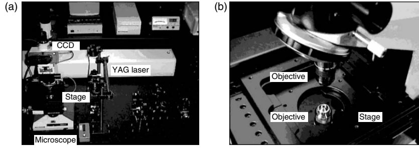
Fig. 3.27. Photograph of optical trapping apparatus. Upper and lower objective lenses are seen around the microscope stage lower left in (a). Two objective lenses used in trapping particles in water with downward-directed and upward-directed laser beams (b)
