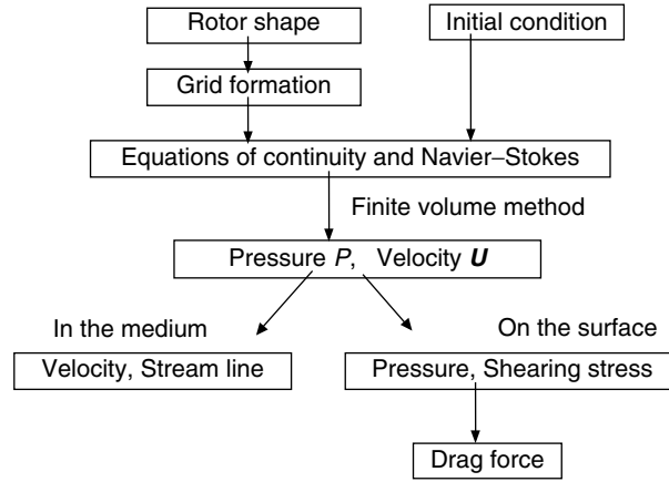
Fig. 4.22. Process for flow field and drag force analyses of optical rotor in water at room temperature by computational fluid dynamics (CFD)
