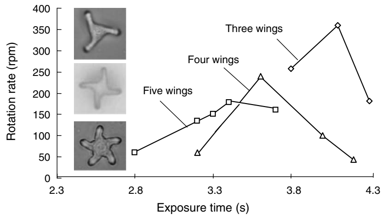
Fig. 4.43. Measured rotation rates for three kinds of rotors
