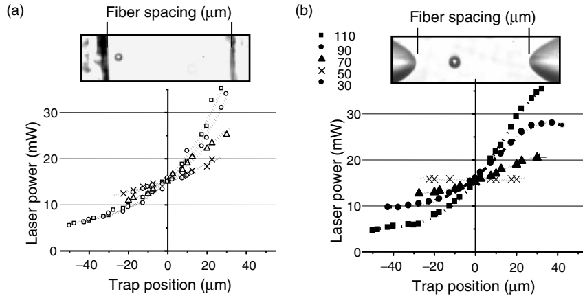
Fig. 3.34. Relationship between trap equilibrium position and output power from left side fiber ranging from 0 to 40 mW when output power is 15 mW from right side fiber for different spacings between fiber lens
