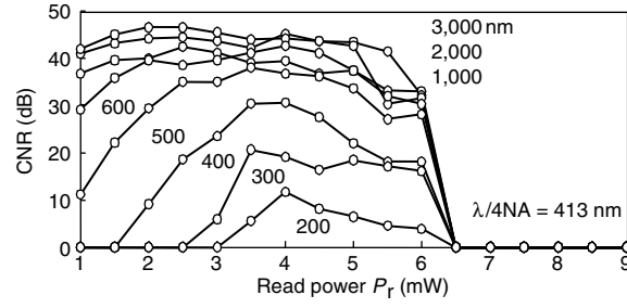
Fig. 5.56. Read power dependence on CNR of mark written at power of P_w = 8.5 mW, with mark length as parameter
