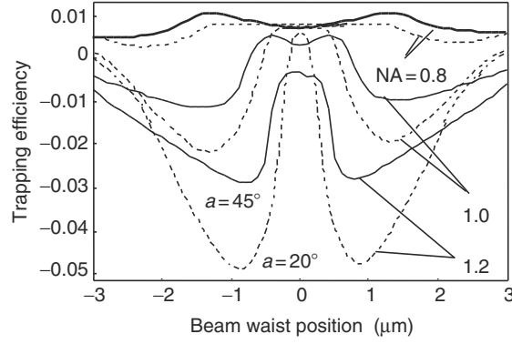
Fig. 4.11. Trapping efficiency Q vs beam waist position for the slope angles of a = 20^\circ (dotted lines) and 45^\circ (solid lines) with numerical aperture NA as a parameter
