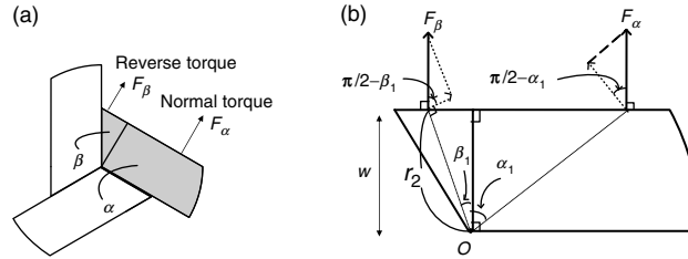
Fig. A.7. Optical torques induced in three-wing rotor. Not only normal torque but also reverse torque is generated.
