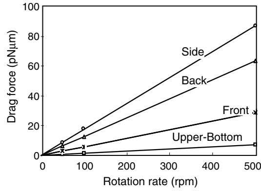
Fig. 4.29. Drag force at different parts of the shuttlecock rotor
