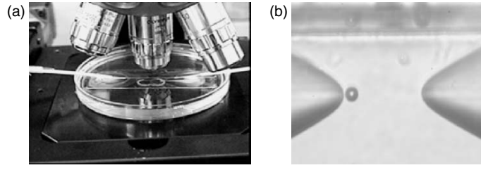
Fig. 3.33. Photographs of setup around fiber ends (a), and dual tapered fiber trap (b)
