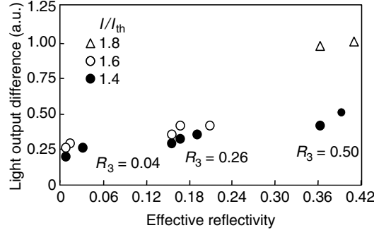
Fig. 2.15. Light output difference versus effective reflectivity, with I/I_{th} as parameters
