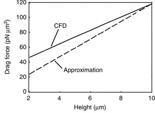
Fig. 4.33. Drag force obtained by CFD and the approximation method with rotor height as a variable
