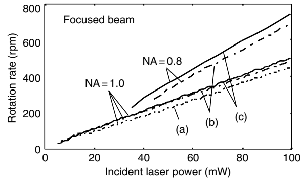
Fig. 4.17. Relationship between rotation rate and incident laser power for different beam profiles
