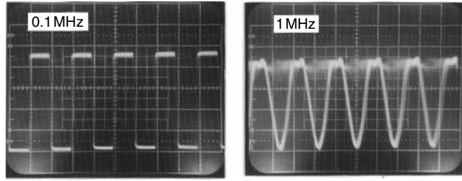
Fig. 2.43. Reproduced signals of the written bit at 0.1 and 1 MHz for a duty cycle of 50%
