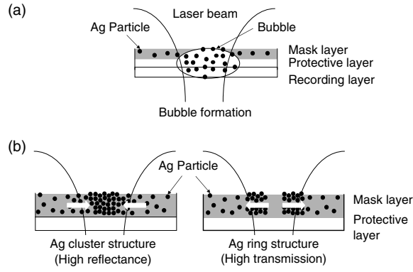
Fig. 5.48. Bubble pit formation and functional structures of scattered-type super-RENS disk using \text{AgO}_x mask layer [5.55]
