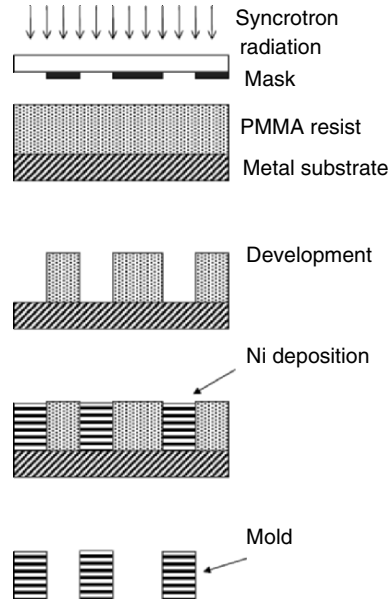
Fig. 1.6. Lithographie galvanofomung abformung (LIGA) involves X-ray lithography and electrodeposition processes
