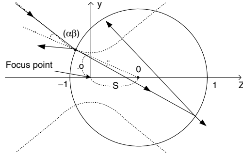
Fig. 3.14. Geometry for calculating exact axial trapping efficiency for microsphere considering beam waist
