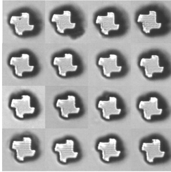
Fig. 4.45. Shuttlecock optical rotors, 30 \mu\text{m} diameter and 15 \mu\text{m} thick, fabricated by photoforming
