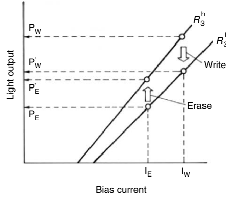
Fig. 2.58. Write-erase performance for a phase change medium. The write-erase power margin, P_W - P'_E and P'_W - P_E , for a phase change medium is shown
