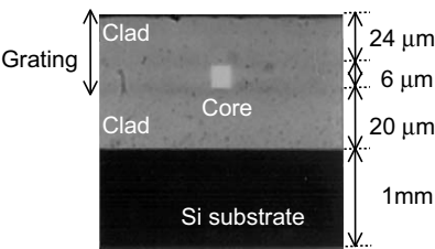
Fig. 5.25. Sectional view of refractive index grating fabricated by UV exposure through phase mask. The grating is formed in a clad layer on a PLC. Courtesy of T. Maruno and Y. Hibino, NTT, Japan
