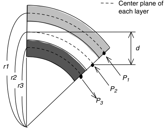
Fig. 2.47. Deflection of a bimorph MC and internal stress due to temperature change
