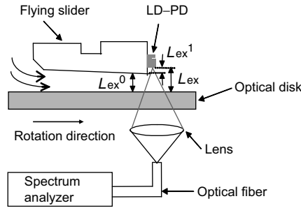
Fig. 2.8. Proposed set up for measurement of wavelength tuning based on ESEC length. An LD attached to an air-bearing slider flies by air resistance caused by disk rotation (upside down in reality)
