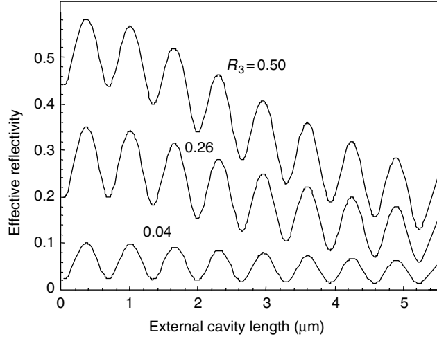
Fig. 2.4. Dependence of effective reflectivity R_2^{\text{eff}} on external-cavity-length L_{\text{ex}}
