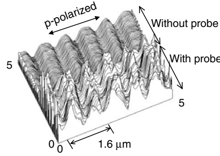
Fig. 5.31. SNOM topography of optical disk tracking groove with/without gold particle probe under p-polarized illumination
