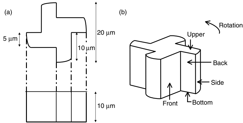
Fig. 4.27. Side view indicating the size of the rotor (a), and sectional view indicating the name of its side parts (b)
