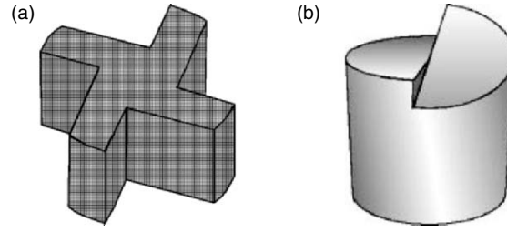
Fig. 1.26. Two kinds of optical rotors: a rotationally but not bilaterally symmetric rotor which uses optical torque exerted on its side surfaces (a), and a cylindrical optical rotor which has slopes for rotation on its upper surfaces (b)
