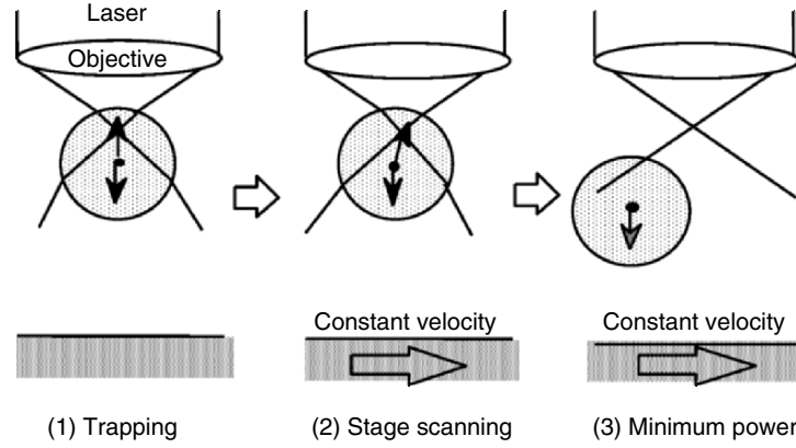
Fig. 3.30. Method of measuring transverse trapping power as minimum power for trapping a particle moving at the constant velocity of v in water
