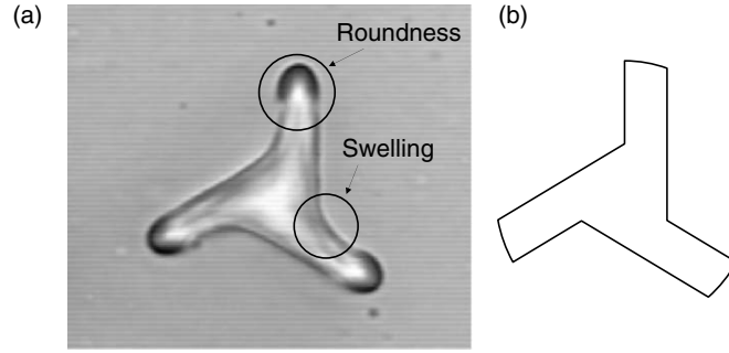
Fig. 4.42. Example of fabricated three-wing rotor shape (a) compared with the mask shape (b)
