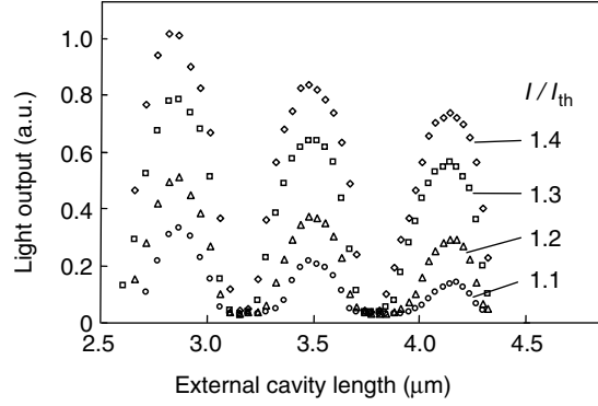
Fig. 2.14. Light output versus external-cavity-length L_{\text{ex}} (= L_{\text{ex}}^0 + L_{\text{ex}}^1) , drive current I/I_{\text{th}} normalized by threshold current as a parameter, where R_1 = 0.32 , R_2 = 0.01 , and R_3 = 0.5
