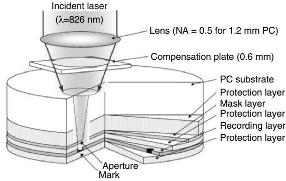
Fig. 5.40. Typical super-RENS disk medium using Sb mask layer. Optical diffraction limit for detection \lambda/4\text{NA} is 413 nm
