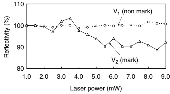
Fig. 5.51. Initialization effect on as-depo medium of the scattered type super-RENS disk with read power of 1 mW, medium velocity of 2 \text{ m s}^{-1} , and mark length of 3,000 nm
