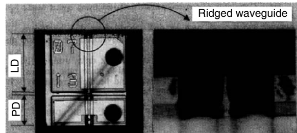
Fig. 1.33. Photograph of a laser diode (LD) integrated with a photodiode (PD). To reduce the beam width parallel to the junction plane, a taper-ridged waveguide is fabricated on the edge of the diode cavity by reactive ion beam etching (RIBE)
