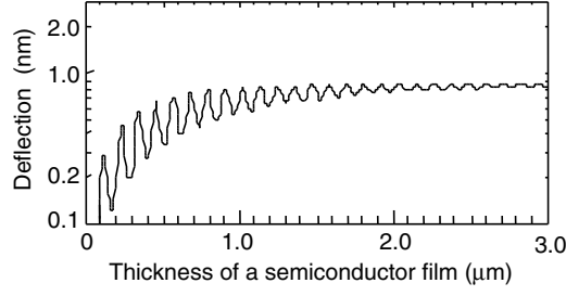
Fig. 2.45. Calculated relationship between photothermal tip deflection and thickness for a GaAs MC
