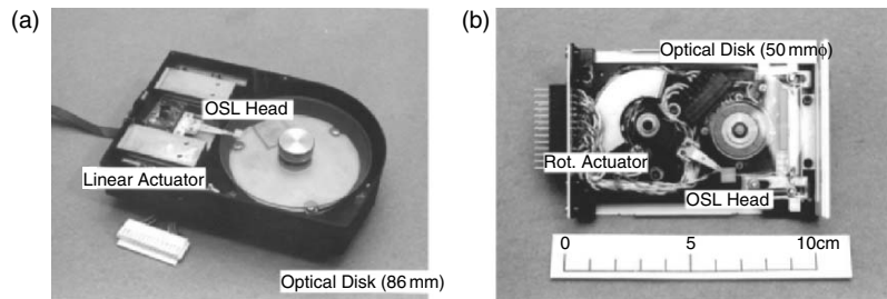
Fig. 2.33. Experimental optical disk drive using an OSL flying head and a phase change recording medium: linear actuator type (a), and rotary actuator type (b)
