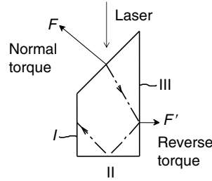
Fig. 4.19. Optical torque exerted for the shuttlecock rotor with slopes
