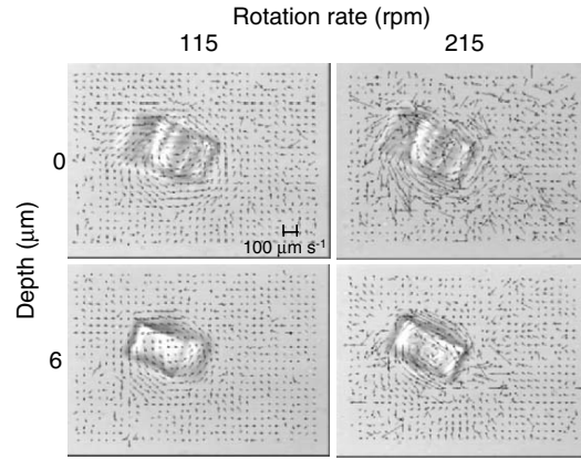
Fig. 4.59. Velocity vectors around optical mixer for vertical rotation, with observation depth and rotation rate as parameters
