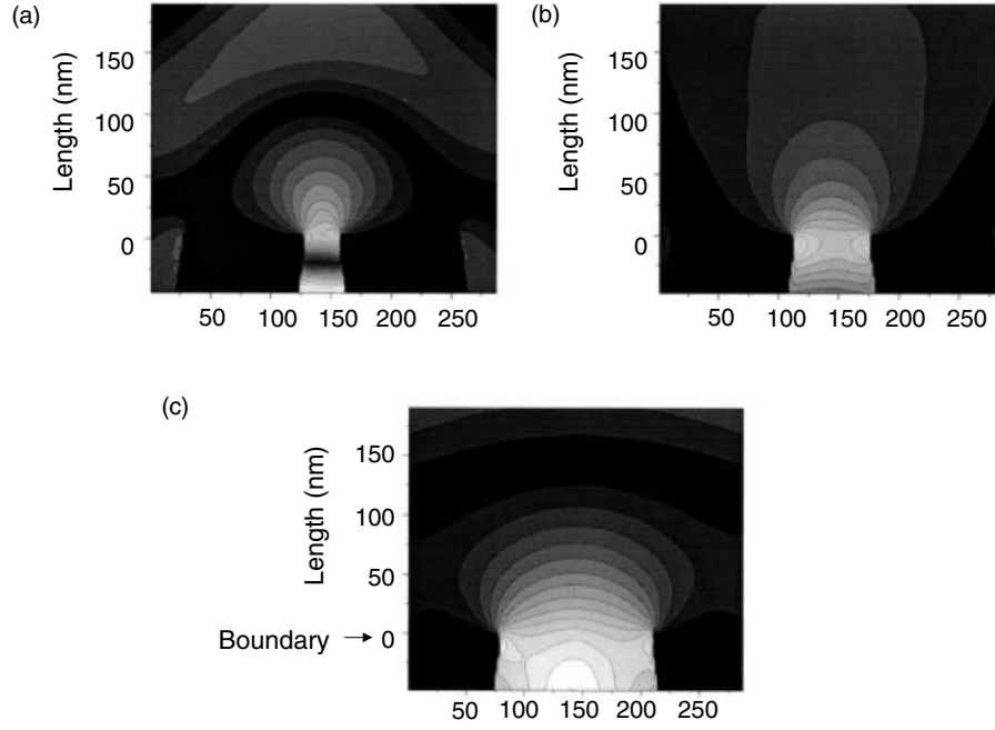
Fig. 5.10. Calculated electric field E_x around aperture for TM plane wave. The evanescent light becomes sharp as the diameter of the aperture becomes small
