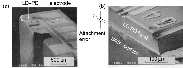
Fig. 2.12. Photograph of the back end of the slider on which an LD-PD chip is bonded to the electrode (a), and the LD-PD facet and the slider surface (b). The attachment error L_{\text{ex}}^1 is less than 1\mu\text{m} . Courtesy of H. Nakata, NTT, Japan
