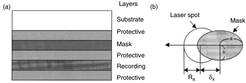
Fig. 5.35. Medium composition with mask layer/protective layer/recording layer (a), and schematic illustration of partial readout principle of superresolution optical disk (b)
