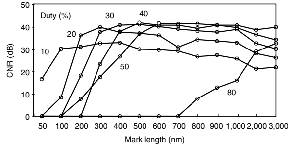
Fig. 5.60. Relationship between CNR and mark length for super-RENS readout ( P_r = 4 \text{ mW} ), with optical pulse duty as parameter
