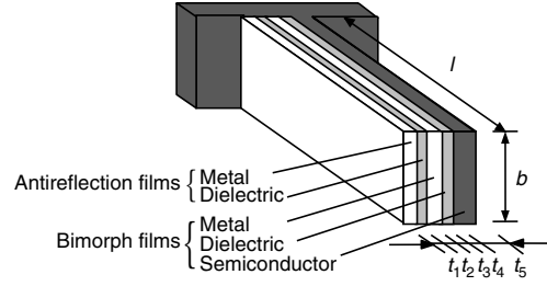
Fig. 2.53. Schematic drawing of a five-layer MC
