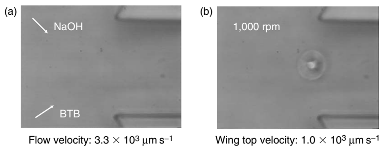
Fig. 4.66. Merging of the flows of NaOH solution ( 4\text{ mmol/L} ) and BTB solution (a), and optical mixer ( d = 20\text{ }\mu\text{m} ) with the rotation rate of 1,000 rpm at the power of 200 mW (b)
