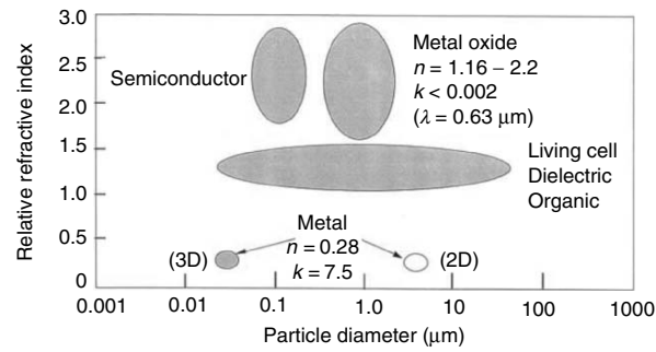
Fig. 3.38. Reported materials and sizes possible for optical trapping by YAG laser beam. Various particles ranging from 20 nm to tens micrometer in size including biological, dielectric, polymer and metal particles are included
