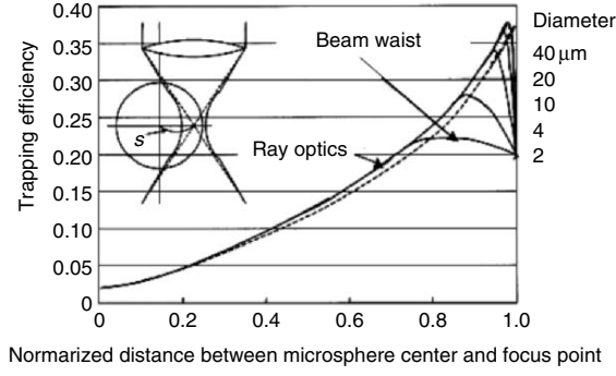
Fig. 3.16. Transverse trapping efficiency of polystyrene microsphere by two converging ray approximations
