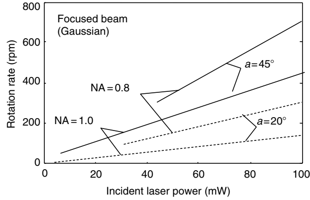
Fig. 4.14. Relationship between rotation rate and laser power for two NAs assuming M_{\text{opt}} = M_{\text{drag}} (= 4\pi\mu r^2 h\omega)
