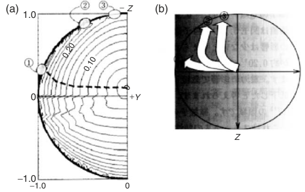
Fig. A.6. Contour lines for total trapping efficiency Q_t of polystyrene particle; broken line indicates along which Q_t is purely horizontal (a). Expected trajectory of trapping position; 1: for diameter less than 20\mu\text{m} , 2: for diameter of 30\mu\text{m} , 3: for diameter greater than 40\mu\text{m} (b)
