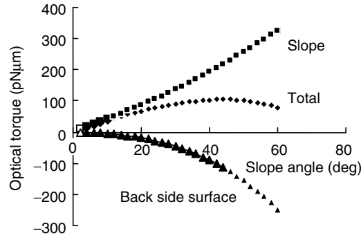
Fig. 4.20. Simulated optical torque dependence on the slope angle of the shuttlecock rotor
