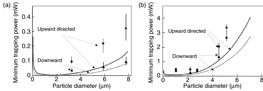
Fig. 3.28. Dependence of minimum axial trapping power on diameter for polystyrene spheres (a), and glass spheres (b)
