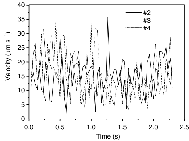
Fig. 4.52. Variation in tracer velocity due to the flow generated by the rotor and the Brownian motion. Notation # corresponds to that of Fig. 4.51
