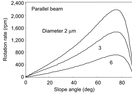
Fig. 4.8. Dependence of rotation rate on slope angle, with rotor diameter as a parameter ( P = 100 \text{ mW} )
