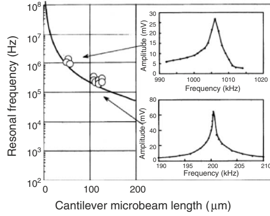
Fig. 2.29. Resonance frequency and frequency spectra as a function of MC length for GaAs
