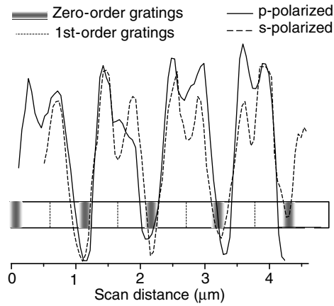
Fig. 5.29. Relationship between scattered light intensity and refractive index grating distribution
