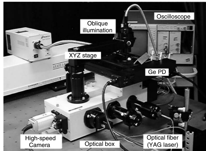
Fig. 4.48. Photograph of experimental apparatus to visualize the microflow around rotor
