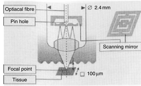
Fig. 1.25. Microconfocal optical scanning microscope fabricated for minimally invasive medical diagnosis and treatment (m-COSM). Reprinted from [1.53] with permission by M. Esashi, Tohoku University, Japan
