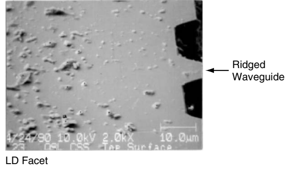
Fig. 2.44. SEM photograph of LD facet after 10,000 contact start/stop (CSS) cycles in an office environment (class 350,000). The disk has an SiN/SbTeGe/SiN/plastic substrate structure and is used at low rotation of 900 rpm
