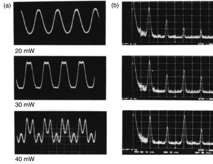
Fig. 2.26. Resonant signal amplitude and spectrum versus LD2 light power. The signal amplitude increases as the light power increases, but an inversion appears in the signal peak for the light power over 30 mW, because the vibration amplitude becomes larger than \lambda/4
