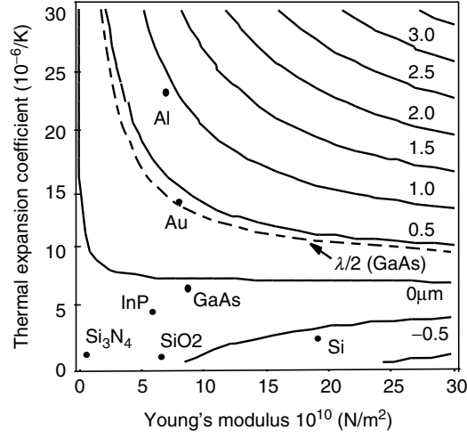
Fig. 2.49. Contour map of an MC deflection, with Young's modulus E and thermal expansion coefficient \alpha as parameters
