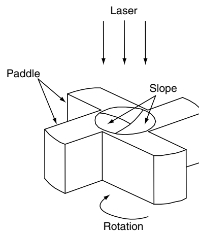
Fig. A.14. Optical mixer suitable for used in a microchannel of future \mu -TAS
