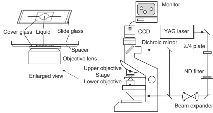
Fig. 3.26. Experimental setup for trapping and manipulating microobjects using upward-directed and downward-directed YAG laser beams with wavelength of 1.06\ \mu\text{m}
