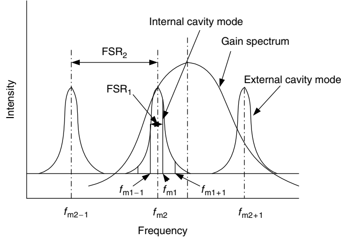
Fig. 2.5. Model of lasing frequency of the ESEC LD. Lasing occurs at the frequency f when the internal mode frequency f_{m1} coincides with the external mode frequency f_{m2} in the gain spectrum curve
