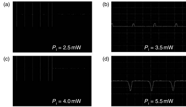
Fig. 5.50. Effect of initialization laser power P_i on reproduced signals
