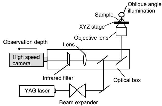
Fig. 4.47. Experimental setup to visualize microflow around mixer. The upward-directed YAG laser traps the rotor. Generated microflows are visualized with oblique angle illumination
