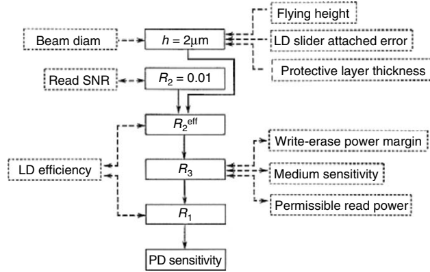
Fig. 2.56. Reflectivity design guideline for an optical disk using OSL head.
