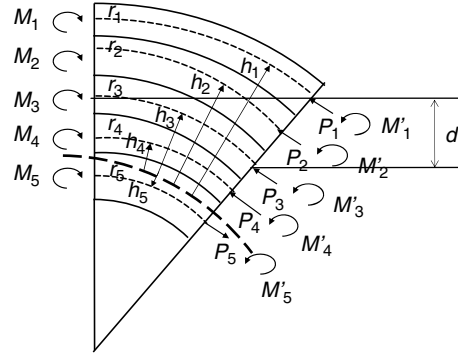
Fig. 2.54. Deflection of a five-layer MC and internal stress due to temperature change
