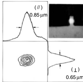
Fig. 2.34. Near field pattern of the emitted light from a 1.2\text{-}\mu\text{m} wide taper-ridged waveguide
