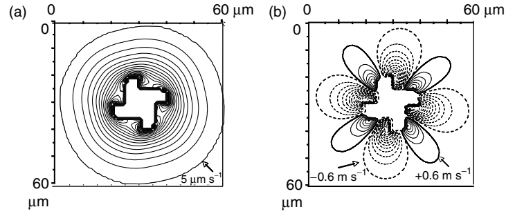
Fig. 4.24. Contour lines around optical rotor for horizontal component (a), and vertical component (b)
