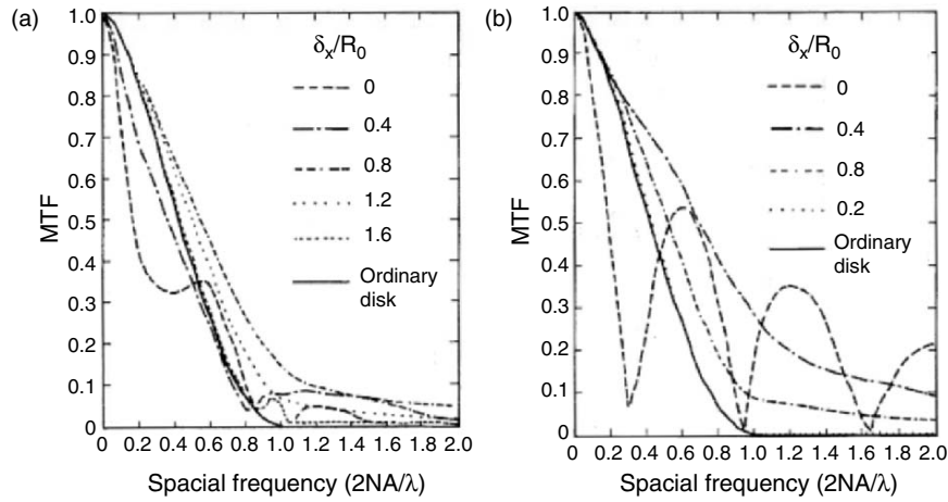
Fig. 5.36. Calculated MTF of system with ideal mask, relative shift \delta x as parameter (a), and with 90^\circ rotation different mask shape (b). Reprinted from [5.38] with permission by Yi hong Wu
