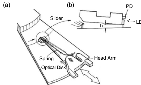
Fig. 2.32. Schematic representation of an optically switched laser (OSL) head flying on an optical disk (a), and detailed view of the flying slider on which an LD–PD is mounted (b)
