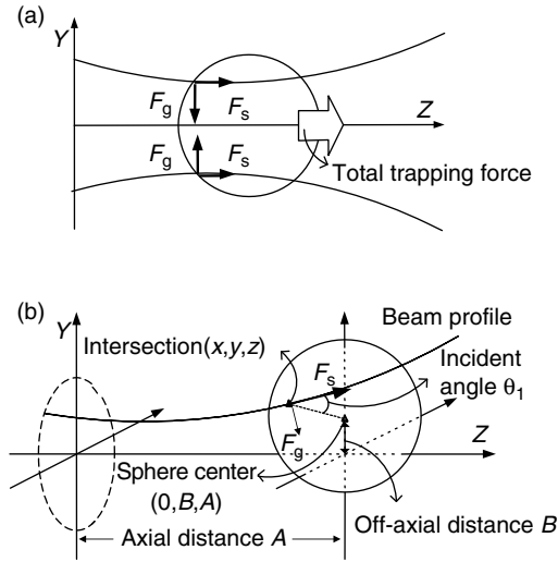
Fig. 3.19. Geometry for calculating trapping efficiency for a microsphere when focus is located on optical axis (a), and at off-axis (b)
