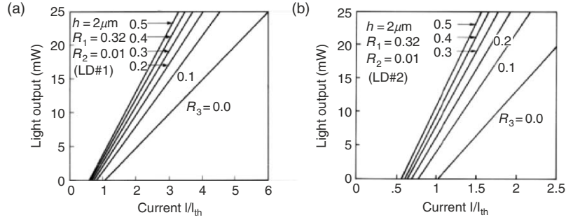
Fig. 2.36. OSL head light output characteristics with the medium reflectivity R_3 as a parameter for (a) an LD#1 ( \lambda = 1.3\mu\text{m} ), (b) an LD#2 ( \lambda = 0.83\mu\text{m} )
