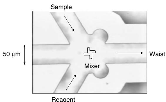
Fig. 4.65. Concept of an optical mixer for use in future \mu -TAS. The integrated system will have components such as inlets, fluidic channels with a mixing chamber, a detector (not shown) and outlets
