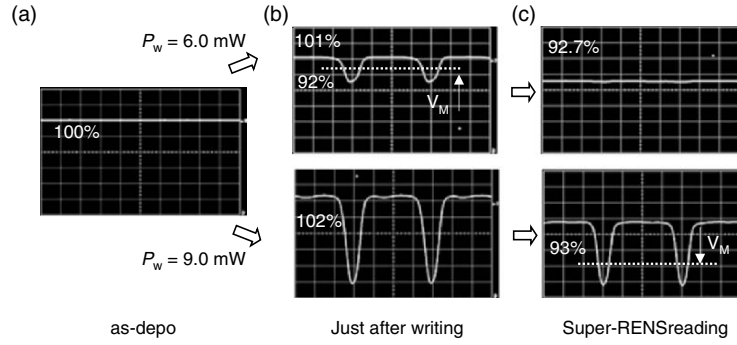
Fig. 5.46. Typical signal levels for (a) as-depo state (no mark, P_r = 1.5 mW), (b) just after writing ( P_r = 1.5 mW), and (c) super-RENS readings at write powers of P_w = 6.0 mW and P_w = 9.0 mW
