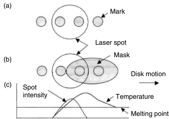
Fig. 5.34. Principle of superresolution readout through crescent-shaped aperture thermally formed in mask layer. Conventional readout (a), superresolution readout (b), and spot intensity profile and temperature distribution in a mask layer (c). Reprinted from [5.36] with permission by A. Fukumoto
