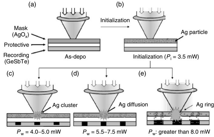
Fig. 5.58. Proposed working mechanism of super-RENS using \text{AgO}_x mask layer
