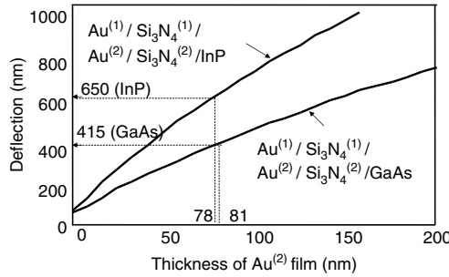
Fig. 2.55. Deflection of bimorph MCs with antireflection coating, \text{Au}^{(2)} thickness as a parameter
