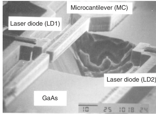
Fig. 2.23. Scanning electron microscope view of the main parts of the tunable LD. The released GaAs/AlGaAs microcantilever (MC) was fabricated by undercutting the sacrificial GaAs. The MC length, thickness and width are 110, 3, and 5 \mu\text{m} and the distances from the facet of LD1 to the side wall of the MC and LD2 to MC are 3 and 30 \mu\text{m} , respectively. Courtesy of O. Ohguchi, NTT, Japan
