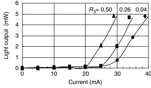
Fig. 2.13. I - L characteristics with an external mirror at the light-output maxima, with external mirror reflectivity R_3 as a parameter, where R_1 = 0.32 and R_2 = 0.01
