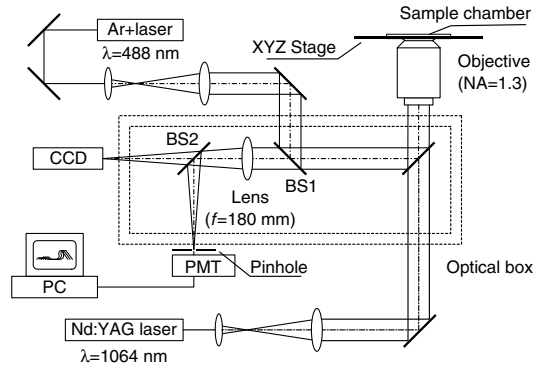
Fig. 5.21. Experimental setup of SNOM using an optically trapped gold particle. An Nd:YAG laser is used for trapping, and an \text{Ar}^+ laser is used for illuminating the gold particle. All the optical elements except mirrors to guide the lasers are installed inside the small optical box ( white box in Fig. 5.22a) for easy operation
