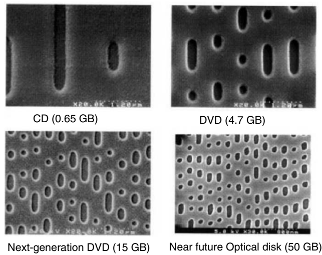
Fig. 5.33. Optical disk pit size comparison between CD, DVD, next-generation DVD and near-future optical disk. Courtesy of S. Sugiura, Pioneer Co., Japan
