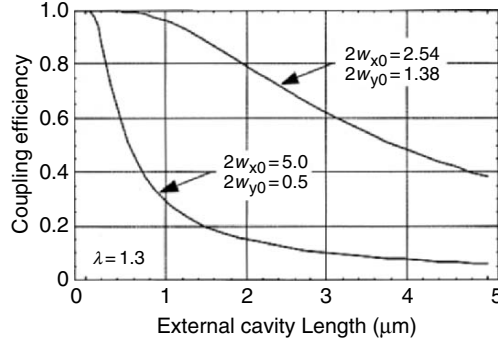
Fig. 2.3. Dependence of coupling efficiency \eta on external-cavity-length L_{\text{ex}}
