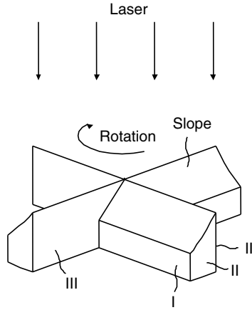
Fig. 4.18. Shuttlecock rotor with slopes on the top surfaces
