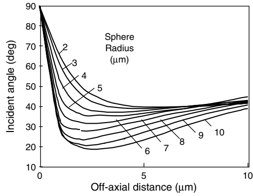
Fig. 3.24. Relationship between optimum fiber incident angle and radius of microsphere for F_{sz} = F_{gz} at maximum F_g on off-axis position
