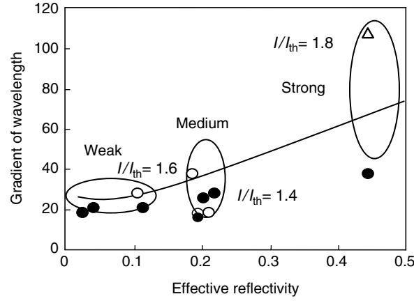
Fig. 2.19. Relationship between the gradient of wavelength variation and the effective reflectivity R_2^{\text{eff}}
