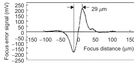
Fig. 5.16. Focus error signal representing typical S-shape curve of optical head
