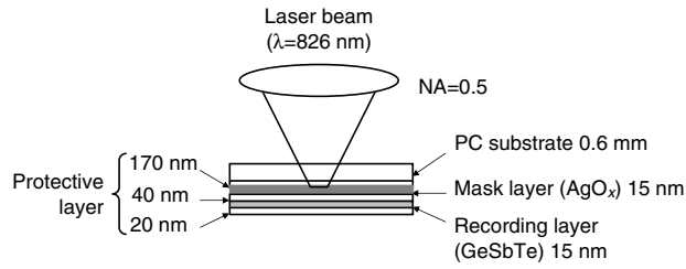
Fig. 5.49. Configuration for super-RENS optical disk using \text{AgO}_x mask layer
