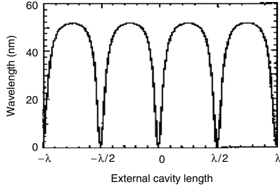
Fig. 2.7. Wavelength variation due to the external cavity length. Total wavelength tuning depends on effects of both mode change and carrier density change
