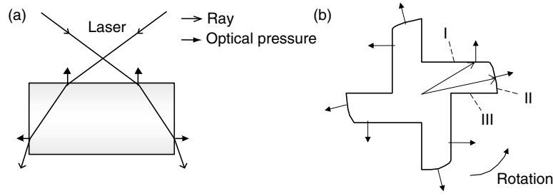
Fig. 4.3. Optical pressure force exerted on the light-incident upper surface lifts the rotor (a), and that exerted on the light-emission side surfaces rotates it (b)
