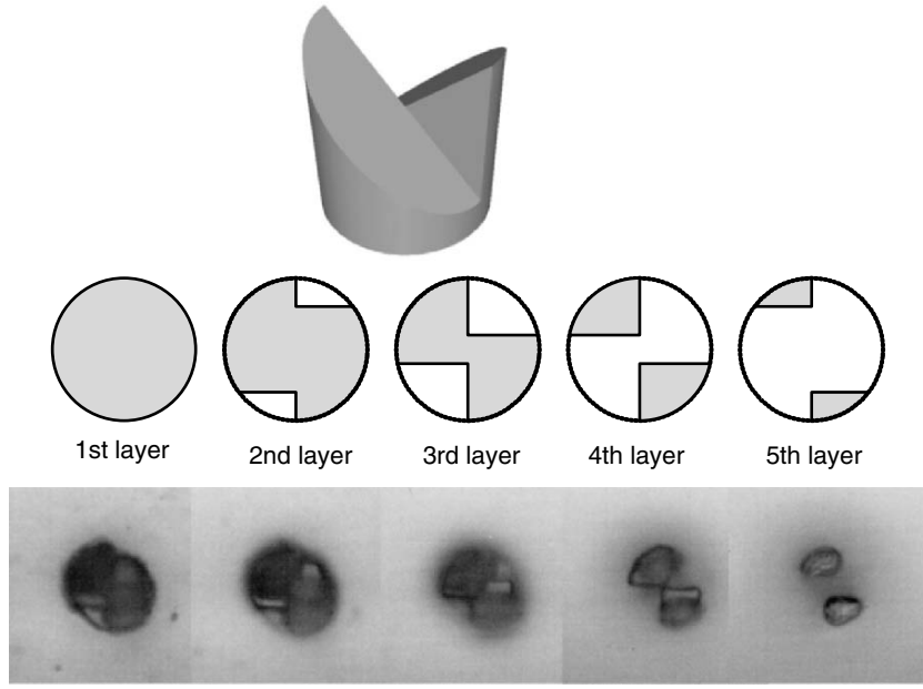
Fig. 4.46. Microstructures with slopes are fabricated by stacking of thin resin layers having the 2-D cross-sectional shape, upper : 3-D designed shape, middle : 2-D cross-sections designed, and lower : fabricated 2-D cross-sectional-shape layers of 5\mu\text{m} thick each
