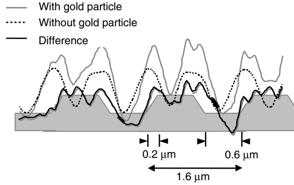
Fig. 5.32. Relationship between scattered light intensity and disk groove profile with and without gold particle
