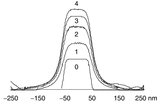
Fig. 5.8. Numerical results for the calculation of E_x , round-trip number as a parameter
