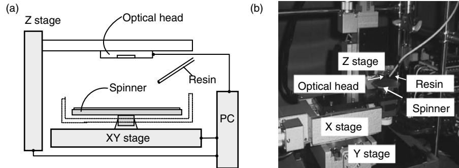
Fig. 4.44. Schematic diagram (a), and photograph (b) of the spinner-type microphotoforming apparatus
