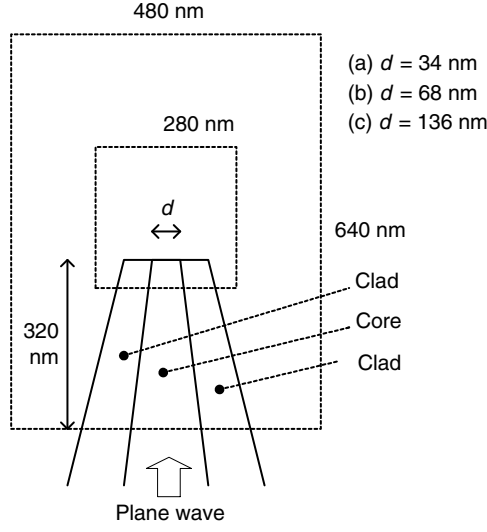
Fig. 5.9. 2-D Cartesian computational domain of 480 \text{ nm} \times 640 \text{ nm} for calculation of E_x around tapered fiber end with silica core and perfect conductor clad. Here, the refractive index and electrical permittivity of silica are 1.46 and 2.25\epsilon_r , ( \epsilon_r : free-space permittivity), respectively
