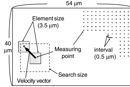
Fig. 4.55. Analytical model used to obtain velocity vectors and measuring points in horizontal plane
