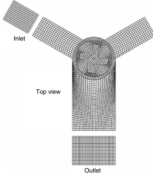
Fig. 4.36. Grid system of Y-shaped microchannel (inlet: 15\mu\text{m} width and 20\mu\text{m} depth, outlet: 30\mu\text{m} width and 20\mu\text{m} depth) and optical rotor ( d = 20\mu\text{m} , w = 4\mu\text{m} , t = 10\mu\text{m} ) [4.13]. Courtesy of Y. Ogami, Ritsumeikan University, Japan
