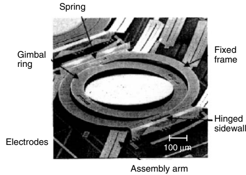
Fig. 1.19. Surface-micromachined beam-steering micromirror [1.7] ©2003 IEEE
