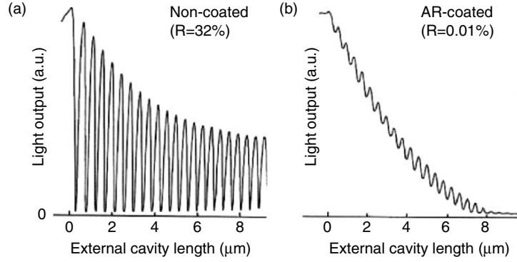
Fig. 2.40. Light output of a composite cavity LD as a function of external-cavity-length L_{\text{ex}} . Light output varies by a half-wavelength period as L_{\text{ex}} varies (a). Variation can be suppressed by an antireflection coating on the LD facet facing the recording medium (b)
