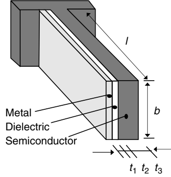
Fig. 2.46. Schematic drawing of a three-layer bimorph MC
