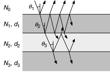
Fig. 2.50. Reflection and transmission of a plane wave in a two-layer film structure
