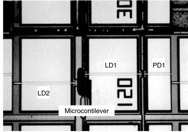
Fig. 2.24. Photograph of a resonant sensor with a MC driven photothermally from one side by LD2 and sensed optically from the other side by LD1 and photodiode (PD1); LD2, MC, LD1, and PD1 are integrated on a GaAs substrate
