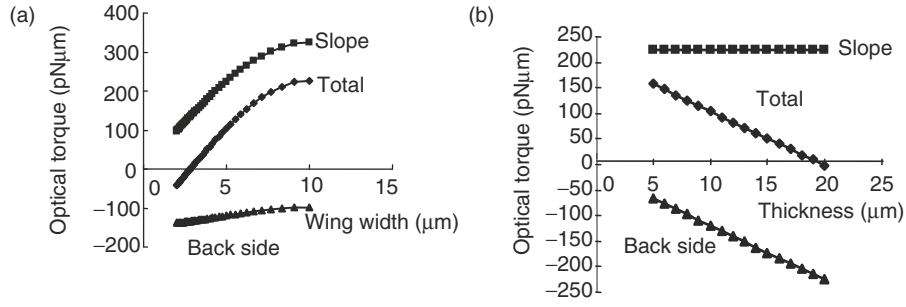
Fig. 4.21. Simulated optical torque dependence on the wing width (a), and on the thickness (b) of the shuttlecock rotor with slopes
