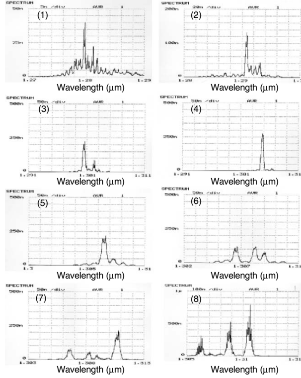
Fig. 2.17. Spectra at (1), (2), . . . , and (8) in Fig. 2.16
