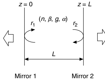
Fig. 2.1. A laser diode (LD) consists of an active region of (n, \beta, g, \alpha) and two mirrors with reflectivities of R_1 and R_2 separated at the length of L , where n is the refractive index, \beta is the propagation constant, g is the gain and \alpha is the extinction coefficient
