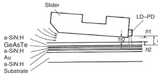
Fig. 1.32. A flying optical head with a laser diode. The optical head consists of a monolithically integrated laser diode (LD) and a photodiode (PD) attached to the slider
