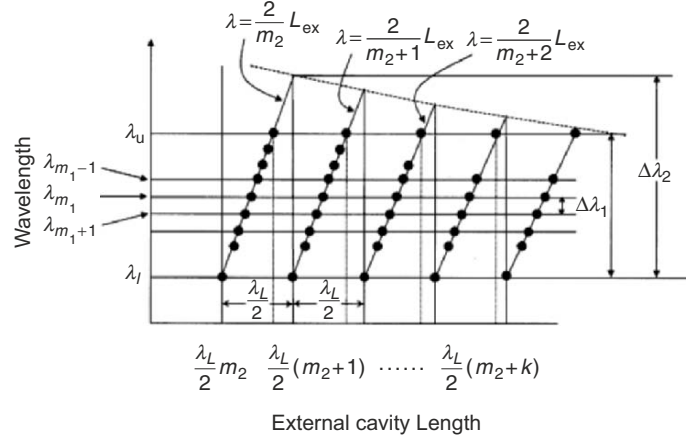
Fig. 2.6. Relationship between the wavelength and the external cavity length. The \lambda_u and \lambda_l on the vertical axis show the gain spectrum range and the \lambda_L/2 on the horizontal axis shows the half-wavelength interval
