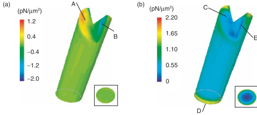
Fig. 4.32. 3-D images of the pressure distribution (a), and the shearing stress distribution (b), for cylindrical rotor of a = 45^\circ , 2r = 3\mu\text{m} and h = 10\mu\text{m} at P = 100\text{ mW}
