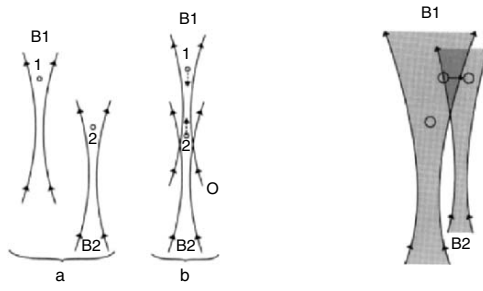
Fig. 3.3. Transfer of optically trapped particle from beam to beam
