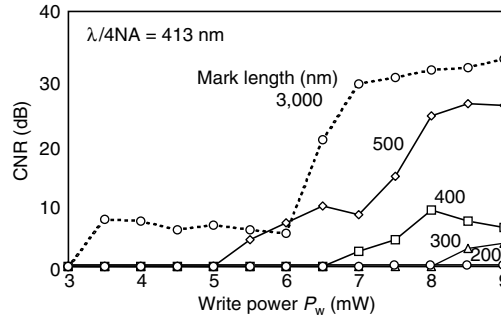
Fig. 5.45. Write power dependence of CNR measured for readout #2
