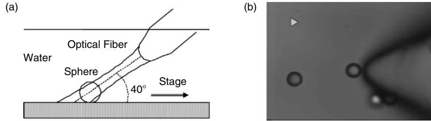
Fig. 3.36. Trapping performance by solitary optical fiber inserted at angle of 40°
