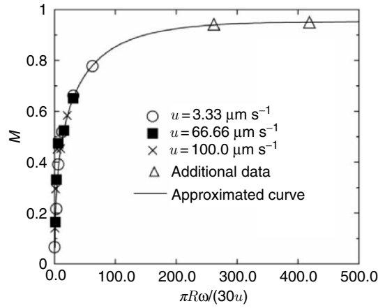
Fig. 4.38. Similarity of mixing rate M at D = 0 , where R is the radius of the rotor [4.13]. Courtesy of Y. Ogami, Ritsumeikan University, Japan
