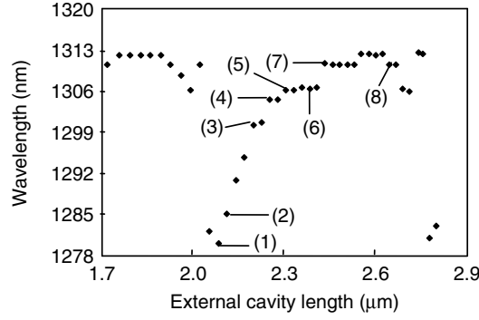
Fig. 2.16. Dependence of wavelength on external cavity length, where drive current I/I_{th} = 1.6 , reflectivities R_1 = 0.32 , R_2 = 0.01 , and R_3 = 0.5
