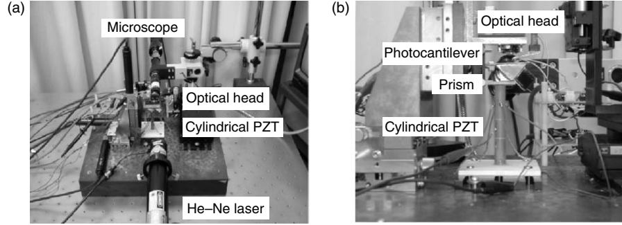
Fig. 5.14. Photograph of AFM/SNOM setup mounted on a vibration-damped table
