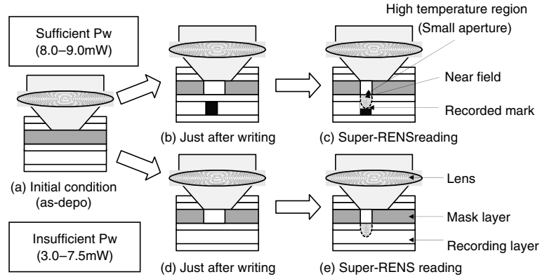
Fig. 5.47. Working mechanism for aperture-type super-RENS disk obtained from experimental results. The disk moves from right to left
