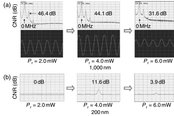
Fig. 5.57. Read power dependence on signal amplitude and spectrum for mark lengths of 1,000 nm with 10 \text{ dB div}^{-1} and 1 \text{ MHz div}^{-1} (a), and 200 nm with 10 \text{ dB div}^{-1} and 10 \text{ kHz div}^{-1} (b), with read power P_r as parameter
