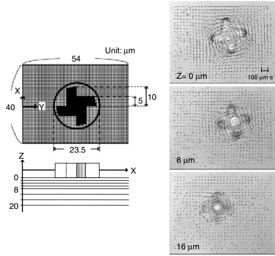
Fig. 4.57. Velocity vectors around optical mixer at different depths for horizontal rotation
