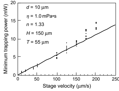
Fig. 3.31. Dependence of minimum transverse trapping power on the velocity for d = 10\mu\text{m} polystyrene particle
