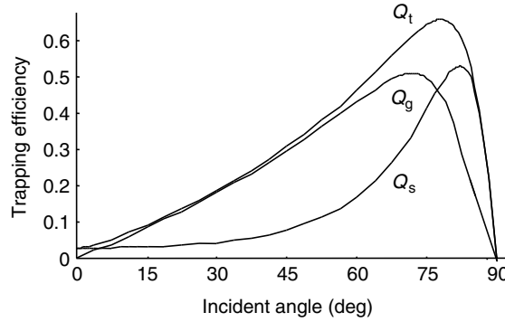
Fig. 3.10. Predicted trapping efficiency dependence on incidence angle \theta_1 for Q_s , Q_g and Q_t .
