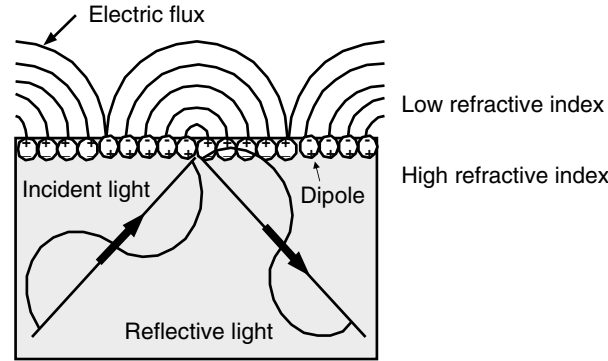
Fig. 5.2. Sketch of the near field produced at the low-refraction medium surface as the electric flux generated by dipoles due to the attenuated total reflection of light
