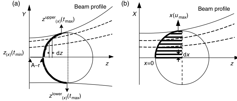
Fig. 3.20. Method of optical pressure integration when a sphere is located at an off-axis, side view (a), and top view (b)
