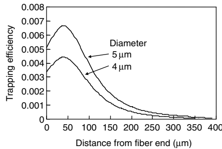
Fig. 3.18. Axial trapping efficiency dependence on distance from optical fiber end of polystyrene sphere
