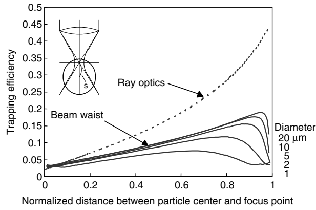
Fig. 3.15. Axial trapping efficiency of polystyrene microsphere suspended in water by converging ray approximations of straight line (ray optics) and parabolic line (beam waist) with beam waist \omega_0
