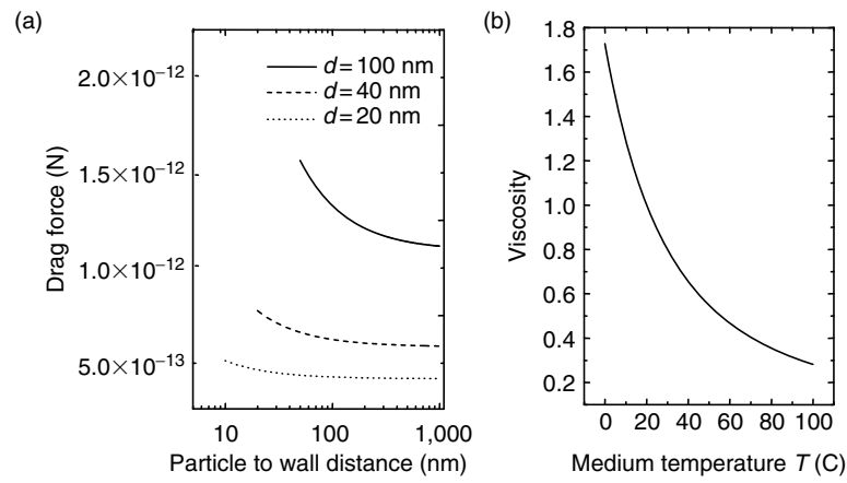
Fig. A.17. Drag force dependence on diameter of microsphere moving at constant speed of v in water (a), and viscosity dependence on temperature of medium (b)
