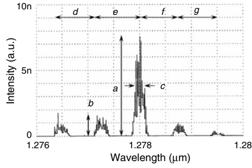
Fig. 2.20. Definitions of side-mode suppression ratio 10 \log(a/b) , spectrum line width (full width half-maximum c ) and mode interval (average of d, e, f , and g in this figure)
