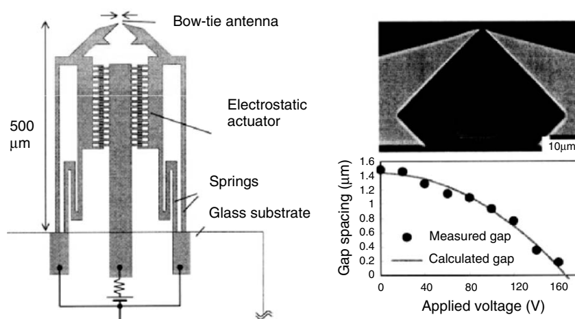
Fig. 1.23. A bow-tie probe with an actuator driven by electrostatic force is fabricated to provide a narrow gap that enhances the intensity of the near field. Reprinted from [1.46] with permission by M. Esashi, Tohoku University, Japan
