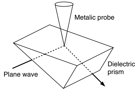
Fig. A.16. 3-D configuration of system for calculation of scattered light by sharpened metal probe [5.20]
