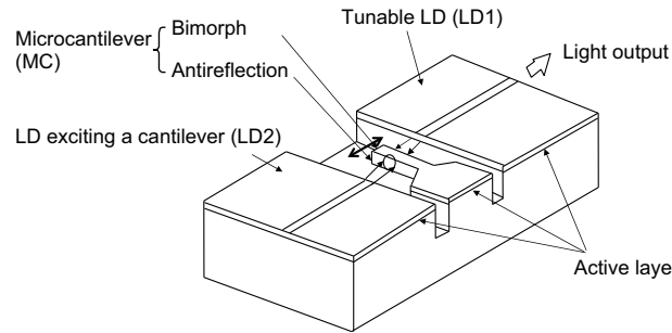
Fig. 1.28. Edge-emitting laser diodes (LDs) with a microcantilever (MC). The microcantilever is driven photothermally by one laser diode (LD2) to adjust the output wavelength from the other laser diode (LD1)
