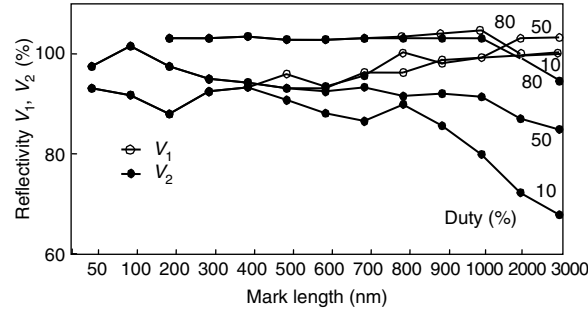
Fig. 5.59. Relationships between reflectivity V_1 (non-mark), V_2 (mark), and mark length for super-RENS readout ( P_r = 4 \text{ mW} ), with optical pulse duty as parameter
