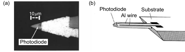
Fig. 5.13. Photograph of photocantilever, in which top photodiode (PD) is fabricated (a), and sketch of that (b)
