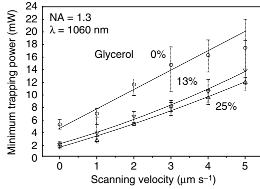
Fig. 5.24. Dependence of minimum trapping power on scanning velocity of optically trapped gold particle at different viscosities
