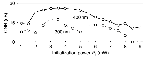
Fig. 5.52. Relationship between CNR of super-RENS readout ( P_r = 4 \text{ mW} ) and initialization laser power P_i , with mark length as parameter
