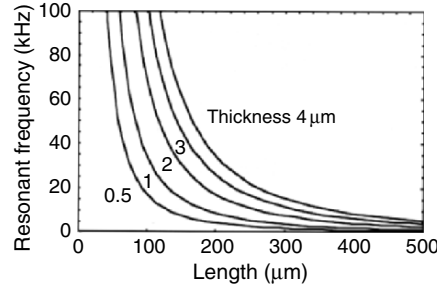
Fig. A.1. Relationship between the cantilever resonant frequency f_0 and the length l , with thickness t as a parameter
