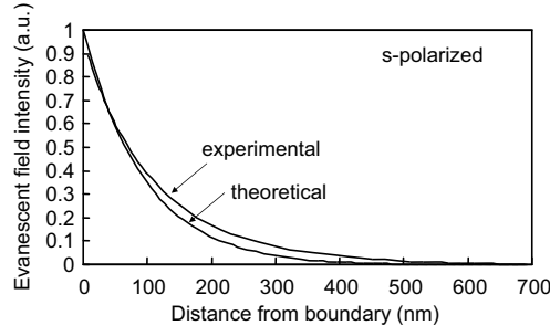
Fig. 5.19. Dependence of measured evanescent field intensity on distance from boundary. Theoretical result is also shown for reference
