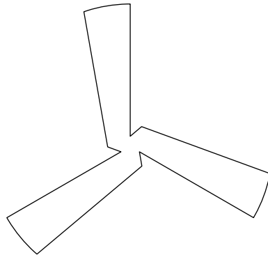
Fig. A.9. Improved shape of the three-wing shuttlecock rotor with \beta = 130^\circ and \alpha_2 = 100^\circ for the rotor of n_2 = 1.6 , d = 20 \mu\text{m} , t = 10 \mu\text{m} , w = 5 \mu\text{m} , and medium n_1 = 1.33
