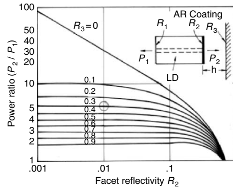
Fig. A.3. Relationships between the power ratio and the medium side LD facet reflectivity R_2 for R_1 = 0.7 with h = 2\mu\text{m} , medium reflectivity R_3 as a parameter.
