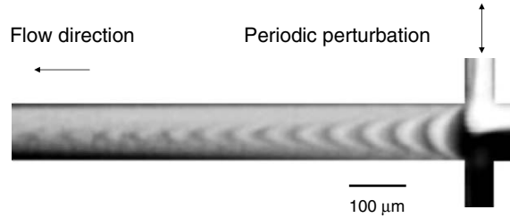
Fig. 4.64. Chaotic mixing by using the mechanical micromixer [4.22]. Courtesy of Y.K. Lee, University of California, USA
