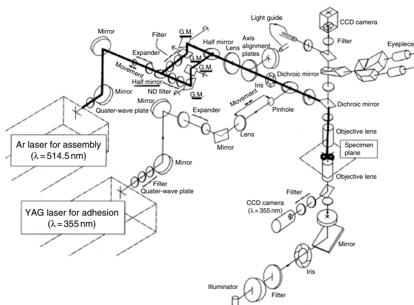
Fig. 3.45. Micro assembly system using two laser beams, one is for trapping (assembly) and the other is for ablation (adhesion).
