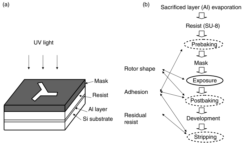
Fig. 4.41. Optical rotor fabrication by photolithography
