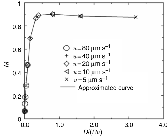
Fig. 4.39. Similarity of mixing rate M at \omega = 0 [4.13] Courtesy of Y. Ogami, Ritsumeikan University, Japan
