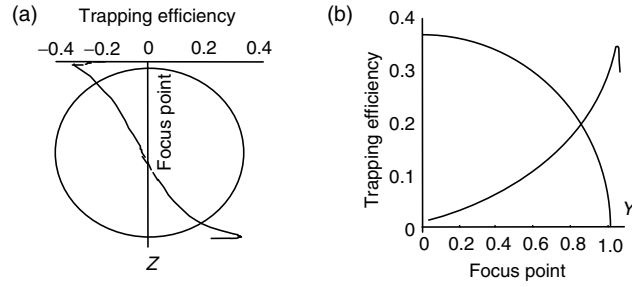
Fig. 3.13. Total trapping efficiency Q_t exerted on a polystyrene microsphere suspended in water by trap with a uniformly filled input aperture of NA = 1.25 for axial (a), and for transversal (b) directions
