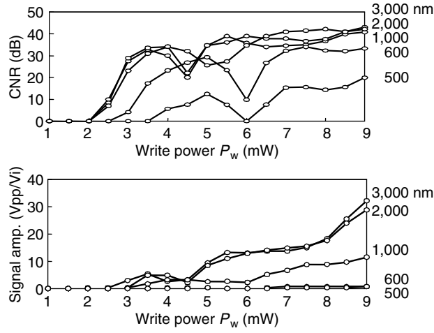
Fig. 5.54. Relationship between CNR, V_{pp}/V_i and write power P_w for read power of P_r = 1 mW, with mark length as parameter
