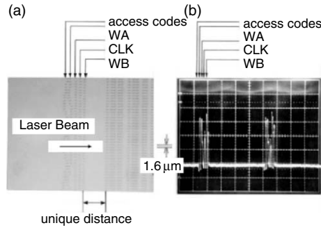
Fig. 2.37. Discrete block format (DBF) marks with a 1.6- \mu\text{m} track-pitch (a), and reproduced signals at 900 rpm. LD bias current is 40 mA (b)
