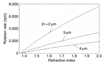
Fig. A.11. Rotation rate dependence on refractive index of cylindrical optical rotor with slope angle of 45^\circ
