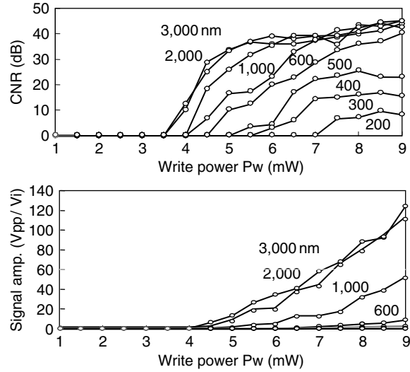
Fig. 5.55. Relationship between CNR, V_{pp}/V_i and write power P_w for read power of P_r = 4 mW (super-RENS readout), with mark length as parameter
