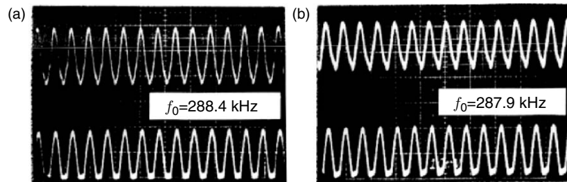
Fig. 2.31. Resonant frequency change of 500 Hz from 288.4 to 287.9 kHz, due to the mass increase of 54 ng for the 1- \mu\text{m} thick phthalocyanine deposition
