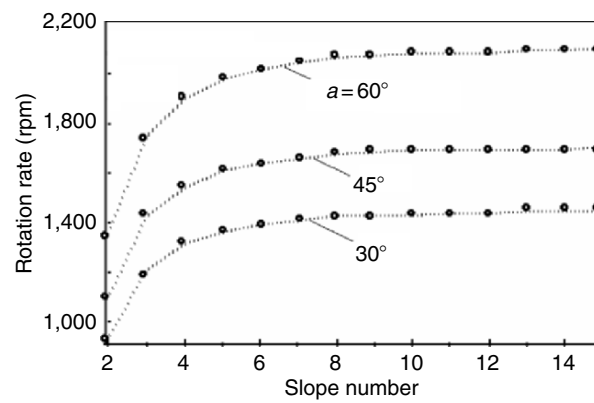
Fig. A.13. Rotation rate and number of slopes of the cylindrical rotor with slope angle of a = 30^\circ , 45^\circ , and 60^\circ
