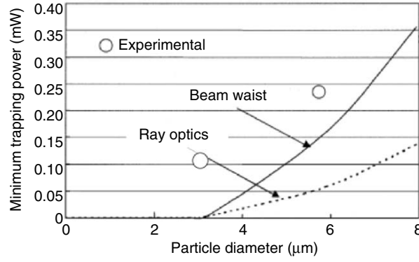
Fig. 3.29. Minimum axial trapping power for polystyrene sphere comparing the experimental measurement with the predicted results for straight ray (ray optics) and parabolic ray (beam waist) optics
