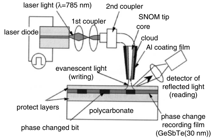
Fig. 5.37. SNOM-based storage using Al-coated fiber probe and phase change medium (GeSbTe). Reprinted from [5.40] with permission by S. Hosaka, Gunma University, Japan
