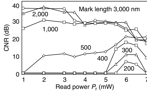
Fig. 5.43. Read power dependence of CNR for various mark lengths written at power of 7.0 mW for medium velocity of 1.9 \text{ m s}^{-1}
