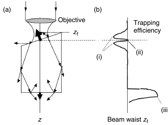
Fig. 4.9. Ray tracing for the rotor illuminated with a focused beam (a), and trapping efficiency along the light beam axis (b)
