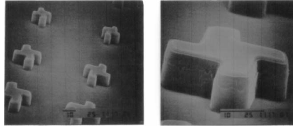
Fig. 4.2. Fabricated shuttlecock optical rotors with shape dissymmetry on their sides
