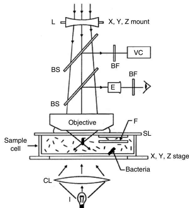
Fig. 3.39. Example of bacterial manipulation and measurement of swimming speed of mitochondria by optical tweezers [3.23]
