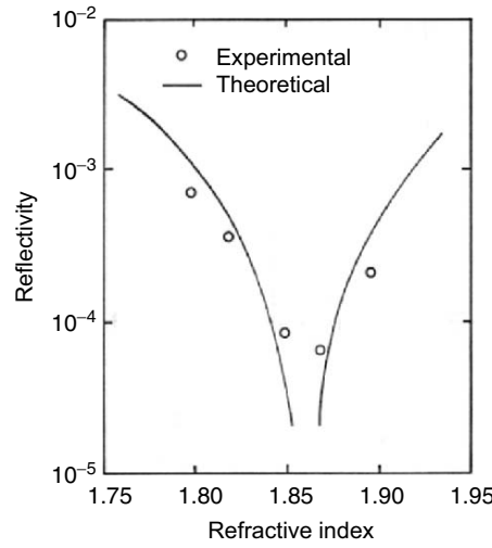
Fig. 2.39. Relationship between antireflection-coated (ARC) facet reflectivity and ARC-film refractive index. Circles show experimental results. Solid lines are fitting curves calculated using a plane wave approximation
