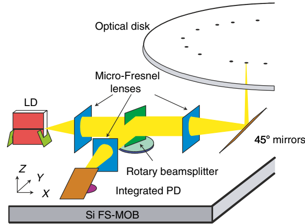
Fig. 1.22. A free-space optical pickup head integrated by surface micromachining [1.20]. Courtesy of Ming Wu, University of California, USA
