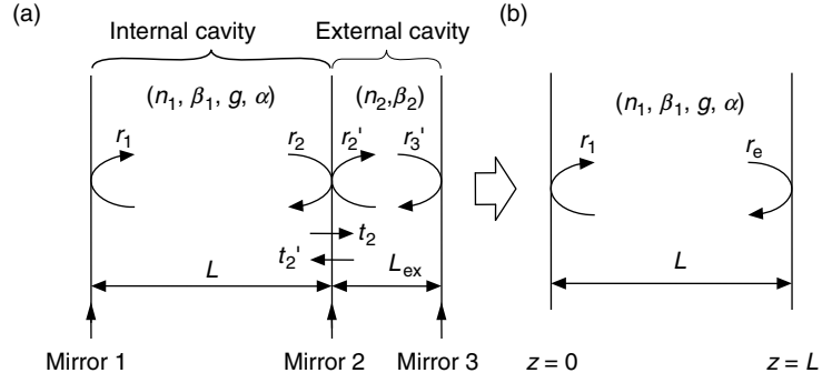
Fig. 2.2. Extremely short-external-cavity LD (ESEC LD) system which consists of the LD facet reflectivities R_1, R_2 , and the external mirror reflectivity R_3 (a), and introduced effective reflectivity R_2^{\text{eff}} instead of R_2 and R_3 (b). We can analyze the behavior of the ESEC LD by analyzing the solitary LD with a resonator composed of R_1 and R_2^{\text{eff}}
