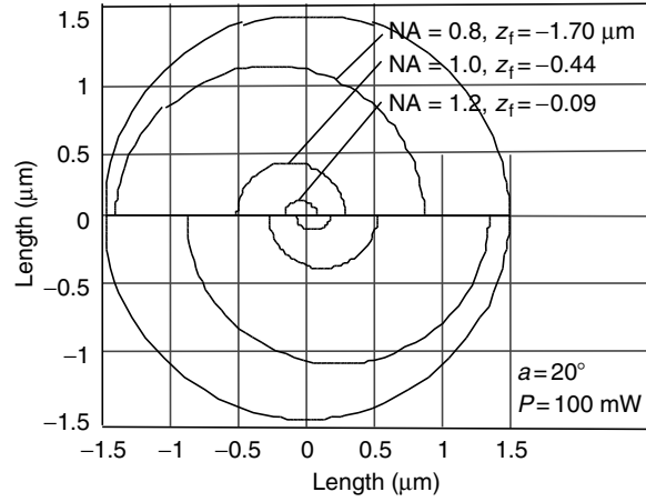
Fig. 4.13. Illuminated region on the upper surface of an a = 20^\circ slope for several NAs. The radius of the illuminated region decreases as NA increases
