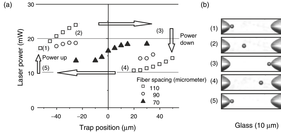
Fig. 3.35. Particle behavior when left power increases for different spacings between fiber lens
