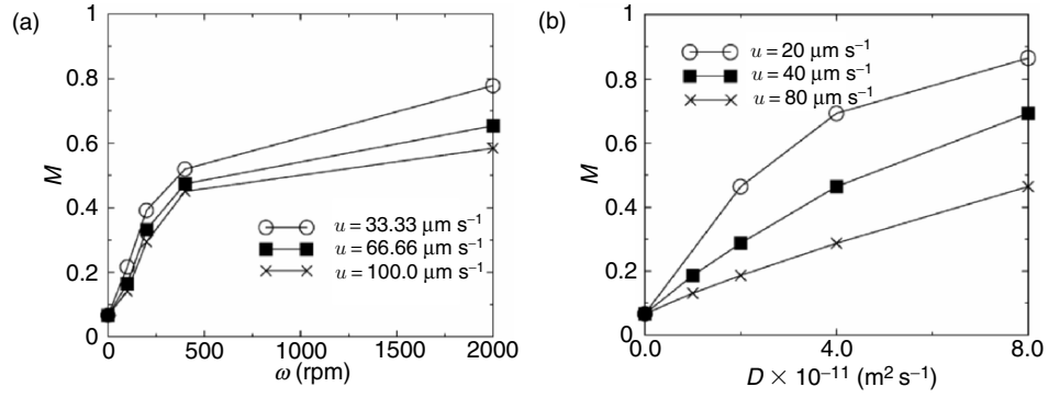
Fig. 4.37. Mixing rate M at various rotation rates \omega and fluid velocities u with D = 0 (a), and M at various diffusion coefficients D and fluid velocities u with \omega = 0 (b) [4.13]
