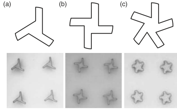
Fig. 4.40. Variation of the shuttlecock wing number for considering the stability, rotation rate and agitation in the medium
