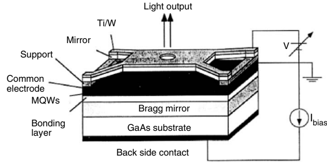
Fig. 1.27. A surface-emitting laser diode with a thin film mirror. A laser driver supplies current for light emission, and the bias applied moves the thin film mirror in the adjustment of the output wavelength [1.16]
