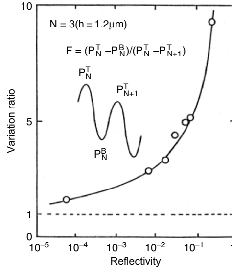
Fig. 2.41. Variation ratio versus facet reflectivity at the optimum bias current for OSL readout operation
