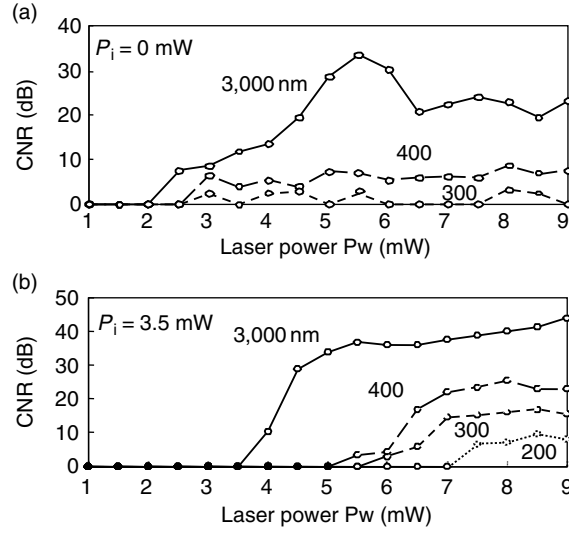
Fig. 5.53. Effect of initialization on CNR for super-RENS readout ( P_r = 4 mW), with write power P_w as parameter
