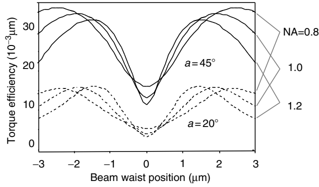
Fig. 4.12. Torque efficiency Q_{\text{torque}} vs beam waist position for the slope angle of a = 20^\circ and 45^\circ with numerical aperture NA as a parameter
