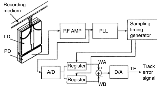
Fig. 2.38. Block diagram of track error signal detection. Track error signal is obtained by the signal amplitude difference between the two wobbling signals of the discrete block format (DBF)
