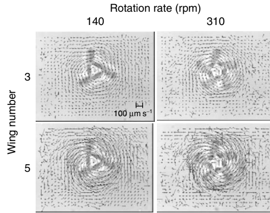
Fig. 4.61. Velocity vectors for rotors with different numbers of wings, with rotation rate as a parameter
