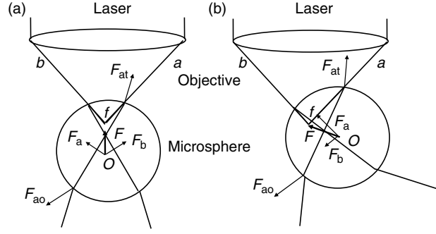
Fig. 3.8. Qualitative description of optical trap. The microsphere is transparent and its refractive index is slightly higher than that of the surrounding medium [3.4]
