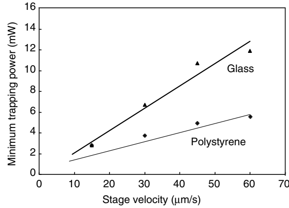
Fig. 3.37. Relationship between minimum trapping power obtained using solitary optical fiber and stage velocity for microsheres of 10 micrometer in diameter
