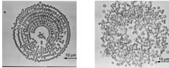
Fig. 3.5. Micrometer-size particle formation due to light intensity formed by interference fringe pattern [3.6]. Courtesy of H. Masuhara, Osaka University, Japan
