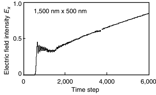
Fig. 5.7. Relationship between electric field E_x and time steps of FDTD
