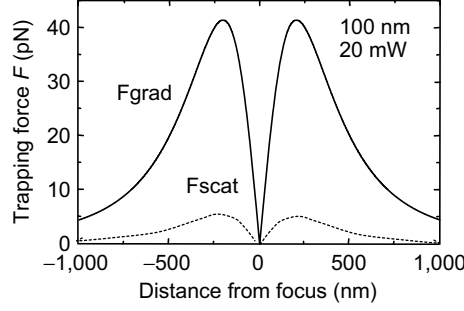
Fig. 5.23. Calculated gradient force F_{\text{grad}} in transverse direction and in axial direction for gold particle with refractive index n_2 = 0.272 + i7.07 , diameter 100 nm, medium refractive index n_1 = 1.33 , objective lens NA = 1.3, and Gaussian laser power 20 mW
