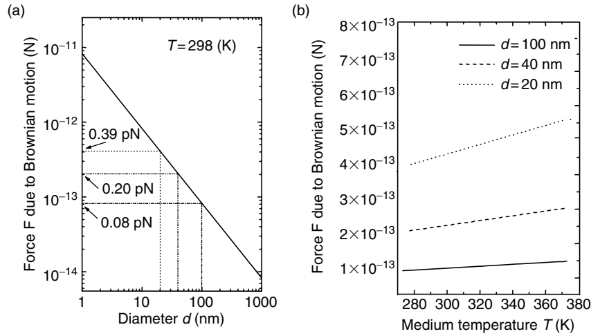
Fig. A.15. Relationships between force due to Brownian motion and diameter of microsphere (a) , and temperature of medium (b)
