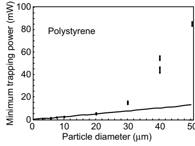
Fig. 3.32. Dependence of minimum transverse trapping power on diameter of polystyrene microspheres
