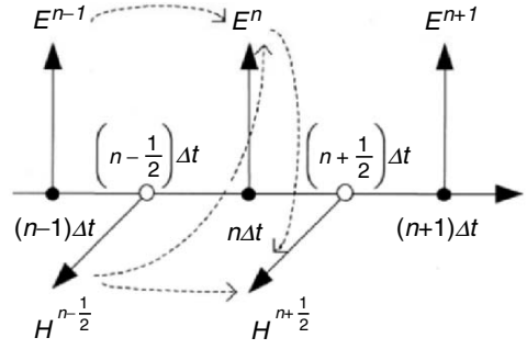
Fig. 5.3. Space-time chart of Yee algorithm in one dimension showing the use of central differences for space derivatives and leapfrog for time derivatives [5.15]
