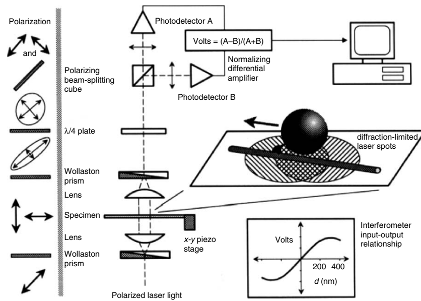
Fig. 3.41. Direct observation of kinesin stepping by optical trapping interferometry [3.25]
