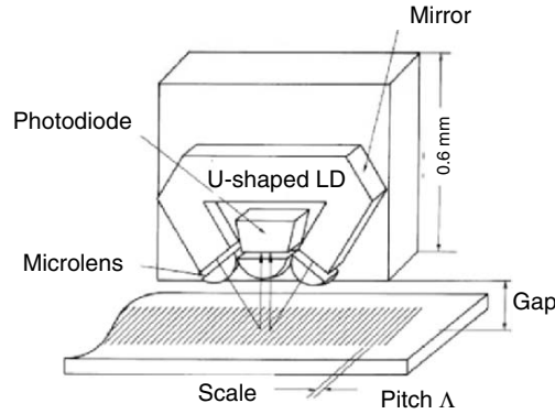
Fig. 1.30. Schematic drawing of an optical encoder consisting of a photodiode (PD), a U-shaped laser diode (LD), and microlenses [1.68]
