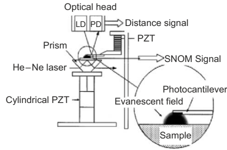
Fig. 5.15. Sketch of experimental setup. Distance signal is used for measuring surface profile and SNOM signal is used for observing surface property by detecting the scattered light from the evanescent field
