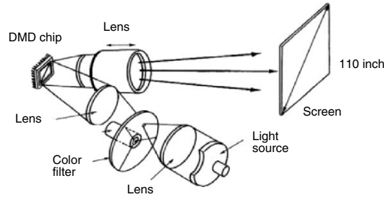
Fig. 1.18. Optical layout of a projector using a DMD [1.5]. Courtesy of Larry J. Hornbeck, Texas Instruments, USA ©1993 IEEE
