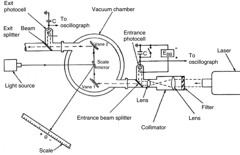
Fig. 3.2. Top view of two-vane torsion pendulum for measuring optical pressure force. Reprinted from [3.1] with permission by American Institute of Physics, Copyright Clearance Center License Number: 1273781240969
