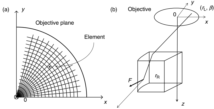
Fig. 4.5. Ray optics to simulate the optical torque of the shuttlecock rotor, where ray incidence (r_L, \beta) on the lens aperture is considered and the torque is estimated at the point r_R on side surface I
