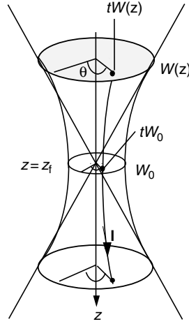
Fig. 4.10. Ray optics model for a focused laser beam considering beam waist. The ray of tW(z) passes tW_0 at the beam waist ( z = z_f ) where 0 \leq t \leq 1
