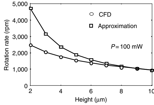
Fig. 4.34. Rotation rate obtained by CFD and approximation with parallel beam illumination at P = 100 mW, a = 45^\circ , 2r = 3\mu\text{m} with rotor height as a parameter
