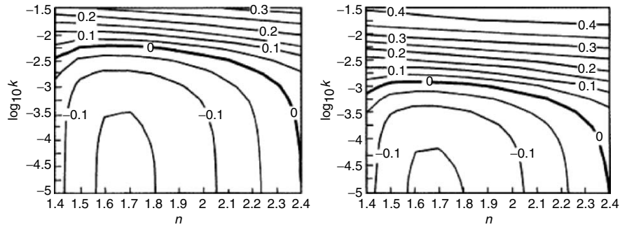
Fig. 3.44. Relationship between optical constant and maximum trapping efficiency Q_{\max} for microsphere with wavelength of 633 nm [3.35]
