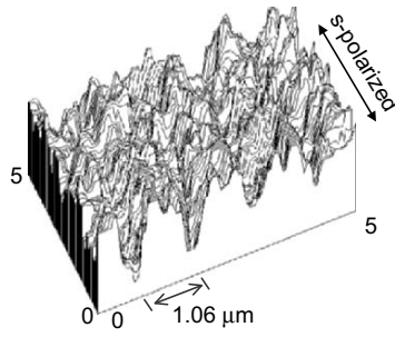
Fig. 5.28. SNOM images (scattered light intensity) of refractive index grating by gold particle probe with s-polarized illumination
