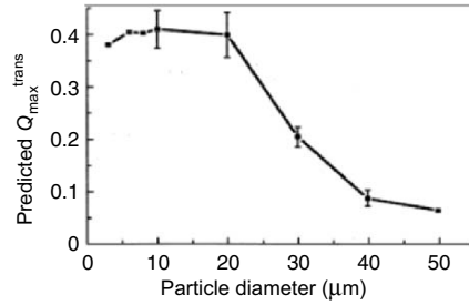
Fig. A.5. Dependence of predicted Q_{\max}^{\text{trans}} on sphere diameter for polystyrene, which is derived from experimental data of Fig. 3.32. Q_{\max}^{\text{trans}} decreases as diameter increases
