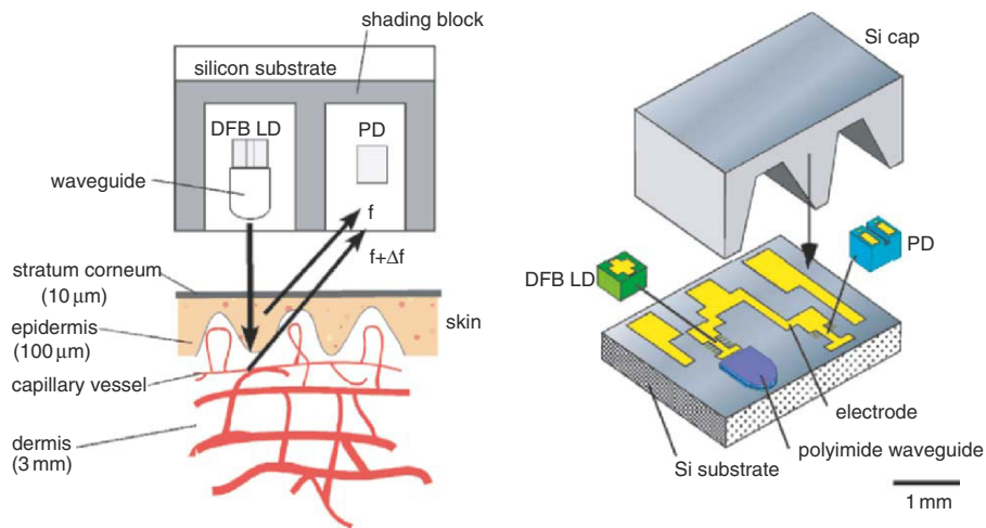
Fig. 1.34. The hybrid integrated structure of the blood flow sensor consists of an InGaAsP-InP distributed feedback laser diode (DFB-LD), a photodiode (PD) and a polyimide waveguide on a silicon (Si) substrate [1.70]. Courtesy of E. Higurashi, NTT, Japan
