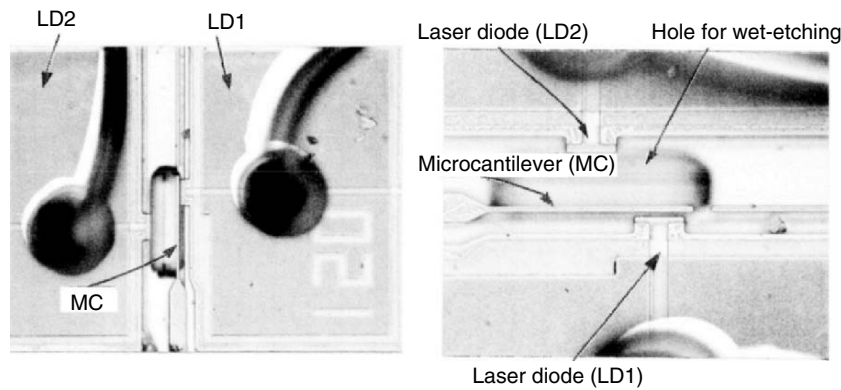
Fig. 2.30. Photograph of a resonant sensor deposited with chemically inductive material phthalocyanine of 1 \mu\text{m} thickness
