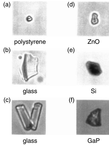
Fig. 4.1. Dissymmetrical/arbitrarily shaped broken microobjects which can be rotated but not controlled the rotational direction by optical pressure. They are a polystyrene (a), a broken glass (b), a glass rod (c), a ZnO (d), an Si (e), and a broken GaP (f)
