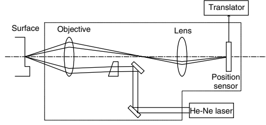
Fig. 2.11. Autofocusing geometry for investigating the attachment error L_{\text{ex}}^1 between an LD-PD facet and a slider surface
