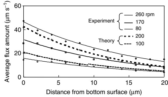
Fig. 4.58. Average flux amount at different depths
