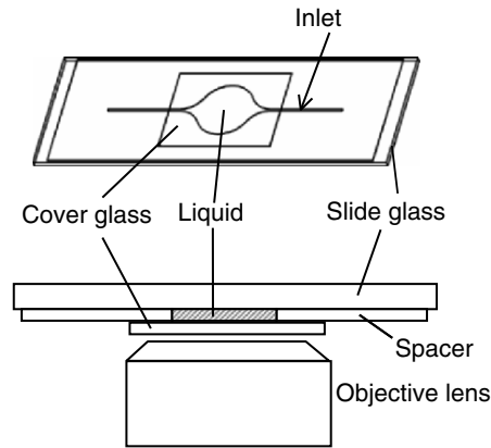
Fig. 4.49. Fabricated sample chamber sealed with cover glass. When liquid is dropped at the edge of the inlet it moves toward the center by surface tension
