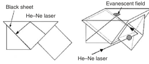
Fig. 5.17. Prism configuration consists of three corner prisms at 45^\circ
