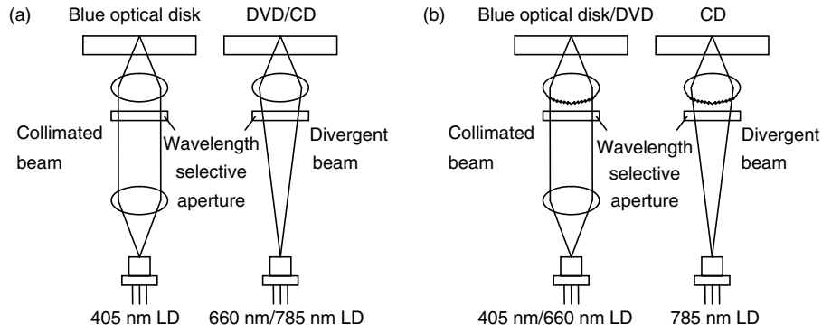
Fig. 1.21. Blue ray/DVD/CD compatible optical head technology. The compatibility principle is based on spherical aberration correction and objective NA control for each disk [1.45]. Courtesy of R. Katayama, NEC, Japan
