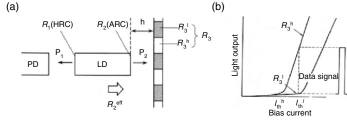
Fig. 2.35. LD used in an OSL flying head forms a complex cavity with the recording medium acting as an external mirror. (a) R_1 and R_2 are the power reflectivities of the LD facets, and R_3^h and R_3^l are those of the two states for the external recording medium. R_2^{\text{eff}} is the effective reflectivity coupled with the external recording medium. (b) Light output versus bias current in the two medium reflectivity states. There are two threshold currents: I_{\text{th}}^h for R_3^h and I_{\text{th}}^l for R_3^l . Data bits are read as the laser switches from R_3^l to R_3^h , biased between I_{\text{th}}^h and I_{\text{th}}^l , by the PD on the opposite side of the medium
