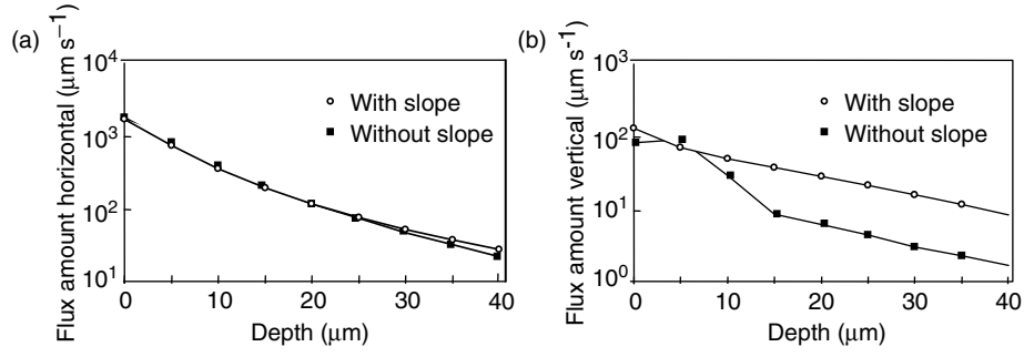
Fig. 4.26. Effect of the slope (angle of 45^\circ ) of the shuttlecock rotor on the flux amount. Horizontal (a), and vertical (b)
