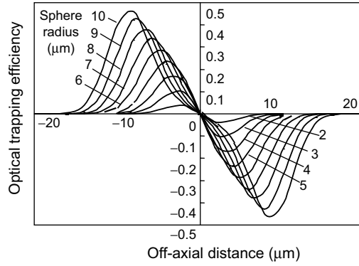
Fig. 3.22. Variation in transverse trapping efficiency at beam waist as function of off-axial distance, with microsphere radius as a parameter
