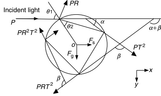
Fig. 3.9. Optical pressure force on microsphere exerted by single incident ray [3.4]
