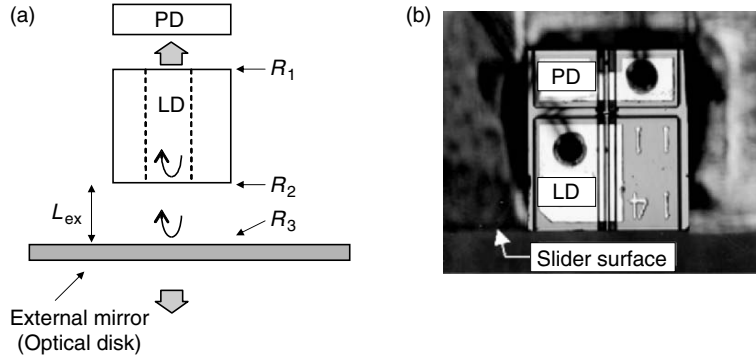
Fig. 2.9. Detailed representation of the ESEC LD system (a), and photograph of a monolithically integrated LD-PD chip on a slider (b)
