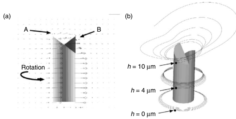
Fig. 4.31. Velocity vectors in the plane 0.5\mu\text{m} before the center plane for the rotor of a = 45^\circ , 2r = 3\mu\text{m} and h = 10\mu\text{m} (a), and streamlines around the rotor (b)
