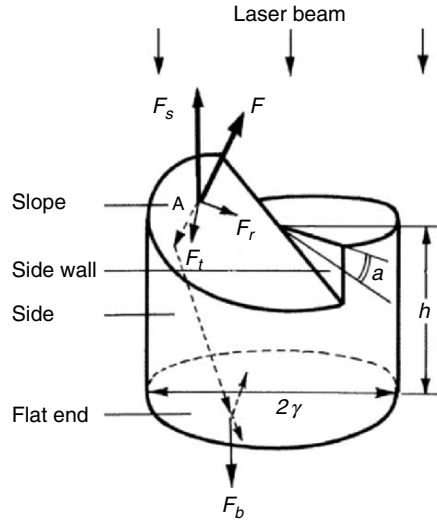
Fig. 4.4. Rotation principle by the optical pressure exerted on the slopes of the light-incident surface and the cylindrical body
