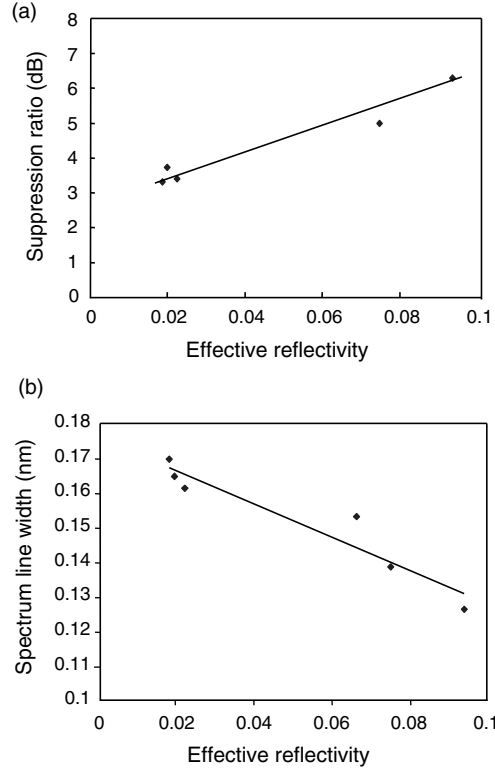
Fig. 2.22. Dependence of side-mode suppression ratio on R_2^{\text{eff}} (a), and dependence of spectrum line width on R_2^{\text{eff}} (b).
