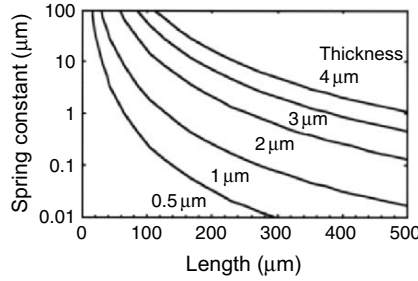
Fig. A.2. Relationship between the cantilever spring constant K and the length l , with thickness t as a parameter
