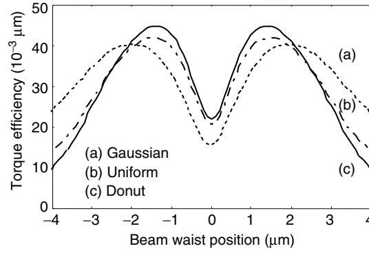
Fig. 4.16. Relationship between torque efficiency Q_{\text{torque}} and beam waist position z_f for different beam profiles
