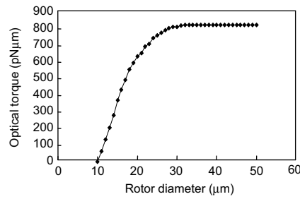
Fig. A.10. Optical torque dependence on diameter of rotor with four wings
