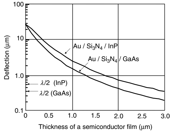
Fig. 2.48. Numerical simulation of the tip deflection versus semiconductor thickness by a temperature increase of 100°C for a metal-dielectric bimorph structure MC for two types of semiconductor materials
