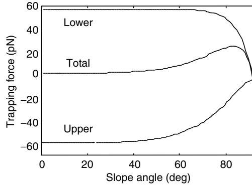
Fig. 4.7. Dependence of trapping forces on slope angle
