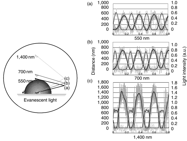
Fig. 5.18. Measured evanescent light intensity with cantilever amplitudes of 550 nm (a), 700 nm (b), and 1,400 nm (c)
