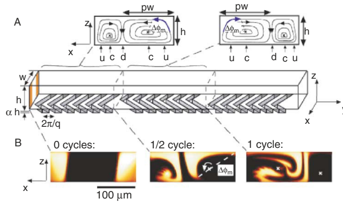
Fig. 4.63. Mixing by intersecting microchannels, which induces chaotic behavior of microflow [4.21]. Courtesy of A. Stroock, Cornell University, USA
