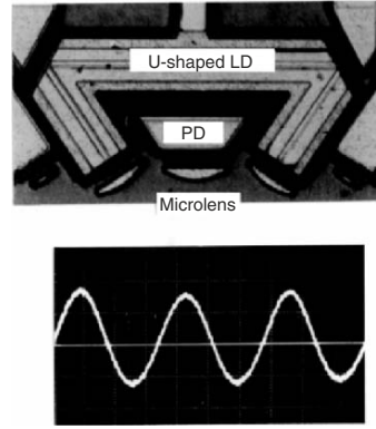
Fig. 1.31. Photograph of the optical encoder. Courtesy of R. Sawada, NTT, Japan
