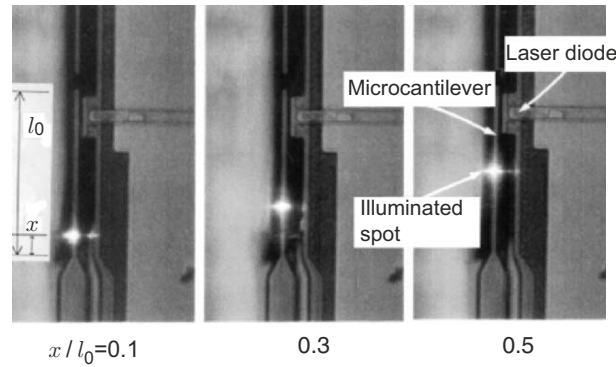
Fig. 2.27. Photograph of the illuminated spot on the MC, for investigating the excitation efficiency depending on the position of the MC
