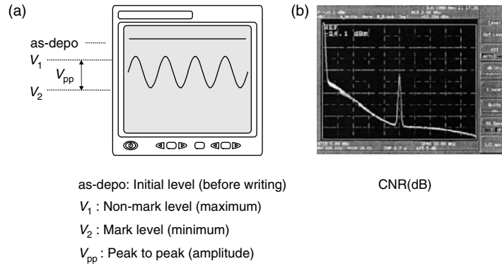
Fig. 5.42. Two measured signals; signal amplitude with oscilloscope (a) and CNR with spectrum analyzer (b)
