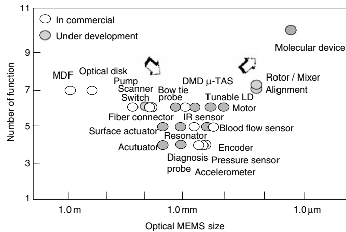
Fig. 1.35. Proposed and commercialized devices/systems fabricated using optical MEMS and micromechanical photonics. The horizontal axis is device/system size and the vertical axis is the number of functions
