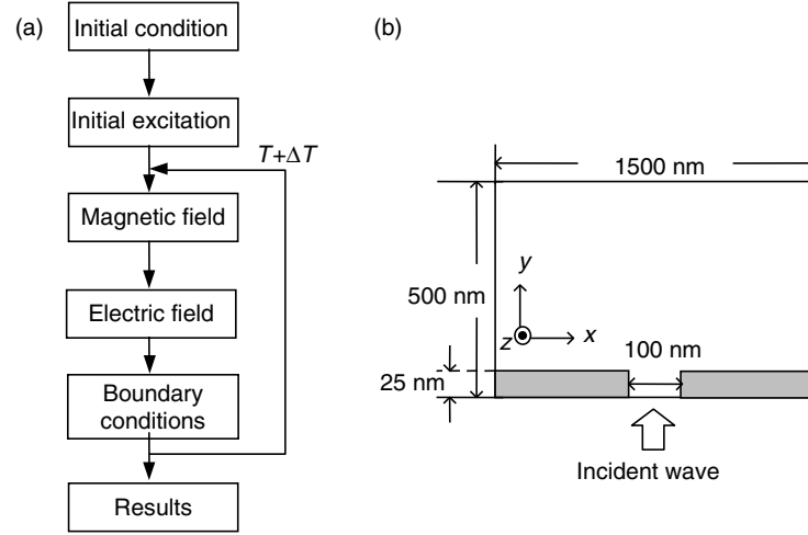
Fig. 5.5. Calculation process for FDTD (a), and computational domain for calculation (b)
