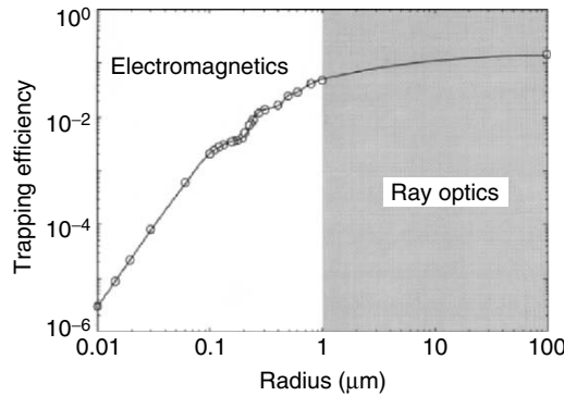
Fig. 3.6. Trapping efficiencies calculated with a ray optics model and an electromagnetic force model. Reprinted from [3.10] with permission by Michael W. Berns
