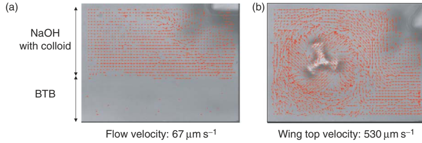
Fig. 4.68. Two-liquid mixing. Velocity vectors appear only in NaOH solution without mixer (a), but they appear in both liquids upon mixing using the optical mixer (b).
