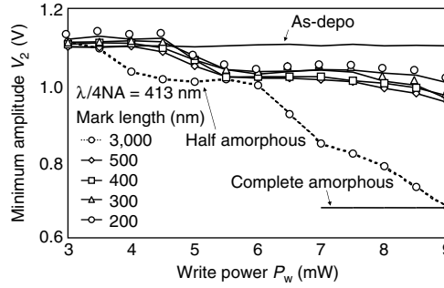
Fig. 5.44. Write power dependence of signal amplitude measured for readout#1
