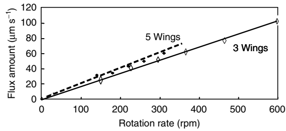
Fig. 4.62. Flux amount generated by shuttlecock optical rotors with different wing numbers
