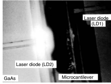
Fig. 1.29. Photograph of central part of a resonant sensor
