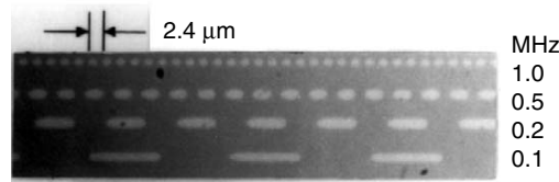
Fig. 2.42. Written bit patterns by 16 mW laser pulses at various frequencies
