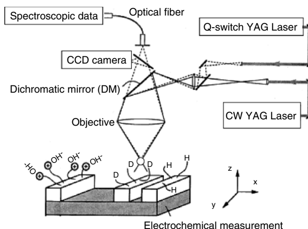
Fig. 3.43. Microchemical conversion system for studies of chemical reaction process. Reprinted from [3.6] with permission by H. Masuhara, Osaka University, Japan
