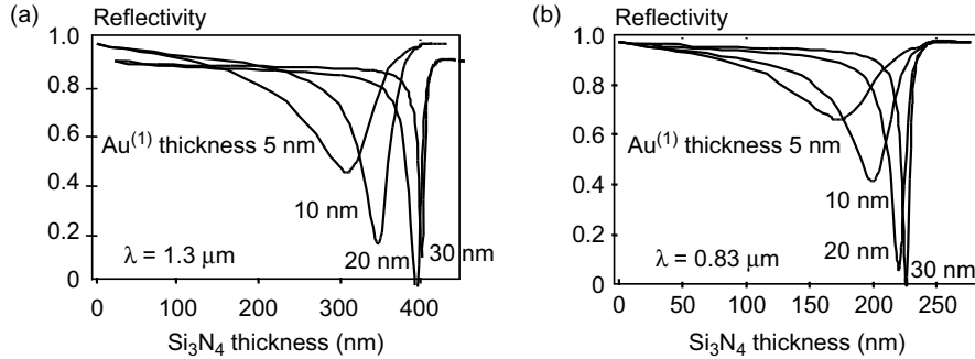
Fig. 2.51. Reflectivity of \text{Au}/\text{Si}_3\text{N}_4/\text{Au} versus the \text{Si}_3\text{N}_4 thickness for the wavelength of 1.3\mu\text{m} (a), and 0.83\mu\text{m} (b)
