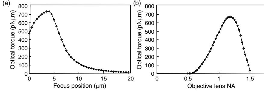
Fig. 4.6. Simulated optical torque dependence on focal position with objective lens \text{NA}=1.2 (a), and dependence on objective lens NA (b) with focus above 5\text{ }\mu\text{m} , for shuttlecock rotor with uniform light beam profile
