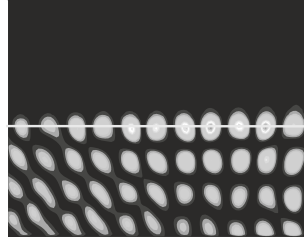
Fig. 5.11. Input plane wave and evanescent field produced at interface ( white line ) by total reflection
