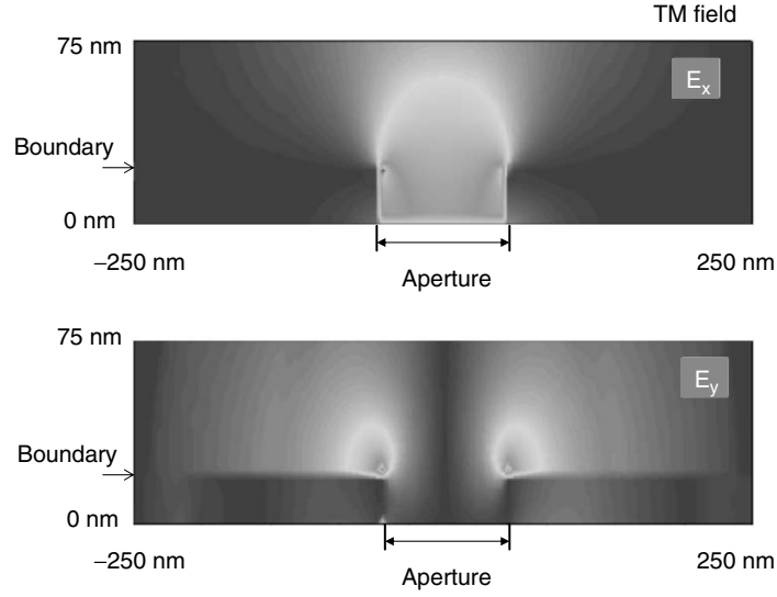
Fig. 5.6. Numerical result indicating that the electric evanescent field is enhanced at the edge and decays rapidly
