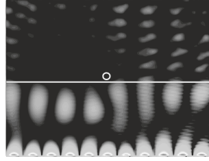
Fig. 5.12. Scattered light field of evanescent field by perfect conductor particle of 100 nm diameter ( white circle ) located 10 nm above the interface ( white line )
