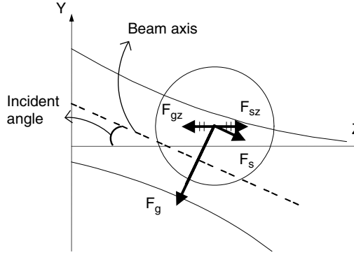
Fig. 3.23. Balancing between scattering force F_s and gradient force F_g at fiber incident angle of \theta [3.15]
