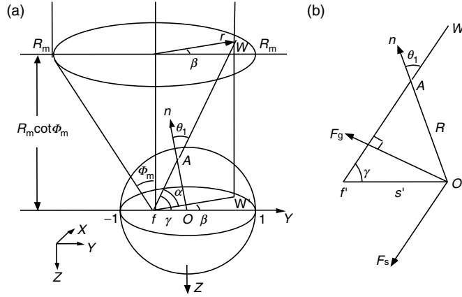
Fig. 3.12. Geometry for calculating the transverse trapping efficiency of polystyrene microsphere. The laser focus is located along the transverse center line of the sphere [3.4]
