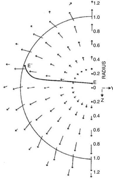
Fig. A.4. Magnitude and direction of total trapping efficiency (optical pressure force) for a microspore of relative refractive index of 1.2 at arbitral focal position in the yz plane. A circularly polarized laser beam uniformly fills the objective aperture of NA = 1.25 [6.4]
