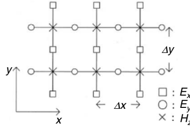
Fig. 5.4. Positions of electric- and magnetic-field vector components in two dimension. E and H components are positioned alternately, i.e., H is on every cell edge and E is between cells [5.15]
