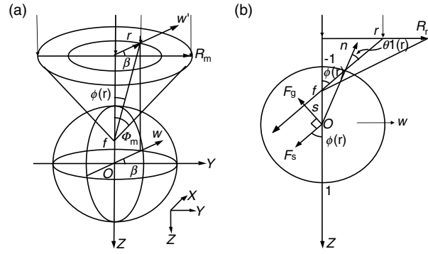
Fig. 3.11. Geometry for calculating axial trapping efficiency of polystyrene microsphere. The laser focus is on the optical axis which is parallel to the center line of the microsphere [3.4]
