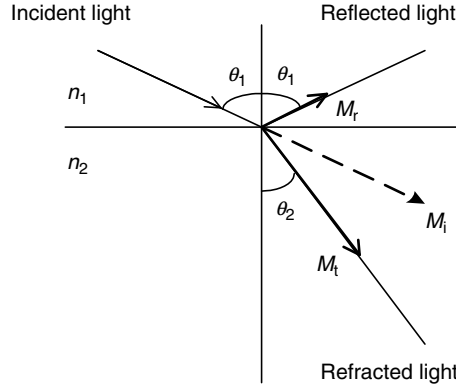
Fig. 3.7. Relationship between incident, reflected, and refracted rays at interface
