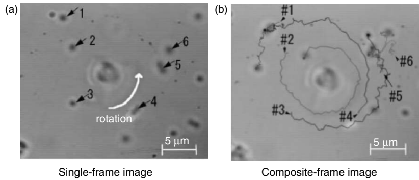
Fig. 4.51. Visualization and pathlines using glass tracers. Single-frame image (a), and analyzed pathlines (b)
