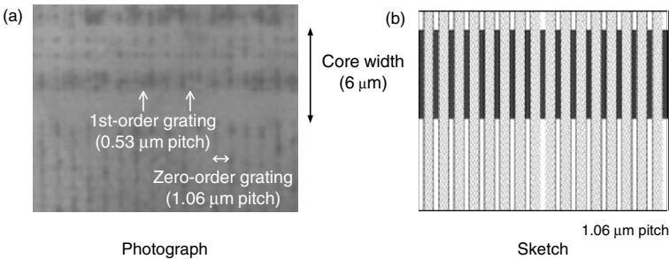
Fig. 5.26. Top view of grating fabricated on PLC (a), and sketch of the grating (b)
