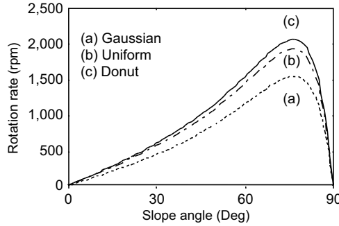
Fig. 4.15. Relationship between rotation rate and slope angle of the rotor of d = 3\mu\text{m} , h = 10\mu\text{m} , and n_2 = 1.53 in water at P = 100\text{ mW} for the Gaussian (a), uniformly filled (b), and donut (c) beam intensity profiles
