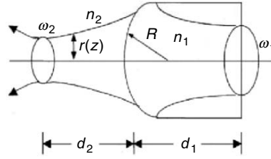
Fig. 3.17. Geometry for calculating trapping efficiency for microsphere along propagation axis by laser beam emitted from tapered lensed optical fiber
