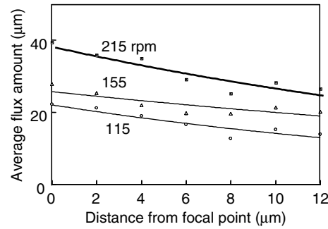
Fig. 4.60. Average flux amount at different depths for vertical rotation, rotation rate as a parameter
