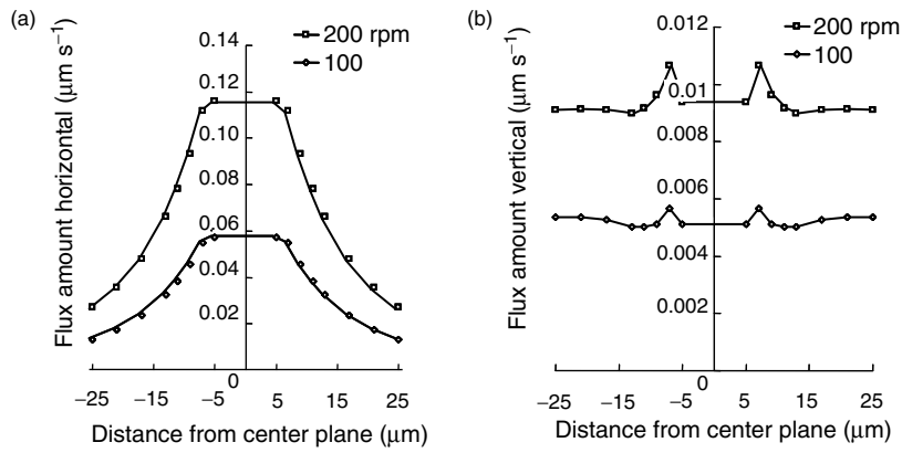
Fig. 4.25. Horizontal component (a), and vertical component (b) of fluid in the proximity of optical rotor
