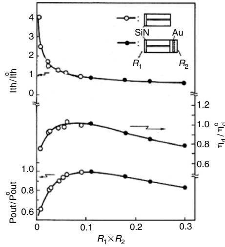
Fig. 2.57. Dependence of normalized I_{th} , \eta_d , and P_{out} on LD reflectivities product R_1 \times R_2 [2.32]
