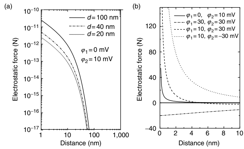
Fig. A.19. Electrostatic force dependence on distance between particle and wall
