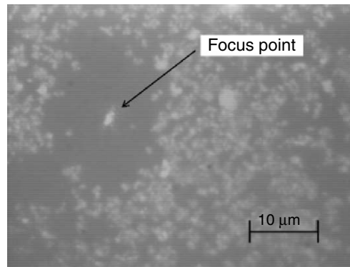
Fig. 4.53. Effect of optical pressure. Gold particles around the laser spot are expelled by the optical pressure
