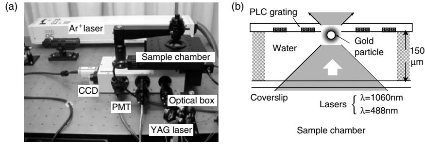
Fig. 5.22. Photograph of experimental setup of SNOM (a), and enlarged view of sample chamber (b)
