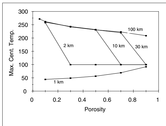
Fig. 10.3. Maximum central temperature for a series of comets of different radii as a function of porosity. Other parameters are like those in the baseline model.
