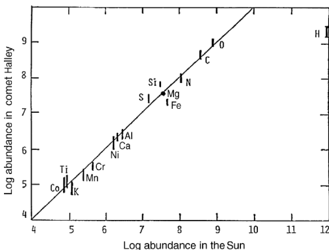
Fig. 2.5. The abundance of known element in comet Halley is compared with the same elements in the Sun. Except hydrogen (and presumably the noble gases) all elements seem to be in solar proportions in comet Halley. A curious exception is the Fe/Si ratio which is only 25% of that in the Sun. The silicon seems to be overabundant by a factor of 2, and the iron underabundant by the same factor, in comet Halley. This diagram is shown to establish that most siderophile elements are in solar proportions in comet Halley and, assumedly in all comets, explaining the surprising “siderophile excess” of the Earth’s crust, as well as their depletion in the upper mantle.
