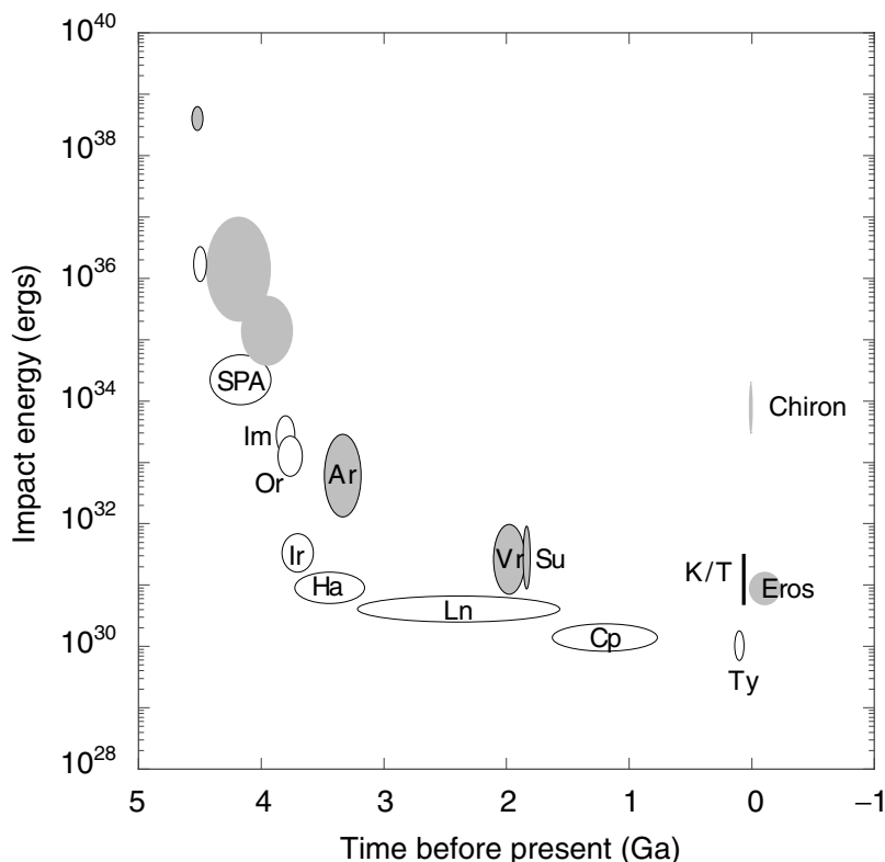
Fig. 7.4. The largest impacts before the present for Moon and the Earth. Open boxes are lunar, and shaded boxes are terrestrial. The dimensions of the boxes indicate uncertainties. The stippled region shows the inferred largest impacts on the Earth. The right-hand axis is the depth of ocean vaporized by the impact. The three earliest events (4.5 BY) shown are the energies of the Earth and Moon formation and the moon-forming impact. Energies and dates of basin-forming impacts are discussed in the text. The lunar craters are Tycho, Copernicus, Langrenus, Hausen, and Iridum; diameters and approximate ages are adapted from Wilhelms (1987). Size and dates of terrestrial impacts at Sudbury and Vredevort are taken from Grieve (1982). Energies of the impacts generating 4 Archean spherule beds between 3.2 and 3.5 Ga are estimated following Kyte et al. (2003). The Chicxulub crater (the K/T crater, 65 Ma) is at least 180 km diameter (Hildebrand et al., 1991). Eros and Chiron remain potential sources of future troubles.
