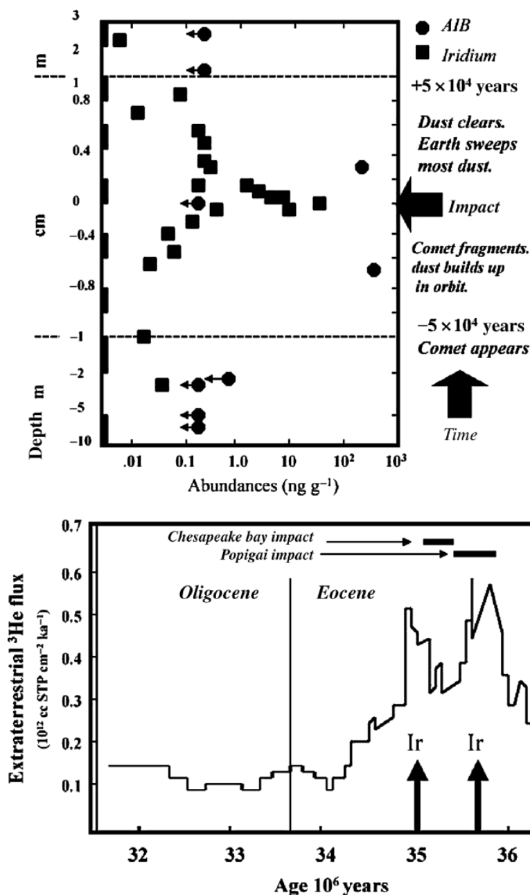
Fig. 8.11. Cometary components associated with impact boundaries. (A) Relations between AIB ( \alpha -amino isobutyric acid) and Ir across the K-T boundary at Stevns Klint (from Zhao and Bada, 1989; Zahnle and Grinspoon, 1990); (B) Extraterrestrial ^3\text{He} flux ( 10^{12} \text{ cc STP cm}^{-2} \text{ ka}^{-1} ) displayed by the late Eocene section at Massignano, Macertata, Italy (from Farley et al., 1998).
