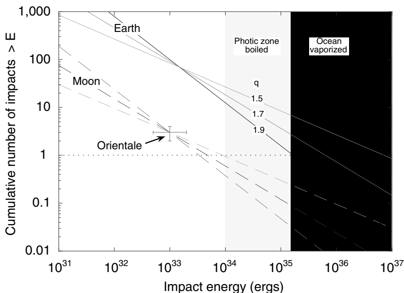
Fig. 7.3. Predicted numbers and energies of terrestrial impacts, scaled from the lunar record at the time of Orientale, Imbrium, and Nectaris. This addresses the period between 3.7 and 4.1 Ga. If extended earlier to include South Pole-Aitken the numbers would be shifted upward by about a factor of 4. The figure shows the number of impacts on the Earth with energies greater than a given energy E as scaled from the energies of the lunar Orientale and Imbrium basins. In this scaling a given object is 23 times more likely to strike the Earth than the Moon, and releases about 50% more energy on the impact. The different curves are labeled by the power law index q , where the cumulative number of impactors with mass greater than m is given by N(> m) \propto m^{1-q} . Distributions with smaller values of q are characterized by markedly more enormous impacts.
