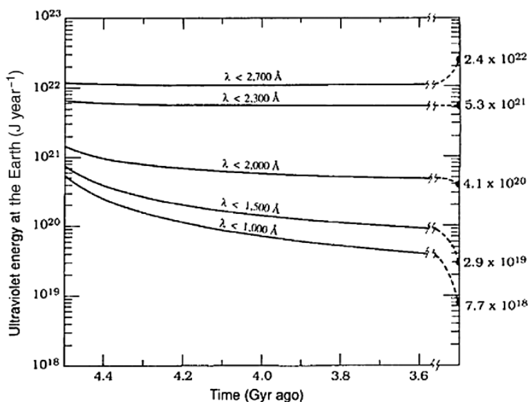
Fig. 6.3. Evolution of the Sun's ultraviolet luminosity through time, beginning with a \sim 10^8 -yr-old Sun at 4.5 Gyr ago, and extending to today. Dashed lines beyond 3.6 Gyr ago indicate qualitative evolution to current values. From Chyba and Sagan (1992).
