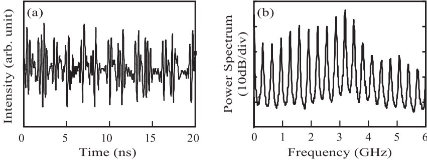
Fig. 10.10. Experimentally measured (a) temporal waveform and (b) power spectrum of a chaotic state of a single-mode semiconductor laser with optical feedback. (Reprinted with permission from [29], ©2002 AIP.)
