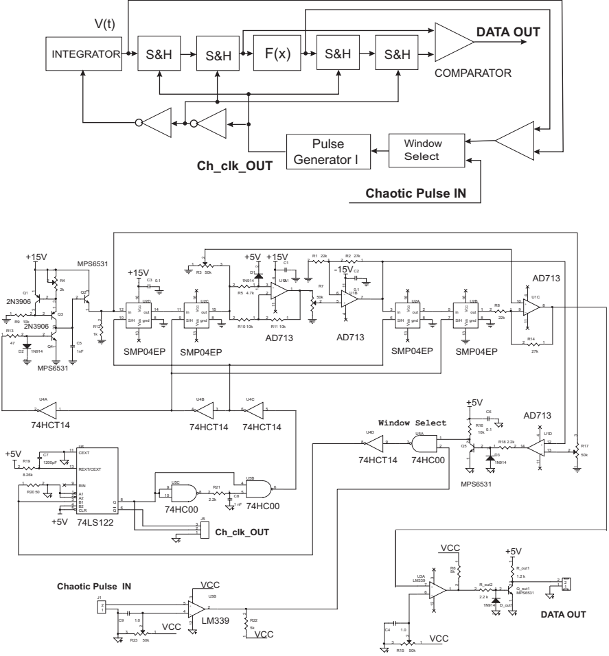
Fig. 2.5. Block diagram (top panel) and schematics (bottom panel) of the chaotic pulse demodulator.
