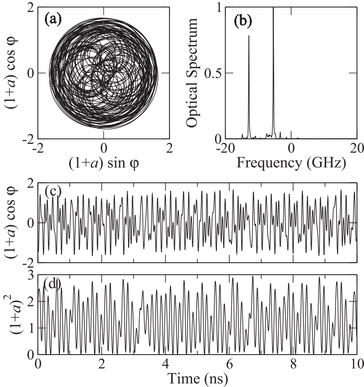
Fig. 10.9. Numerically calculated (a) attractor, (b) optical spectrum, (c) optical field, and (d) optical intensity of the chaotic state at the operating condition of \bar{J} = 2/3 , \xi = 0.1 , and \tau f_r = 0.3 for a single-mode semiconductor laser with optical feedback that has the parameters listed in Table 10.1.
