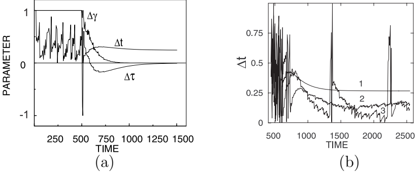
Fig. 3.3. (a) The normalized time shift between the oscillations \Delta\tilde{t} = \frac{\Delta t}{\Delta t_{\max}} and the adjusted parameters: \Delta\tilde{\tau} = \frac{\tau_{re}(n) - \tau_{tr}}{\Delta\tau_{\max}} , \Delta\tilde{\gamma} = \frac{\gamma_{re}(n) - \gamma_{tr}}{\Delta\gamma_{\max}} versus the time for \alpha_{tr} = \alpha_{re} = 16 , \delta_{tr} = \delta_{re} = 0.43 , \sigma_{tr} = \sigma_{re} = 0.72 , \gamma_{tr} = 0.1 , \gamma_{re}(0) = 0.11 . (b) The influence of mismatch of parameters \alpha_{tr, re} on the amplitude of fluctuations of the time shift \Delta t in the synchronous regime: \delta_{tr} = \delta_{re} = 0.43 , \sigma_{tr} = \sigma_{re} = 0.72 , \gamma_{tr} = 0.1 , \gamma_{re}(0) = 0.11 , \alpha_{re} = 16 , and \alpha_{tr} = 16 — (1); 16.7 — (2); 16.9 — (3). (Reprinted from [21], ©1997 IEEE.)
