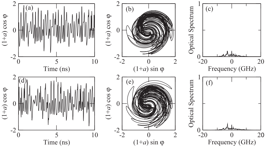
Fig. 9.2. Nonlinear effect of intrinsic laser noise on the chaotic state at \xi = 0.03 and f = 0 GHz: (a) Waveform, (b) attractor, and (c) optical spectrum are for R_{\text{sp}} = 0 . (d) Waveform, (e) attractor, and (f) optical spectrum are for R_{\text{sp}} = 4.7 \times 10^{18} \text{ V}^2 \text{ m}^{-2} \text{ s}^{-1} .
