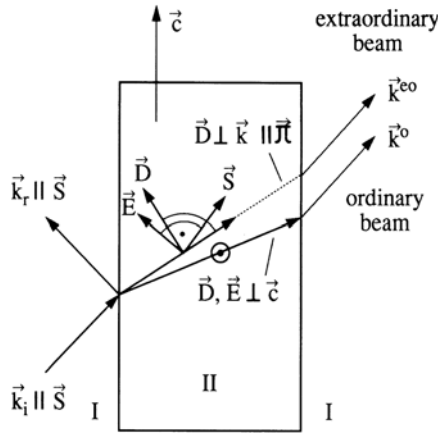
Fig. 3.11. Birefringence for an unpolarized beam falling on a birefringent material at a given angle with the crystallographic axis \vec{c} parallel to the interface
