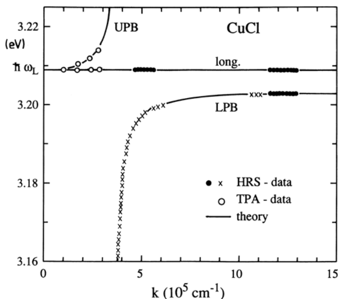
Fig. 13.20. The polariton dispersion of the lowest \Gamma_5 -exciton resonance in CuCl measured by two-photon absorption and by hyper-Raman scattering [71F1, 81K2, 85H1]
