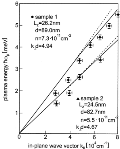
Fig. 12.5. The in-plane dispersion relation of plasmons in two different modulation doped GaAs/ \text{Al}_{1-y}\text{Ga}_y\text{As} samples [82O1]
