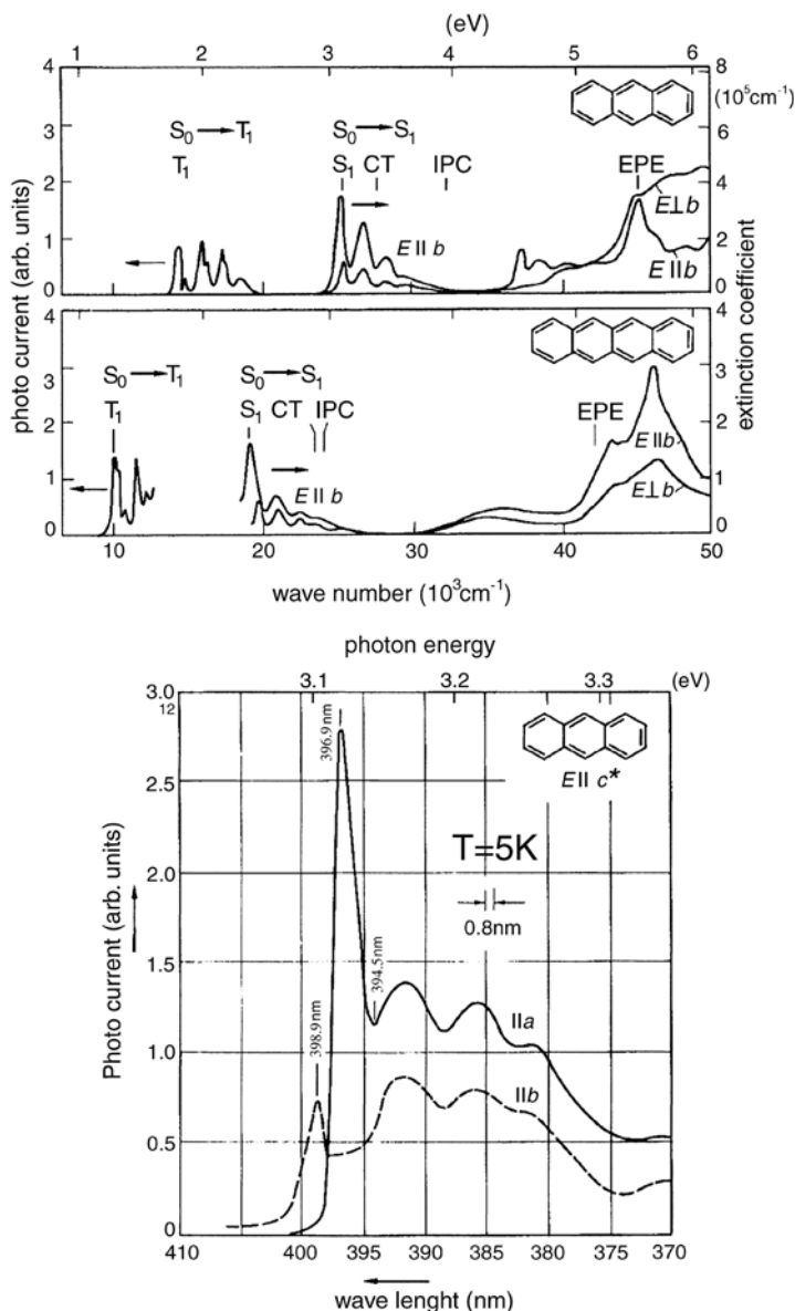
Fig. 13.22. Overview of the absorption spectra of anthracene (a) and tetracene (b) and photocurrent excitation spectra (PCE) of the singulet exciton in anthracene. According to [77C1,79S2] and [82L1] of Chap. 1
