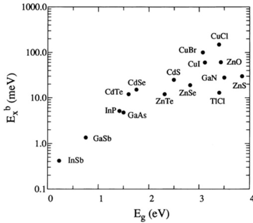
Fig. 9.3. The exciton binding energy E_{\text{ex}}^b as a function of the band-gap for various direct gap semiconductors ([82L1, 93H1, 93P1] of Chap. 1)
