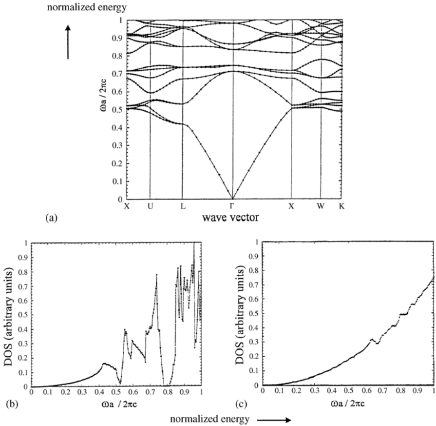
Fig. 17.5. (a) The calculated photonic band-structure of close-packed air spheres in Si, a so-called inverted opal. (b) The resulting density of states (DOS), showing clearly a gap around \omega a / 2\pi c \approx 0.8 for this system and for (c) SiO 2 spheres in air corresponding to natural opal [99J1]
