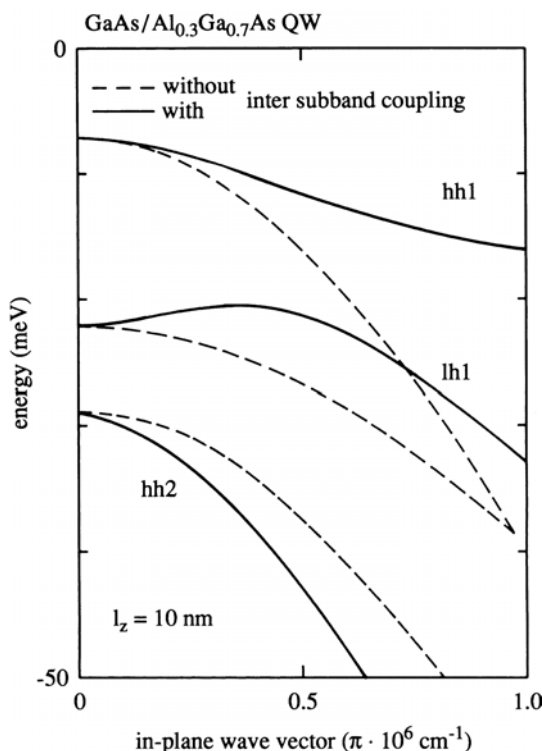
Fig. 8.24. The in-plane dispersion relation of the first three valence subbands in a \text{GaAs}/\text{Al}_{1-y}\text{Ga}_y\text{As} quantum well without (---) and with (—) intersubband interaction ([86B1] or [01L1] of Chap. 1)
