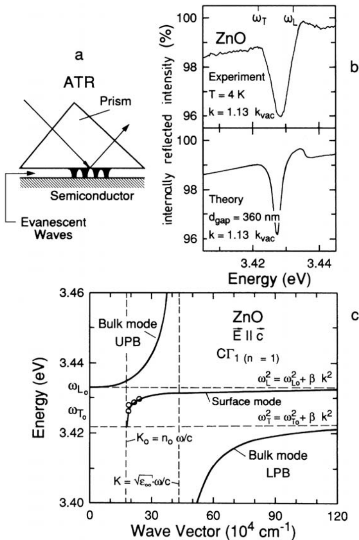
Fig. 13.21. The principle of the experimental technique of attenuated total reflection (ATR) (a) experimental and calculated ATR spectra for the n_B = 1\Gamma_1 -exciton in ZnO (b) and the resulting dispersion of the surface and volume polaritons (c). According to [78L1]
