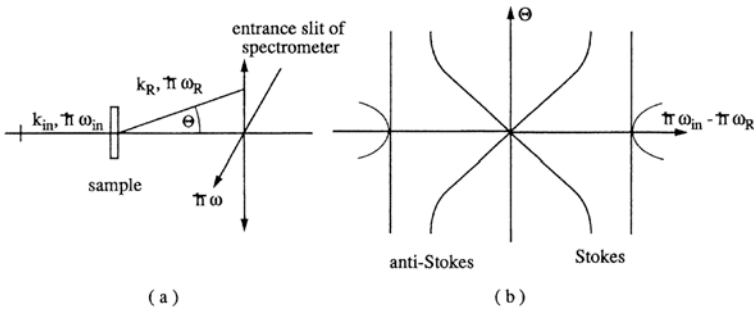
Fig. 11.3. Schematics of a Raman scattering experiment in the forward direction with a spectrometer (a) and the visualization of the relation between \Theta and \hbar\Omega of a in the output plane of the spectrometer (b)
