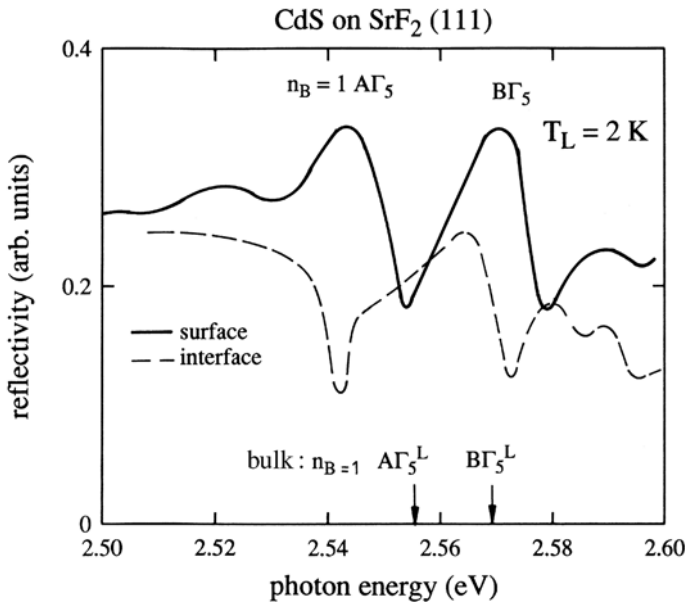
Fig. 16.18. Reflection spectra of the n_B = 1A\Gamma_5 and B\Gamma_5 excitons of a CdS layer grown on \text{SrF}_2 and measured at the surface and at the interface. The positions of the longitudinal eigenenergies in the bulk are indicated by vertical arrows [92B1]
