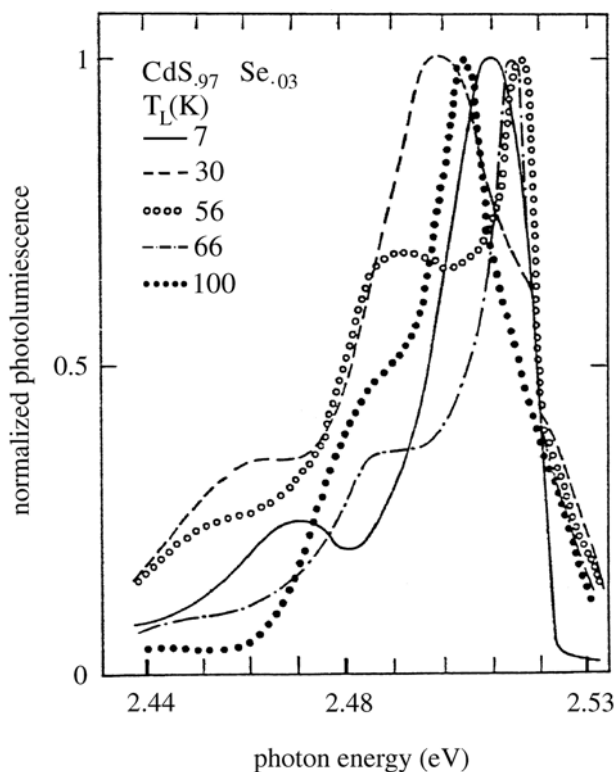
Fig. 14.15. The low excitation photoluminescence spectra of \text{CdS}_{.97}\text{Se}_{.03} for various lattice temperatures T_l [88S1]
