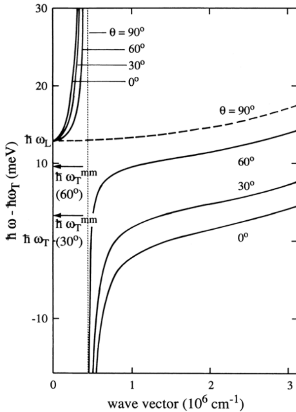
Fig. 13.8. Dispersion of the exciton polariton in a uniaxial material for various angles between \mathbf{k} and \mathbf{c} . Data for the CT_1 exciton polariton in ZnO. According to [78H1]
