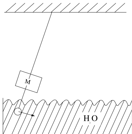
Fig. 23.26. A mechanical model to realize the difference between Markovian and non-Markovian damping. According to [01W1]
