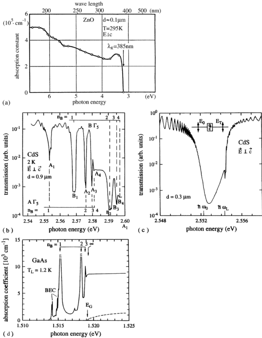
Fig. 13.9. An experimental absorption spectrum of ZnO at RT (a), an experimental transmission spectrum of CdS for the orientation E \perp c in the region of the A and B exciton resonances (b); a calculated one for the A \Gamma_5 resonance for n_B = 1 (c); and an absorption spectrum for a thin GaAs sample (d). According to [43M1] to [79V1, 82R1] and to [91U1], respectively
