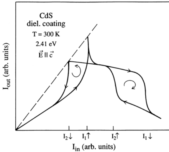
Fig. 24.8. “Butterfly” type hysteresis loops in CdS [87W1]
