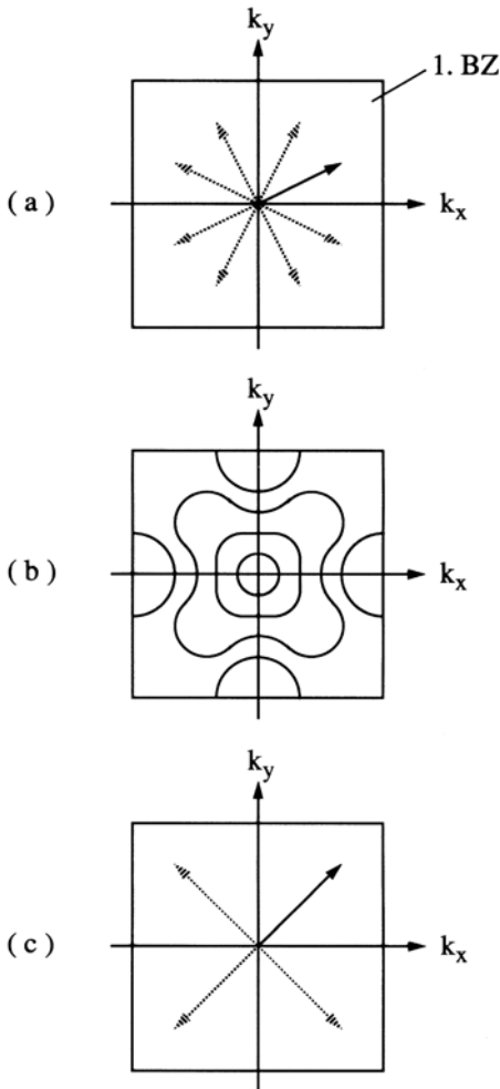
Fig. 26.5. The star of \mathbf{k} , (a) the qualitative shape of surfaces of constant energy E(\mathbf{k}) (b); and a \mathbf{k} -vector of higher symmetry (c)
