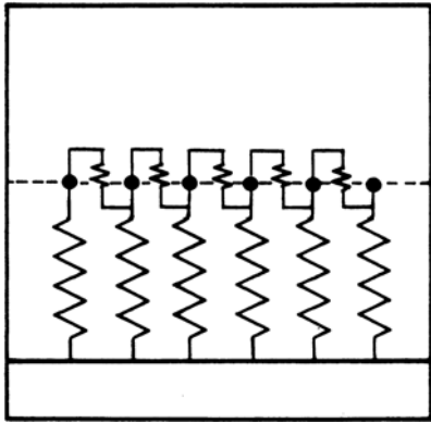
Fig. 5.8. An ensemble of coupled oscillators. Compare with Fig. 4.1. After [63H1]
