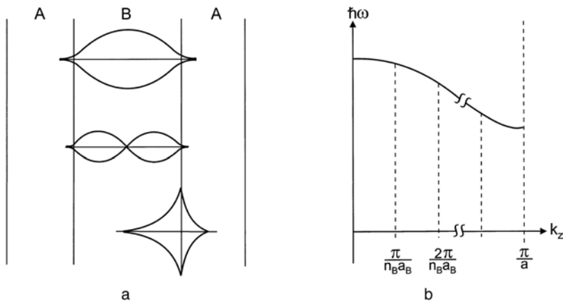
Fig. 7.24. Schematic representation of the envelope of an optical phonon mode confined to material B in a superlattice and of an interface phonon (a) and the discrete values of k_z on an optical phonon branch of material B. (b)
