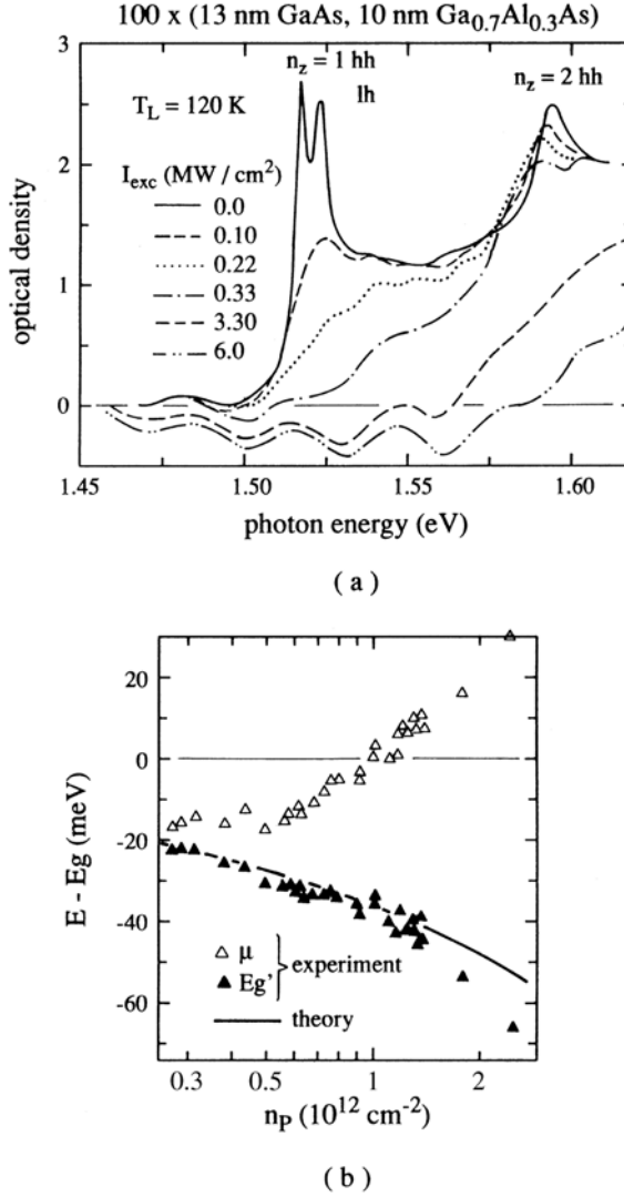
Fig. 21.14. Transmission spectra of an \text{Al}_{1-y}\text{Ga}_y\text{As}/\text{GaAs} MQW sample for various pump intensities (a) and the resulting dependence of the reduced gap E_g' (b) and of the chemical potential \mu on the electron-hole pair density per unit area n_P [89K4, 91S1]
