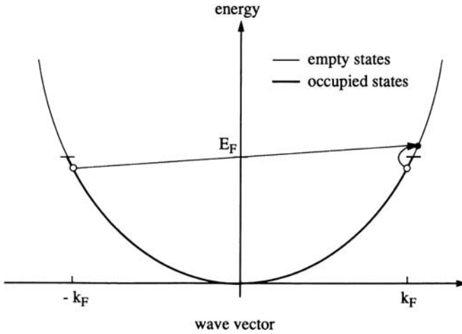
Fig. 10.3. Two-particle excitations within one band with degenerate population
