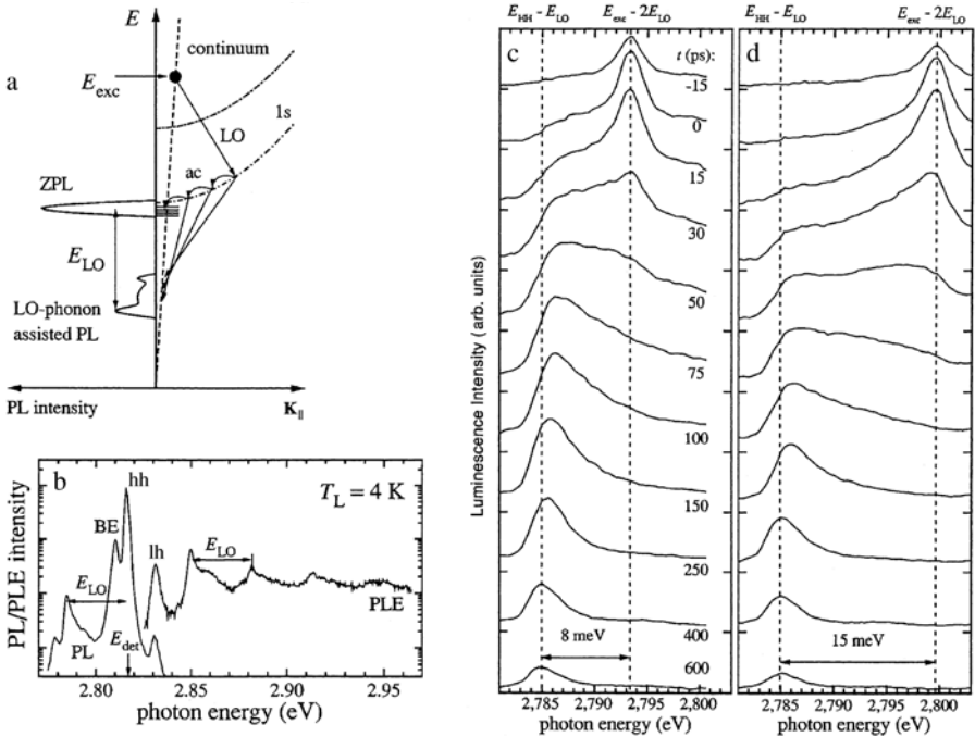
Fig. 23.33. (a) Schematics of the luminescence spectrum and of the exciton relaxation process in ZnSe/ZnS 1-x Se x superlattices (b) A time-integrated luminescence spectrum c, d Time-resolved spectra for two different excess energies [98U1]
