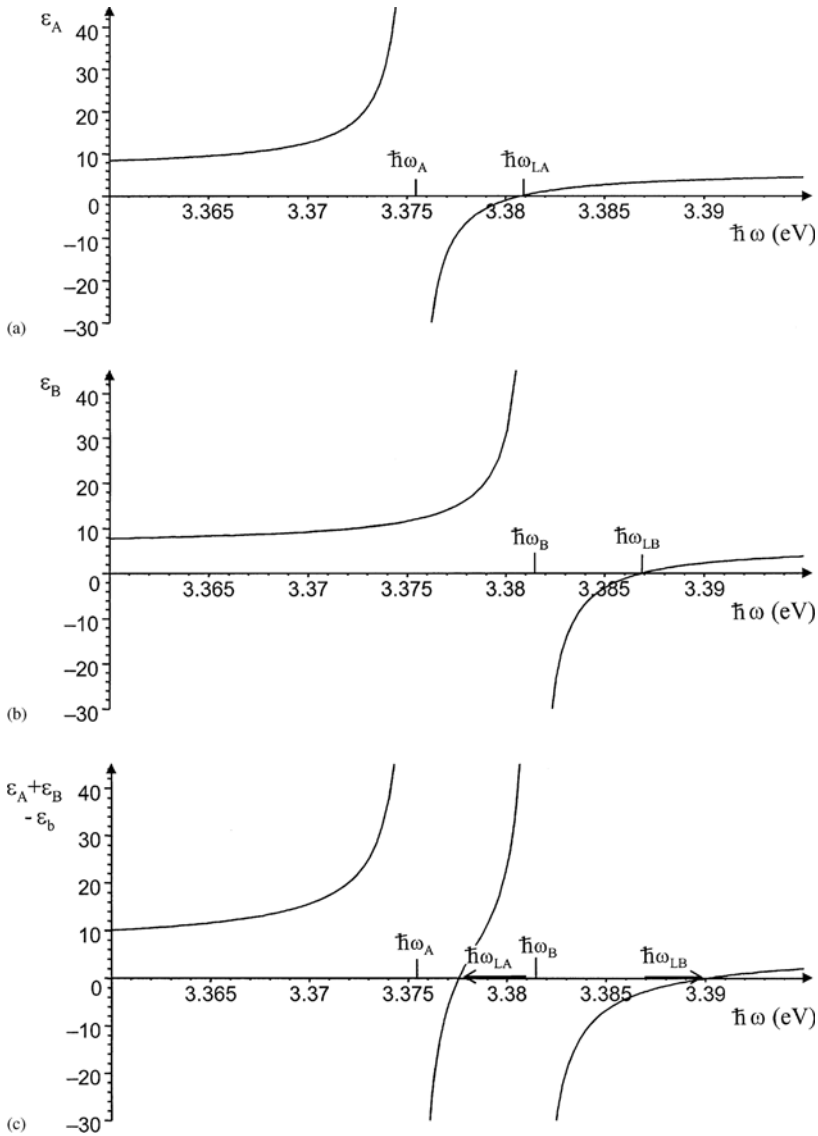
Fig. 4.9. The real part of \varepsilon(\hbar\omega) for two resonances separately (a, b) and for two close lying resonances (c). Numbers on the x -axis refer roughly to ZnO
