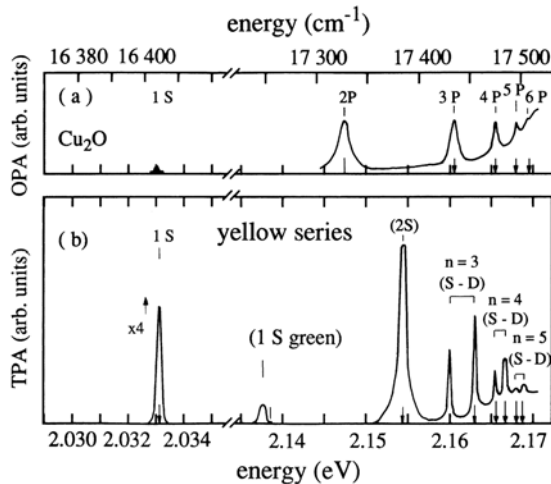
Fig. 13.30. The absorption of the forbidden “yellow” exciton series in \text{CuO}_2 in one and two absorption (OPA and TPA, respectively). According to [81U1]
