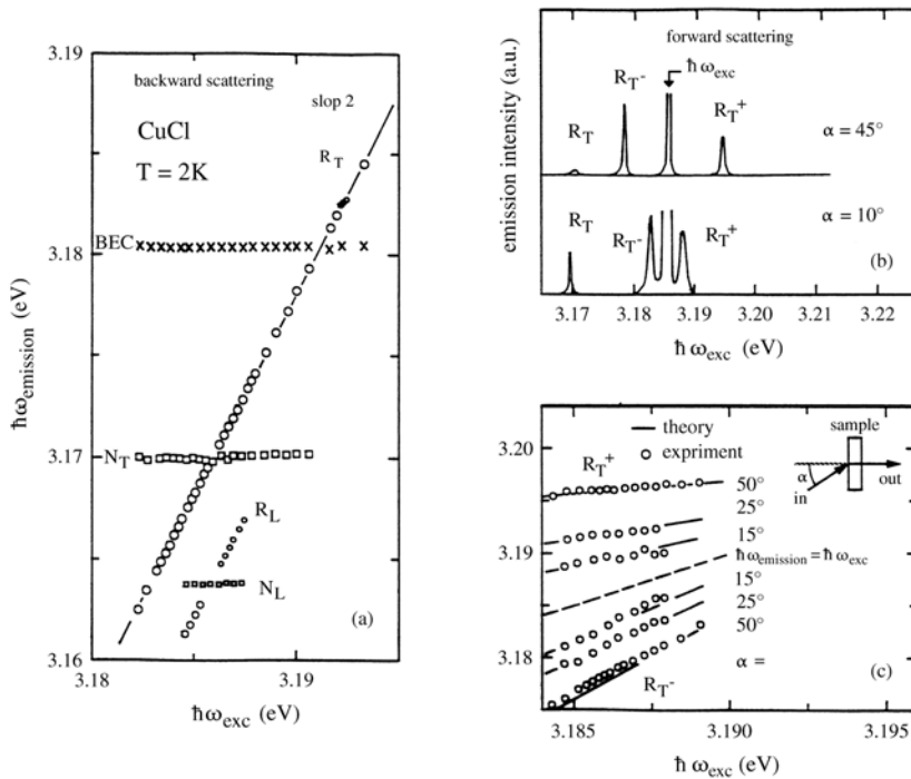
Fig. 20.10. The dependence on \hbar\omega_{\text{exc}} of the two-photon Raman emission via an intermediate biexciton state in CuCl for various scattering geometries (a,c) and a set of spectra for forward scattering (b). According to [85H1]
