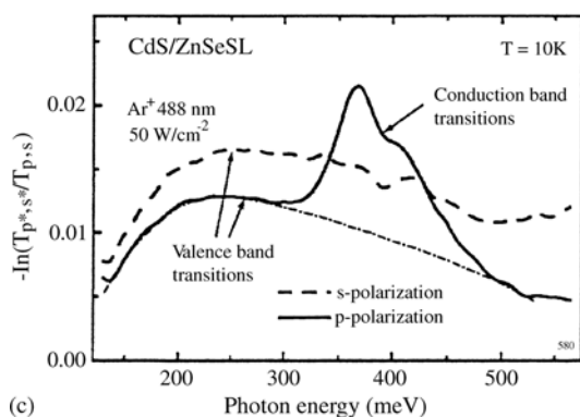
Fig. 21.17. (a) The inter-subband absorption of an n -modulation doped GaAs/Al 1-y Ga y As MQW sample. (b) The inter-miniband absorption of a homogeneously n -doped 200 \times (7.5\text{ nm GaAs}/2.5\text{ nm Al}_{1-y}\text{Ga}_y\text{As}) superlattice [95T1, 93H1] and (c) of an optically pumped 140 \times (2\text{ nm CdS}/1.9\text{ nm ZnSe}) superlattice [00G1, 02G1]
