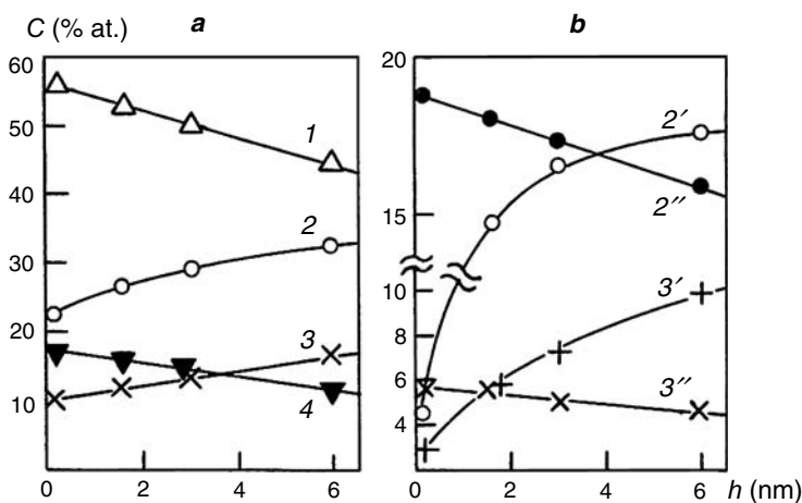
Fig. 2.51. Variations of elemental composition (C, % at) across depth (h, nm) of the adsorptive protecting Tet layer on steel. (a) gross composition: (1) N, (2) O, (3) Fe, (4) C; (b) O and Fe elements bound into iron oxide (2', 3') and CC (2'', 3'')
