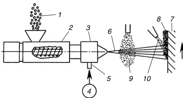
Fig. 3.32. Layout chart of coating deposition by extrusion. (1) polymer granulate, (2) extruder, (3) spray head, (4) gas jet generator, (5) socket, (6) gas-polymer flow, (7) article, (8) coating, (9) aerosol, (10) powder flow
