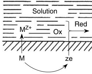
Fig. 1.1. Scheme of electrochemical corrosion mechanism of metals [1]
