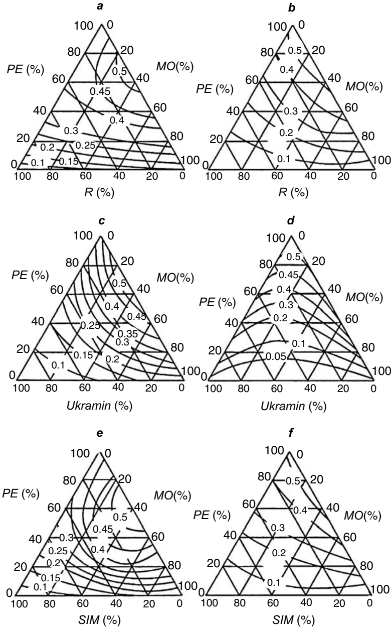
Fig. 2.45. Steel isocorrns under PE films modified by mineral oil (MO) and CI: (a) and (b) AKOR; (c) and (d) Ukramin; (e) and (f) SIM; (a), (c) and (e) in 0.1 N solution of HCl; (b, d) and (f) in 1 N solution of \text{Na}_2\text{SO}_4 . Test duration – 14 days
