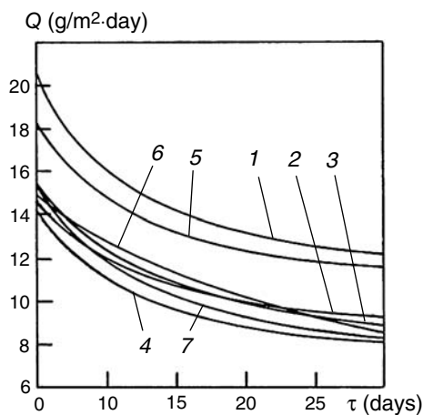
Fig. 2.37. Kinetic curves of vapor-penetrability of LDPE-based films: (1) without CI; (2–4) with volume distribution and (5–7) with surface distribution of inhibitors; (2) G-2; (3, 4, 6) and (7) NDA; (5) IFHANGAZ. CI concentrations: (2) 0.5; 3 and (6) 1; (5) 3; (7) 2.5 wt%
