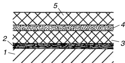
Fig. 3.20. A scheme for a combined polymer antirust coating. (1) metal substrate, (2) passivating layer, (3) a layer of organic metal, (4) a layer containing corrosion inhibitors, (5) electret polymer layer
