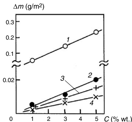
Fig. 2.32. The amount of PHC ( \Delta m ) isolated from PE films in 200 hours at 25°C depending on the initial concentration ( C ) of these VCI in the films: (1) Tr; (2) Tet; (3) KPhTet; (4) ATr
