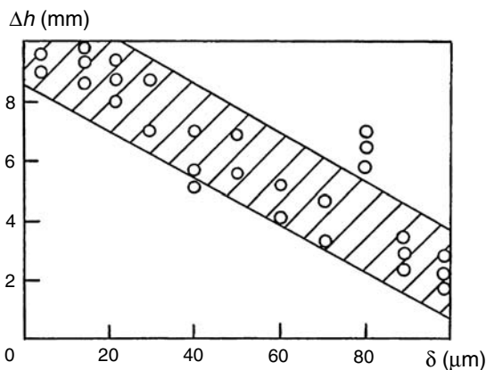
Fig. 3.8. Water level variation in a capillary as a function of polyethylene coating thickness over which the water spreads
