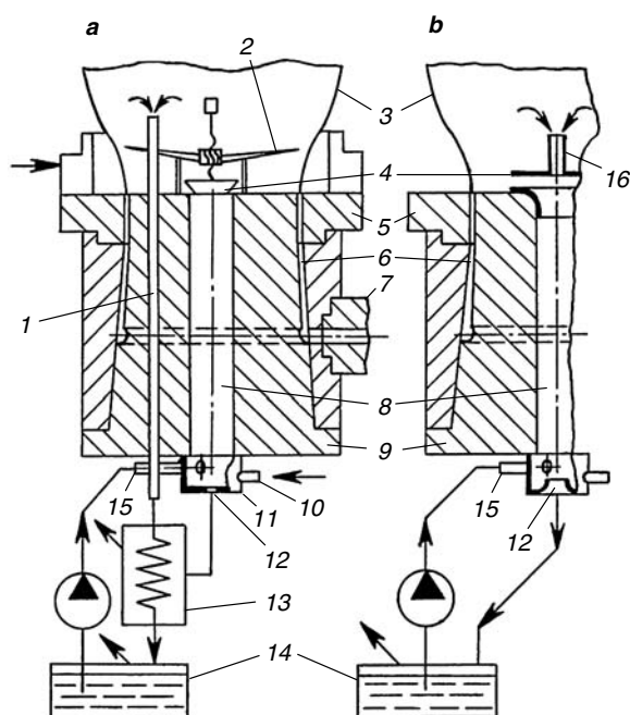
Fig. 2.21. An extrusion head with a vortical unit for CI feeding to the mandrel
