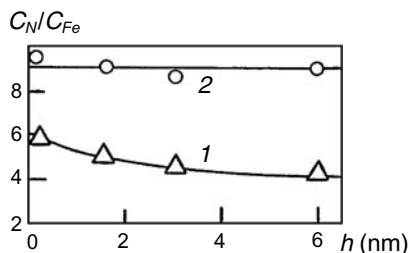
Fig. 2.52. Change of atomic ratio C_N/C_{Fe} through depth of protective layer Tet on steel versus relative total amount of iron (1) and combined in the complex iron (2)
