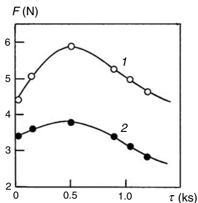
Fig. 4.9. Variation kinetics of friction force in the polymer composite-steel pair. The composite is based on HDPE (75 wt%) and fluoroplastic F-3 powder: (1) non-activated powder; (2) mechanically activated powder
