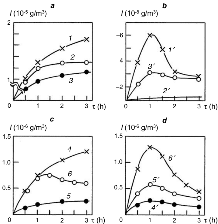
Fig. 4.27. Wear rate of steel (a, b) and polymer materials (c, d) in 0.1 N solution of \text{H}_2\text{SO}_4 (a, c) and in air (b, d). Polymer materials: 1, 1', 4, 4' – PE; 2, 2', 5, 5' – PE (65 wt%) + MO; 3, 3', 6, 6' – PE (65 wt%) + MO + CI
