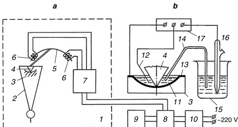
Fig. 4.14. Scheme of a pendulum tribometer (a) and electrochemical cell for polarization of the friction zone (b): (1) tribometer; (2) pendulum; (3) support; (4) prism; (5) bow-shaped core; (6) inductive pickup; (7) rectifier unit with a generator; (8) amplifier; (9) self-recording potentiometer; (10) voltage stabilizer; (11) electrolyte; (12) platinum electrode; (13) metal tray; (14) electrolytic switch; (15) vessel with electrolyte; (16) reference electrode; (17) potentiostat
