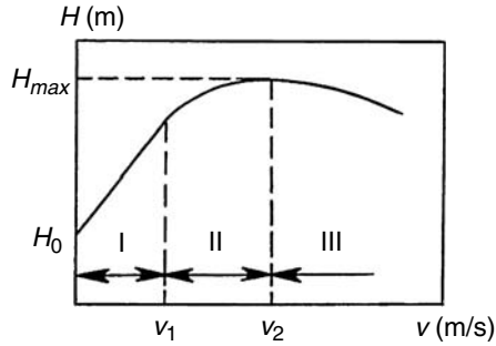
Fig. 3.25. Dependence of the height H of the powder layer fluidized by a vibrovortex method on the gas flow velocity v under a constant vibration regime
