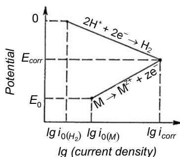
Fig. 1.3. Evans' diagram
