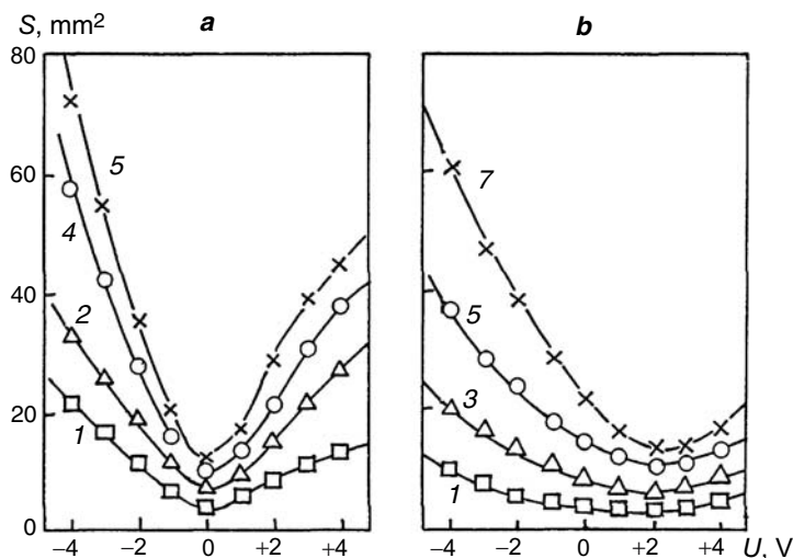
Fig. 1.8. Delamination kinetics of polyethylene coatings from graphite (a) and steel (b) substrates in a 5% solution of \text{H}_2\text{SO}_4 versus potential value U fed to the substrate and exposure time in electrolyte (numbers on curves indicate exposure time in hours)
