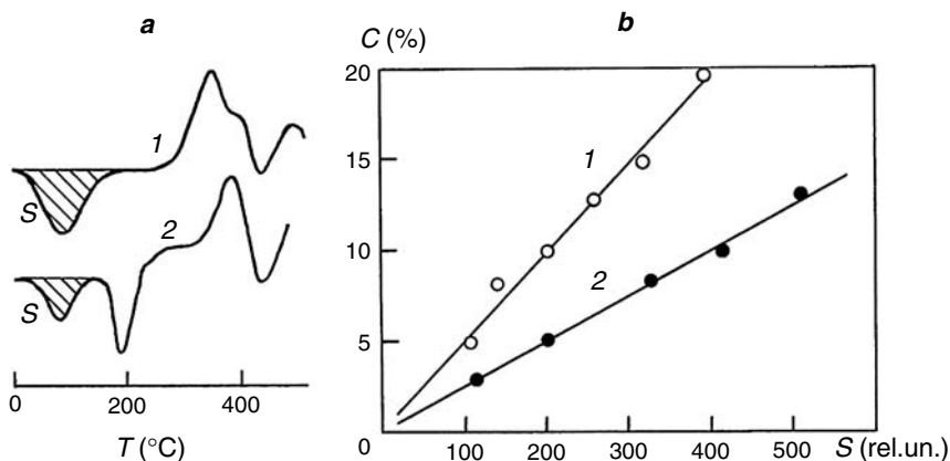
Fig. 2.53. Derivatographic analysis of CI content in polymer films. (a) DTA curves: (1) MSDA inhibitor; (2) PE film with 5 wt% of MSDA. (b) calibrating dependencies of CI concentration ( C ) in PE films upon area ( S ) of endothermic peaks of inhibitor evaporation on DTA curves of film samples: (1) MSDA; (2) IFHANGAZ
