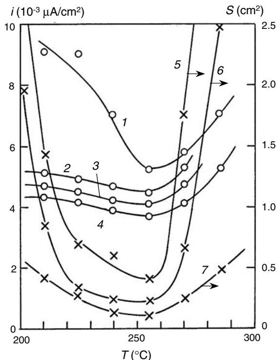
Fig. 3.4. Anodic current density ( i , 1–4) in electrodes with pentaplast coatings (0.5 N solution of \text{H}_2\text{SO}_4 , 20^{\circ}\text{C} ) and delamination area ( S , 5 – 7) of the coatings round a puncture (pregnant solution of \text{NaCl} , 20^{\circ}\text{C} ) versus coating formation temperature ( T ). Curves (1) 4 correspond to polarization potentials 4.0; 3.0; 2.0 and 0 V. Curves 7, 6 and (5) after 75, 125 and 150 hours of exposition
