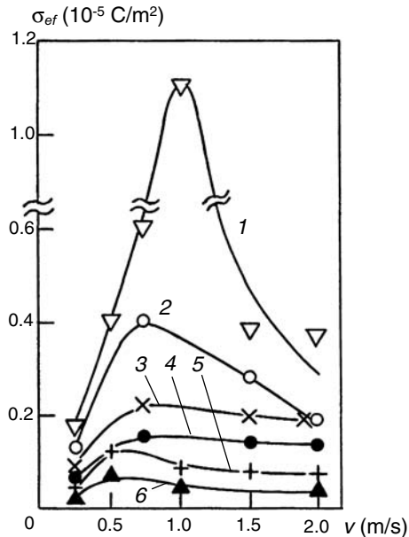
Fig. 4.7. Effect of friction velocity of HDPE over steel in different media on ESCD ( \sigma_{ef} ): (1) water; (2) Vaseline oil; (3) 0.1 N solution of KCl; (4) 1 N solution of KCl; (5) glycerin; (6) castor oil [47]
