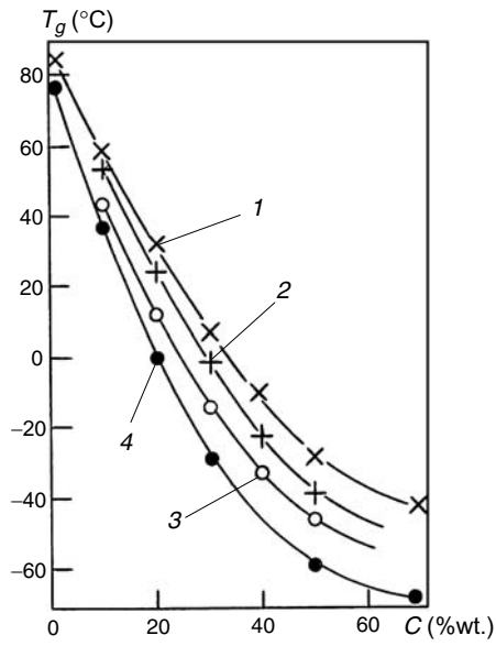
Fig. 1.13. Glass transition temperature ( T_g ) of PVC versus diethyl phthalate content ( C ). T_g determined by: (1) dynamometric balance; (2) thermo-mechanical method; (3) DTA; (4) DSC
