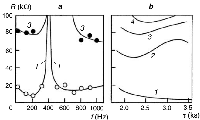
Fig. 2.59. Changes in electrical resistance R of the electrolyte PE film with a puncture (100 \mu m diameter) – substrate system depending on (a) frequency of mechanical oscillations of the sample, f , and (b) time at f = 0 . Plasticizer content in the film, wt%: (1) 0; (2) 30; (3) 40; (4) 50
