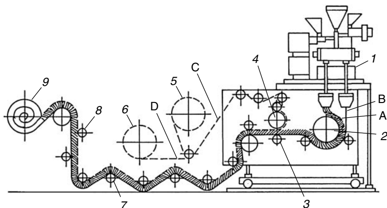
Fig. 2.16. Production line for air-bubble films
