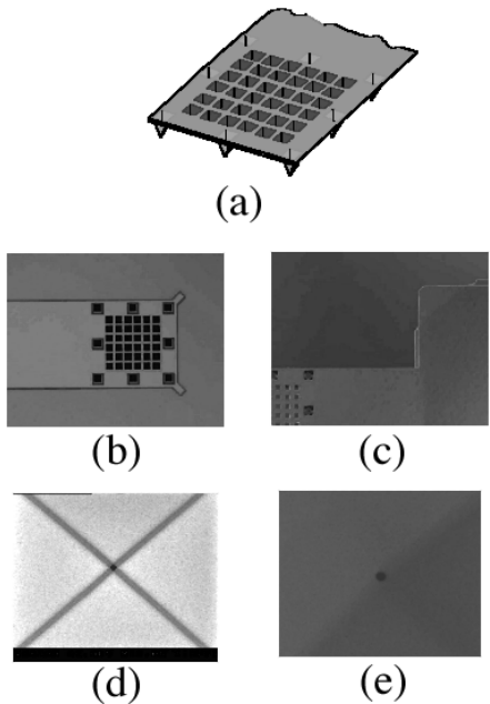
Fig. 4.4. a–e. Flying near-field head with 6 \times 6 array apertures designed in LAOTECH. a Schematic picture of the array head, b and c are the SEM images, d and f are the soom images of each aperture. Each aperture size was 60 nm. Courtesy of Dr. C. Mihalcea
