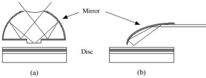
Fig. 4.18. a–b. SIL-related technologies using catadioptric mirror (SIM) (a) and hemi-paraboloidal SIM (b)
