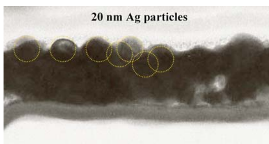
Fig. 5.13. Cross section of Ag nanoparticles formed on a polycarbonate disc substrate. A ZnS-SiO 2 dielectric thin layer (10 nm) was covered with the plastic substrate (TEM image)
