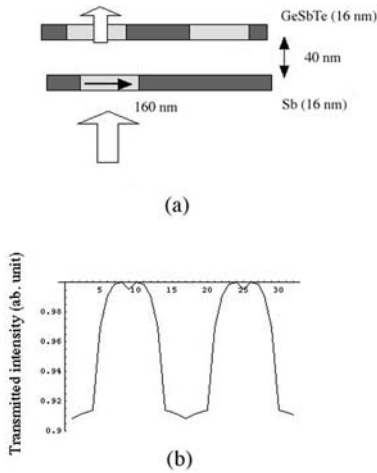
Fig. 3.14. a 2-D FDTD simulation model of super-resolution near-field structure (super-RENS). b The transmitted light intensity form the structure
