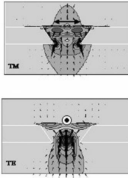
Fig. 3.10. Near-field distributions and Poynting vectors in a small aperture. Top: TM waves comes in the aperture, and bottom: TE waves. The slit size is 200 nm and Al film thickness is 125 nm. The incident light wavelength is 488 nm and the beam profile is Gaussian
