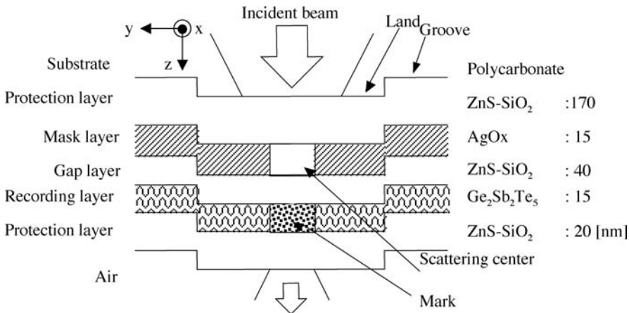
Fig. 3.16. FDTD model for super-RENS disc
