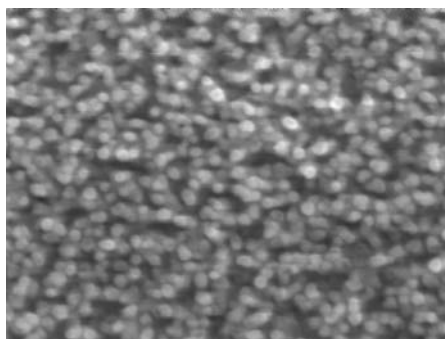
Fig. 5.12. SEM image Ag nanoparticles (size of each nanoparticle is 20nm) fabricated by oxygen reduction from AgOx film
