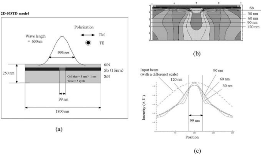
Fig. 3.13. a–c. Two-dimensional FDTD computer simulation of near-field characteristics of Sb thin film and aperture formation. Incident light transmits the 99-nm aperture (amorphous phase). a The simulation model. b The near-field generated around the aperture (incident light is polarized in TM-mode). c Intensity profiles from each aperture position [Courtesy of Mr. A. Sato and Dr. T. Nakano]
