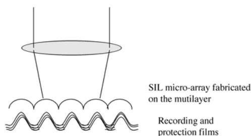
Fig. 4.17. Pre-fabricated SIL micro-array on the optical disc surface by vacuum deposition method by Guerra et al.
