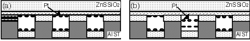
Fig. 3.21. a–b. Simulation model for super-RENS disc with plarinum nanoparticles. a Pt nanoparticles have a same configuration in each gas bubble. b The central gas bubble has only a condensation
