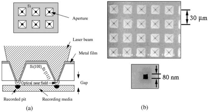
Fig. 4.3. a–b. Small-size apertures for NFR fabricated by Si processing. a Aperture design and recording schematic. b Scanning electron microscope (SEM) images of the apertures in our group. Reprinted by permission of the publisher [34]
