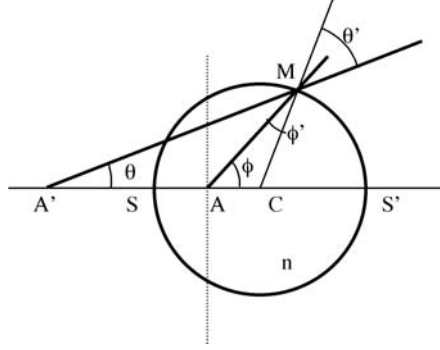
Fig. 4.15. Focal image points inside and outside medium with refractive index, n
