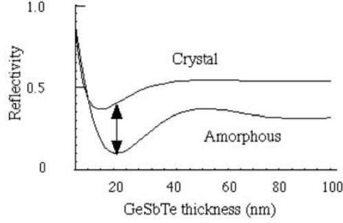
Fig. 2.17. The second ZnS-SiO 2 layer's thickness is fixed at 30 nm, and instead the recording layer thickness is changed. The simulation structure is thus PC/ZnS-SiO 2 (100 nm)/Ge 2 Sb 2 Te 5 (x nm)/ ZnS-SiO 2 (30 nm)/Al alloy (100 nm)
