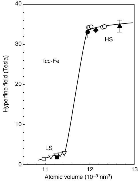
Fig. 10.9. Hyperfine field B_{\text{hf}} as a function of the atomic volume for fcc \gamma -Fe anti-Invar [22]. Data from Mössbauer experiments on epitaxial films grown on Cu (001) (filled square, filled circle), \text{Cu}_3\text{Au} (filled triangle), \text{CuAu} (filled diamond), and coherent precipitates in Cu–Al (open down triangle, open square)
