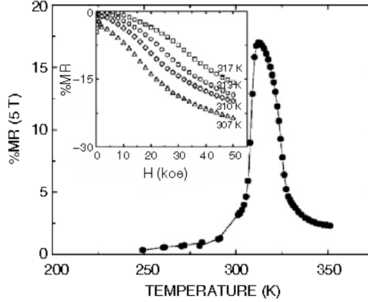
Fig. 4.5. Magnetoresistance ratio MR = \{[\rho(0) - \rho(5\text{ T})] / \rho(0)\} \times 100 versus temperature of MnAs. Inset: MR versus H [27]
