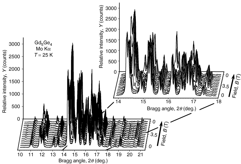
Fig. 11.7. Fragments of the X-ray powder diffraction patterns of \text{Gd}_5\text{Ge}_4 collected at 25 K with the magnetic field varying from 0 to 3.5 T and then back to 0 with a 0.5 T step
