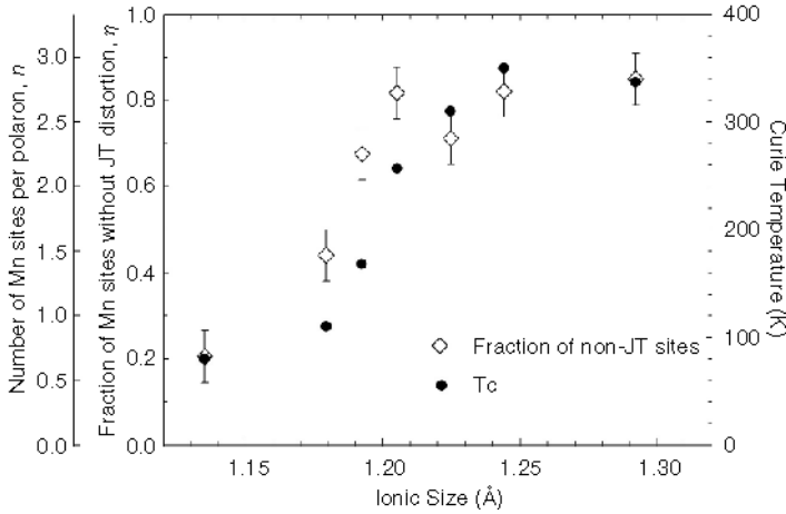
Fig. 5.4. The fraction of the Mn sites without the local Jahn–Teller distortion in \text{A}_{0.7}\text{A}'_{0.3}\text{MnO}_3 with various A and A' ions, as a function of the average ionic size, \langle r_A \rangle , determined by the PDF analysis of the pulsed neutron diffraction data [24]. It gives the size of the polaron when divided by the charge density in terms of the number of Mn sites involved
