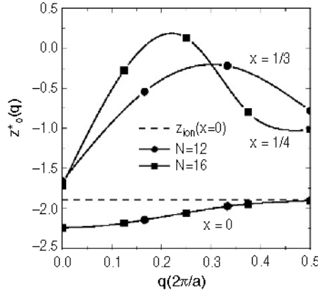
Fig. 5.11. The q dependence of the effective charge of oxygen in the 1-d Hubbard model due to the LO phonon mode, calculated for the ring of N = 12 sites with doping level x = 0, 1/3 and for N = 16 with x = 0, 1/4 . The dashed line indicates the ionic value (static charge) [48]
