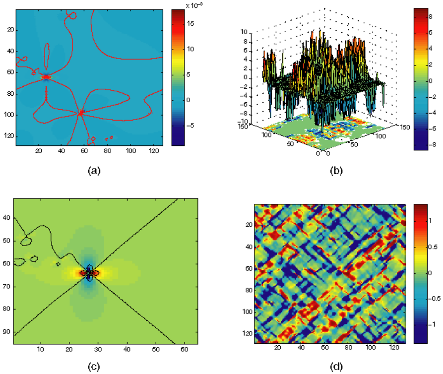
Fig. 2.4. “Manganite” parameters: see text. (a) Two charges showing compressional strain of two textured polarons. (b) Multipolaron magnetization for random-position doping fraction x = 0.15 . “Cuprate” parameters: see text. (c) Single textured polaron. (d) Multipolaron deviatoric strain for doping fraction x = 0.1 showing stripe-like texturing
