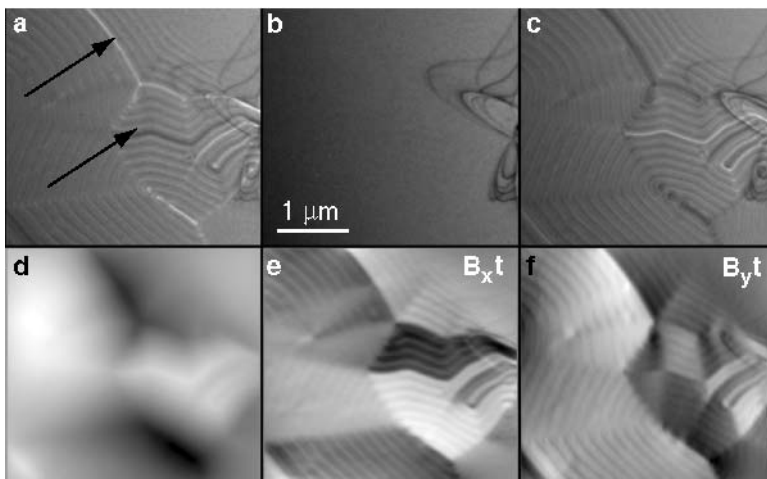
Fig. 8.4. (a–c) Four hundred kilo volt through-focus series of a relatively featureless region in a [001] oriented \text{Ni}_2\text{MnGa} foil; (d) reconstructed phase, and (e–f) are the components of the projected in-plane magnetic induction
