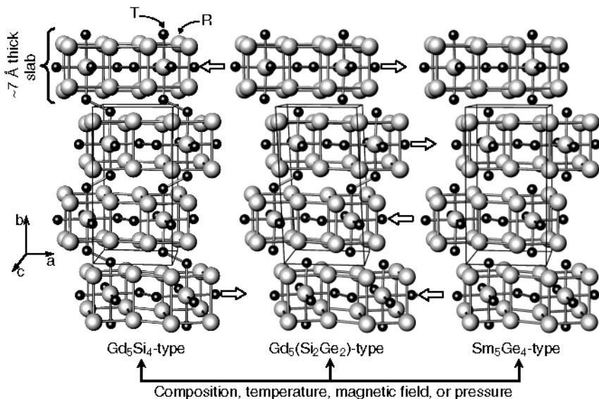
Fig. 11.4. Crystallography of the Gd_5T_4 system: the Gd_5Si_4 -type where all slabs are linked via T-T bonds (the bonding distances shown as T-T dumbbells are \sim 2.5 \text{ \AA} ); the Gd_5(Si_2Ge_2) -type with the slabs connected into pairs, i.e., with half of the interslab T-T bonds broken; and the Sm_5Ge_4 -type where no interslab T-T bonds exist. The interslab T-T distances increase from the bonding \sim 2.5 \text{ \AA} to nonbonding \sim 3.5 \text{ \AA} as the slabs slide by \sim 0.2 to \sim 0.4 \text{ \AA} in the directions indicated by short open arrows. To date, the Gd_5(Si_2Ge_2) -type \leftrightarrow Sm_5Ge_4 -type transitions have been induced only by varying composition; the other two transformations can be triggered by any one or a combination of the listed thermodynamic variables
