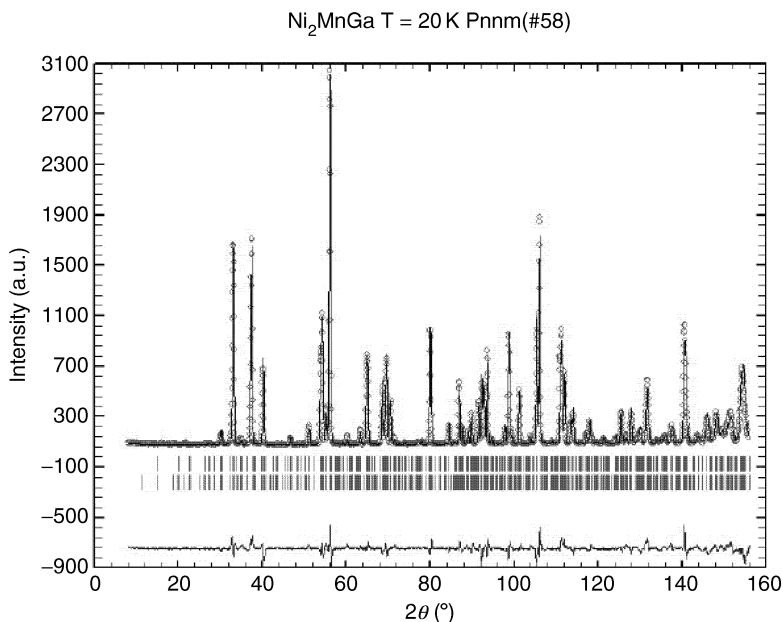
Fig. 7.10. The observed and calculated neutron diffraction patterns of ferromagnetic \text{Ni}_2\text{MnGa} in the transformed phase at 20 K, together with the difference pattern
