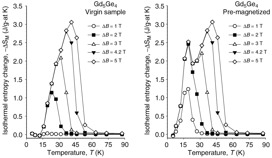
Fig. 11.11. The MCE of Gd 5 Ge 4 calculated using (11.3). The plot on the left is obtained from M(H)_{T=\text{const}} data measured during magnetizing a sample cooled in zero magnetic field from \sim 150 K to each measurement temperature. The plot on the right is for M(H)_{T=\text{const}} data measured after the same sample was magnetized by a 5 T field and then demagnetized
