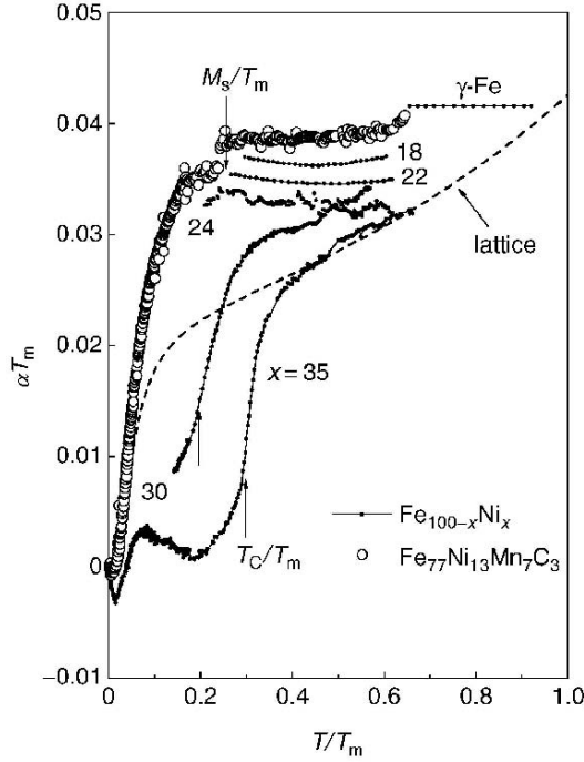
Fig. 10.4. \alpha T_m vs. T_m (melting temperature) for Fe-rich Fe–Ni alloys. The curves for 0 \leq x \leq 30 are measured down to their corresponding martensite start temperatures M_s/T_m . Dashed : lattice reference curve (Grüneisen). Open circles : anti-Invar alloy \text{Fe}_{77}\text{Ni}_{13}\text{Mn}_7\text{C}_3 [17]
