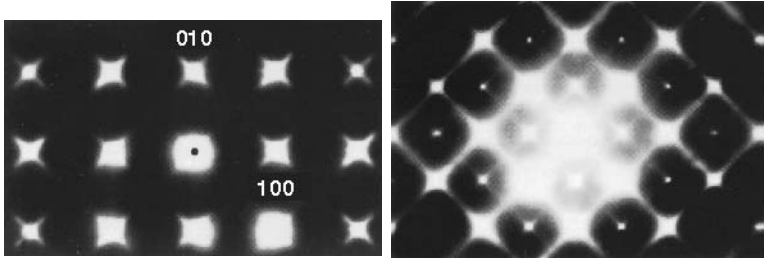
Fig. 3.4. ED pattern of samples with [001] normal of Ni-Al ( left ) and Cu-Zn-Al ( right ). Data from [33]
