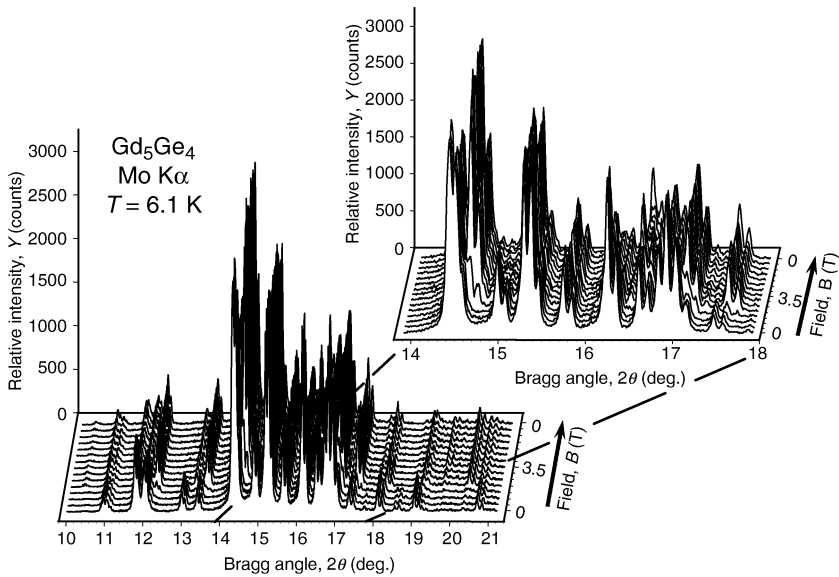
Fig. 11.6. Fragments of the X-ray powder diffraction patterns of \text{Gd}_5\text{Ge}_4 collected at 6.1 K with the magnetic field varying from 0 to 3.5 T and then back to 0 with a 0.5 T step
