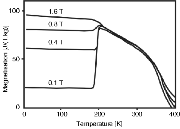
Fig. 7.3. The thermal dependence of the magnetisation of stoichiometric \text{Ni}_2\text{MnGa} measured in different applied fields
