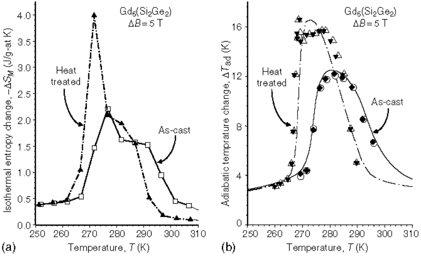
Fig. 11.3. The giant MCE of \text{Gd}_5(\text{Si}_2\text{Ge}_2) in the as-prepared and annealed (1570 K, 1 h) states: (a) -\Delta S_M calculated from magnetization data using Eq. (11.3) [29]; (b) -\Delta T_{ad} calculated from heat capacity data using Eq. (11.2) (lines) and measured directly during increasing (solid symbols) and decreasing (open symbols) magnetic fields [30]
