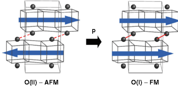
Fig. 4.2. Schematic representation of the crystallographic and magnetic structures of \text{Gd}_5(\text{Si}_{0.1}\text{Ge}_{0.9})_4 in the (a,b) plane at T < T_N . Only the X = \text{Si}, \text{Ge} atoms participating in the X - X covalent-like bonds are depicted as solid spheres . A solid line linking the X atoms represents a formed bond [O(I)] whereas a dashed line is used for a broken one [O(II)]. Solid arrows are used to illustrate the change in the magnetic coupling as a function of magnetic field
