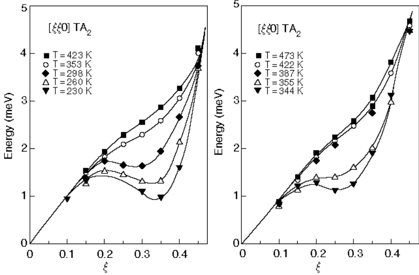
Fig. 3.7. Phonon dip anomaly for \text{Ni}_{52.0}\text{Mn}_{23.0}\text{Ga}_{25.0} (left) and \text{Ni}_{50.5}\text{Mn}_{29.5}\text{Ga}_{20.0} (right) crystals, which transform, respectively, to different modulated structures. Note the difference in the location of the dip. Lines are guides to the eye. Data from [44]
