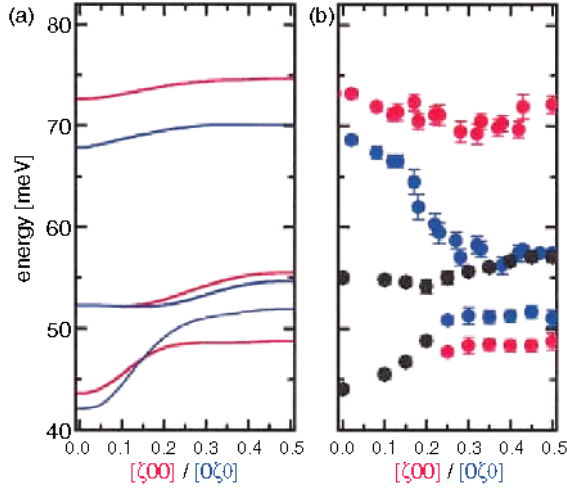
Fig. 6.6. Dispersion curves of the high energy longitudinal phonons in YBCO 0.66 . (a) Calculated curves from an interaction potential mode. The red (blue) curve corresponds to the [\zeta 00] ( [0\zeta 0] ) direction. (b) Measured dispersion curves. Red (blue) correspond to the [\zeta 00] ( [0\zeta 0] ) direction. The black symbols denote phonon peaks where the assignment could not be resolved. From [19]
