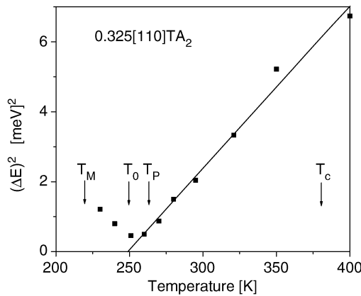
Fig. 7.4. The temperature dependence of the soft mode behaviour of the \text{TA}_2[110] phonon with q = 0.325 . T_M , T_P and T_0 are the martensitic, pre-martensitic and extrapolated transition temperatures
