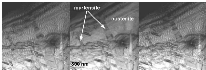
Fig. 8.9. Through-focus series in a two-phase \text{Ni}_{50}\text{Mn}_{29}\text{Ga}_{21} thin foil. The austenite grain, with wavy domain walls, contains several martensite plates ( arrowed )
