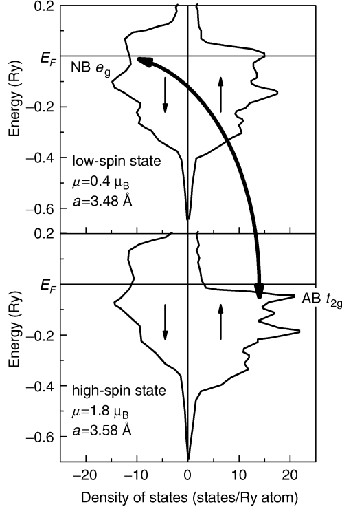
Fig. 10.13. Ab initio calculated electronic density of states for \text{Fe}_{62.5}\text{Ni}_{37.5} in the high-spin and the low-spin state [10,11]. The arrow indicates the t_{2g\uparrow} \rightleftharpoons e_{g\downarrow} transitions possibly taking place at finite temperatures
