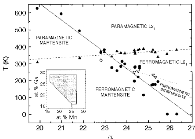
Fig. 6.11. Phase diagram of \text{Ni}_2\text{MnGa} from [25]. The filled circles and filled triangles are the Martensitic and Curie temperatures, respectively. The open triangles represent the transition to the intermediate modulated phase. The hatched region in the inset represents the composition range from which the data have been taken
