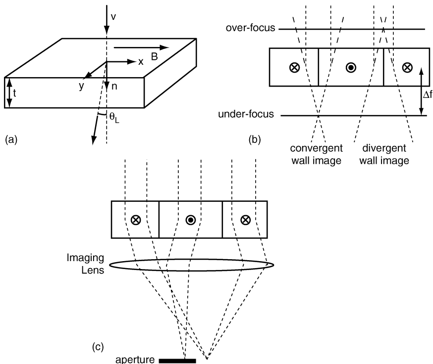
Fig. 8.1. (a) Illustration of a high energy electron traveling through a foil with a permanent magnetic induction; electron trajectories for the Fresnel (out-of-focus) imaging mode (b), and the Foucault mode (c)
