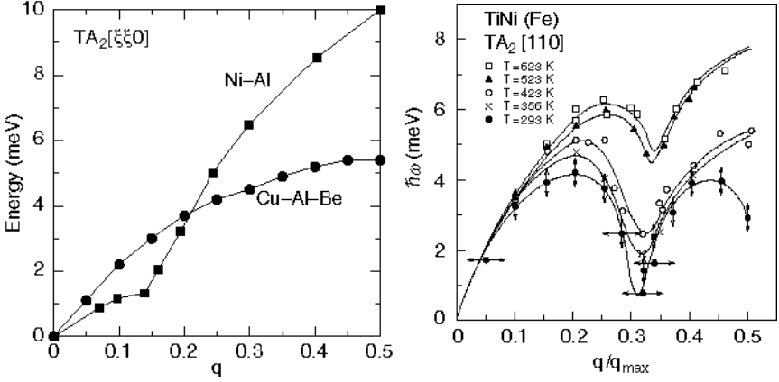
Fig. 3.3. TA_2 phonon branch in Ni_{0.625}Al_{0.375} , Cu_{0.7373}Al_{0.2272}Be_{0.0355} and NiTi (Fe). Right panel shows the temperature softening of the phonon dip anomaly for NiTi (Fe). Lines are guides to the eyes. Data from [26, 27]
