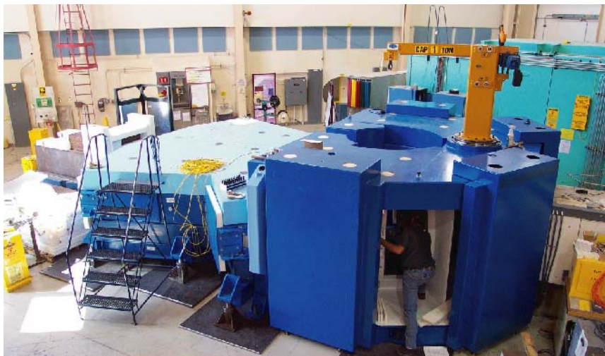
Fig. 5.1. The Neutron Powder Diffractometer (NPDF) of the Lujan Center, Los Alamos National Laboratory, during the upgrading work supported by the National Science Foundation DMR00-76488. A large backscattering detector frame for position-sensitive ^3\text{He} detectors is seen with a technician inside
