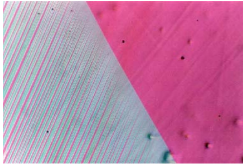
Fig. 9.1. Austenite/martensite interface in the \beta_1 \rightarrow \gamma'_1 transformation of \text{Cu}_{69}\text{Al}_{27.5}\text{Ni}_{13.5} . (Picture courtesy: C. Chu)
