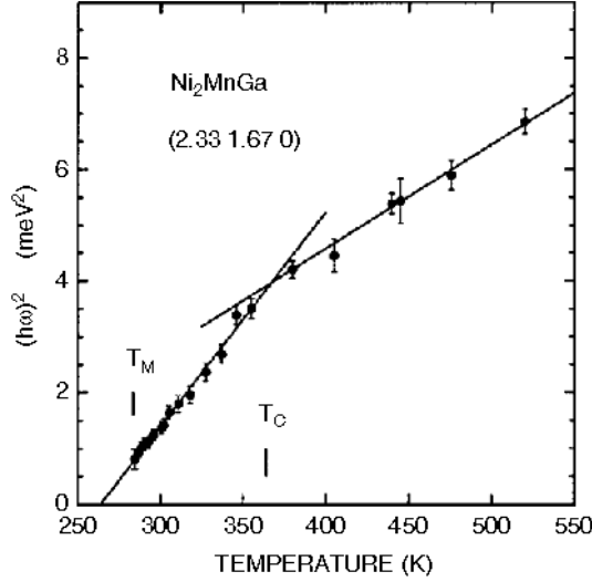
Fig. 6.14. Square of phonon energy of [\zeta\zeta 0] -TA 2 mode, \zeta = 0.33 vs. temperature for \text{Ni}_{2.06}\text{Mn}_{0.94}\text{Ga} . The Curie temperature for this alloy is T_C = 364 K and T_M = 284 K. Data from [28]
