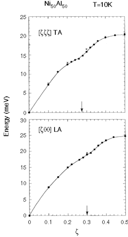
Fig. 6.2. The measured phonon dispersion curve of the [ \zeta\zeta\zeta ]-TA ( top ) and the [ \zeta 00 ]-LA ( bottom ) branch in the \text{Ni}_{50}\text{Al}_{50} alloy. The arrows indicated the predicted q -values of the anomaly by Zhao and Harmon [8]. Data from [7]
