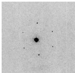
Fig. 7.6. A neutron Laue photograph in the premartensitic phase of \text{Ni}_2\text{MnGa} showing the fundamental -2-20 reflection and the \frac{1}{3}\frac{1}{3}0 satellite reflections
