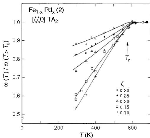
Fig. 6.9. Temperature dependence of the [\zeta\zeta 0] -TA 2 phonons for Fe 72 Pd 28 , normalized by the phonon energy above T_c . Data from [23]
