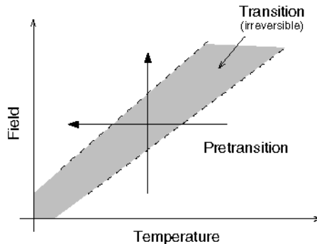
Fig. 3.10. Schematic phase diagram of an extended first-order phase transition as a function of the conjugated field and temperature. Pretranslational and transitional regions are indicated. Arrows denote that the transition can be induced either by cooling or by applying an external field
