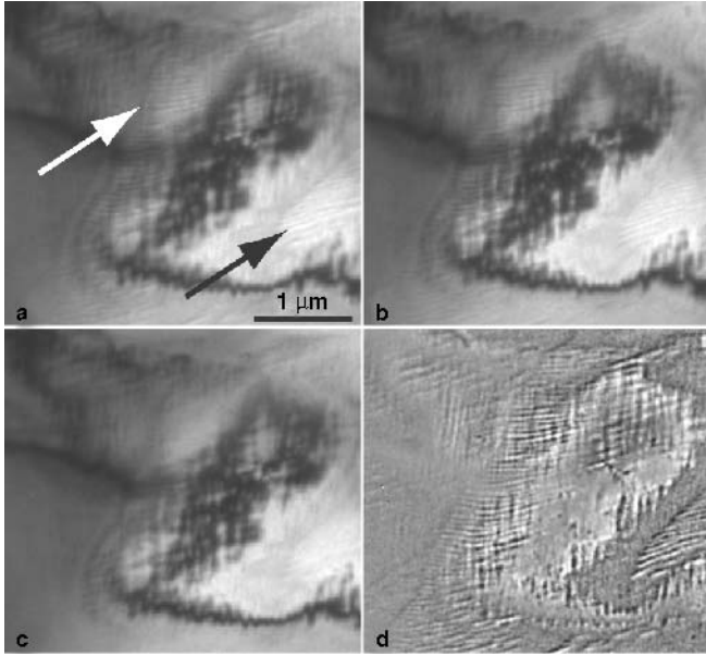
Fig. 8.11. Zero-loss under-focus (a) and over-focus (b) images (Fresnel imaging mode, 400 kV) of a region near a bend contour. The in-focus image (c) shows tweed contrast, and the out-of-focus images reveal the presence of an additional modulated structure ( arrowed ) which is magnetic in nature. (d) shows the difference between (a) and (b), and is proportional to the Laplacian of the phase of the electron wave. Contrast variations in (d) are indicative of magnetic contrast
