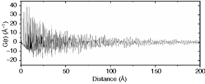
Fig. 5.2. The pair-density function (PDF) of crystalline Ni powder at T = 10 K obtained by the NPDF [13]
