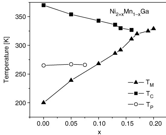
Fig. 7.15. Magnetic phase diagram of \text{Ni}_{2+x}\text{Mn}_{1-x}\text{Ga}
