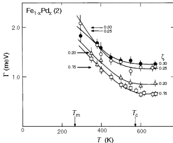
Fig. 6.10. Temperature dependence of the phonon linewidth of the [\zeta\zeta 0] -TA 2 branch for \text{Fe}_{72}\text{Pd}_{28} . Data from [23]
