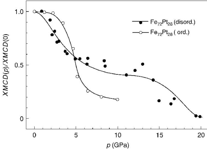
Fig. 10.12. Normalized X-ray magnetic circular dichroism signal, \text{XMCD}(p)/\text{XMCD}(0) , vs. pressure as measured at room temperature for disordered \text{Fe}_{72}\text{Pt}_{28} Invar [28]
