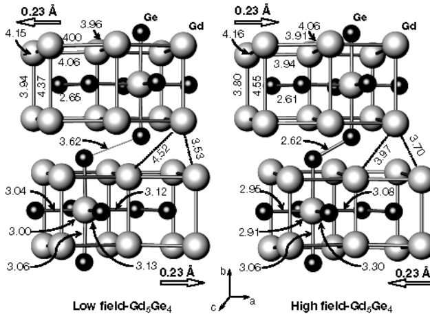
Fig. 11.8. Fragments of the low field (antiferromagnetic) and high field (ferromagnetic) crystal structures of \text{Gd}_5\text{Ge}_4 with selected distances labeled in Å (after [63]). The intraslab distances vary by a maximum of \sim 5\% , while the interslab distances change up to \sim 28\% during the transformation. The open arrows indicate the directions and the magnitudes of the shifts of the slabs during the respective transitions (from low to high field and vice versa)
