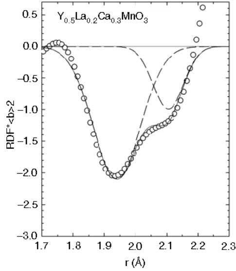
Fig. 5.3. The RDF of \text{Y}_{0.5}\text{La}_{0.2}\text{Ca}_{0.3}\text{MnO}_3 in the range of r from 1.7 to 2.3 Å, showing the peak for the Mn–O bonds, determined by pulsed neutron diffraction [23]. Here the \text{RDF} = 4\pi r^2 \rho(r) , where \rho(r) is the PDF and \langle b \rangle is the composition average of the neutron scattering length. The Mn–O peak can be fit by two sub-peaks corresponding to short and long Mn–O bonds
