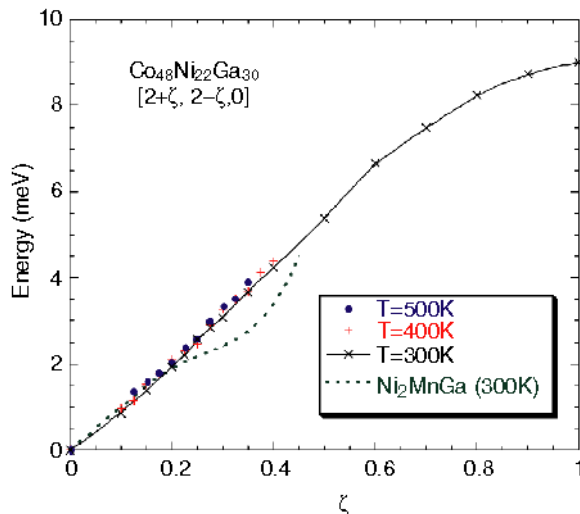
Fig. 6.15. The [\zeta\zeta 0] -TA 2 phonon branch measured in Co 1.92 Ni 0.88 Ga 1.2 at several temperatures within the cubic phase. The dashed line shows the same branch measured in Ni 2 MnGa. Data from [34]
