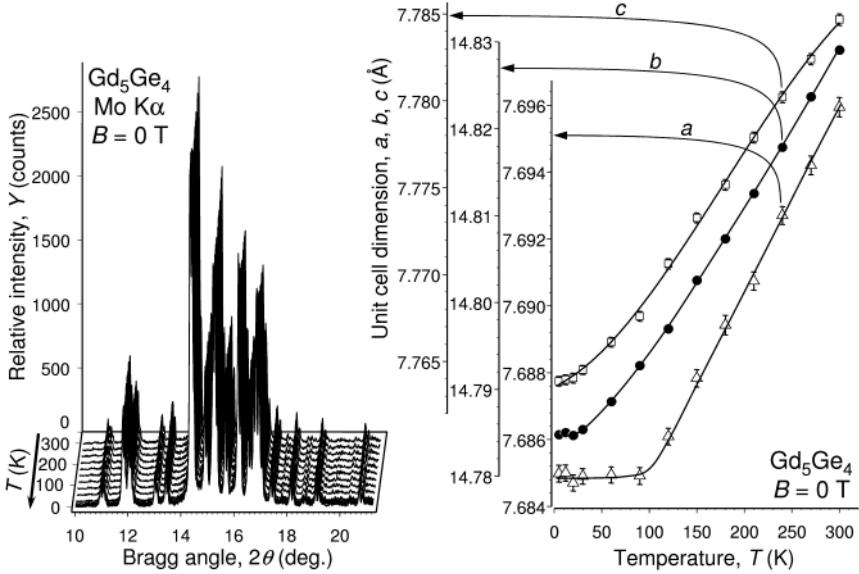
Fig. 11.5. Fragments of X-ray powder diffraction data of \text{Gd}_5\text{Ge}_4 collected using \text{Mo K}\alpha radiation during cooling from 300 to 5 K in a zero magnetic field ( left ) and temperature dependencies of the unit cell dimensions determined from X-ray powder diffraction data ( right ). The lines drawn through the data points on the right are guides to the eye
