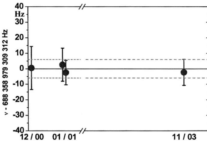
Figure 8-7. Frequency measurements of laser-cooled \text{Yb}^+ optical frequency standards over the past three years. The first three data points represent published data from Reference [41].
