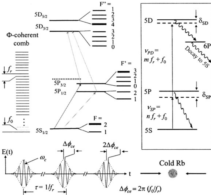
Figure 1-4. Top: Schematic of the relevant energy levels of the ^{87}\text{Rb} atom and the frequency-domain perspective of the atom-light interaction. Bottom: Time-domain picture showing a sequence of mode-locked pulses, with the relevant interaction parameters in f_r and \Delta\phi_{ce} . The inset at right shows the relevant “three-level” model used for construction of the Bloch equations to solve for population-transfer dynamics. An example for the on-resonance, stepwise transition is shown with relevant detunings at \delta_{SP} and \delta_{SD} for the pair of comb modes that make the dominant contribution to the transition probability amplitude.
