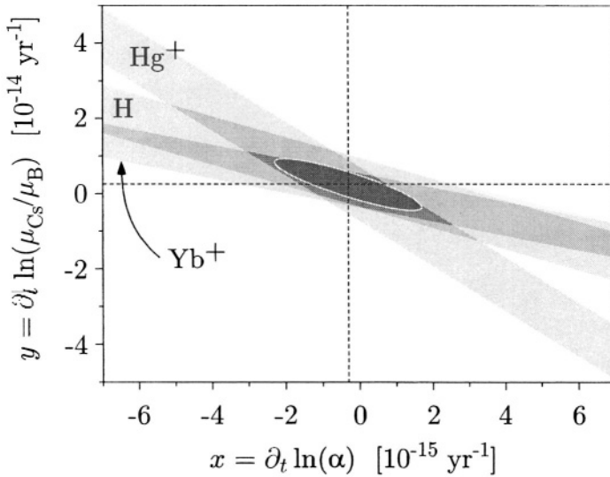
Figure 7-9. Combining the drift rates of optical transitions in hydrogen, \text{Hg}^+ and \text{Yb}^+ . The experimentally allowed region for the drift rates of \alpha and \mu_{\text{Cs}}/\mu_{\text{B}} is shown in the form of an ellipse.
