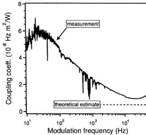
Figure 5-9. Transfer function of laser intensity noise into fluctuations of the CEO frequency [16]. These measurements were done in a prismless laser in the absence of spectral shifting. The measurements reflect Kerr contributions to the APC and thermally induced amplitude-to-phase conversion (APC) effects at low frequencies.
