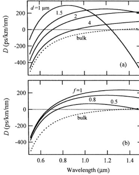
Figure 4-3. Plots of the group-velocity-dispersion parameter D for (a) various values of the diameters d and an air-filling fraction f= 1 and (b) various values of f for a core diameter d = 1.7 . The dashed line represents the dispersion curve for bulk-fused-silica glass.
