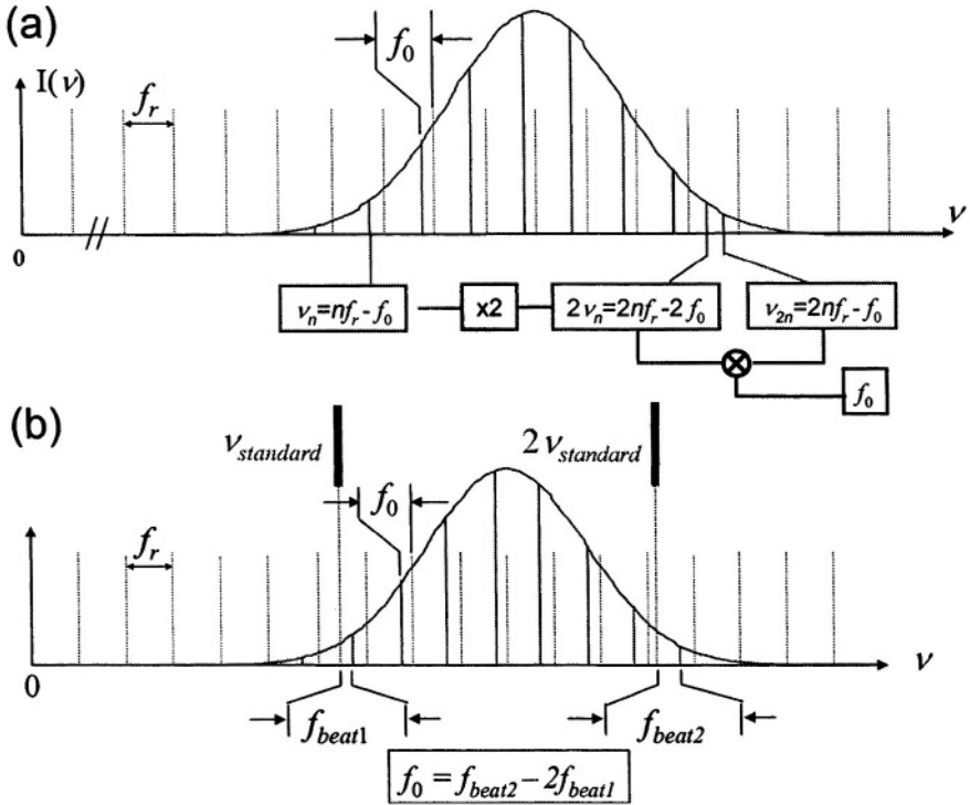
Figure 1-2. Two equivalent schemes for the measurement of f_0 using an octave-spanning optical frequency comb. In the self-referencing approach, shown in (a), frequency doubling and comparison are accomplished with the comb itself. In the second approach shown in (b), the fundamental frequency ( \nu_{\text{standard}} ) and its second harmonic of a cw optical standard are used to determine f_0 . These two basic schemes are employed for absolute optical frequency measurement and implementation of optical atomic clocks.
