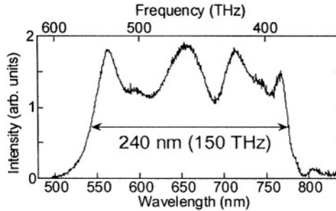
Figure 6-19. Spectrum of the signal pulses under a full-bandwidth operation.
