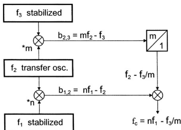
Figure 8-8. Using an intermediate oscillator in the transfer mode. The signal f_c is independent from f_2 .
