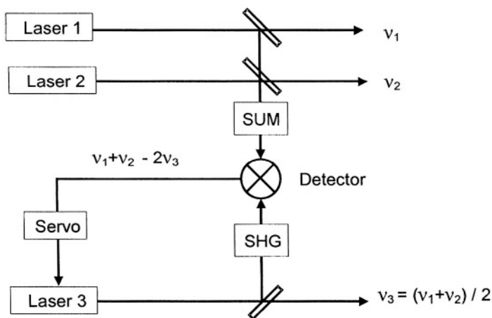
Figure 8-3. Diagram of an optical difference-frequency divider for frequency-interval bisection (adapted from Reference [6]).
