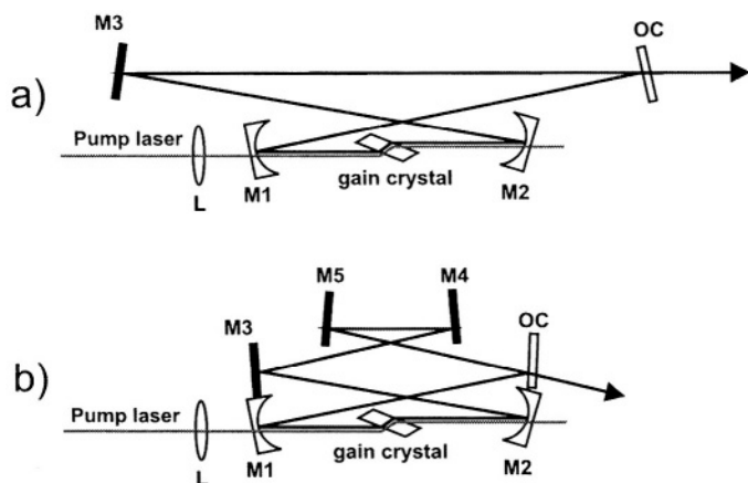
Figure 3-2. (a) Four-mirror cavity with the gain crystal enclosed by focusing mirrors M1 and M2. The flat mirror M3 and the output coupler (OC) form the collimated part of the cavity. The pump light enters the crystal through lens L and M1. (b) Equivalent to (a) but with extra folding using flat mirrors M4 and M5.
