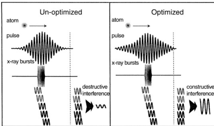
Figure 11-1. Illustration of intra-atomic phase matching. When the optimized pulse shape is used, a particular harmonic constructively adds over each half cycle (from [9]).
