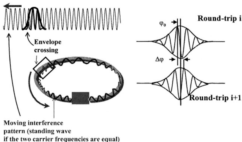
Figure 12-3. Topological representation of a mode-locked ring laser. The pulse envelopes overlap at the same location of the cavity at each round trip.
