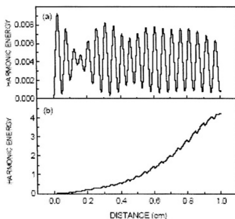
Figure 11-5. (a) Calculation of the signal of the 95th harmonic for a straight waveguide as a function of propagation distance. (b) Calculation for a 0.5 mm period modulated waveguide (from [11]).
