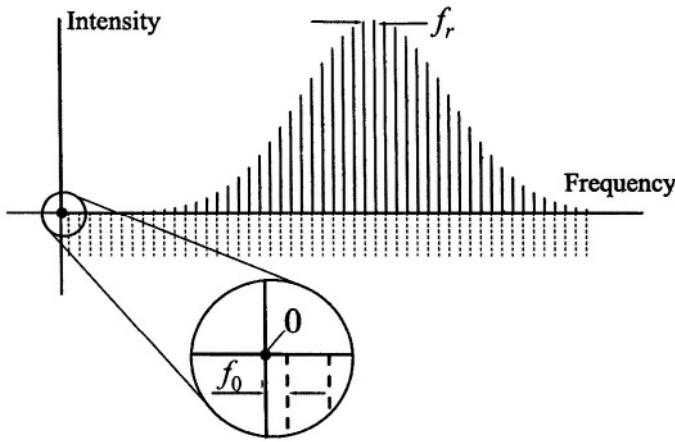
Figure 5-2. Equidistant frequency comb of a mode-locked laser. The comb lines are spaced by the repetition rate f_r and exhibit a nonvanishing offset frequency f_0 at zero frequency unless the electric-field pattern exactly reproduces from pulse to pulse (compare to the time domain picture in Figure 5-1).
