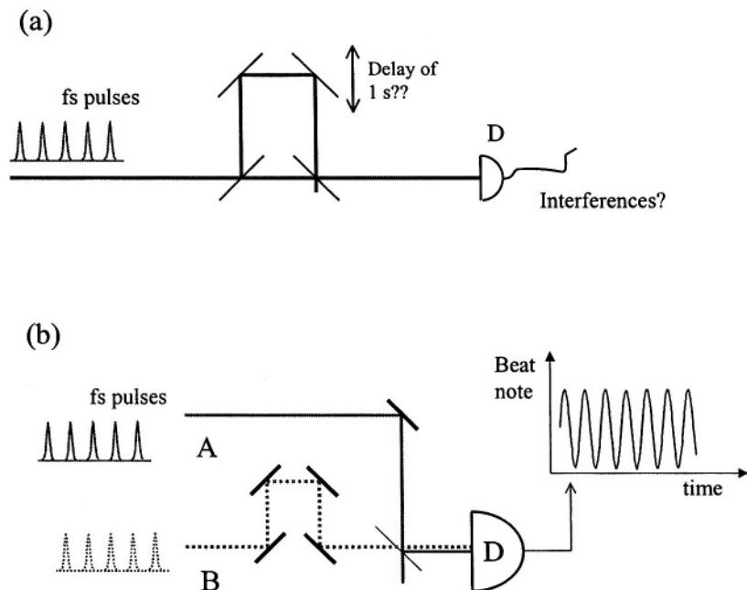
Figure 12-1. Coherence measured by a Mach-Zehnder interferometer. (a) In the case of a regular pulse train, by providing the near perfect frequency comb as discussed in previous chapters, interferences could be observed even in a delay of the interferometer approaching 1 s, or 14 orders of magnitude larger than the pulse duration. (b) The coherence of an unknown source A can be measured by optical beating with a reference source B, provided both sources have the same repetition rate. An optical delay is required to ensure that the pulse of each train interfere at detection.
