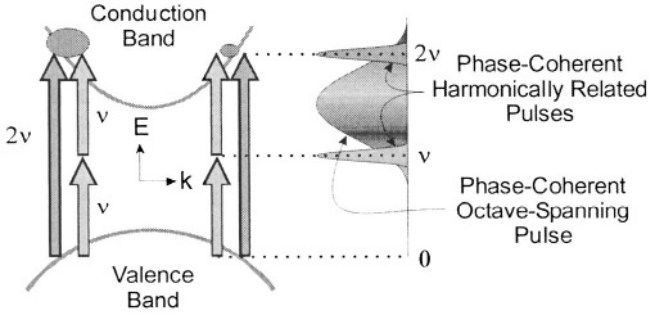
Figure 1-8. Conceptual diagram of quantum interference between one- and two-photon absorption in a direct-gap semiconductor. The two interfering absorption pathways are driven by the spectral wings of a single octave-spanning pulse. An imbalance in the otherwise symmetric carrier-population distribution in momentum space (represented by ovals) occurs due to interference and results in a net current. The resulting photocurrent is sensitive to \phi_{ce} .
