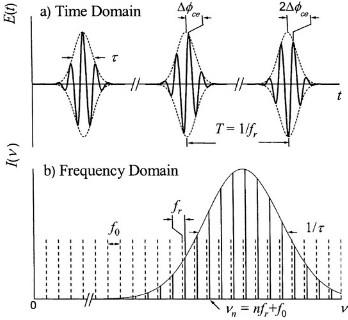
Figure 1-1. Summary of the time-frequency correspondence for a pulse train with evolving carrier-envelope phase.
