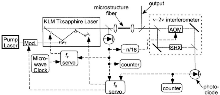
Figure 1-3. Schematic of a femtosecond comb generator. AOM: acousto-optic modulator; SHX: second-harmonic-generation crystal.
