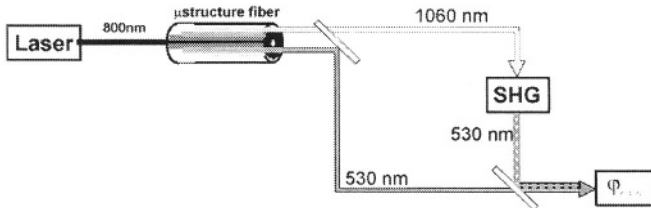
Figure 5-6. Schematic drawing of a practical implementation of Equation (6) and Figure 5-4. The laser is spectrally broadened to more than an optical octave using continuum generation in a microstructure fiber. Two wavelengths forming one octave are separated. The long-wavelength component is frequency doubled and heterodyned with the fundamental signal. The beat note contains an rf component at the CEO frequency. Specific wavelengths shown are meant as example values.
