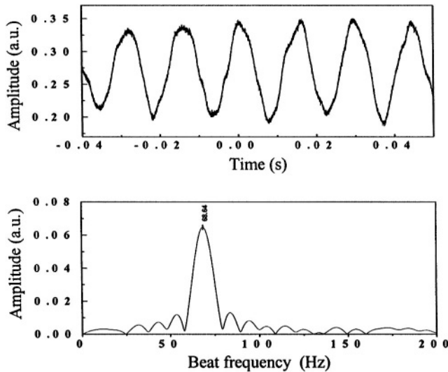
Figure 12-6. Beat frequency (a) taken by a sensitive InGaAs detector (D in Figure 12-5) and (b) its Fourier transform.
