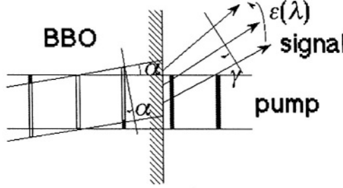
Figure 6-13. Schematic of the noncollinear interaction between the pump pulse and signal pulse. The crystal is on the left side. The volumes occupied by the pump pulse are shown by rectangular shapes elongated perpendicular to the propagation direction. Those for probe pulse are shown by closed gray rectangles. The gain volume introduced by the pump pulse causes the tilting of the wave front of the signal pulse by \alpha in the crystal, resulting in the spectral and angular dispersions of the exiting signal pulse.
