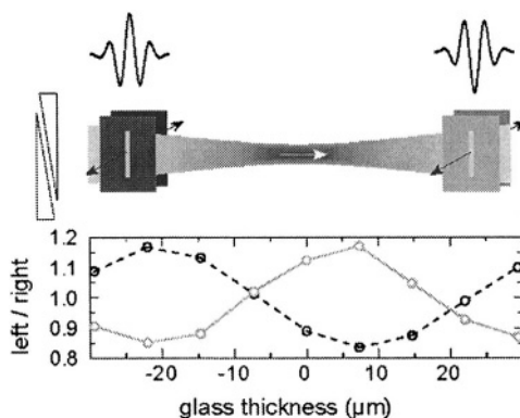
Figure 10-15. Variation of glass thickness in the beam path to change the carrier-envelope phase of the pulses. The left/right ratio of the electron yield exhibits clear oscillations with a periodicity consistent with glass dispersion at the wavelength of the laser. The measurement was performed before (dashed line) and after (solid line) the focus. The \pi phase shift is due to the Gouy carrier-envelope phase shift resulting from the passage through the focus.
