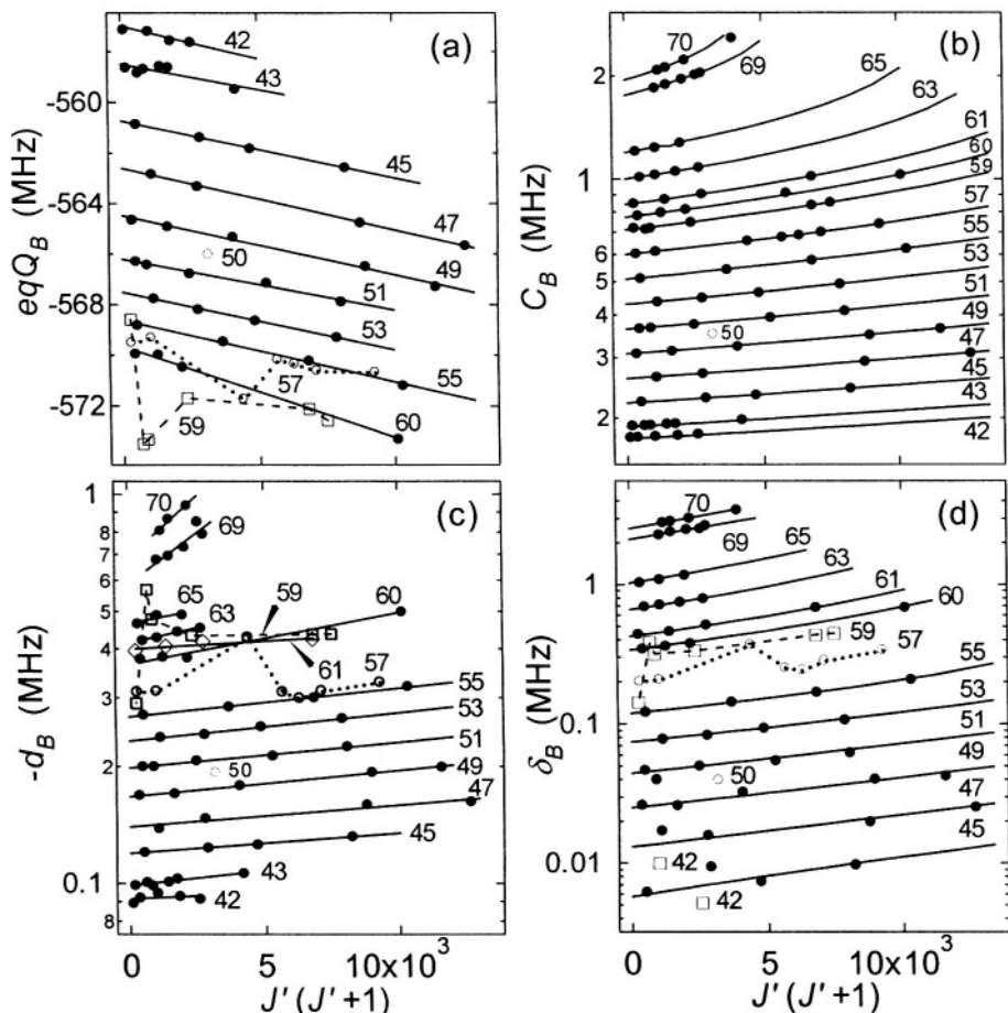
Figure 1-6. Rovibrational dependence of the B-state hyperfine parameters: (a) eqQ_B , (b) C_B , (c) d_B , and (d) \delta_B . Graphs (b), (c), and (d) are semilog plots and the vertical scale of (c) has been inverted. Each solid line is a fit for J -dependence for each vibrational level ( \nu' indicated in the figure). Experimental data in squares and open circles show abnormal variations of eqQ_B , d_B , and \delta_B around \nu' = 57 and 59 .
