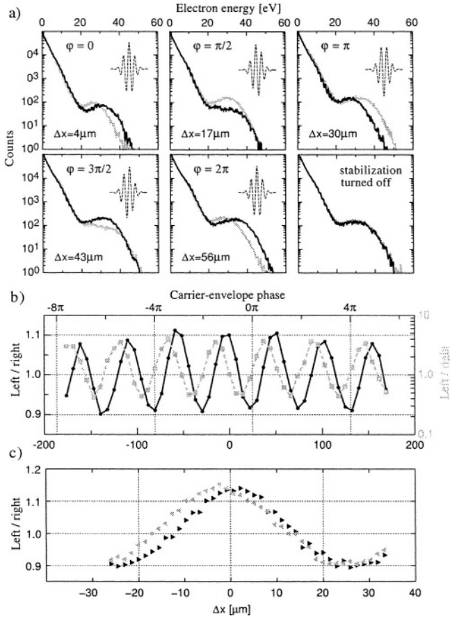
Figure 10-13. (a) Photoelectron spectra for different CE phases controlled by fine movement of one of the wedges. \Delta x indicates the glass added hereby. The black curves correspond to emission to the right (positive direction), the gray ones to the opposite direction. The insets show the corresponding real time variation of the electric field, as deduced from the phase assignment shown in Figure 10-14. Only without phase stabilization were identical spectra measured to both left and right as expected. (b) Left-right ratio of the total electron yield (solid black curve) and high-energy electrons (dashed gray curve) as a function of glass thickness \Delta x added or subtracted by moving one of the wedges. \Delta x = 0 corresponds to optimal dispersion compensation, i.e., the shortest pulses. Maximal left/right ratio for the total yield does not coincide with that for high-energy electrons. Note the different scales for low- and high-energy electrons. The upper horizontal scale indicates the CE envelope phase of the pulse, as deduced from the comparison with theory shown in Figure 10-14. (c) Fine-increment phase scan indicating long-term CE phase stabilization drift of the laser setup. The measurement was performed over \geq 10 min by slowly scanning the wedges forth (triangles pointing to the right) and back (triangles pointing to the left) using a fine increment of the glass thickness. The mismatch at the start and the end indicates a phase drift of \sim 50 mrad/min.
