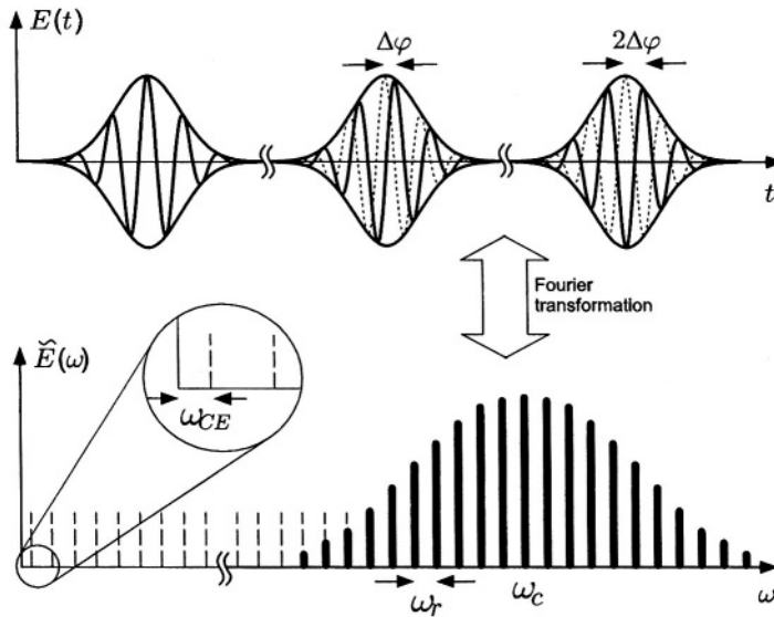
Figure 7-1. Three consecutive pulses of the pulse train emitted by a mode-locked laser and the corresponding spectrum. The pulse-to-pulse phase shift \Delta\phi results in an offset frequency \omega_{CE} = \Delta\phi/T because the optical carrier wave at \omega_c moves with the phase velocity while the envelope moves with the group velocity.
