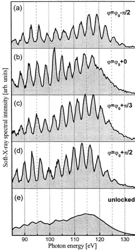
Figure 10-9. Measured spectral intensity of soft x-ray emission from ionizing atoms driven by 5 fs pulses. (a)–(d) Data obtained with phase-stabilized pulses for different carrier-envelope-phase settings are shown. (e) Spectrum measured without carrier-envelope-phase stabilization. X-ray CCD exposure was 0.5 s in all cases.
