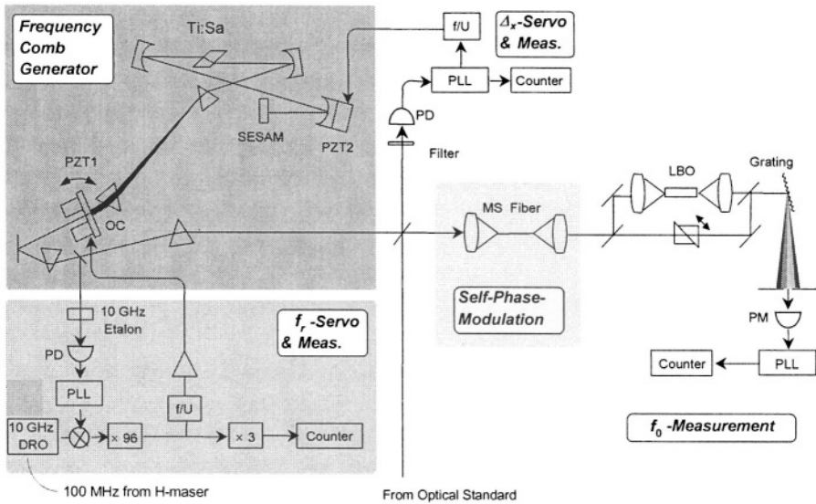
Figure 8-5. Femtosecond laser as frequency comb generator and generated comb spectrum. LBO: Lithium \beta -Borate crystal and SESAM: Semiconductor Saturable Absorber Mirror.
