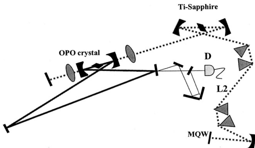
Figure 12-5. Illustration of the intracavity optical parametric oscillator (OPO) pumped by the Ti:sapphire laser. Four LaKL21 prisms are incorporated in the pump cavity to compensate for the group-velocity dispersion (GVD) from the Ti:sapphire crystal, the Periodically Poled Lithium Niobate (PPLN) crystal, and other intracavity elements such as lenses and mirrors. This four-prisms configuration was necessitated by the desire to have large GVD compensation (needed because of the large positive GVD of \text{LiNbO}_3 ) and a reasonably short cavity length ( 1/2 of the perimeter of the OPO cavity). The main control of the GVD compensation is the prism spacing L2. Two quantum wells (MQW) of AlGaAs on top of a mirror structure are used in the cavity as a saturable absorber to mode lock the laser.
