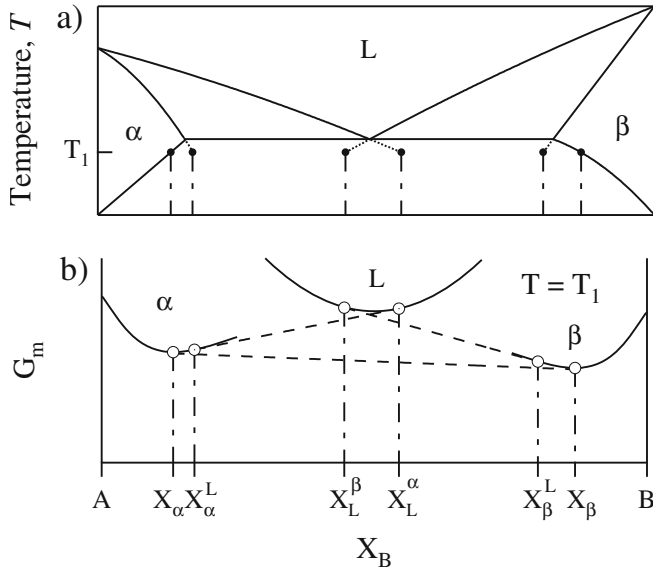
Fig. 4. Schematic phase diagram (a) and free energy vs. composition diagram (b) for a binary alloy that exhibits a eutectic reaction: L \rightarrow \alpha + \beta . The relationship between the phase boundaries in the phase diagram and the common tangents is illustrated for a temperature T_1 where both a stable \alpha + \beta and the metastable L + \alpha and L + \beta two-phase equilibria could occur for different kinetic conditions.
