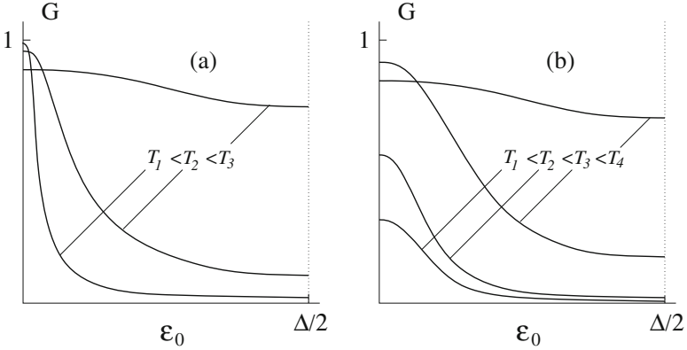
Fig. 4. Weak barriers: Conductance G (in units of e^2/h ) as a function of \epsilon_0 for symmetric (a) and asymmetric (b) barriers
