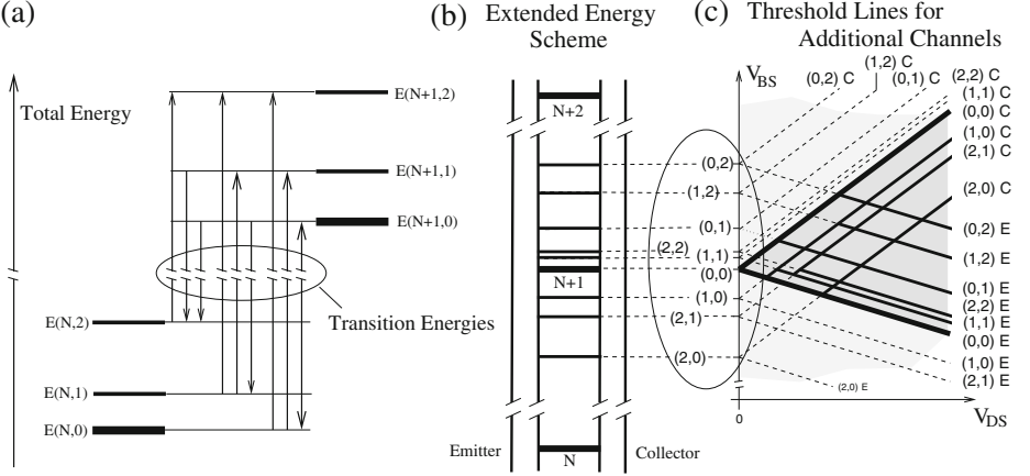
Fig. 9. (a) Fictitious total energy spectra of N and N + 1 electrons confined in the quantum dot. Bold are the groundstate energies. (b) Plot of the transition energies E(n, k; \{V_i\}) - E(n - 1, l; \{V_i\}) as energy levels. Energy levels representing differences between groundstate energies are bold and marked the respective n \in \{\dots, N - 1, N, N + 1, \dots\} . (b) Threshold lines for additional channels extracted from (a). Whether all are visible depends in detail on (quasi-)selection rules and the dynamic of the system.
