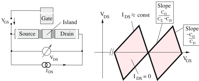
Fig. 11. SET as voltage signal amplifier.
