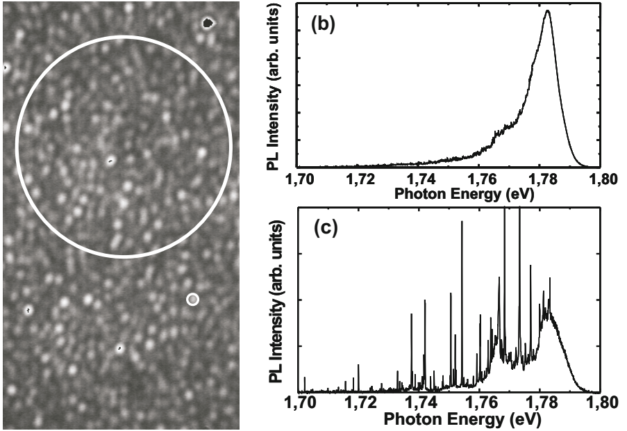
Fig. 3. (a) \mu -PL image of a type-II GaAs/AlAs quantum well showing local type-I band alignment. (b) macro-PL and (c) \mu -PL of the sample [11]
