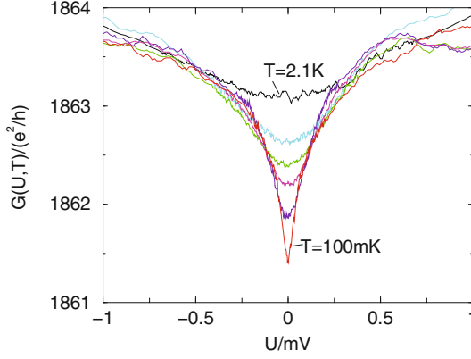
Fig. 14. Raw data of the differential conductance as a function of voltage for different temperatures. For lower temperatures, a narrow anomaly occurs, which is due to interaction effects
