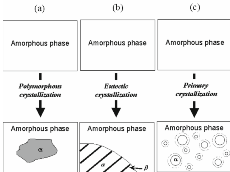
Fig. 17. Schematic illustration of the characteristic microstructural morphologies that develop during nanocrystallization by (a) polymorphic, (b) eutectic, and (c) primary phase reactions. In (c) the dotted curve around primary phase nanocrystals denotes the extent of the solute diffusion field.
