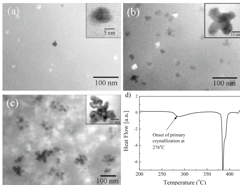
Fig. 19. TEM bright-field images from an \text{Al}_{88}\text{Y}_7\text{Fe}_5 melt-spun ribbon that was isothermally annealed at 245°C for (a) ten minutes; (b) 30 minutes; (c) 100 minutes and (d) continuous heating DSC trace at 40 K/min showing a primary crystallization onset at 276°C.
