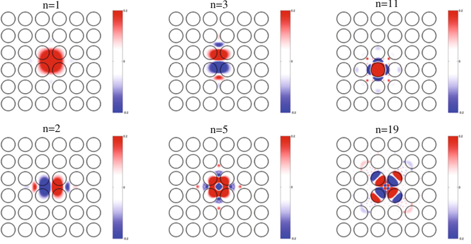
Fig. 3. Photonic Wannier functions, W_{n0}(\mathbf{r}) , for the six bands that are most relevant for the description of the localized defect mode shown in Fig. 4b. These optimally localized Wannier functions have been obtained by minimizing the corresponding spread functional, (28). Note, that in contrast to the other bands, the Wannier center of the eleventh band is located at the center of the air pore. The parameters of the underlying PBG material are the same as those in Fig. 1
