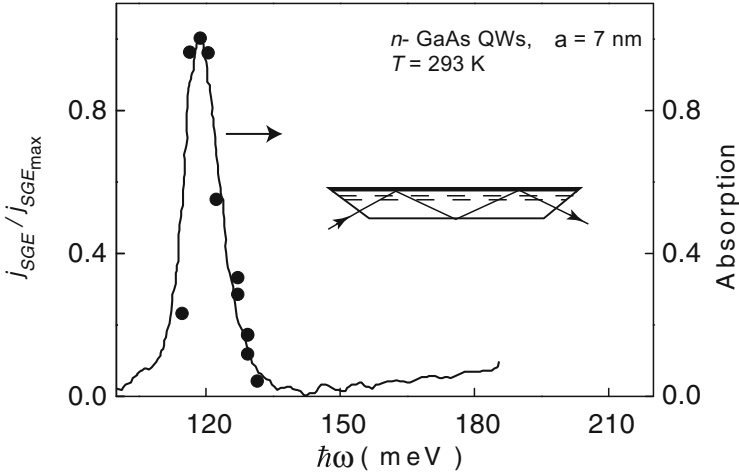
Fig. 6. Absorption spectrum (full line) of an n -doped (001)-grown GaAs/AlGaAs MQW structure ( a = 70 \text{ \AA} ) obtained from transmission in a multiple-reflection waveguide geometry, see the inset. Points show spectral dependence of the spin-galvanic current caused by spin orientation due to direct optical transitions between e1 and e2 conduction subbands [16]
