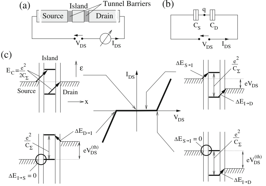
Fig. 2. (a) Two-terminal arrangement for discussing the Coulomb blockade effect in electrical transport. (b) The respective capacitance circuit. Note C_{\Sigma} = C_S + C_D . (c) Sketch of the expected non-linear I_{DS}(V_{DS}) characteristic with energy schemes for distinct V_{DS} values reflecting the energetical position of the Fermi levels of the island for charge states q = -e and q = e relatively to the Fermi level of source and drain.
