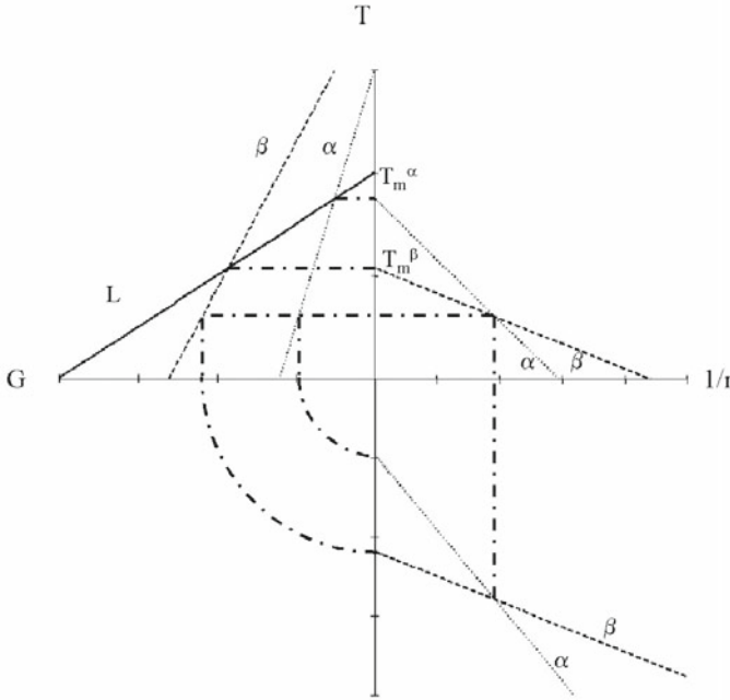
Fig. 9. Schematic illustration of the influence of curvature ( 1/r ) on the melting point of the \alpha phase and the \beta phase and on the relative phase stability when \sigma_\alpha L V_M / \Delta S_{\alpha f} > \sigma_\beta L V_M / \Delta S_{\beta f} .
