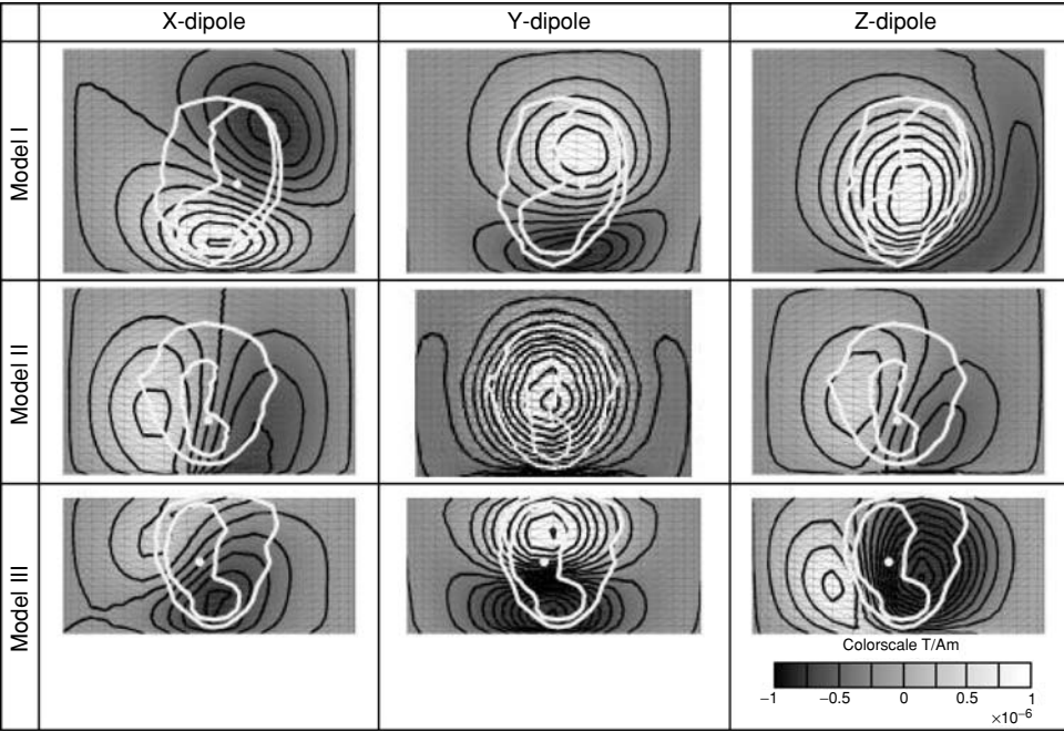
Figure 18. The distribution of the z-component of the magnetic field due to a dipole in the x, y or z direction. Models are shown in Fig. 17.
