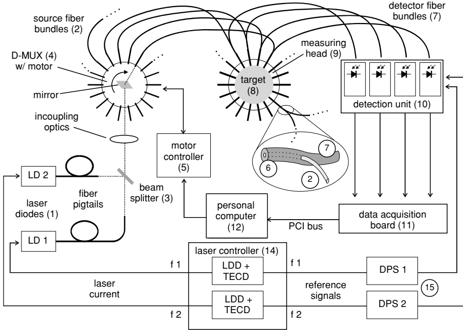
Figure 5. A continuous wave instrument with time-multiplexed source fibers. LDD = laser diode driver, TECD = thermoelectric cooling driver, f1, f2: laser diode modulation frequencies, LD1, LD2: laser diodes, D-MUX: optical demultiplexer, DPS1, DPS2: digital phase shifters. Reproduced with permission from (Schmitz et al., 2002).
