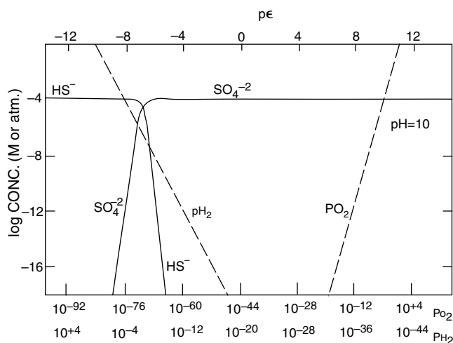
FIGURE 8 Equilibrium distribution of sulfur compounds as a function of p\epsilon at pH = 10 and 25^\circ C . Total concentration is 10^{-4} M. The dotted curve shows that solid sulphur cannot exist thermodynamically at pH = 10 , since its activity never becomes unity. Figure from Stumm, W. and J. Morgan, Aquatic Chemistry , Wiley-Interscience, New York, 1970, p. 311.
