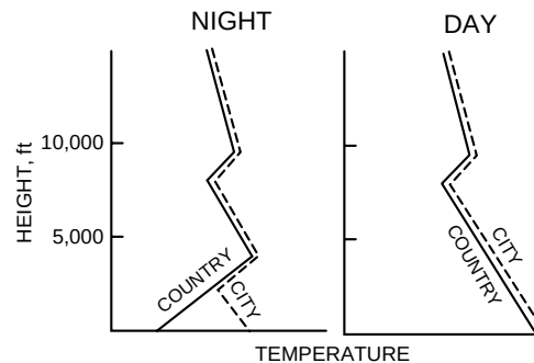
FIGURE 5 Vertical temperature distribution (schematic) over city and country, day and night.
