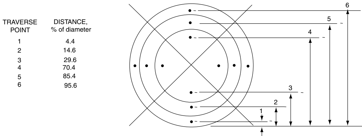
FIGURE 2 Example showing circular stack cross section divided into 12 equal areas, with location of traverse points indicated.
