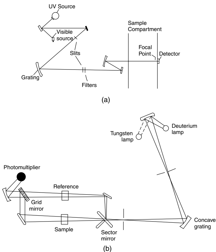
FIGURE 9 Single- and double-beam uv-visible spectrophotometers. (a) Beckman DU R Series 60, single-beam. (Courtesy of Beckman Instruments, Inc., Fullerton, CA.) (b) Hitachi Model 100-60, double-beam. (Courtesy of Hitachi Instruments, Inc., Danbury, CT.)
