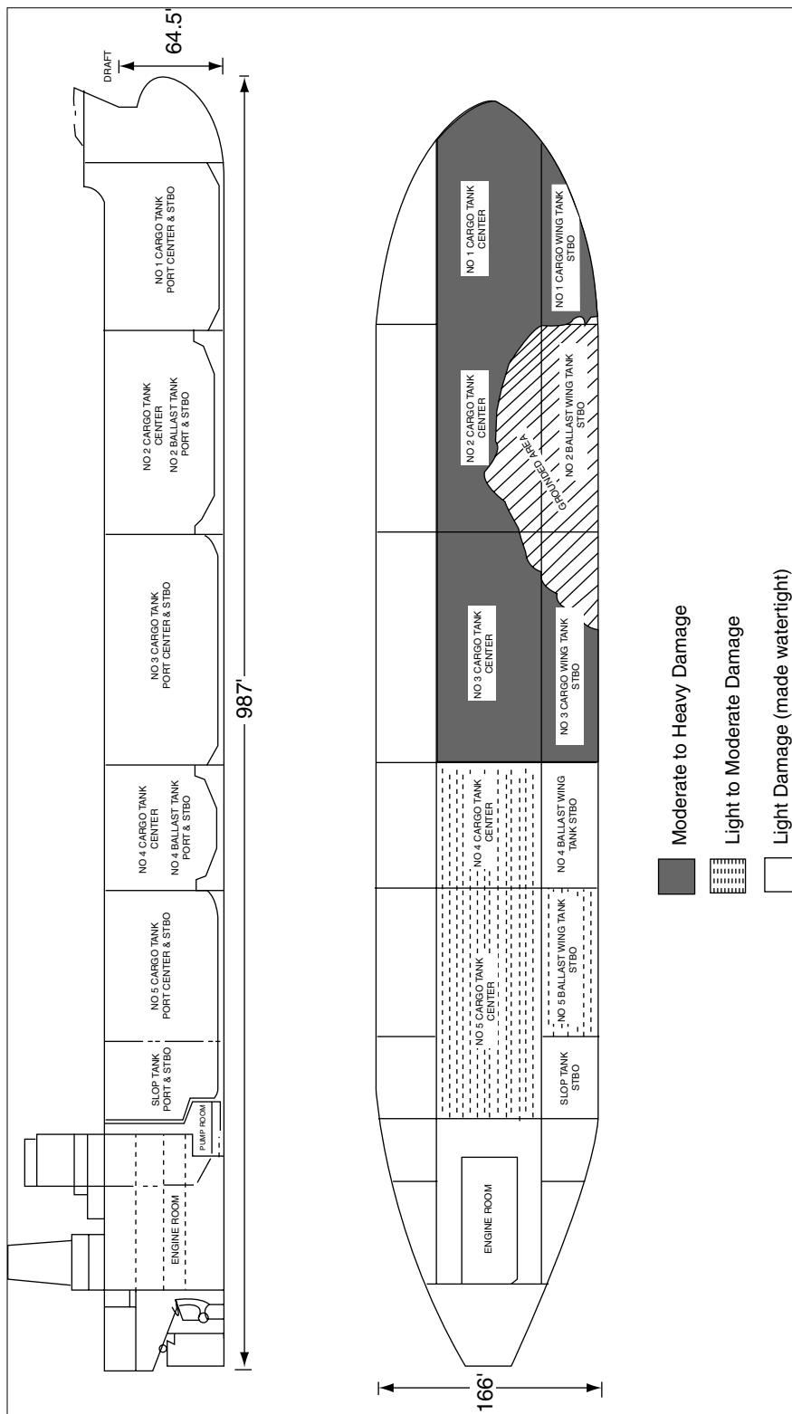
FIGURE 6 Estimated grounding damage to the EXXON VALDEZ. Permission for use granted by Exxon Corporation, Houston, Texas.
