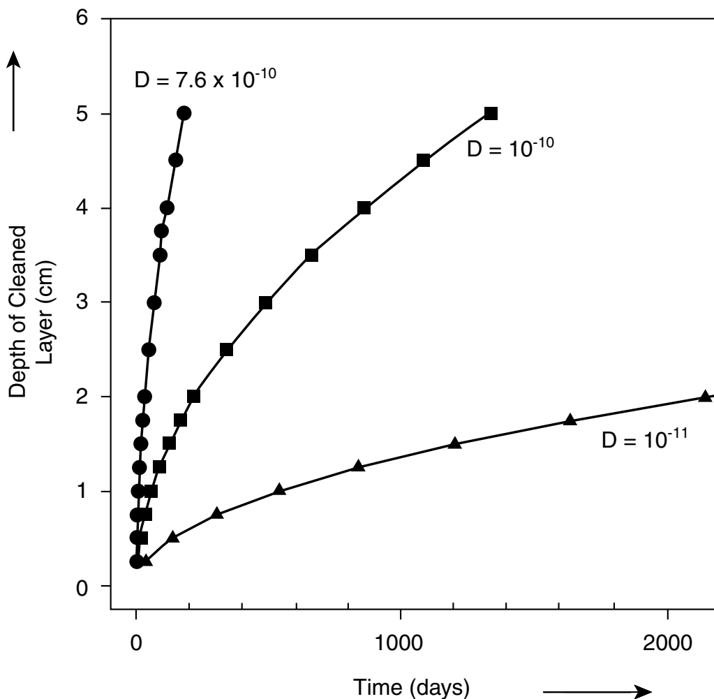
FIGURE 43 Correlations between the depth of the cleaned layer and the time to reach 50 ppm PCB in the bulk retrofill fluid.
