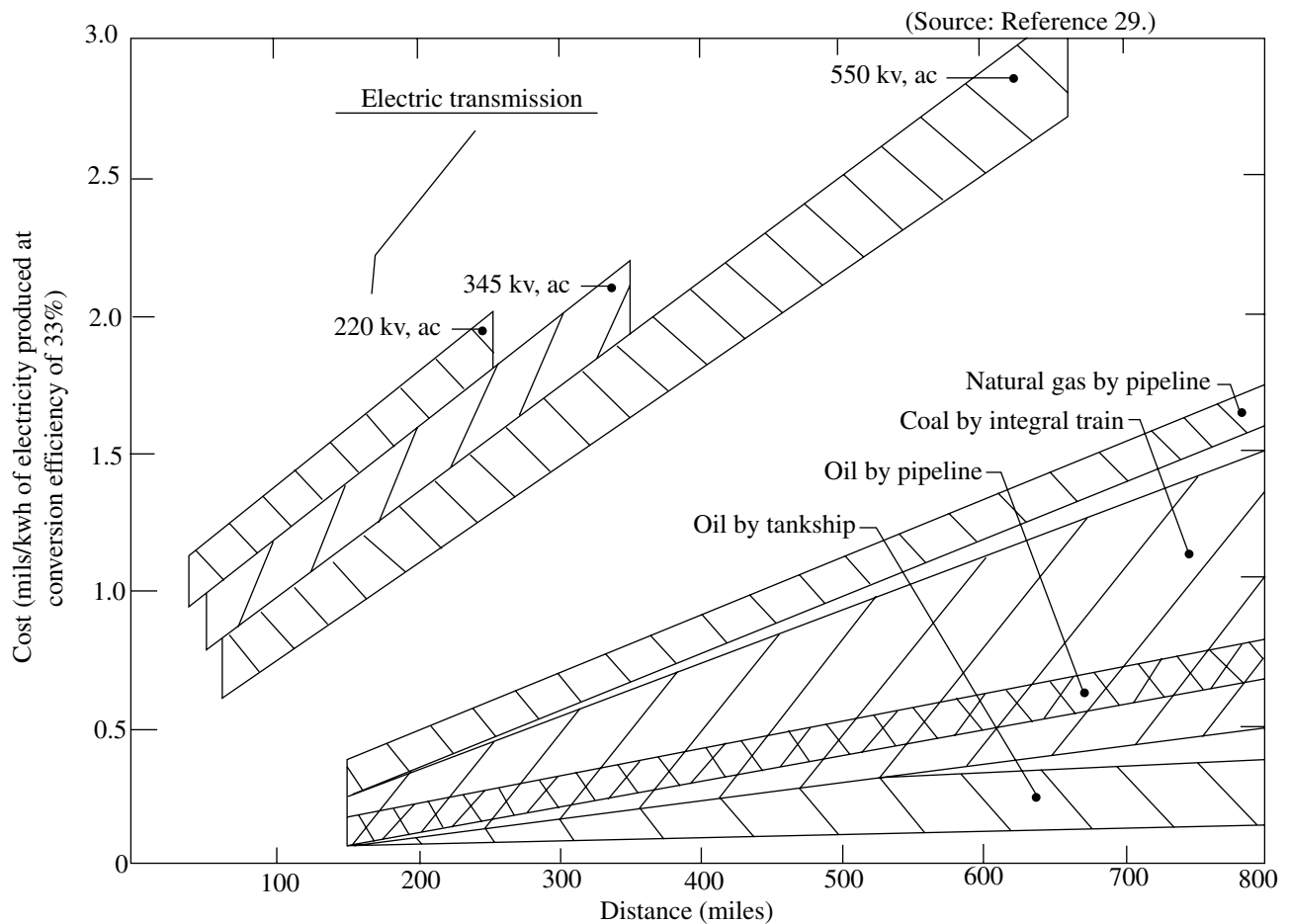
FIGURE 4 Portion of central station electric cost attributable to the transportation of energy.
