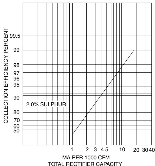
FIGURE 7 Precipitator design curve.
