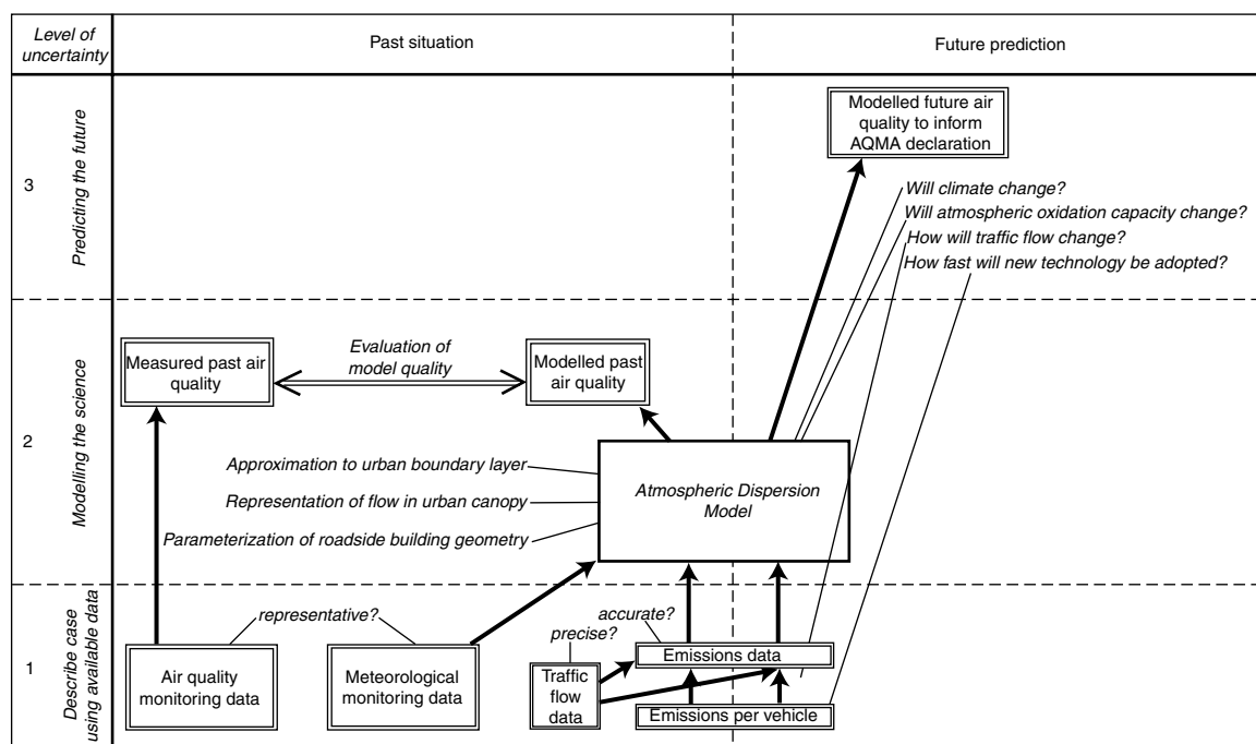
FIGURE 1 Schematic diagram showing flow of data into and out of the atmospheric dispersion model, and three categories of uncertainty that can be introduced (From Colville et al., 2002, with permission from Elsevier).
