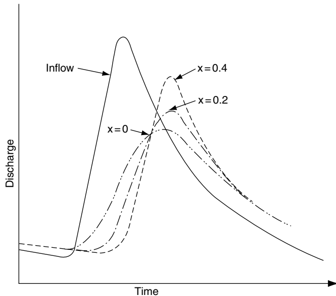
FIGURE 6 Muskingum routing: to illustrate the influence of x on outflow hydrograph (after Linsey 2 ).
