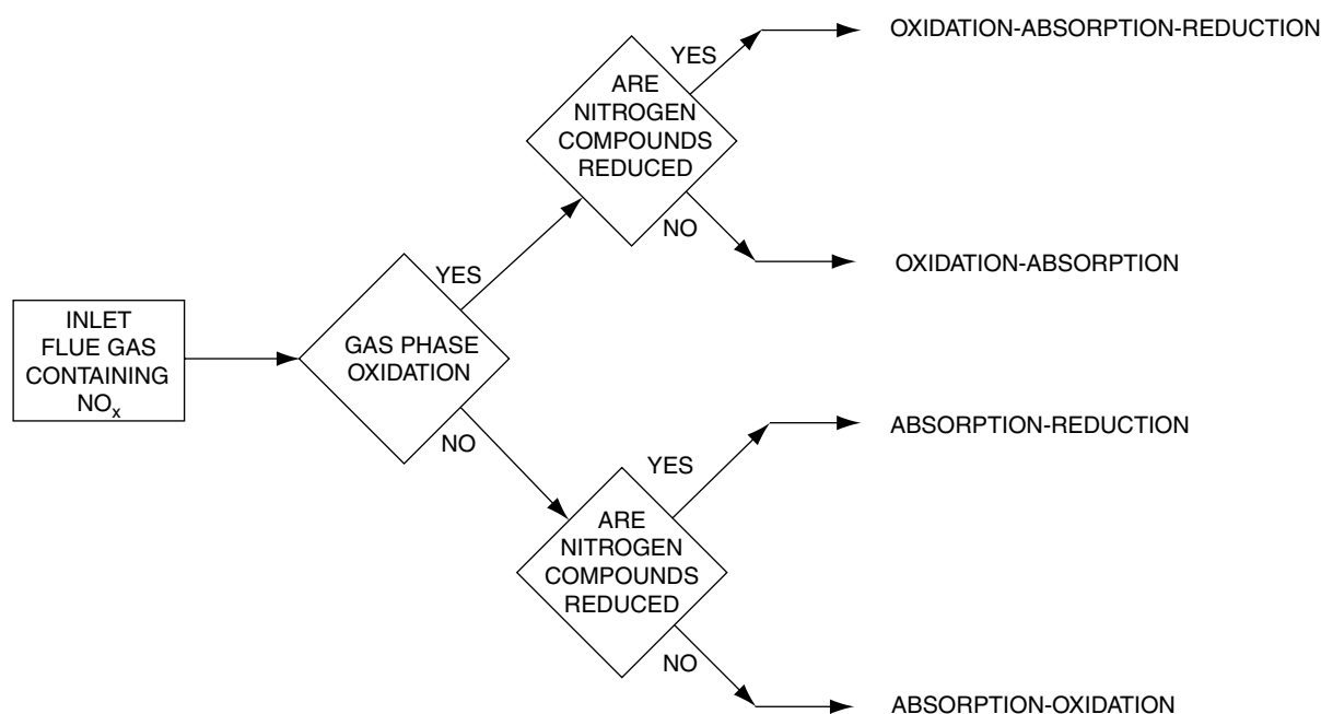
FIGURE 20 Classification system for wet NO x removal processes (Fawcett et al. , 1977).
