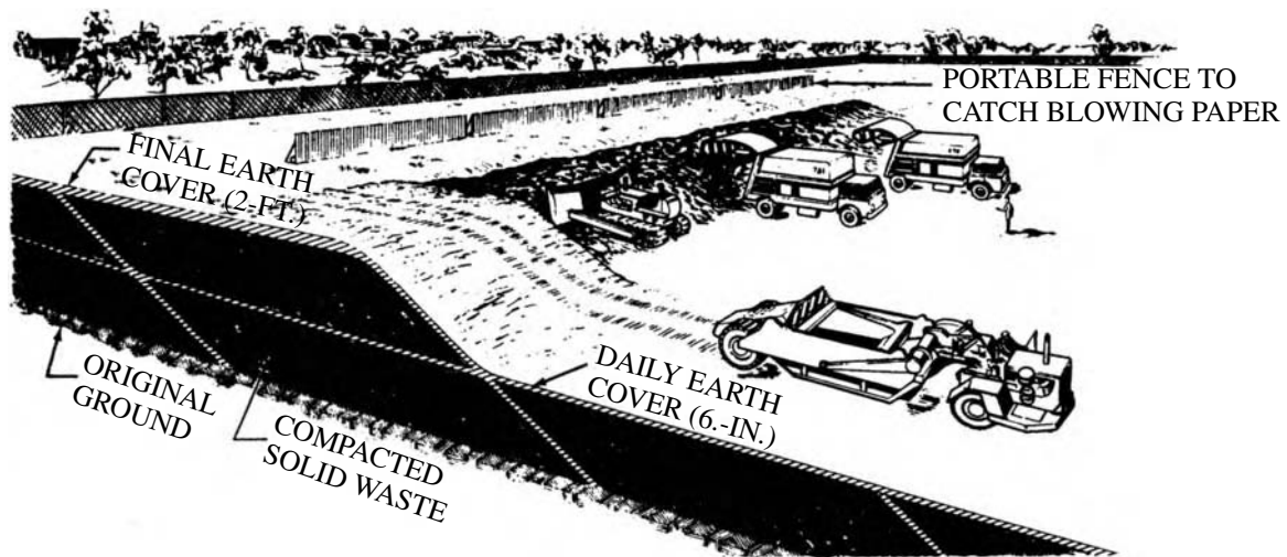
FIGURE 13 Area method. The bulldozer spreads and compacts solid wastes. The scraper (foreground) is used to haul the cover material at the end of the day's operations. Note the portable fence that catches any blowing debris. This is used with any landfill method.
