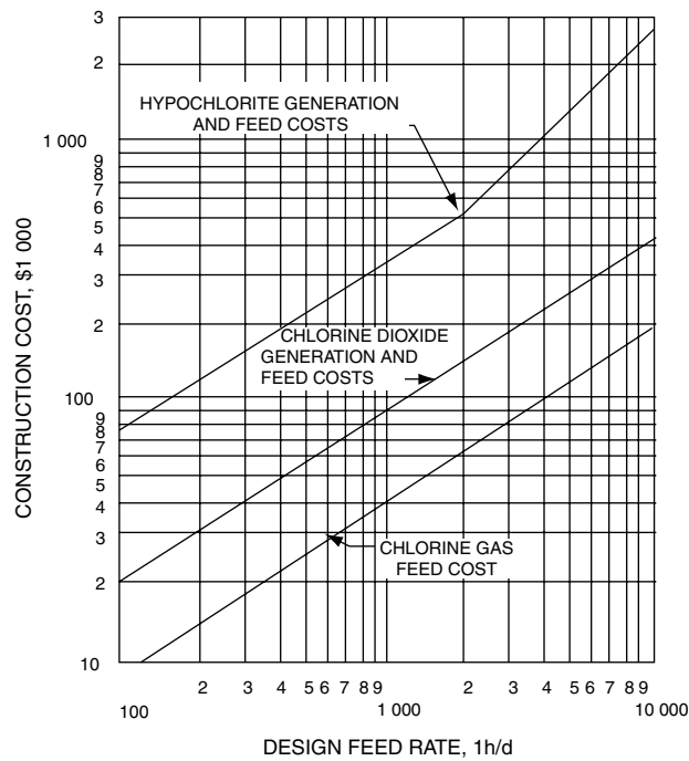
FIGURE 15 Chlorine disinfection feed facilities cost curves: ENR = 2,000.
