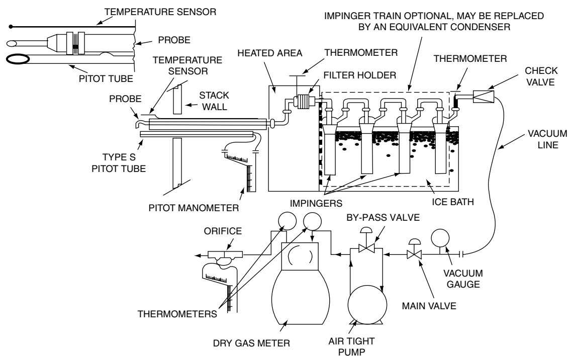
Schematic of Method 5 sampling train.
