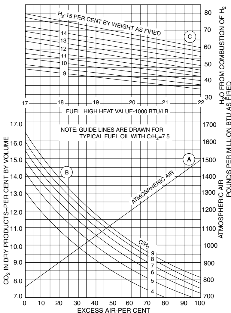
FIGURE 17 Chart for fuel oil (Fryling, 1966).
