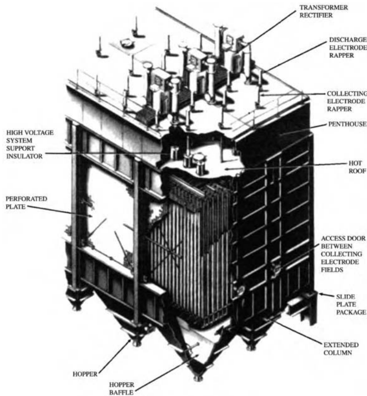
FIGURE 8 Perspective view of electrostatic precipitator showing main features of construction. (Courtesy Research Cottrell.)
