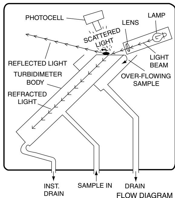
FIGURE 17 Surface scatter turbidimeter. (Used with permission of Hach Co., Loveland, CO.)
