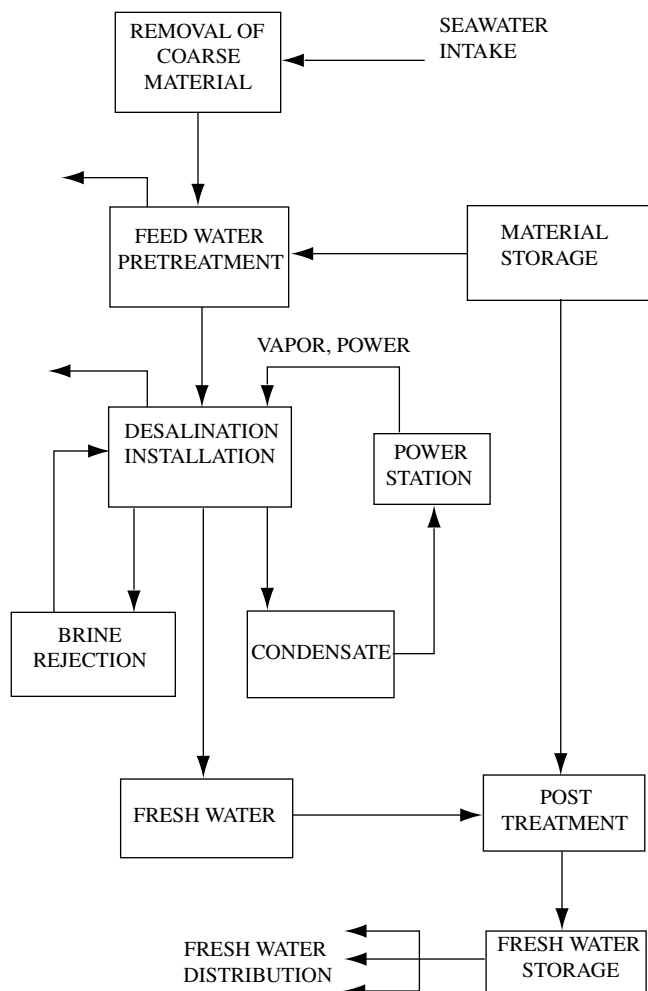
FIGURE 2 Flow diagram of the main procedures to be followed in the operation of a desalination plant.
