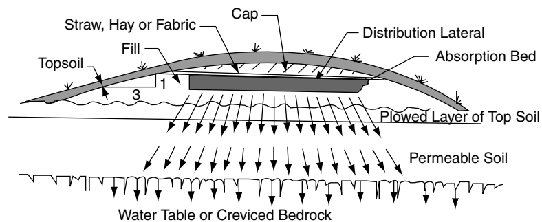
(d) Typical mound system for a permeable soil with high groundwater or shallow creviced bedrock
