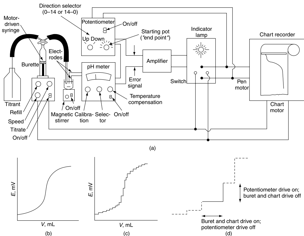
FIGURE 29 (a) An automated, curve-recording titrator. (b) Theoretical titration curve. (c) Recorded curve with endpoint anticipation. (d) Enlarge portion of (c) with explanation. (From G. Svehla, Automatic Potentiometric Titrations , p. 176, Pergamon Press. Copyright © 1978 by Prof. G. Svehla. Reprinted with permission.)
