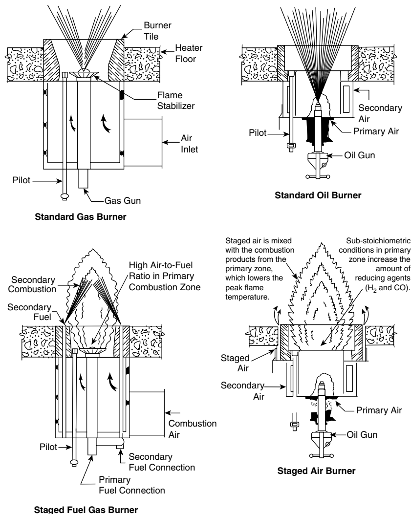
FIGURE 6 Burner configurations. 23
