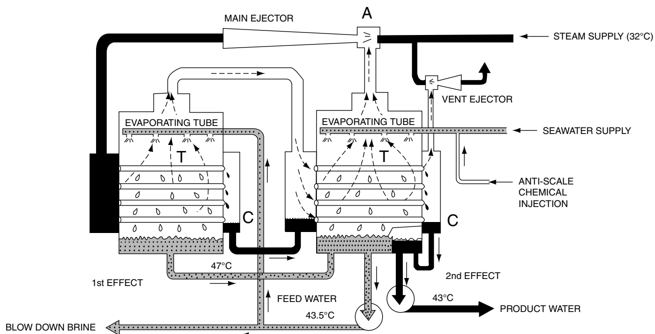
FIGURE 8 A two effect reheat or thermal compression unit. The low pressure, low temperature vapors from the second effect are sucked by the steam jet ejector A, driven by a small quantity of high pressure boiler steam, and delivers a hotter compressed mixture of steam and vapors to the condenser tubes T of the first effect. The seawater feed is sprayed onto the outside of the horizontal condenser tubes T. Part of the rejected brine from the last stage is used as feed to the first stage. Condensate, or product fresh water is collected in the last stage chamber C and distributed through the pump P. (Courtesy Sasakura Engineering Co., Ltd., Japan.)
