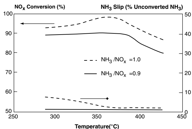
FIGURE 8 \text{NO}_x Conversion and \text{NH}_3 Slip for VNX™ SCR Catalyst. 30
