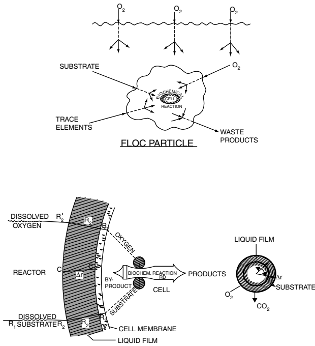
FIGURE 5 Mass transfer in biofloc.
