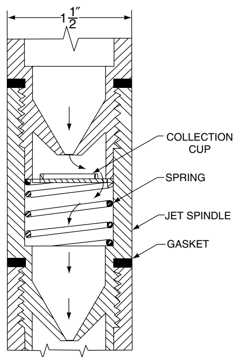
FIGURE 11 Stage of typical cascade impactor (Monsanto).
