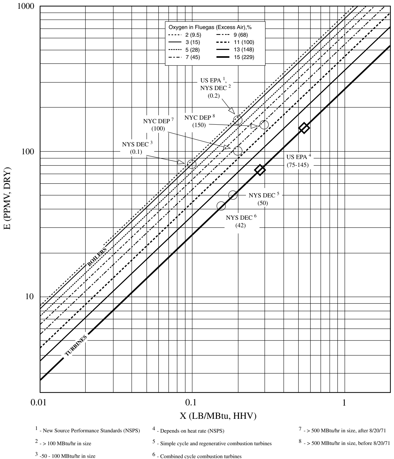
FIGURE 2 Conversion of emission units and comparison of various standards for NO x natural gas units.
