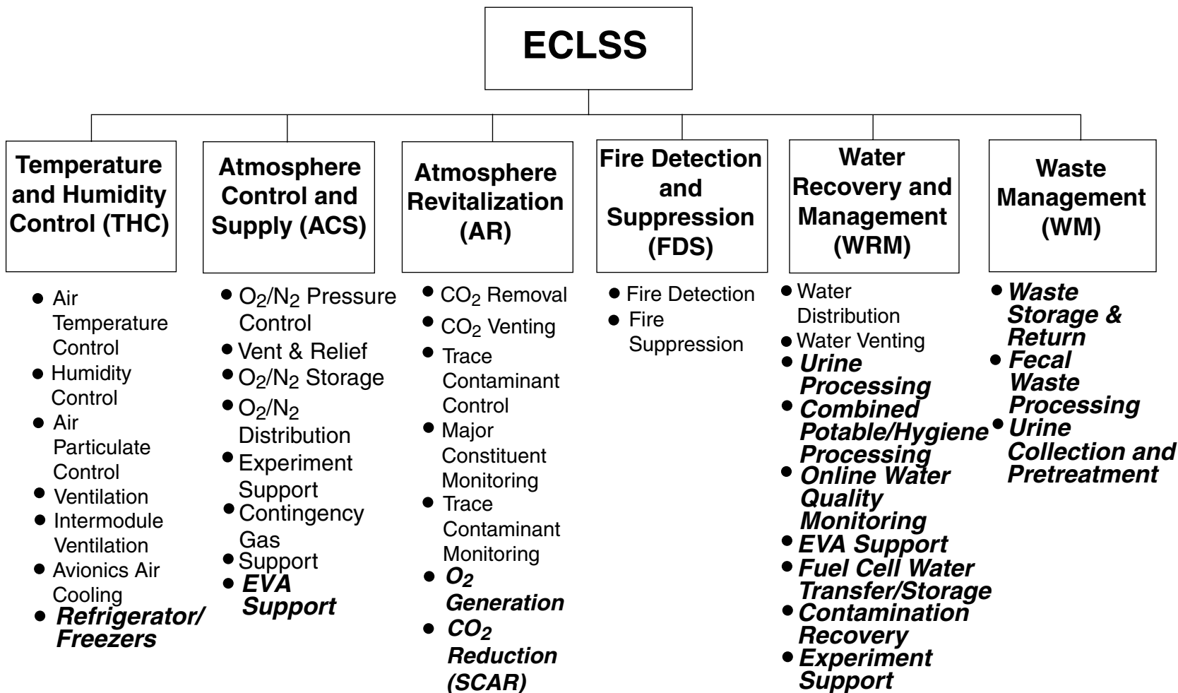
FIGURE 1 Space Station Alpha Environmental Control and Life Support System (ECLSS) Functions. Source: Ref. 4.
