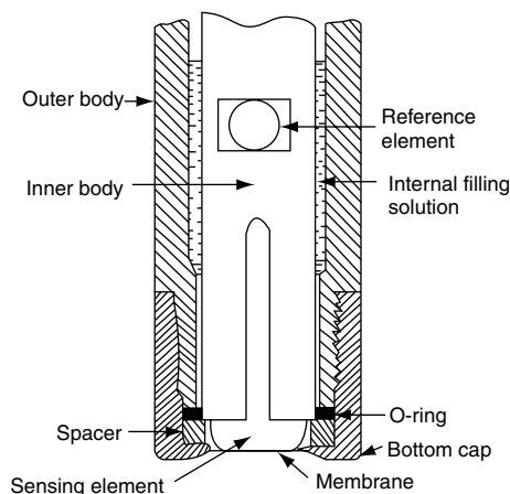
FIGURE 23 Construction of the gas-sensing electrode. For example, in the CO_2 gas-sensing electrode, the filling solution containing bicarbonate ion, HCO_3^- , forms a thin film between the sensing element, a glass electrode, and the membrane. A suitable reference electrode, e.g., SCE or Ag/AgCl can be the reference element. The CO_2 gas diffusing into the thin film reacts chemically with the HCO_3^- forming hydrogen ion, H^+ , that is detected by the glass electrode. See the text and equations 24–26 for the chemical mechanism of the CO_2 gas-sensing electrode. (Orion Research Inc.: Boston, MA with permission.)
