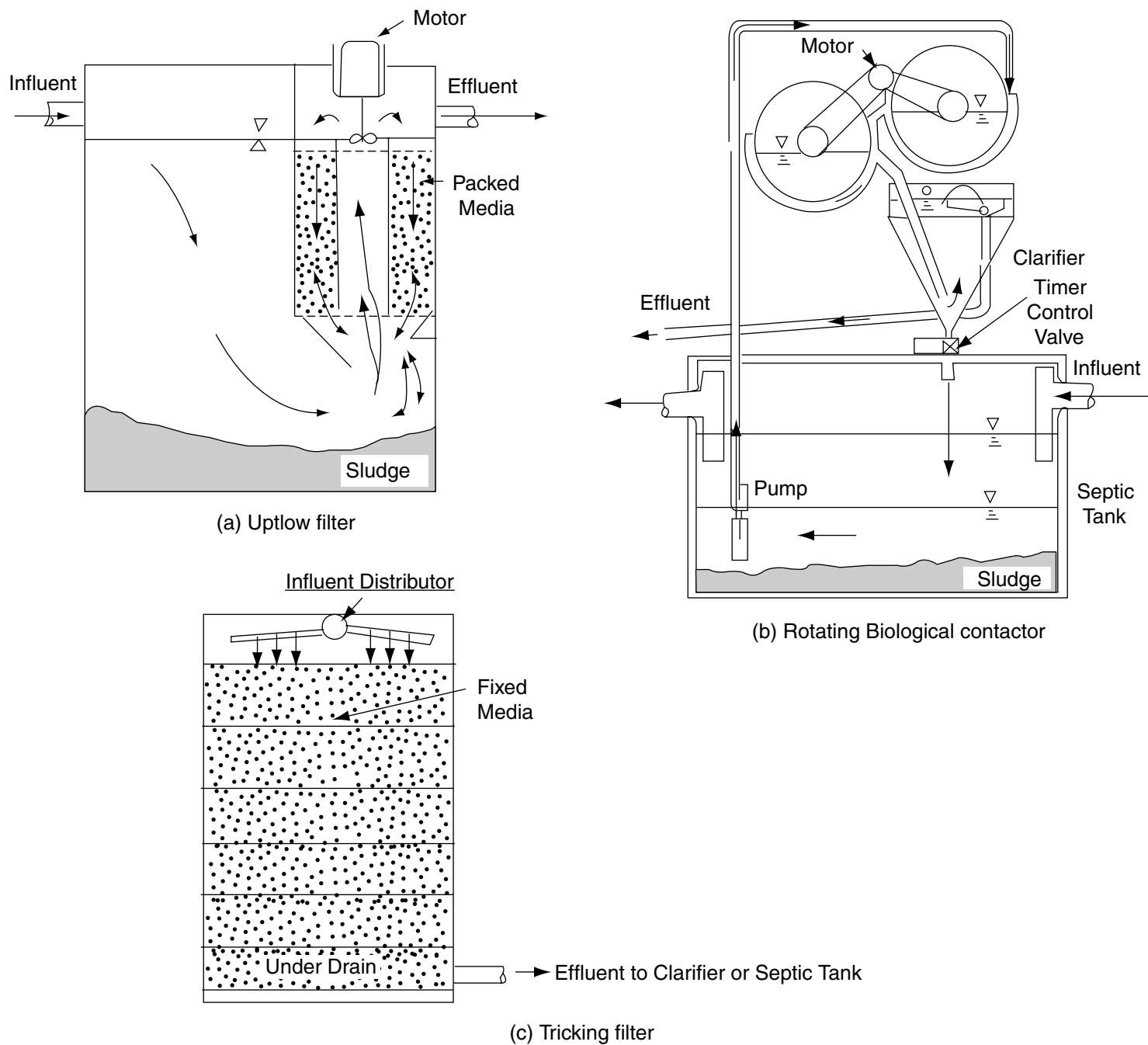
FIGURE 4 System components of aerobic attached growth biological treatment process. (Adapted from Ref. 2.)
