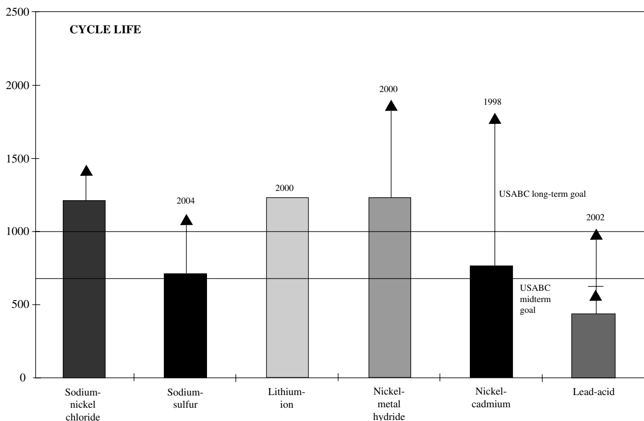
FIGURE 4: Performance Parameter Comparison for Electric Vehicles as a Function of Advanced Battery Type (After Moore 38 ).
