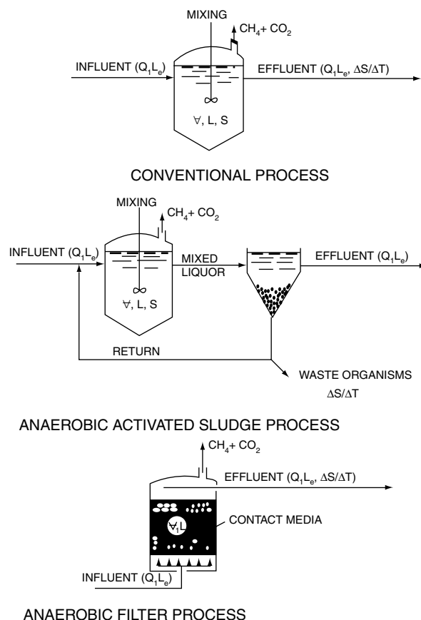
FIGURE 21 Basic anaerobic process designs.
