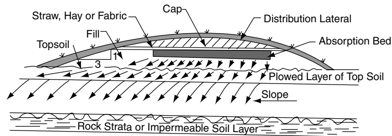
(c) Typical mound for a slowly permeable soil on sloping site
