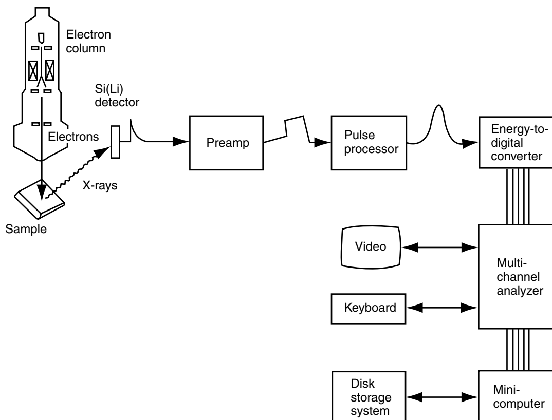
FIGURE 16 Components of a typical energy-dispersive microanalysis system. The Si(Li) detector is cooled in a liquid nitrogen cryostat. The charge pulse from the Si(Li) detector is converted in the preamp to a step on a voltage ramp. The pulse processor converts the signal to a well-shaped voltage pulse with an amplitude proportional to the energy of the x-ray. (Courtesy of the Kevex Instruments, Inc.)
