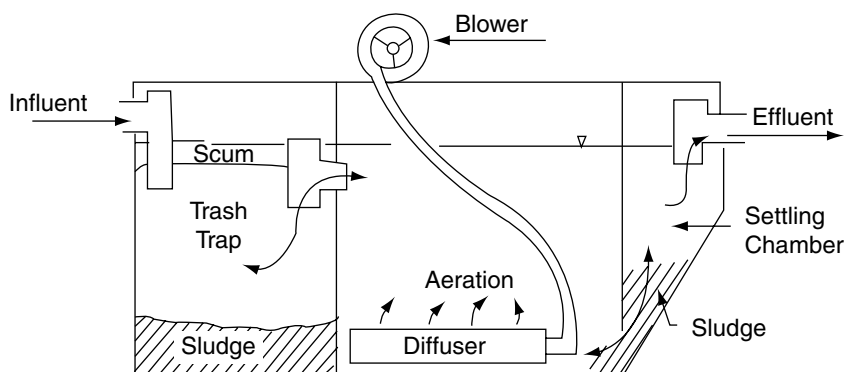
(a) Diffused aeration
