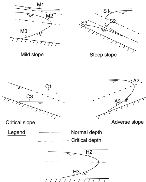
FIGURE 10 Surface water profiles.
