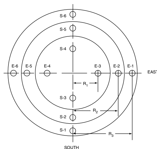
FIGURE 4 Velocity and sampling traverse positions in circular ducts.
