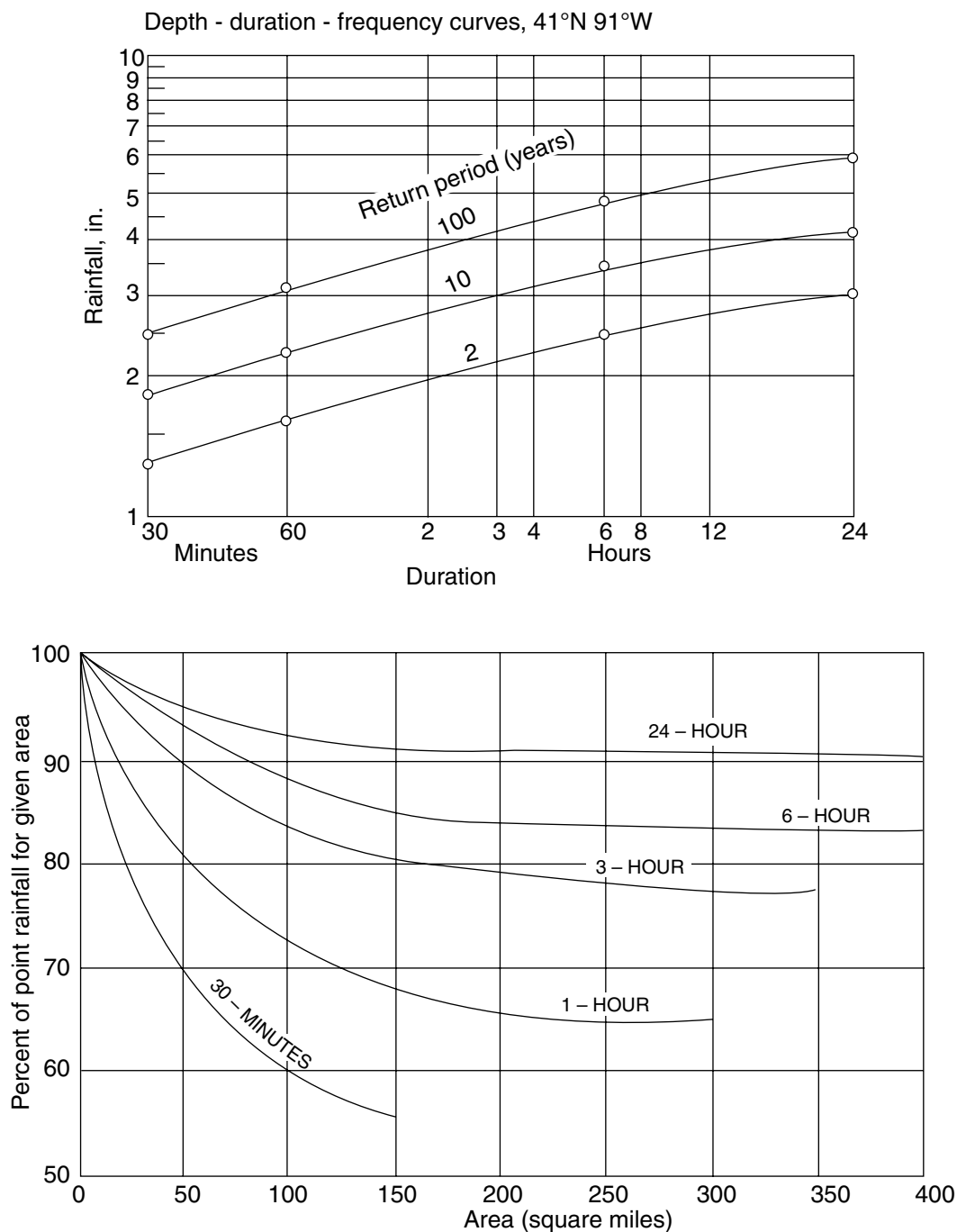
FIGURE 2 Rainfall depth-duration and area-frequency curves (US Weather Bureau, after Chow 1 ).
