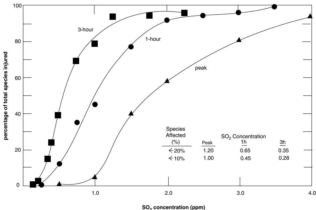
FIGURE 5 Percentage of plant species visibly injured as a function of peak 1-hour and 3-hour \text{SO}_2 concentrations. Source: McLaughlin and Lee (1974); McLaughlin (1980). (Air Quality Criteria for Particulate Matter and Sulfur Oxide, 1981.)
