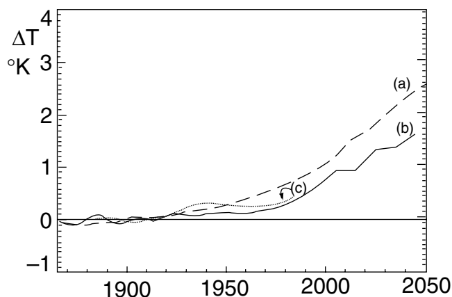
FIGURE 7 Changes in the globally-averaged mean surface temperatures relative to the mean for 1850–1920; dotted curve—observed change since 1880; dashed curve—model computations of the effects of increasing greenhouse gases from 1850–1990 and extrapolated to 2050 AD; solid curve—model predictions of changes caused by both greenhouse gases and aerosols from 1850–2040.
