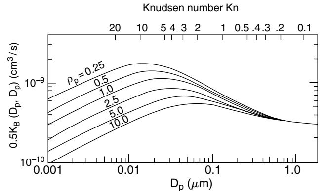
FIGURE 6 Brownian coagulation coefficient for coagulation of equal-sized particles in air at standard conditions as a function of particle density.
