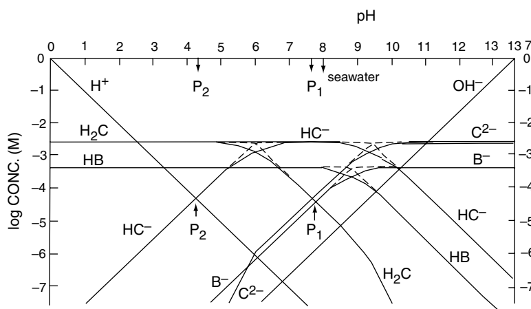
FIGURE 3 Logarithmic concentration—pH equilibrium diagram for seawater as a closed system. For seawater \log B_T = -3.37 , \log C_T = -2.62 and the following \text{pK} values: 6.0 for \text{H}_2\text{CO}_3^* , 9.4 for and \text{pK} = 13.7 . B_T = total borate boron and C_T = total carbonate carbon. Arrows gives [\text{H}^+] for seawater ( \text{pH} = 8.0 ) and for two equivalence points (points of minimum buffer intensity): P_1 , corresponding to a proton reference level of \text{HB} + \text{HC}^- + \text{H}_2\text{O} , and P_2 , corresponding to a proton reference level of \text{HB} + \text{H}_2\text{C} + \text{H}_2\text{O} (From Dyrssen, D. and L.G. Sillén, Tellus , 19, 110, 1967).
