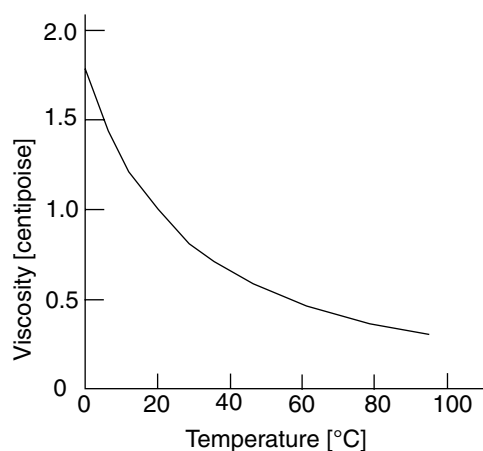
FIGURE 8 The shear viscosity of water as a function of temperature. (1 centipoise = 10^{-3} N s m ^{-2} ). (Data from Stokes and Millis, 1965.)
