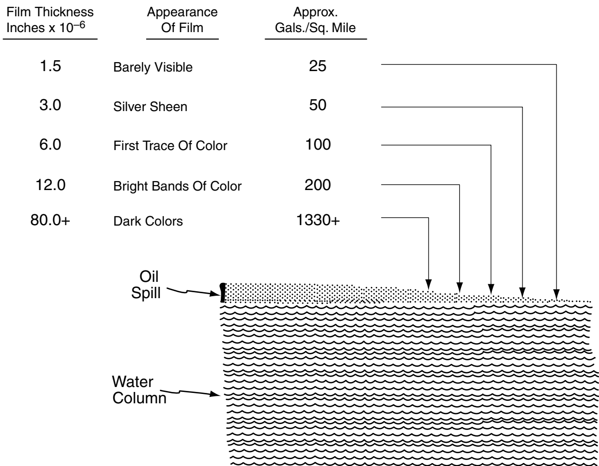
FIGURE 3 Oil slick appearance during spreading.
