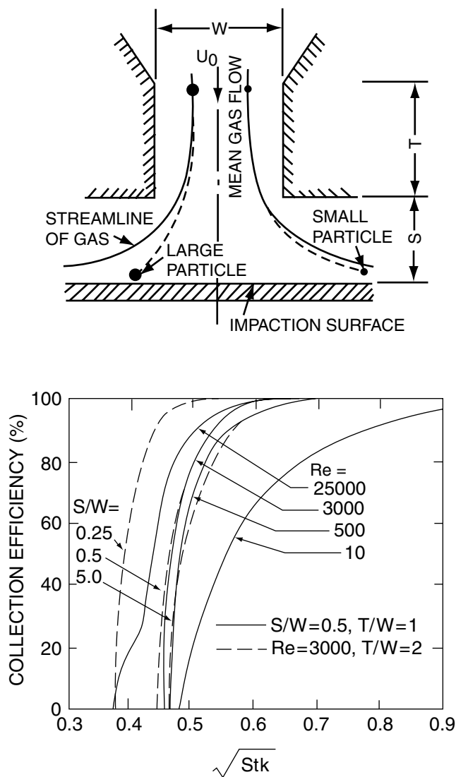
FIGURE 8 Principle of operation of an impactor. Collection efficiency of one stage of an impactor as a function of Stokes number, Stk , Reynolds number, Re , and geometric ratios.
