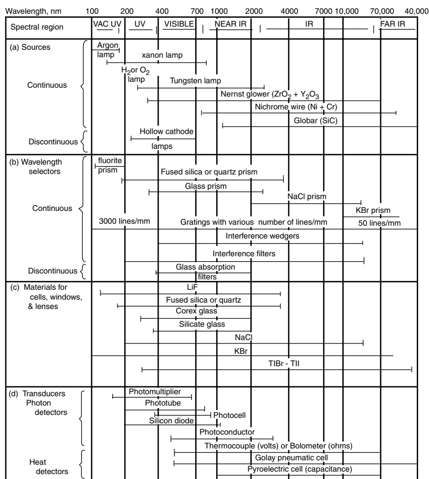
FIGURE 3 Components and materials for optical spectroscopic instruments. (Courtesy of Prof. A. R. Armstrong, College of William and Mary.)
