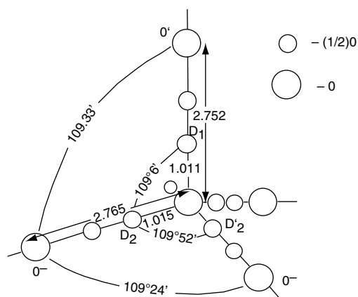
FIGURE 3 Structural relationships in one tetrahedron of the ice structure. The distances and angles are those at -50^{\circ}\text{C} . From Krindel (1971).
