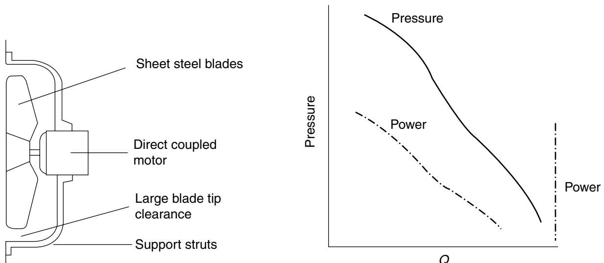
FIGURE 4 Propeller fan and graph showing its characteristic curves.
