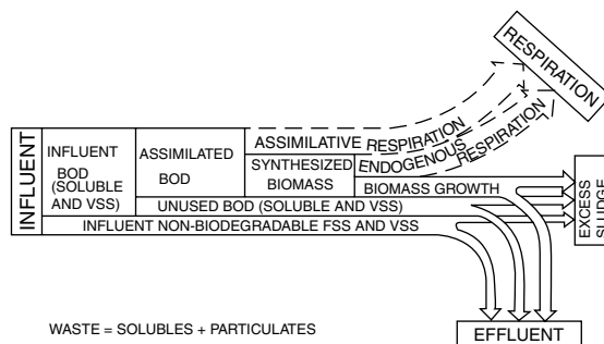
FIGURE 3 Metabolism and process reactions.
