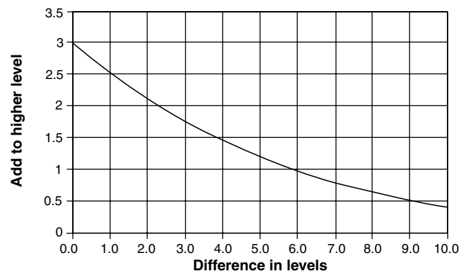
FIGURE 1 Combining noise levels.
