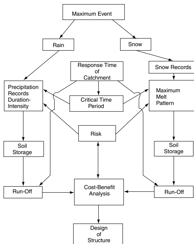
FIGURE 13 Estimation of design flood for a small spillway or road culvert, etc.
