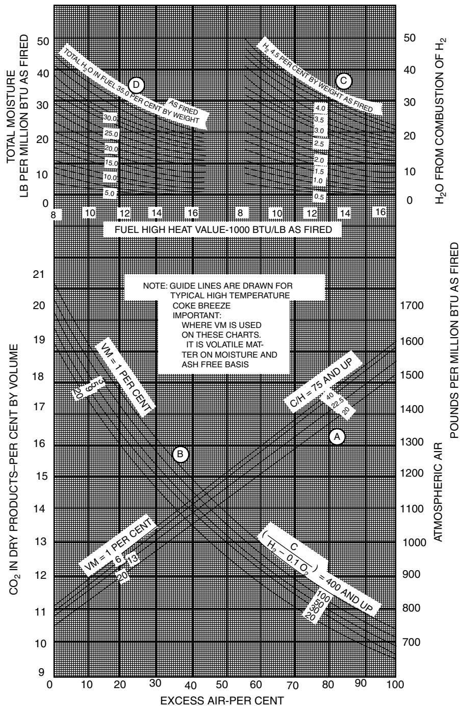
FIGURE 17 Graphical calculation curves for coal—million Btu basis (Frying, 1966).
