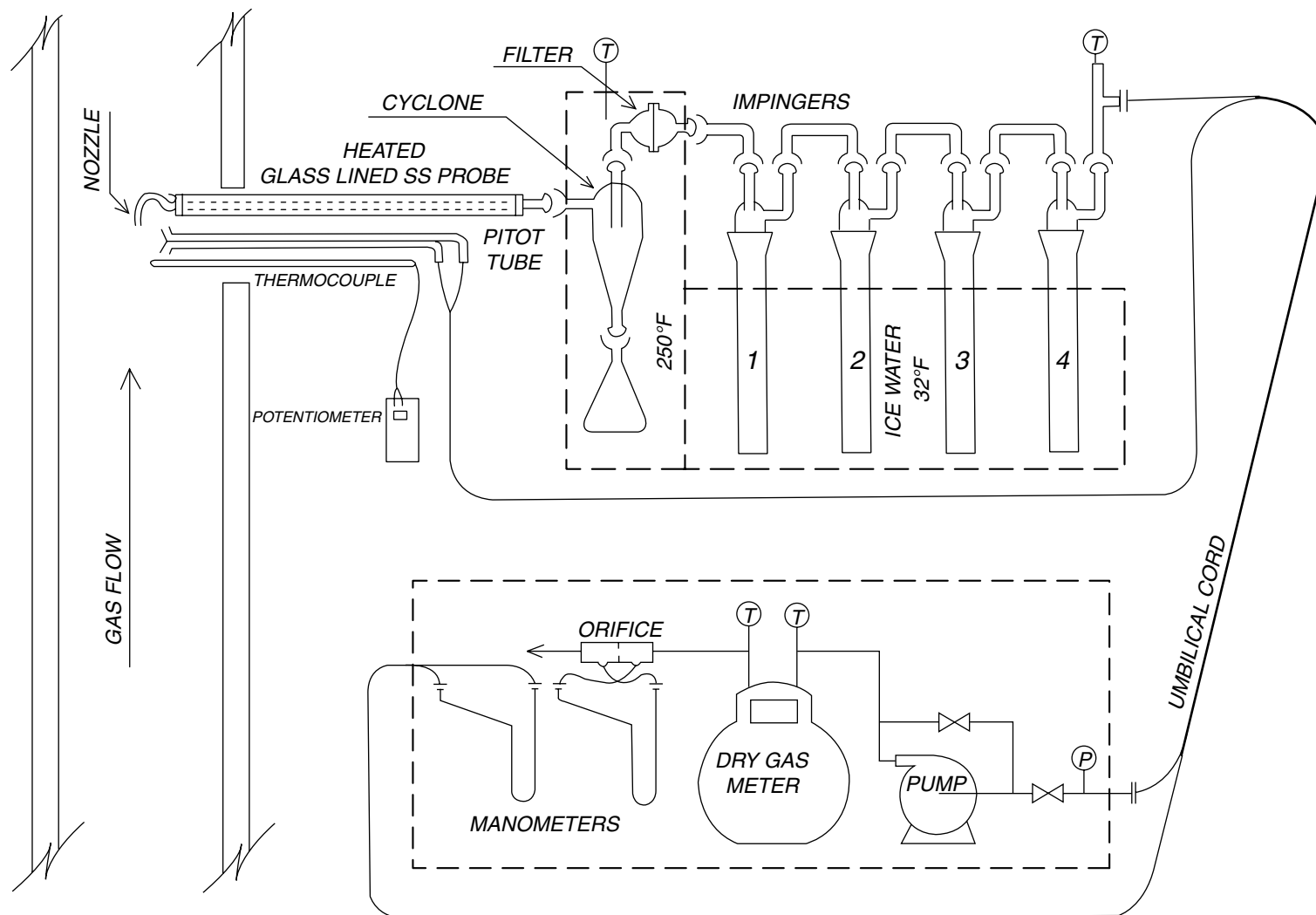
FIGURE 3 Method 8 schematic.
