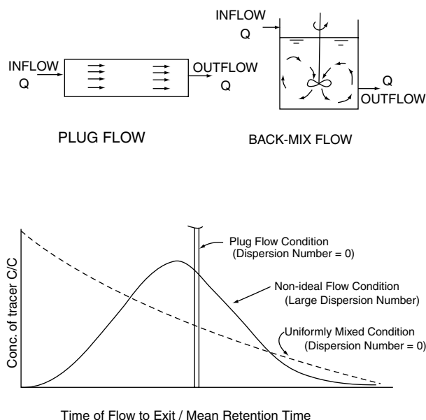
FIGURE 10 Hydraulic characteristics of basins.
