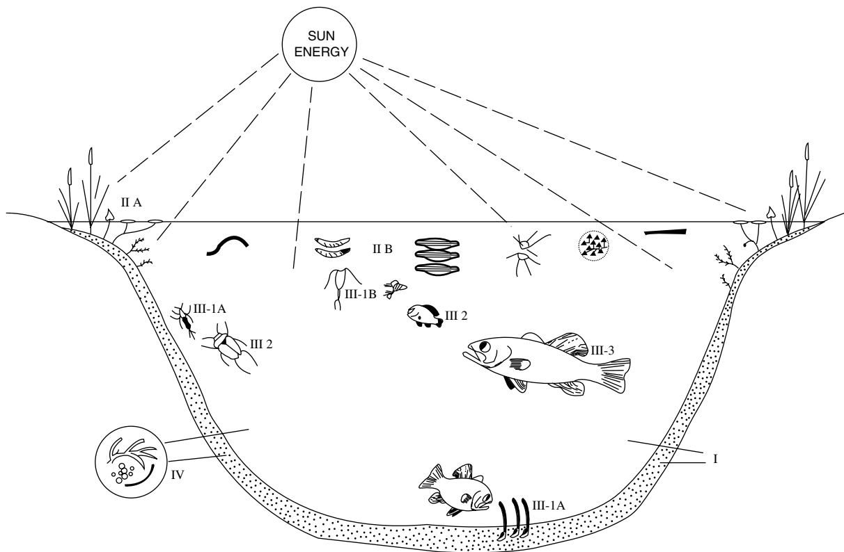
FIGURE 3 Diagram of the pond ecosystem. Basic units are as follows? I, abiotic substances—basic inorganic and organic compounds; II A, producers—rooted vegetation; II B, producers-phytoplankton; III-1A, primary consumers (herbivores)—bottom forms; III-1B, primary consumers (herbivores)—zooplankton; III-2, secondary consumers (carnivores); III-3, tertiary consumers (secondary carnivores); IV, saprotrophs—bacteria and fungi of decay. The metabolism of the system runs on sun energy, while the rate of metabolism and relative stability of the pond depend on the rate of inflow of materials from rain and from the drainage basin in which the pond is located. (From Odum, 1971.)
