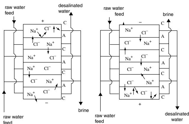
FIGURE 14 Flow diagram of an electrodialysis reversal cell. B represents the one-way operation and D the operation after the reversing of the polarity. Cathode or anode are reversing and become anode and cathode respectively. Ion movement reverses as well and concentration compartment acts as dilution compartment. Blowdown brine circulates in fresh water tubes and vice-versa.
