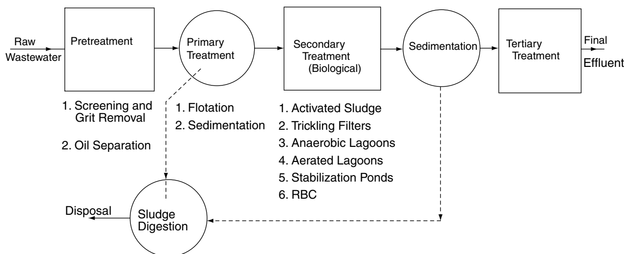
FIGURE 12 Typical wastewater treatment sequence.
