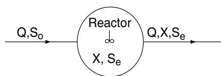
I- Completely Mixed-No biological solids recycle
