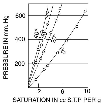
FIGURE 13 Adsorption isotherms for the system \text{CO}_2 -silica gel (note that t_c = 31^\circ\text{C} ). Patrick, Preston and Owens: J. Phys. Chem. 29 , 421 (1925) (Fig. 1).
