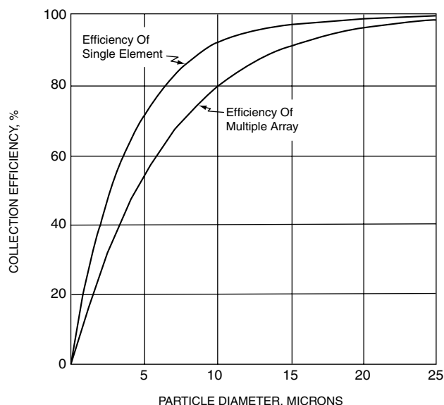
FIGURE 7 Performance debit for manifolding of multicellones.
