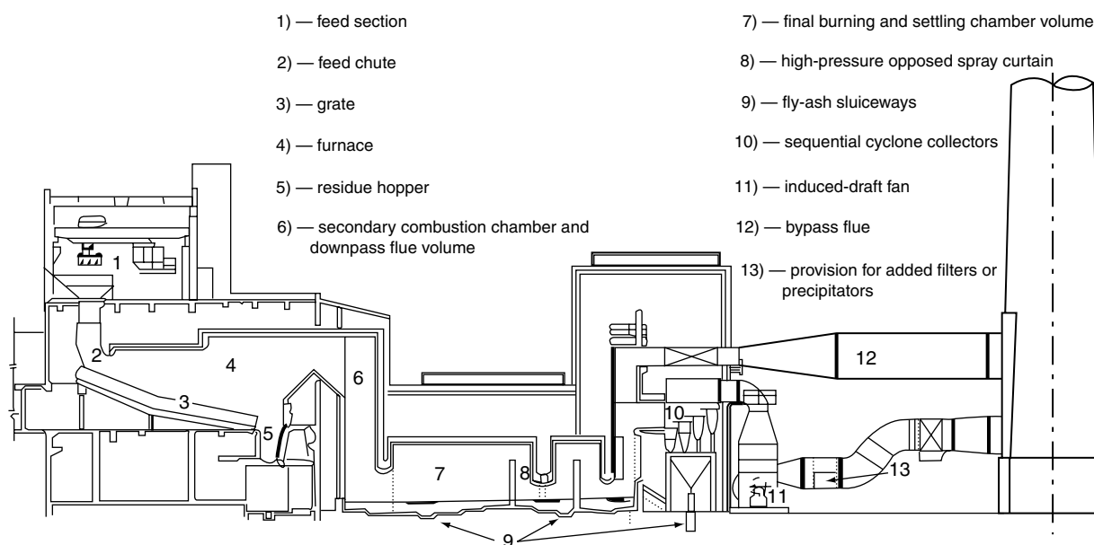
FIGURE 3 Large incinerator schematic.
