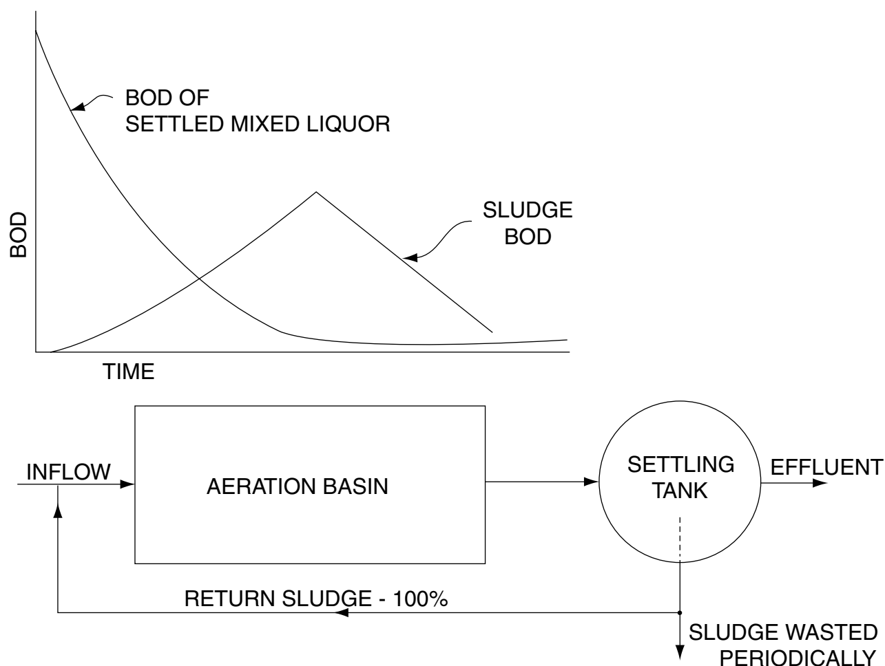
FIGURE 19 Extended aeration activated sludge.
