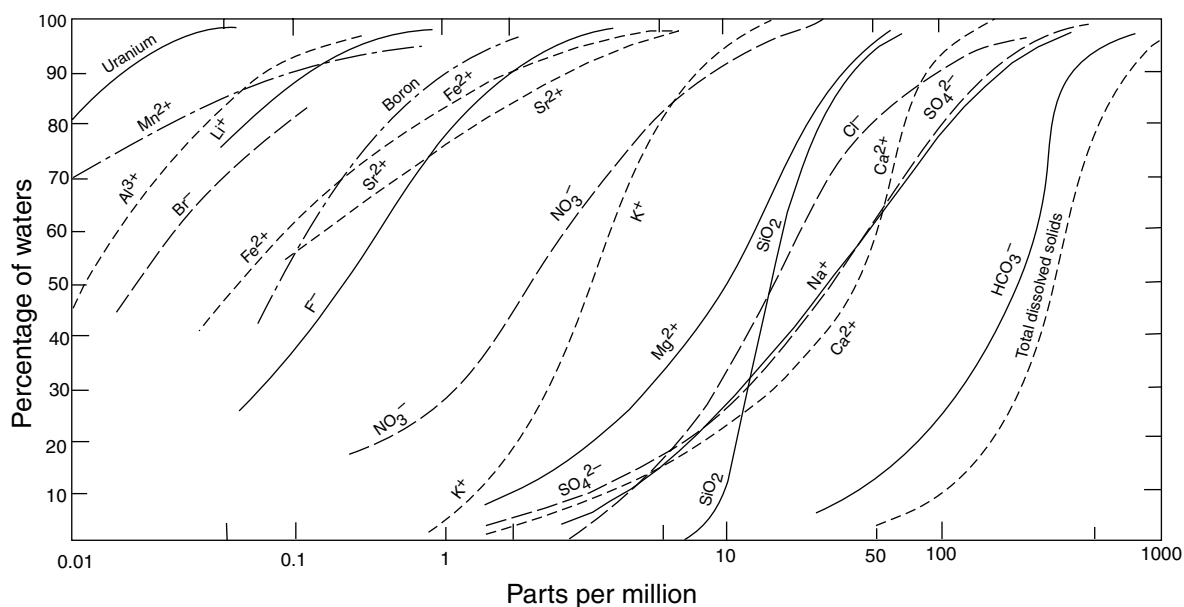
FIGURE 11 Cumulative distribution of inorganic species in terrestrial waters. The curves represent the percentage of waters with concentrations below that indicated on the horizontal axis. Data are mostly from the United States from various sources. S.N. Davies and R.C.M. Dewiest, Hydrogeology , Wiley, New York, 1966.
