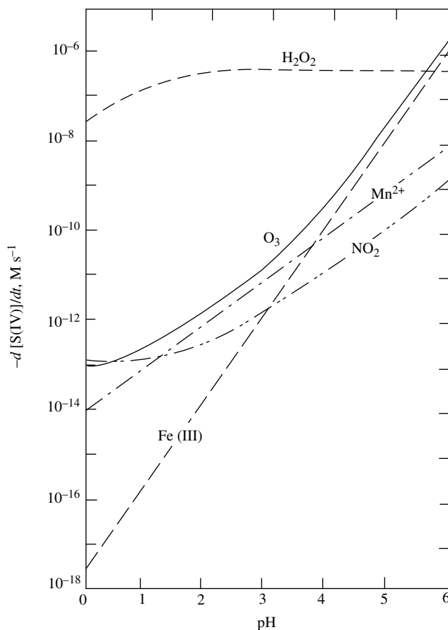
FIGURE 8 Comparison of aqueous-phase oxidation paths; the rate of conversion of \text{S(IV)} to \text{S(VI)} as a function of pH. Conditions assumed are: [\text{SO}_2(\text{g})] = 5 ppb; [\text{NO}_2(\text{g})] = 1 ppb; [\text{H}_2\text{O}_2(\text{g})] = 1 ppb; [\text{O}_3(\text{g})] = 50 ppb; [\text{Fe(III)}] = 0.3 \mu\text{M} ; and [\text{Mn(II)}] = 0.03 \mu\text{M} . From Seinfeld and Pandis (1998). With permission.
