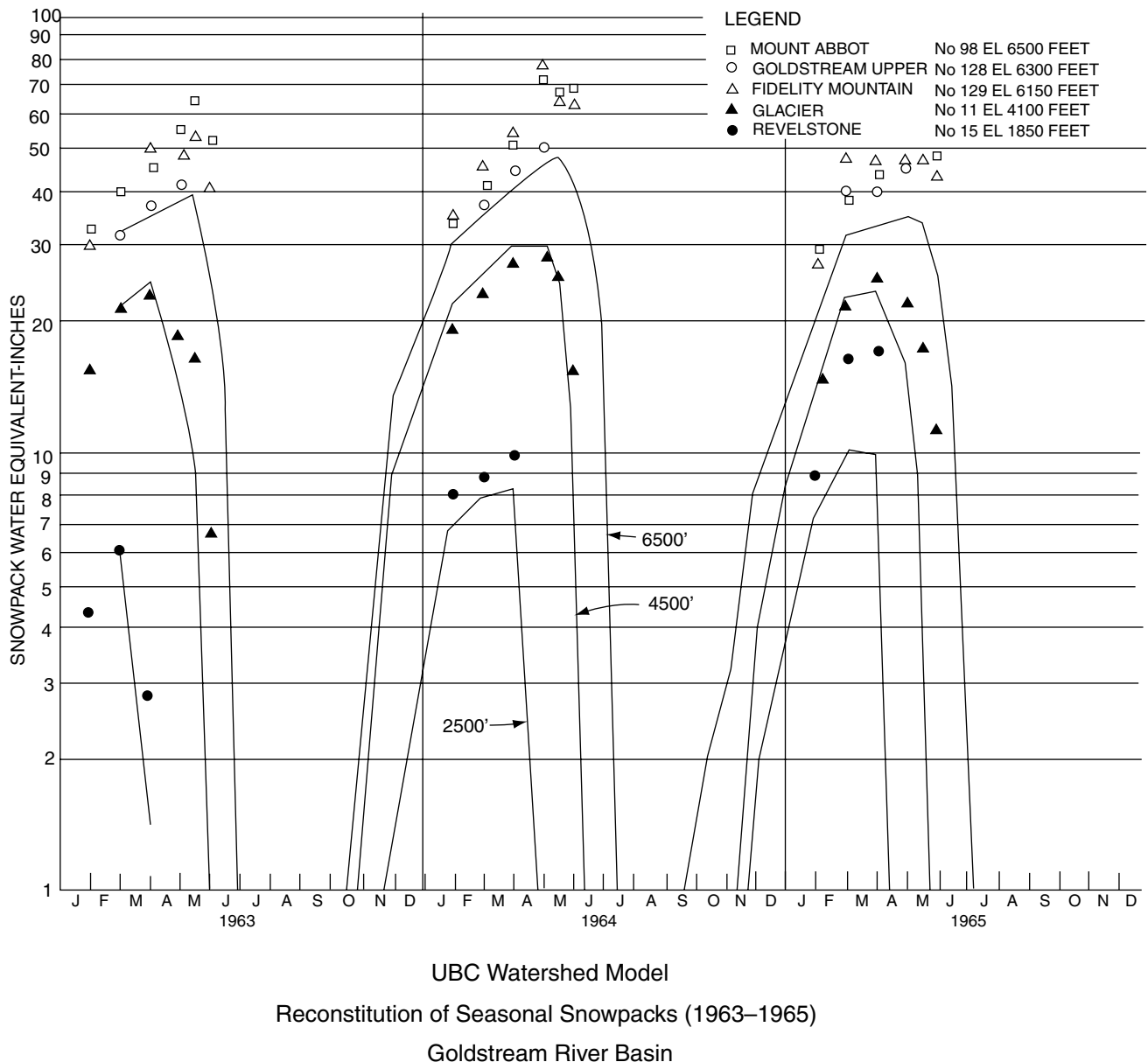
FIGURE 10 Comparison of computed snowpacks and snowcourse data.
