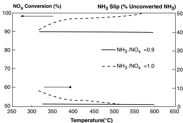
FIGURE 9 \text{NO}_x Conversion and \text{NH}_3 Slip for ZNX™ SCR Catalyst. 30
