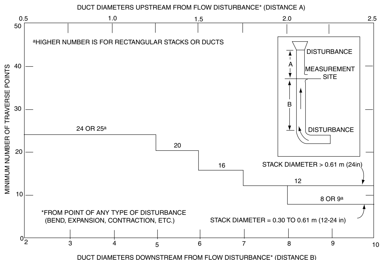
FIGURE 1 Minimum number of traverse points for particulate traverses.
