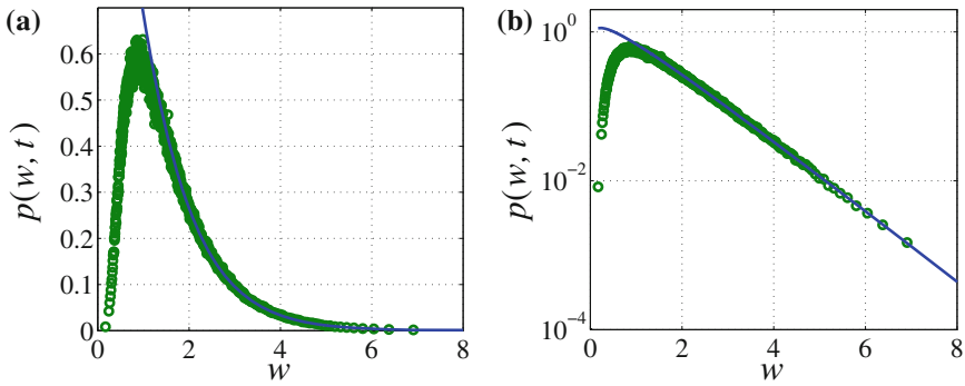
Fig. 6.5 Simulated work distribution (symbols) at time t = 1 for a protocol k(t) = k_0 \exp(-\gamma t) with \gamma = -1 , and otherwise the same parameters as in Fig. 6.4. In a p(w, t) is plotted in a linear representation and in b in a semi-logarithmic one. The solid blue line is a fit of Eq. (6.50) to the right tail with the best parameters are r(1) \approx 1.916 , D\xi_0(1) \approx 1.124 . In the simulations 10^6 trajectories were generated with time step \Delta t = 10^{-3}
