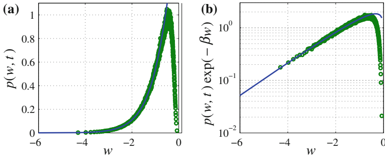
Fig. 6.4 a Simulated work distribution p(w, t) (symbols) at time t = 1 for the protocol k(t) = k_0 \exp(-\gamma t) with k_0 = 1 , \gamma = 1 , and parameters g = 1.5 and D = 1 ; in b the associated Jarzynski integrand p(w, t) \exp(-\beta w) is displayed in a semi-logarithmic representation. The solid blue line is a fit of Eq. (6.50) to the left tail. The best parameters are r(1) \approx 2.833 , D\xi_0(1) \approx 1.757 . In the simulations 10^6 trajectories were generated with time step \Delta t = 10^{-3}
