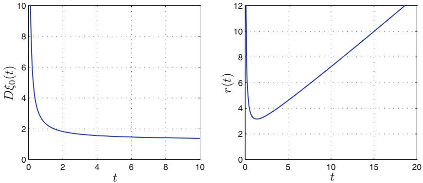
Fig. 6.2 Positions of the singularity in the expression (6.48) (left panel), and the prefactor (6.49) (right panel) as functions of time. These functions control, through Eq. (6.50), the large |w| asymptotics of the work PDF. In the right panel we have taken D = 1 and g = 1 (Reproduced from Ref. [25] with kind permission of IOP)
