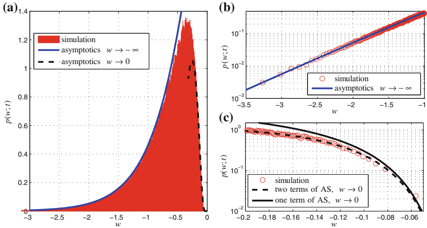
Fig. 6.3 a Simulated work PDF in comparison with the asymptotic behavior predicted by Eq. (6.50) ( |w| large, solid line ) and Eq. (6.51) ( |w| small, dashed line ) for parameters g = 1.5 , D = 1 and t = 1 . In the simulations 10^6 trajectories were generated with the time step \Delta t = 0.001 (adapted when the particle is near the origin, see text). b Semi-logarithmic plot of simulated p(w, t) versus w ( circles ), demonstrating the agreement with Eq. (6.50) ( solid line ) for large |w| . c Semi-logarithmic plot of simulated p(w; t) versus w ( circles ) in comparison with the first leading term of the asymptotic expansion for small |w| (Eq. (6.46), solid line ), and when including the second leading term according to Eq. (6.51) ( dashed line ) (Reproduced from Ref. [25] with kind permission of IOP)
