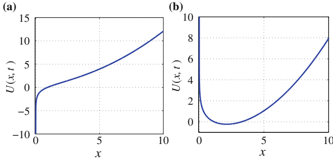
Fig. 6.1 Sketch of the potential in Eq. (6.1) for k(t) = 0.2 and a negative g = -0.9 and b positive g = 0.9 . The analysis in the main text corresponds to the case g \geq 0 . Decreasing the force constant k(t) , the well broadens and its minimum shifts further from the origin
