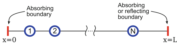
Fig. 4.1 Schematic illustration of the finite interval containing N particles. The left boundary is absorbing. The right boundary is either absorbing (Sect. 4.2) or reflecting (Sect. 4.3)
