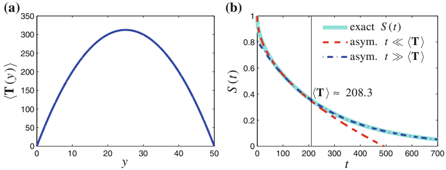
Fig. 4.2 First-passage properties of a single particle for L = 50 , D = 1 . Panel (a) shows the MFPT (4.4) against the initial position of the particle. Panel (b) depicts the exact survival probability (4.7) (the solid line), the long-time asymptotic representation (4.9) (the dot-dashed line), and the short-time asymptotic representation (4.11) (the dashed line). Note an excellent agreement of asymptotic expressions with the exact curve even for t \approx \langle T \rangle . The MFPT \langle T \rangle is given by Eq. (4.5)
