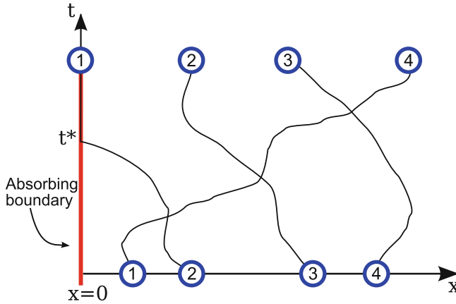
Fig. 3.1 Schematic illustration of space-time trajectories of four particles. At time t^* the leftmost particle hits the absorbing boundary. After this event the leftmost particle exits the interval and will never return. Equivalently we can imagine that for all times t, t > t^* , the absorbed particle resides in the trap located at x = 0
