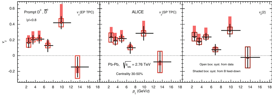
Fig. 7.6 D^0 meson v_2 as a function of p_T in the 30–50 % centrality class, with the event-plane, scalar product and two-particle cumulant methods. For the first method, the event plane was estimated with TPC tracks in the positive \eta region; for the other methods, TPC tracks in -0.8 < \eta < 0.8 were used as reference particles [3]
