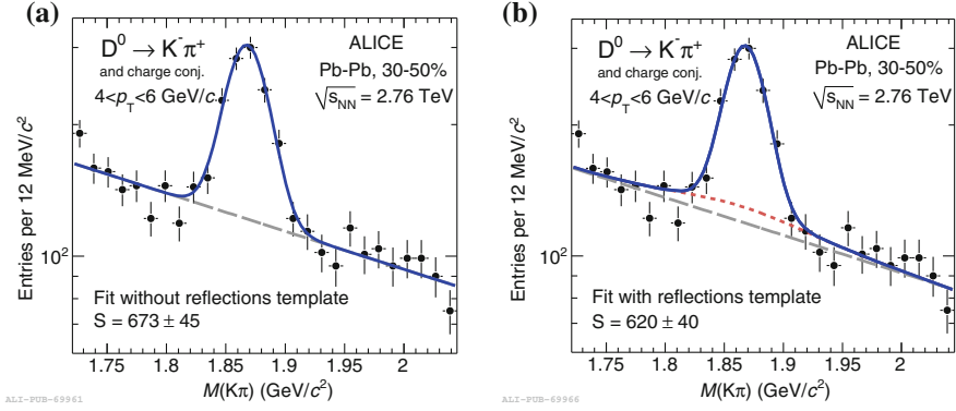
Fig. 5.23 Invariant mass distribution of D^0 candidates with 4 < p_T < 6 GeV/c in Pb–Pb collisions in the centrality class 30–50%: a fit without template for reflections and b with template for reflections ( dotted lines ). The raw yield obtained as integral of the signal Gaussian is reported [3]
