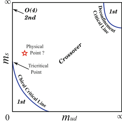
Fig. 1.5 Schematic figure of the Columbia phase diagram in 3-flavour QCD at \mu_B = 0 on the plane with the light and heavy-quark masses [18]
