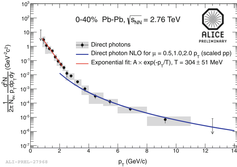
Fig. 1.12 ALICE preliminary direct photons p_T spectrum measured in Pb–Pb collisions at \sqrt{s_{NN}} = 2.76 TeV for 40% most central collisions compared at low p_T with an exponential fit and with a direct-photon NLO calculation for pp collisions at \sqrt{s} = 2.76 TeV scaled by the number of nucleon–nucleon binary collisions
