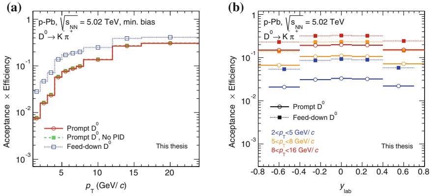
Fig. 5.28 a D^0 \rightarrow K^- \pi^+ ( \text{Acc} \times \epsilon ) as a function of p_T for prompt (solid line) and feed-down (dotted line) D^0 in minimum-bias p-Pb collisions at \sqrt{s_{NN}} = 5.02 TeV. The values for prompt D^0 mesons obtained without PID selection (dashed line) are also displayed. b Product of acceptance and efficiency as a function of rapidity for D^0 mesons in p-Pb collisions. The values of ( \text{Acc} \times \epsilon ) for prompt (open circles) and feed-down (filled squares) D^0 are shown for three p_T intervals
