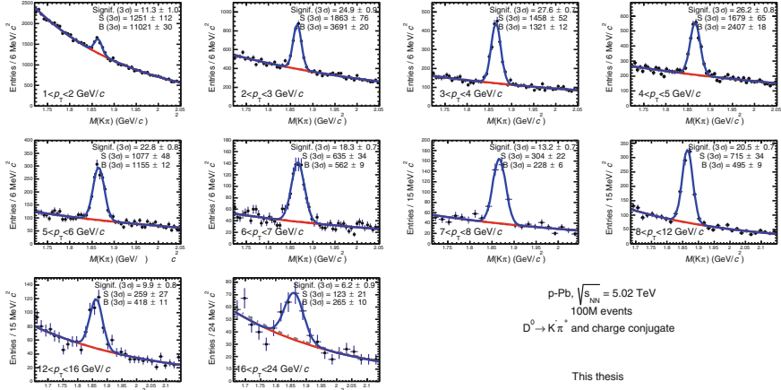
Fig. 5.7 D^0 invariant mass distributions in p-Pb collisions. The signal was extracted in 10 p_T intervals in the range 1 < p_T < 24 GeV/c
