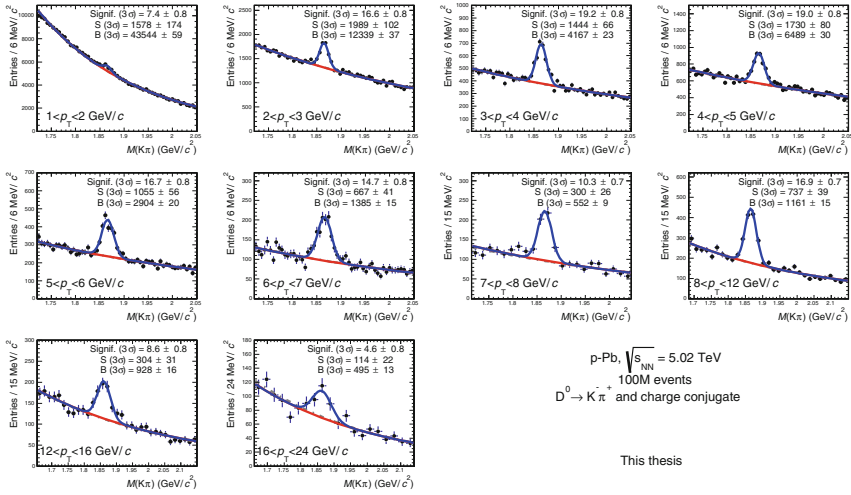
Fig. 6.13 Distributions of the invariant mass for D^0 in p-Pb collisions obtained without applying PID selection. The raw signals include the reflection contribution
