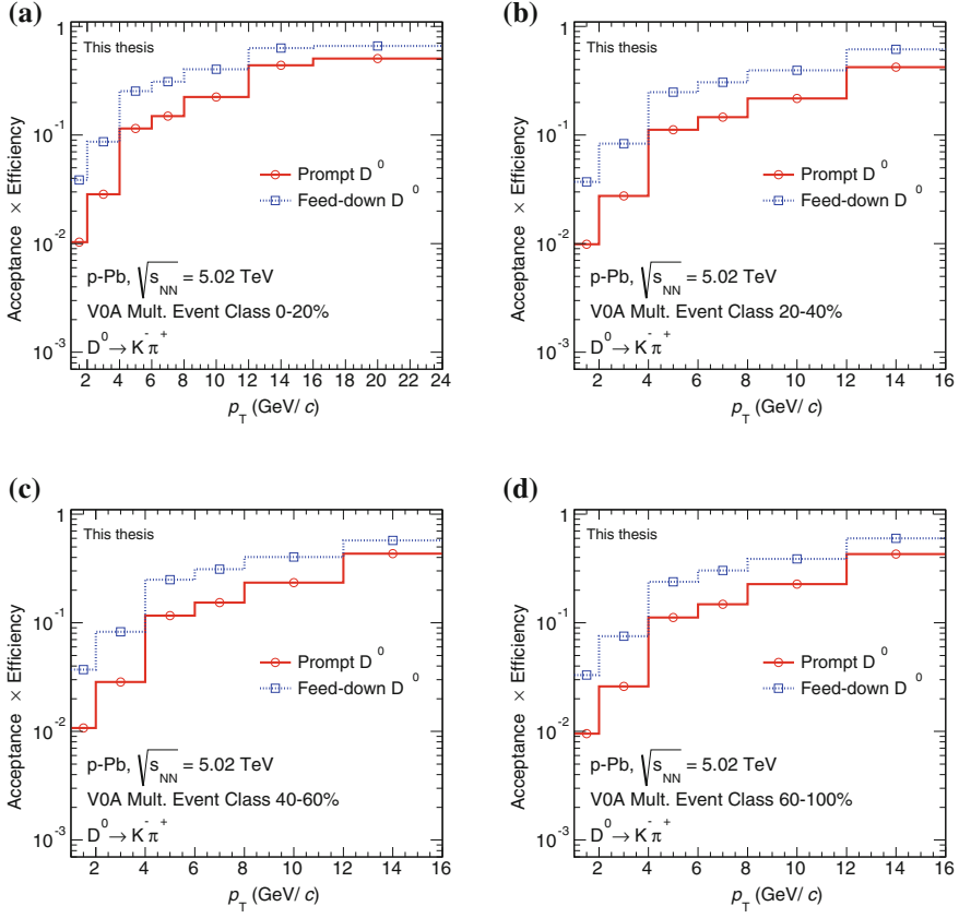
Fig. 5.30 ( \text{Acc} \times \epsilon ) as a function of p_T for prompt and feed-down D^0 in 0–20 % (a), 20–40 % (b), 40–60 % (c), and 60–100 % (d) event-activity classes defined with the V0A estimator
