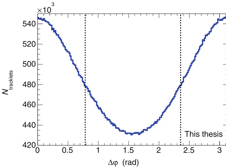
Fig. 5.26 Distributions of the number of SPD tracklets ( N_{\text{tracklets}} ) in |\eta| < 1.6 as a function of \Delta\varphi in 30–50 % Pb–Pb collisions. The in-plane and the out-of-plane regions are indicated
