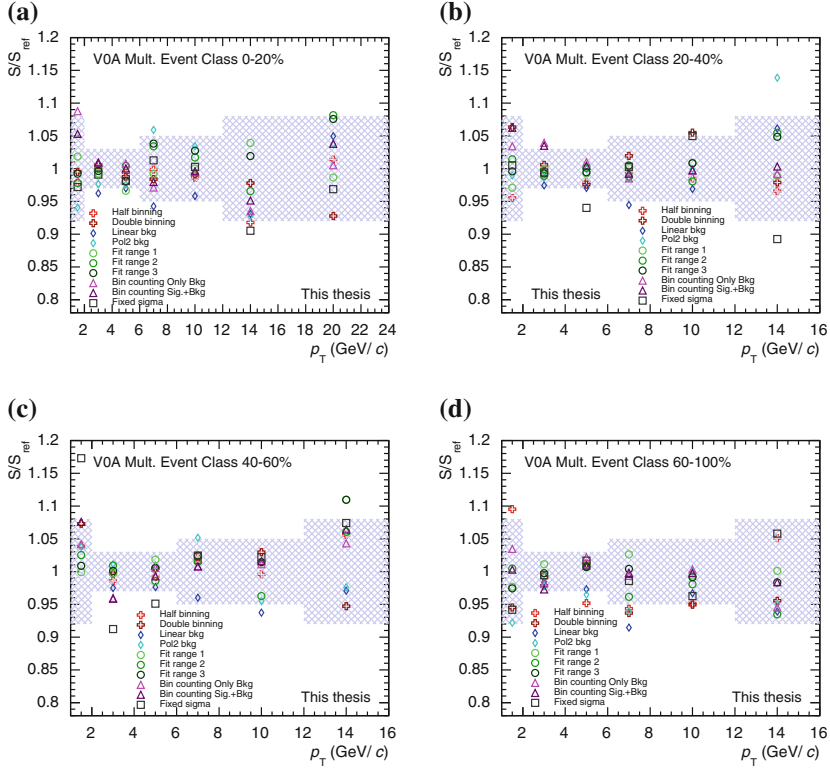
Fig. 6.5 Raw yield ratios relative to the signal yield extracted with the default fit procedure as a function of p_T for 0–20 % (a), 20–40 % (b), 40–60 % (c), and 60–100 % (d) event-activity classes defined with the VOA estimator in p–Pb collisions
