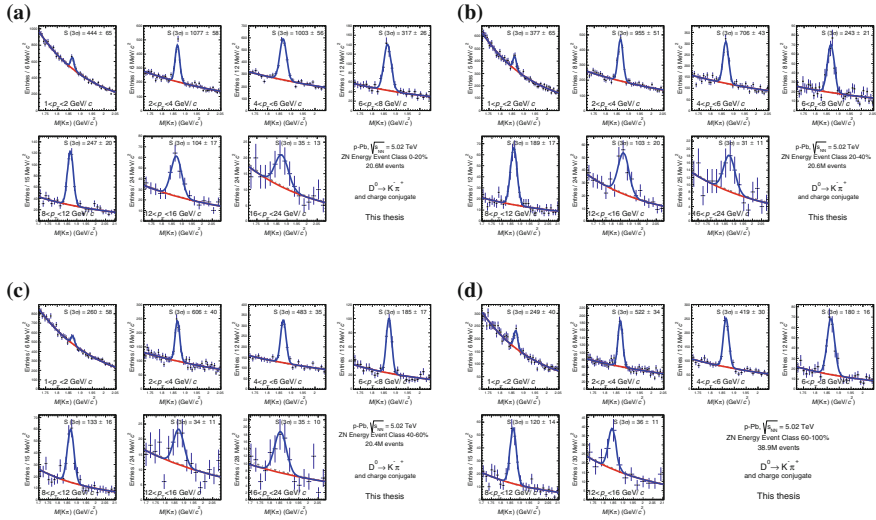
Fig. 5.13 D^0 invariant mass distributions for 0–20% (a), 20–40% (b), 40–60% (c), and 60–100% (d) event-activity classes defined with the ZNA estimator
