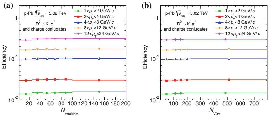
Fig. 5.32 Efficiencies for prompt D^0 as a function of N_{\text{tracklets}} (a) and N_{V0A} (b) for the five p_T intervals considered for the analysis
