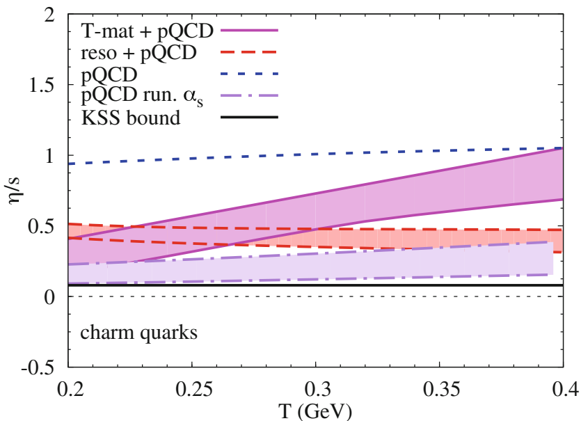
Fig. 2.9 Ratio of shear viscosity to entropy density \eta/s estimates using charm-quark diffusion constants based on schematic LO pQCD elastic scattering ( \alpha_s = 0.4 ) in the weakly-interacting limit ( dashed line ), pQCD elastic scattering with running coupling constant (band enclosed by dash-dotted lines using the weak- and strong-coupling limits), the effective resonance plus pQCD model in the strong-coupling limit (band enclosed by long-dashed lines ), and the LQCD potential based T -matrix approach with pQCD scattering off gluons (band enclosed by solid lines constructed from weak- and strong-coupling limits)
