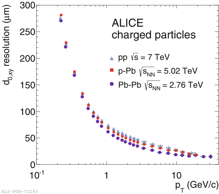
Fig. 3.13 Resolution of the r\varphi projection of the impact parameter for ITS-TPC tracks. The contribution from the vertex resolution is included [7]
