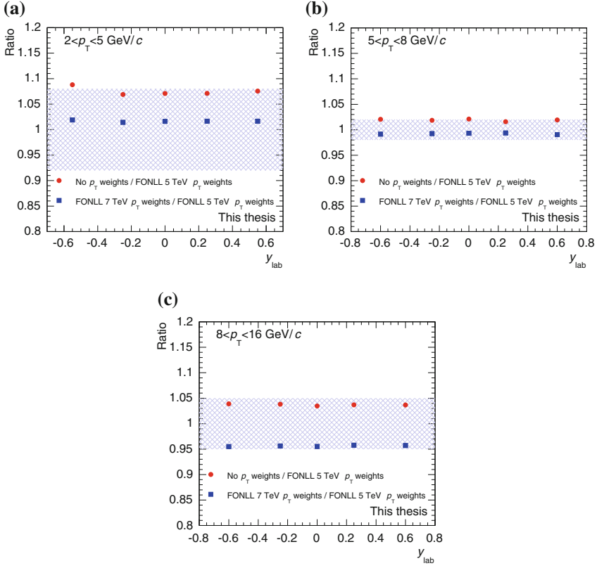
Fig. 6.15 Efficiencies ratios as a function of y_{\text{lab}} for 2 < p_T < 5 \text{ GeV}/c (a), 5 < p_T < 8 \text{ GeV}/c (b), and 8 < p_T < 16 \text{ GeV}/c (c) calculated to estimate the systematic uncertainty due to the simulated D^0 momentum distribution in p-Pb collisions
