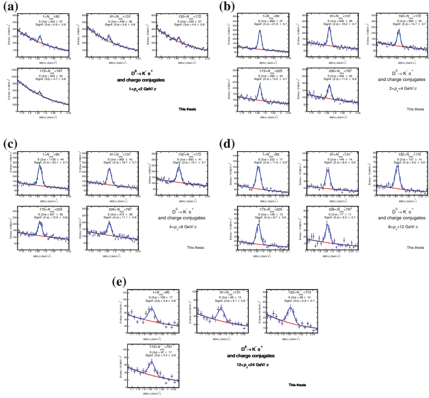
Fig. 5.18 D^0 invariant mass distributions as a function N_{V0A} for the five p_T intervals considered for the analysis
