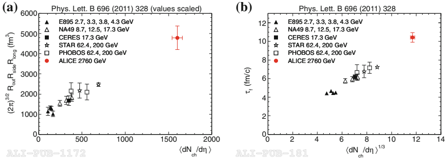
Fig. 1.11 a Product of the three pion HBT radii measured by ALICE in red compared to those obtained for central gold and lead collisions at lower energies at the AGS, SPS and RHIC. b The system lifetime (decoupling time) \tau_f measured by ALICE (red filled dot) compared to results from lower energies [24]
