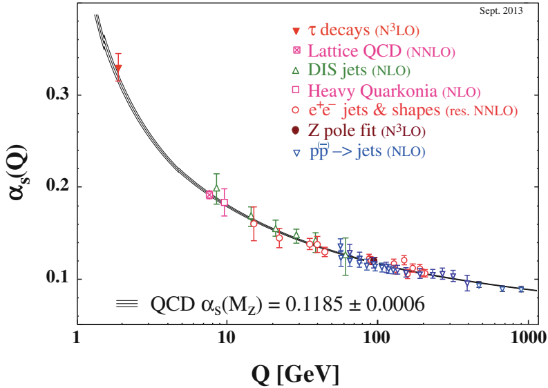
Fig. 1.2 Summary of measurements of \alpha_s as a function of the energy scale Q . The respective degree of QCD perturbation theory used in the extraction of \alpha_s is indicated in brackets (NLO: next-to-leading order; NNLO: next-to-next-to leading order; res. NNLO: NNLO matched with resummed next-to-leading logs; N 3 LO: next-to-NNLO) [12]
