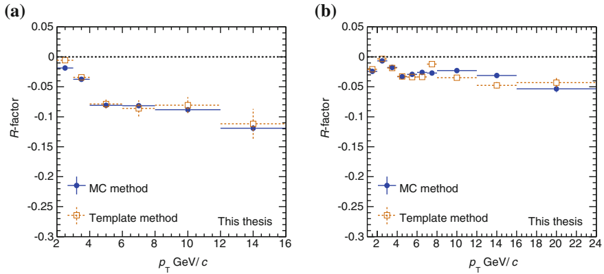
Fig. 5.24 R -factor as a function of D^0 p_T obtained with Monte Carlo ( blue ) and template fit ( orange ) methods for Pb–Pb collisions in the 30–50% centrality class ( a ) and for minimum-bias p–Pb collisions ( b ). The comparison is shown for the case with PID selection applied for all momenta
