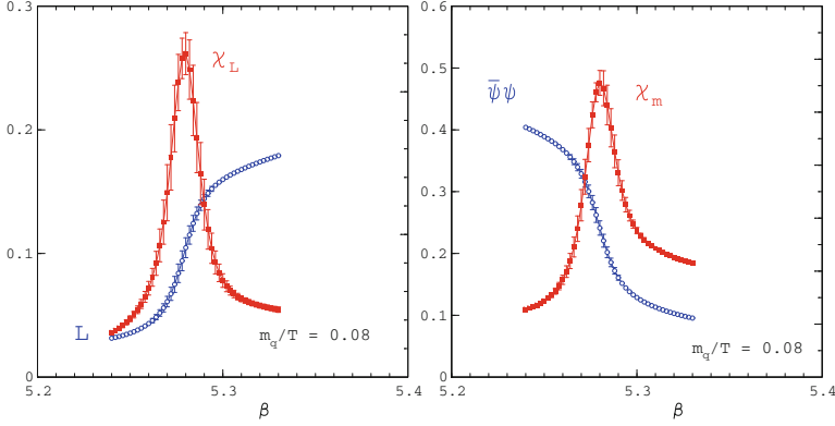
Fig. 1.4 Deconfinement and chiral symmetry restoration in 2-flavour QCD: \langle L \rangle , the order parameter for deconfinement in the limit of m_q \rightarrow \infty , and its susceptibility (left), and \bar{\psi}\psi , the order parameter for chiral symmetry breaking in the chiral limit ( m_q \rightarrow 0 ) and its susceptibility (right) as a function of the coupling \beta = 6/g^2 [16]
