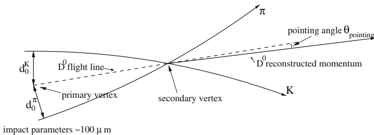
Fig. 5.2 Schematic representation of the D^0 \rightarrow K^- \pi^+ decay with the impact parameters ( d_0 ) and the pointing angle ( \theta_{\text{pointing}} )
