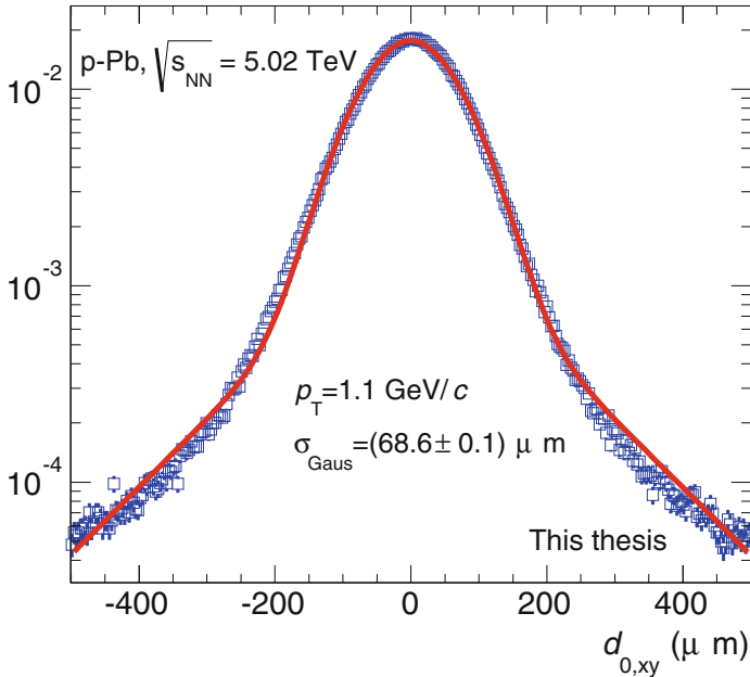
Fig. 3.12 Fit to the distribution of the r\varphi component of the impact parameter for tracks of p_T = 1.1 GeV/ c in p-Pb collisions. The fit function (red) is the sum of a Gaussian and two exponential functions. The width of the Gaussian, which is indicated, represents the estimate of the d_0 resolution at that p_T
