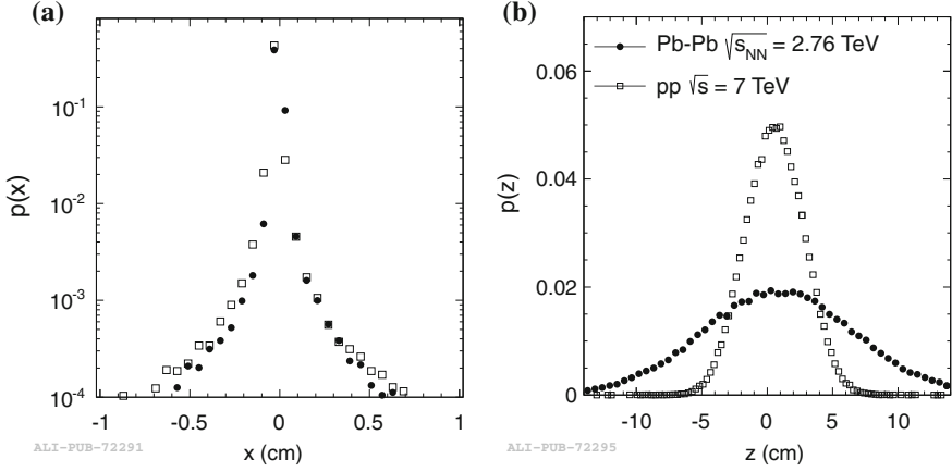
Fig. 3.7 The x (a) and z (b) projections of the luminous region obtained from reconstructed vertices in pp and Pb–Pb collisions (folded with vertex resolution) [7]
