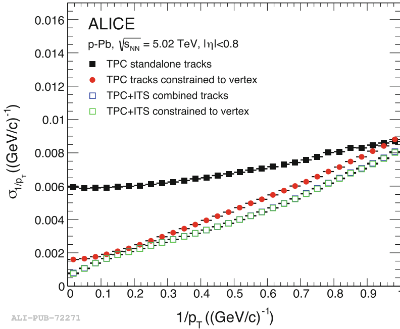
Fig. 3.6 The p_T -resolution for standalone TPC and ITS-TPC matched tracks with and without constraint to the vertex. The vertex constraint significantly improves the resolution of TPC standalone tracks. For ITS-TPC tracks, it has no effect (green and blue squares overlap) [7]
