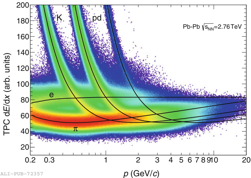
Fig. 3.9 Specific energy loss ( dE/dx ) in the TPC versus particle momentum in Pb–Pb collisions at \sqrt{s_{NN}} = 2.76 TeV. The lines show the parametrization of the expected mean energy loss [7]
