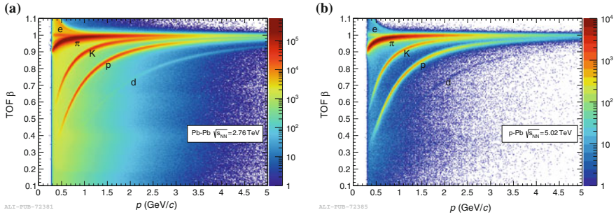
Fig. 3.10 Distribution of \beta as measured by the TOF detector as a function of momentum for particles reaching TOF in Pb-Pb interaction (a) and in p-Pb interactions (b). The background of mismatched tracks is lower in p-Pb than in higher occupancy Pb-Pb collisions [7]
