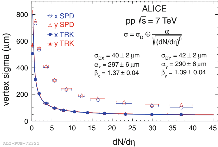
Fig. 3.8 Transverse width of the final vertex distribution ( solid points ), decomposed into the finite size of the luminous region \sigma_D and the vertex resolution \alpha/\sqrt{(dN_{ch}/d\eta)^\beta} . The widths of preliminary (SPD) interaction vertices are shown as open points [7]
