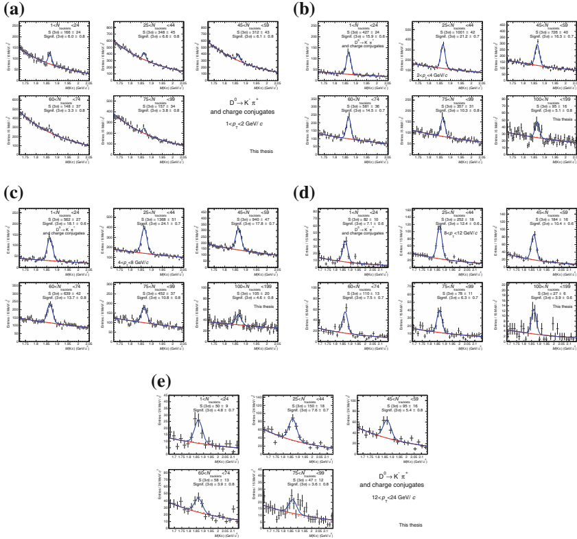
Fig. 5.16 D^0 invariant mass distributions as a function N_{\text{tracklets}} for the five p_T intervals considered for the analysis
