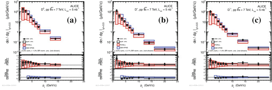
Fig. 2.1 p_T -differential inclusive cross section in pp collisions at \sqrt{s} = 7 TeV of prompt D^0 (a), D^+ (b), and D^{*+} (c) compared with pQCD calculations [11]
