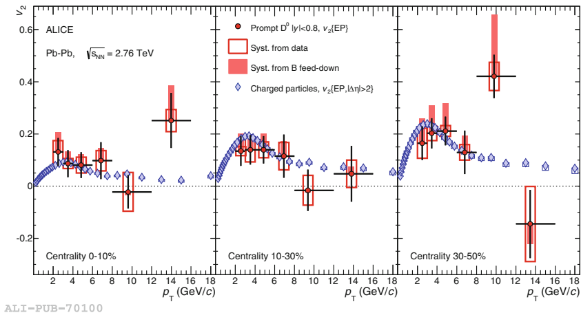
Fig. 7.4 Comparison of prompt D^0 meson and charged-particle v_2 [2] in three centrality classes as a function of p_T . Both measurements were done with the event-plane method [3]
