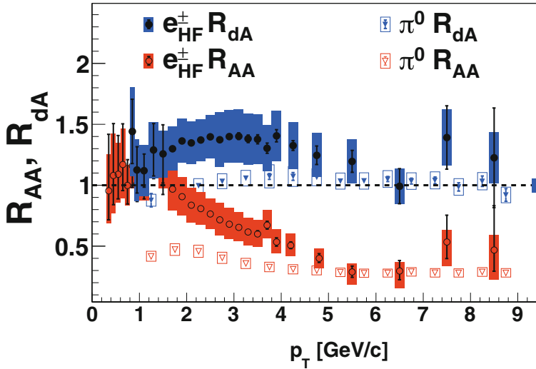
Fig. 2.15 The nuclear modification factors for minimum-bias d–Au and Au–Au collisions for \pi^0 and heavy-flavour electrons [69]
