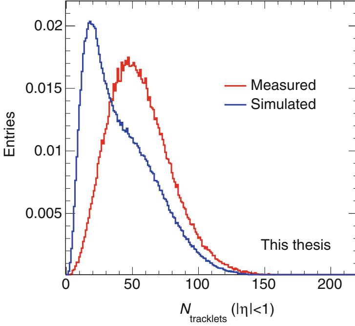
Fig. 5.27 Distributions of the number of SPD tracklets ( N_{\text{tracklets}} ) in |\eta| < 1 obtained from data (red) and from simulation (blue). The two distributions are normalized to their integral
