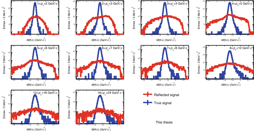
Fig. 5.19 Invariant mass distributions of the simulated true and reflected signal in p–Pb collisions
