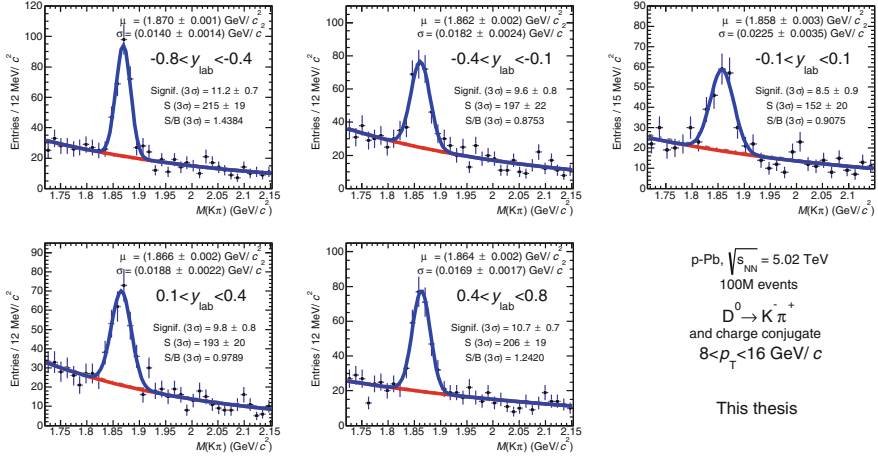
Fig. 5.10 Distributions of the invariant mass of D^0 candidates in p-Pb collisions in five rapidity intervals for 8 < p_T < 16 \text{ GeV}/c
