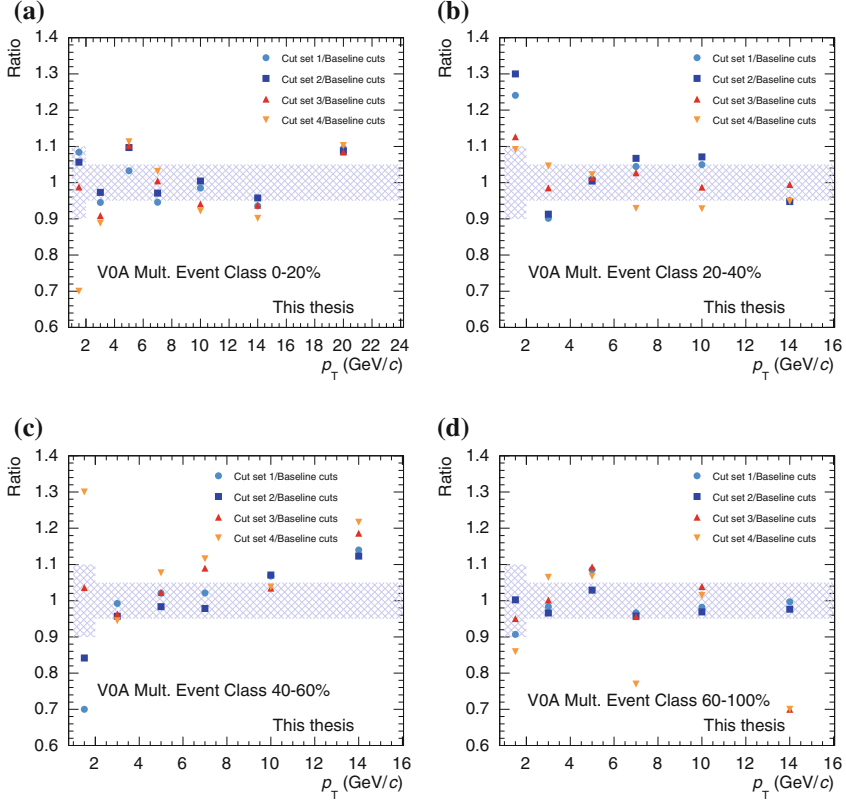
Fig. 6.11 Ratios of the corrected yields obtained with different cuts to those obtained with the baseline cut values as a function of p_T for 0–20% (a), 20–40% (b), 40–60% (c), and 60–100% (d) event-activity classes defined with the V0A estimator in p–Pb collisions
