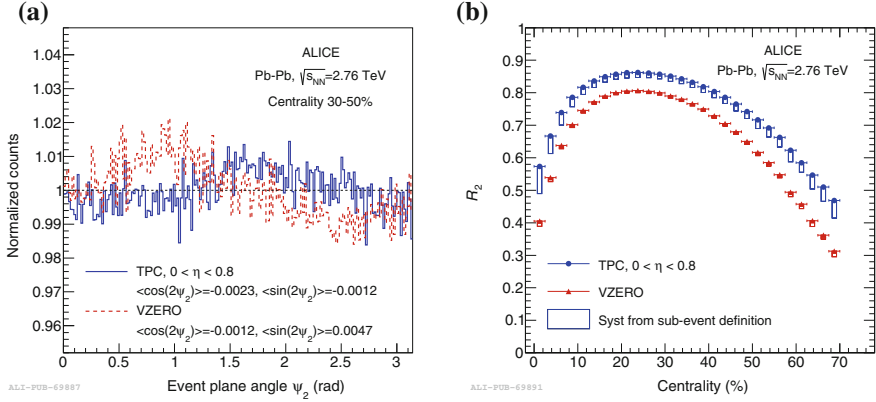
Fig. 5.1 a Distribution of event-plane angle \psi_2 , estimated from TPC tracks with 0 < \eta < 0.8 (solid line) or with the VZERO detector signals (dashed line) in the centrality range 30–50%. The distributions are normalized by their integral [3]. b Event-plane resolution correction factor R_2 as a function of centrality for the TPC and VZERO detectors. The boxes represent the systematic uncertainties estimated from the variation of R_2 when changing the subevents used for its determination [3]
