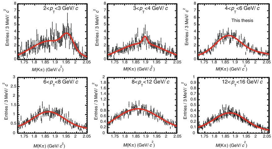
Fig. 5.22 Double gaussian fit to the simulated invariant mass distributions of reflections in Pb–Pb collisions in the 30–50% centrality class. The obtained fit functions (red lines) were included as templates of the reflected signal in the invariant mass fit procedure on data
