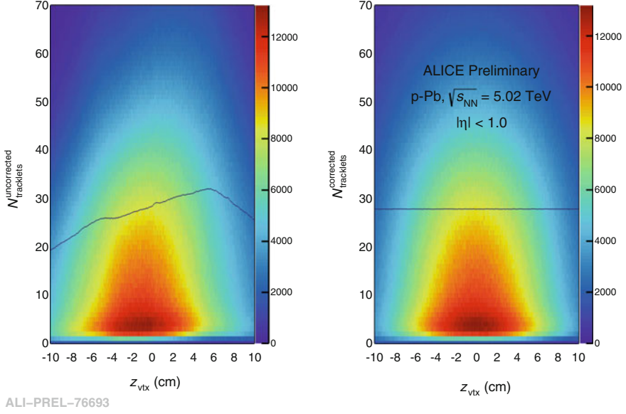
Fig. 5.14 z_{\text{vtx}} distributions of multiplicity estimated with N_{\text{tracklets}} in |\eta| < 1 . In the left panel is reported the raw distribution which demonstrates the variation of the SPD acceptance with time and z_{\text{vtx}} . In the right panel the corrected distribution is shown
