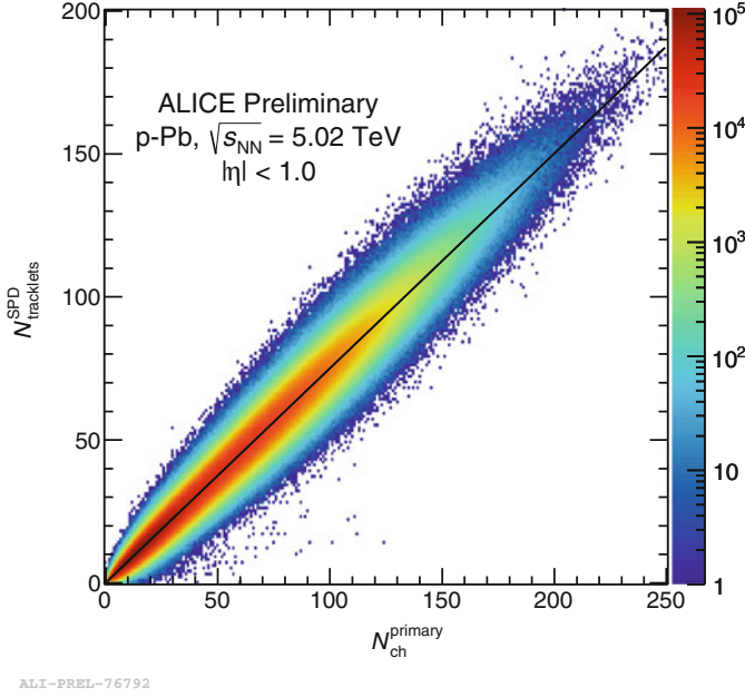
Fig. 5.15 SPD N_{\text{tracklets}} multiplicity as a function of the primary charged-particle multiplicity in Monte Carlo simulations. The black line indicates the profile of the distribution: linear proportionality was found with a factor of 0.75
