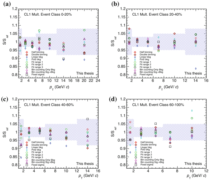
Fig. 6.4 Raw yield ratios relative to the signal yield extracted with the default fit procedure as a function of p_T for 0–20 % (a), 20–40 % (b), 40–60 % (c), and 60–100 % (d) event-activity classes defined with the CL1 estimator in p–Pb collisions
