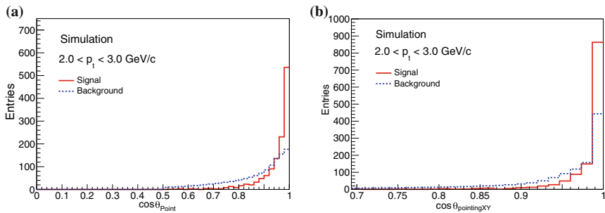
Fig. 5.5 a Distribution of the cosine of the pointing angle \cos \theta_{\text{pointing}} for signal ( red ) and background ( blue ) candidates in Pb–Pb Monte Carlo. b Distribution of the cosine of the pointing angle measured in the transverse plane \cos \theta_{\text{pointing}}^{xy} for signal and background candidates measured in a HIJING charm enriched Monte Carlo
