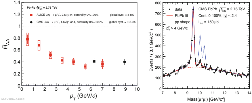
Fig. 1.13 a Transverse momentum dependence of the centrality integrated nuclear modification factor of the J/\psi p_T distribution in Pb–Pb at \sqrt{s_{NN}} = 2.76 TeV with respect to pp collisions. ALICE result refer to the rapidity range 2.5 < y < 4 [29], CMS one to 1.6 < y < 2.4 [30]. b Dimuon invariant mass distribution from Pb–Pb data at \sqrt{s_{NN}} = 2.76 TeV. The red line shows the fit to Pb–Pb data. The blue dashed line shows the shape obtained from the fit to pp data. For a better comparison, the background shape, background yield, mass peak width, mass peak tail shape and the \Upsilon(1S) yields in the blue line are fixed to the Pb–Pb fit, while the \Upsilon(2S)/\Upsilon(1S) and \Upsilon(3S)/\Upsilon(1S) ratios are fixed to the pp fit values [31]
