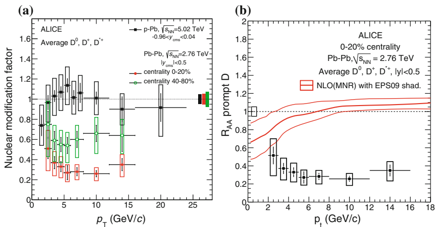
Fig. 8.6 (a) Average R_{\text{pPb}} of prompt D^0 , D^+ , and D^{*+} mesons as a function of p_{\text{T}} [1] compared to D meson R_{\text{AA}} in the 20 % most central and in the 40–80 % Pb–Pb collisions at \sqrt{s_{\text{NN}}} = 2.76 TeV [9]. (b) Average D meson R_{\text{AA}} in the 20 % most central Pb–Pb collisions at \sqrt{s_{\text{NN}}} = 2.76 TeV compared to the expectation from NLO pQCD with nuclear shadowing
