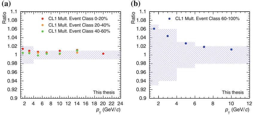
Fig. 6.16 Corrected yield ratios relative to the yield obtained with the reference N_{\text{tracklets}} weight function as a function of p_T for 0–20 %, 20–40 %, 40–60 % (a), and 60–100 % (b) event-activity classes defined with the CL1 estimator in p–Pb collisions
