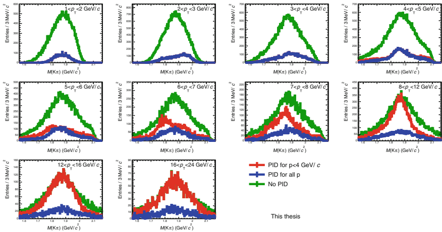
Fig. 5.20 Invariant mass distributions of the simulated reflections in p–Pb collisions. The distributions are reported for three different PID selections: PID not applied ( green lines ), PID applied only for tracks with momentum p < 4 \text{ GeV}/c ( red lines ), and PID applied for all the tracks ( blue lines )
