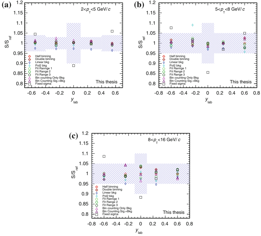
Fig. 6.3 Raw yield ratios relative to the signal yield extracted with the default fit procedure as a function of y_{\text{lab}} for 2 < p_T < 5 \text{ GeV}/c (a), 5 < p_T < 8 \text{ GeV}/c (b), and 8 < p_T < 16 \text{ GeV}/c (c) in p–Pb collisions. The shaded area indicates the assigned uncertainty due to yield extraction
