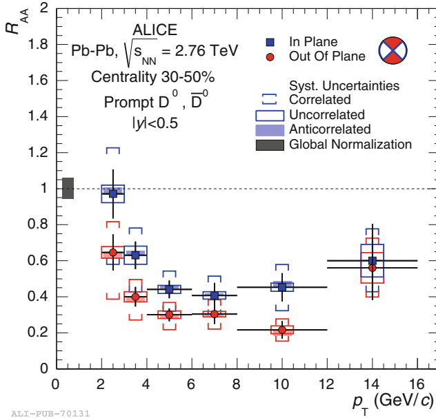
Fig. 7.8 Nuclear modification factor R_{AA} of D^0 in the 30–50% centrality class in two 90^\circ -wide azimuthal intervals centered on the in-plane and on the out-of-plane directions. The correlated, uncorrelated and anti-correlated contributions to the systematic uncertainty are shown separately [3]
