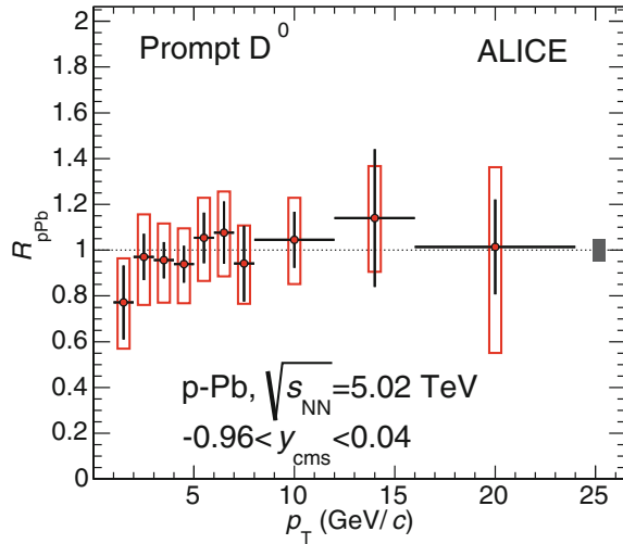
Fig. 8.3 R_{\text{pPb}} as a function of p_T for prompt D^0 mesons in p-Pb collisions at \sqrt{s_{\text{NN}}} = 5.02 TeV [1]
