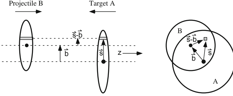
Fig. 1.8 Schematic representation of the optical Glauber model geometry with transverse and longitudinal views
