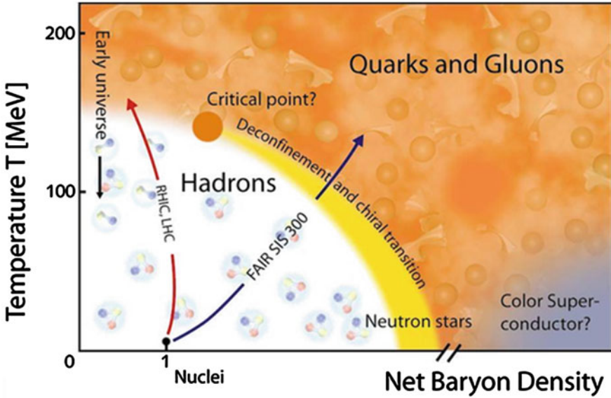
Fig. 1.3 Phase diagram of QCD matter as a function of temperature and net baryon density \rho_B
