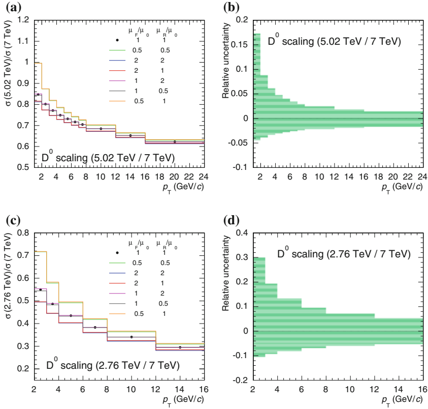
Fig. 6.20 FONLL scaling factor from 7 to 5.02 TeV (a) and its relative uncertainty (b), and from 7 to 2.76 TeV (c) and its relative uncertainty (d)
