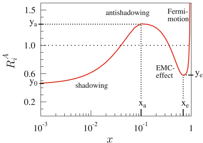
Fig. 2.12 Illustration of the nuclear modification of bound nucleons
