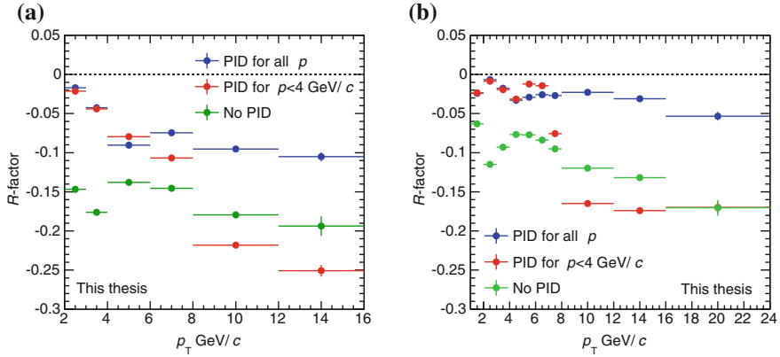
Fig. 5.21 R -factor as a function of D^0 p_T obtained with Monte Carlo method for Pb–Pb collisions in the 30–50% centrality class (a) and for minimum-bias p–Pb collisions (b) for three PID strategies: TPC and TOF 3\sigma compatibility band for all tracks (blue points), for tracks with p < 4 GeV/c (red points), and PID selection not applied
