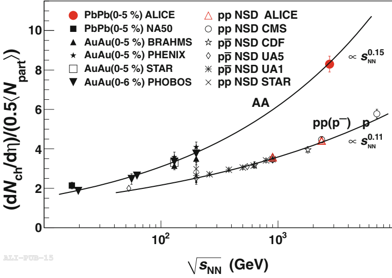
Fig. 1.10 Charged-particle pseudorapidity density per participant pair for central A–A and non-single diffractive pp ( \bar{p}\bar{p} ) collisions as a function of \sqrt{s_{NN}} . The solid lines \propto s_{NN}^{0.15} and \propto s_{NN}^{0.11} are superimposed on the heavy-ion and pp ( \bar{p}\bar{p} ) data, respectively [22]
