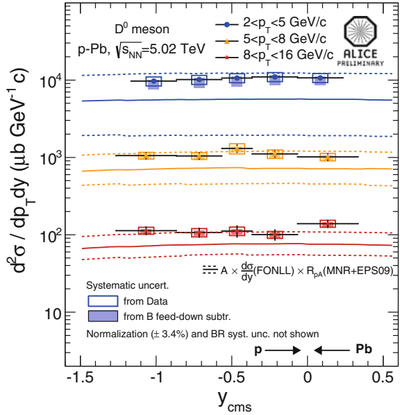
Fig. 8.2 y -differential production cross section of prompt D^0 mesons in p-Pb collisions at \sqrt{s_{NN}} = 5.02 TeV. The D^0 cross section is compared to a calculation based on NLO pQCD including the nuclear modification of the PDFs as parametrized in EPS09NLO [2], indicated with its uncertainty, by the curves
