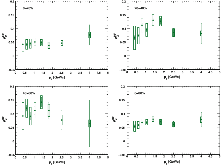
Fig. 2.11 Elliptic flow v_2 of electrons coming from semileptonic decays of heavy-flavour mesons measured in Au–Au collisions at \sqrt{s_{NN}} = 200 GeV by PHENIX for different collision centralities [17]
