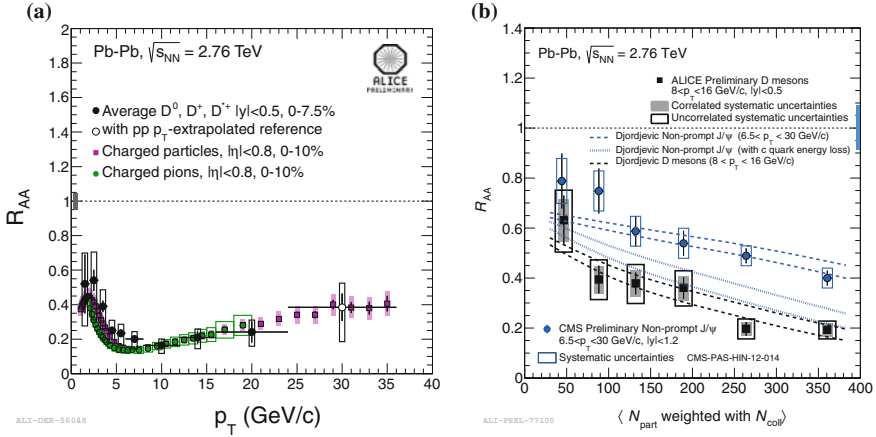
Fig. 2.8 a Nuclear modification factor R_{AA} as a function of p_T for D mesons, charged particles and charged pions measured in the central rapidity region for the most central Pb–Pb collisions [36]. b Centrality dependence of the R_{AA} of prompt D mesons [36] and of J/\psi from B meson decay [37] compared with a pQCD model including mass dependent radiative and collisional energy loss
