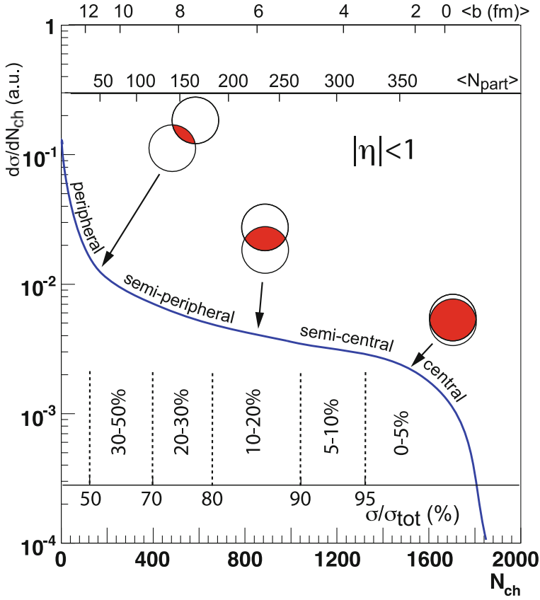
Fig. 1.9 Illustration of the correlation between the final state observable N_{\text{ch}} and Glauber calculated quantities ( b , N_{\text{part}} )
