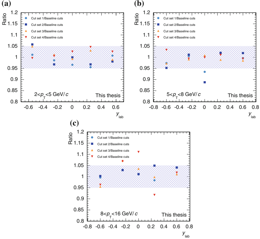
Fig. 6.10 Ratios of the corrected yields obtained with different sets of cuts to those resulting with the baseline cuts in p-Pb collisions. The variations are presented as a function of y_{\text{lab}} for the three p_T intervals considered in the analysis
