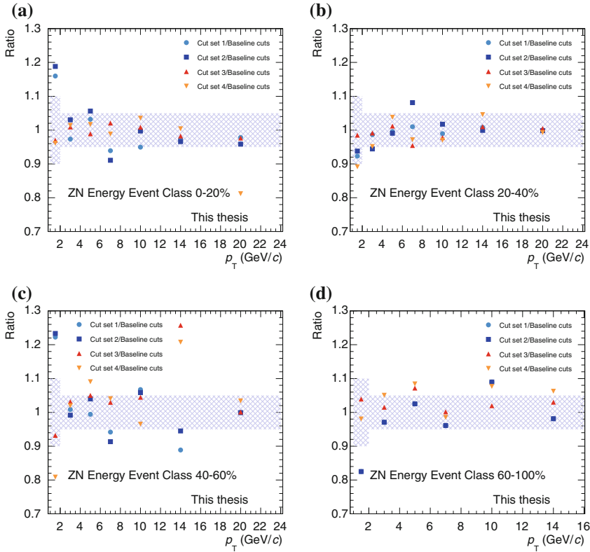
Fig. 6.12 Ratios of the corrected yields obtained with different cuts to those obtained with the baseline cut values as a function of p_T for 0–20% (a), 20–40% (b), 40–60% (c), and 60–100% (d) event-activity classes defined with the ZNA estimator in p-Pb collisions
