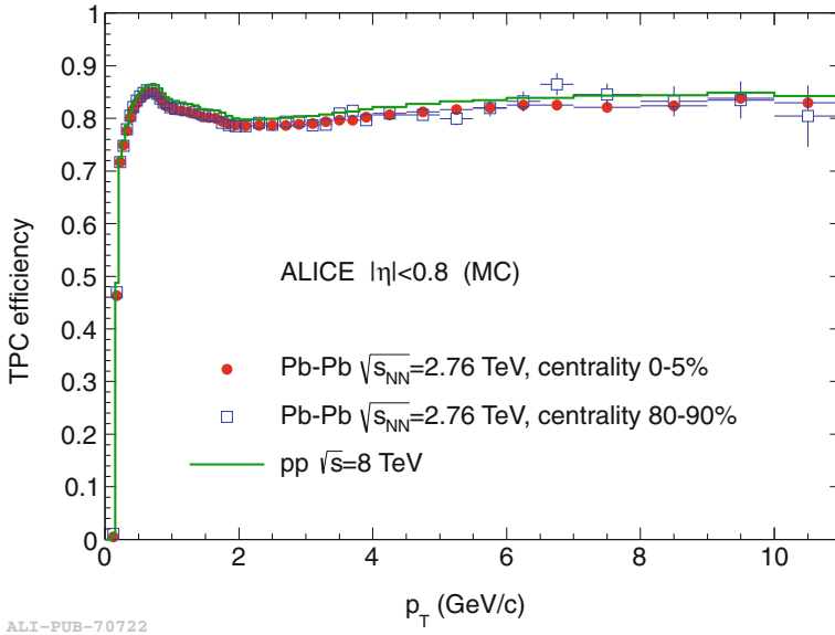
Fig. 3.4 TPC track finding efficiency for primary particles in pp and Pb–Pb collisions (simulation). The efficiency does not depend on the detector occupancy [7]
