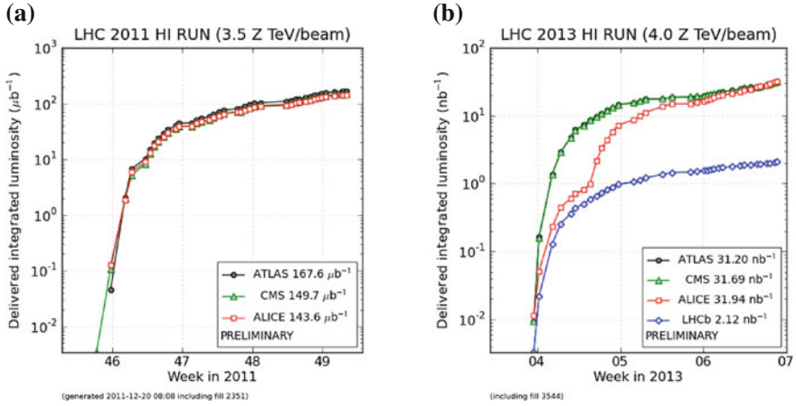
Fig. 3.2 LHC delivered integrated luminosity to the experiments during 2011 Pb–Pb run (a) and during 2013 p–Pb run (b) [4]
