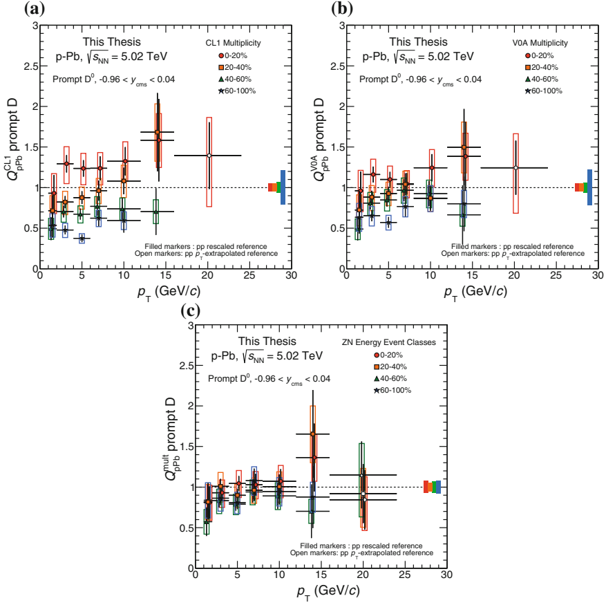
Fig. 8.7 Q_{pPb} as a function of p_T for prompt D^0 measured in four event-activity classes: 0–20 % (red), 20–40 % (orange), 40–60 % (green), and 60–100 % (blue). The results are shown for the three event-activity estimators considered: CL1 (a), V0A (b), and ZNA (c)
