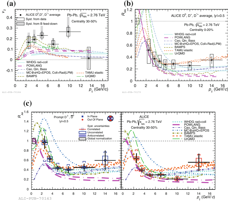
Fig. 7.9 Model comparison for average D meson v_2 in the 30–50 % centrality class [4] (a), average D meson R_{AA} in the 0–20 % centrality class [5] (b), D^0 R_{AA} in-plane and out-of-plane in the 30–50 % centrality class [3] (c). The seven models calculations are described in the text. The models WHDG rad+coll, POWLANG, TAMU elastic and UrQMD are shown by two lines that represent their uncertainty
