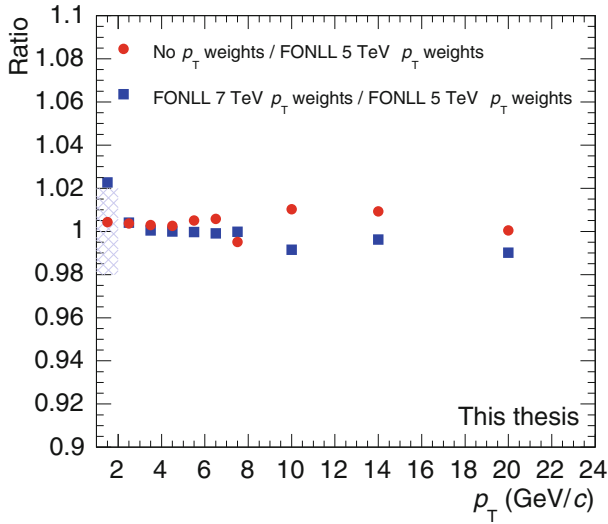
Fig. 6.14 Rapidity integrated efficiencies ratios as a function of p_T calculated to estimate the systematic uncertainty due to the simulated D^0 momentum distribution in p-Pb collisions
