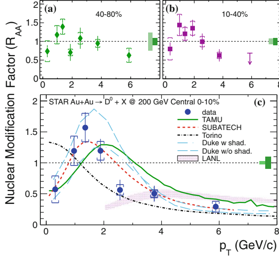
Fig. 2.7 D^0 R_{AA} measured by STAR for peripheral 40–80 % (a) and semi-central 10–40 % (b) collisions. c D^0 R_{AA} for 0–10 % most central events compared with model calculations [35]
