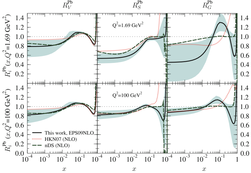
Fig. 2.13 Comparison of the average valence and sea quark, and gluon modifications at Q^2 = 1.69 \text{ GeV}^2 and Q^2 = 100 \text{ GeV}^2 for Pb nucleus from different global fits [46–48]
