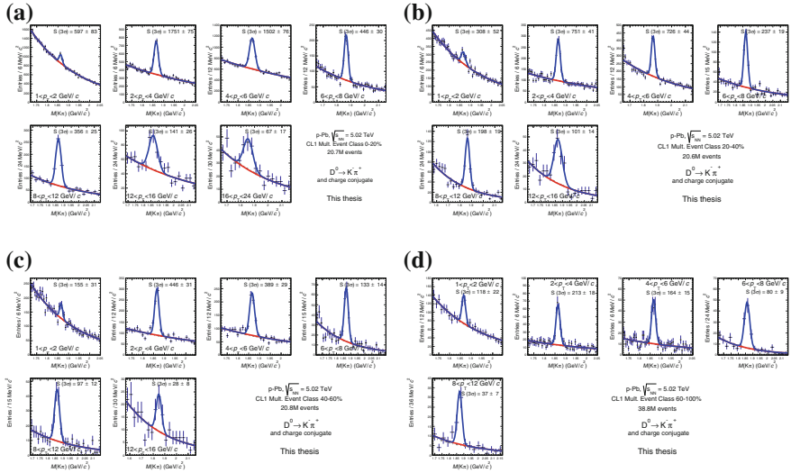
Fig. 5.11 D^0 invariant mass distributions for 0–20% (a), 20–40% (b), 40–60% (c), and 60–100% (d) event-activity classes defined with the CL1 estimator
