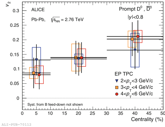
Fig. 7.5 D^0 meson v_2 with the event-plane method in three p_T intervals as a function of centrality [3]
