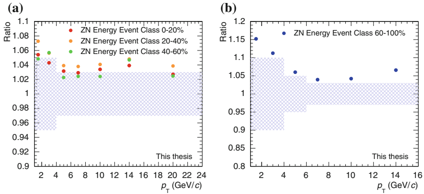
Fig. 6.18 Corrected yield ratios relative to the yield obtained with the reference N_{\text{tracklets}} weight function as a function of p_T for 0–20 %, 20–40 %, 40–60 % (a), and 60–100 % (b) event-activity classes defined with the ZNA estimator in p–Pb collisions
