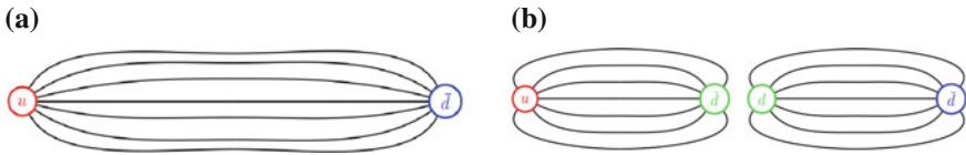
Fig. 1.1 a Bound quark-antiquark pair. Gluons exchange is responsible of the binding and it is represented by the flux tube containing the field lines. b Pulling apart the quarks, the energy of the gluon field increases until the flux tube breaks up in a new quark-antiquark pair
