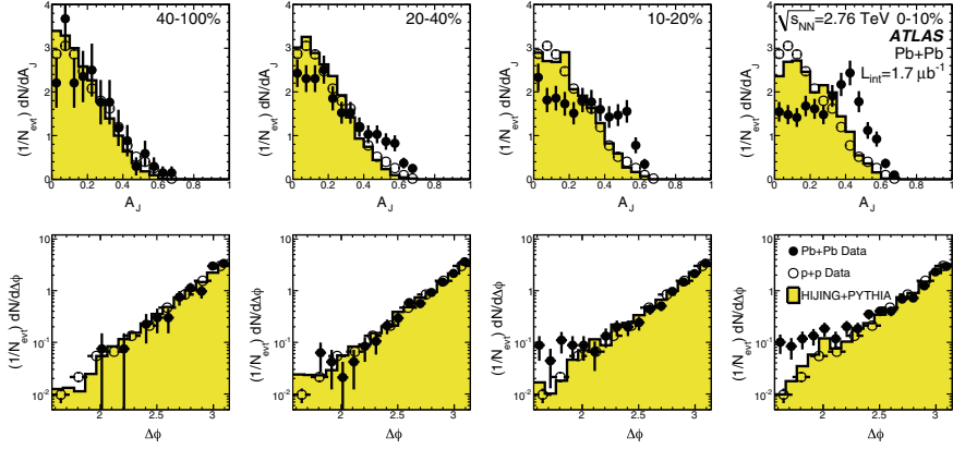
Fig. 2.6 Dijet asymmetry ( top ) and azimuthal angle between the leading and subleading jets ( bottom ) as a function of collision centrality (from peripheral to central) for pp and Pb–Pb collisions [33]
