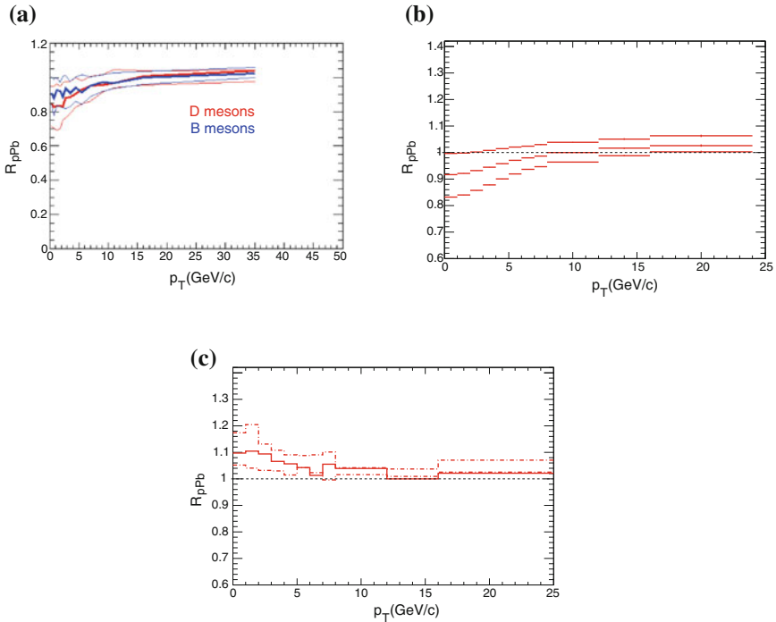
Fig. 5.34 a Calculation of the D and B meson nuclear modification factor including EPS09 shadowing. b Nuclear modification factor of D^0 from B decays obtained with EvtGen decayer and including shadowing. c Ratio of D^0 from B and prompt D^0 nuclear modification factors
