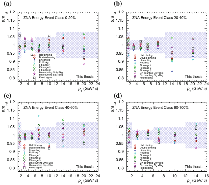
Fig. 6.6 Raw yield ratios relative to the signal yield extracted with the default fit procedure as a function of p_T for 0–20 % (a), 20–40 % (b), 40–60 % (c), and 60–100 % (d) event-activity classes defined with the ZNA estimator in p–Pb collisions
