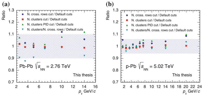
Fig. 6.19 Ratio of the corrected yields obtained when applying different single track quality cuts to those obtained with default cuts for 30–50 % Pb–Pb (a) and p–Pb collisions (b)
