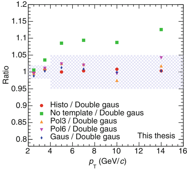
Fig. 6.1 Raw yield ratios relative to the signal yield extracted with the double-Gaussian template for the reflection contribution in Pb–Pb collisions in the 30–50% centrality class. The green points are obtained without subtracting the reflected signal, thus represent the bias on the signal. The red points are obtained using the generated reflections distributions as templates, the orange , magenta and blue points indicate the variation of the raw signal when the template function is varied and were used to extract the systematic uncertainty on c_{\text{refl}} factor (color figure online)
