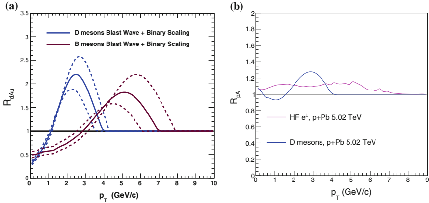
Fig. 2.14 a R_{dAu} obtained from the comparison of the blast-wave and FONLL [7–9] D and B meson p_T distributions with binary scaling. The dashed lines show the changes in the blast-waves expectations from the uncertainties on the blast-wave parameters. b R_{pA} predicted for p–Pb collisions at \sqrt{s_{NN}} = 5.02 TeV. Blast-wave fit results from the 5 % highest multiplicity p–Pb collisions [68] and FONLL [7–9] heavy-meson spectra have been used to generate these results [66]
