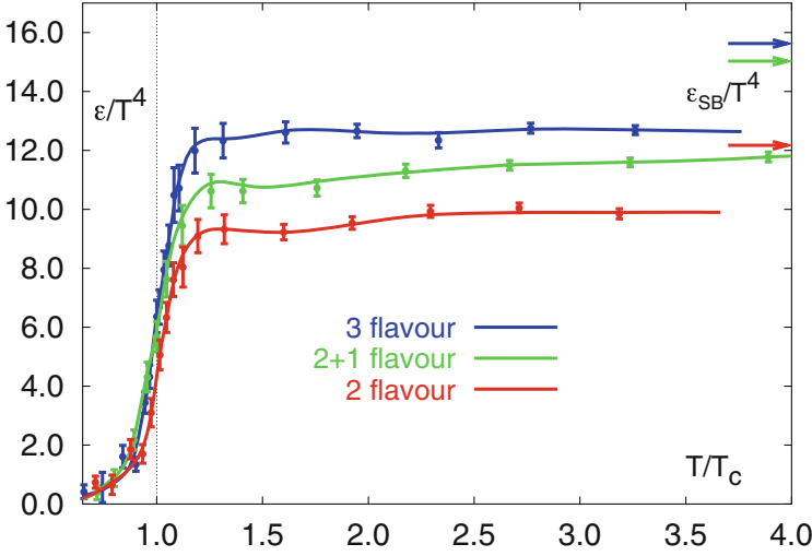
Fig. 1.6 The energy density in lattice QCD with different number of degrees of freedom (2 and 3 light quarks and 2 light plus 1 heavier quarks) as a function of temperature [19]
