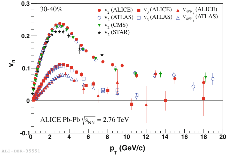
Fig. 2.10 Comparison of the ALICE results on v_n(p_T) to the analogous measurements from ATLAS and CMS collaborations, as well as v_2 measurements by STAR [40–43]
