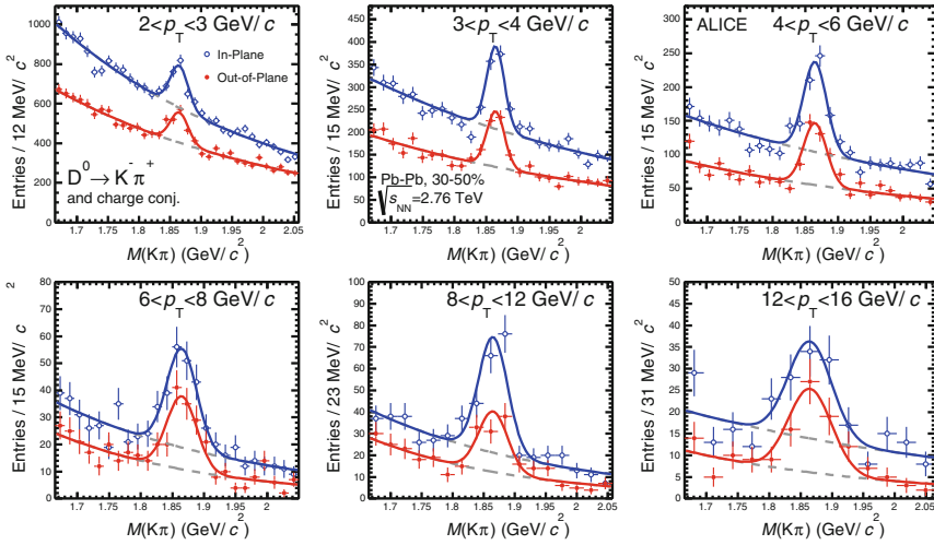
Fig. 5.6 Distributions of the invariant mass for D^0 in the two \Delta\varphi intervals, for Pb–Pb collisions in the 30–50 % centrality class [3]
