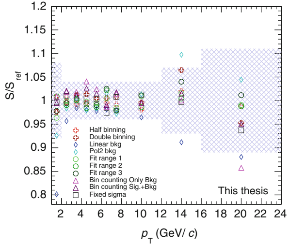
Fig. 6.2 Raw yield ratios relative to the signal yield extracted with the default fit procedure as a function of p_T in p–Pb collisions. The shaded area indicates the assigned uncertainty due to yield extraction
