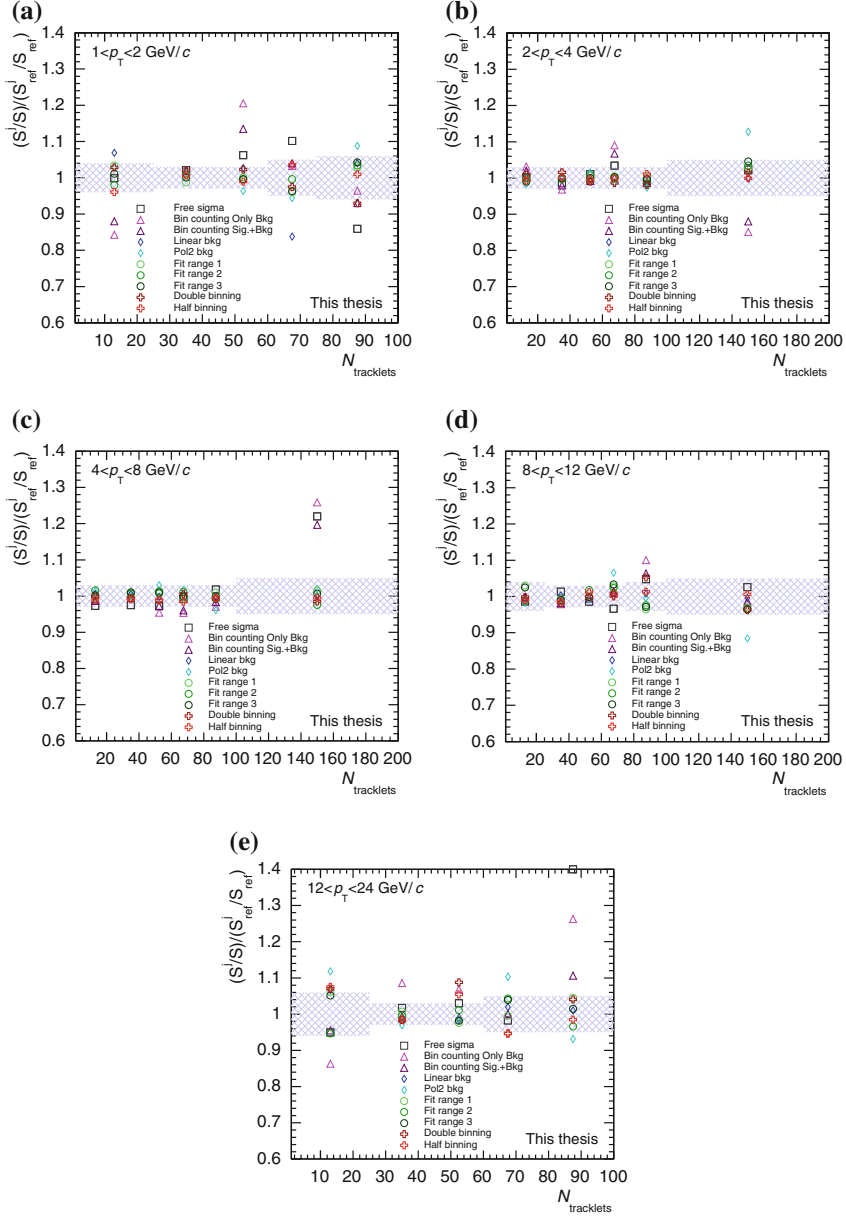
Fig. 6.7 D^0 yield extraction systematics as a function of N_{\text{tracklets}} for the five p_T intervals considered, in p-Pb collisions. The points represent the ratio of the relative yields extracted varying the fit procedure and the signal obtained with the standard fit procedure
