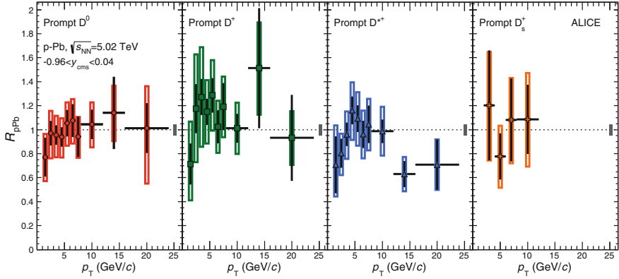
Fig. 8.4 R_{pPb} as a function of p_T for prompt D^0 , D^+ , D^{*+} and D_s^+ mesons in p-Pb collisions at \sqrt{s_{NN}} = 5.02 TeV [1]
