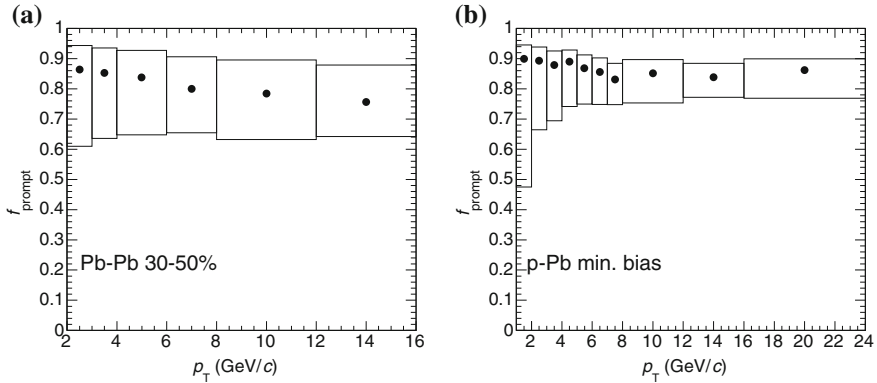
Fig. 5.33 a Fraction of prompt D^0 mesons obtained in Pb–Pb collisions in the 30–50 % centrality class with the hypothesis R_{AA}^{\text{feed-down}} = 2 \cdot R_{AA}^{\text{prompt}} . b Fraction of prompt D^0 mesons obtained in p–Pb collisions with the hypothesis R_{p\text{Pb}}^{\text{feed-down}} = R_{p\text{Pb}}^{\text{prompt}} . The open boxes indicate the uncertainty (see Chap. 6) obtained considering the variation of the hypothesis and the two methods to calculate f_{\text{prompt}}
