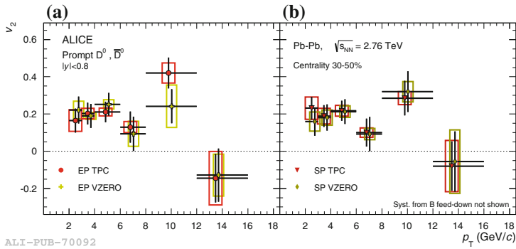
Fig. 7.7 D^0 meson v_2 as a function of p_T in the 30–50 % centrality class, with reference particles from TPC or from the VZERO detectors. a Event-plane method. b Scalar product method [3]
