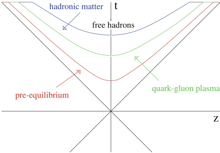
Fig. 1.7 Schematic representation of the expected space-time evolution of an ultra-relativistic heavy-ion collision
