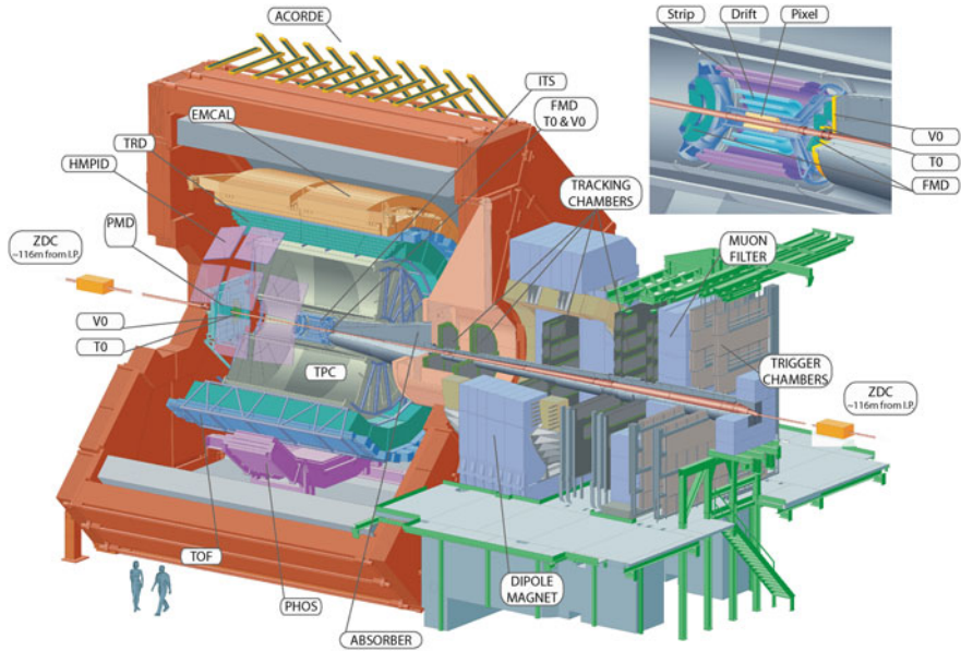
Fig. 3.3 The ALICE experiment at the CERN LHC. The central-barrel detectors are embedded in a solenoid with magnetic field B = 0.5 T and address particle production at midrapidity. The cosmic-ray trigger detector ACORDE is positioned on top of the magnet. Forward detectors are used for triggering, event characterization, and multiplicity studies. The Muon Spectrometer covers -4.0 < \eta < -2.5
