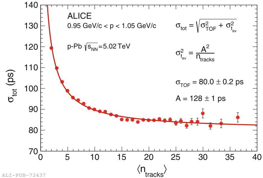
Fig. 3.11 Time resolution of pion track with 0.95 < p < 1.05 \text{ GeV}/c as a function of the number of tracks used to define the start time of the collision t_{ev} . The data are from p-Pb collisions [7]
