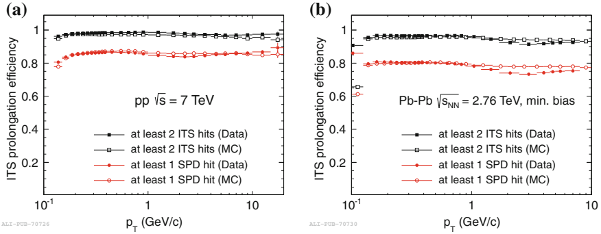
Fig. 3.5 ITS-TPC matching efficiency versus p_T for data and Monte Carlo for pp (a) and Pb-Pb (b) collisions [7]
