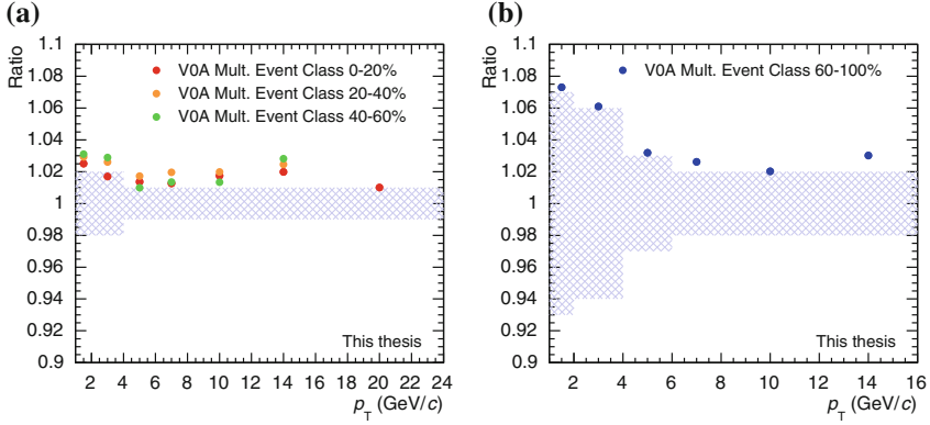
Fig. 6.17 Corrected yield ratios relative to the yield obtained with the reference N_{\text{tracklets}} weight function as a function of p_T for 0–20 %, 20–40 %, 40–60 % (a), and 60–100 % (b) event-activity classes defined with the V0A estimator in p–Pb collisions
