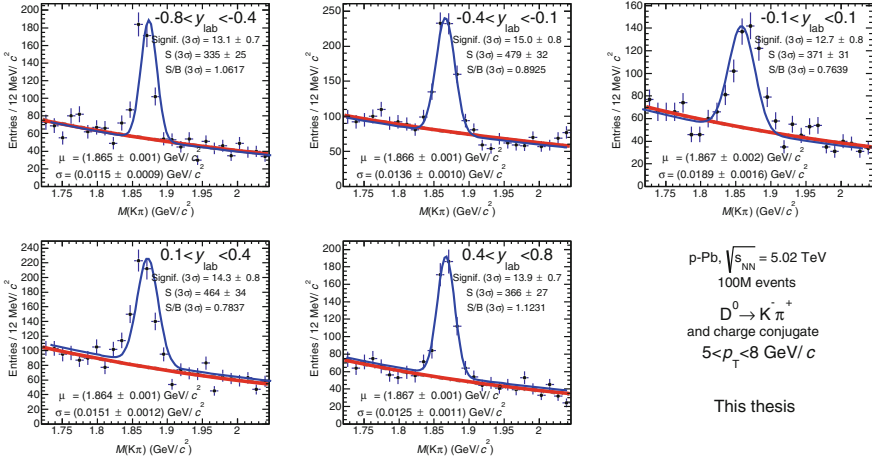
Fig. 5.9 Distributions of the invariant mass of D^0 candidates in p-Pb collisions in five rapidity intervals for 5 < p_T < 8 \text{ GeV}/c
