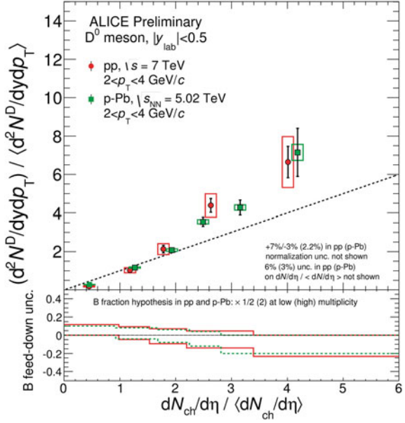
Fig. 8.9 D^0 meson relative yields as a function of relative charged-particle multiplicity in p–Pb collisions at \sqrt{s_{NN}} = 5.02 TeV and in pp at \sqrt{s} = 7 TeV. The relative yields, measured in the 2 < p_T < 4 GeV/c interval, are presented in the top panel with their statistical and systematic uncertainties, the relative uncertainty due to the B feed-down fraction is reported in the bottom panel . The points are located on the x -axis at the average value of (dN_{ch}/d)/\langle dN_{ch}/d \rangle for every N_{tracklets} interval
