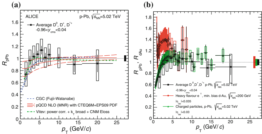
Fig. 8.5 Average R_{pPb} of prompt D^0 , D^+ , and D^{*+} mesons as a function of p_T (black) [1] compared to model calculations (a), and to heavy-flavour electron R_{dAu} measured in minimum bias d–Au collisions at \sqrt{s_{NN}} = 200 GeV [4], and to charged-particle R_{pPb} in minimum bias p–Pb collisions at \sqrt{s_{NN}} = 5.02 TeV [5] (b)
