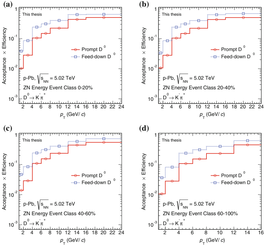
Fig. 5.31 (Acc \times \epsilon ) as a function of p_T for prompt and feed-down D^0 in 0–20% (a), 20–40% (b), 40–60% (c), and 60–100% (d) event-activity classes defined with the ZNA estimator
