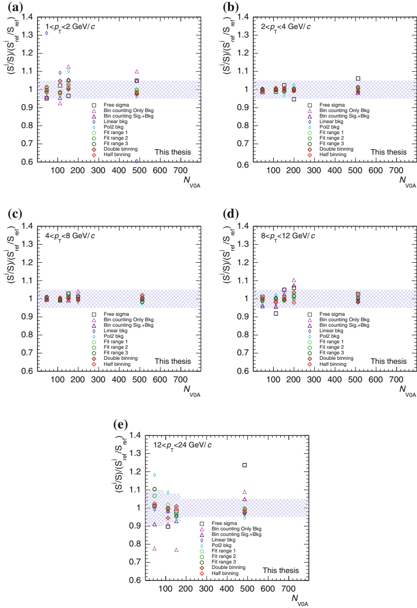
Fig. 6.8 D^0 yield extraction systematics as a function of N_{V0A} for the five p_T intervals considered, in p-Pb collisions. The points represent the ratio of the relative yields extracted varying the fit procedure and the signal obtained with the standard fit procedure
