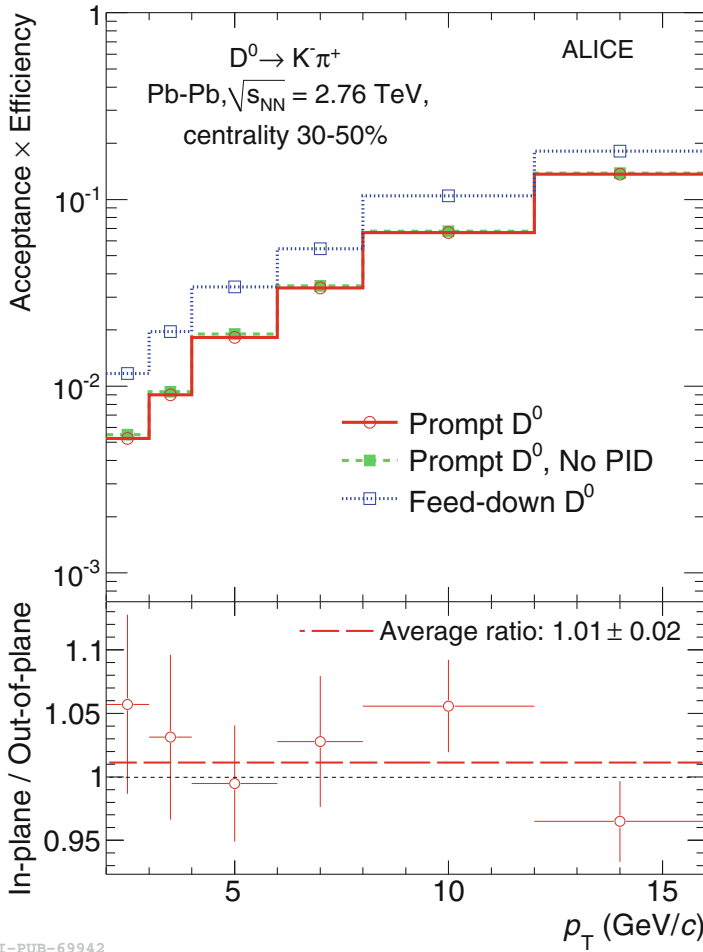
Fig. 5.25 Product of acceptance and efficiency for D^0 mesons in Pb-Pb collisions for 30–50% centrality class ( upper panel ). The values for prompt ( solid line ) and feed-down ( dotted line ) D^0 mesons are shown. The dashed line stands for the values obtained without PID selection. The lower panel shows the ratio of the efficiencies for prompt D^0 in the in-plane and the out-of-plane regions used for the analysis. The ratio was estimated using simulation samples with a difference in particle multiplicity similar to that observed in data for the two azimuthal regions [3]
