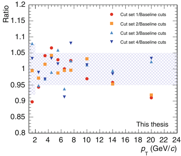
Fig. 6.9 Ratios of the corrected yields obtained with different sets of cuts to those resulting with the baseline cuts in p–Pb collisions
