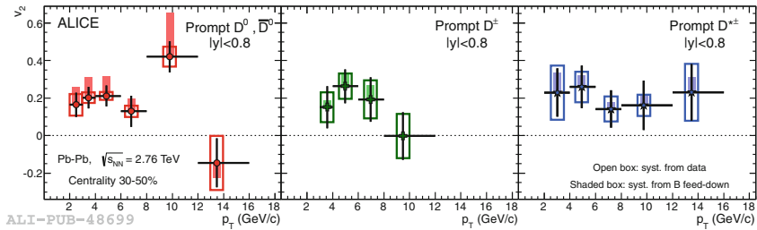
Fig. 7.2 v_2 as a function of p_T for prompt D^0 , D^+ , and D^{*+} mesons for Pb–Pb collisions in the 30–50 % centrality class [4]
