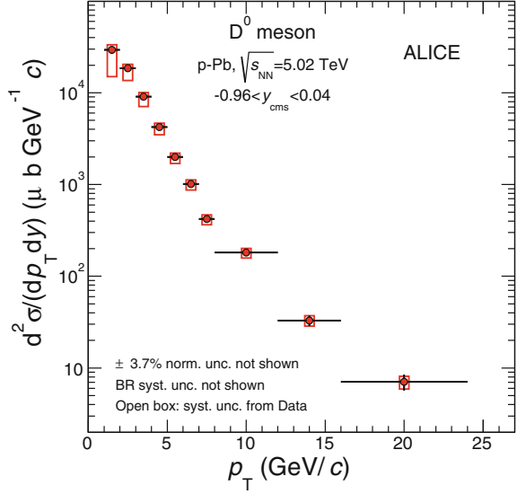
Fig. 8.1 p_T -differential inclusive production cross section of prompt D^0 mesons in p-Pb collisions at \sqrt{s_{NN}} = 5.02 TeV [1]
