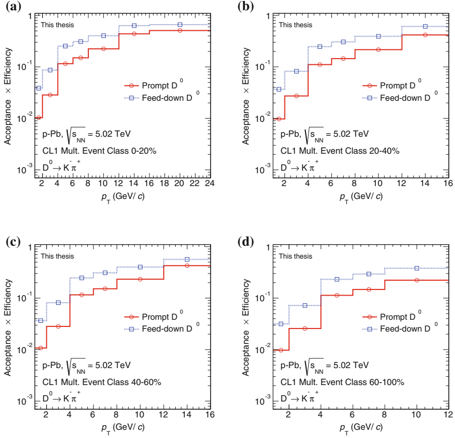
Fig. 5.29 ( \text{Acc} \times \epsilon ) as a function of p_T for prompt (red) and feed-down (blue) D^0 in 0–20 % (a), 20–40 % (b), 40–60 % (c), and 60–100 % (d) event-activity classes defined with the CL1 estimator
