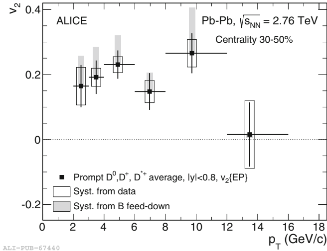
Fig. 7.3 Average of D^0 , D^+ , and D^{*+} v_2 as a function of p_T in the 30–50% centrality class, measured with the event-plane method. The symbols are positioned horizontally at the average p_T of the three D meson species [4]
