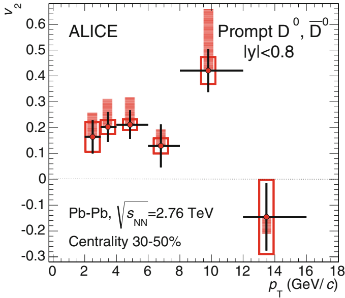
Fig. 7.1 Elliptic flow v_2 as a function of p_T for prompt D^0 mesons measured with the event-plane method in Pb–Pb collisions in the 30–50 % centrality class [4]
