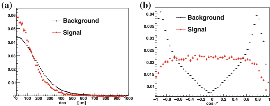
Fig. 5.3 a Distance of closest approach ( dca ) of signal ( red ) and background ( black ) D^0 candidates obtained with a pp PYTHIA simulation. b Distribution of the \theta^* angle for signal and background candidates. For signal the distribution is almost flat due to the isotropic emission of the pion and the kaon in the centre-of-mass system
