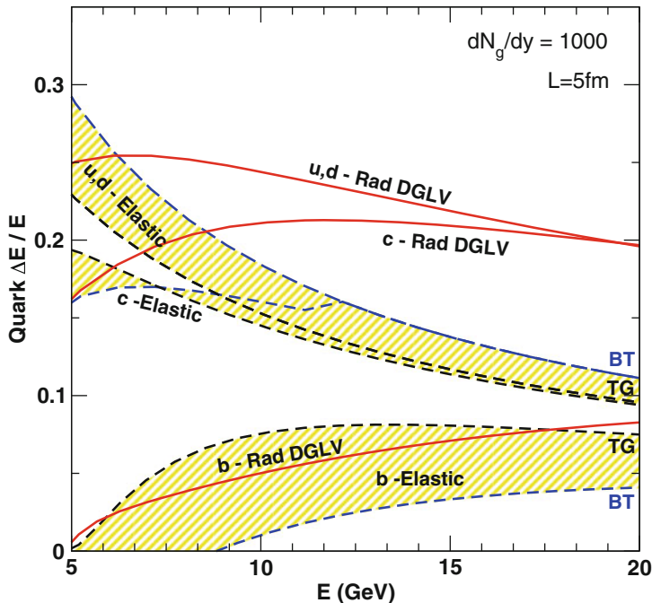
Fig. 2.5 Average relative energy loss, \Delta E/E , for u , c and b quarks as a function of the energy in a longitudinally expanding QGP with fixed path length L = 5 fm, initial gluon density dN_g/dy = 1000 and fixed \alpha_s = 0.3 . Solid lines indicate radiative energy loss while collisional (elastic) energy loss is indicated with dashed bands [25]
