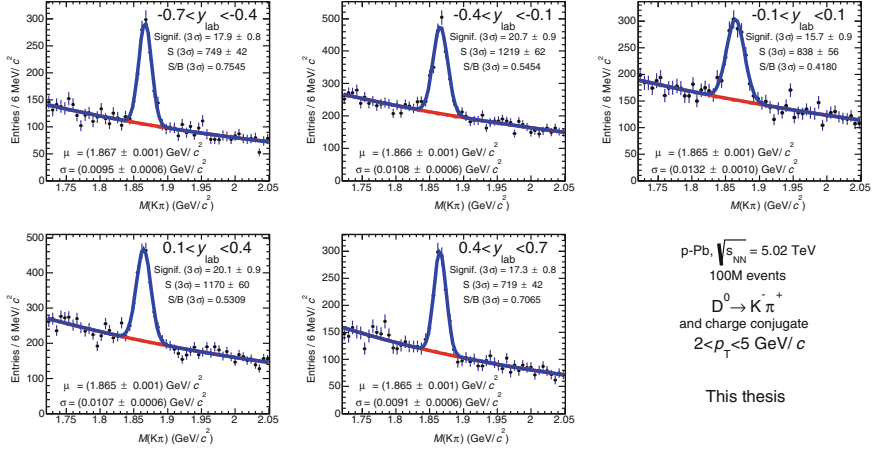
Fig. 5.8 Distributions of the invariant mass of D^0 candidates in p-Pb collisions in five rapidity intervals for 2 < p_T < 5 \text{ GeV}/c
