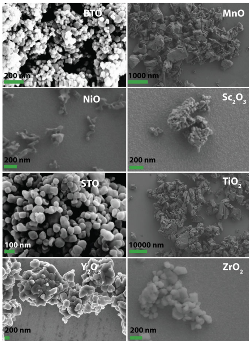
Fig. 4.5 SEM images of powders showing the large difference in particle sizes. Scale bars are shown in green
