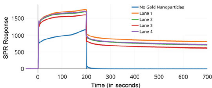
Fig. A.4 Control studies to show no interaction of PEG with the chemically active linker surface. Lanes 1, 2, 3 and 4 have gold nanoparticles and PEG is seen to adsorb onto the captured nanoparticles. When there are no captured gold nanoparticles, PEG doesn't adsorb at all onto the chip surface
