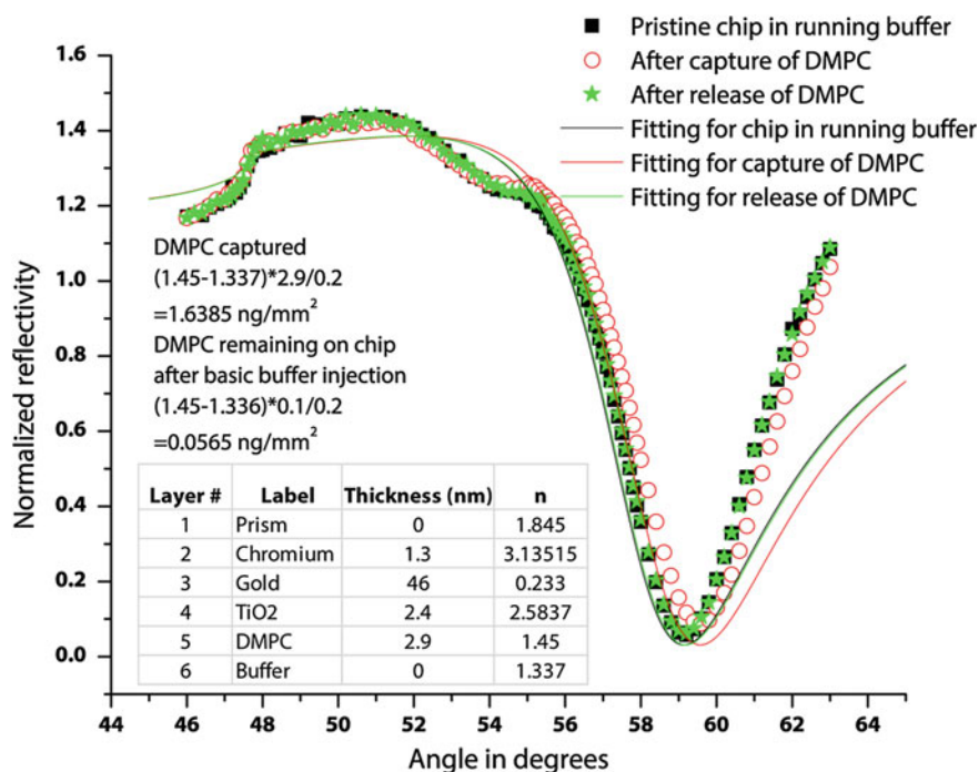
Fig. 4.10 Angular spectrum showing shifts in resonant dips upon binding and unbinding DMPC. The actual and fitted data is shown. The estimation of mass on the TiO 2 surface is derived and displayed in the inset. n is refractive index. Details of calculation can be found in Sect. 4.4.5
