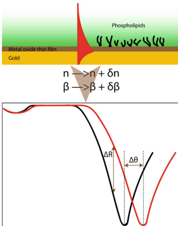
Fig. 2.9 Working principle of SPR biosensor in angular mode of operation, used in Chap. 4 to find amount of phospholipid bound to thin film of metal oxide
