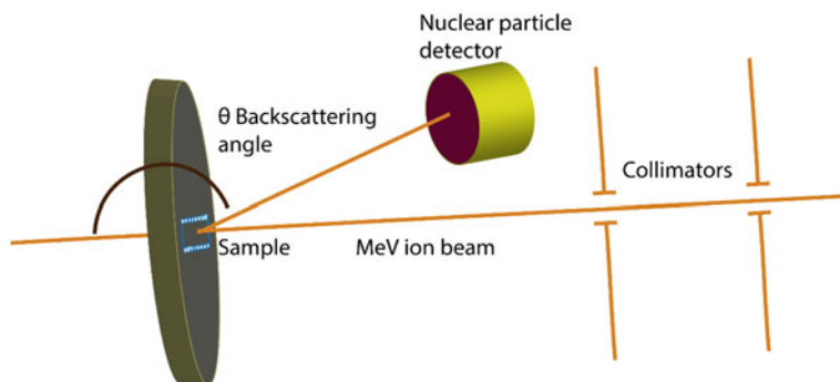
Fig. 2.10 Rutherford backscattering spectroscopy layout
