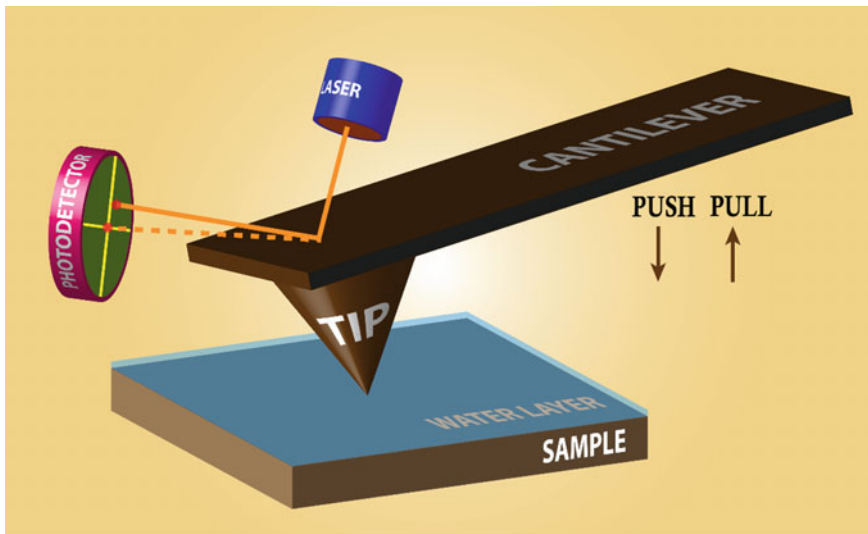
Fig. 2.2 Schematic of an AFM setup
