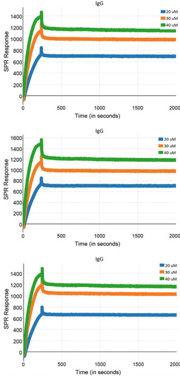
Fig. A.3 SPR Sensorgram for IgG interacting with AuNPs. Different colours represent different concentrations. Concentrations shown in legend. 3 sets of data have been shown
