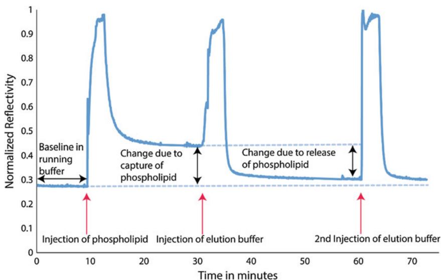
Fig. 4.9 The capture and release of the phospholipid DMPC from a 3 nm film of \text{TiO}_2 observed through surface plasmon resonance. Various events have been marked on the plot
