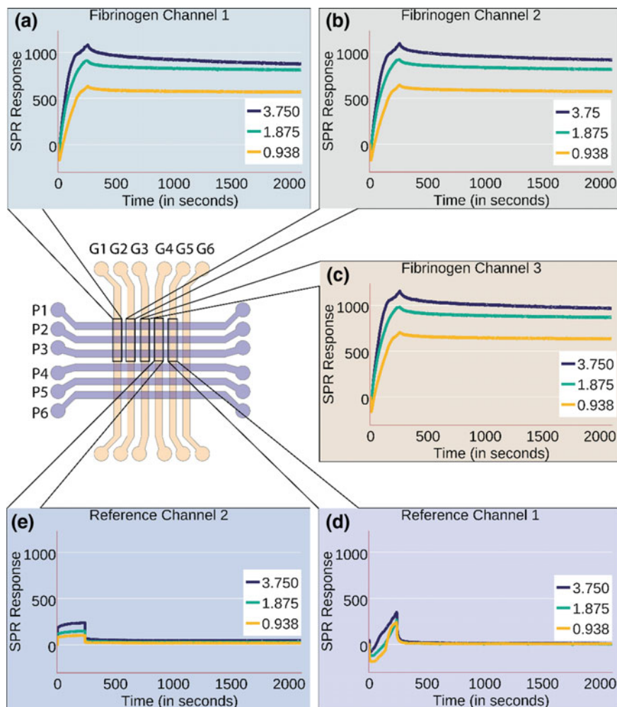
Fig. 5.3 The microfluidic channel setup allowing multiplexed data collection is shown. AuNPs are immobilized in 3 channels G1, G2 and G3 using EDC/S-NHS coupling as described. Two control channels (G4 and G5) are employed. G4 channel is modified with all the linker chemistry used to capture AuNPs (but AuNPs are not injected). G5 channel is in as received condition (alginate layer with inactive -\text{COOH} groups). Fibrinogen in three concentrations (3.750, 1.775 and 0.938 \mu\text{M} ) is injected along channels P1, P2 and P3 respectively. The three colored lines (blue, green, yellow) in each panel correspond to 3 different concentrations of fibrinogen used in the experiment (legend in white box in each panel) a , b and c Sensorgrams showing the interaction of fibrinogen with bare AuNPs available in channels G1, G2 and G3. d Sensorgram resulting from the interaction of fibrinogen with the chemically active lane without the AuNPs. e Sensorgram showing the interaction of fibrinogen with the unmodified surface (alginate polymer layer)
