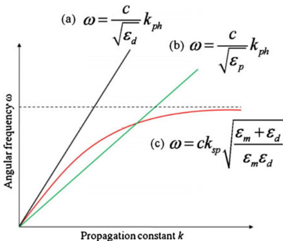
Fig. 2.5 The dispersion relation of free photons in a dielectric (a), and in a coupling prism (b) with \epsilon_p > \epsilon_d , compared to the dispersion relation of non-radiative surface plasmons (c) at the metal/dielectric interface
