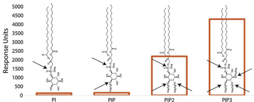
Fig. 4.12 Differences in adhesion based on number of phosphate groups. Phosphate groups have been marked with black arrow
