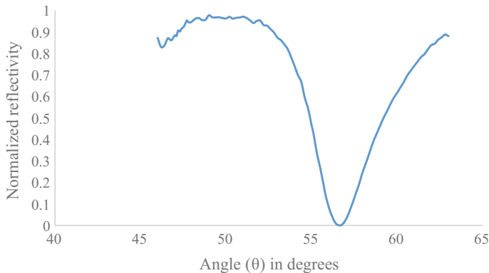
Fig. 2.7 Angular spectrum of reflectivity showing a dip at 56^\circ
