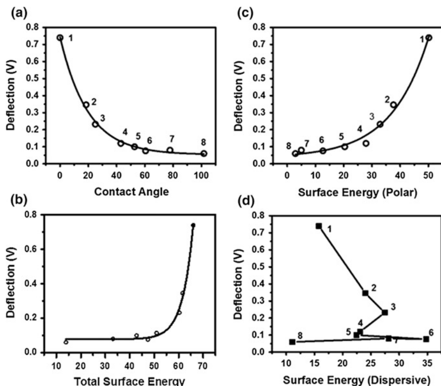
Fig. 3.5 The maximum pulling force plotted versus different parameters obtained from macroscale contact angle measurements, the maximum pull-off force versus a water contact angle b total surface energy c polar component of surface energy d dispersive component of surface energy (1 mica, 2 VO 2 (B) grown on STO, 3 VO 2 (M) grown on STO, 4 cover slip glass, 5 hard disk media, 6 STO substrate, 7 Lu 2 O 3 grown on YSZ, 8 lubricated hard disk media)
