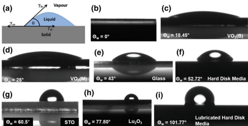
Fig. 3.1 Water contact angle measurement a schematic of measurement b–i different surfaces having contact angle ranging from 0^\circ to \sim 102^\circ
