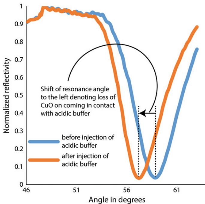
Fig. 4.11 Angular spectrum showing the etching of CuO film when it comes in contact with the 0.1% TFA (acidic buffer) used to inject the phospholipid DMPC into the setup
