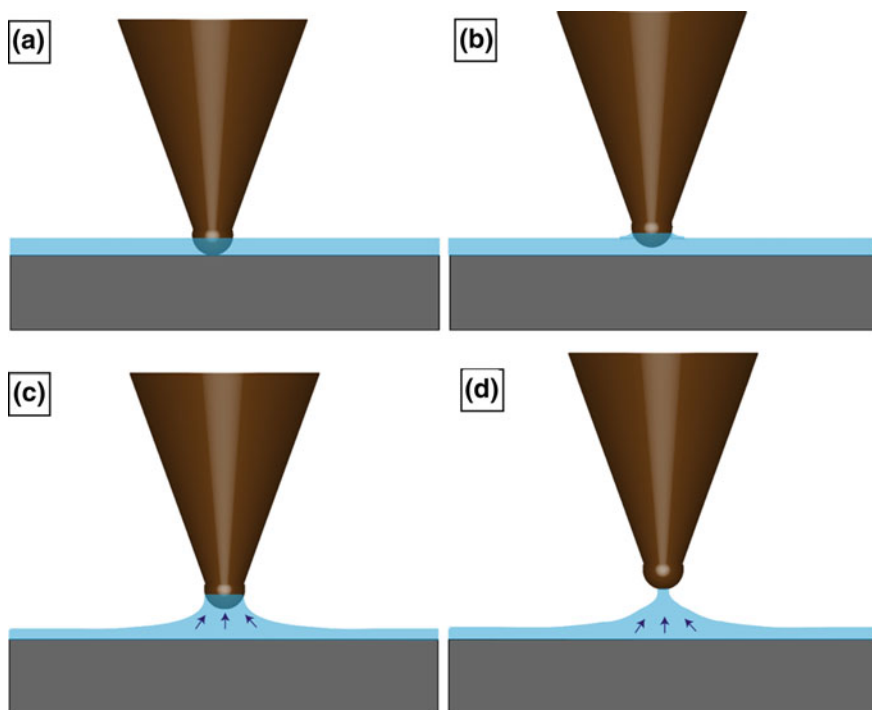
Fig. 3.4 Illustration depicting the various phases of tip interaction with the surface in the case of retraction (going away) from the sample. a Tip leaves the solid surface, b tip travels through the film of adsorbed water, c tip extends the neck of the meniscus formed by the water, d ultimately, the tip breaks free from the film of water
