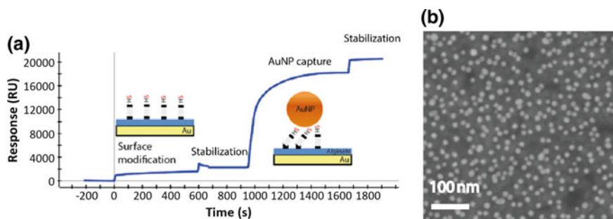
Fig. 5.1 a SPR sensorgram of surface modification using a hetero-bifunctional linker and subsequently, the immobilization of AuNPs. b SEM image of the sensor surface after AuNP injection
