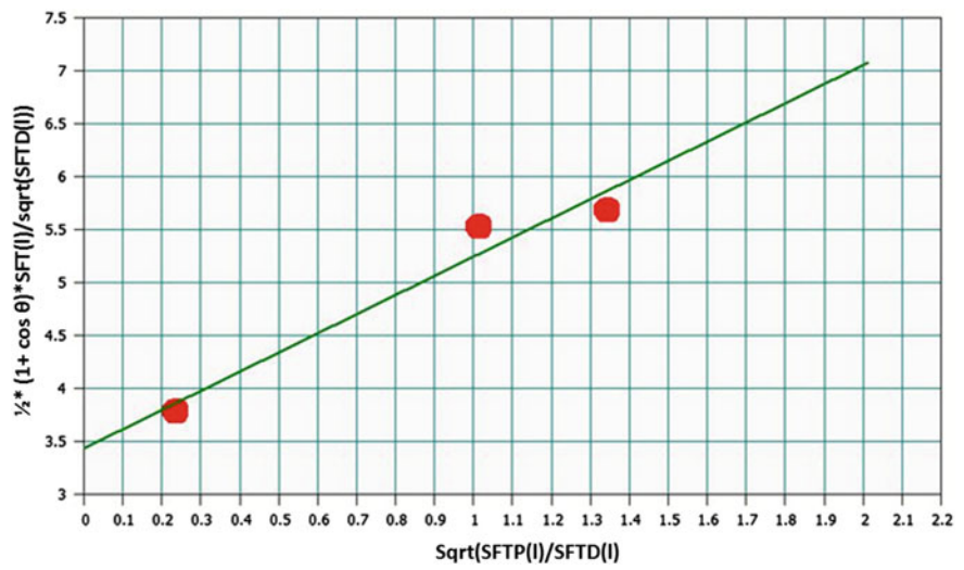
Fig. 2.4 Surface energy (polar and dispersive) calculation graph based on OWRK model for lubricated hard disk media
