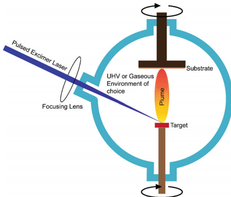
Fig. 2.1 A schematic layout of a simple PLD setup
