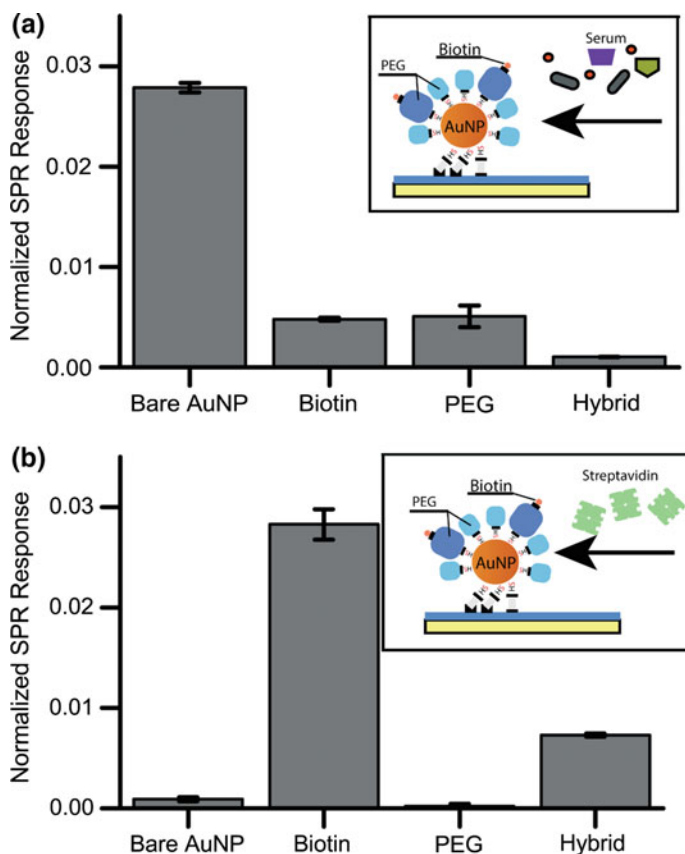
Fig. 5.6 a Normalized SPR response for interaction of 20% human serum with AuNPs modified with PEG5K-biotin (referred to as “Biotin”), PEG2K and 1:1 mixture of Biotin:PEG2K (referred to as “Hybrid”) compared to unmodified AuNPs. The inset illustrates the schematic of the experiment b Normalized SPR response showing the ability of AuNPs with previously described functionalizations to bind intended target streptavidin. The inset illustrates the schematic of the experiment ( p -value \ll 0.05 )
