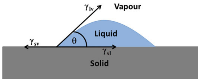
Fig. 2.3 Schematic diagram of a liquid drop on a solid surface showing the interfacial tensions at three phase boundary
