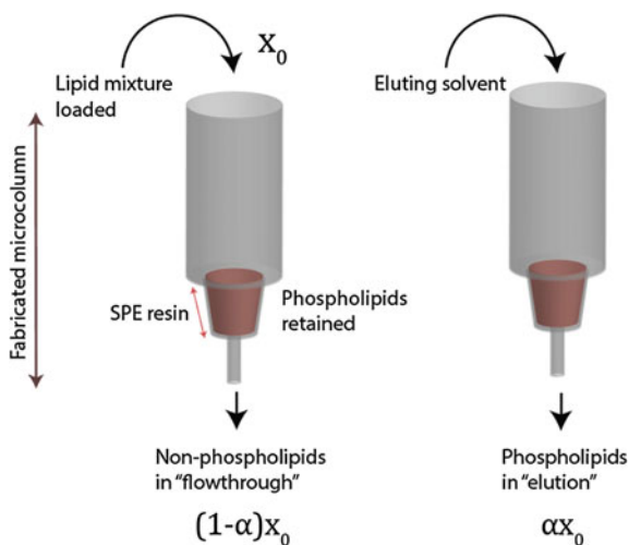
Fig. 4.7 Evaluation of \alpha used to compare between various metal oxides. x_0 is the number of molecules in the original mixture. \alpha x_0 denotes the number of molecules captured by the column. (1 - \alpha)x_0 molecules are not able to find capture sites on the SPE resin and are present in the flowthrough. D is obtained by dividing peak intensities of flowthrough and elution as obtained through ESI-MS. \alpha will be 1 for a perfect SPE and 0 for a material which has no affinity for phospholipids
