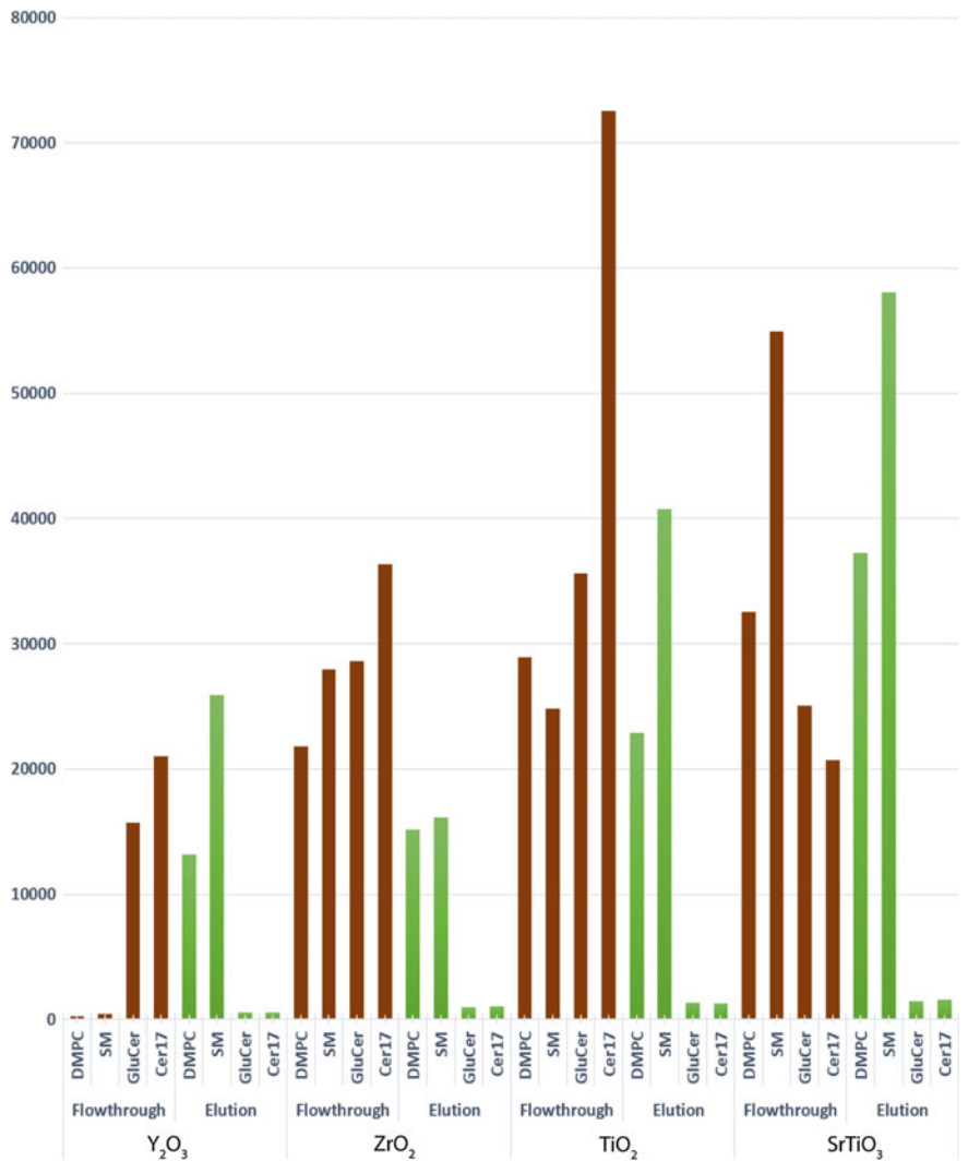
Fig. 4.6 Comparison between 4 oxides with respect to selective phospholipid enrichment. (Brown denotes flowthrough component, which should ideally have only GluCer and Cer 17; green denotes the elution component which should have only DMPC and SM. Y Axis is in arbitrary signal strength units
