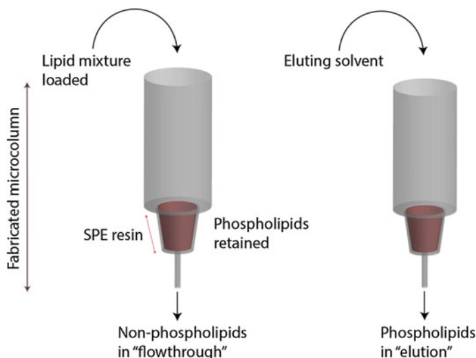
Fig. 4.2 A schematic illustration of the concept of SPE applied to lipidomics
