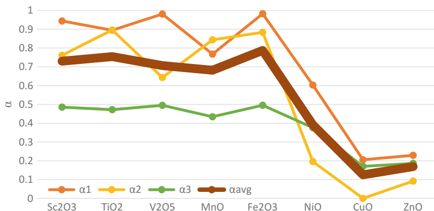
Fig. 4.8 \alpha as obtained for all stable 3d transition metal oxides
