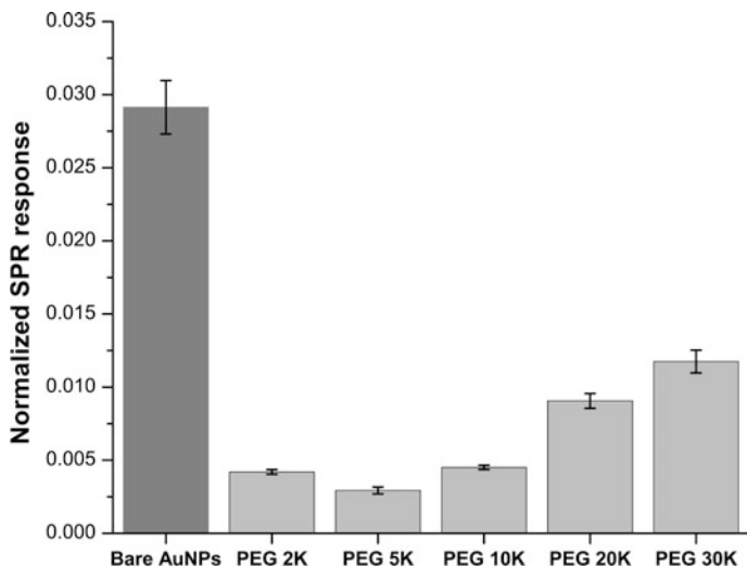
Fig. 5.5 Normalized SPR response for interaction of 20% (W/V) human serum (diluted with PBS buffer) with AuNPs modified with PEG2K, PEG5K, PEG10K, PEG20K and PEG30K compared to unmodified AuNPs. With the exception of PEG 2K and PEG 5K, all sets of data were statistically different from all other sets ( p -value \ll 0.05 )
