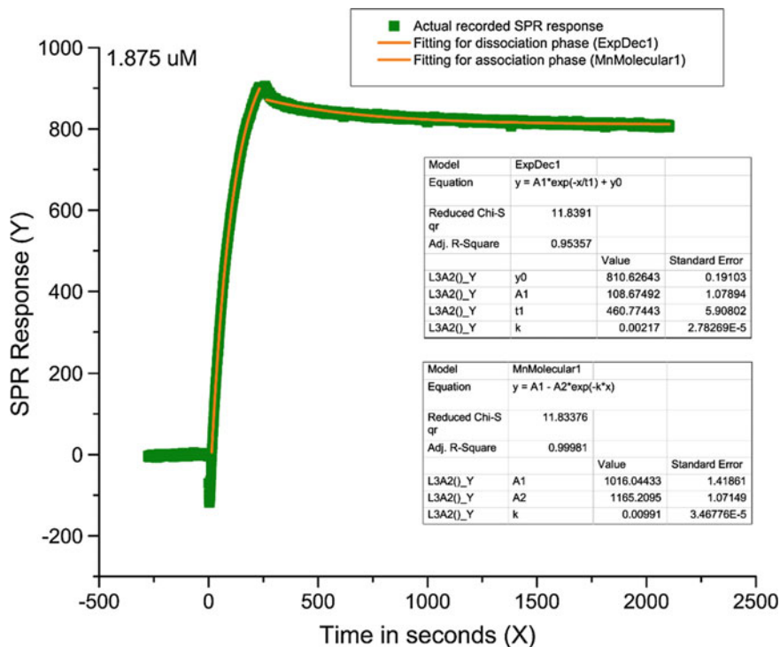
Fig. 5.7 Example of curve fitting on origin software package on experimentally collected data to obtain kinetic parameters
