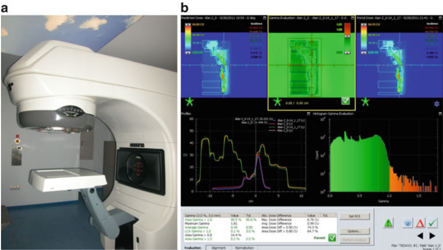
Fig. 20.5 a Electronic portal imaging device (EPID); b a sample of EPID dosimetry
